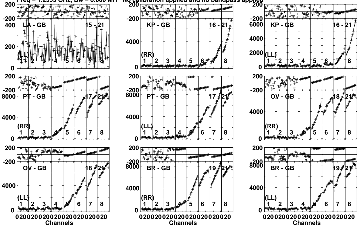
Lower frame: Micro Ampl Jy Top frame: Phas deg Vector averaged cross-power spectrum Several baselines displayed Timerange: 01/09:03:31 to 01/09:04:59
