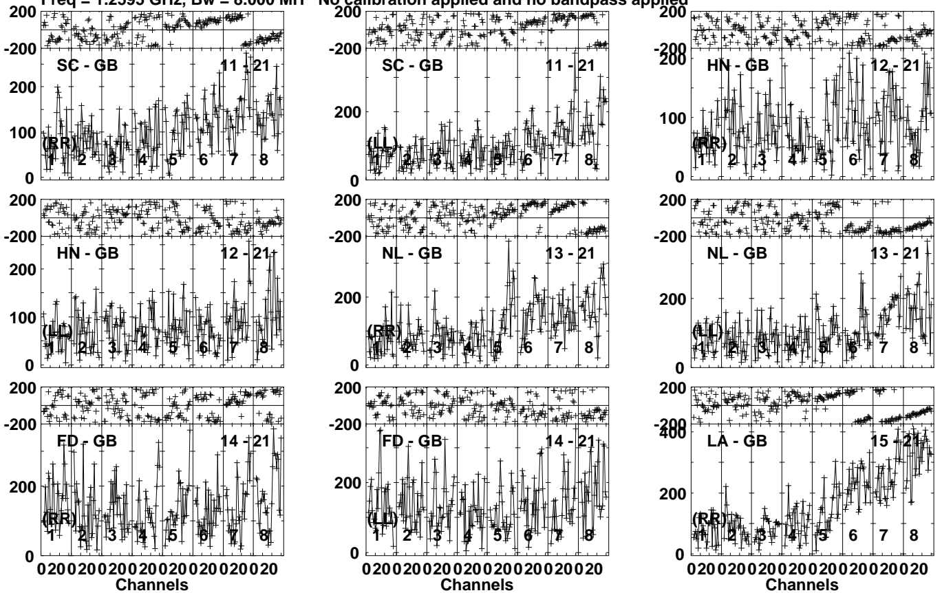
Lower frame: Micro Ampl Jy Top frame: Phas deg Vector averaged cross-power spectrum Several baselines displayed Timerange: 01/04:41:13 to 01/04:47:59
