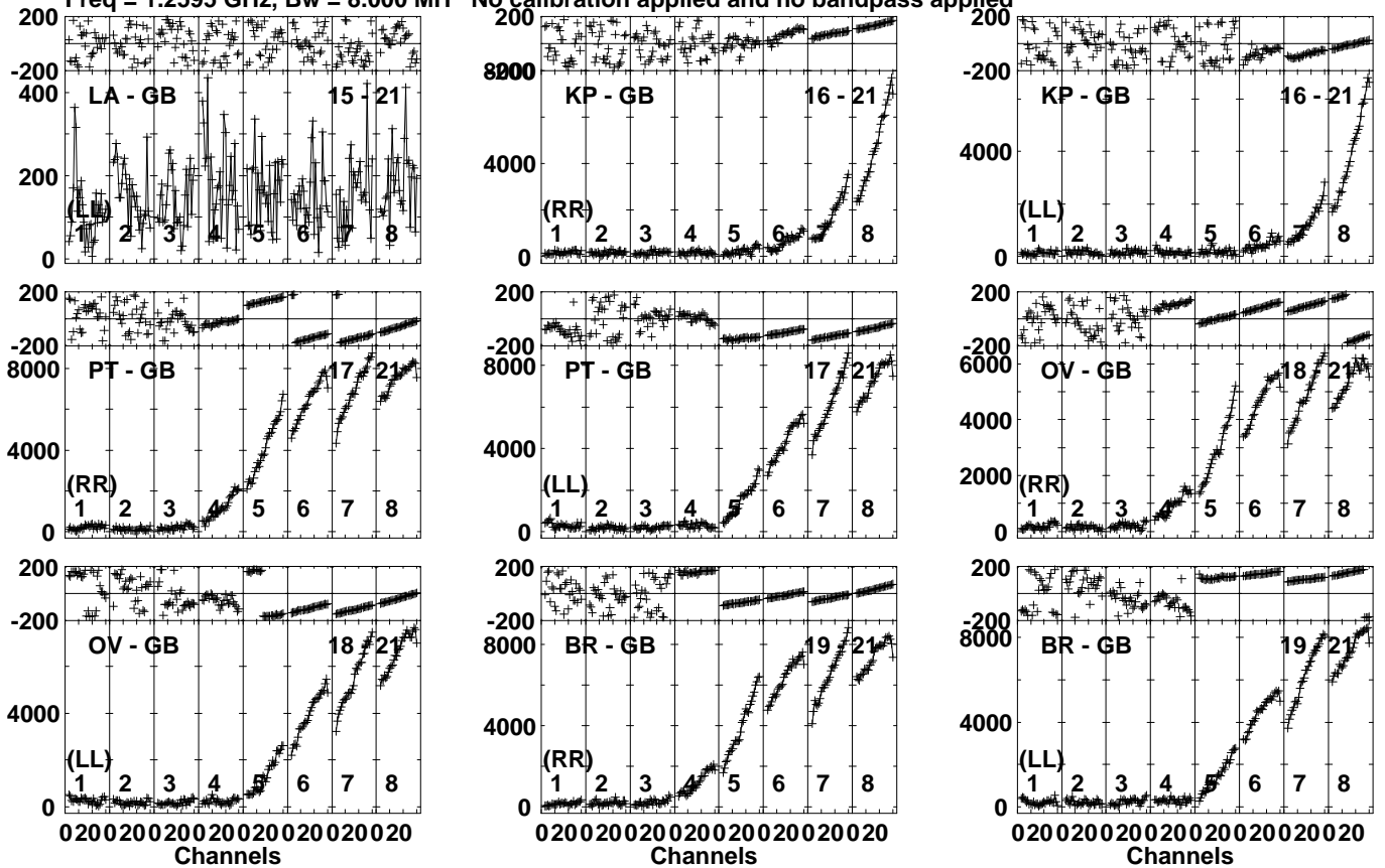
Lower frame: Micro Ampl Jy Top frame: Phas deg Vector averaged cross-power spectrum Several baselines displayed Timerange: 01/07:33:31 to 01/07:34:59
