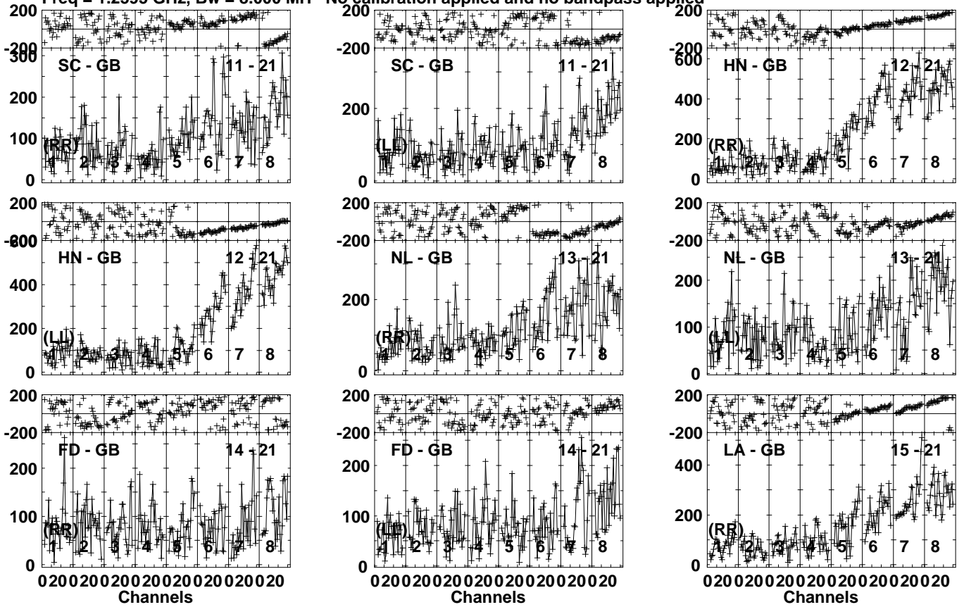
Lower frame: Micro Ampl Jy Top frame: Phas deg Vector averaged cross-power spectrum Several baselines displayed Timerange: 01/07:44:11 to 01/07:50:59
