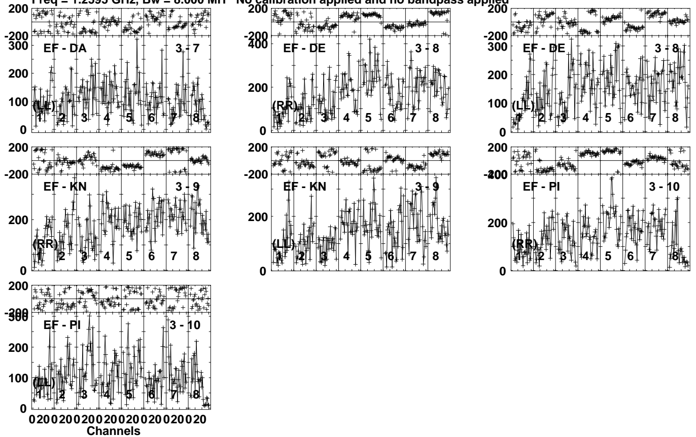
Lower frame: Micro Ampl Jy Top frame: Phas deg Vector averaged cross-power spectrum Several baselines displayed Timerange: 00/19:38:01 to 00/19:42:59
