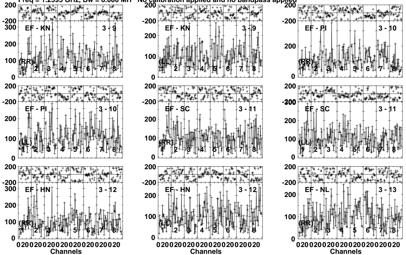
Lower frame: Micro Ampl Jy Top frame: Phas deg Vector averaged cross-power spectrum Several baselines displayed Timerange: 01/02:17:01 to 01/02:21:59
