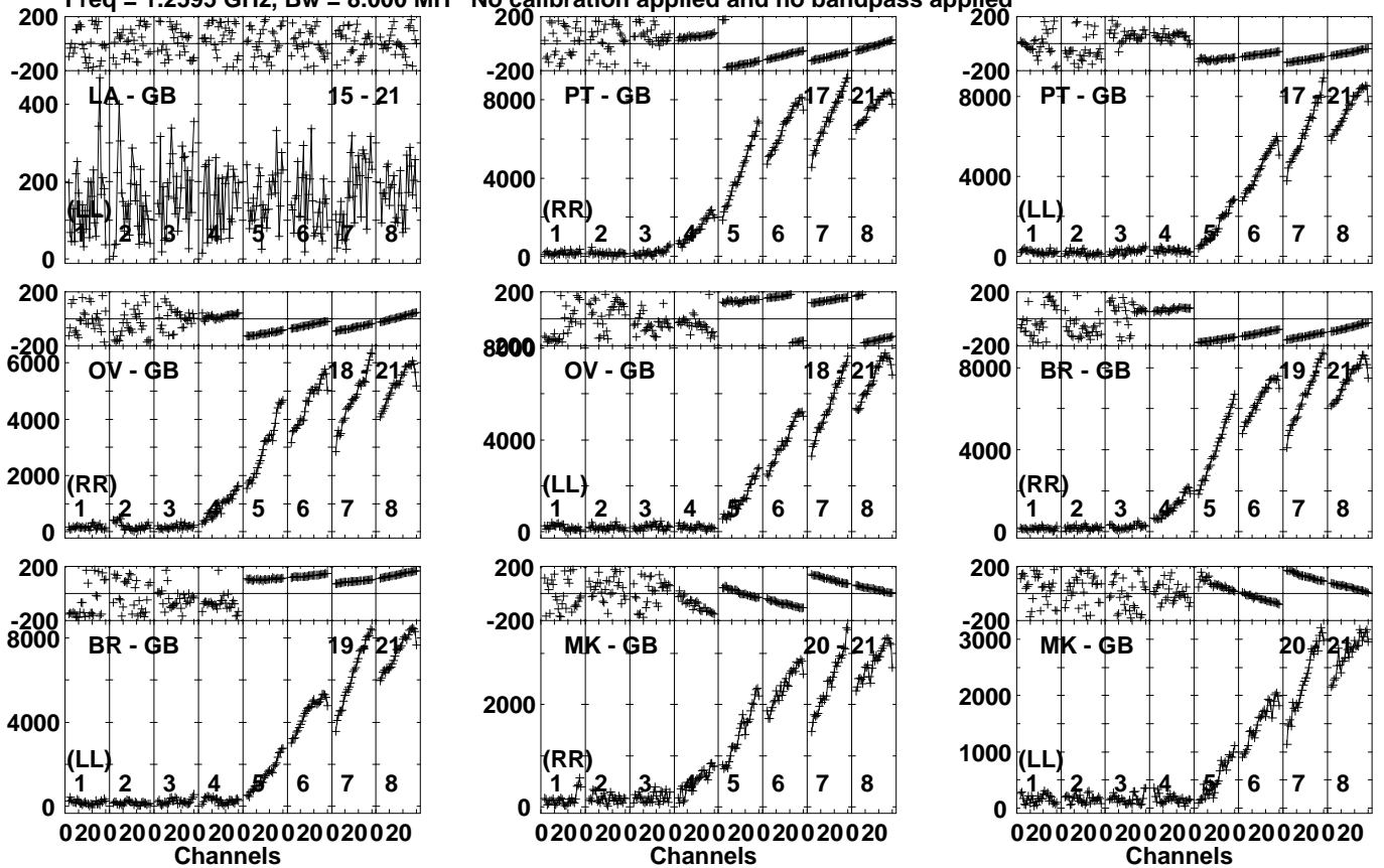
Lower frame: Micro Ampl Jy Top frame: Phas deg Vector averaged cross-power spectrum Several baselines displayed Timerange: 01/04:39:31 to 01/04:40:59
