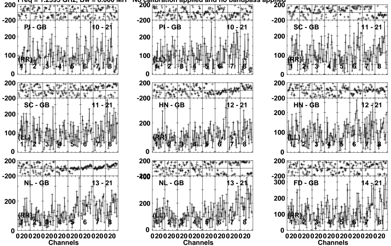
Lower frame: Micro Ampl Jy Top frame: Phas deg Vector averaged cross-power spectrum Several baselines displayed Timerange: 01/02:45:01 to 01/02:49:59
