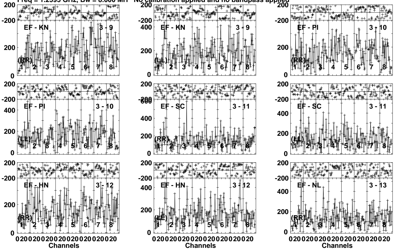
Lower frame: Micro Ampl Jy Top frame: Phas deg Vector averaged cross-power spectrum Several baselines displayed Timerange: 01/03:41:01 to 01/03:43:59
