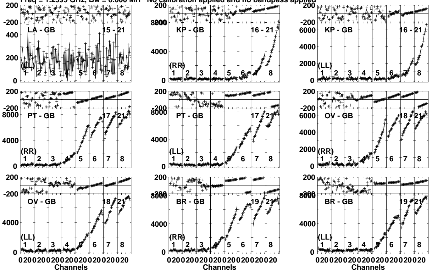
Lower frame: Micro Ampl Jy Top frame: Phas deg Vector averaged cross-power spectrum Several baselines displayed Timerange: 01/10:06:31 to 01/10:07:59
