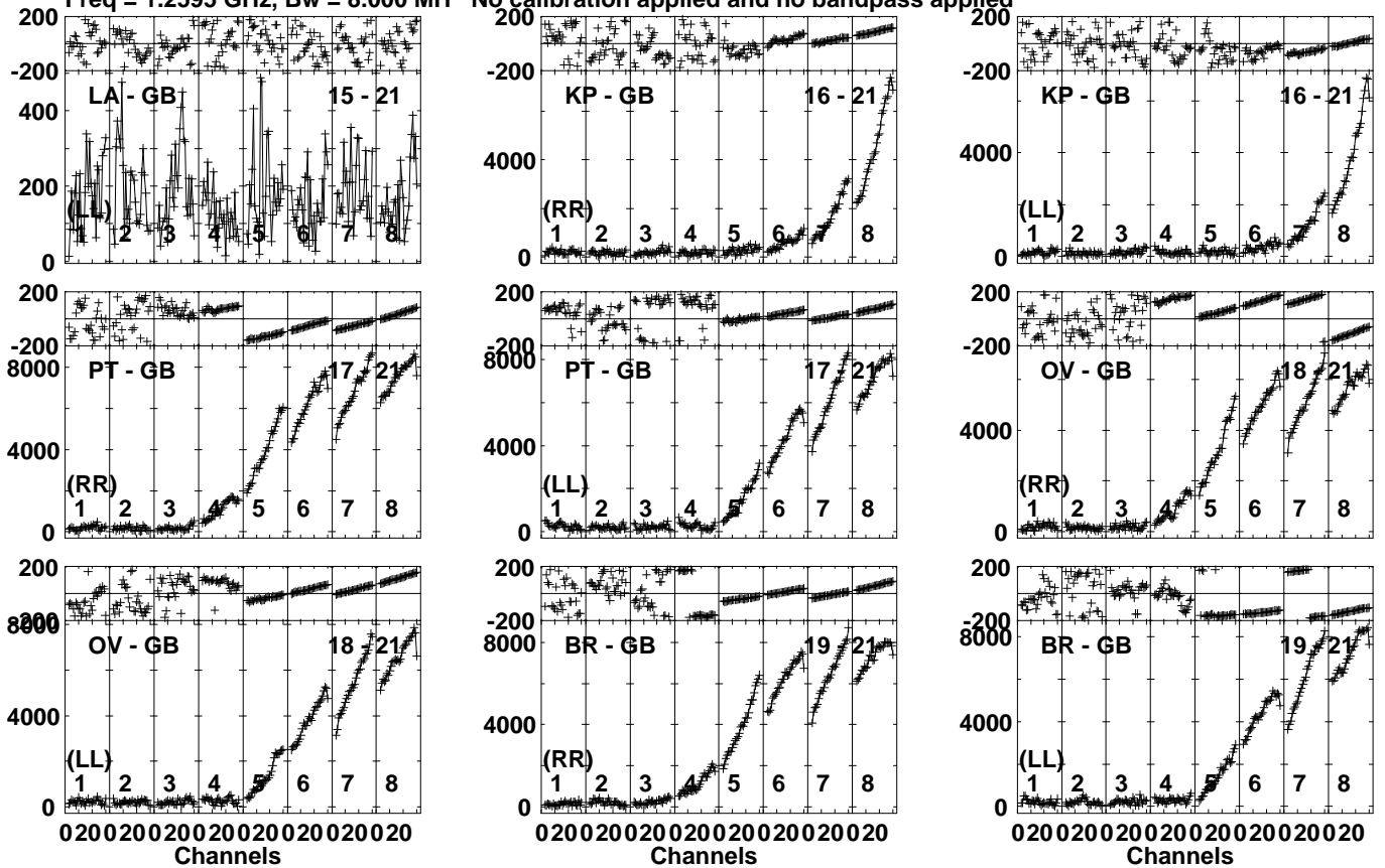
Lower frame: Micro Ampl Jy Top frame: Phas deg Vector averaged cross-power spectrum Several baselines displayed Timerange: 01/08:36:31 to 01/08:37:59
