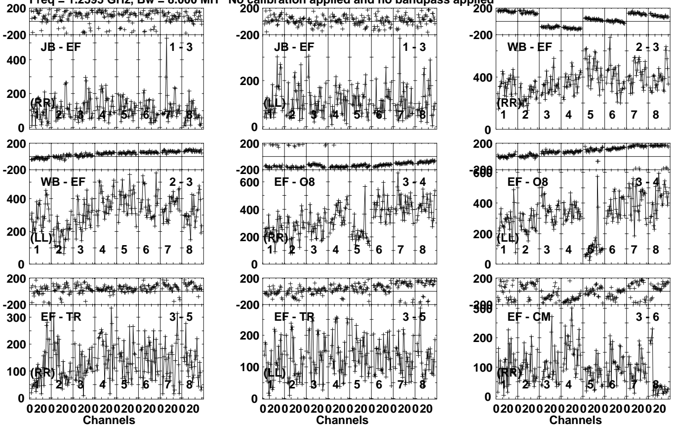
Lower frame: Micro Ampl Jy Top frame: Phas deg Vector averaged cross-power spectrum Several baselines displayed Timerange: 01/00:37:01 to 01/00:41:59
