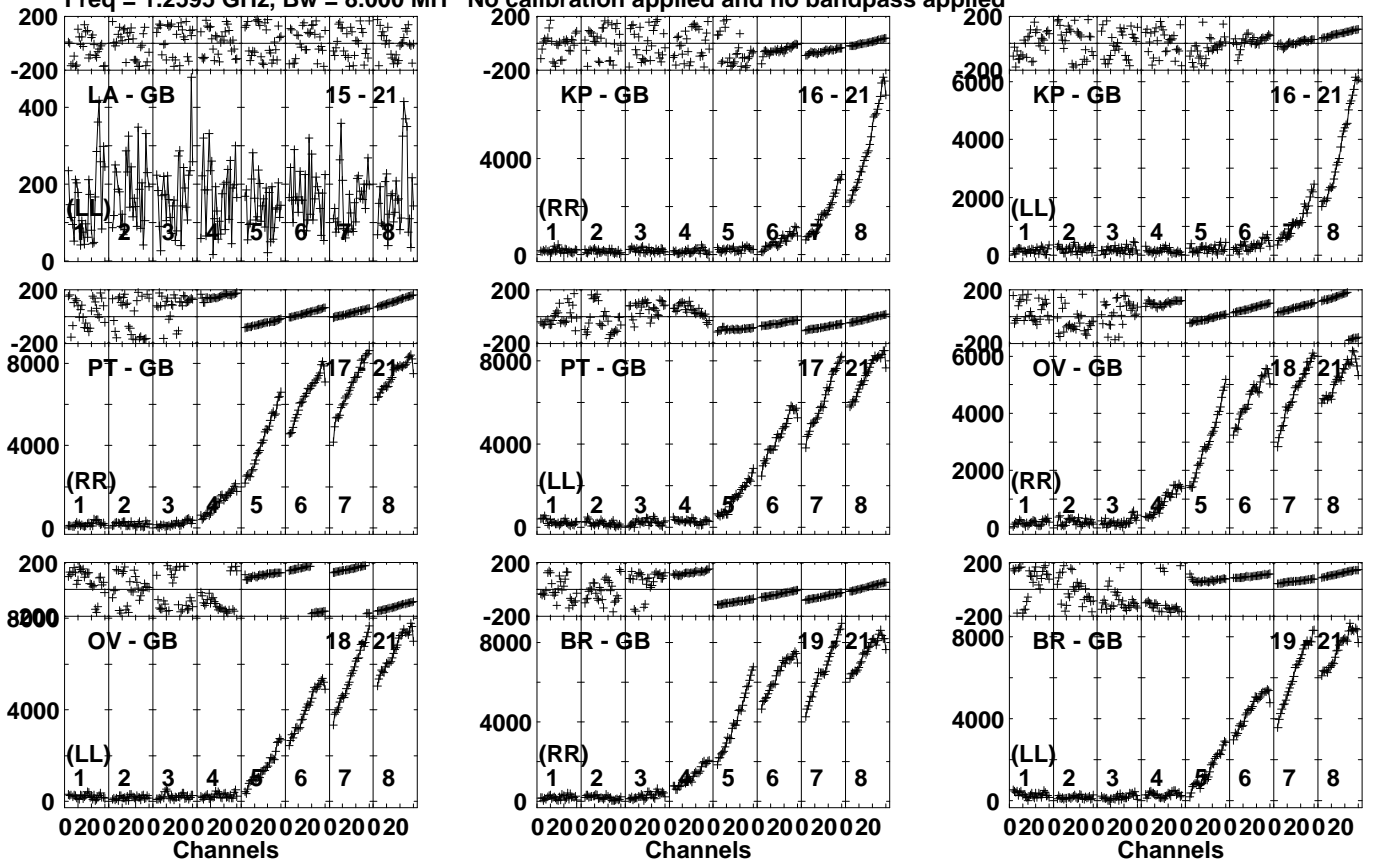
Lower frame: Micro Ampl Jy Top frame: Phas deg Vector averaged cross-power spectrum Several baselines displayed Timerange: 01/06:27:31 to 01/06:28:59
