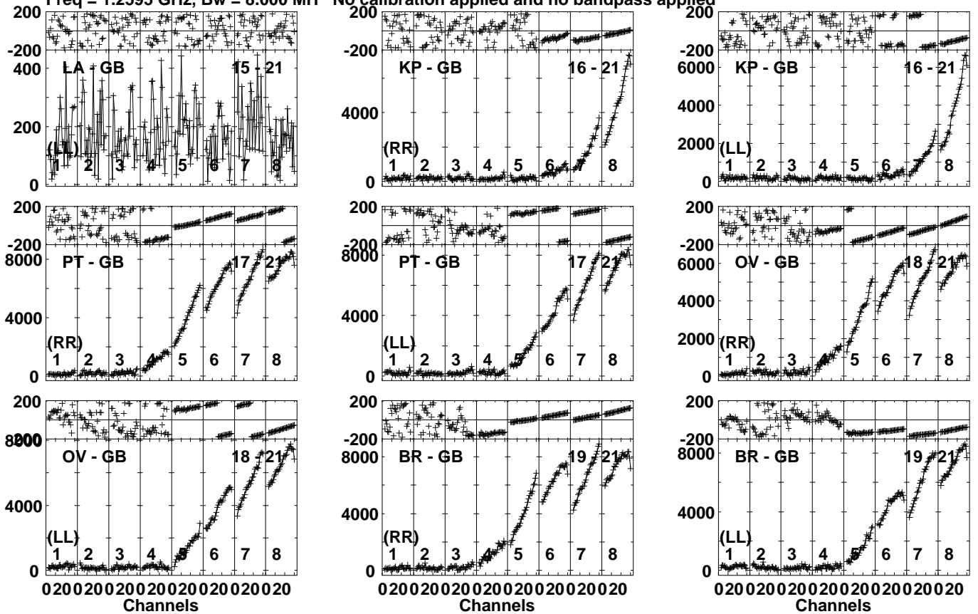
Lower frame: Micro Ampl Jy Top frame: Phas deg Vector averaged cross-power spectrum Several baselines displayed Timerange: 01/08:27:31 to 01/08:28:59
