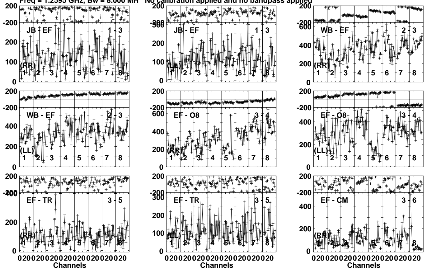
Lower frame: Micro Ampl Jy Top frame: Phas deg Vector averaged cross-power spectrum Several baselines displayed Timerange: 01/00:23:01 to 01/00:27:59
