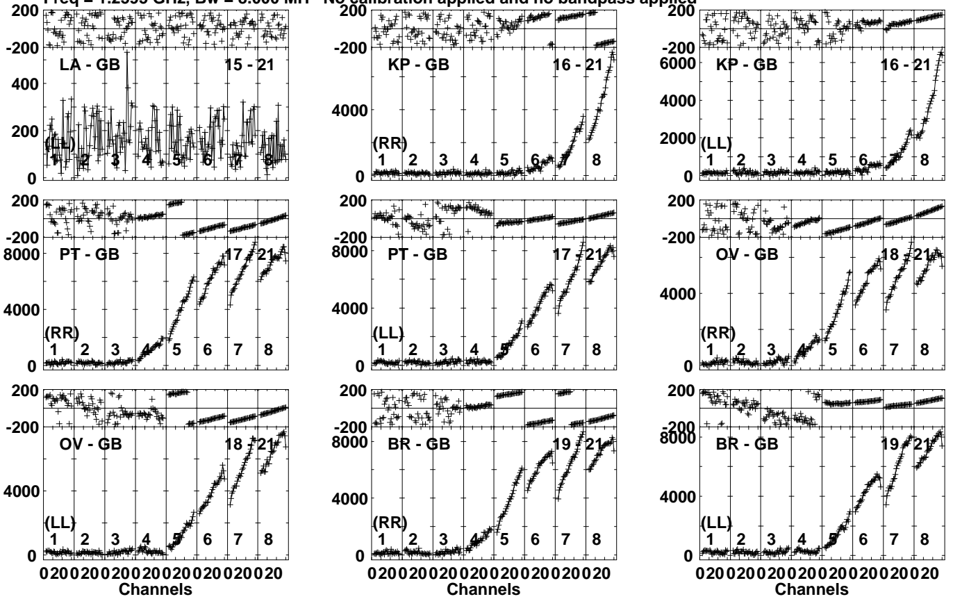
Lower frame: Micro Ampl Jy Top frame: Phas deg Vector averaged cross-power spectrum Several baselines displayed Timerange: 01/09:12:31 to 01/09:13:59
