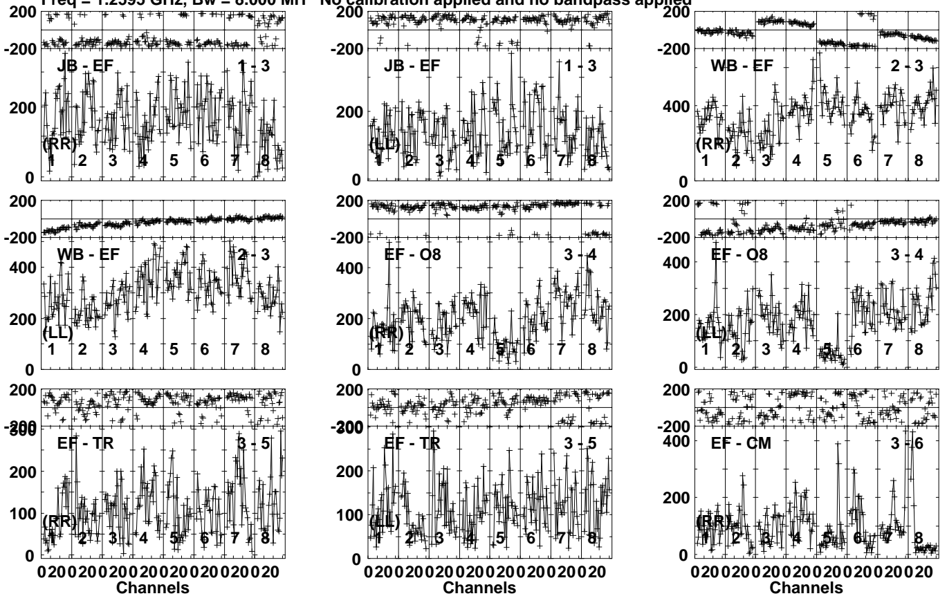
Lower frame: Micro Ampl Jy Top frame: Phas deg Vector averaged cross-power spectrum Several baselines displayed Timerange: 00/22:31:01 to 00/22:35:59
