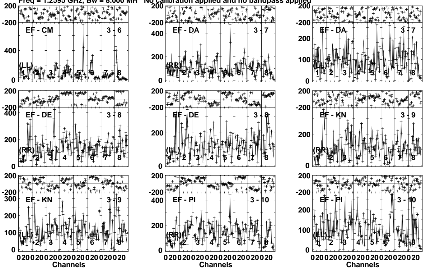
Lower frame: Micro Ampl Jy Top frame: Phas deg Vector averaged cross-power spectrum Several baselines displayed Timerange: 00/21:16:01 to 00/21:20:59
