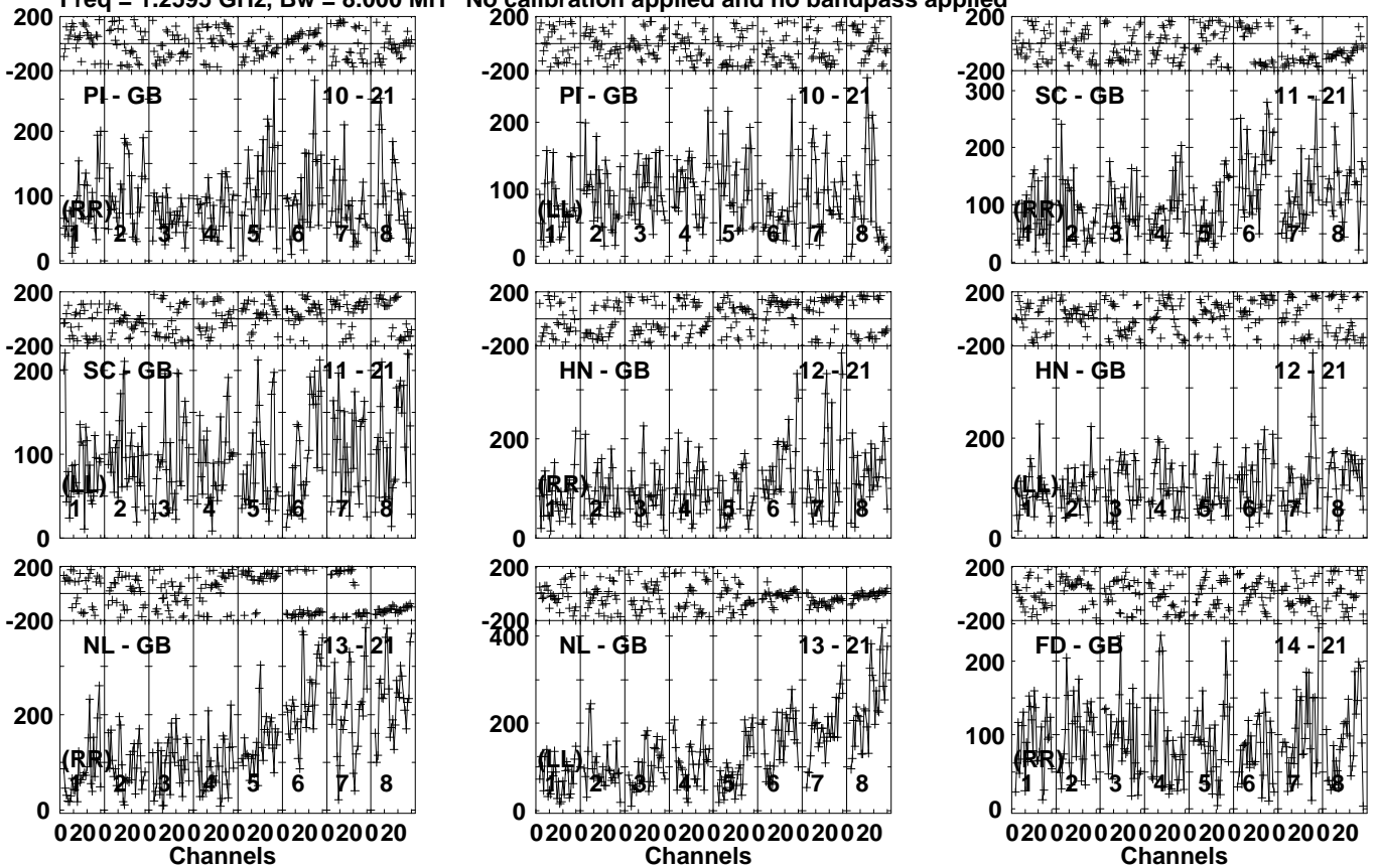
Lower frame: Micro Ampl Jy Top frame: Phas deg Vector averaged cross-power spectrum Several baselines displayed Timerange: 01/02:31:01 to 01/02:35:59
