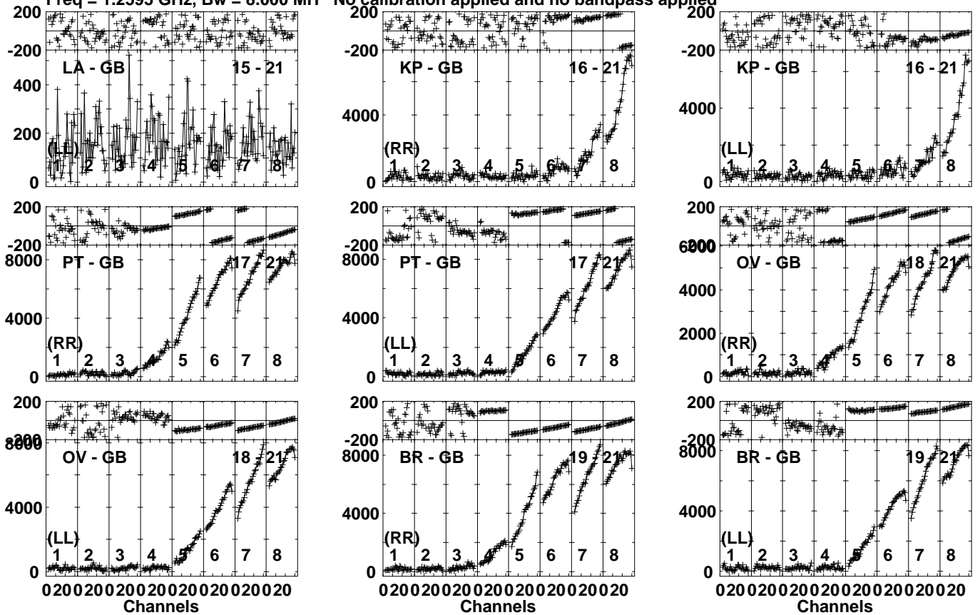
Lower frame: Micro Ampl Jy Top frame: Phas deg Vector averaged cross-power spectrum Several baselines displayed Timerange: 01/05:06:31 to 01/05:07:59
