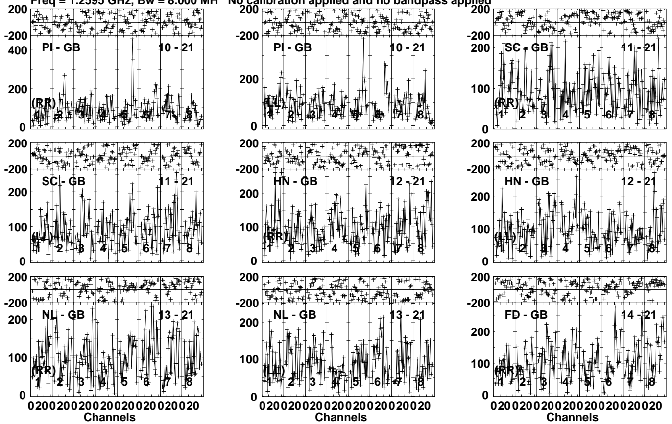
Lower frame: Micro Ampl Jy Top frame: Phas deg Vector averaged cross-power spectrum Several baselines displayed Timerange: 01/02:52:01 to 01/02:56:59
