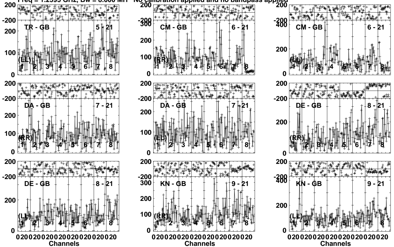
Lower frame: Micro Ampl Jy Top frame: Phas deg Vector averaged cross-power spectrum Several baselines displayed Timerange: 01/03:34:01 to 01/03:38:59
