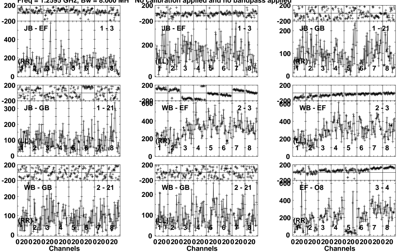
Lower frame: Micro Ampl Jy Top frame: Phas deg Vector averaged cross-power spectrum Several baselines displayed Timerange: 01/02:59:01 to 01/03:03:59
