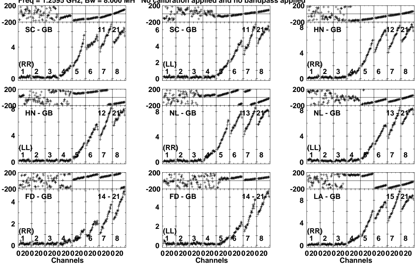
Lower frame: Milli Ampl Jy Top frame: Phas deg Vector averaged cross-power spectrum Several baselines displayed Timerange: 01/09:03:31 to 01/09:04:59
