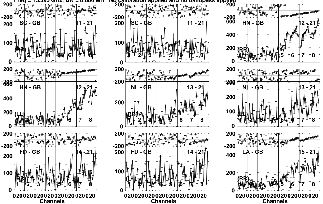
Lower frame: Micro Ampl Jy Top frame: Phas deg Vector averaged cross-power spectrum Several baselines displayed Timerange: 01/07:35:11 to 01/07:41:59
