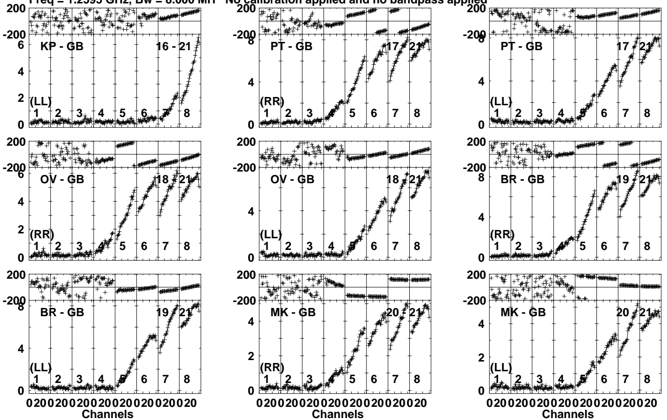
Lower frame: Milli Ampl Jy Top frame: Phas deg Vector averaged cross-power spectrum Several baselines displayed Timerange: 01/05:42:31 to 01/05:43:59
