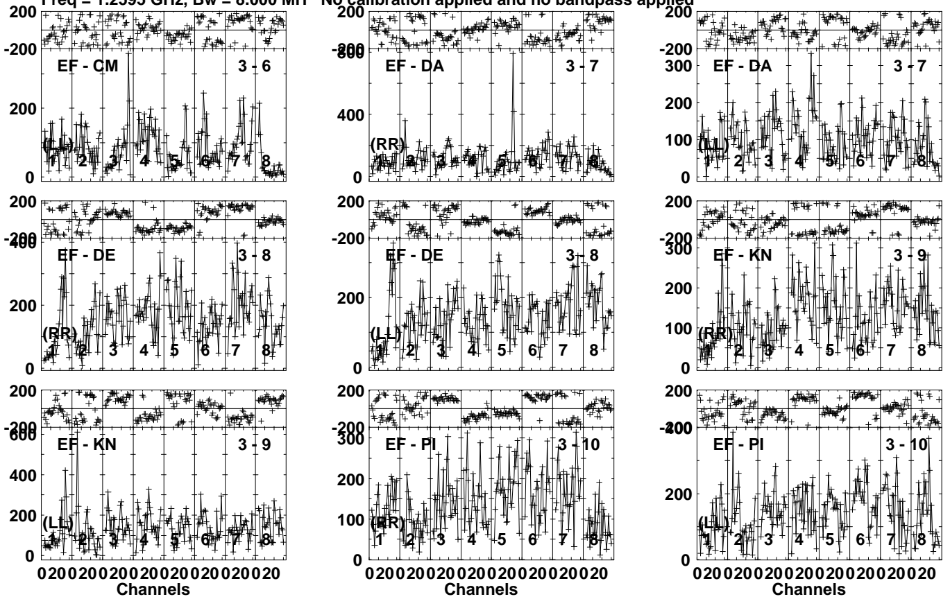
Lower frame: Micro Ampl Jy Top frame: Phas deg Vector averaged cross-power spectrum Several baselines displayed Timerange: 00/21:51:01 to 00/21:55:59
