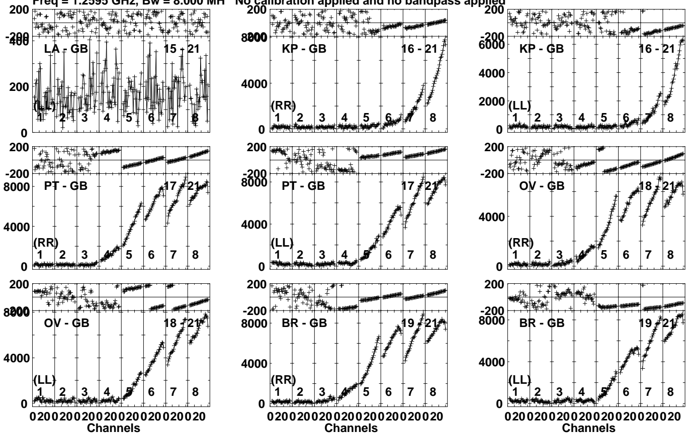
Lower frame: Micro Ampl Jy Top frame: Phas deg Vector averaged cross-power spectrum Several baselines displayed Timerange: 01/08:54:31 to 01/08:55:59
