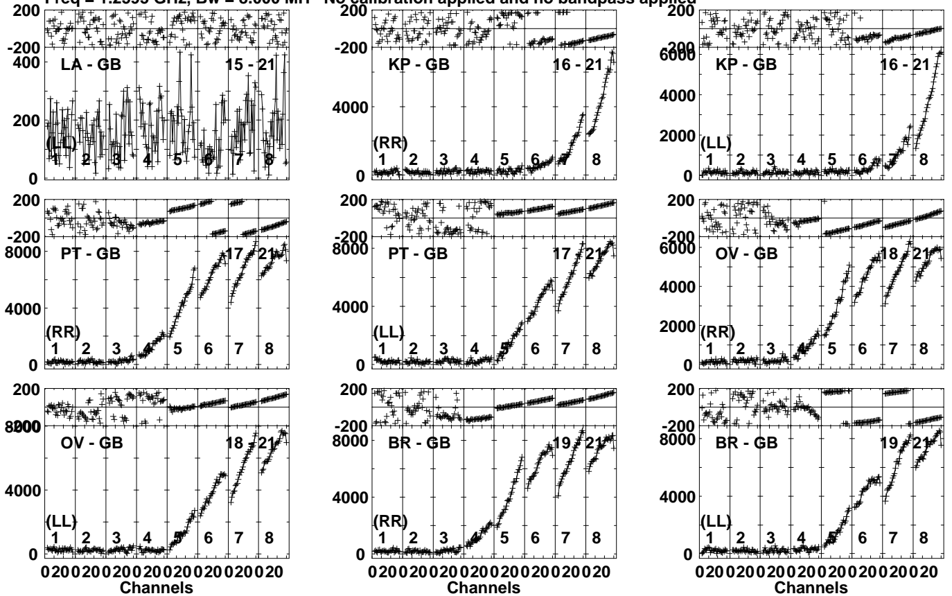
Lower frame: Micro Ampl Jy Top frame: Phas deg Vector averaged cross-power spectrum Several baselines displayed Timerange: 01/06:18:31 to 01/06:19:59
