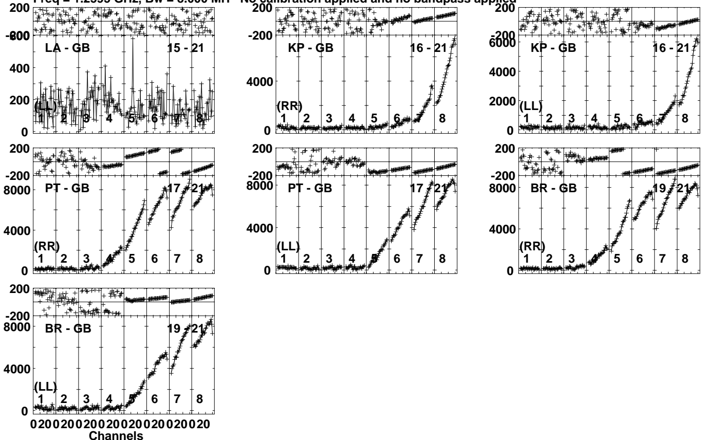
Lower frame: Micro Ampl Jy Top frame: Phas deg Vector averaged cross-power spectrum Several baselines displayed Timerange: 01/08:09:31 to 01/08:10:59
