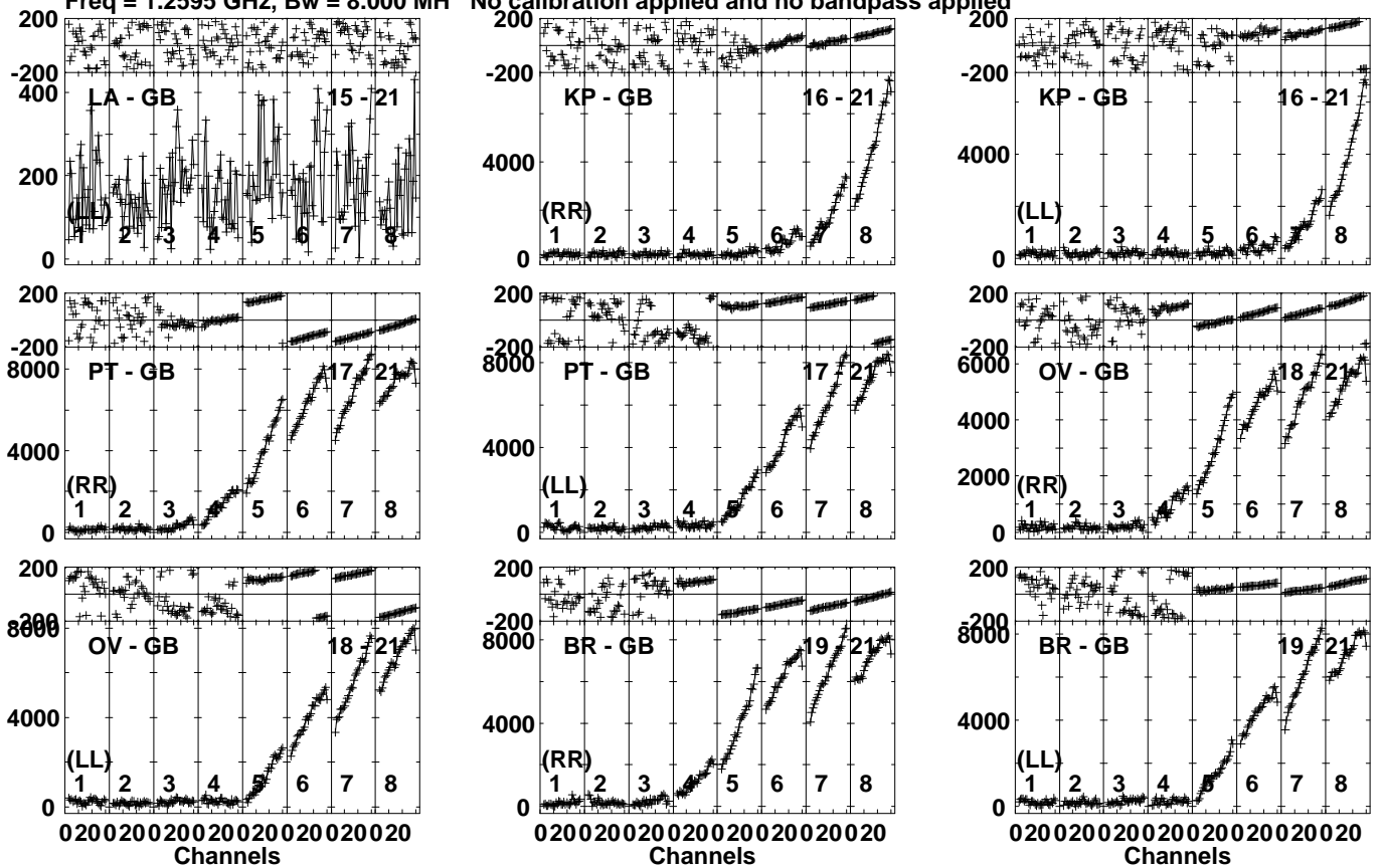
Lower frame: Micro Ampl Jy Top frame: Phas deg Vector averaged cross-power spectrum Several baselines displayed Timerange: 01/06:00:31 to 01/06:01:59
