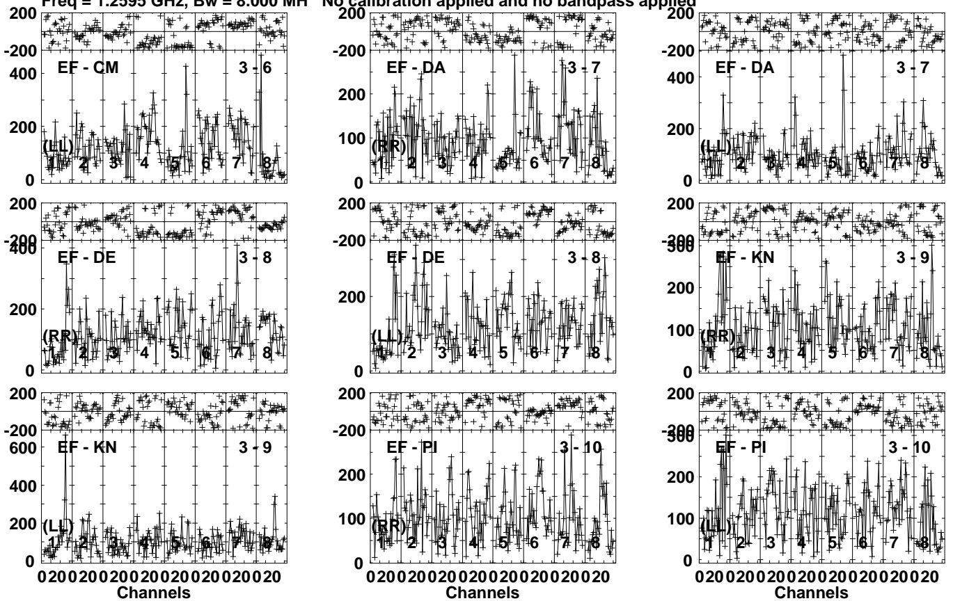
Lower frame: Micro Ampl Jy Top frame: Phas deg Vector averaged cross-power spectrum Several baselines displayed Timerange: 00/23:48:01 to 00/23:52:59
