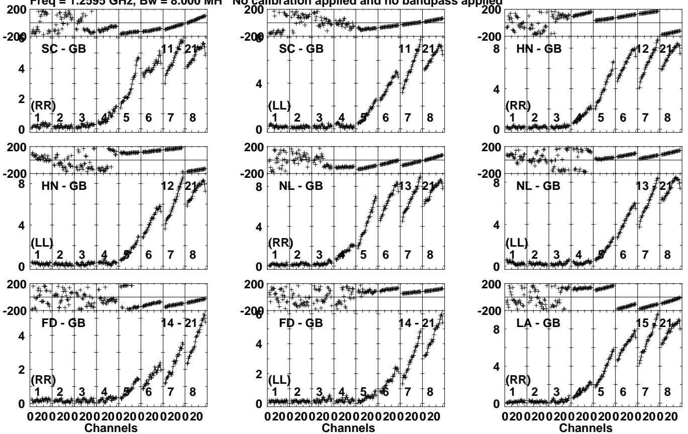
Lower frame: Milli Ampl Jy Top frame: Phas deg Vector averaged cross-power spectrum Several baselines displayed Timerange: 01/04:21:31 to 01/04:22:59
