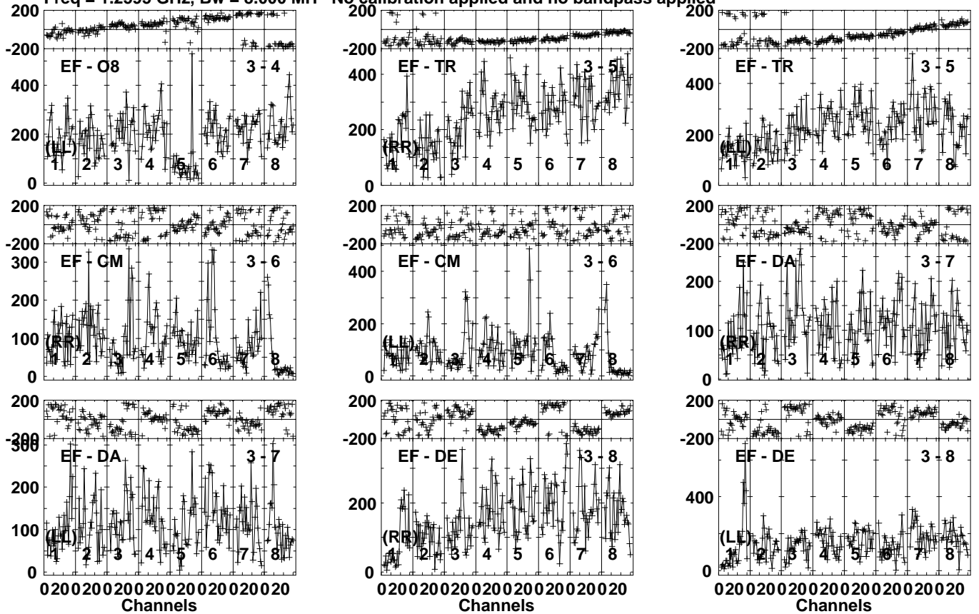
Lower frame: Micro Ampl Jy Top frame: Phas deg Vector averaged cross-power spectrum Several baselines displayed Timerange: 01/03:13:01 to 01/03:17:59
