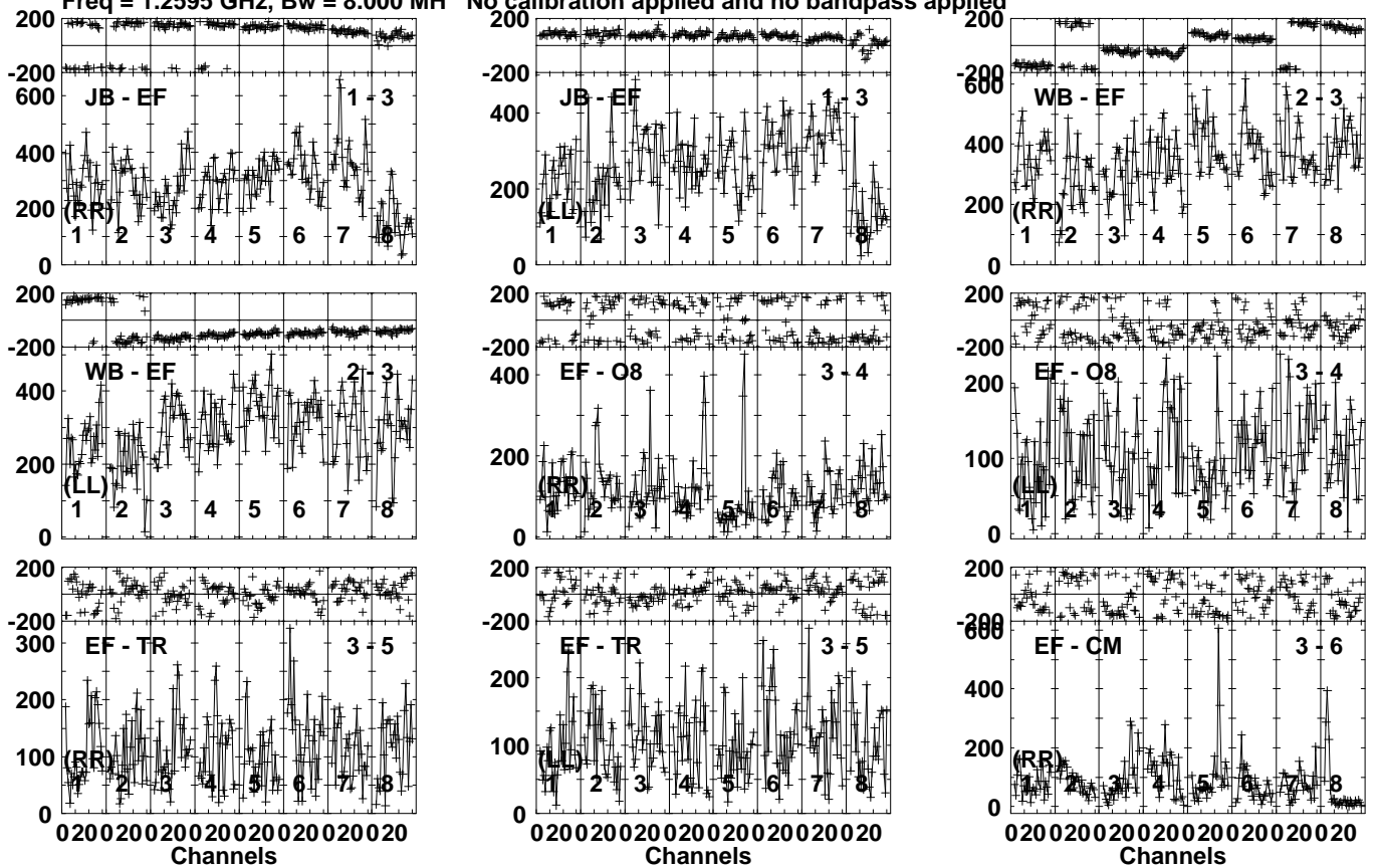
Lower frame: Micro Ampl Jy Top frame: Phas deg Vector averaged cross-power spectrum Several baselines displayed Timerange: 00/20:13:01 to 00/20:17:59
