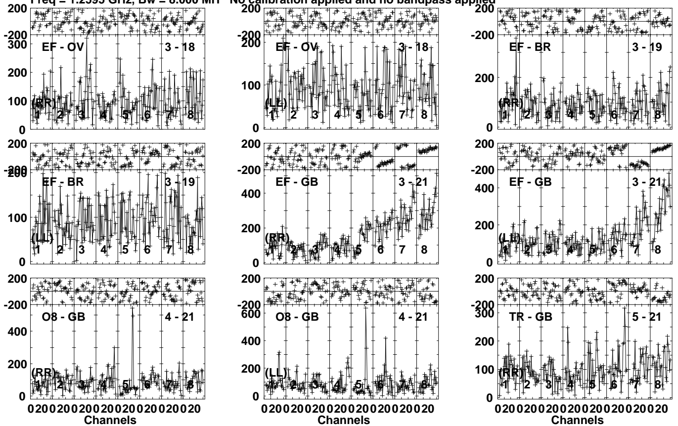
Lower frame: Micro Ampl Jy Top frame: Phas deg Vector averaged cross-power spectrum Several baselines displayed Timerange: 01/02:03:01 to 01/02:07:59
