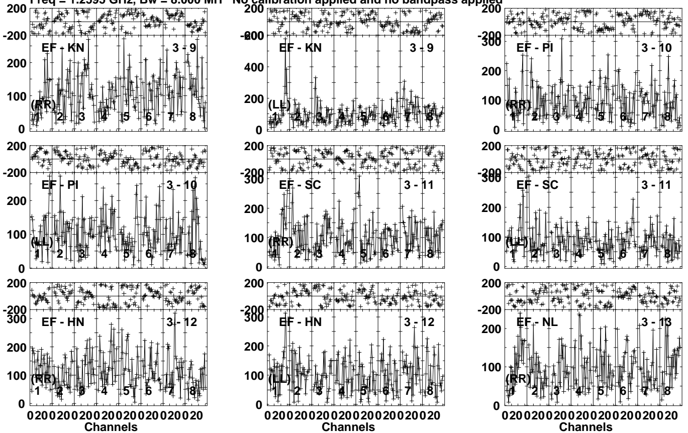
Lower frame: Micro Ampl Jy Top frame: Phas deg Vector averaged cross-power spectrum Several baselines displayed Timerange: 01/01:42:01 to 01/01:46:59
