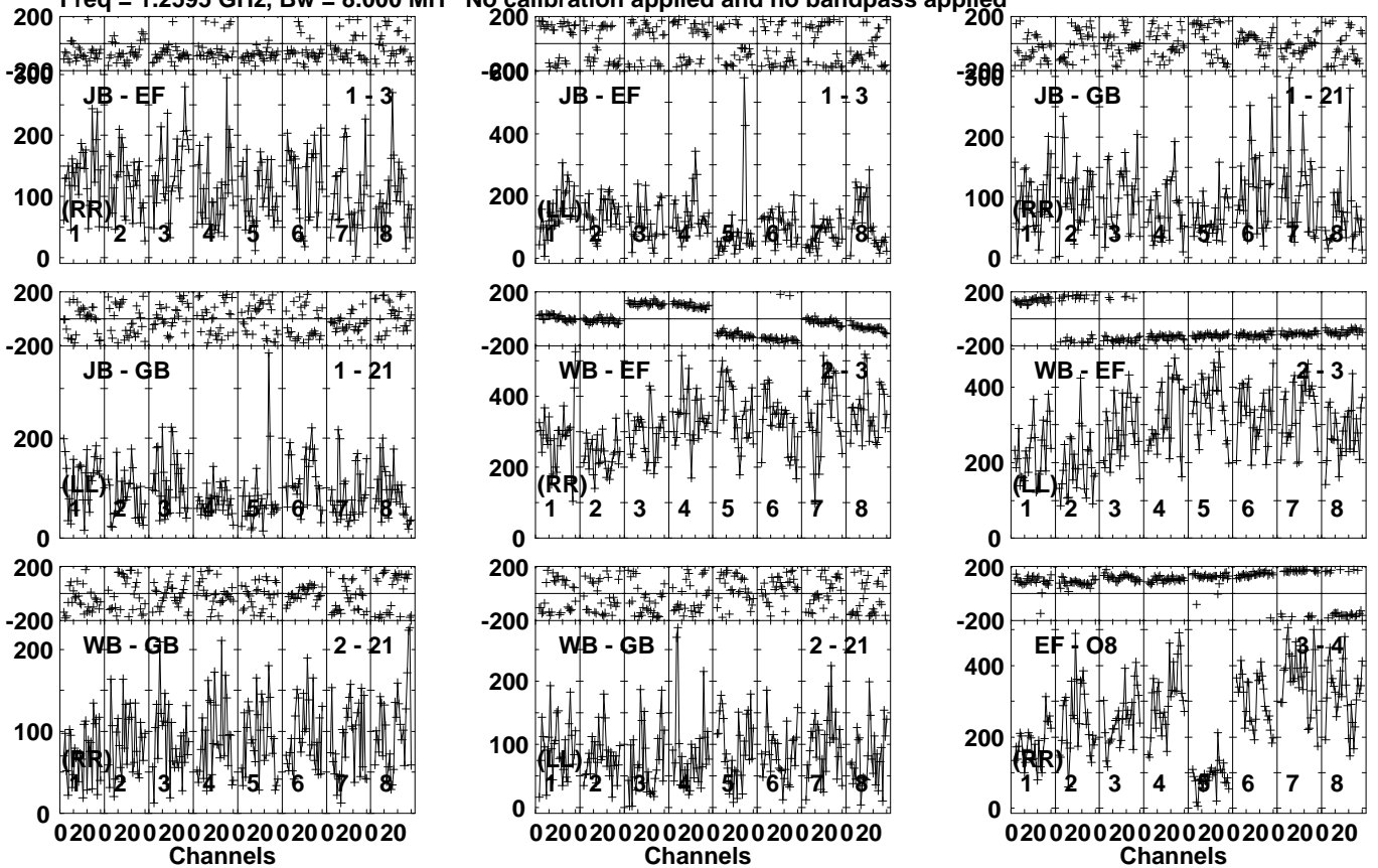
Lower frame: Micro Ampl Jy Top frame: Phas deg Vector averaged cross-power spectrum Several baselines displayed Timerange: 01/02:24:01 to 01/02:28:59
