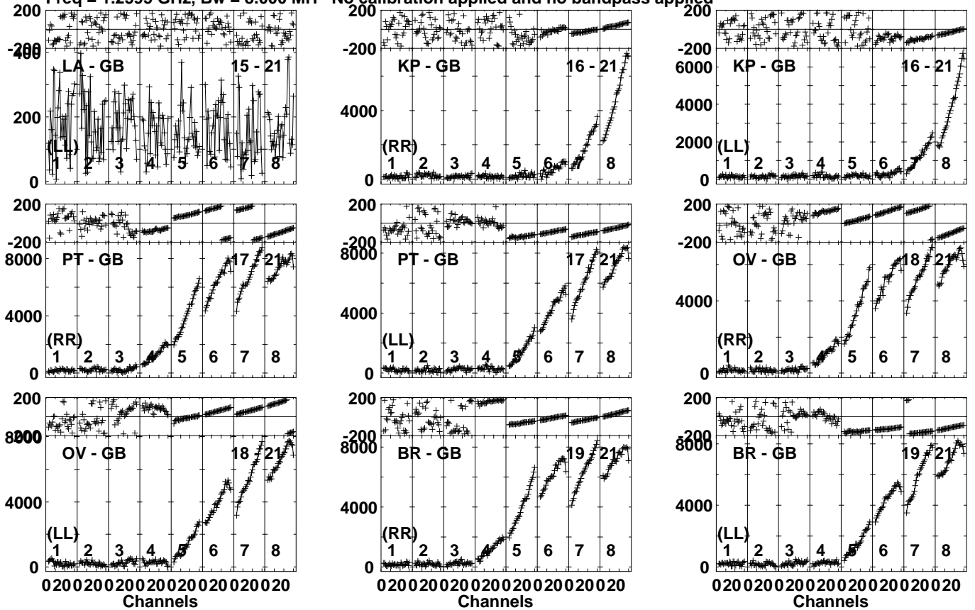
Lower frame: Micro Ampl Jy Top frame: Phas deg Vector averaged cross-power spectrum Several baselines displayed Timerange: 01/09:48:31 to 01/09:49:59
