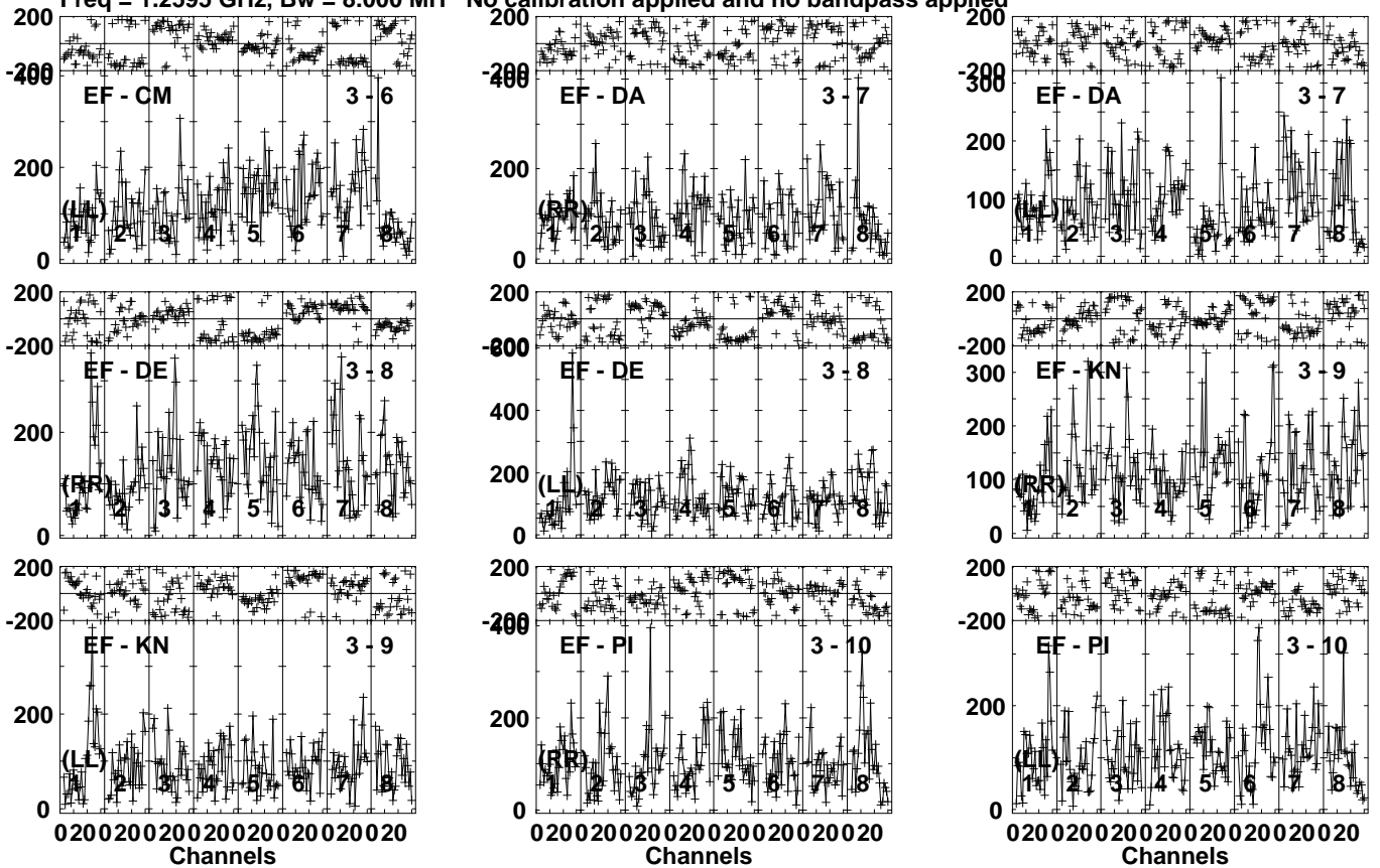
Lower frame: Micro Ampl Jy Top frame: Phas deg Vector averaged cross-power spectrum Several baselines displayed Timerange: 00/23:27:01 to 00/23:31:59
