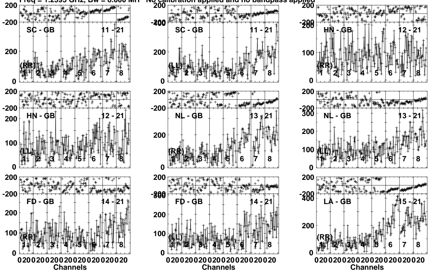
Lower frame: Micro Ampl Jy Top frame: Phas deg Vector averaged cross-power spectrum Several baselines displayed Timerange: 01/05:17:13 to 01/05:23:59
