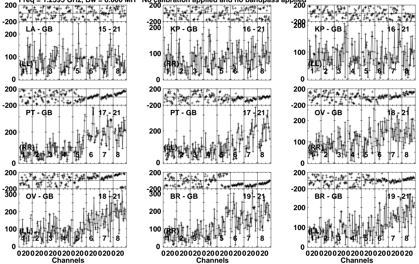
Lower frame: Micro Ampl Jy Top frame: Phas deg Vector averaged cross-power spectrum Several baselines displayed Timerange: 01/06:47:11 to 01/06:53:59
