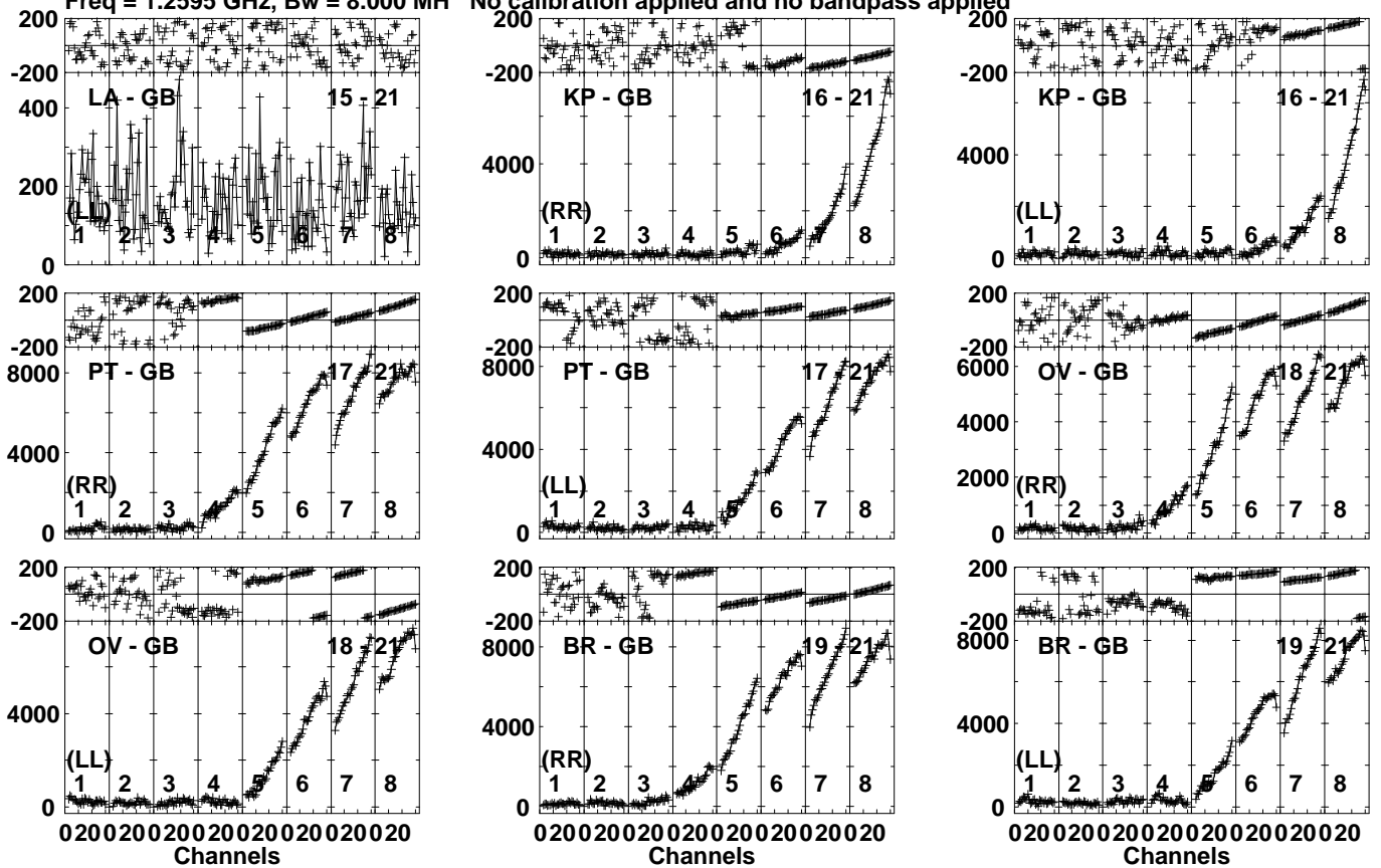
Lower frame: Micro Ampl Jy Top frame: Phas deg Vector averaged cross-power spectrum Several baselines displayed Timerange: 01/07:42:31 to 01/07:43:59
