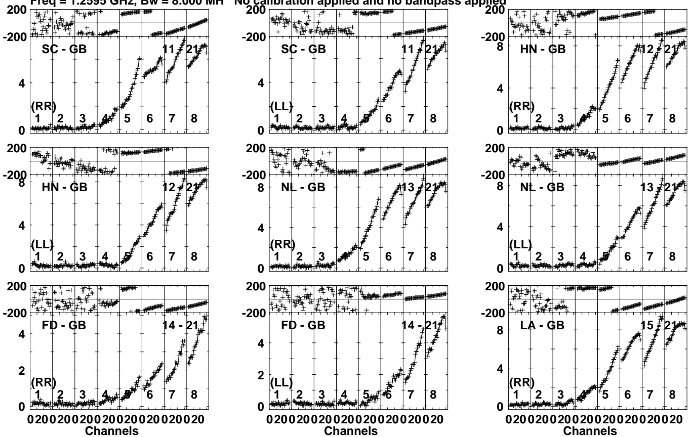
Lower frame: Milli Ampl Jy Top frame: Phas deg Vector averaged cross-power spectrum Several baselines displayed Timerange: 01/04:39:31 to 01/04:40:59
