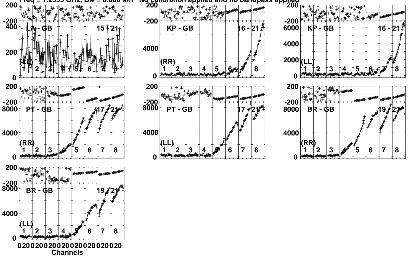
Lower frame: Micro Ampl Jy Top frame: Phas deg Vector averaged cross-power spectrum Several baselines displayed Timerange: 01/07:51:31 to 01/07:52:59
