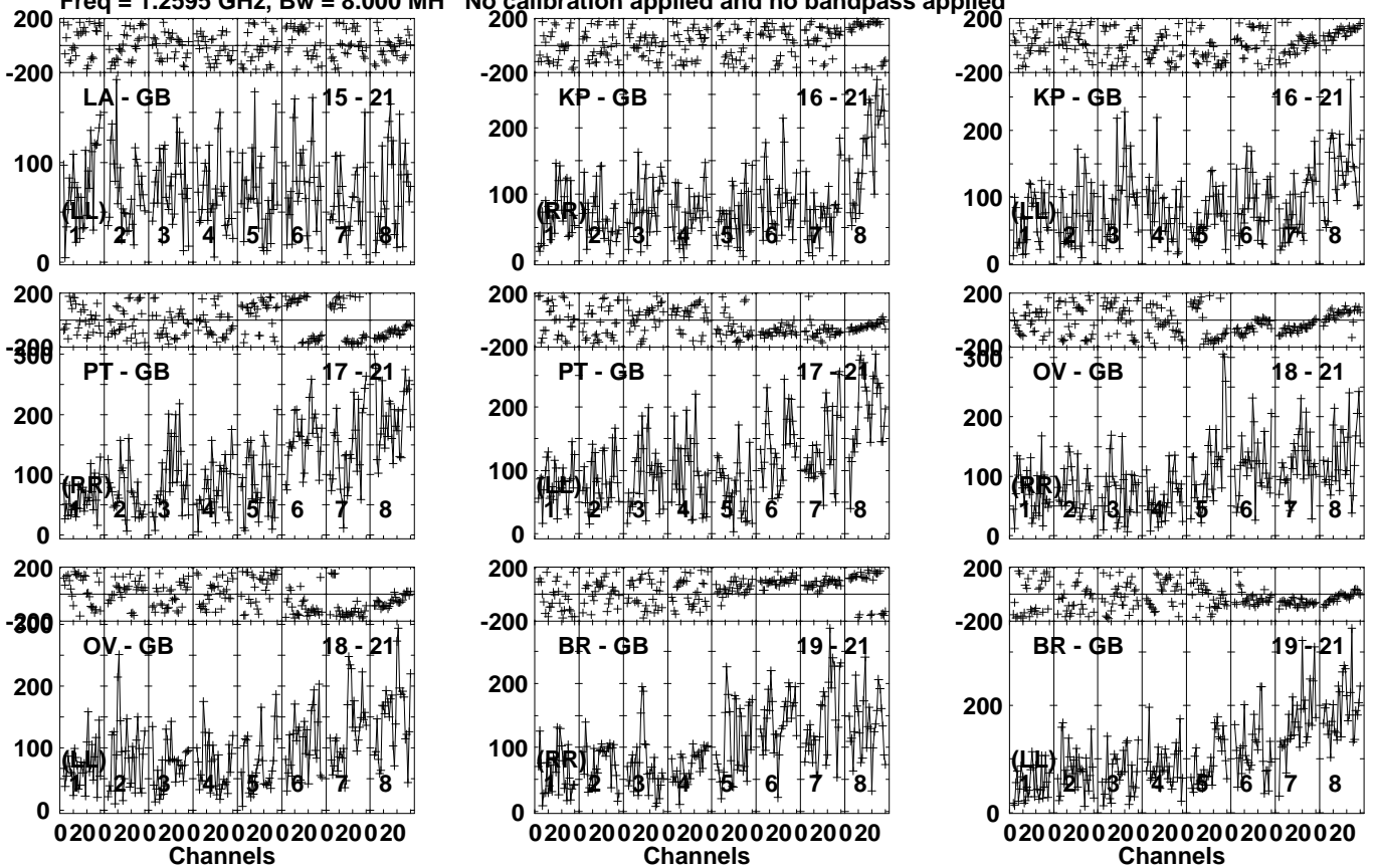
Lower frame: Micro Ampl Jy Top frame: Phas deg Vector averaged cross-power spectrum Several baselines displayed Timerange: 01/08:56:11 to 01/09:02:59
