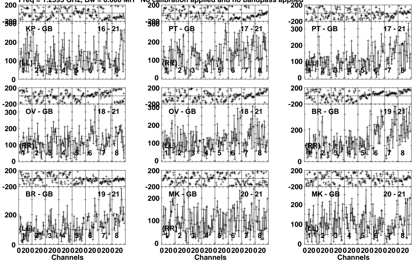
Lower frame: Micro Ampl Jy Top frame: Phas deg Vector averaged cross-power spectrum Several baselines displayed Timerange: 01/10:17:11 to 01/10:21:29
