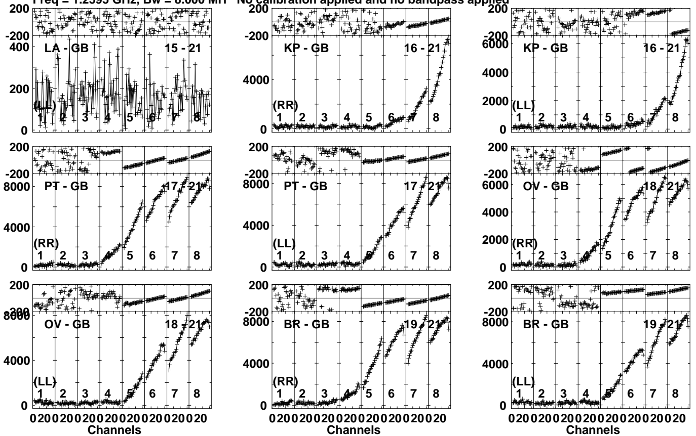
Lower frame: Micro Ampl Jy Top frame: Phas deg Vector averaged cross-power spectrum Several baselines displayed Timerange: 01/07:24:31 to 01/07:25:59
