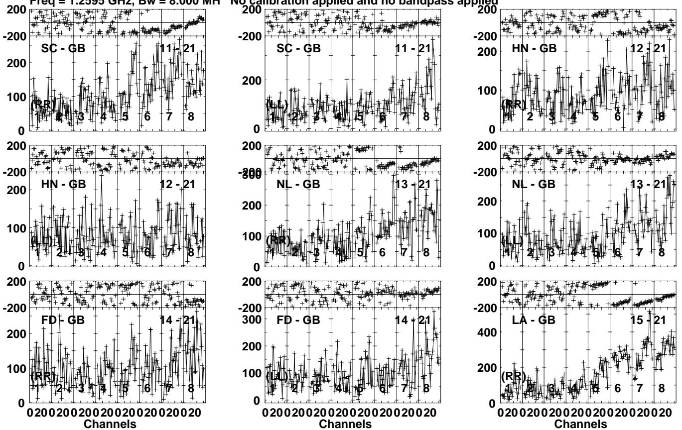
Lower frame: Micro Ampl Jy Top frame: Phas deg Vector averaged cross-power spectrum Several baselines displayed Timerange: 01/04:23:13 to 01/04:29:59
