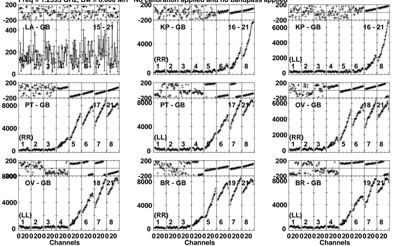
Lower frame: Micro Ampl Jy Top frame: Phas deg Vector averaged cross-power spectrum Several baselines displayed Timerange: 01/06:09:31 to 01/06:10:59
