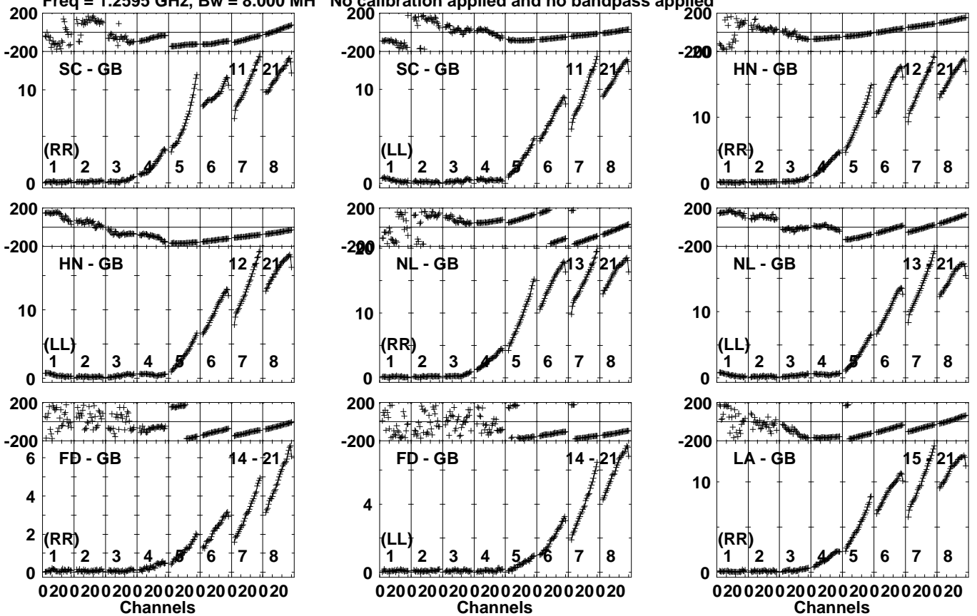
Lower frame: Milli Ampl Jy Top frame: Phas deg Vector averaged cross-power spectrum Several baselines displayed Timerange: 01/10:25:01 to 01/10:29:59
