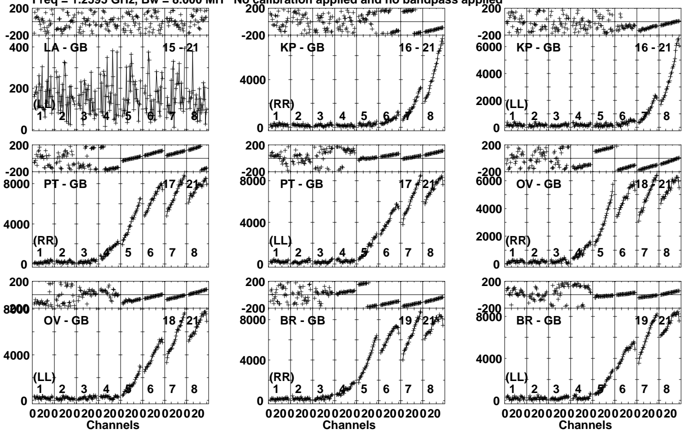
Lower frame: Micro Ampl Jy Top frame: Phas deg Vector averaged cross-power spectrum Several baselines displayed Timerange: 01/06:54:31 to 01/06:55:59
