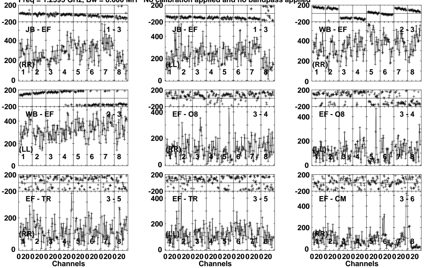
Lower frame: Micro Ampl Jy Top frame: Phas deg Vector averaged cross-power spectrum Several baselines displayed Timerange: 00/20:41:01 to 00/20:45:59
