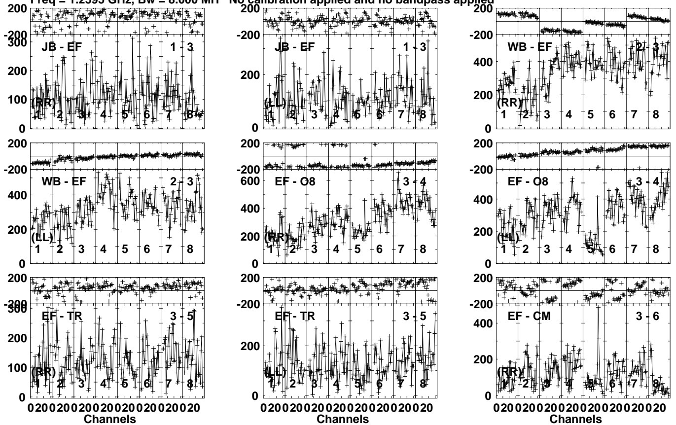
Lower frame: Micro Ampl Jy Top frame: Phas deg Vector averaged cross-power spectrum Several baselines displayed Timerange: 01/00:44:01 to 01/00:48:59
