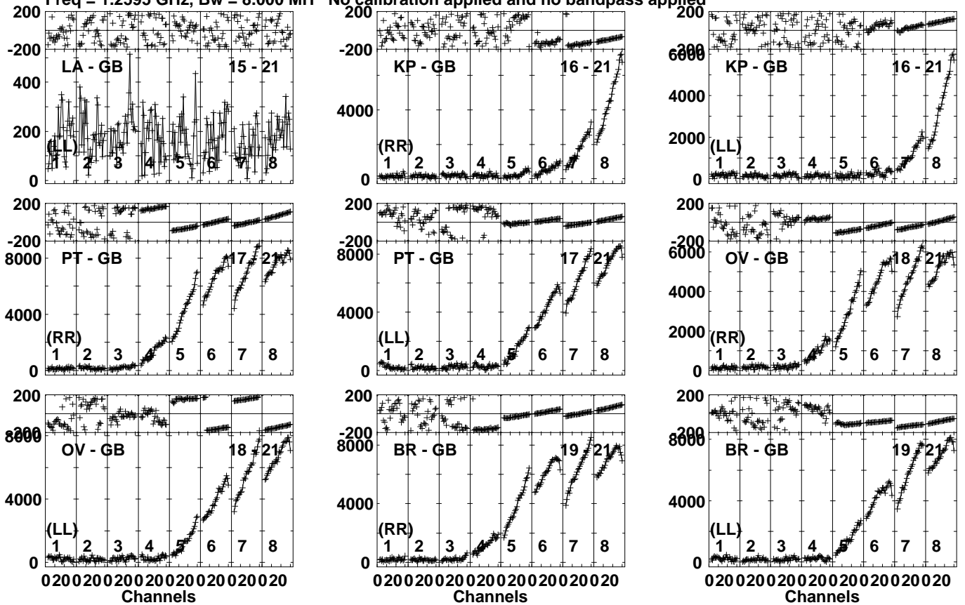
Lower frame: Micro Ampl Jy Top frame: Phas deg Vector averaged cross-power spectrum Several baselines displayed Timerange: 01/04:30:31 to 01/04:31:59
