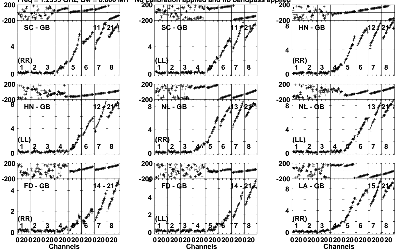
Lower frame: Milli Ampl Jy Top frame: Phas deg Vector averaged cross-power spectrum Several baselines displayed Timerange: 01/08:36:31 to 01/08:37:59
