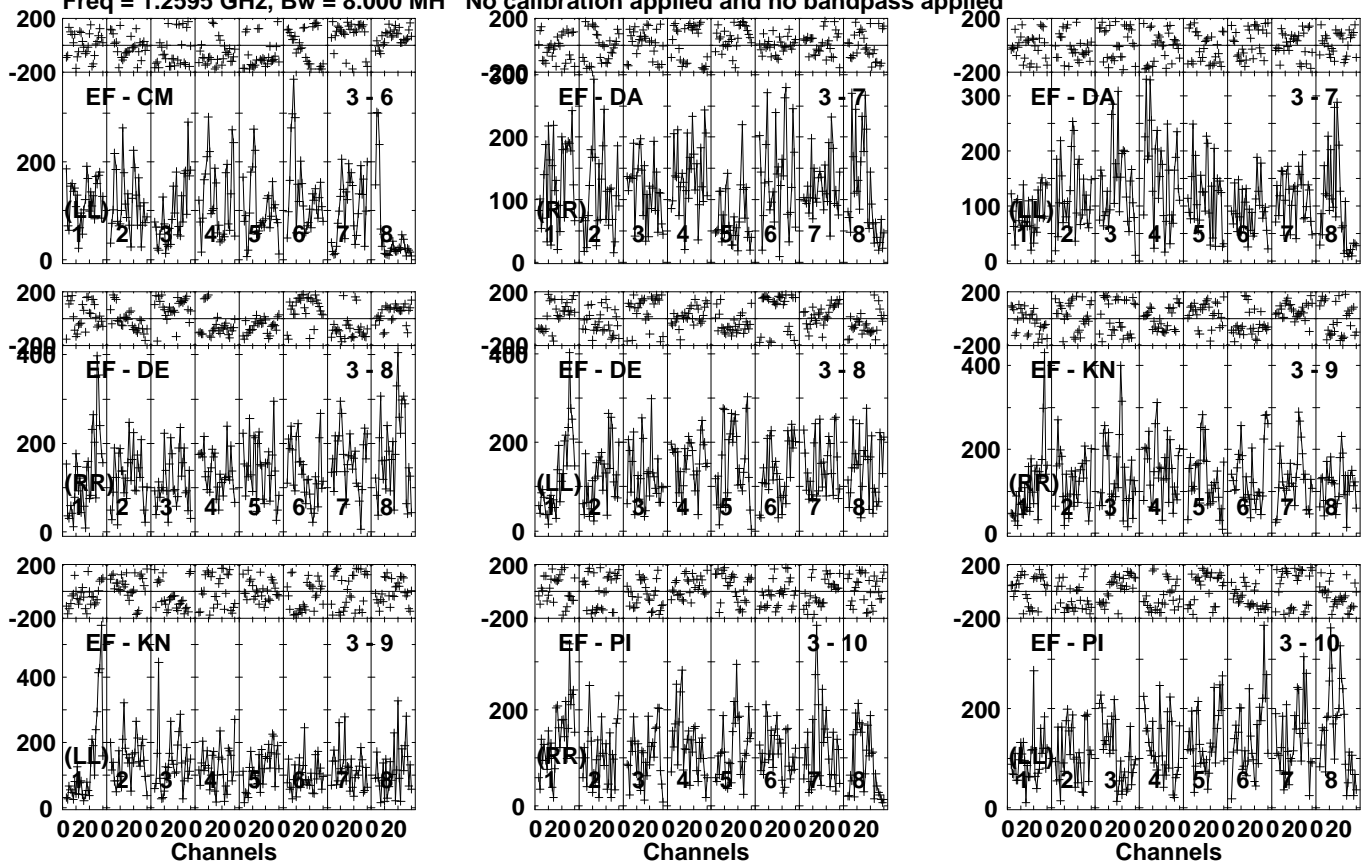
Lower frame: Micro Ampl Jy Top frame: Phas deg Vector averaged cross-power spectrum Several baselines displayed Timerange: 01/01:19:01 to 01/01:22:29
