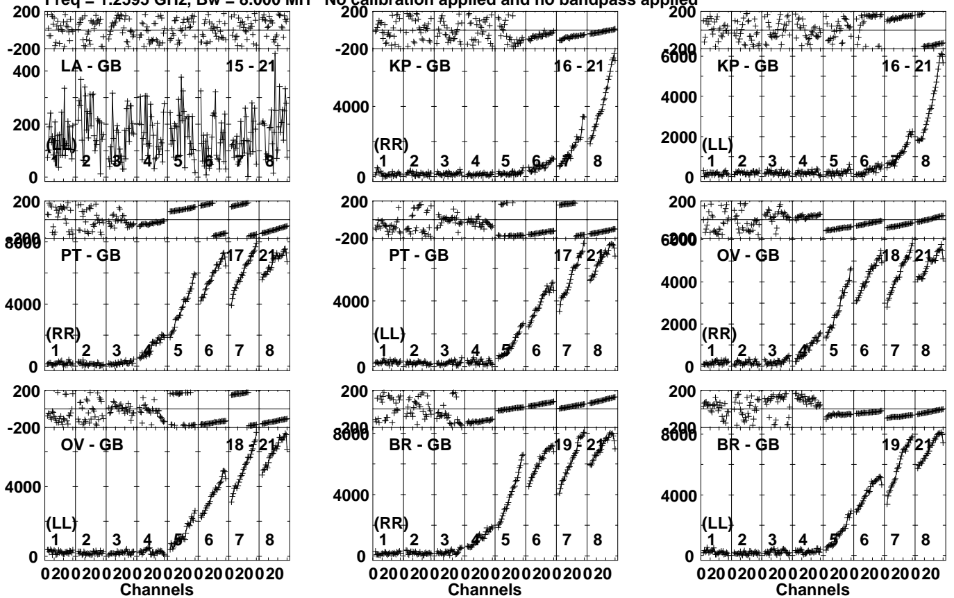
Lower frame: Micro Ampl Jy Top frame: Phas deg Vector averaged cross-power spectrum Several baselines displayed Timerange: 01/04:12:31 to 01/04:13:59
