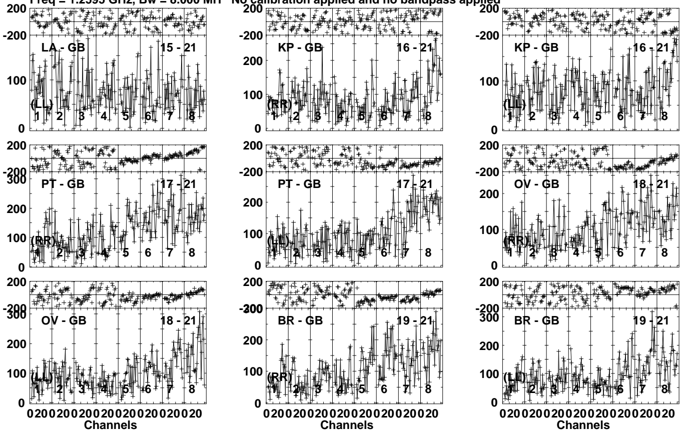
Lower frame: Micro Ampl Jy Top frame: Phas deg Vector averaged cross-power spectrum Several baselines displayed Timerange: 01/06:11:11 to 01/06:17:59
