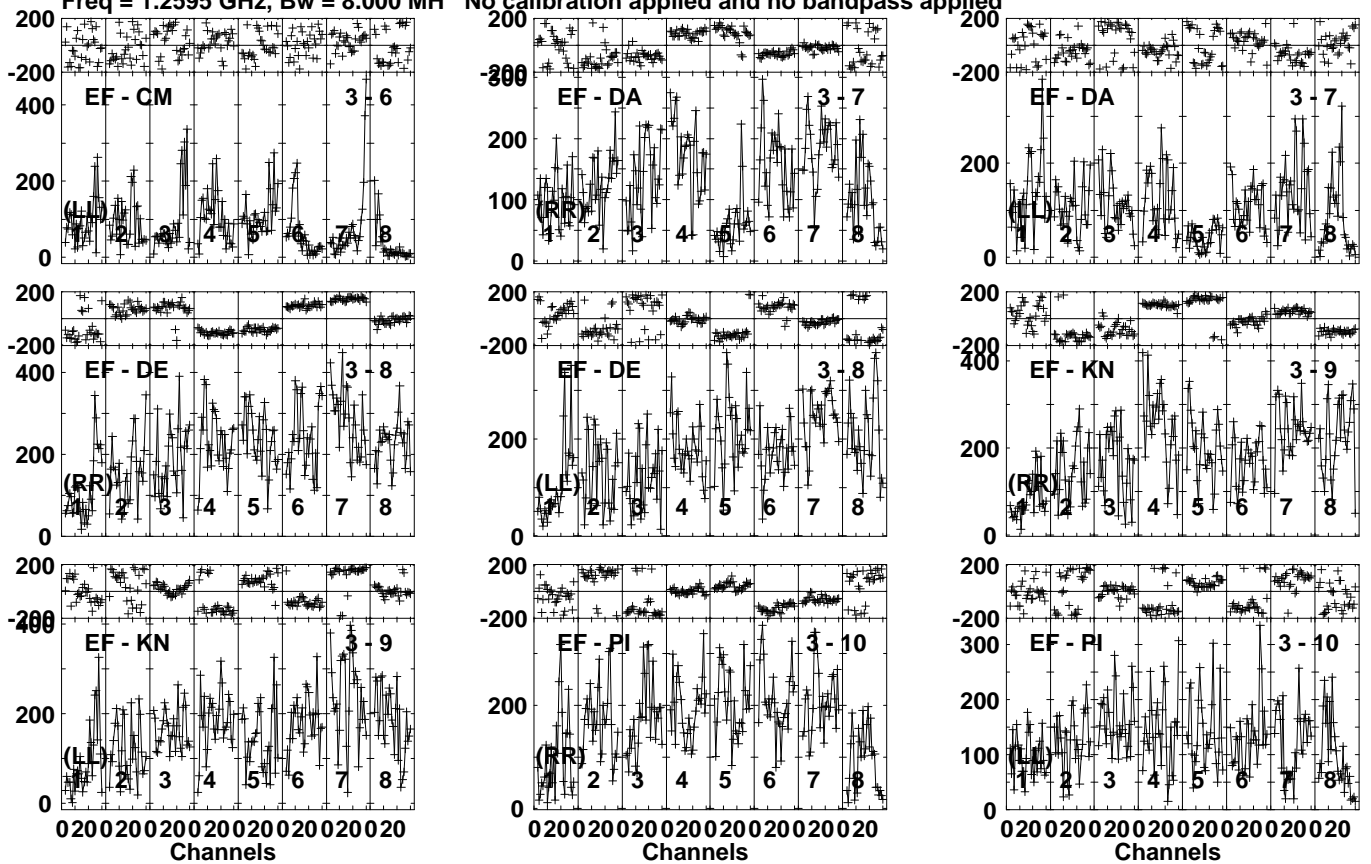
Lower frame: Micro Ampl Jy Top frame: Phas deg Vector averaged cross-power spectrum Several baselines displayed Timerange: 00/20:48:01 to 00/20:52:59
