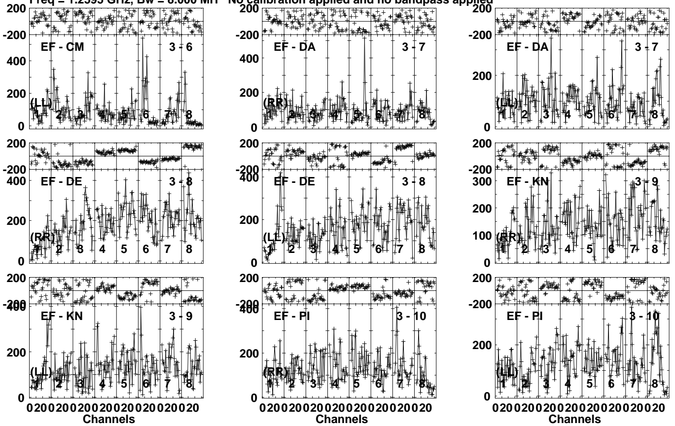
Lower frame: Micro Ampl Jy Top frame: Phas deg Vector averaged cross-power spectrum Several baselines displayed Timerange: 00/21:30:01 to 00/21:34:59
