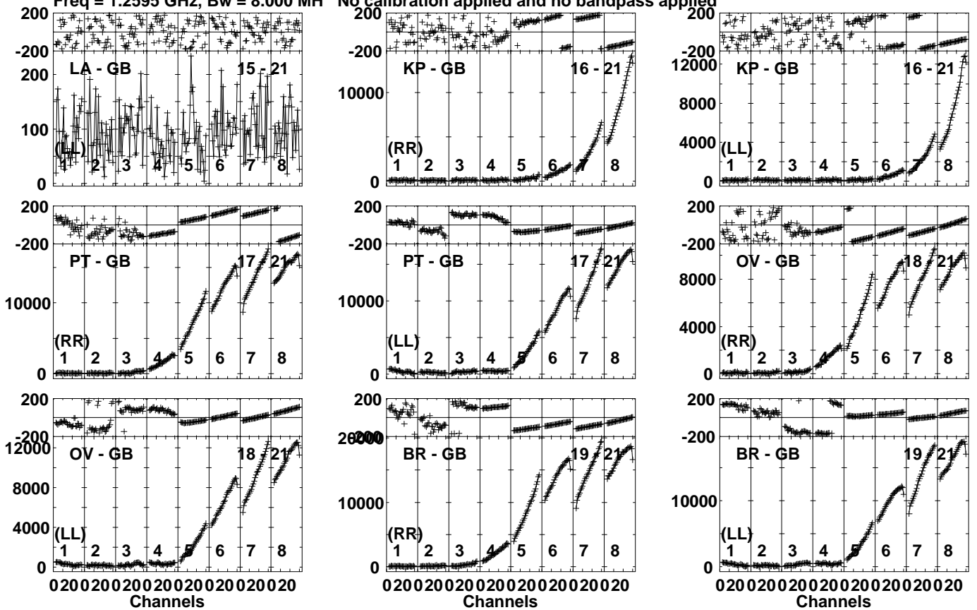
Lower frame: Micro Ampl Jy Top frame: Phas deg Vector averaged cross-power spectrum Several baselines displayed Timerange: 01/07:07:01 to 01/07:11:59
