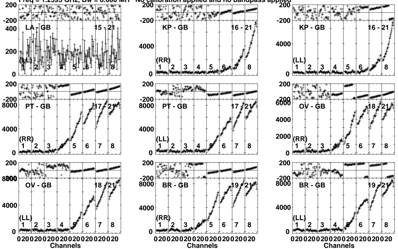
Lower frame: Micro Ampl Jy Top frame: Phas deg Vector averaged cross-power spectrum Several baselines displayed Timerange: 01/05:24:31 to 01/05:25:59
