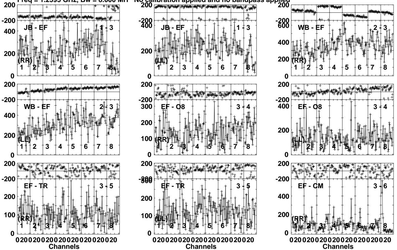
Lower frame: Micro Ampl Jy Top frame: Phas deg Vector averaged cross-power spectrum Several baselines displayed Timerange: 00/21:23:01 to 00/21:27:59
