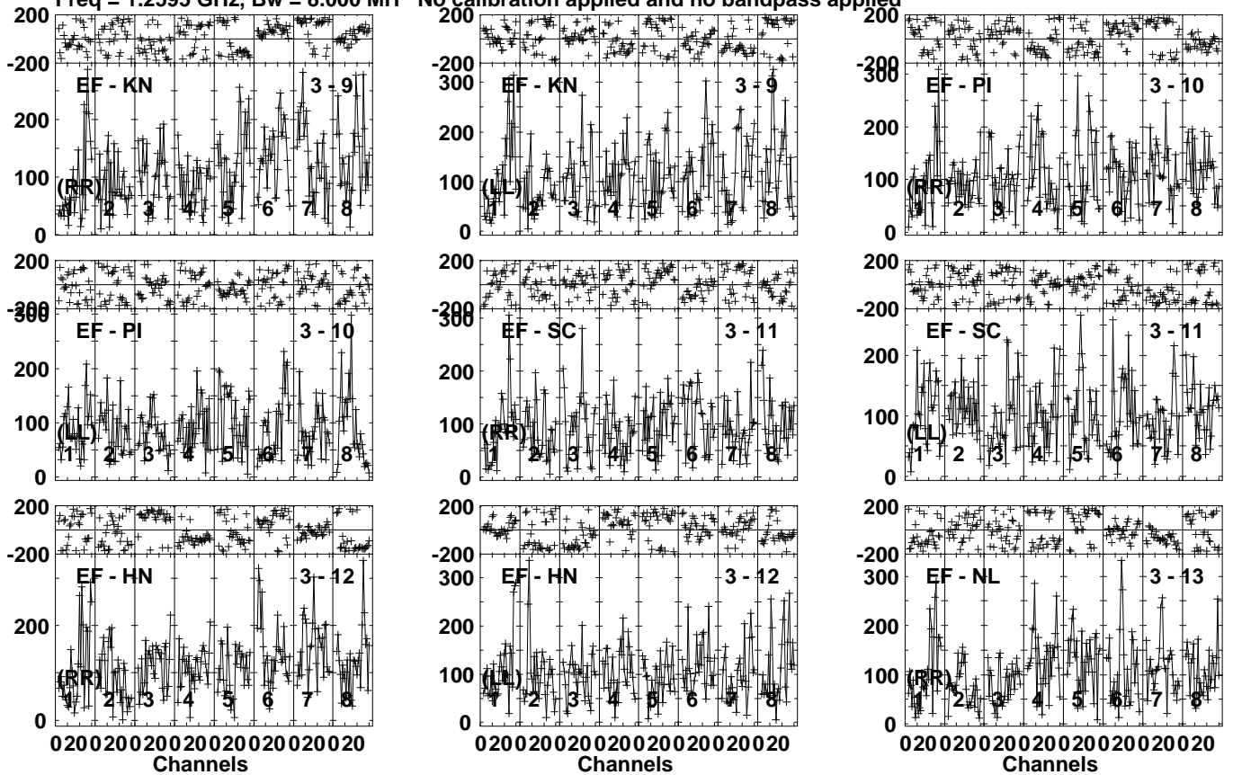
Lower frame: Micro Ampl Jy Top frame: Phas deg Vector averaged cross-power spectrum Several baselines displayed Timerange: 01/02:38:01 to 01/02:42:59
