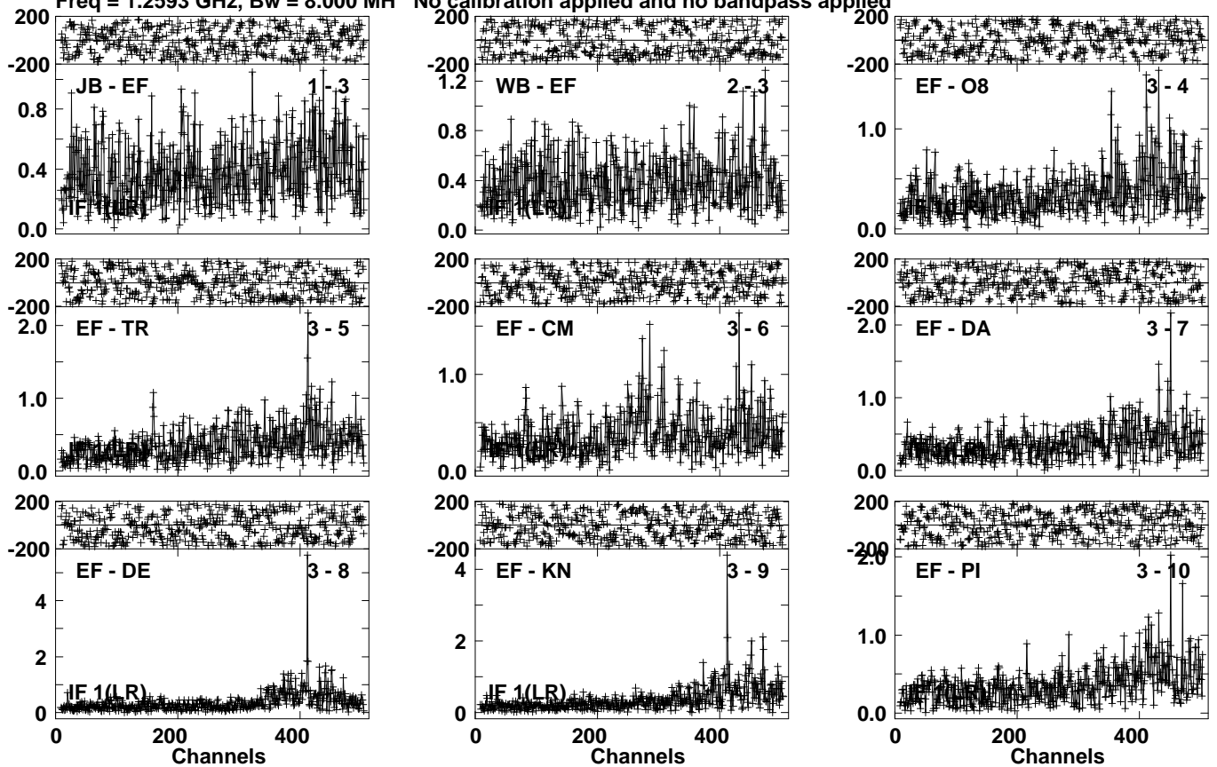
Lower frame: Milli Ampl Jy Top frame: Phas deg Vector averaged cross-power spectrum Several baselines displayed Timerange: 00/23:48:01 to 00/23:52:59
