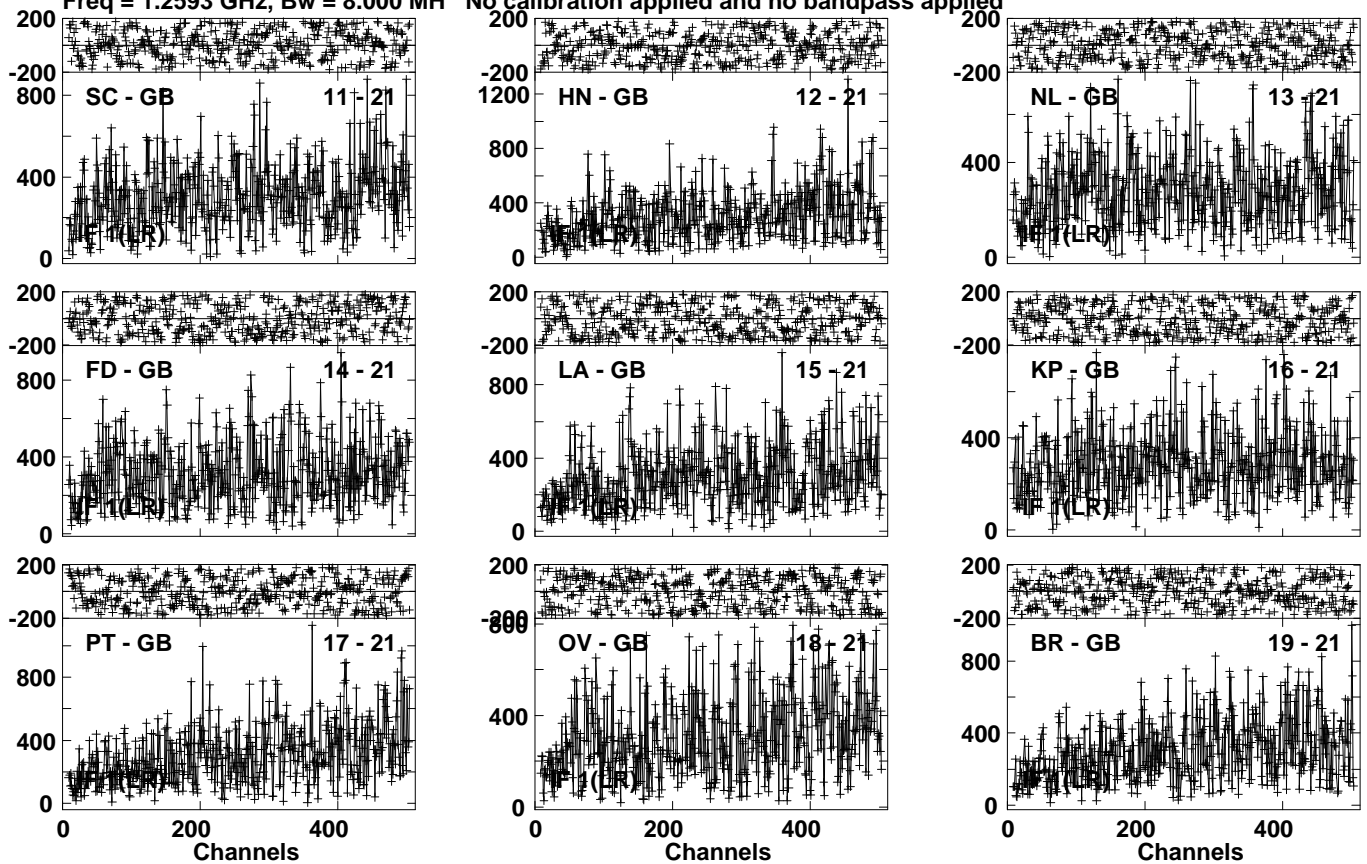
Lower frame: Micro Ampl Jy Top frame: Phas deg Vector averaged cross-power spectrum Several baselines displayed Timerange: 01/05:53:13 to 01/05:59:59
