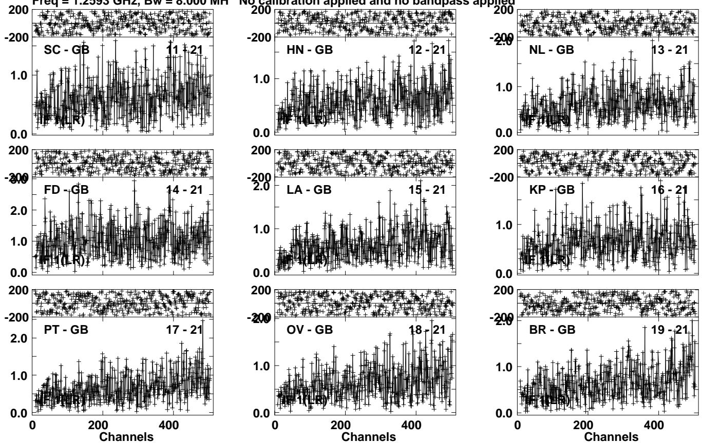
Lower frame: Milli Ampl Jy Top frame: Phas deg Vector averaged cross-power spectrum Several baselines displayed Timerange: 01/04:02:01 to 01/04:04:59
