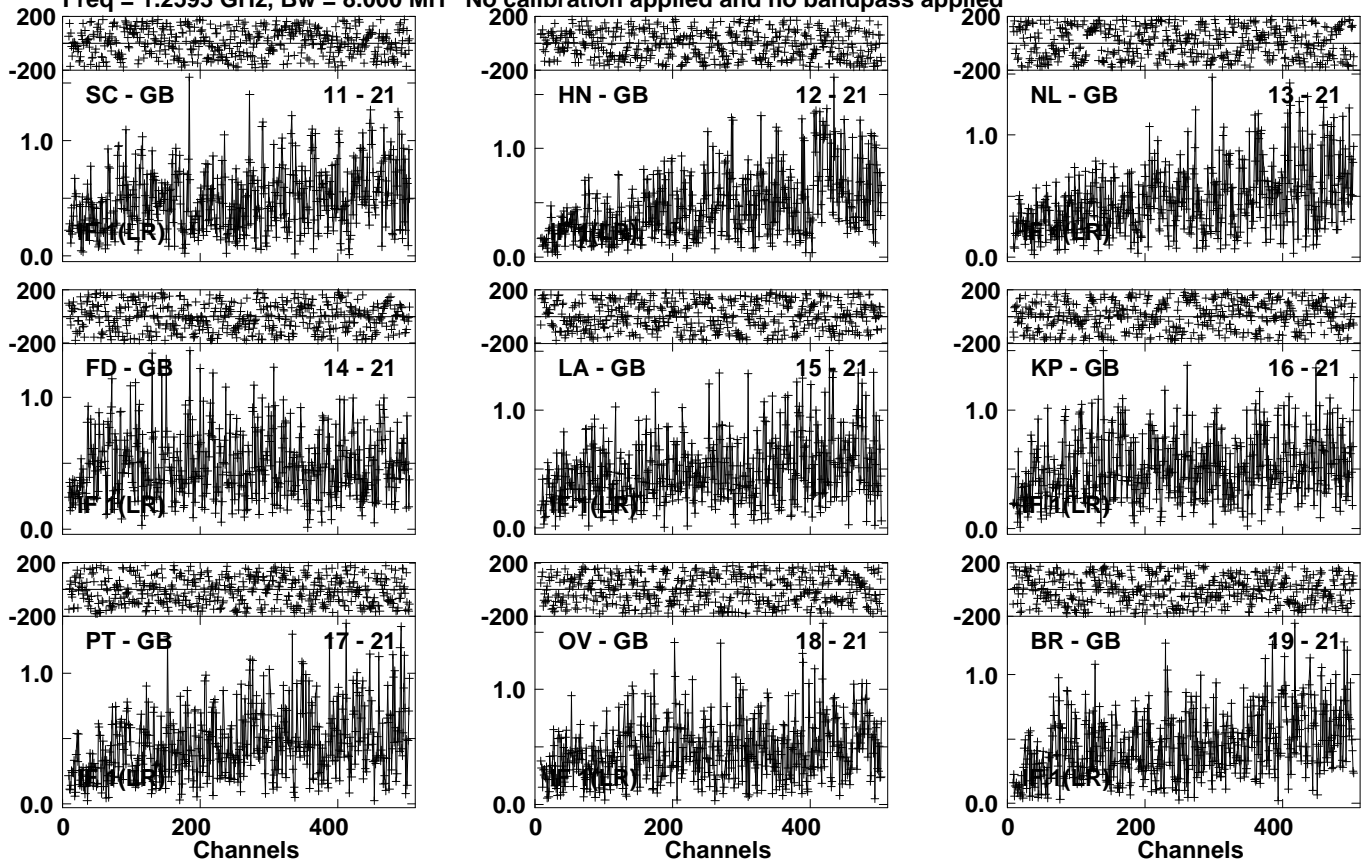
Lower frame: Milli Ampl Jy Top frame: Phas deg Vector averaged cross-power spectrum Several baselines displayed Timerange: 01/07:14:01 to 01/07:16:59
