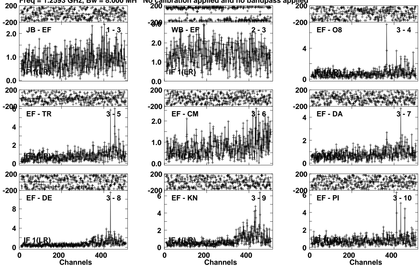
Lower frame: Milli Ampl Jy Top frame: Phas deg Vector averaged cross-power spectrum Several baselines displayed Timerange: 00/23:46:31 to 00/23:47:59
