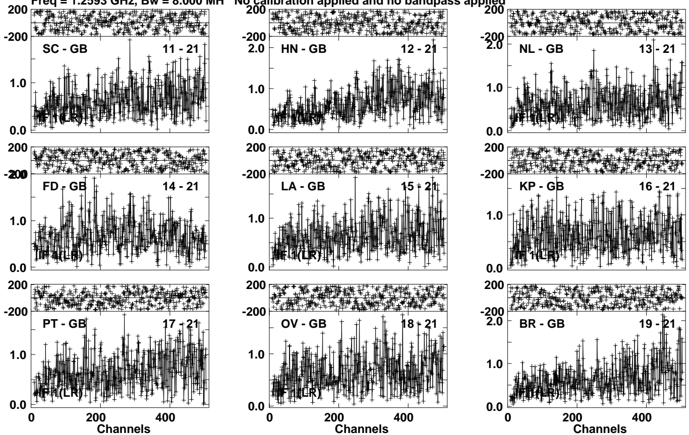
Lower frame: Milli Ampl Jy Top frame: Phas deg Vector averaged cross-power spectrum Several baselines displayed Timerange: 01/09:48:31 to 01/09:49:59
