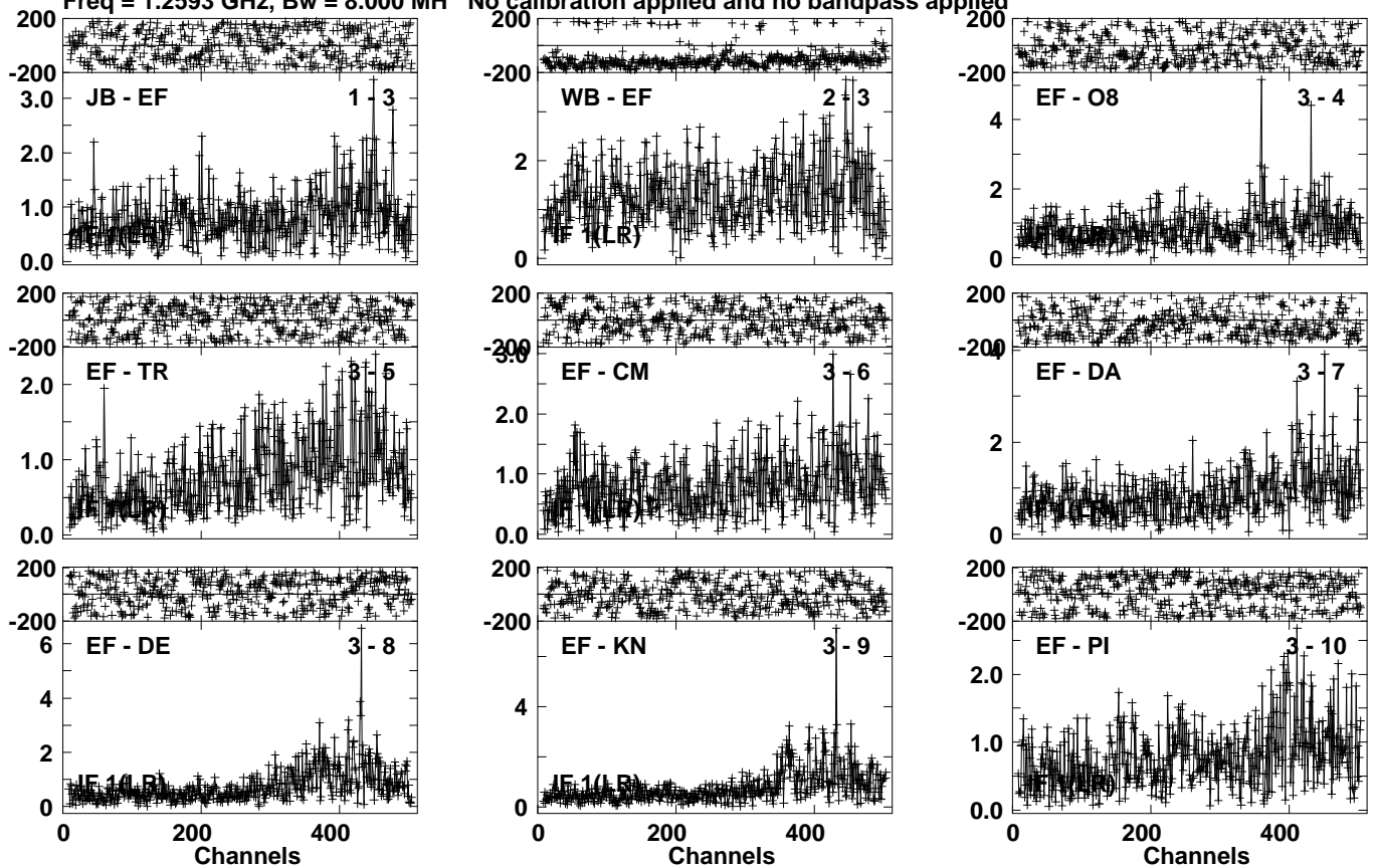
Lower frame: Milli Ampl Jy Top frame: Phas deg Vector averaged cross-power spectrum Several baselines displayed Timerange: 00/23:18:31 to 00/23:19:59
