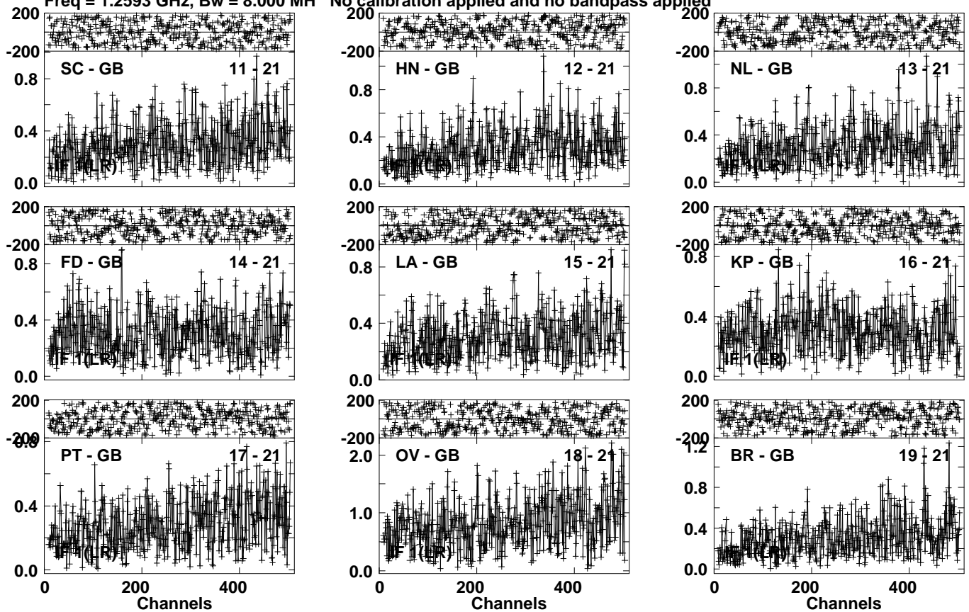
Lower frame: Milli Ampl Jy Top frame: Phas deg Vector averaged cross-power spectrum Several baselines displayed Timerange: 01/07:44:11 to 01/07:50:59
