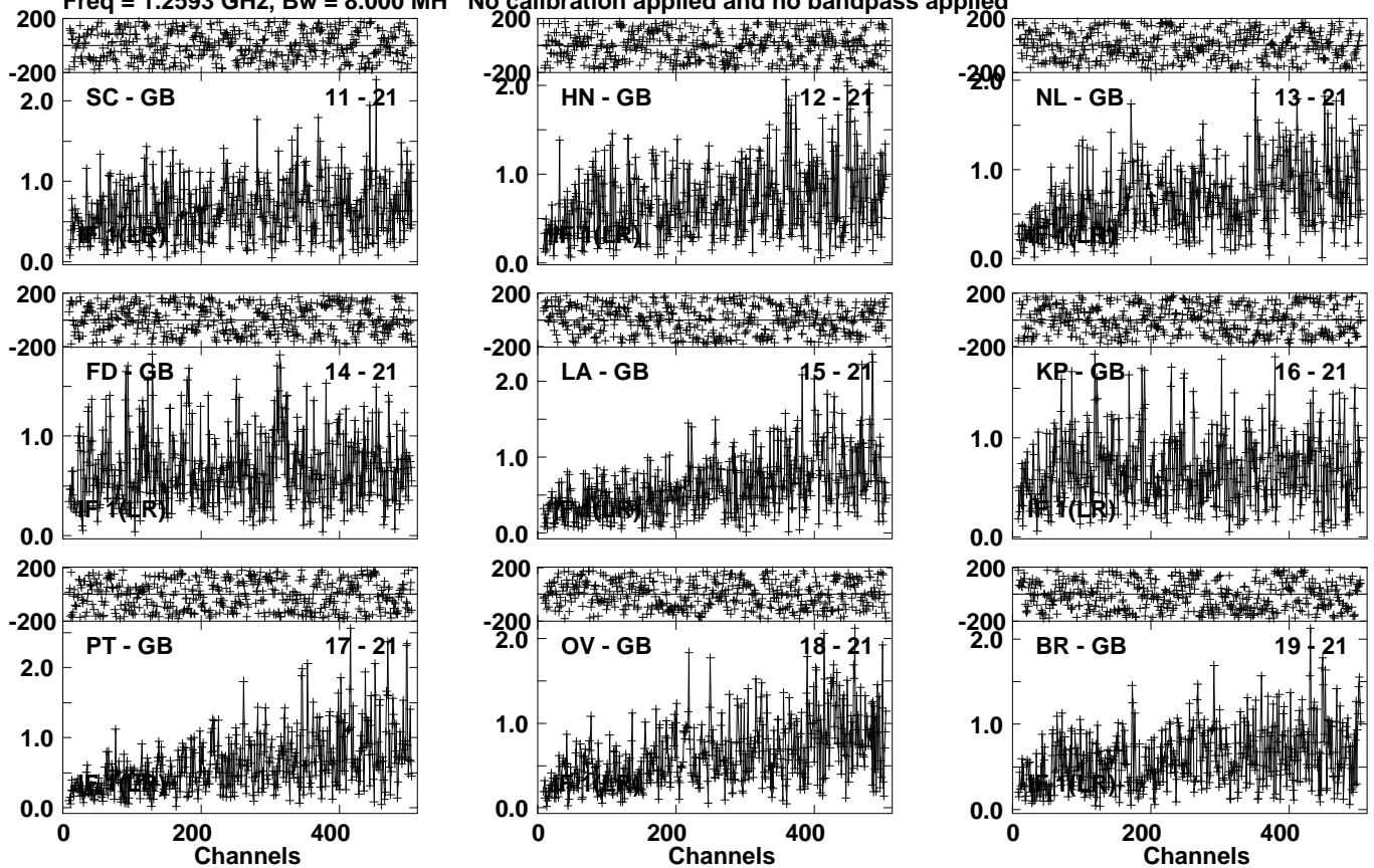
Lower frame: Milli Ampl Jy Top frame: Phas deg Vector averaged cross-power spectrum Several baselines displayed Timerange: 01/08:45:31 to 01/08:46:59
