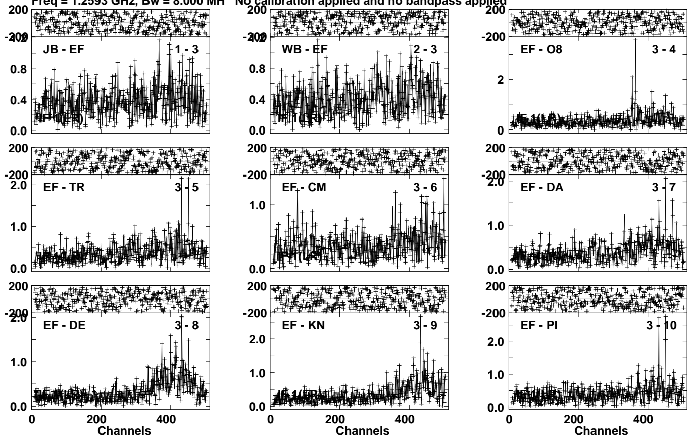
Lower frame: Milli Ampl Jy Top frame: Phas deg Vector averaged cross-power spectrum Several baselines displayed Timerange: 00/20:55:01 to 00/20:59:59
