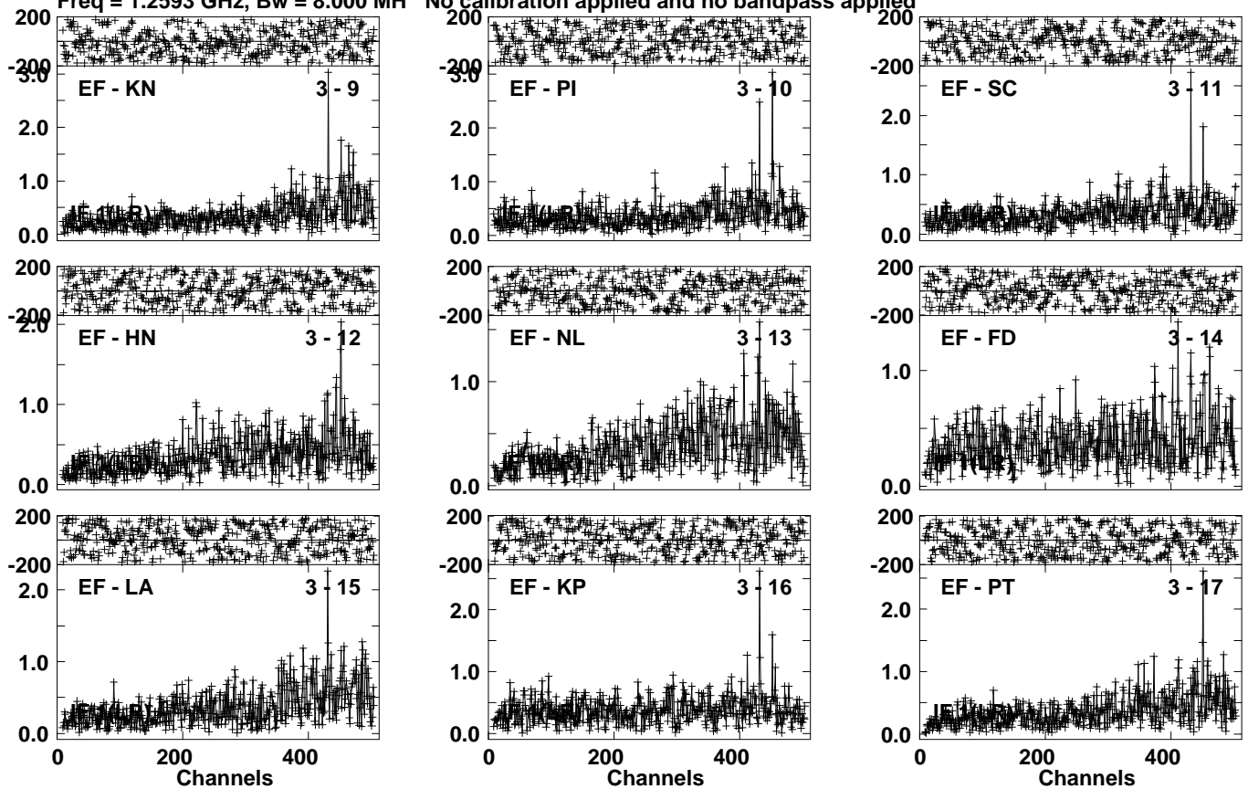
Lower frame: Milli Ampl Jy Top frame: Phas deg Vector averaged cross-power spectrum Several baselines displayed Timerange: 01/02:24:01 to 01/02:28:59
