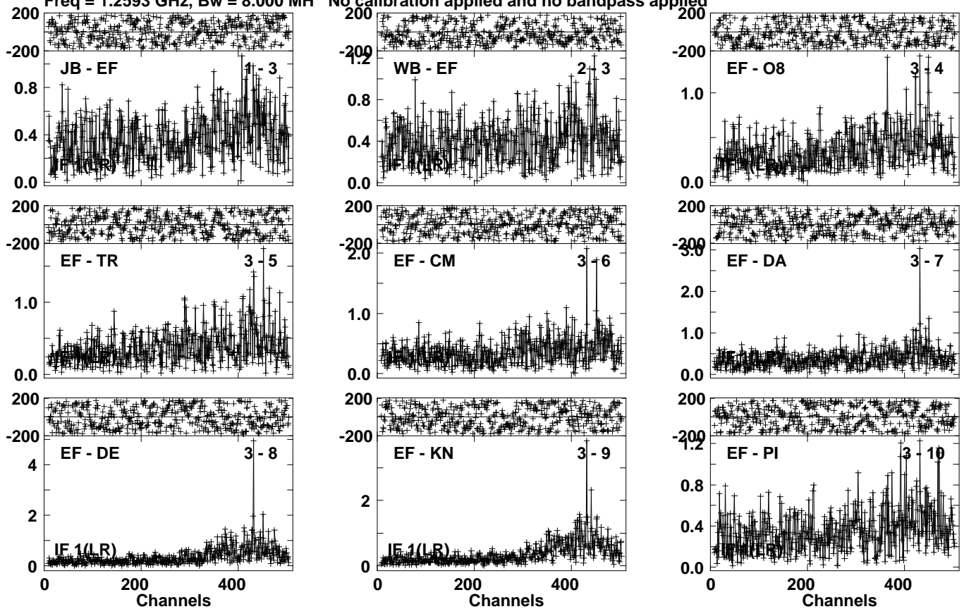
Lower frame: Milli Ampl Jy Top frame: Phas deg Vector averaged cross-power spectrum Several baselines displayed Timerange: 00/22:52:01 to 00/22:56:59
