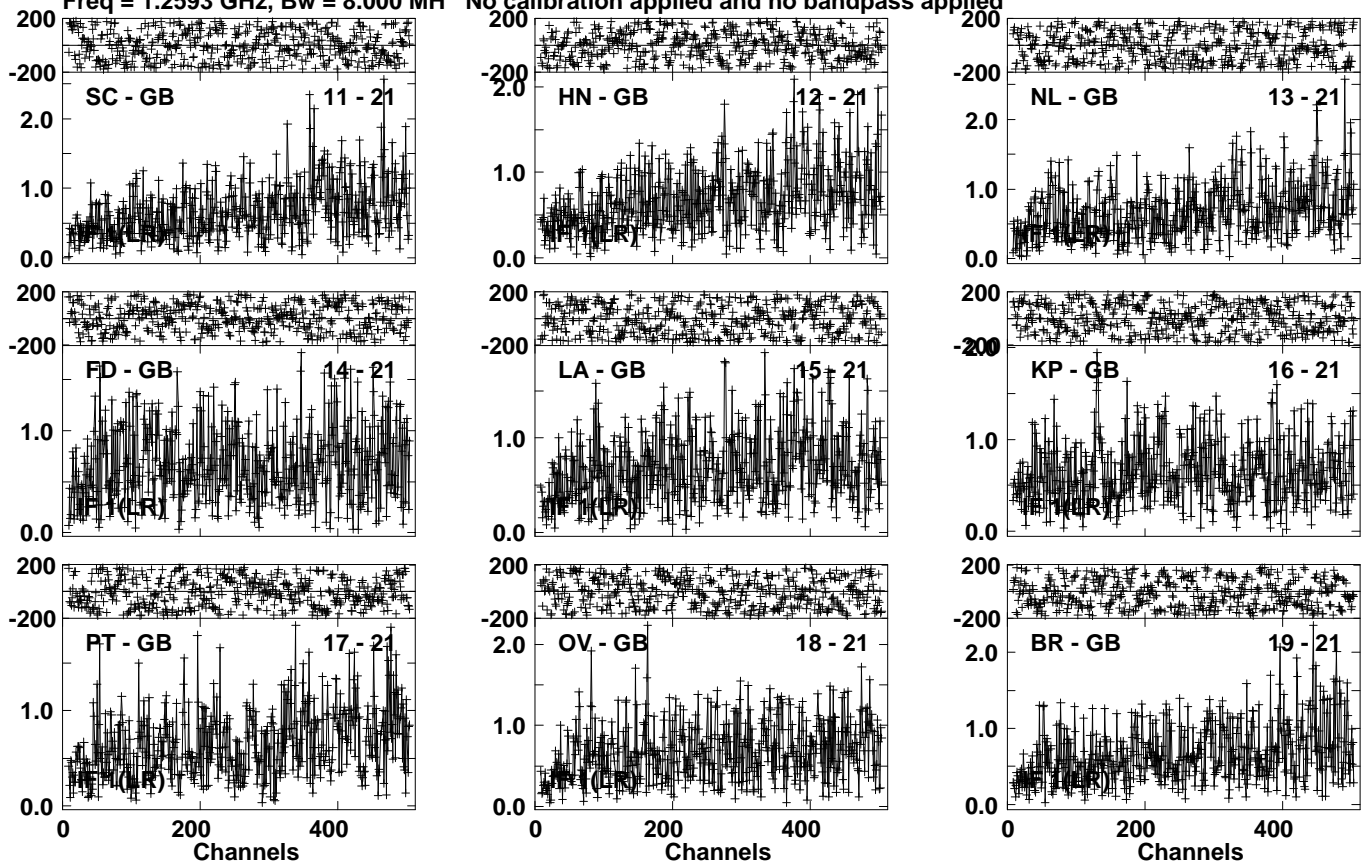
Lower frame: Milli Ampl Jy Top frame: Phas deg Vector averaged cross-power spectrum Several baselines displayed Timerange: 01/07:24:31 to 01/07:25:59
