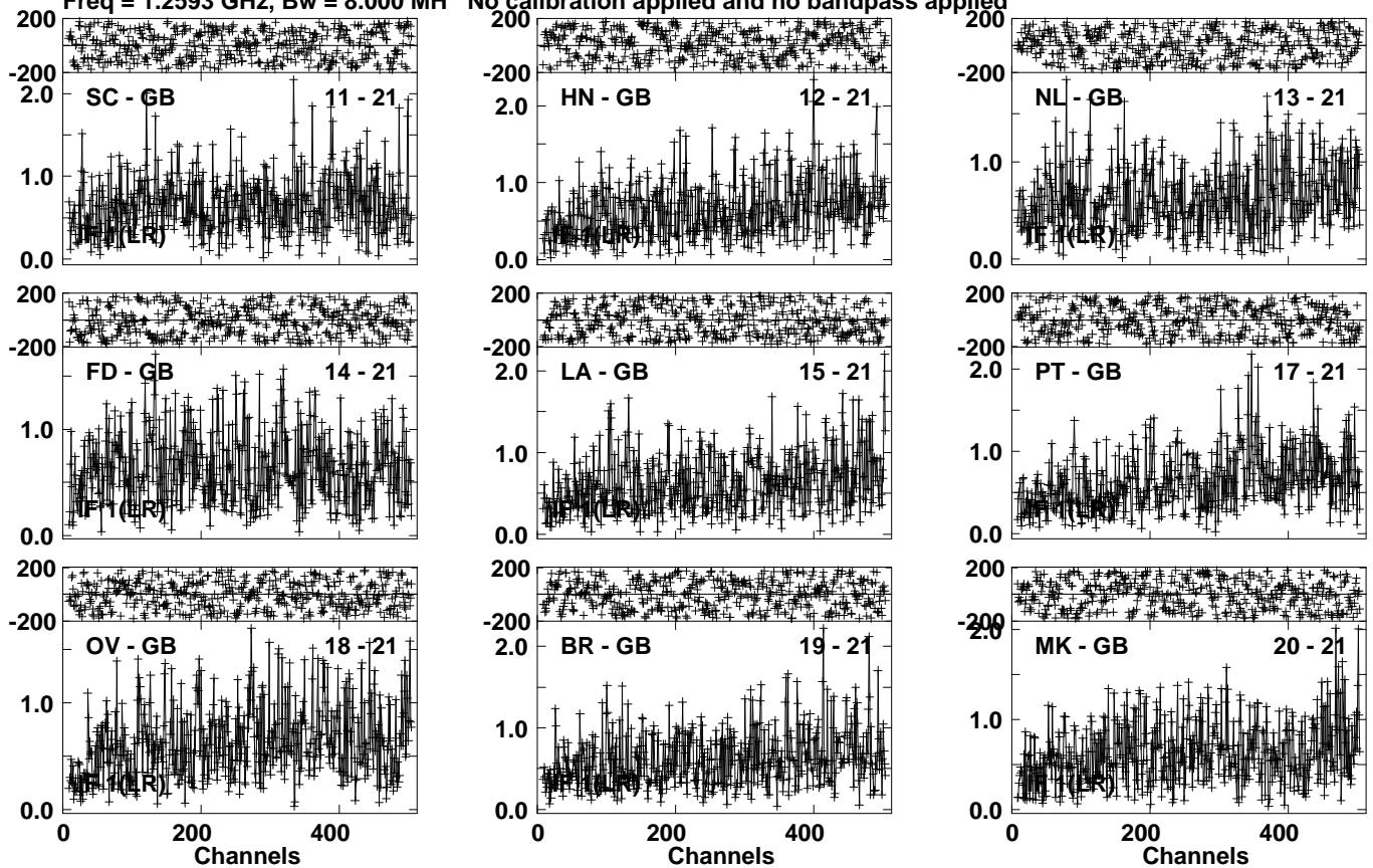
Lower frame: Milli Ampl Jy Top frame: Phas deg Vector averaged cross-power spectrum Several baselines displayed Timerange: 01/04:48:31 to 01/04:49:59
