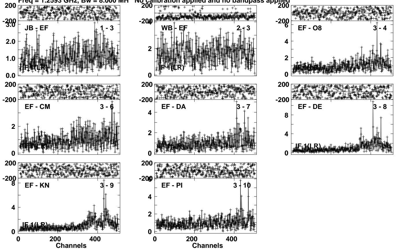
Lower frame: Milli Ampl Jy Top frame: Phas deg Vector averaged cross-power spectrum Several baselines displayed Timerange: 00/22:07:01 to 00/22:09:59
