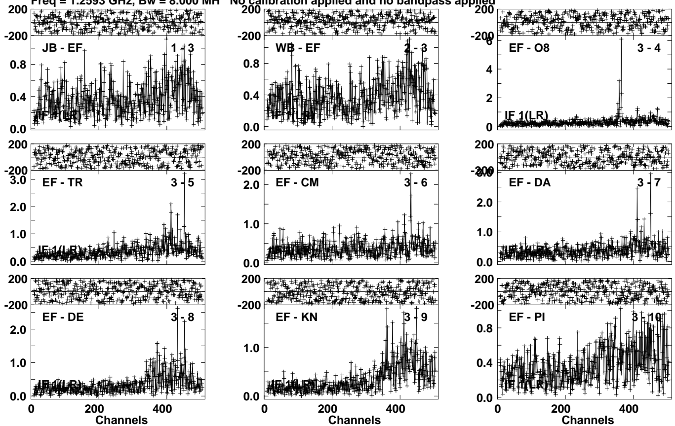
Lower frame: Milli Ampl Jy Top frame: Phas deg Vector averaged cross-power spectrum Several baselines displayed Timerange: 01/01:12:01 to 01/01:16:59
