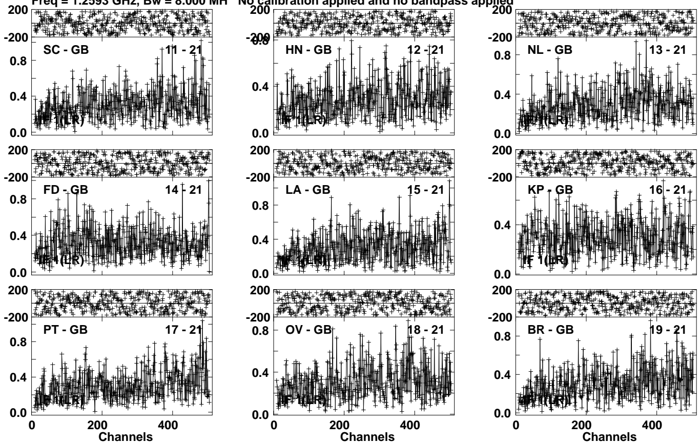
Lower frame: Milli Ampl Jy Top frame: Phas deg Vector averaged cross-power spectrum Several baselines displayed Timerange: 01/06:38:11 to 01/06:44:59
