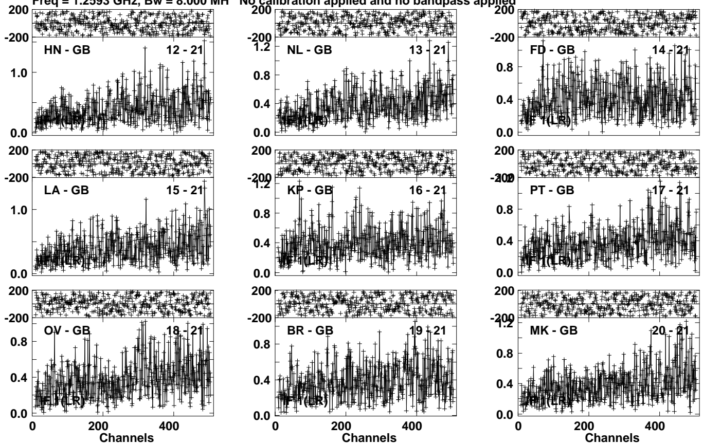
Lower frame: Milli Ampl Jy Top frame: Phas deg Vector averaged cross-power spectrum Several baselines displayed Timerange: 01/10:17:11 to 01/10:21:29
