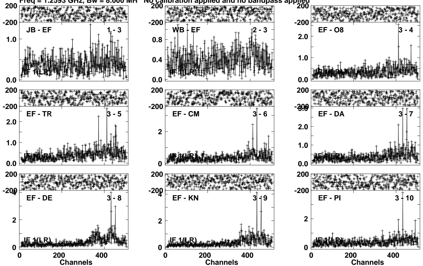
Lower frame: Milli Ampl Jy Top frame: Phas deg Vector averaged cross-power spectrum Several baselines displayed Timerange: 01/00:30:01 to 01/00:34:59
