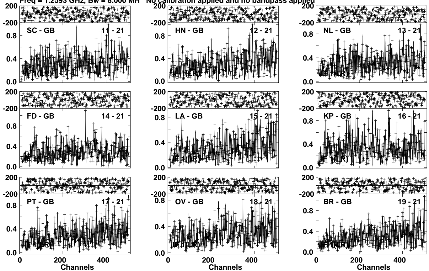
Lower frame: Milli Ampl Jy Top frame: Phas deg Vector averaged cross-power spectrum Several baselines displayed Timerange: 01/06:20:11 to 01/06:26:59
