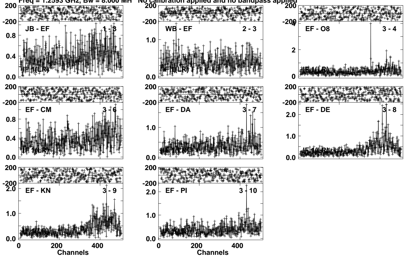
Lower frame: Milli Ampl Jy Top frame: Phas deg Vector averaged cross-power spectrum Several baselines displayed Timerange: 00/20:06:01 to 00/20:10:59
