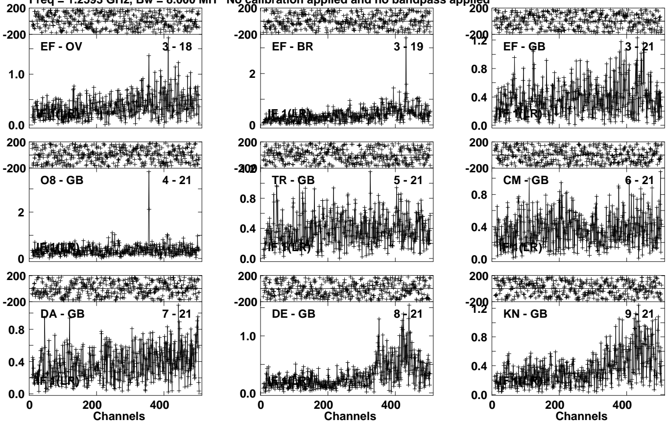
Lower frame: Milli Ampl Jy Top frame: Phas deg Vector averaged cross-power spectrum Several baselines displayed Timerange: 01/02:17:01 to 01/02:21:59
