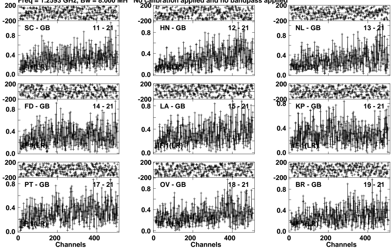
Lower frame: Milli Ampl Jy Top frame: Phas deg Vector averaged cross-power spectrum Several baselines displayed Timerange: 01/07:17:11 to 01/07:23:59
