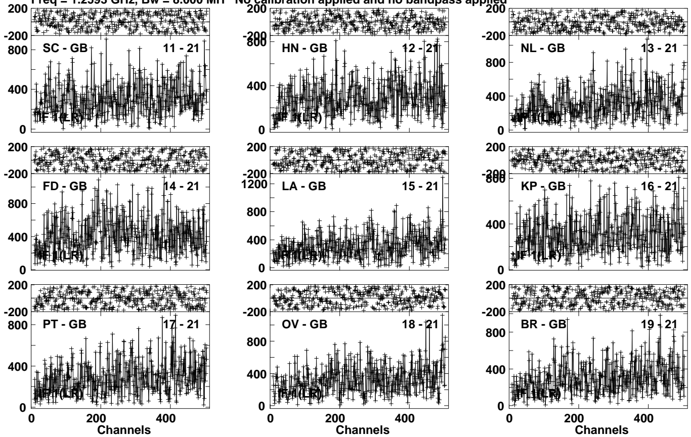
Lower frame: Micro Ampl Jy Top frame: Phas deg Vector averaged cross-power spectrum Several baselines displayed Timerange: 01/04:32:13 to 01/04:38:59
