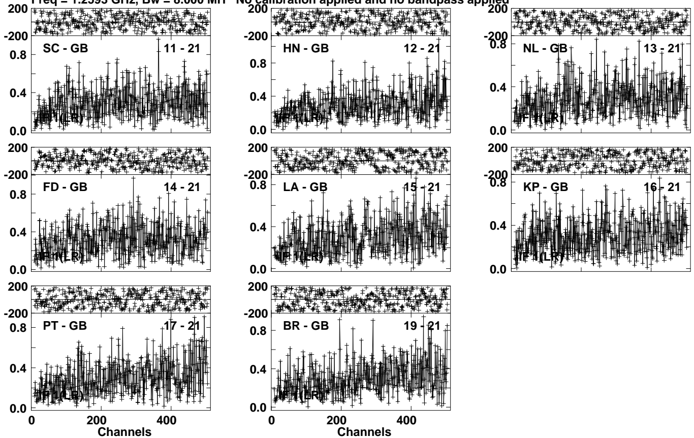
Lower frame: Milli Ampl Jy Top frame: Phas deg Vector averaged cross-power spectrum Several baselines displayed Timerange: 01/08:11:11 to 01/08:17:59
