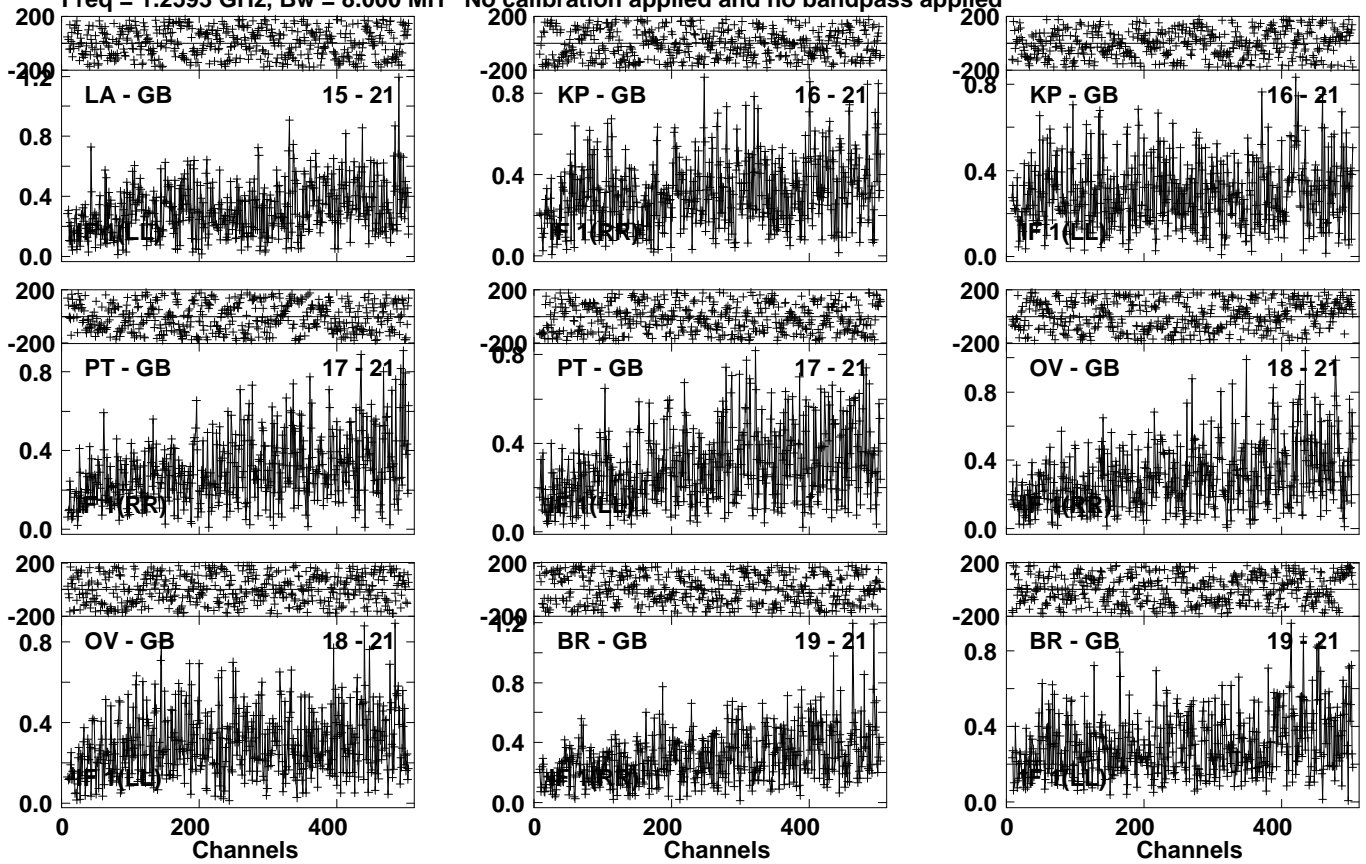
Lower frame: Milli Ampl Jy Top frame: Phas deg Vector averaged cross-power spectrum Several baselines displayed Timerange: 01/07:26:11 to 01/07:32:59
