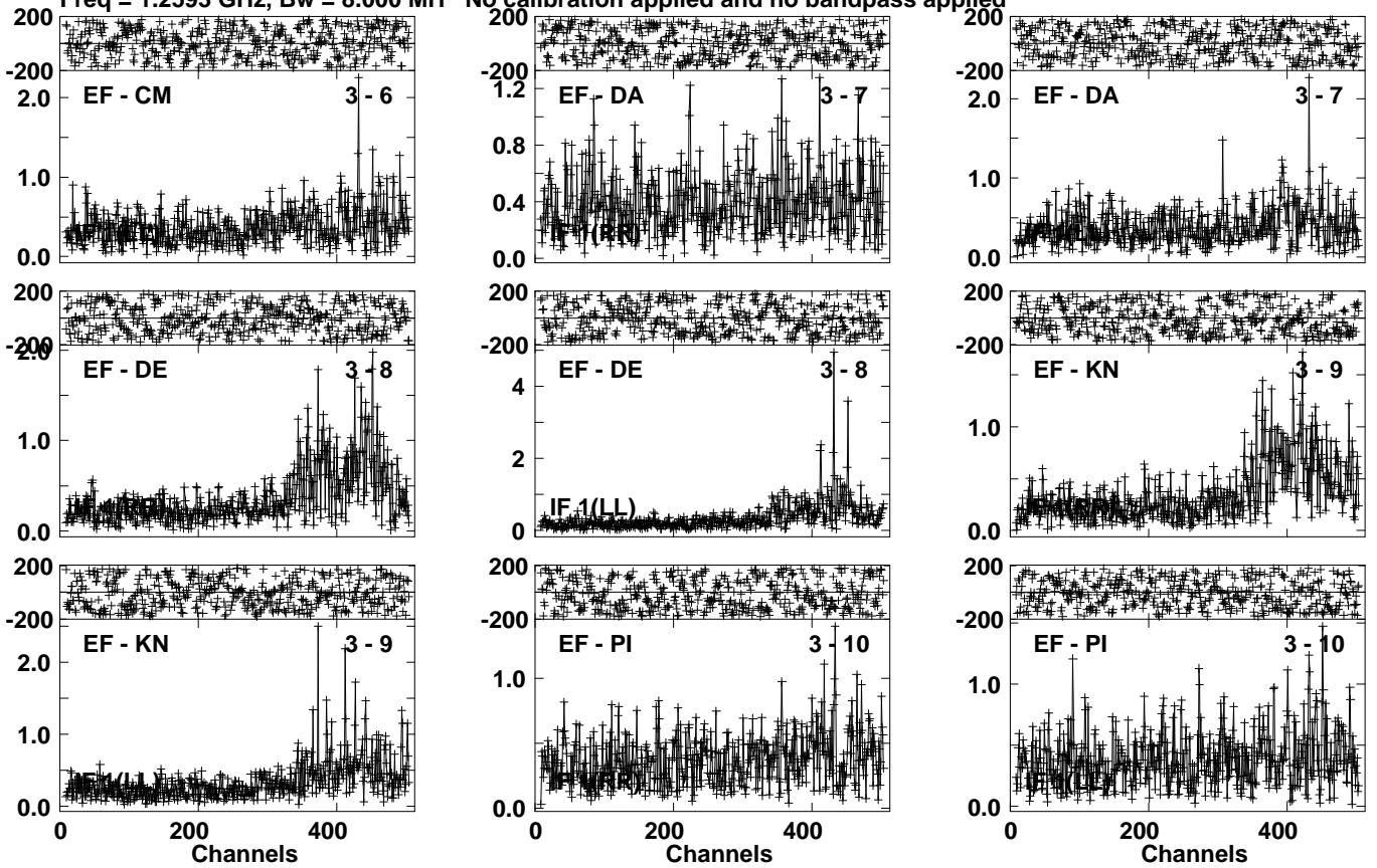
Lower frame: Milli Ampl Jy Top frame: Phas deg Vector averaged cross-power spectrum Several baselines displayed Timerange: 00/21:16:01 to 00/21:20:59
