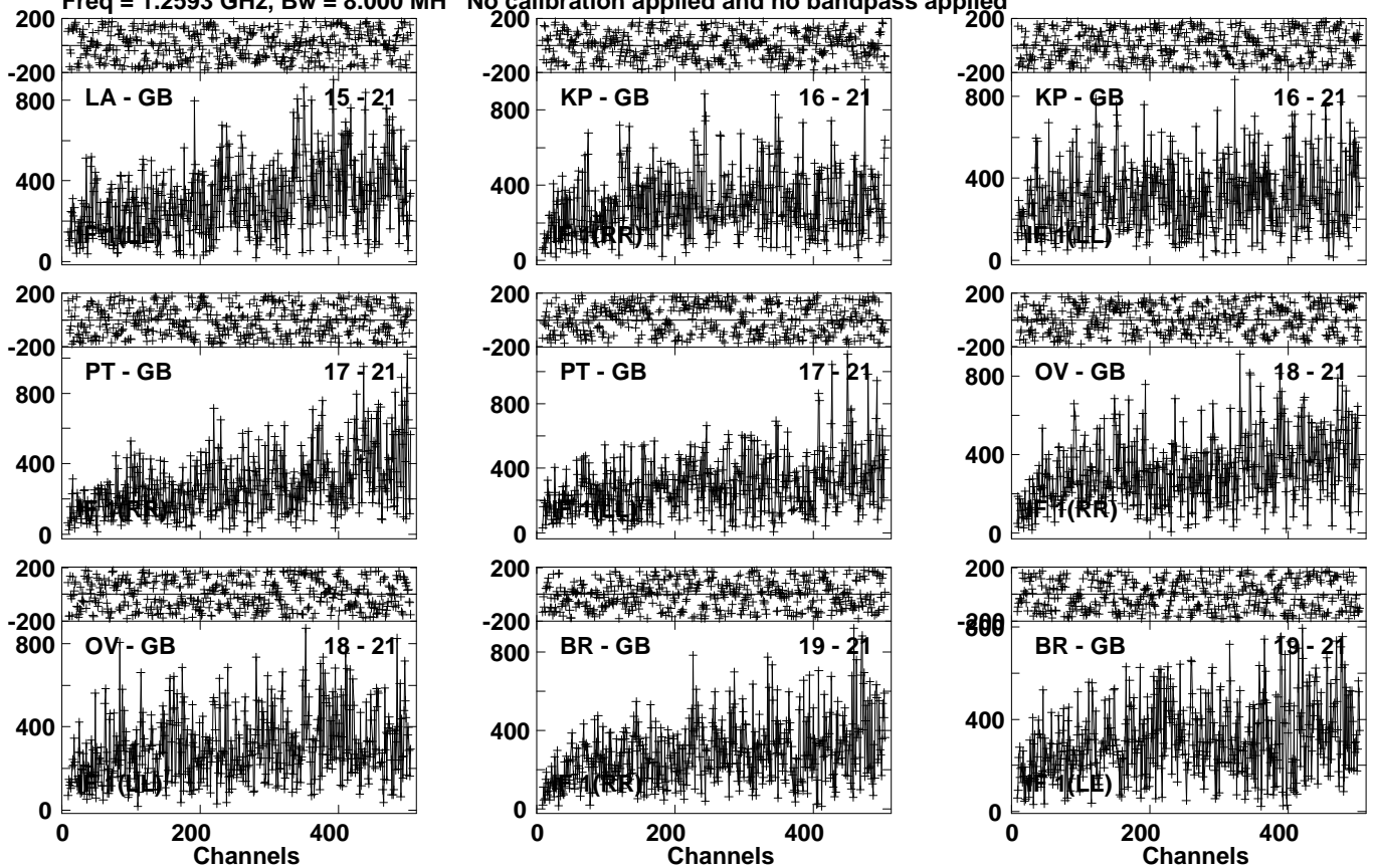
Lower frame: Micro Ampl Jy Top frame: Phas deg Vector averaged cross-power spectrum Several baselines displayed Timerange: 01/09:50:11 to 01/09:56:59
