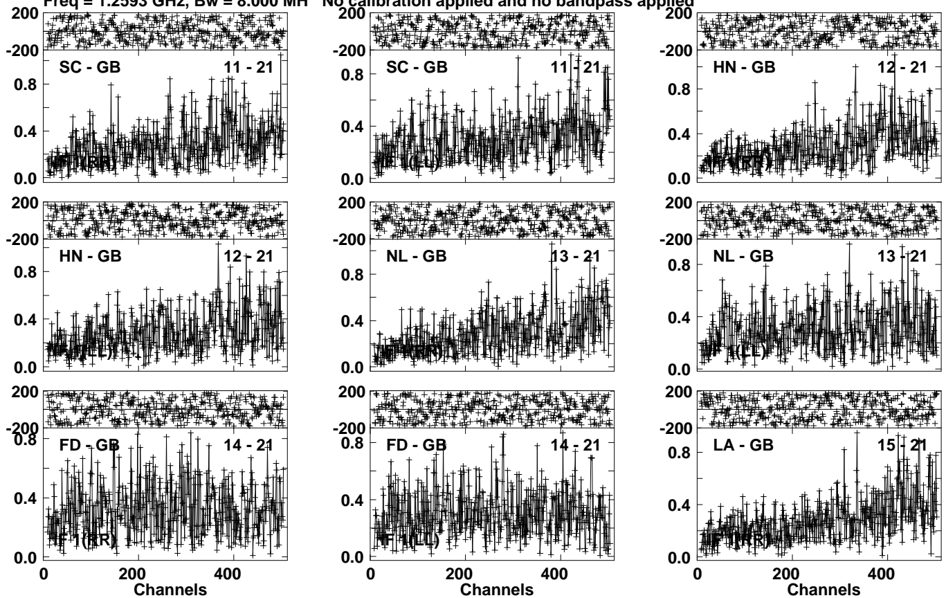
Lower frame: Milli Ampl Jy Top frame: Phas deg Vector averaged cross-power spectrum Several baselines displayed Timerange: 01/08:29:11 to 01/08:35:59
