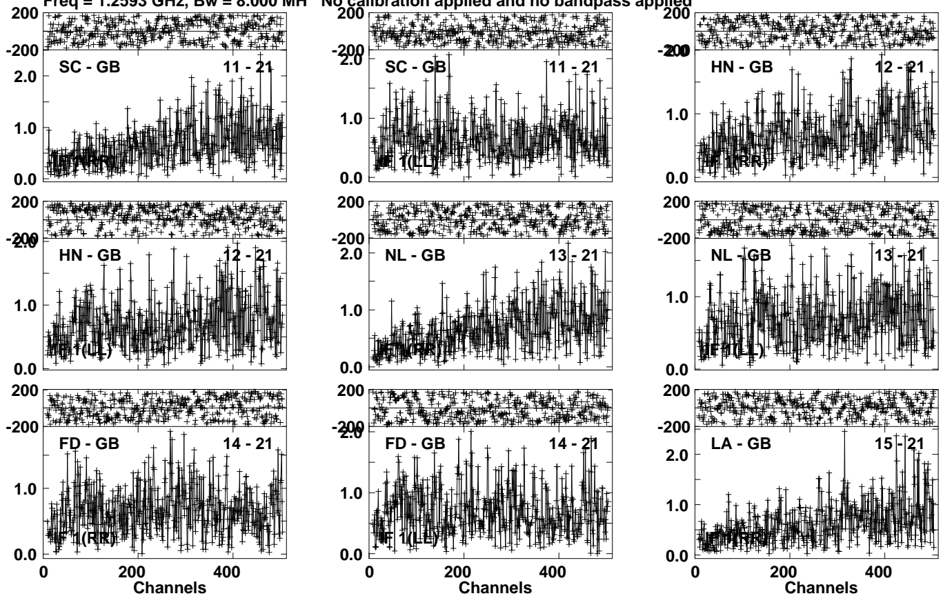
Lower frame: Milli Ampl Jy Top frame: Phas deg Vector averaged cross-power spectrum Several baselines displayed Timerange: 01/05:24:31 to 01/05:25:59
