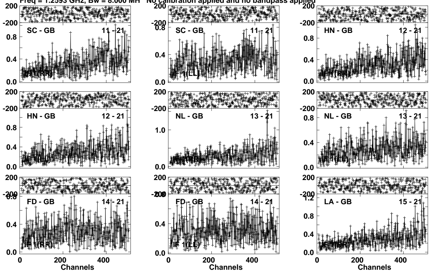
Lower frame: Milli Ampl Jy Top frame: Phas deg Vector averaged cross-power spectrum Several baselines displayed Timerange: 01/09:32:11 to 01/09:38:59
