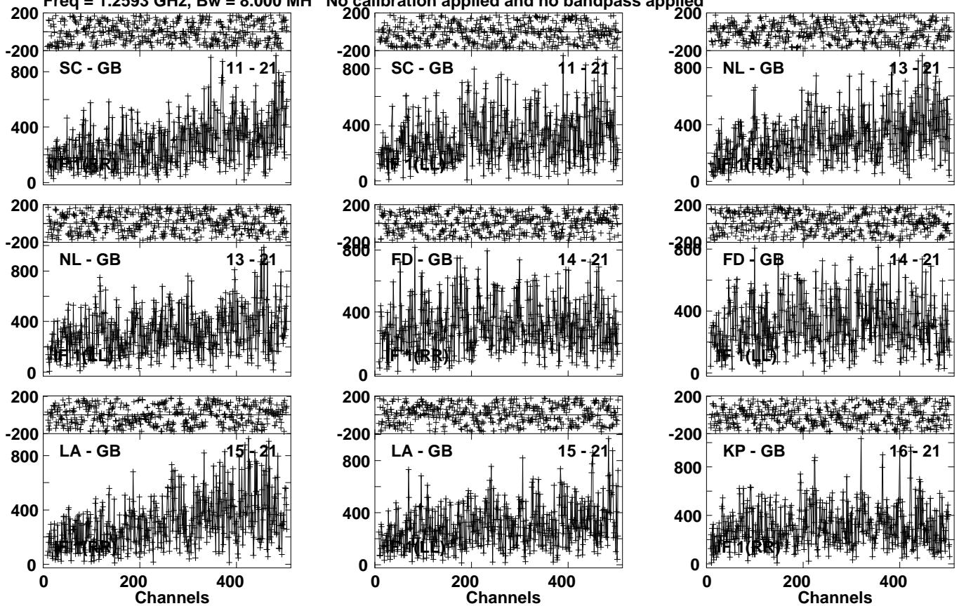
Lower frame: Micro Ampl Jy Top frame: Phas deg Vector averaged cross-power spectrum Several baselines displayed Timerange: 01/05:44:13 to 01/05:50:59
