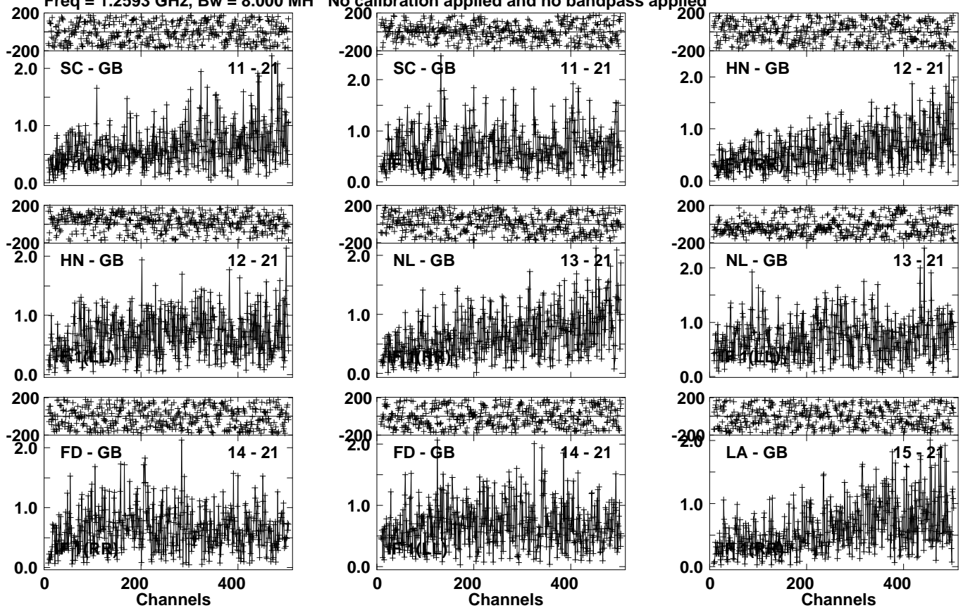
Lower frame: Milli Ampl Jy Top frame: Phas deg Vector averaged cross-power spectrum Several baselines displayed Timerange: 01/09:39:31 to 01/09:40:59
