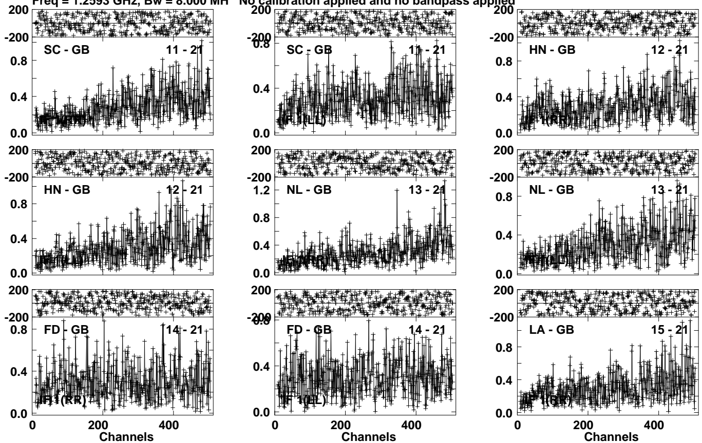
Lower frame: Milli Ampl Jy Top frame: Phas deg Vector averaged cross-power spectrum Several baselines displayed Timerange: 01/08:56:11 to 01/09:02:59
