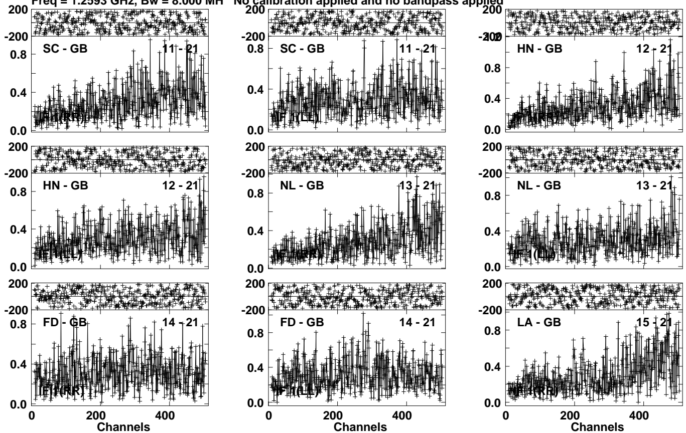
Lower frame: Milli Ampl Jy Top frame: Phas deg Vector averaged cross-power spectrum Several baselines displayed Timerange: 01/06:56:11 to 01/07:02:59
