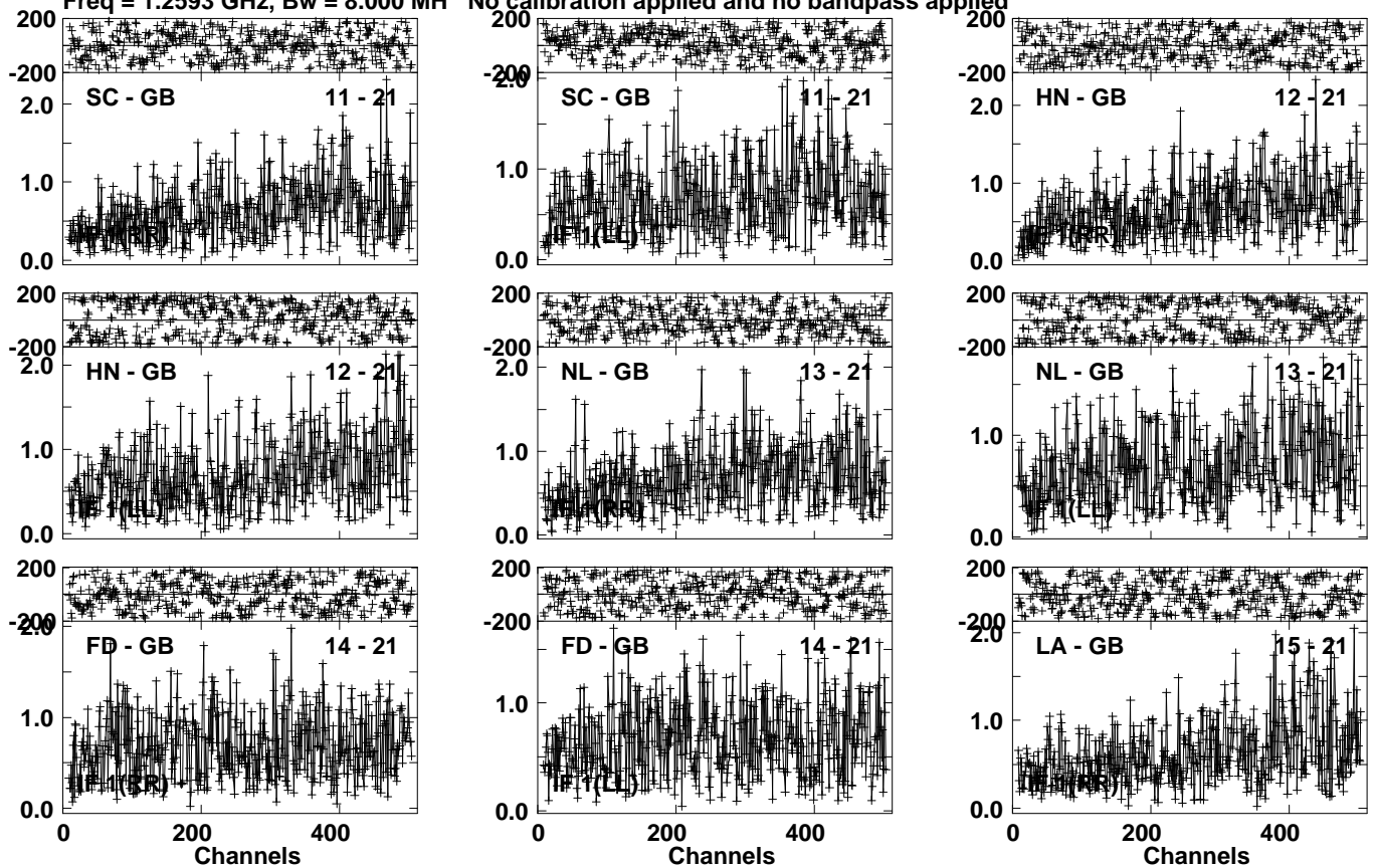
Lower frame: Milli Ampl Jy Top frame: Phas deg Vector averaged cross-power spectrum Several baselines displayed Timerange: 01/06:36:31 to 01/06:37:59
