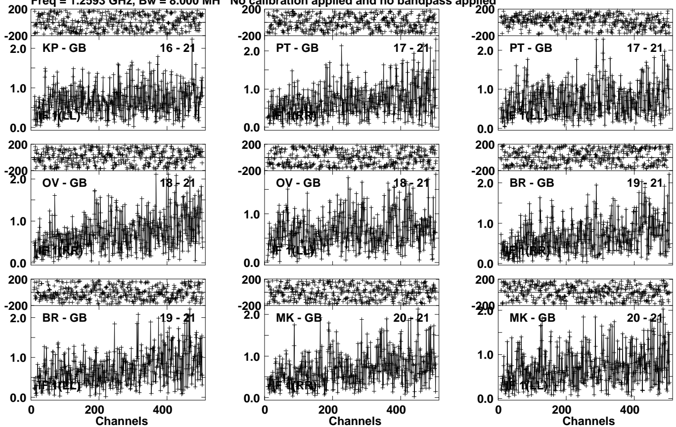
Lower frame: Milli Ampl Jy Top frame: Phas deg Vector averaged cross-power spectrum Several baselines displayed Timerange: 01/05:33:31 to 01/05:34:59
