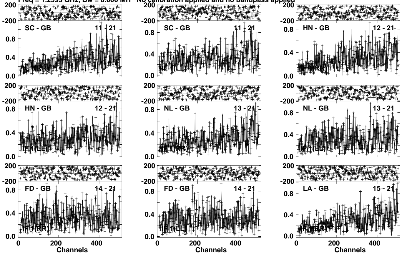
Lower frame: Milli Ampl Jy Top frame: Phas deg Vector averaged cross-power spectrum Several baselines displayed Timerange: 01/06:02:11 to 01/06:08:59
