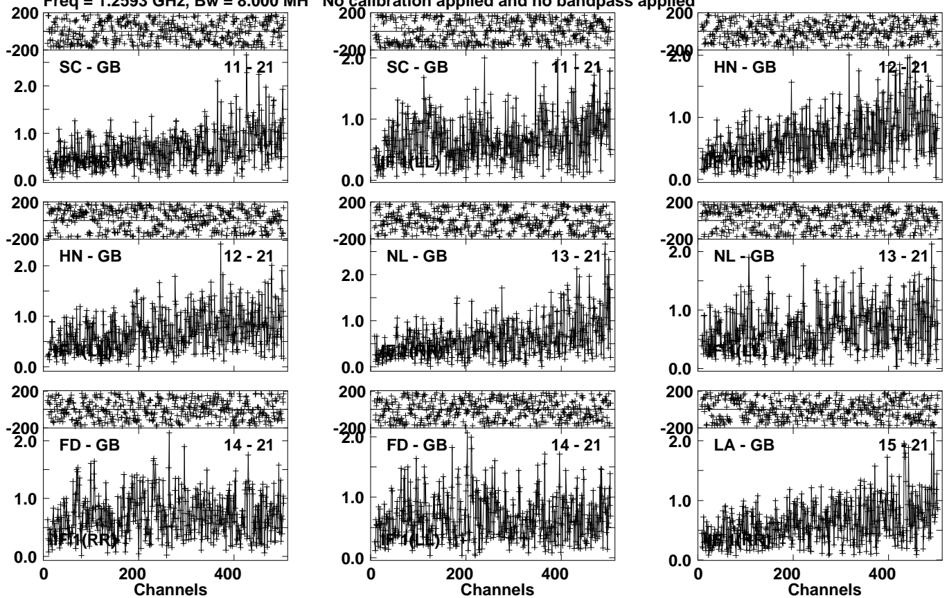
Lower frame: Milli Ampl Jy Top frame: Phas deg Vector averaged cross-power spectrum Several baselines displayed Timerange: 01/06:54:31 to 01/06:55:59
