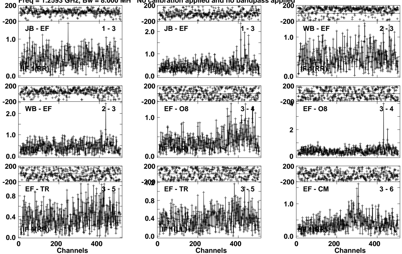
Lower frame: Milli Ampl Jy Top frame: Phas deg Vector averaged cross-power spectrum Several baselines displayed Timerange: 00/19:10:01 to 00/19:14:59
