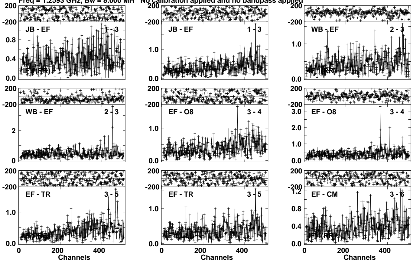
Lower frame: Milli Ampl Jy Top frame: Phas deg Vector averaged cross-power spectrum Several baselines displayed Timerange: 00/22:59:01 to 00/23:03:59
