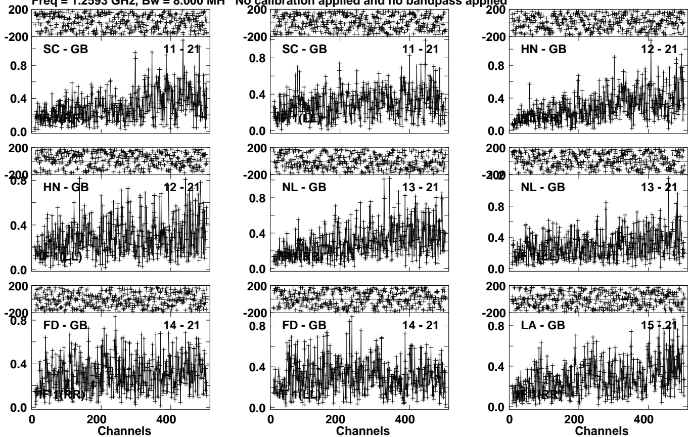
Lower frame: Milli Ampl Jy Top frame: Phas deg Vector averaged cross-power spectrum Several baselines displayed Timerange: 01/08:02:11 to 01/08:08:59
