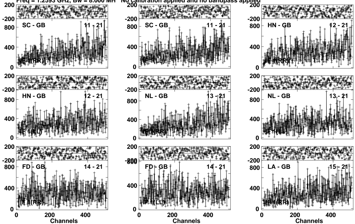
Lower frame: Micro Ampl Jy Top frame: Phas deg Vector averaged cross-power spectrum Several baselines displayed Timerange: 01/06:29:11 to 01/06:35:59
