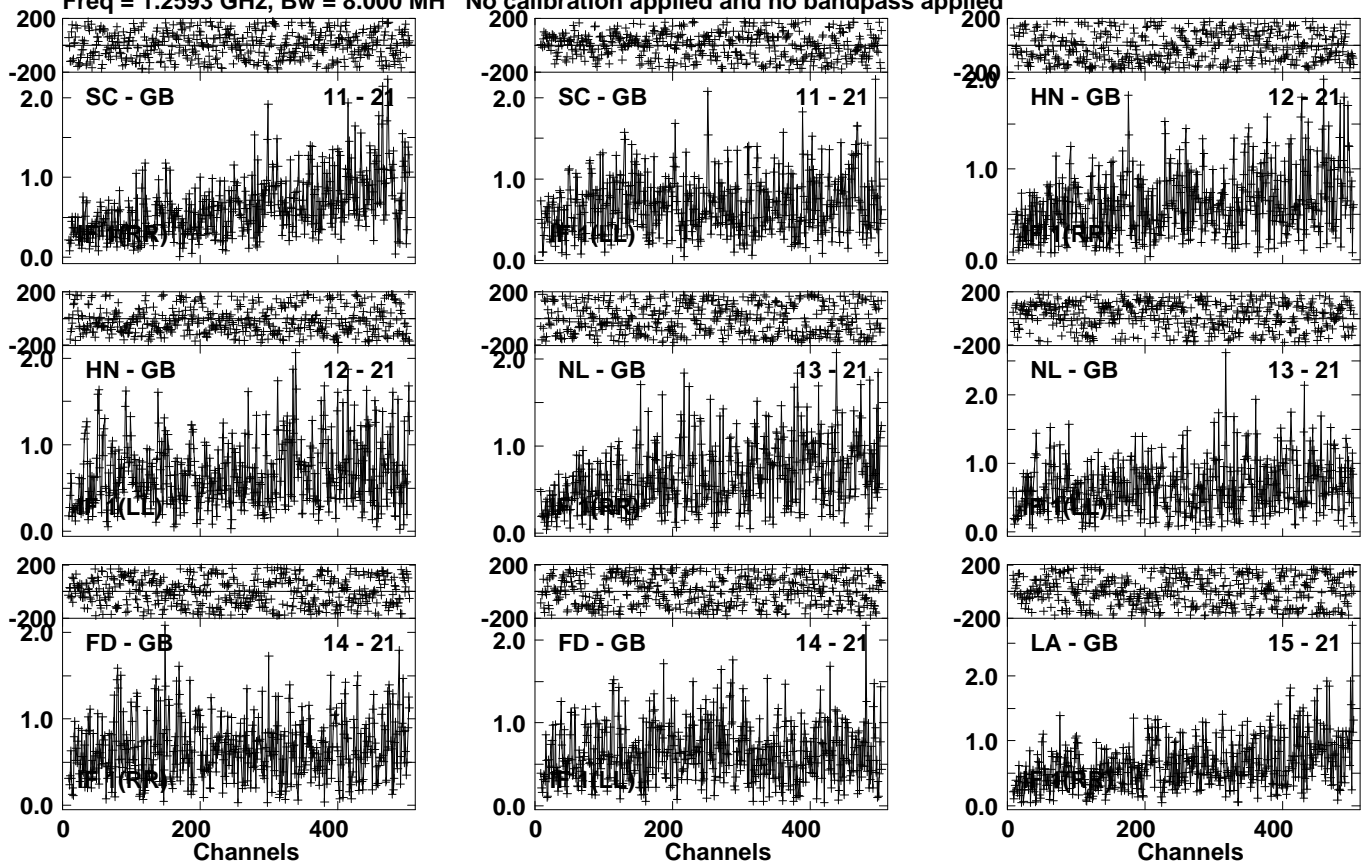
Lower frame: Milli Ampl Jy Top frame: Phas deg Vector averaged cross-power spectrum Several baselines displayed Timerange: 01/04:57:31 to 01/04:58:59
