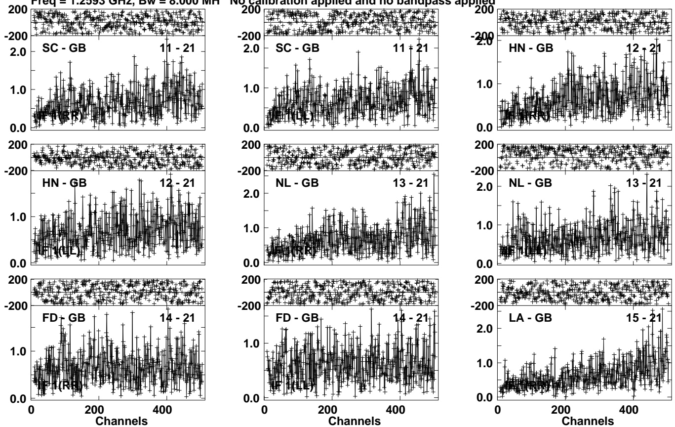
Lower frame: Milli Ampl Jy Top frame: Phas deg Vector averaged cross-power spectrum Several baselines displayed Timerange: 01/08:09:31 to 01/08:10:59
