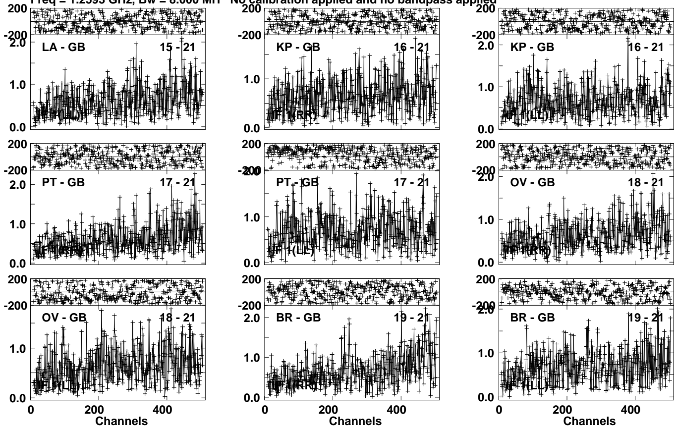
Lower frame: Milli Ampl Jy Top frame: Phas deg Vector averaged cross-power spectrum Several baselines displayed Timerange: 01/04:30:31 to 01/04:31:59
