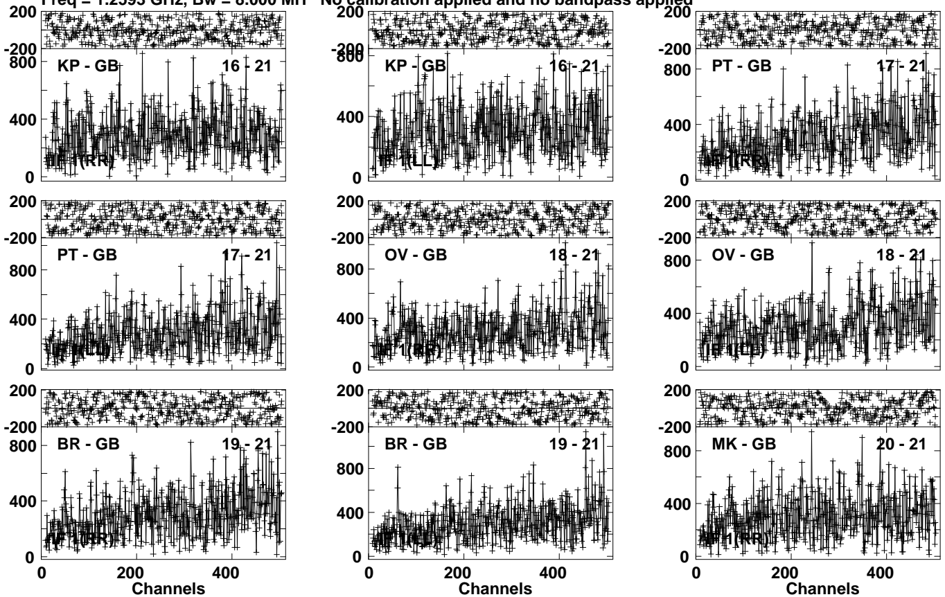
Lower frame: Micro Ampl Jy Top frame: Phas deg Vector averaged cross-power spectrum Several baselines displayed Timerange: 01/04:50:13 to 01/04:56:59
