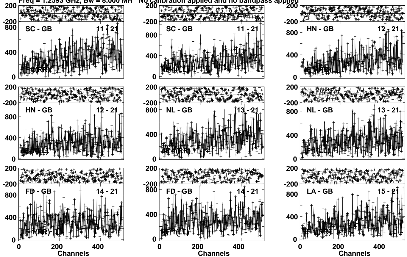
Lower frame: Micro Ampl Jy Top frame: Phas deg Vector averaged cross-power spectrum Several baselines displayed Timerange: 01/06:20:11 to 01/06:26:59
