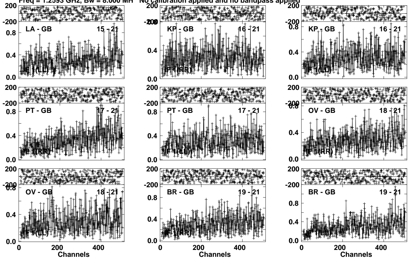
Lower frame: Milli Ampl Jy Top frame: Phas deg Vector averaged cross-power spectrum Several baselines displayed Timerange: 01/04:23:13 to 01/04:29:59
