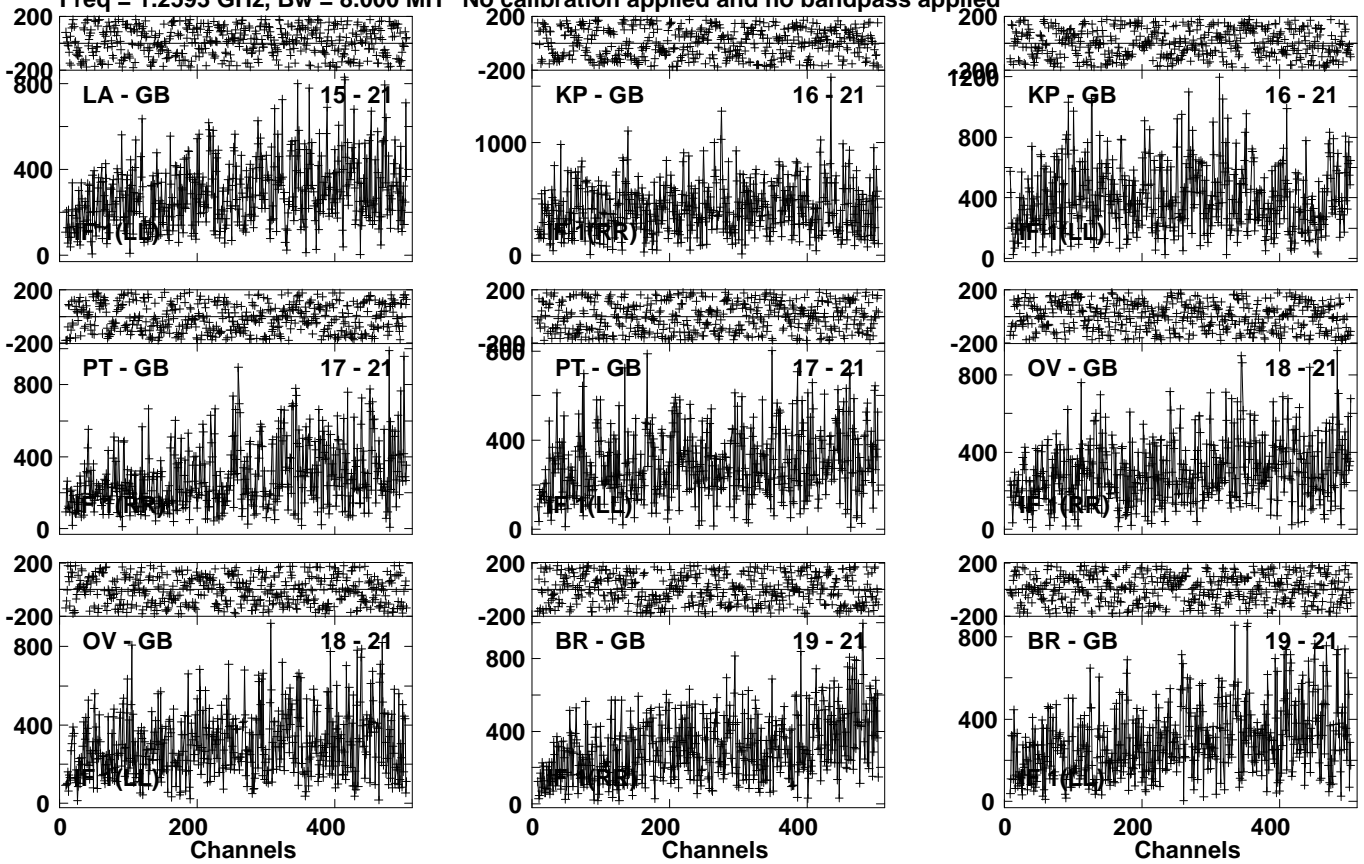
Lower frame: Micro Ampl Jy Top frame: Phas deg Vector averaged cross-power spectrum Several baselines displayed Timerange: 01/04:59:13 to 01/05:05:59
