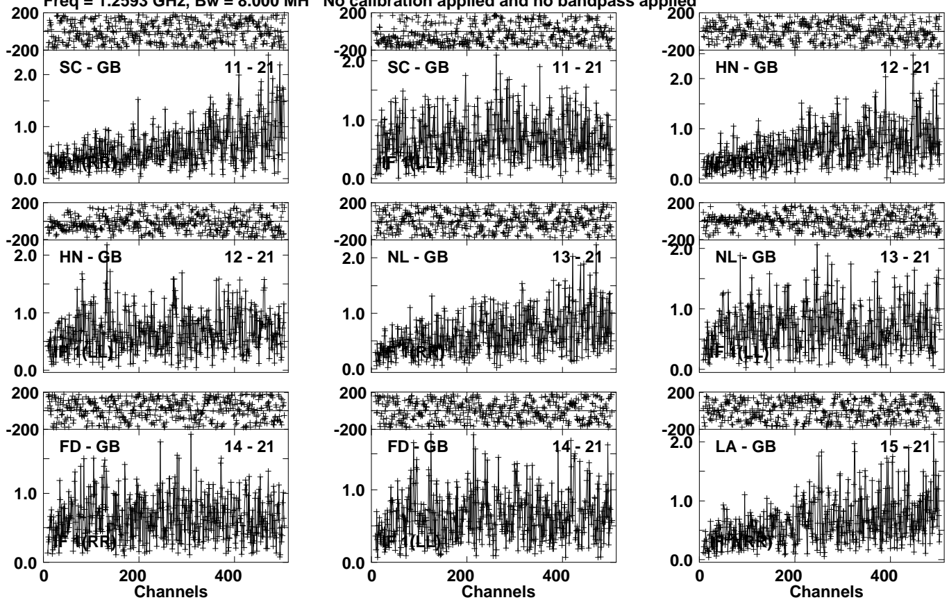
Lower frame: Milli Ampl Jy Top frame: Phas deg Vector averaged cross-power spectrum Several baselines displayed Timerange: 01/08:00:31 to 01/08:01:59
