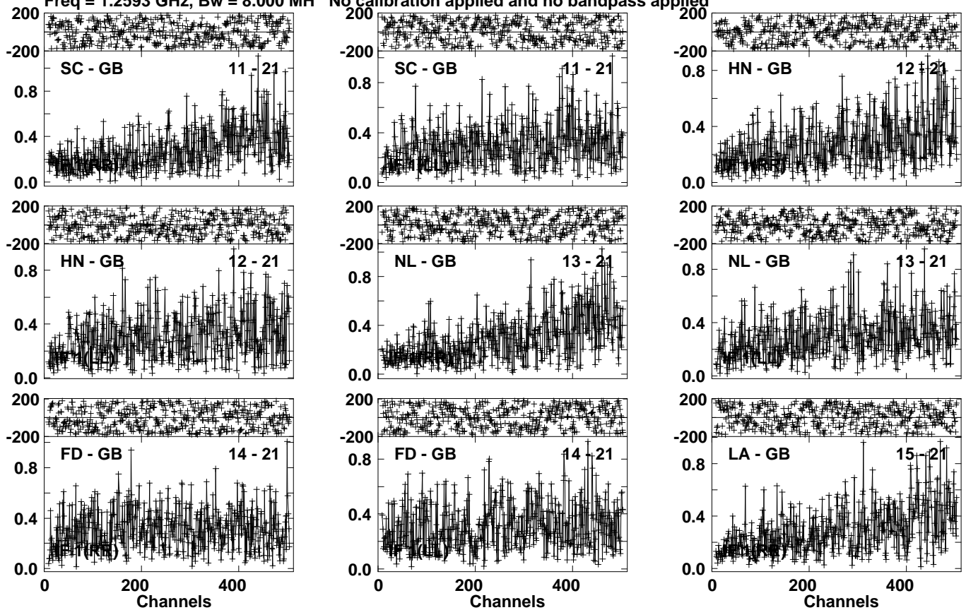
Lower frame: Milli Ampl Jy Top frame: Phas deg Vector averaged cross-power spectrum Several baselines displayed Timerange: 01/07:53:11 to 01/07:59:59
