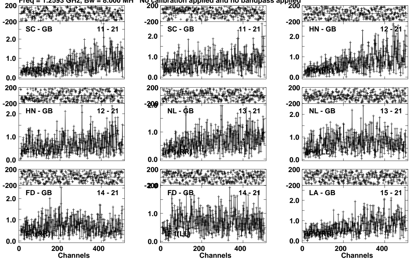
Lower frame: Milli Ampl Jy Top frame: Phas deg Vector averaged cross-power spectrum Several baselines displayed Timerange: 01/06:00:31 to 01/06:01:59
