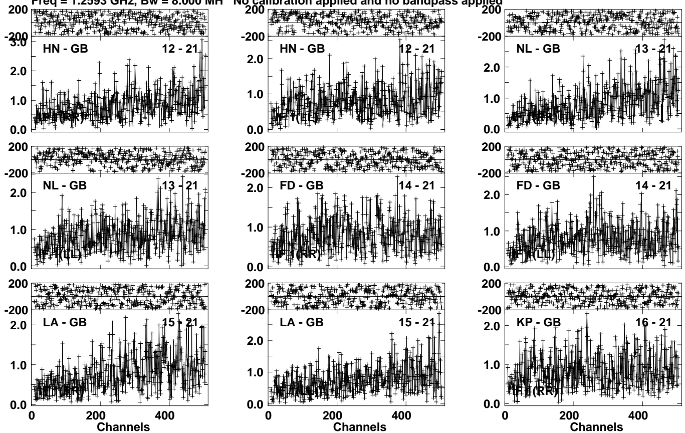
Lower frame: Milli Ampl Jy Top frame: Phas deg Vector averaged cross-power spectrum Several baselines displayed Timerange: 01/10:21:41 to 01/10:22:59
