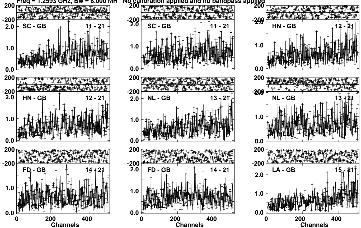
Lower frame: Milli Ampl Jy Top frame: Phas deg Vector averaged cross-power spectrum Several baselines displayed Timerange: 01/07:33:31 to 01/07:34:59
