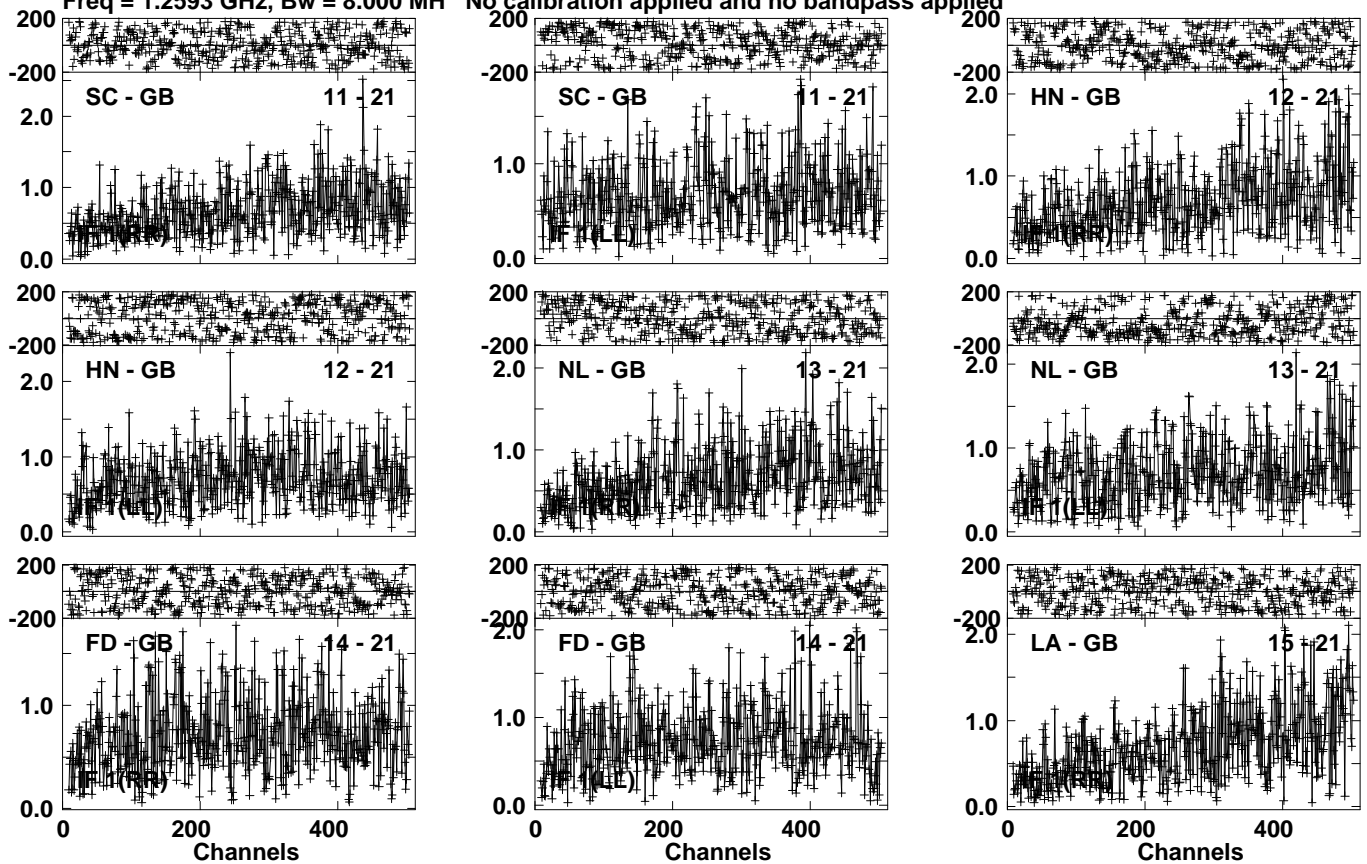
Lower frame: Milli Ampl Jy Top frame: Phas deg Vector averaged cross-power spectrum Several baselines displayed Timerange: 01/05:51:31 to 01/05:52:59
