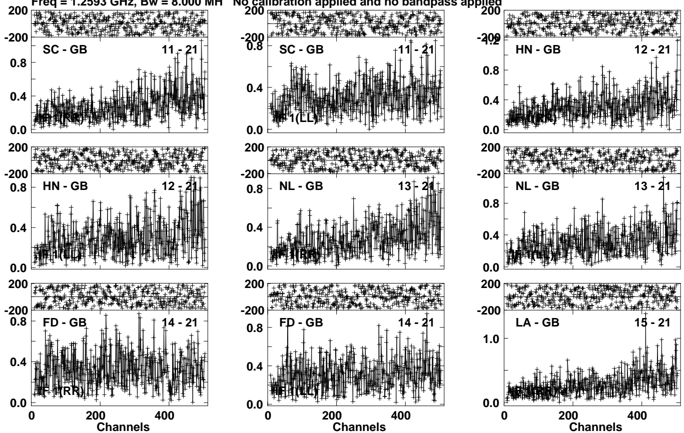
Lower frame: Milli Ampl Jy Top frame: Phas deg Vector averaged cross-power spectrum Several baselines displayed Timerange: 01/09:14:11 to 01/09:20:59
