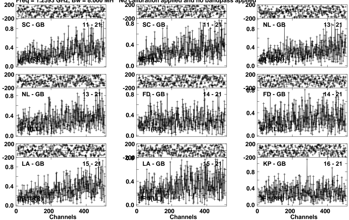
Lower frame: Milli Ampl Jy Top frame: Phas deg Vector averaged cross-power spectrum Several baselines displayed Timerange: 01/05:35:13 to 01/05:41:59
