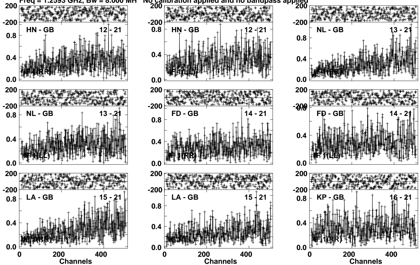
Lower frame: Milli Ampl Jy Top frame: Phas deg Vector averaged cross-power spectrum Several baselines displayed Timerange: 01/10:08:11 to 01/10:14:59
