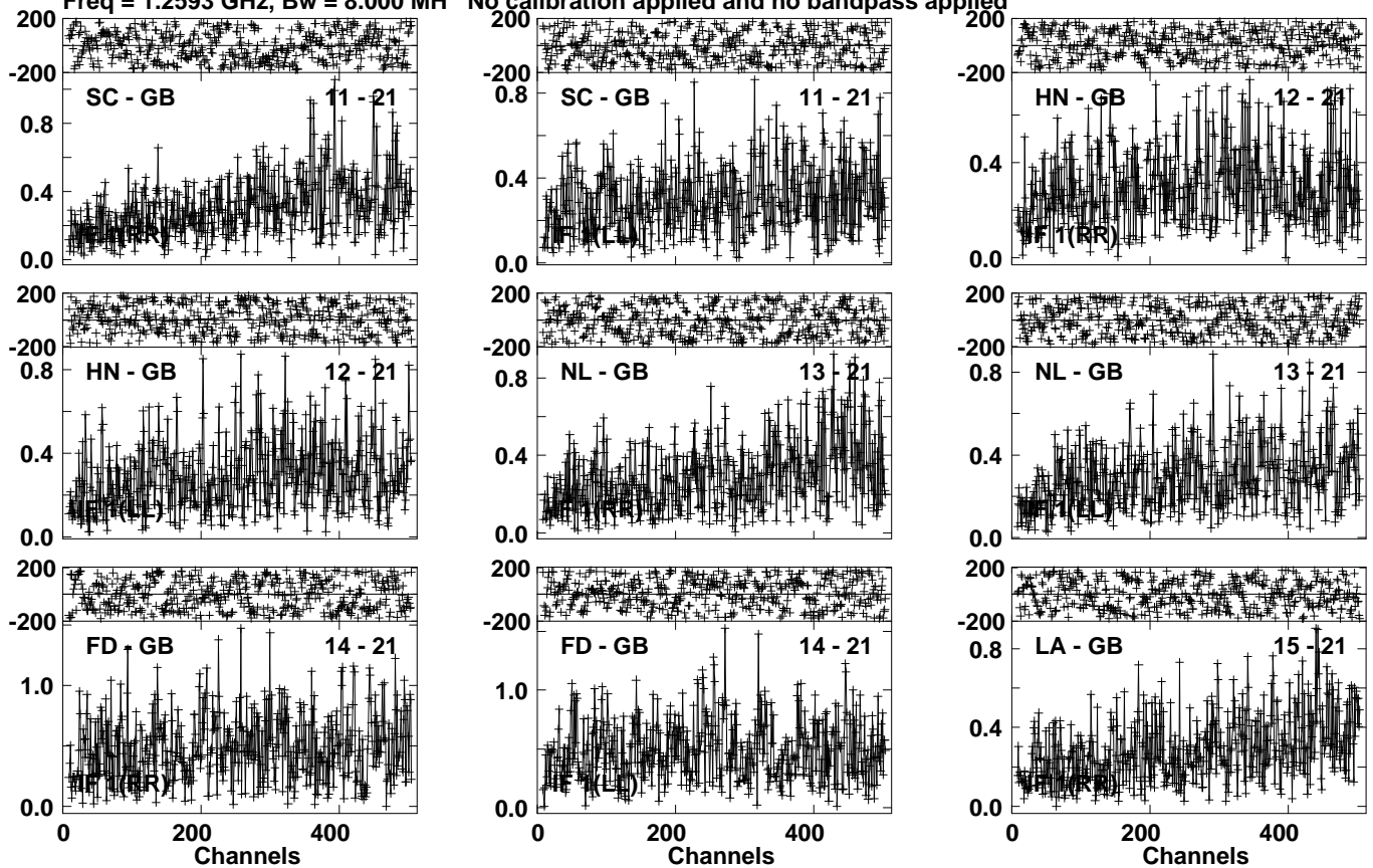
Lower frame: Milli Ampl Jy Top frame: Phas deg Vector averaged cross-power spectrum Several baselines displayed Timerange: 01/04:41:13 to 01/04:47:59
