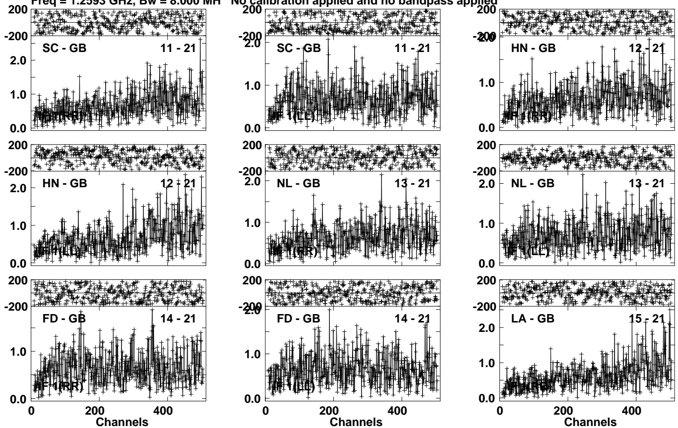
Lower frame: Milli Ampl Jy Top frame: Phas deg Vector averaged cross-power spectrum Several baselines displayed Timerange: 01/08:18:31 to 01/08:19:59
