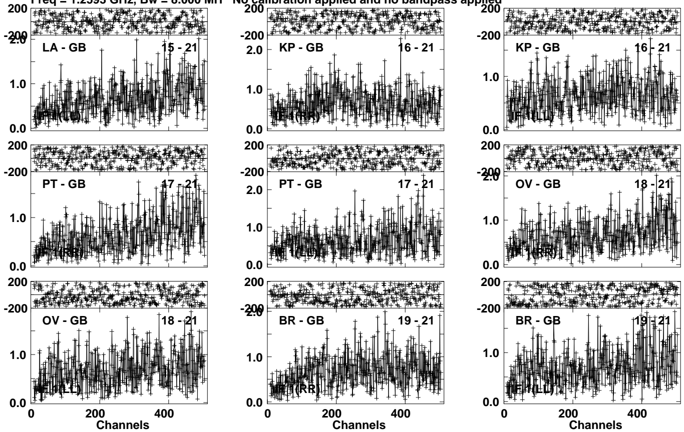
Lower frame: Milli Ampl Jy Top frame: Phas deg Vector averaged cross-power spectrum Several baselines displayed Timerange: 01/09:57:31 to 01/09:58:59
