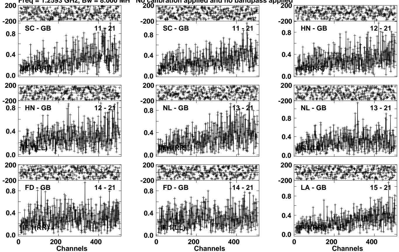
Lower frame: Milli Ampl Jy Top frame: Phas deg Vector averaged cross-power spectrum Several baselines displayed Timerange: 01/08:20:11 to 01/08:26:59
