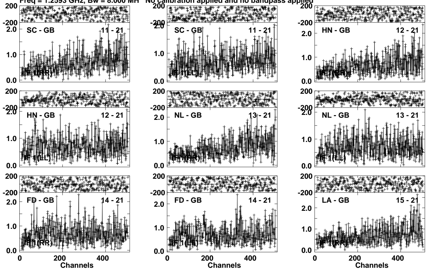
Lower frame: Milli Ampl Jy Top frame: Phas deg Vector averaged cross-power spectrum Several baselines displayed Timerange: 01/06:09:31 to 01/06:10:59
