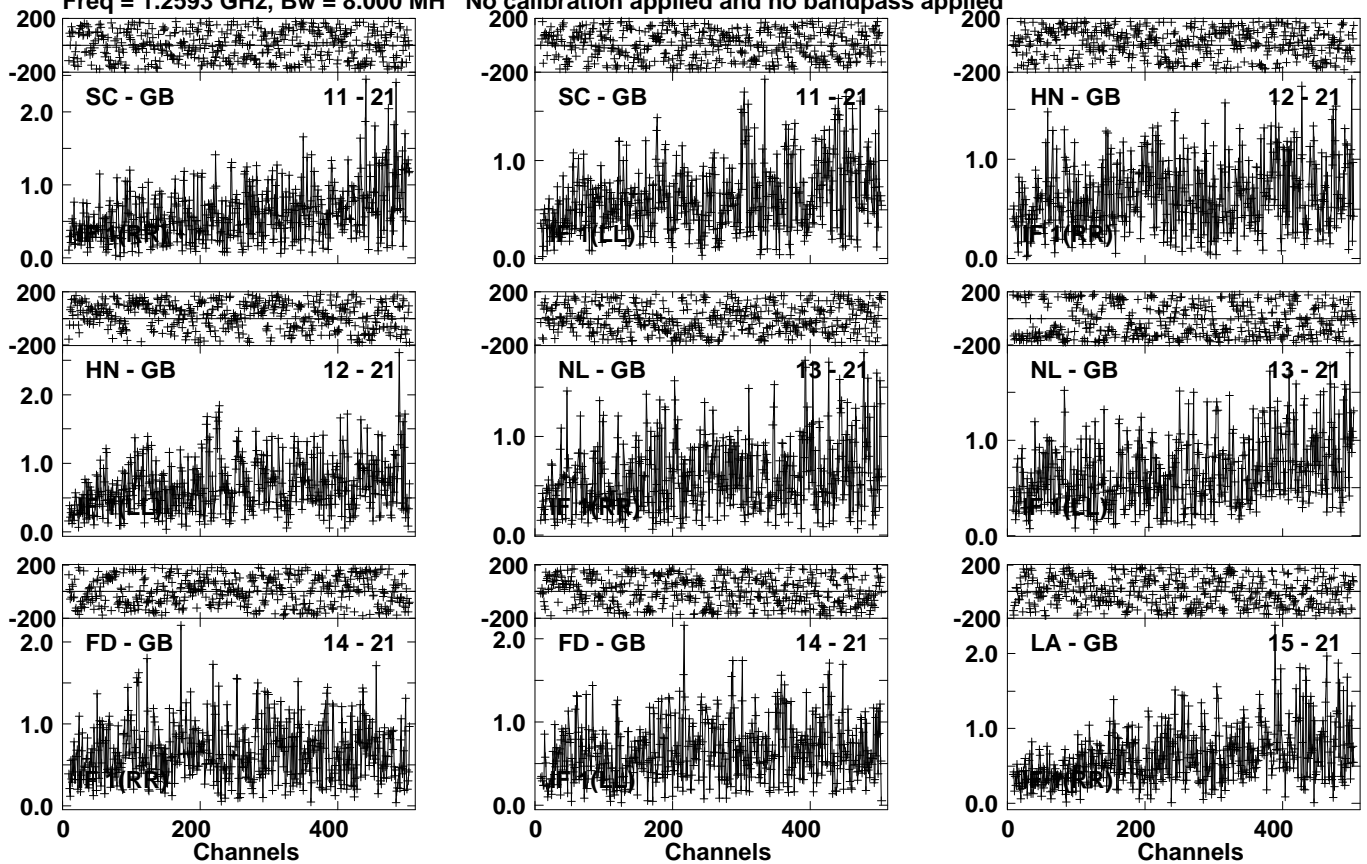
Lower frame: Milli Ampl Jy Top frame: Phas deg Vector averaged cross-power spectrum Several baselines displayed Timerange: 01/10:06:31 to 01/10:07:59
