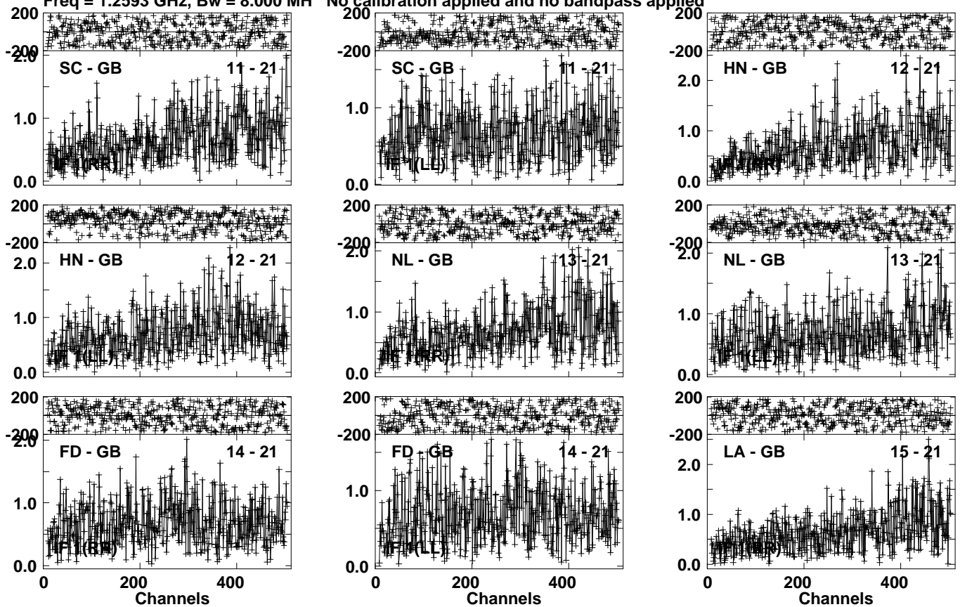
Lower frame: Milli Ampl Jy Top frame: Phas deg Vector averaged cross-power spectrum Several baselines displayed Timerange: 01/07:42:31 to 01/07:43:59
