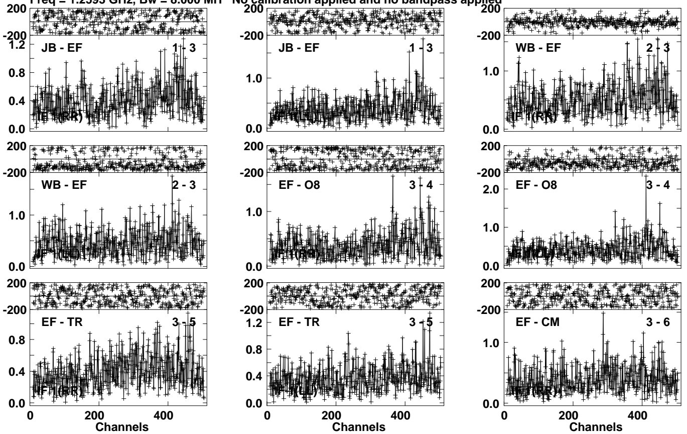
Lower frame: Milli Ampl Jy Top frame: Phas deg Vector averaged cross-power spectrum Several baselines displayed Timerange: 00/23:13:01 to 00/23:17:59
