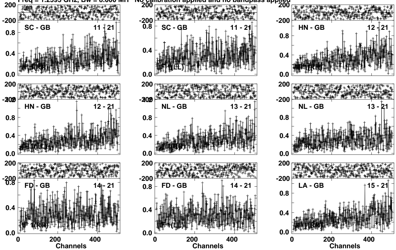
Lower frame: Milli Ampl Jy Top frame: Phas deg Vector averaged cross-power spectrum Several baselines displayed Timerange: 01/09:05:11 to 01/09:11:59
