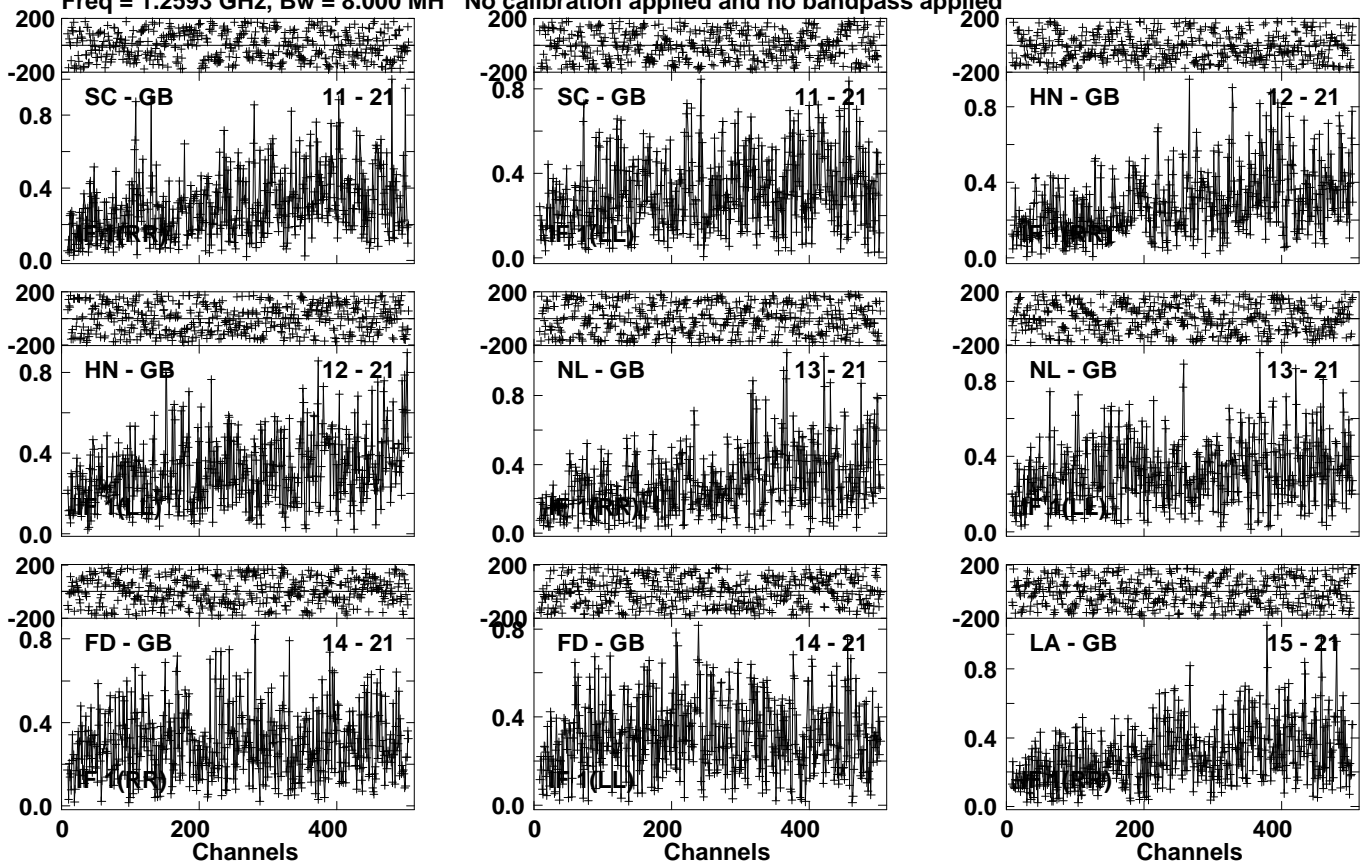
Lower frame: Milli Ampl Jy Top frame: Phas deg Vector averaged cross-power spectrum Several baselines displayed Timerange: 01/05:17:13 to 01/05:23:59
