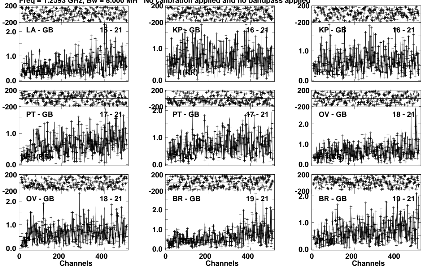
Lower frame: Milli Ampl Jy Top frame: Phas deg Vector averaged cross-power spectrum Several baselines displayed Timerange: 01/04:12:31 to 01/04:13:59
