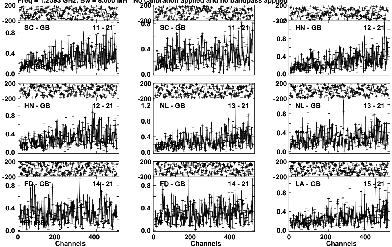
Lower frame: Milli Ampl Jy Top frame: Phas deg Vector averaged cross-power spectrum Several baselines displayed Timerange: 01/07:35:11 to 01/07:41:59
