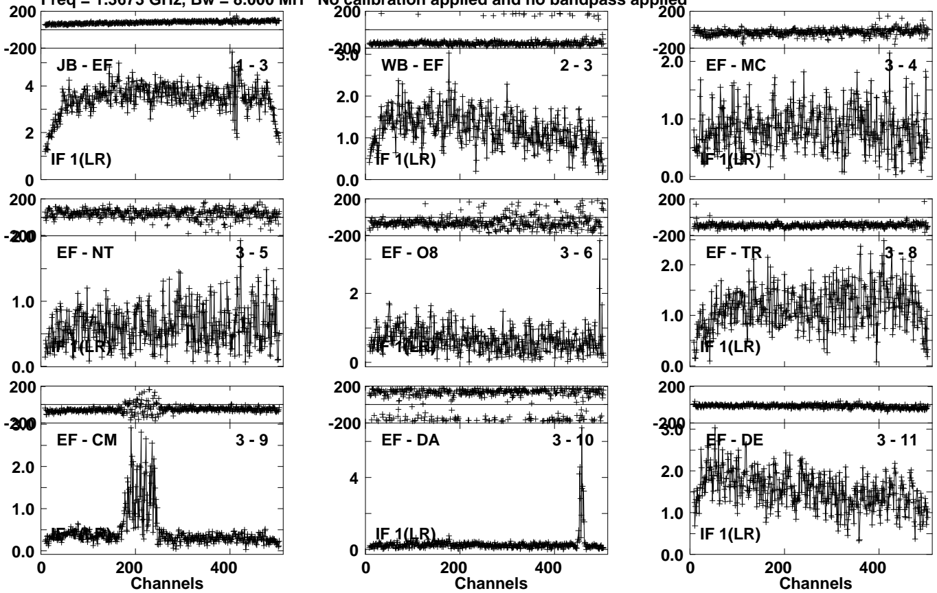
Lower frame: Milli Ampl Jy Top frame: Phas deg Vector averaged cross-power spectrum Several baselines displayed Timerange: 00/10:30:01 to 00/10:35:59
