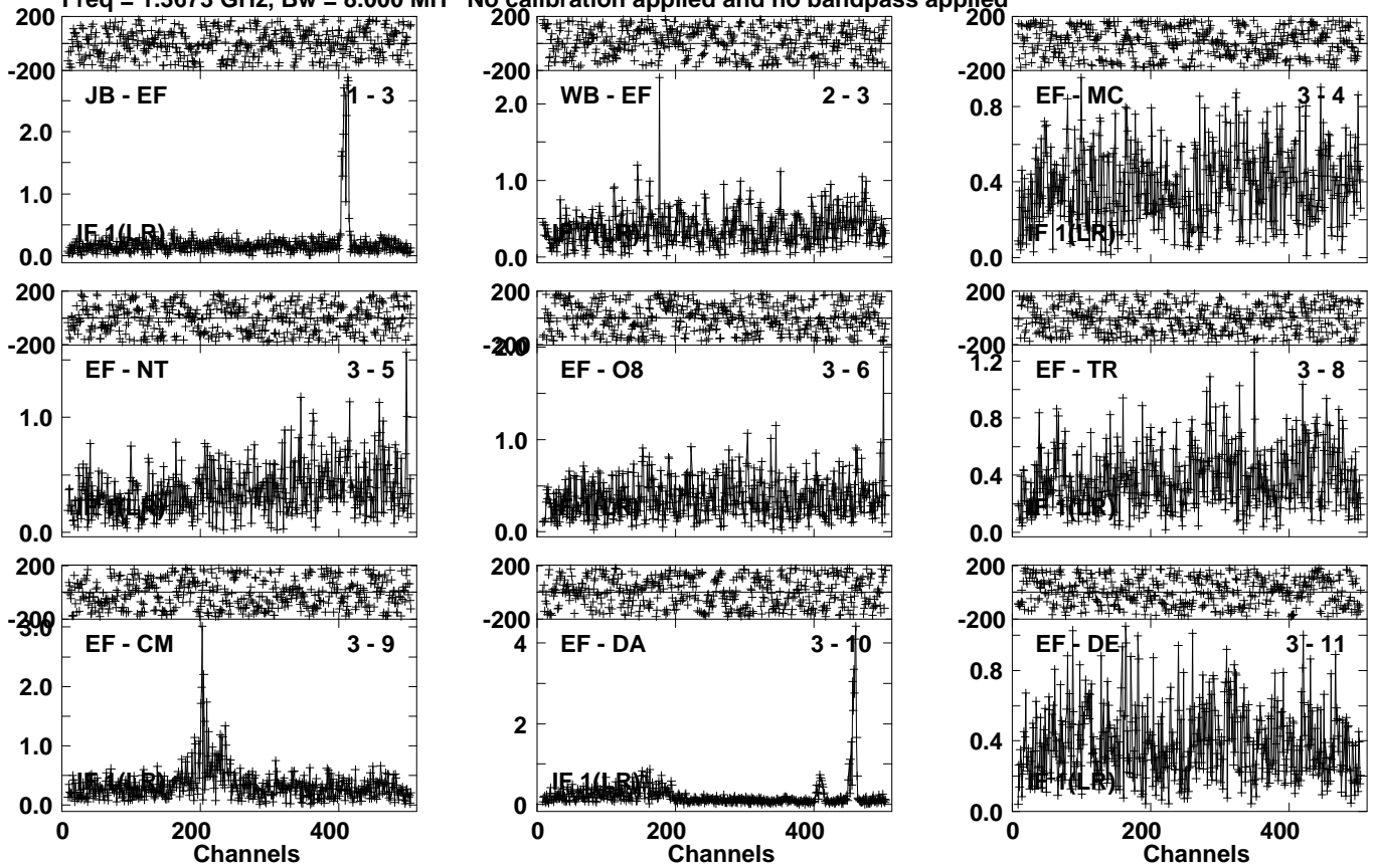
Lower frame: Milli Ampl Jy Top frame: Phas deg Vector averaged cross-power spectrum Several baselines displayed Timerange: 00/06:55:01 to 00/06:59:59
