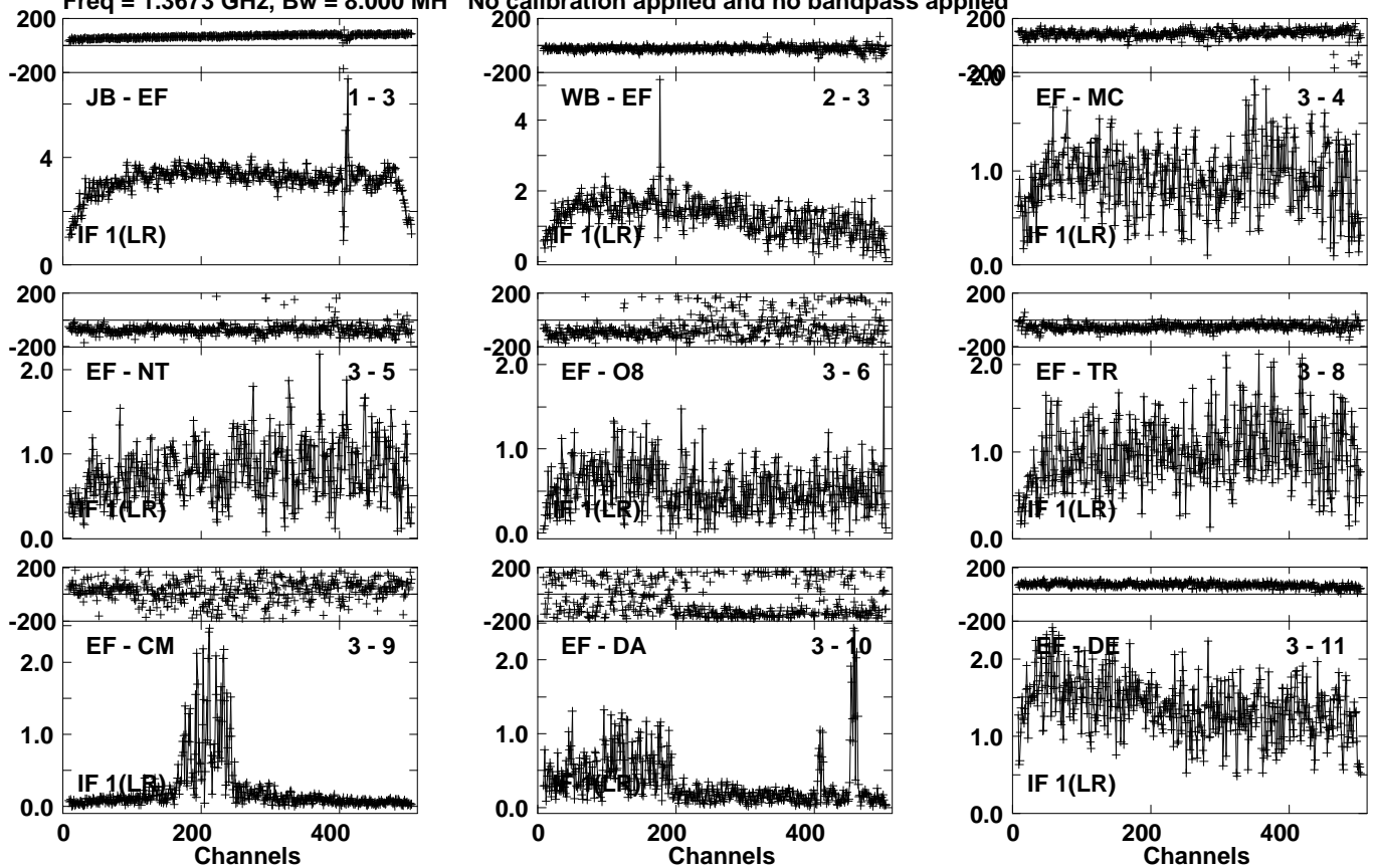
Lower frame: Milli Ampl Jy Top frame: Phas deg Vector averaged cross-power spectrum Several baselines displayed Timerange: 00/08:33:01 to 00/08:39:59
