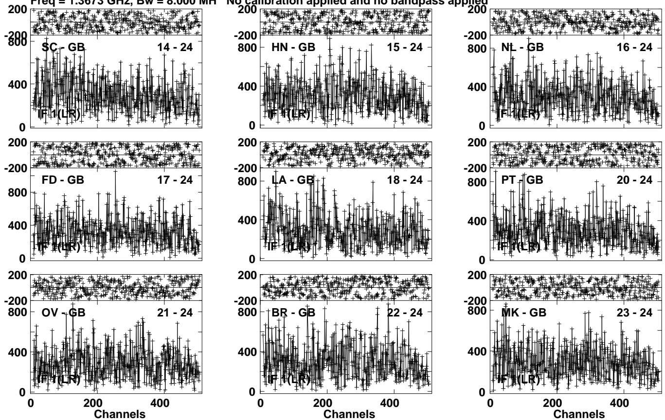
Lower frame: Micro Ampl Jy Top frame: Phas deg Vector averaged cross-power spectrum Several baselines displayed Timerange: 00/13:47:11 to 00/13:53:59
