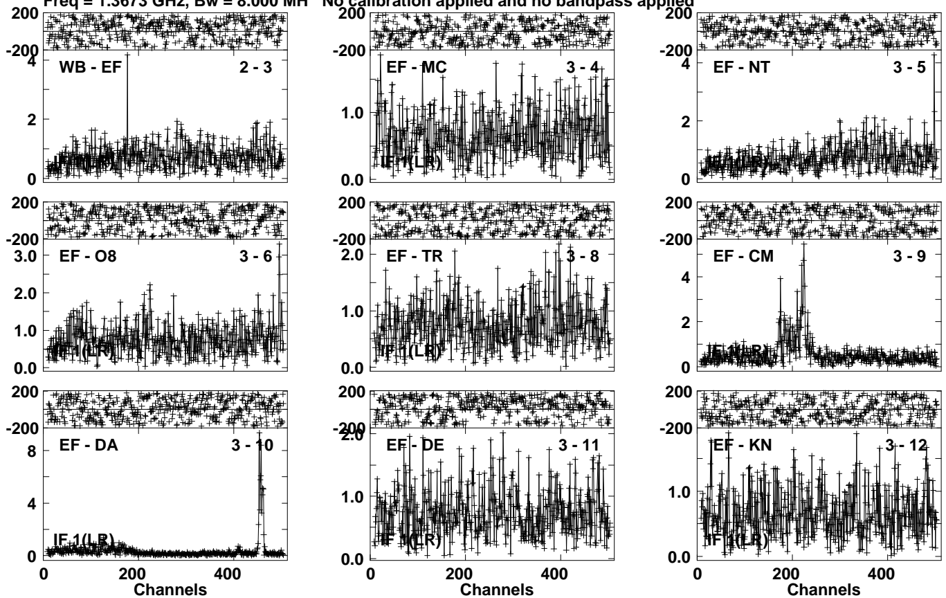
Lower frame: Milli Ampl Jy Top frame: Phas deg Vector averaged cross-power spectrum Several baselines displayed Timerange: 00/09:55:11 to 00/09:56:39
