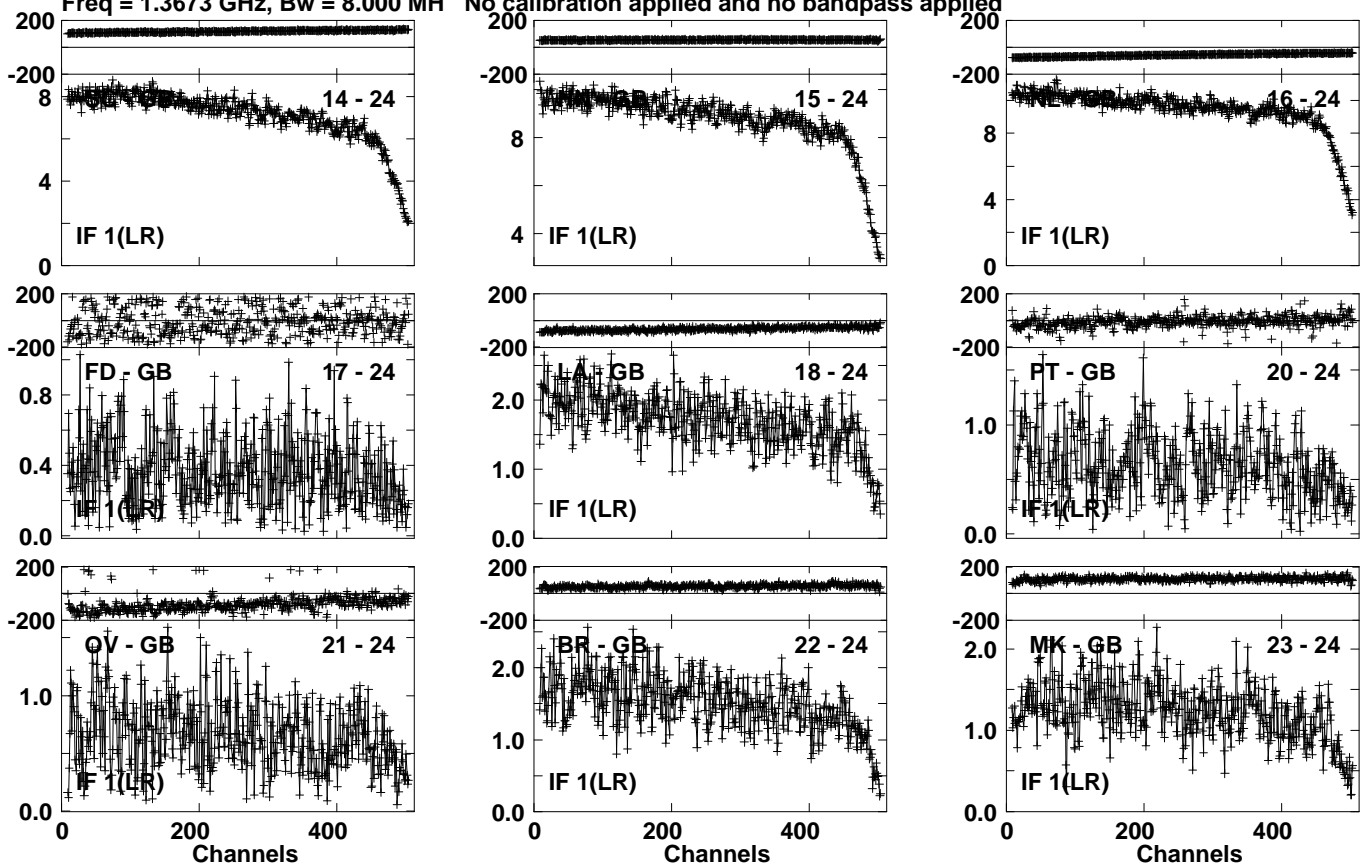
Lower frame: Milli Ampl Jy Top frame: Phas deg Vector averaged cross-power spectrum Several baselines displayed Timerange: 00/18:55:01 to 00/18:59:59
