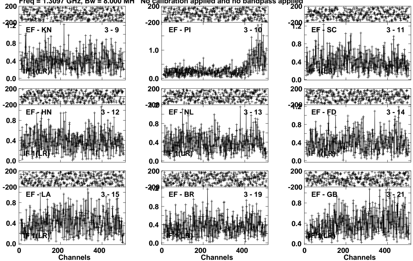
Lower frame: Milli Ampl Jy Top frame: Phas deg Vector averaged cross-power spectrum Several baselines displayed Timerange: 00/09:47:01 to 00/09:51:59
