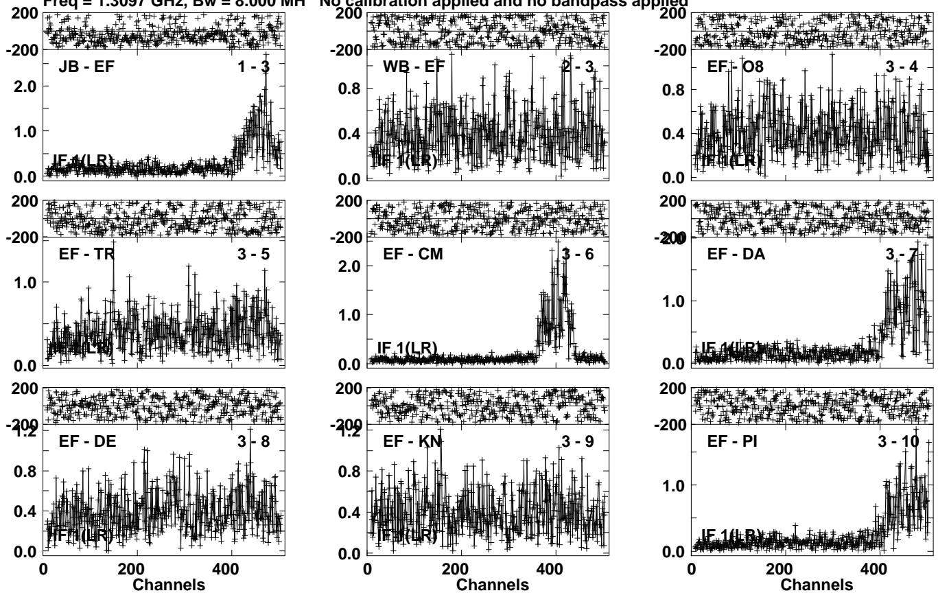
Lower frame: Milli Ampl Jy Top frame: Phas deg Vector averaged cross-power spectrum Several baselines displayed Timerange: 00/05:45:01 to 00/05:49:59
