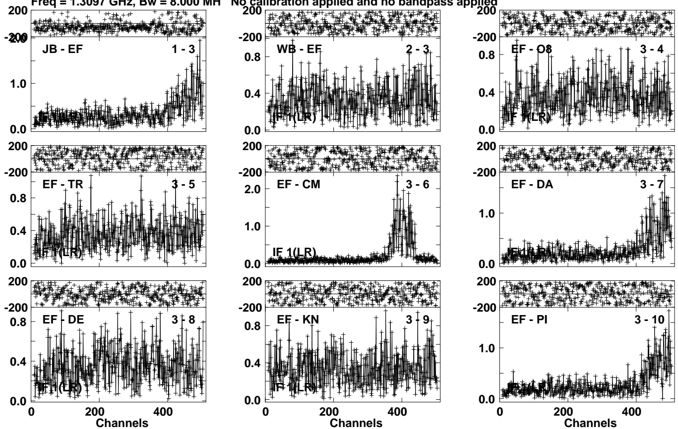
Lower frame: Milli Ampl Jy Top frame: Phas deg Vector averaged cross-power spectrum Several baselines displayed Timerange: 00/08:52:01 to 00/08:57:59
