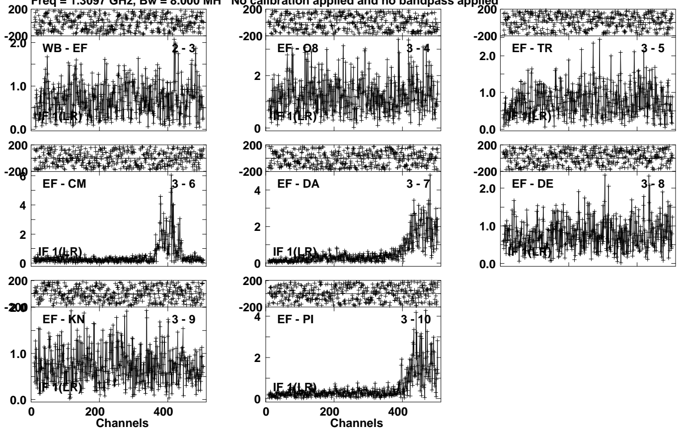
Lower frame: Milli Ampl Jy Top frame: Phas deg Vector averaged cross-power spectrum Several baselines displayed Timerange: 00/02:50:31 to 00/02:51:59
