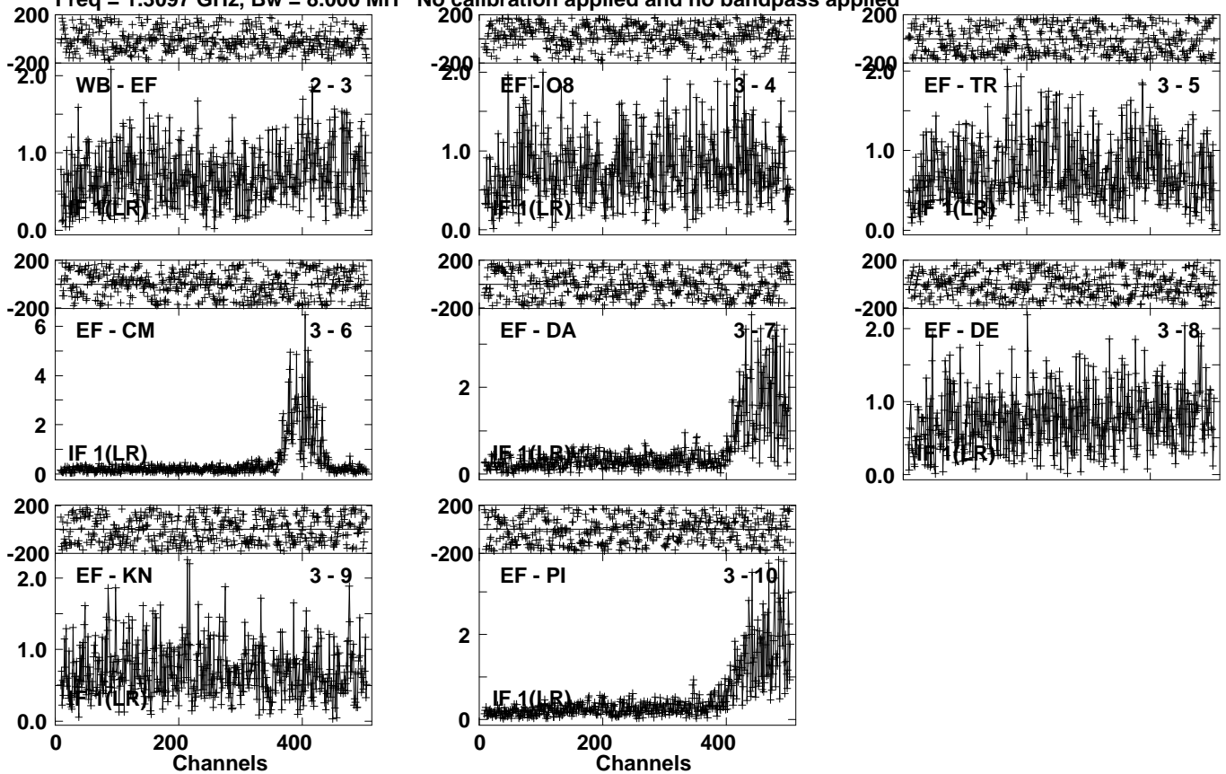
Lower frame: Milli Ampl Jy Top frame: Phas deg Vector averaged cross-power spectrum Several baselines displayed Timerange: 00/07:40:31 to 00/07:41:59
