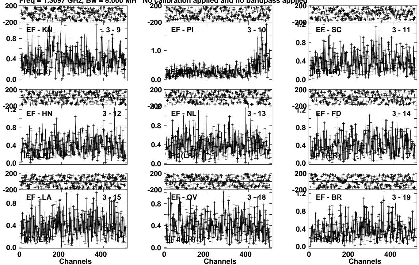
Lower frame: Milli Ampl Jy Top frame: Phas deg Vector averaged cross-power spectrum Several baselines displayed Timerange: 00/10:57:01 to 00/11:01:59
