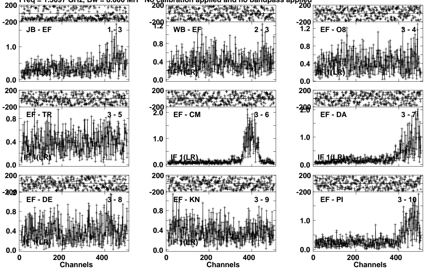
Lower frame: Milli Ampl Jy Top frame: Phas deg Vector averaged cross-power spectrum Several baselines displayed Timerange: 00/02:24:01 to 00/02:28:59
