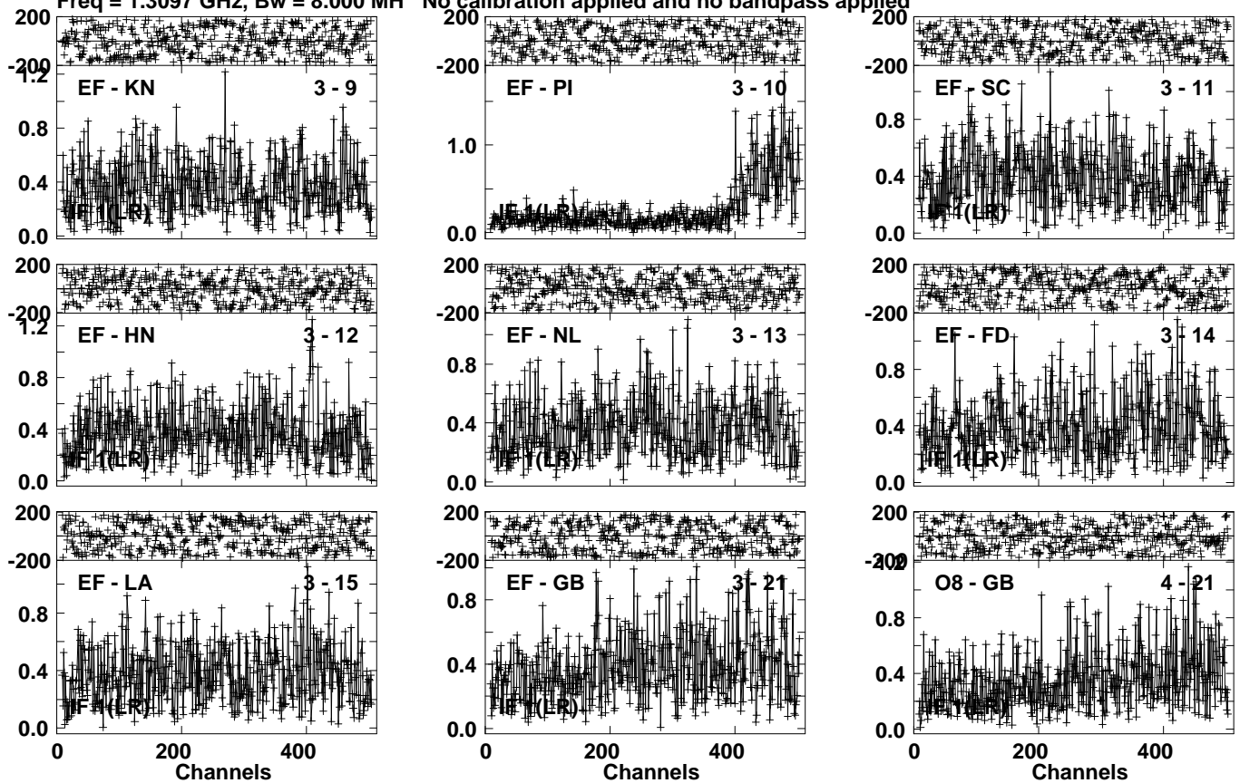
Lower frame: Milli Ampl Jy Top frame: Phas deg Vector averaged cross-power spectrum Several baselines displayed Timerange: 00/09:40:01 to 00/09:44:59
