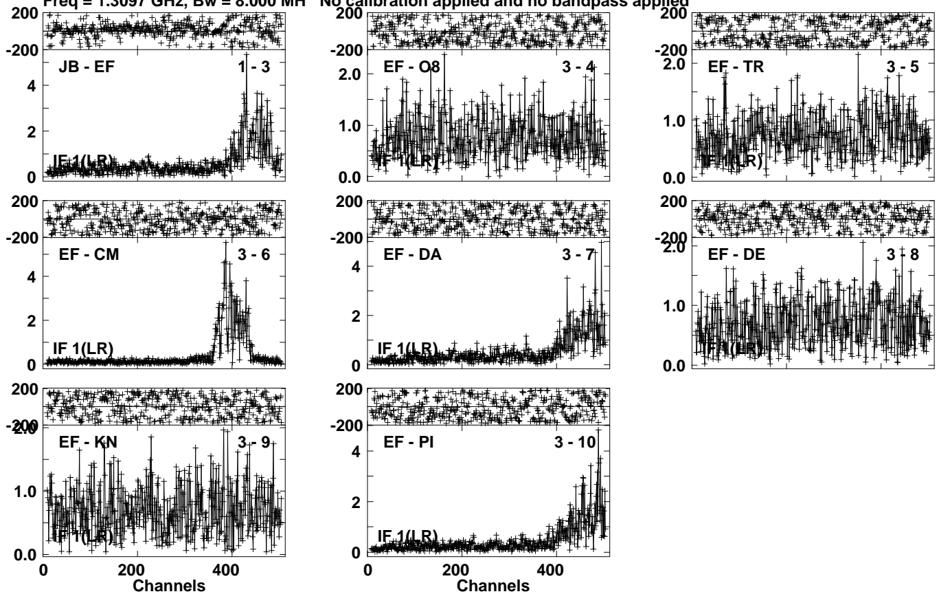
Lower frame: Milli Ampl Jy Top frame: Phas deg Vector averaged cross-power spectrum Several baselines displayed Timerange: 00/06:51:01 to 00/06:52:59
