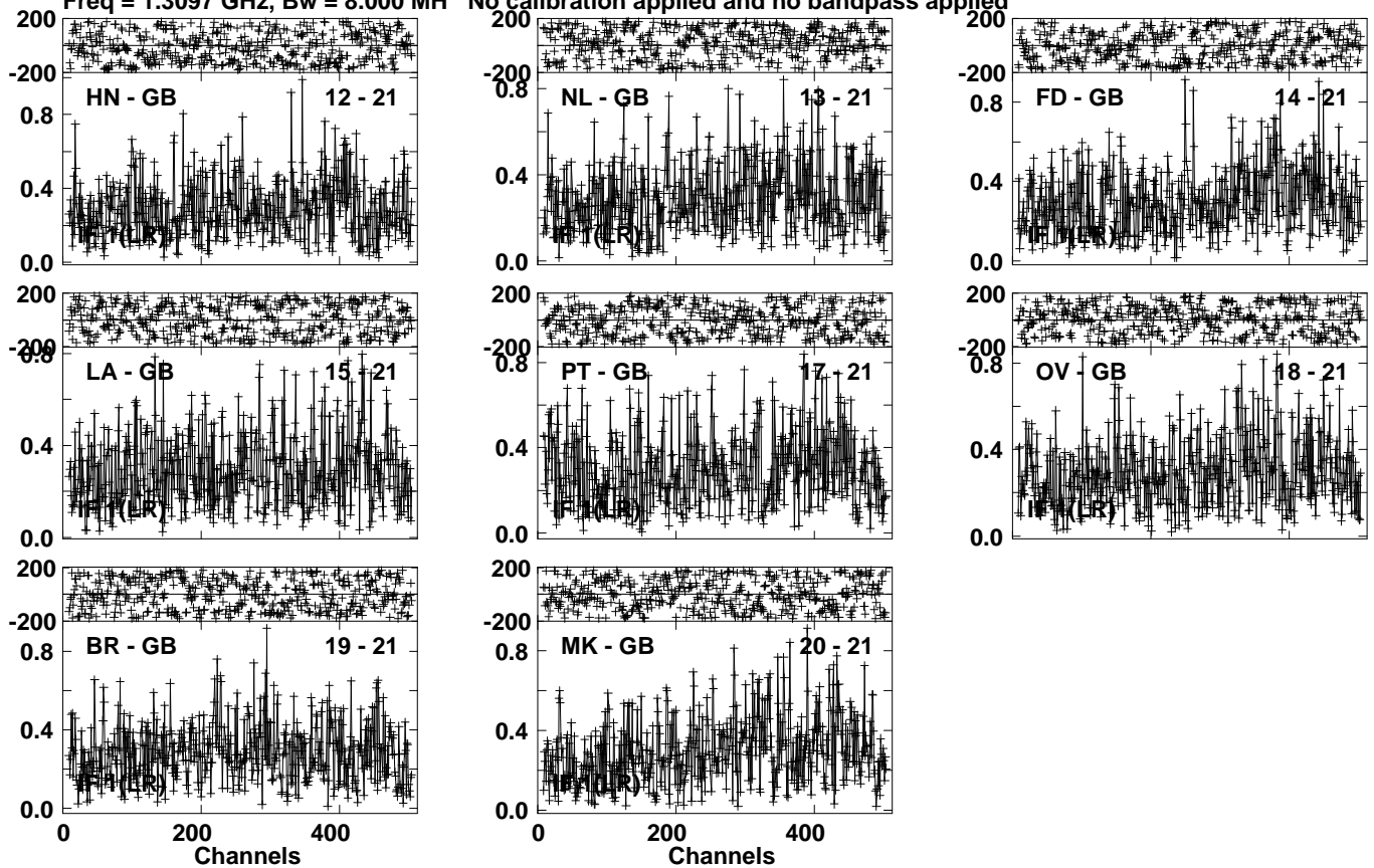
Lower frame: Milli Ampl Jy Top frame: Phas deg Vector averaged cross-power spectrum Several baselines displayed Timerange: 00/18:39:11 to 00/18:45:59
