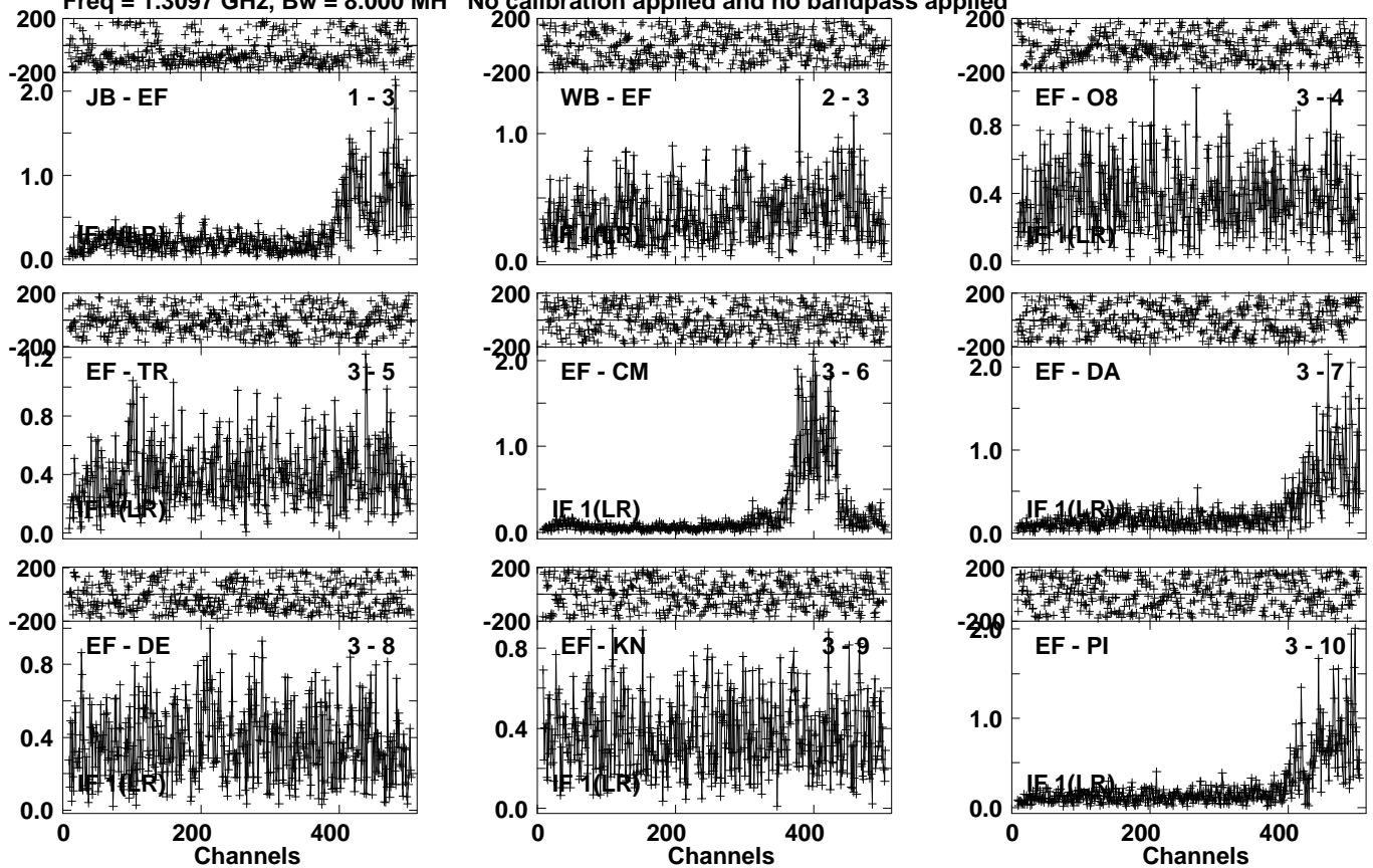
Lower frame: Milli Ampl Jy Top frame: Phas deg Vector averaged cross-power spectrum Several baselines displayed Timerange: 00/04:02:01 to 00/04:06:59
