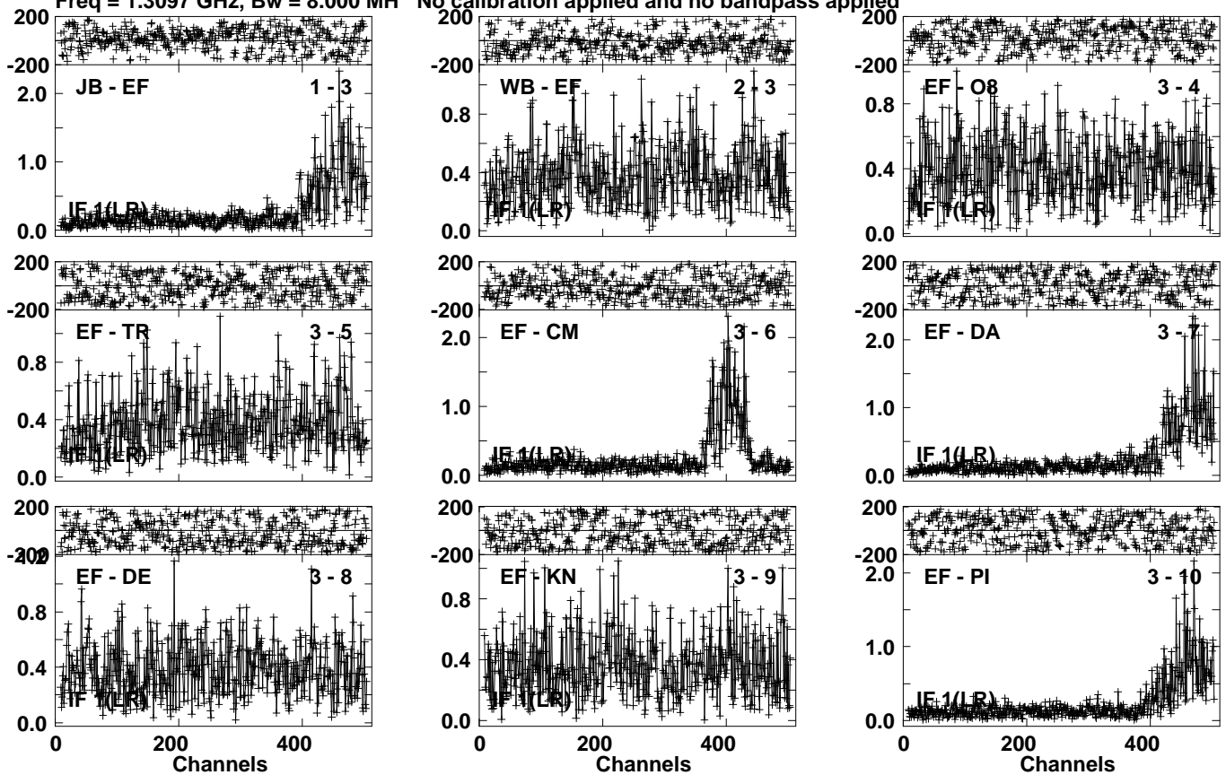
Lower frame: Milli Ampl Jy Top frame: Phas deg Vector averaged cross-power spectrum Several baselines displayed Timerange: 00/07:07:01 to 00/07:11:59
