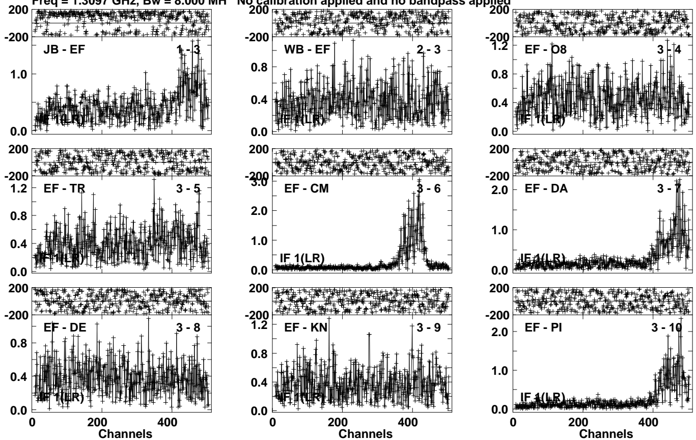
Lower frame: Milli Ampl Jy Top frame: Phas deg Vector averaged cross-power spectrum Several baselines displayed Timerange: 00/03:20:01 to 00/03:24:59
