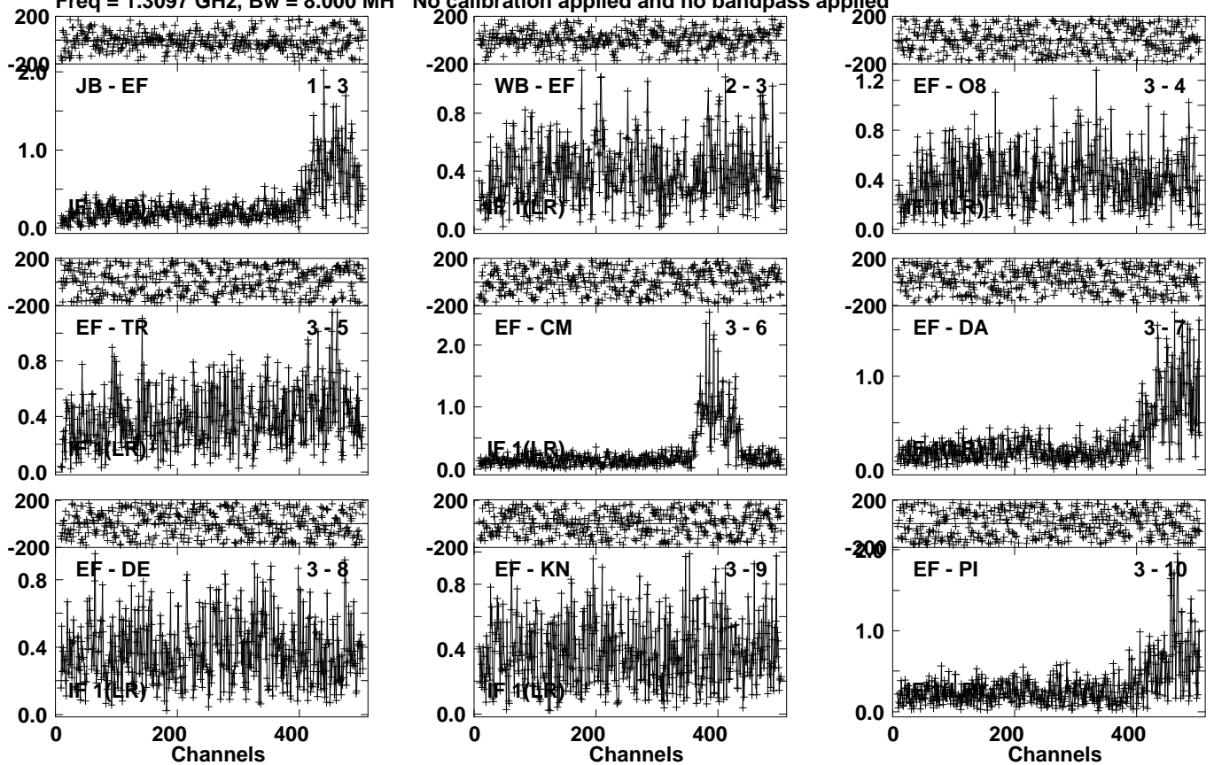
Lower frame: Milli Ampl Jy Top frame: Phas deg Vector averaged cross-power spectrum Several baselines displayed Timerange: 00/07:28:01 to 00/07:32:59
