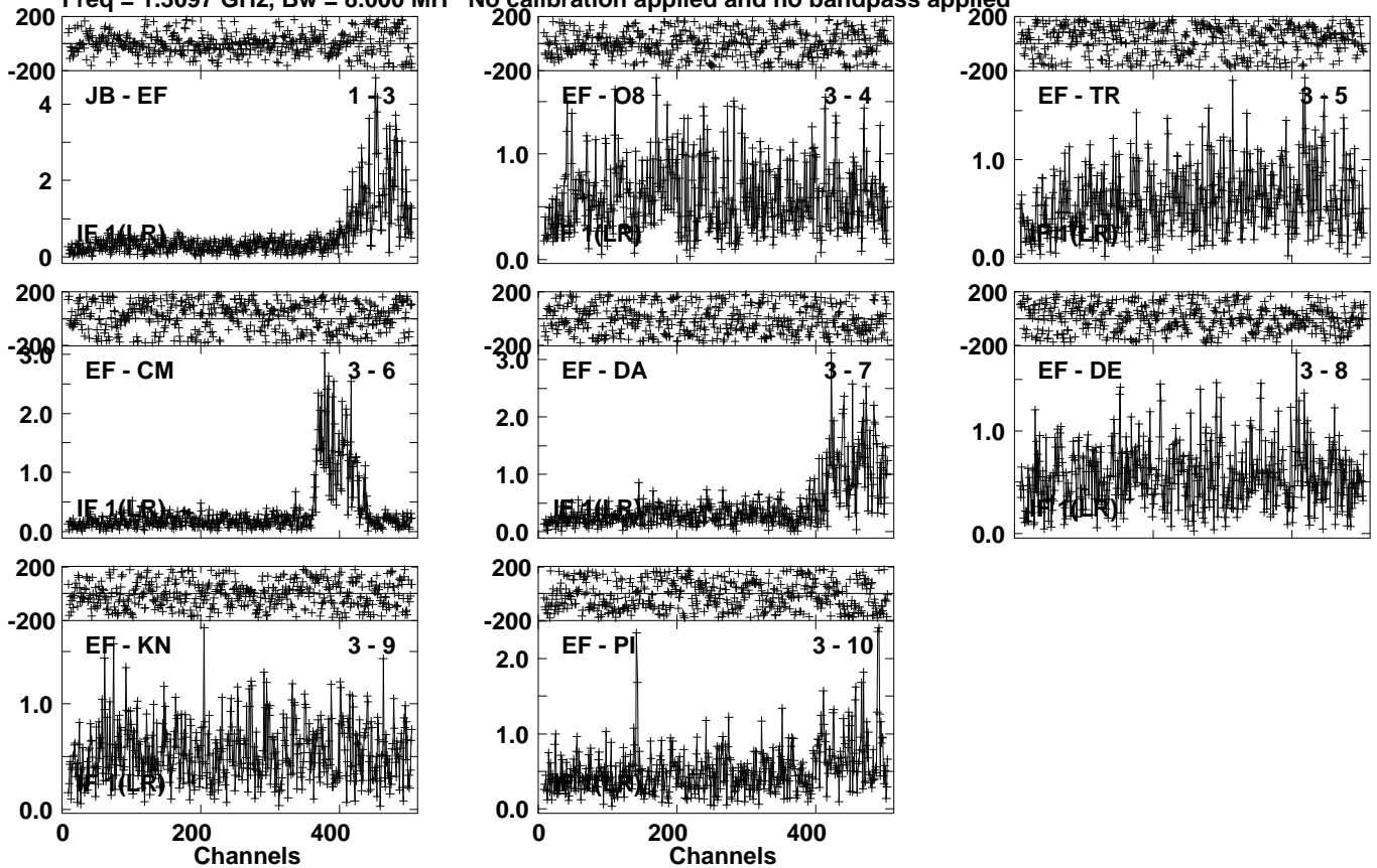
Lower frame: Milli Ampl Jy Top frame: Phas deg Vector averaged cross-power spectrum Several baselines displayed Timerange: 00/06:42:01 to 00/06:45:59
