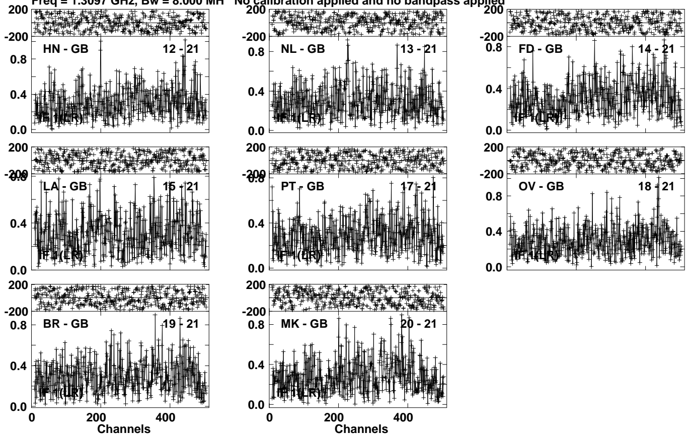
Lower frame: Milli Ampl Jy Top frame: Phas deg Vector averaged cross-power spectrum Several baselines displayed Timerange: 00/18:21:11 to 00/18:27:59
