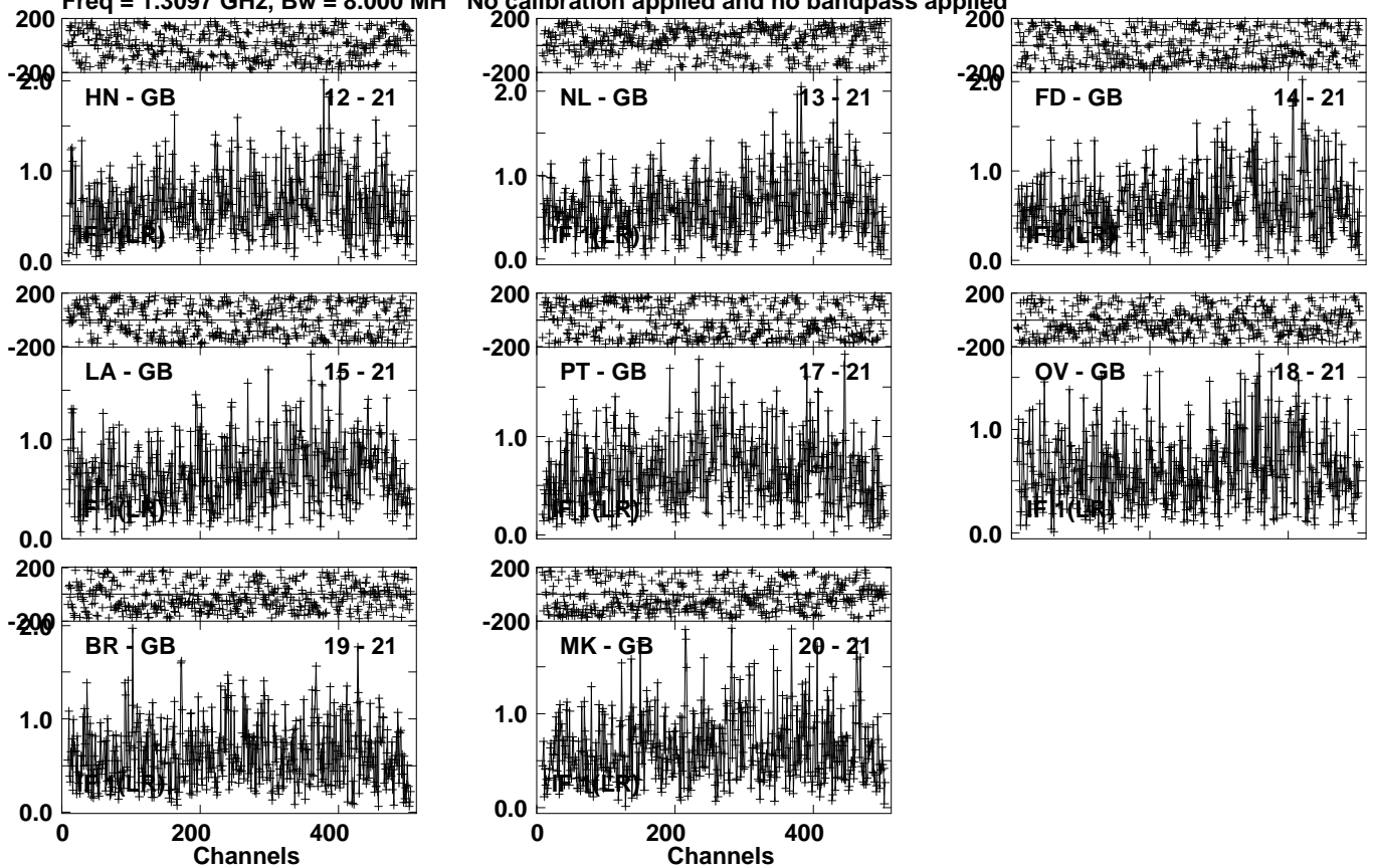
Lower frame: Milli Ampl Jy Top frame: Phas deg Vector averaged cross-power spectrum Several baselines displayed Timerange: 00/18:55:31 to 00/18:56:59
