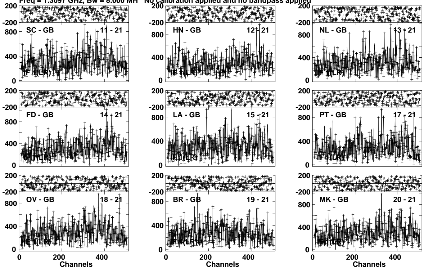
Lower frame: Micro Ampl Jy Top frame: Phas deg Vector averaged cross-power spectrum Several baselines displayed Timerange: 00/18:01:11 to 00/18:07:59
