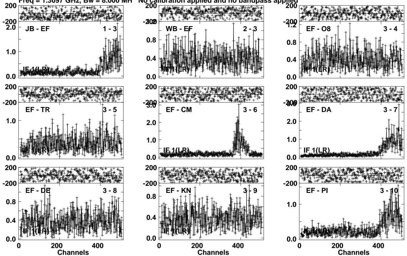
Lower frame: Milli Ampl Jy Top frame: Phas deg Vector averaged cross-power spectrum Several baselines displayed Timerange: 00/07:35:01 to 00/07:39:59
