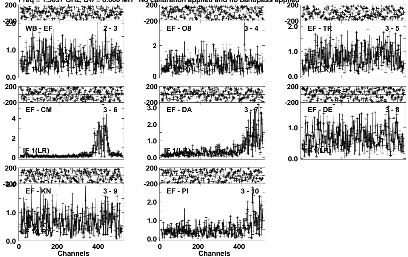
Lower frame: Milli Ampl Jy Top frame: Phas deg Vector averaged cross-power spectrum Several baselines displayed Timerange: 00/03:46:31 to 00/03:47:59
