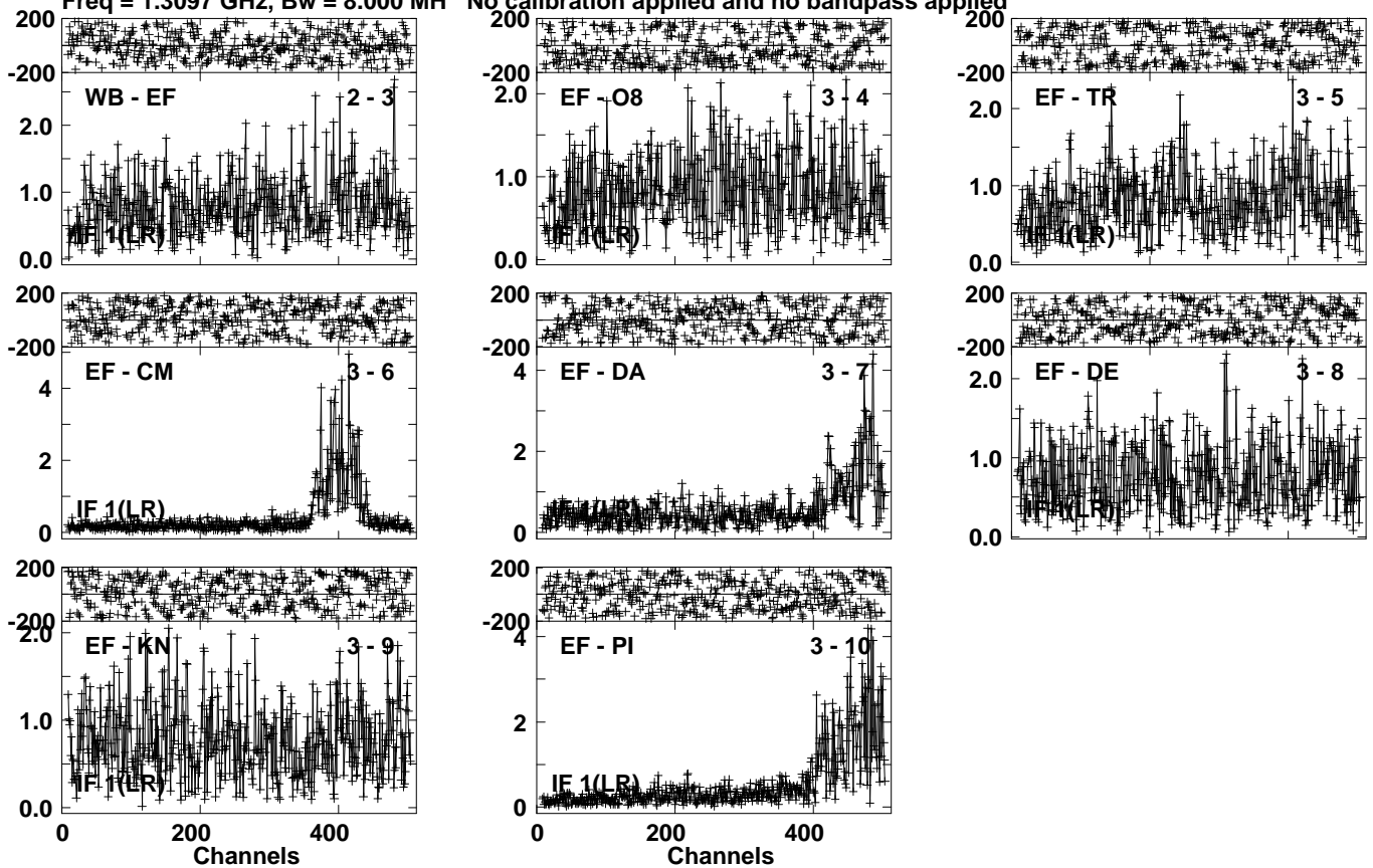
Lower frame: Milli Ampl Jy Top frame: Phas deg Vector averaged cross-power spectrum Several baselines displayed Timerange: 00/05:22:31 to 00/05:23:59
