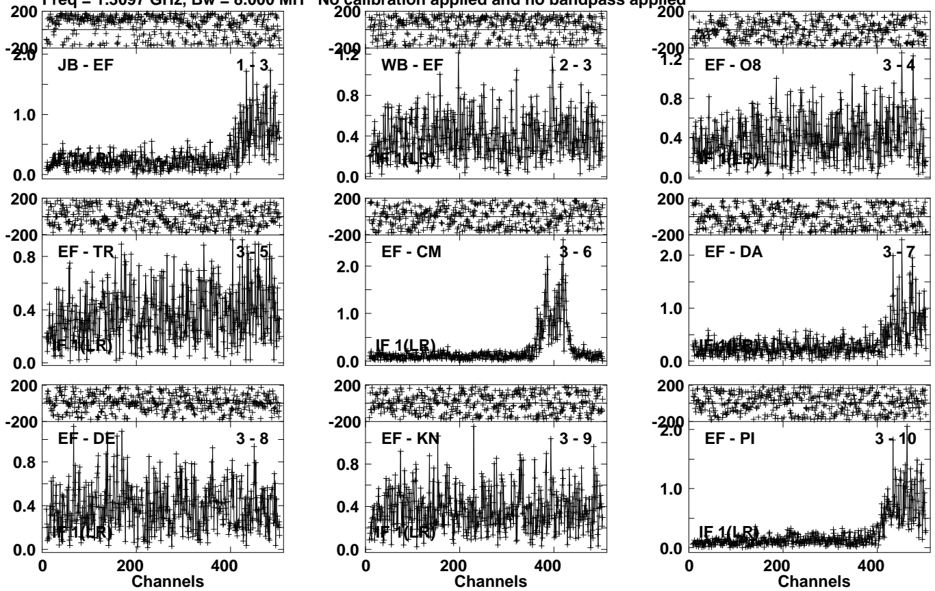
Lower frame: Milli Ampl Jy Top frame: Phas deg Vector averaged cross-power spectrum Several baselines displayed Timerange: 00/07:56:01 to 00/08:00:59
