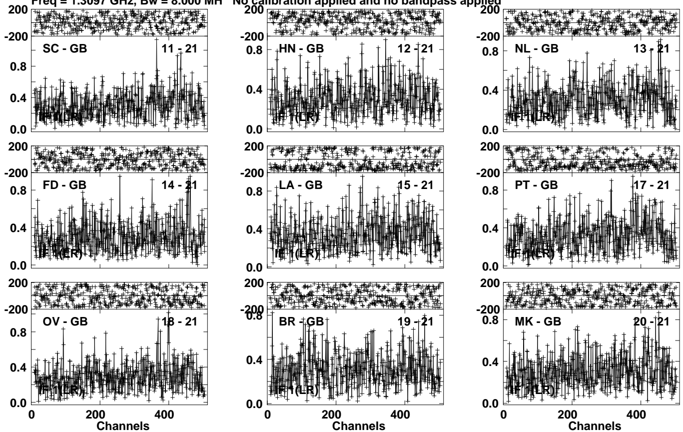
Lower frame: Milli Ampl Jy Top frame: Phas deg Vector averaged cross-power spectrum Several baselines displayed Timerange: 00/15:53:11 to 00/15:59:59
