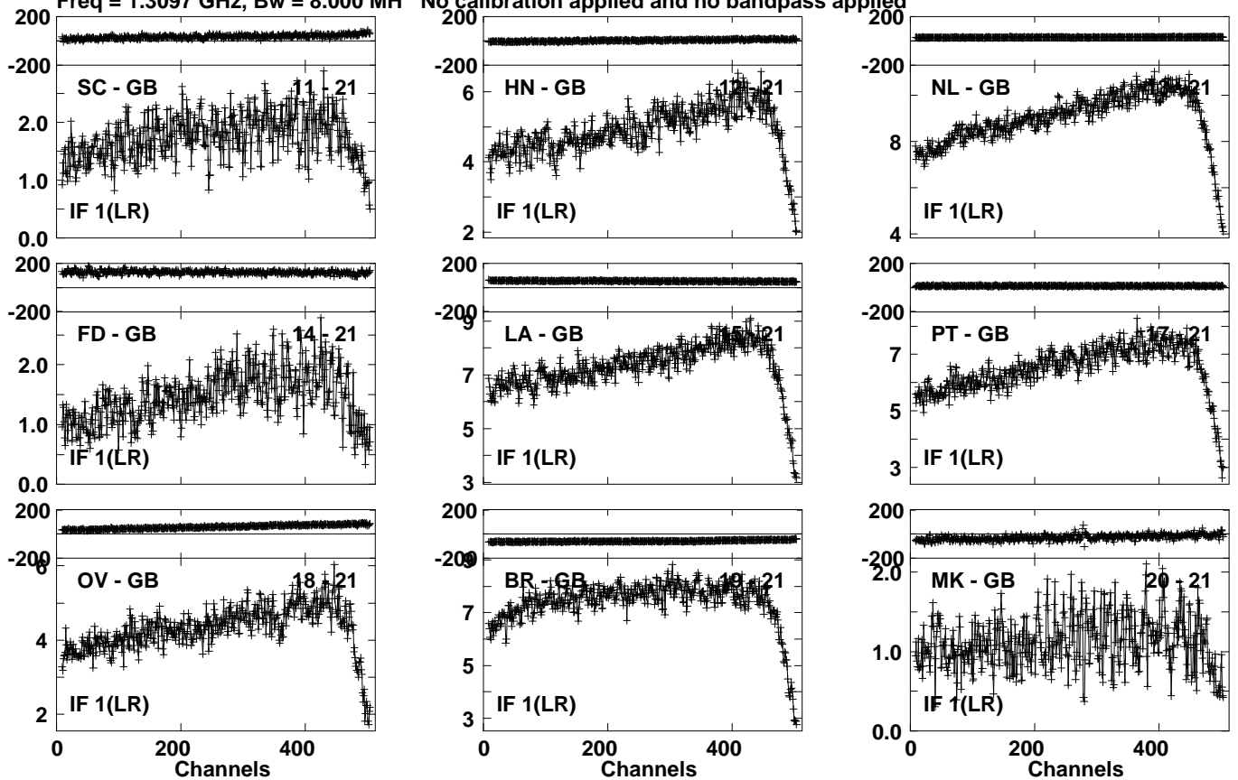
Lower frame: Milli Ampl Jy Top frame: Phas deg Vector averaged cross-power spectrum Several baselines displayed Timerange: 00/16:03:01 to 00/16:07:59
