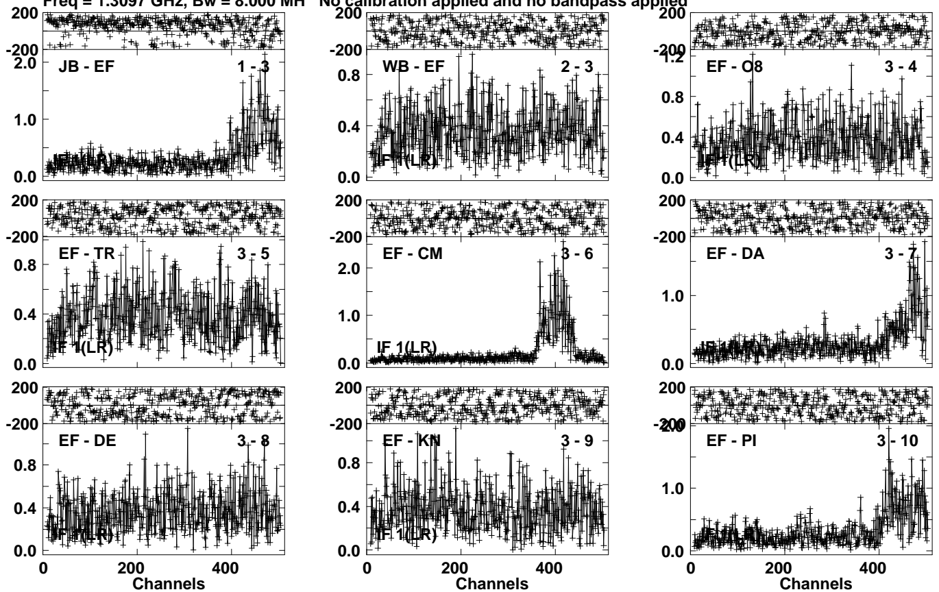
Lower frame: Milli Ampl Jy Top frame: Phas deg Vector averaged cross-power spectrum Several baselines displayed Timerange: 00/05:03:01 to 00/05:07:59
