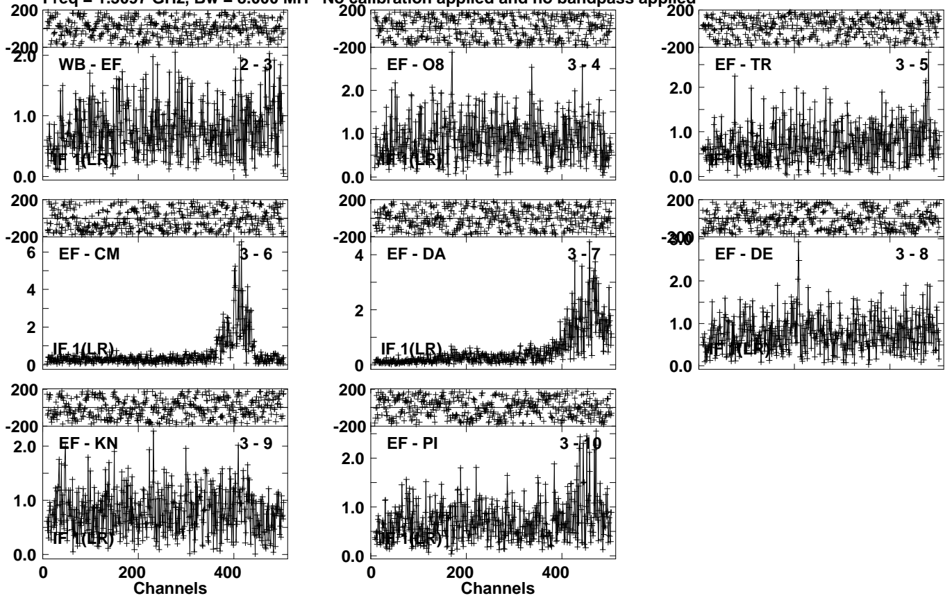
Lower frame: Milli Ampl Jy Top frame: Phas deg Vector averaged cross-power spectrum Several baselines displayed Timerange: 00/02:36:31 to 00/02:37:59
