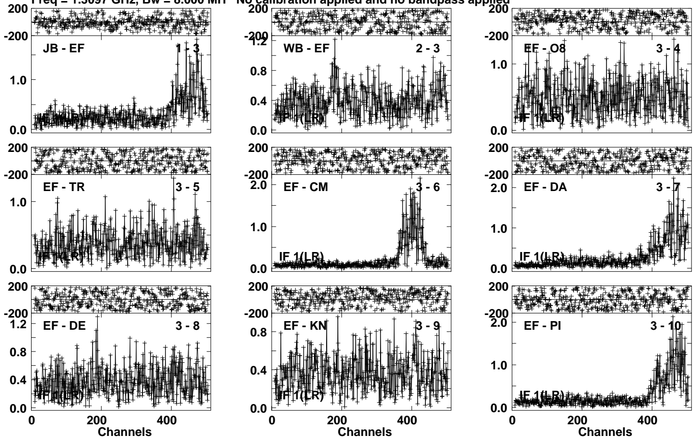
Lower frame: Milli Ampl Jy Top frame: Phas deg Vector averaged cross-power spectrum Several baselines displayed Timerange: 00/02:10:01 to 00/02:14:59
