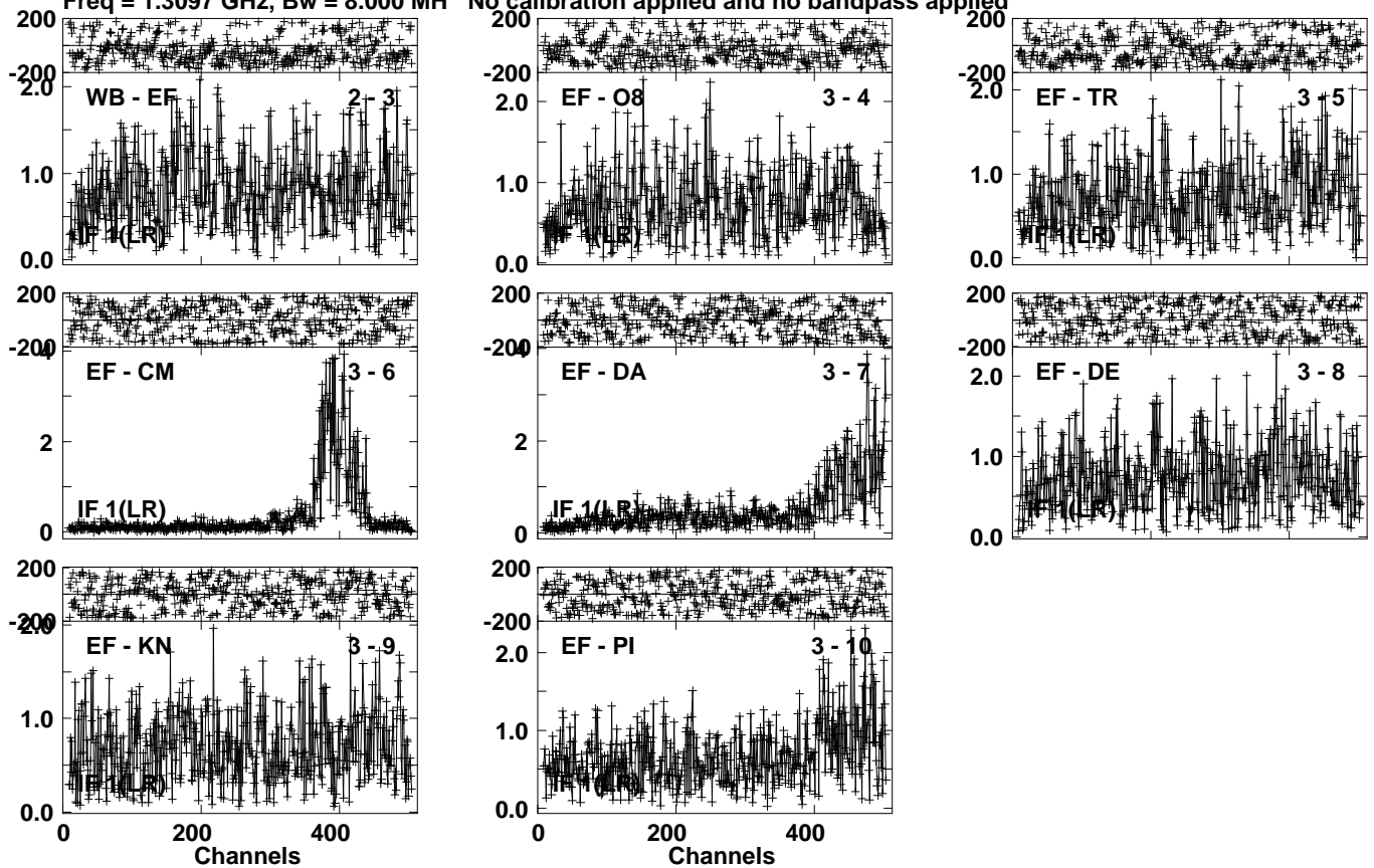
Lower frame: Milli Ampl Jy Top frame: Phas deg Vector averaged cross-power spectrum Several baselines displayed Timerange: 00/07:26:31 to 00/07:27:59
