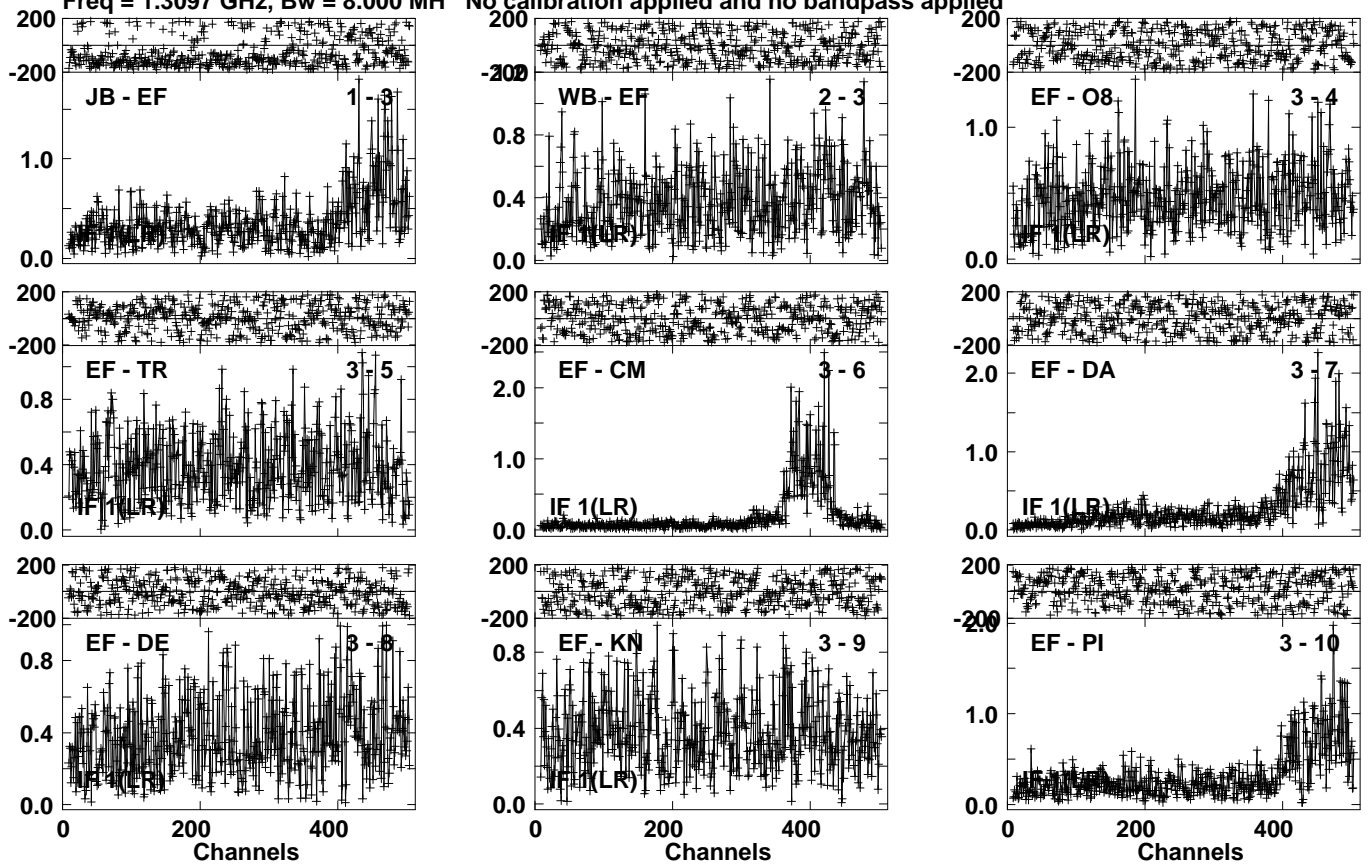
Lower frame: Milli Ampl Jy Top frame: Phas deg Vector averaged cross-power spectrum Several baselines displayed Timerange: 00/02:45:01 to 00/02:49:59
