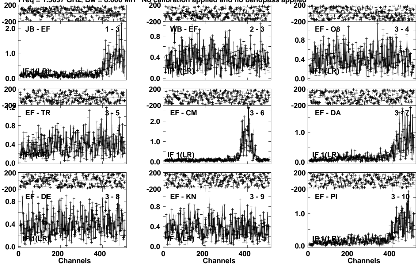
Lower frame: Milli Ampl Jy Top frame: Phas deg Vector averaged cross-power spectrum Several baselines displayed Timerange: 00/04:28:01 to 00/04:32:59
