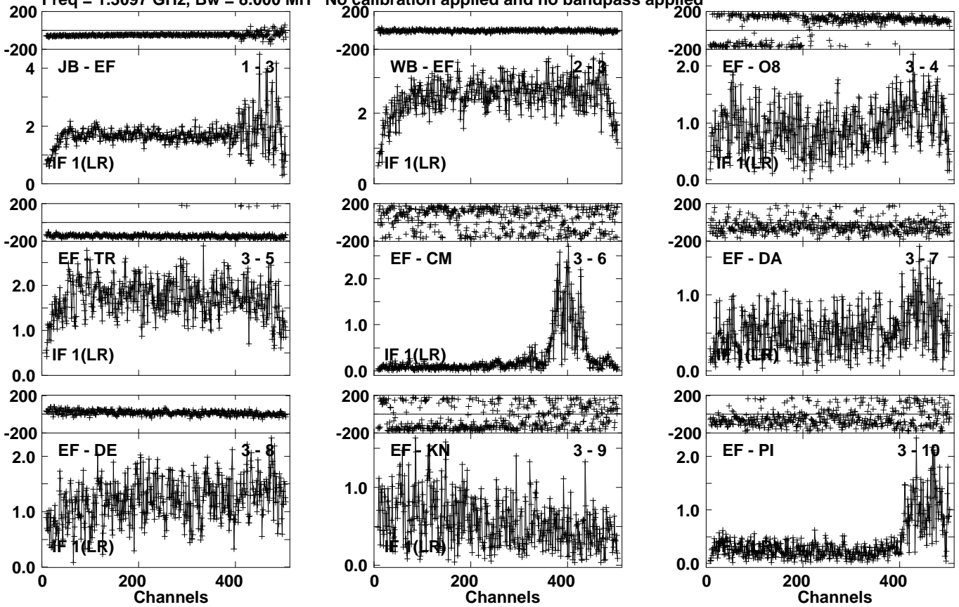
Lower frame: Milli Ampl Jy Top frame: Phas deg Vector averaged cross-power spectrum Several baselines displayed Timerange: 00/09:00:01 to 00/09:05:59
