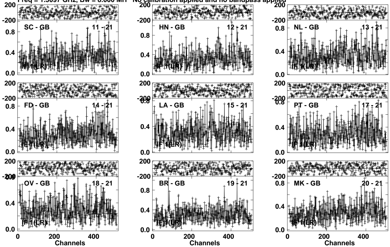
Lower frame: Milli Ampl Jy Top frame: Phas deg Vector averaged cross-power spectrum Several baselines displayed Timerange: 00/15:44:11 to 00/15:50:59
