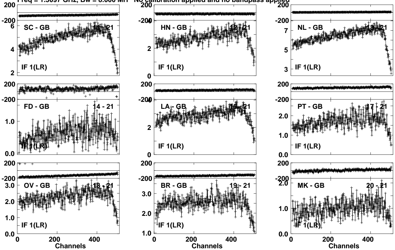
Lower frame: Milli Ampl Jy Top frame: Phas deg Vector averaged cross-power spectrum Several baselines displayed Timerange: 00/18:11:01 to 00/18:15:59
