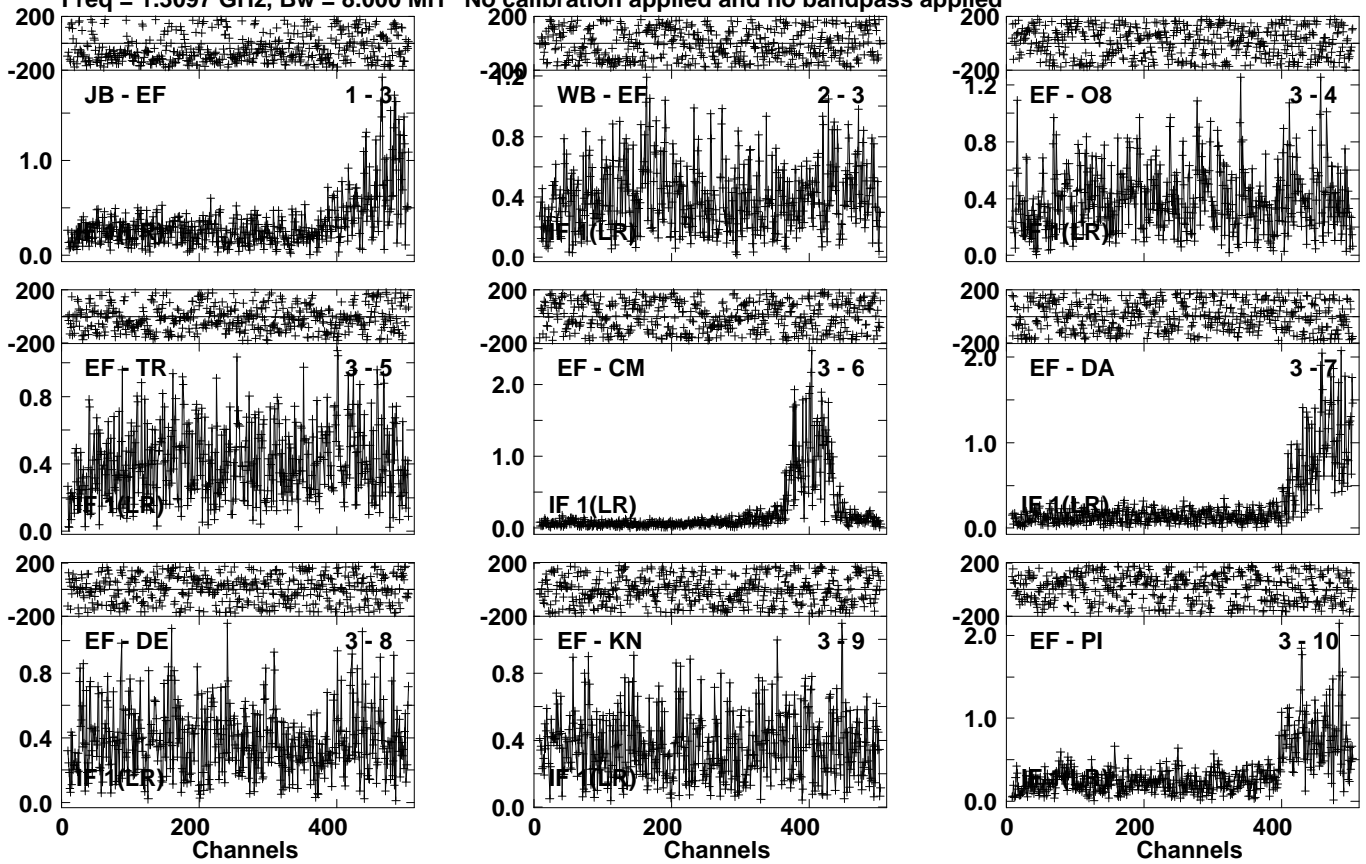
Lower frame: Milli Ampl Jy Top frame: Phas deg Vector averaged cross-power spectrum Several baselines displayed Timerange: 00/03:34:01 to 00/03:38:59
