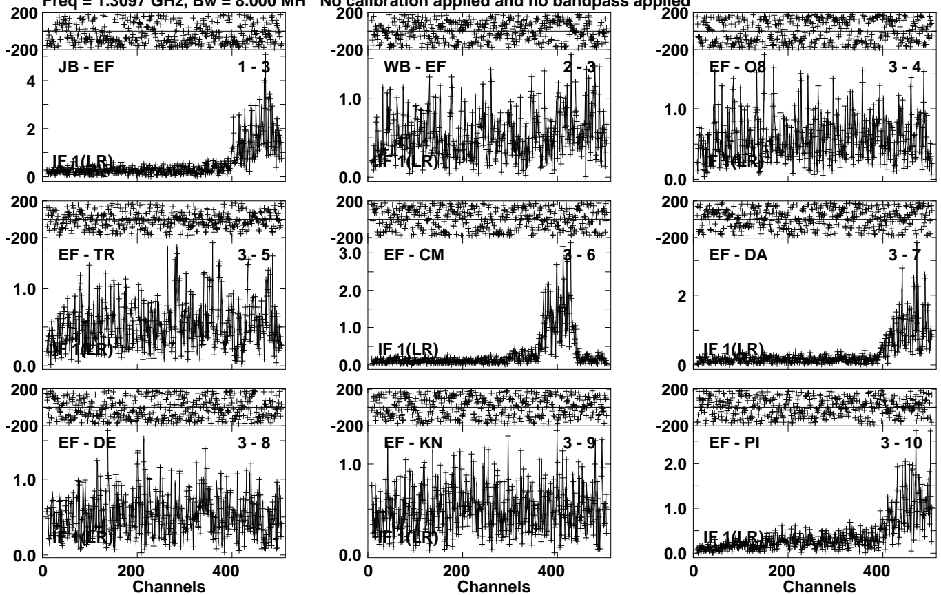
Lower frame: Milli Ampl Jy Top frame: Phas deg Vector averaged cross-power spectrum Several baselines displayed Timerange: 00/04:24:01 to 00/04:27:59
