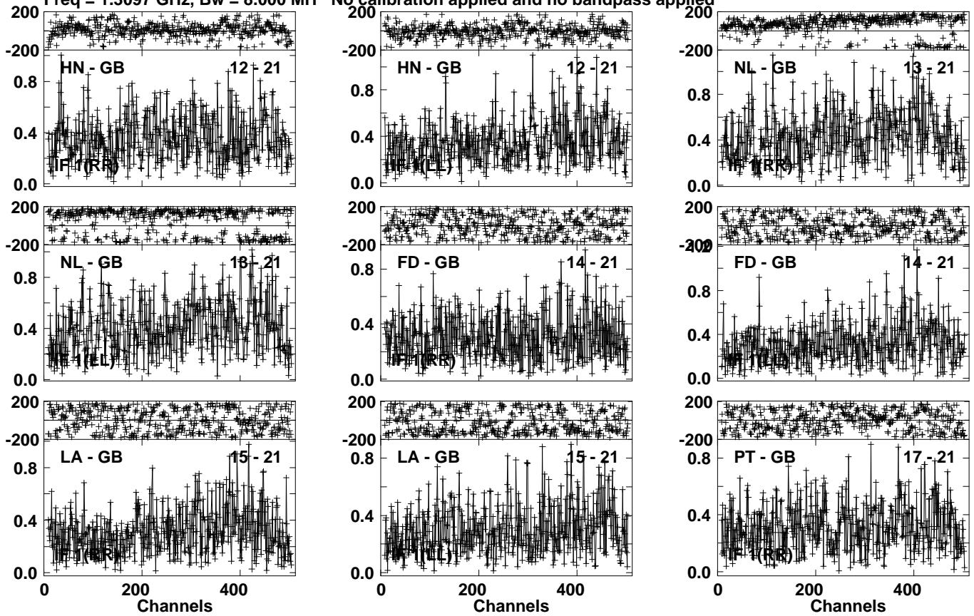
Lower frame: Milli Ampl Jy Top frame: Phas deg Vector averaged cross-power spectrum Several baselines displayed Timerange: 00/18:30:11 to 00/18:36:59
