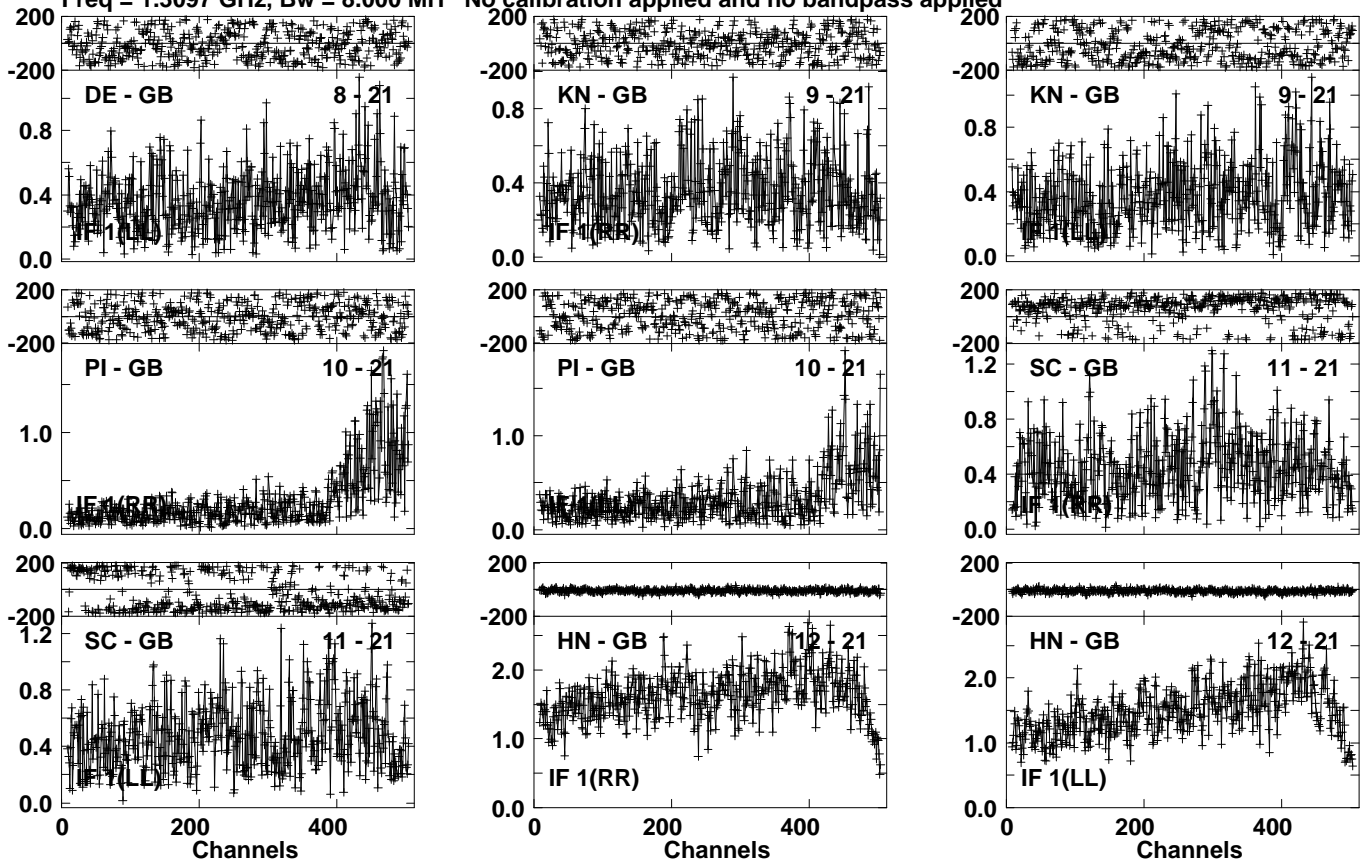
Lower frame: Milli Ampl Jy Top frame: Phas deg Vector averaged cross-power spectrum Several baselines displayed Timerange: 00/09:54:01 to 00/09:58:59
