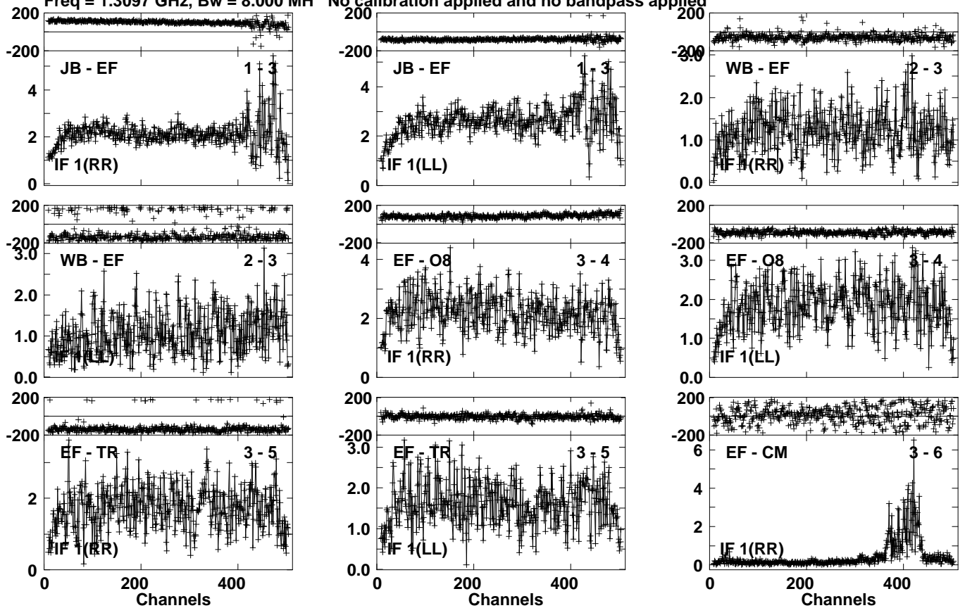
Lower frame: Milli Amp Jy Top frame: Phas deg Vector averaged cross-power spectrum Several baselines displayed Timerange: 00/03:39:01 to 00/03:40:59
