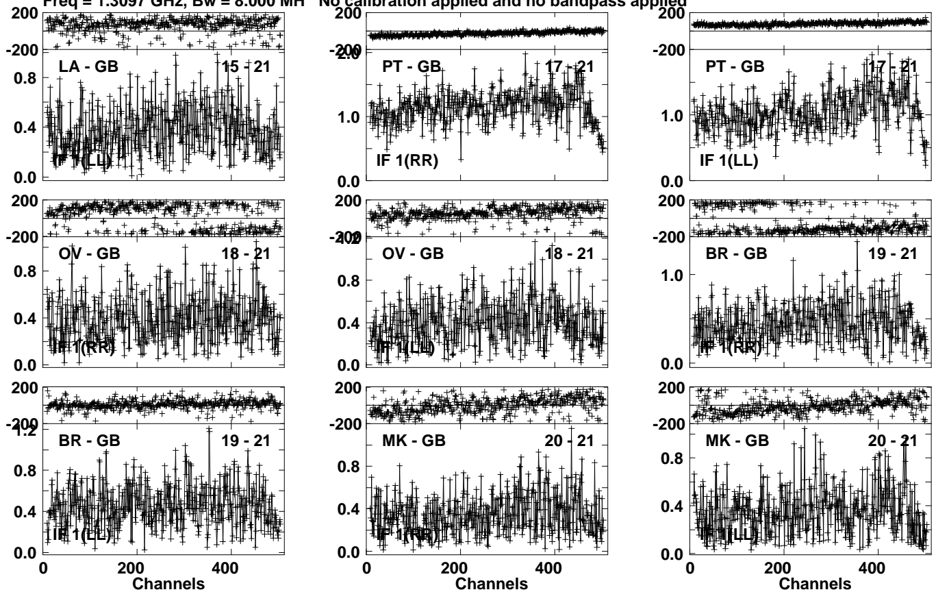
Lower frame: Milli Ampl Jy Top frame: Phas deg Vector averaged cross-power spectrum Several baselines displayed Timerange: 00/15:35:11 to 00/15:41:59
