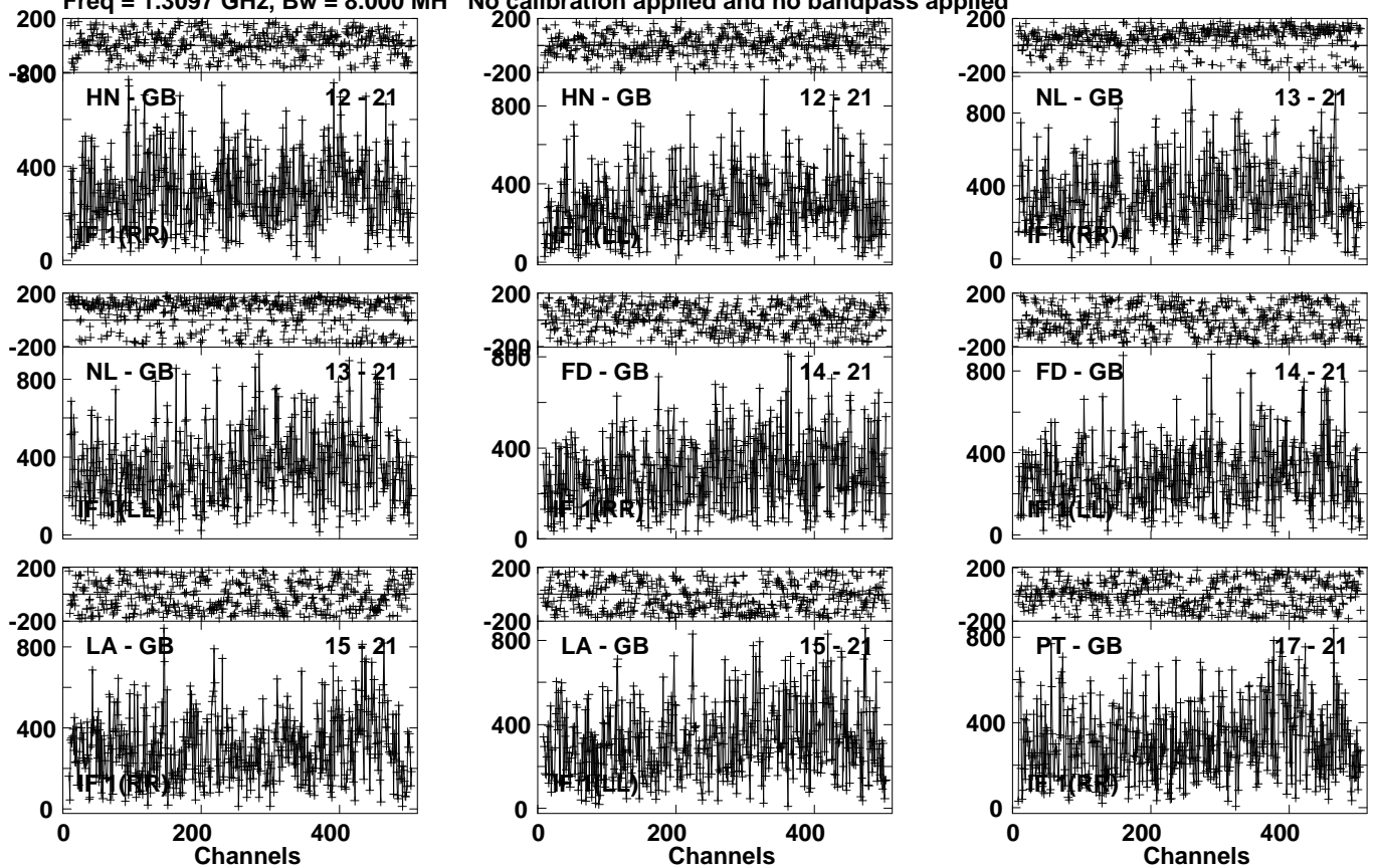
Lower frame: Micro Ampl Jy Top frame: Phas deg Vector averaged cross-power spectrum Several baselines displayed Timerange: 00/18:48:11 to 00/18:54:59
