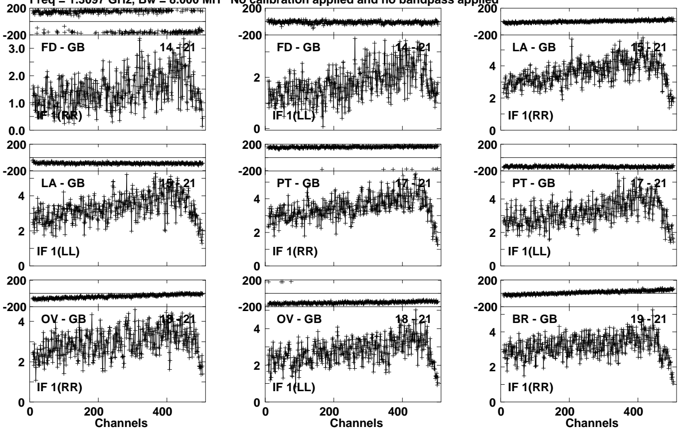
Lower frame: Milli Ampl Jy Top frame: Phas deg Vector averaged cross-power spectrum Several baselines displayed Timerange: 00/13:34:31 to 00/13:35:59
