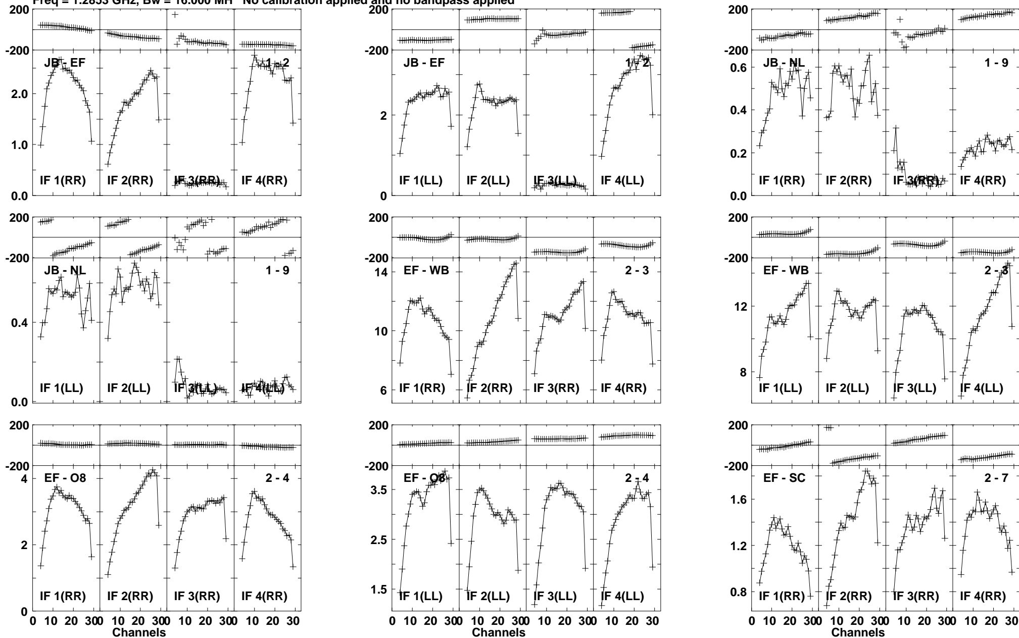
Lower frame: Milli Ampl Jy Top frame: Phas deg Vector averaged cross-power spectrum Baseline: JB (01) - EF (02) Timerange: 00/19:50:44 to 00/19:54:18
