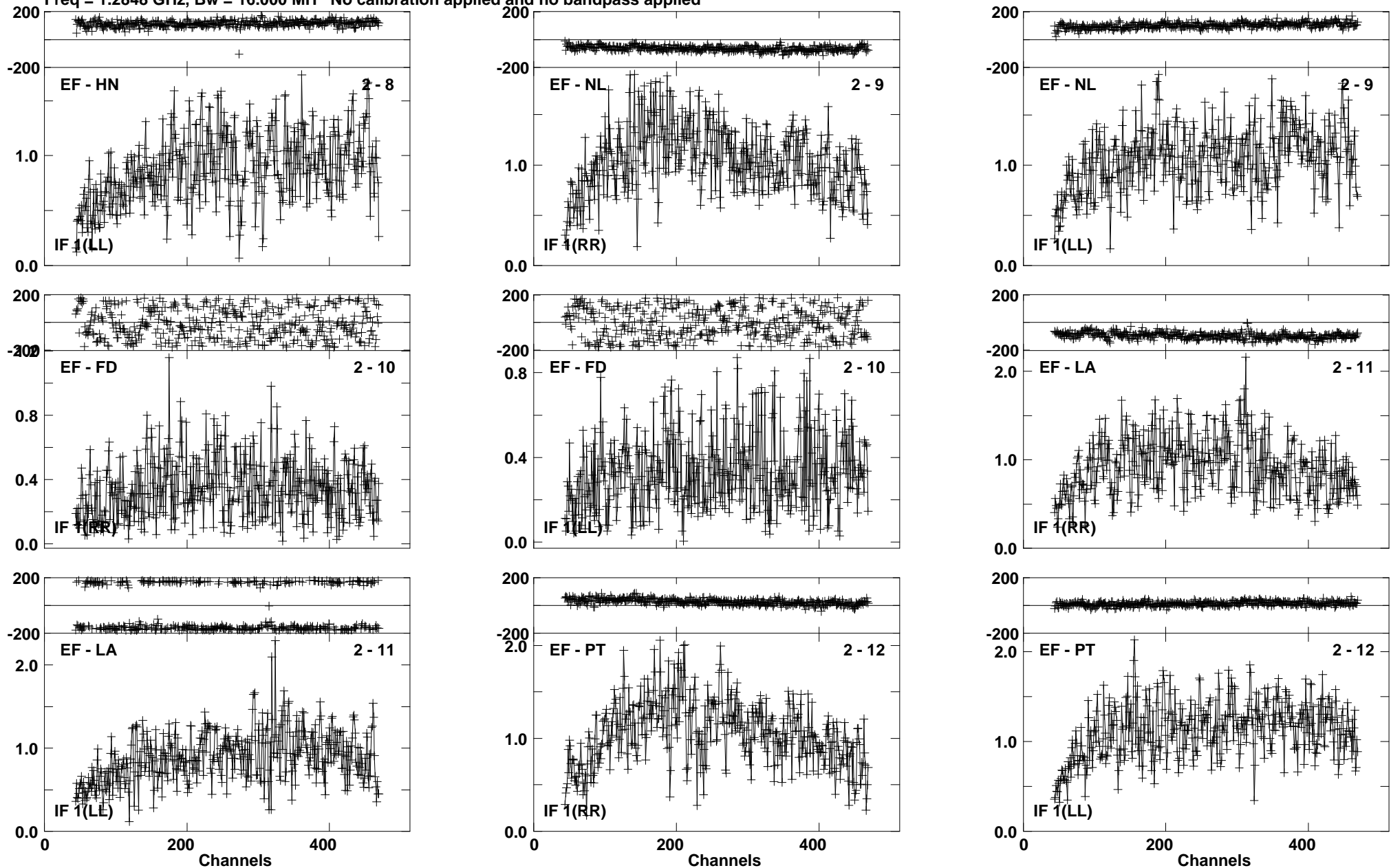
Lower frame: Milli Ampl Jy Top frame: Phas deg Vector averaged cross-power spectrum Baseline: EF (02) - HN (08) Timerange: 00/23:30:34 to 00/23:33:58
