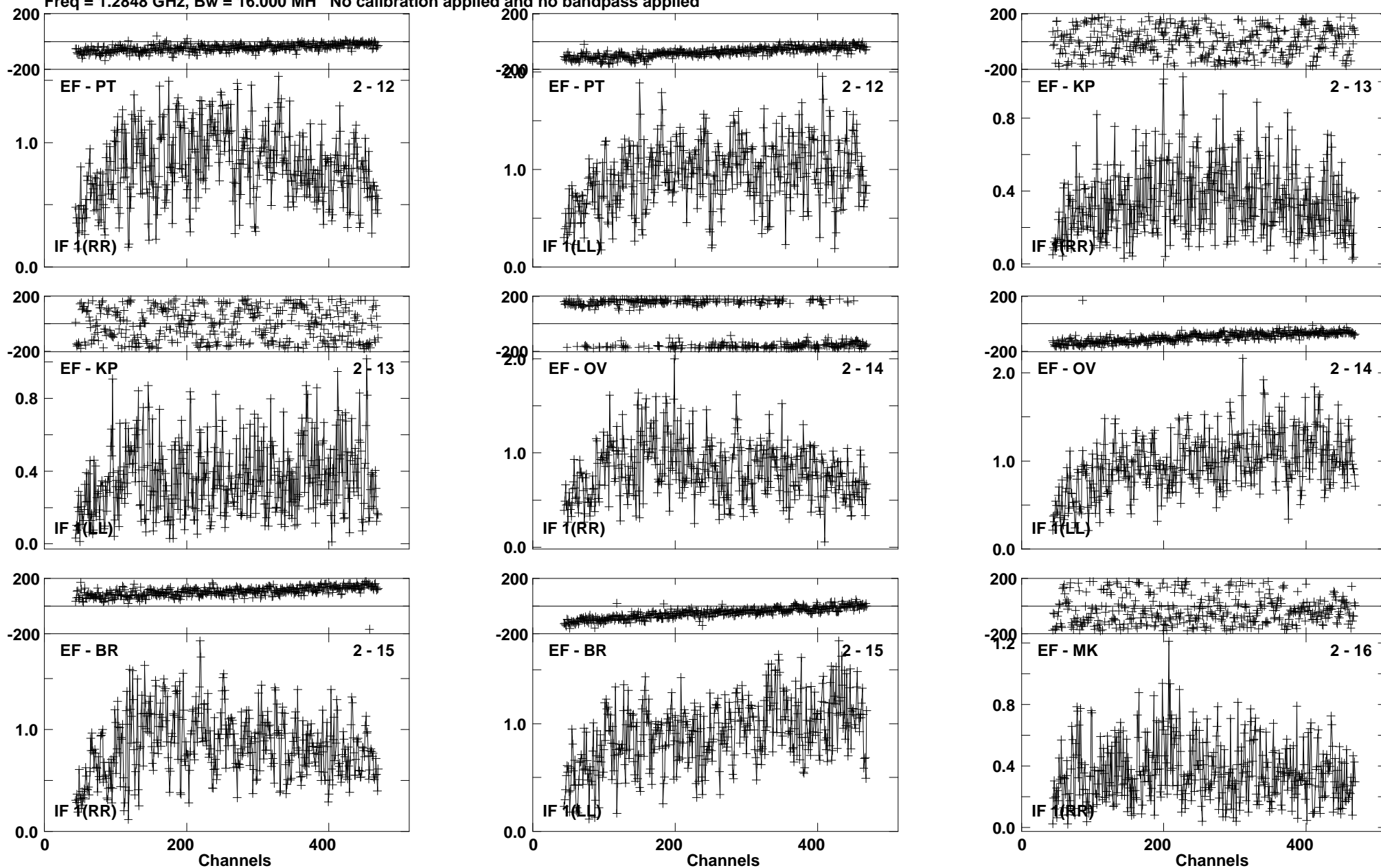
Lower frame: Milli Ampl Jy Top frame: Phas deg Vector averaged cross-power spectrum Baseline: EF (02) - PT (12) Timerange: 00/21:44:34 to 00/21:47:48
