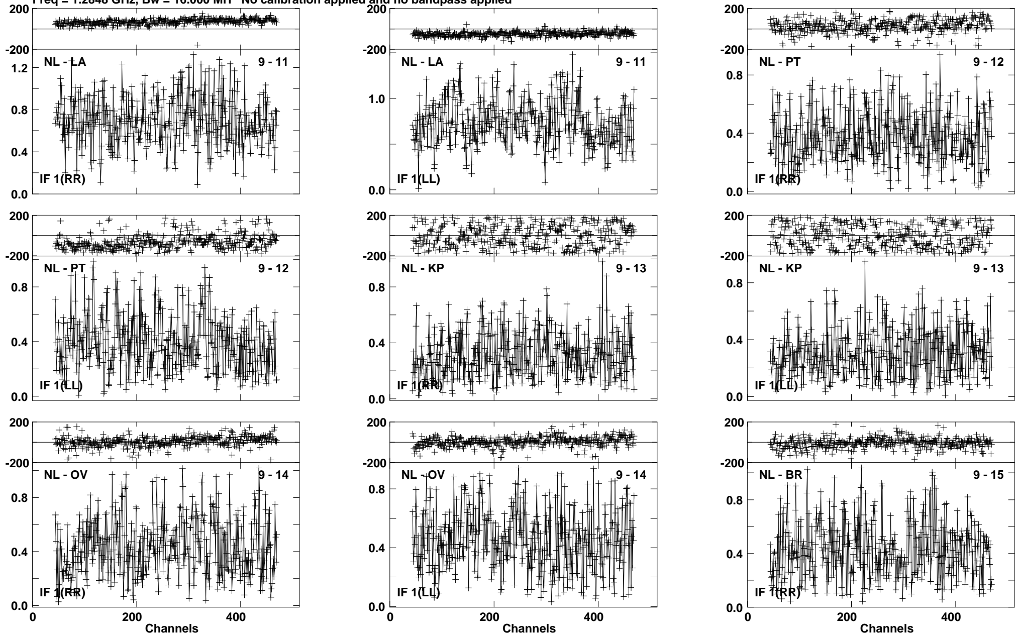
Lower frame: Milli Ampl Jy Top frame: Phas deg Vector averaged cross-power spectrum Baseline: NL (09) - LA (11) Timerange: 00/18:29:59 to 00/18:33:19
