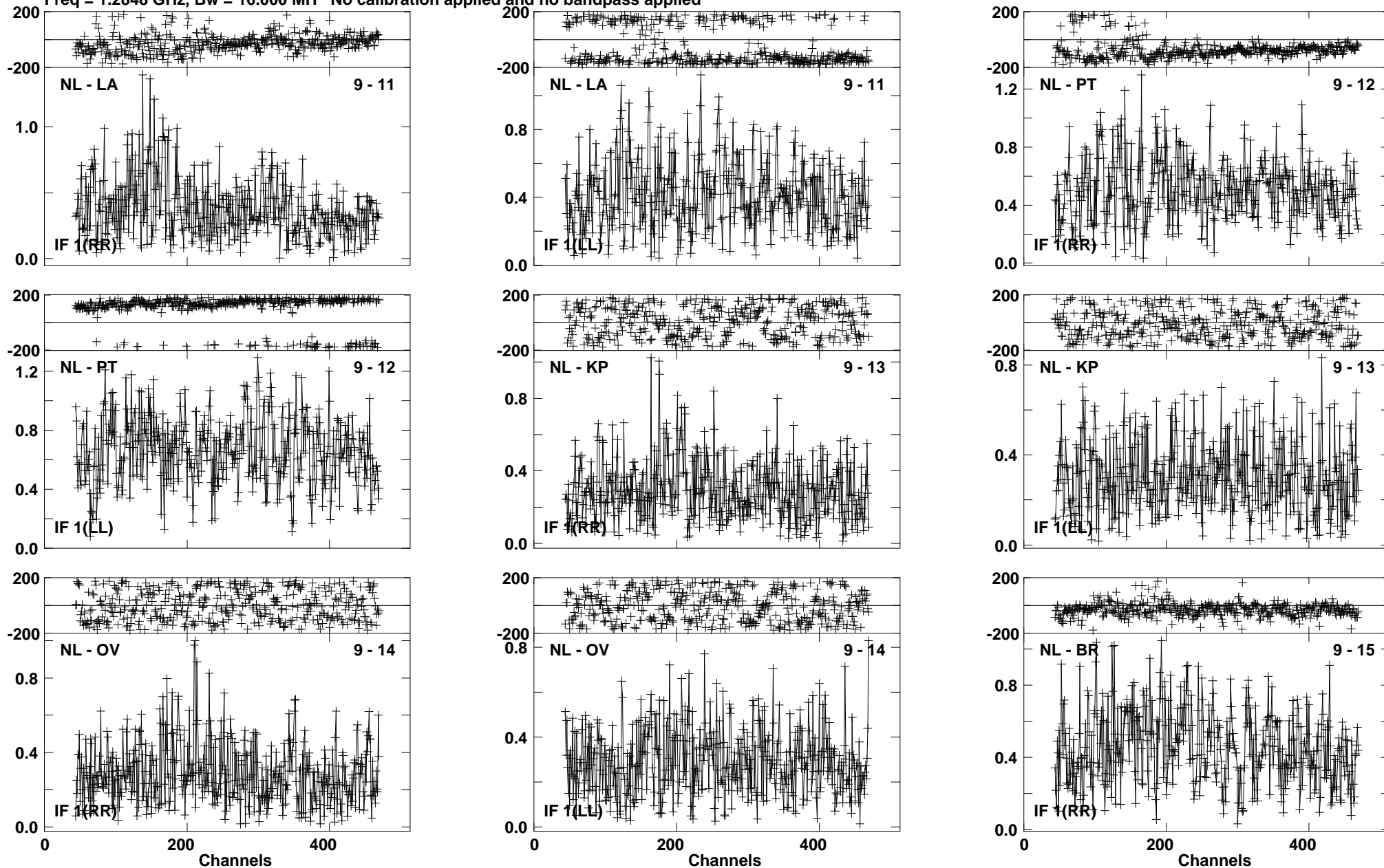
Lower frame: Milli Ampl Jy Top frame: Phas deg Vector averaged cross-power spectrum Baseline: NL (09) - LA (11) Timerange: 00/17:35:49 to 00/17:39:19
