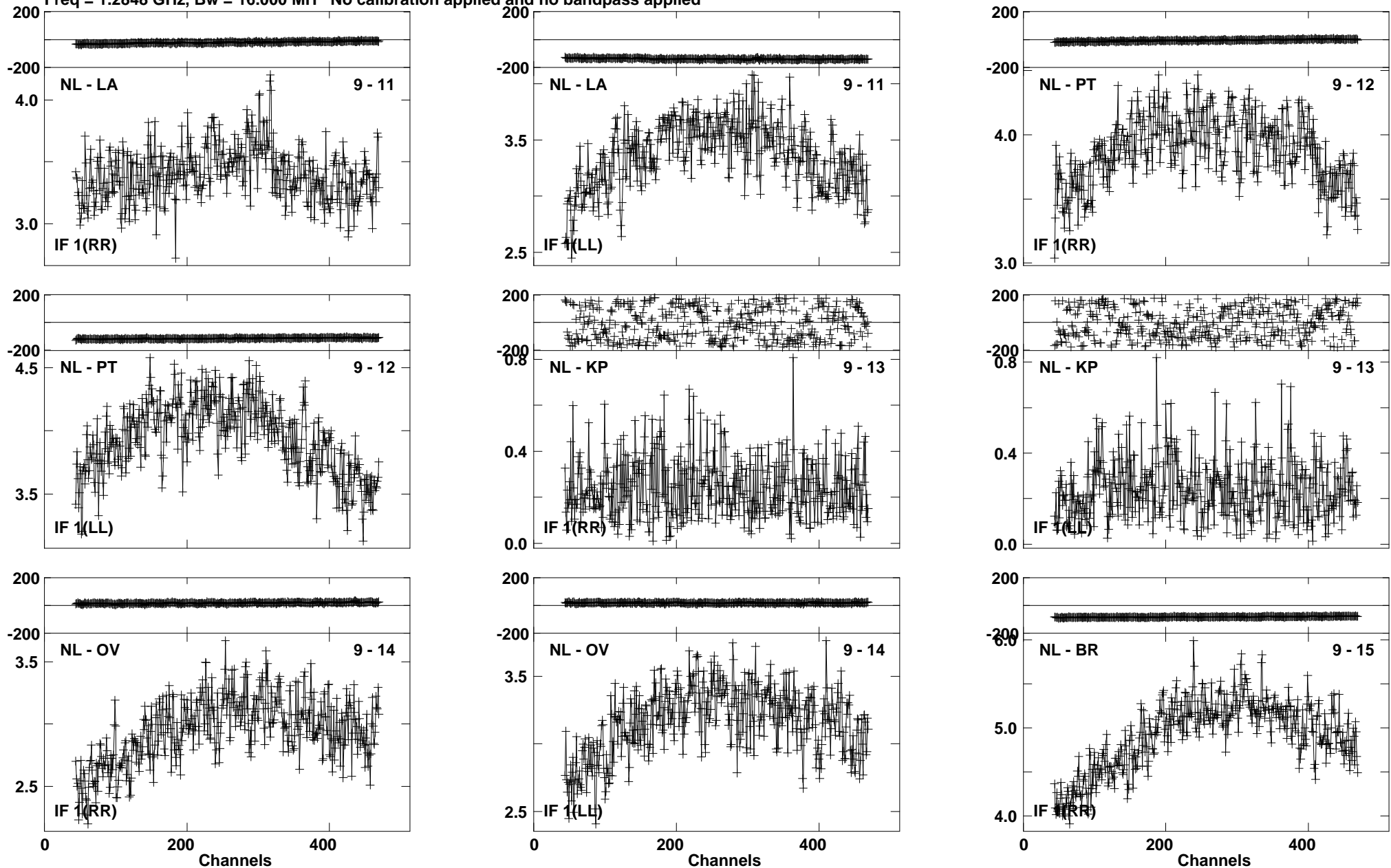
Lower frame: Milli Ampl Jy Top frame: Phas deg Vector averaged cross-power spectrum Baseline: NL (09) - LA (11) Timerange: 00/18:21:51 to 00/18:26:49
