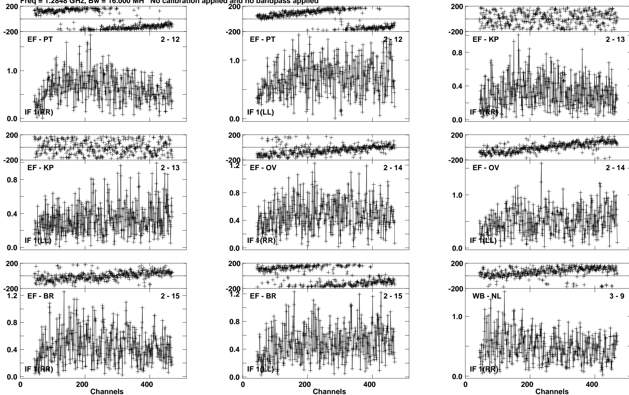
Lower frame: Milli Ampl Jy Top frame: Phas deg Vector averaged cross-power spectrum Baseline: EF (02) - PT (12) Timerange: 00/19:24:54 to 00/19:28:18
