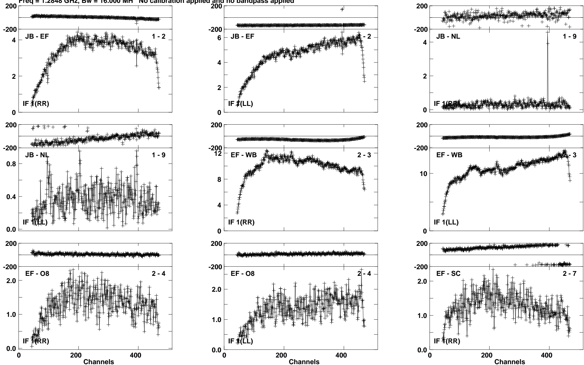
Lower frame: Milli Ampl Jy Top frame: Phas deg Vector averaged cross-power spectrum Baseline: JB (01) - EF (02) Timerange: 00/18:57:30 to 00/19:00:48
