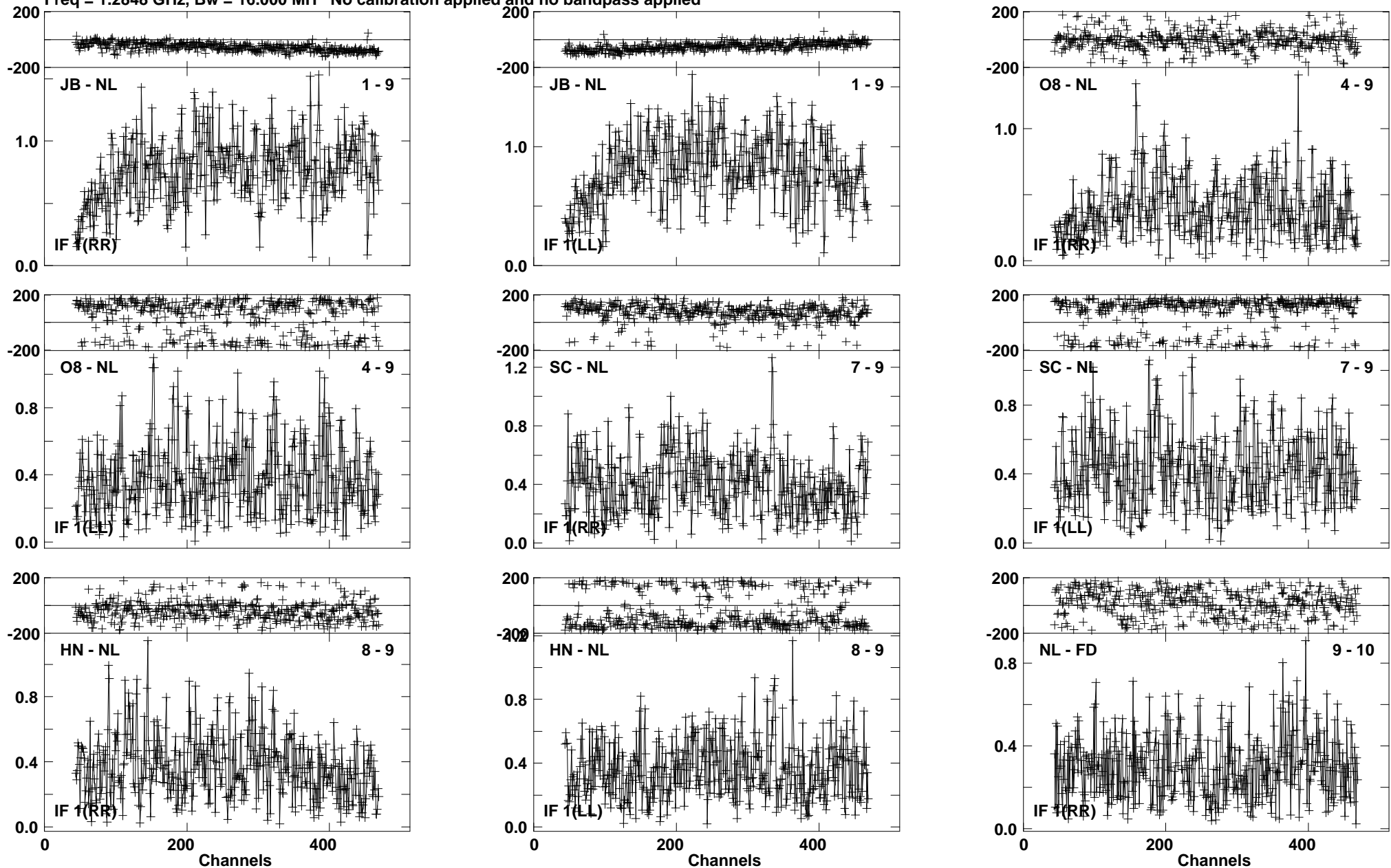
Lower frame: Milli Ampl Jy Top frame: Phas deg Vector averaged cross-power spectrum Baseline: JB (01) - NL (09) Timerange: 01/01:22:14 to 01/01:25:38
