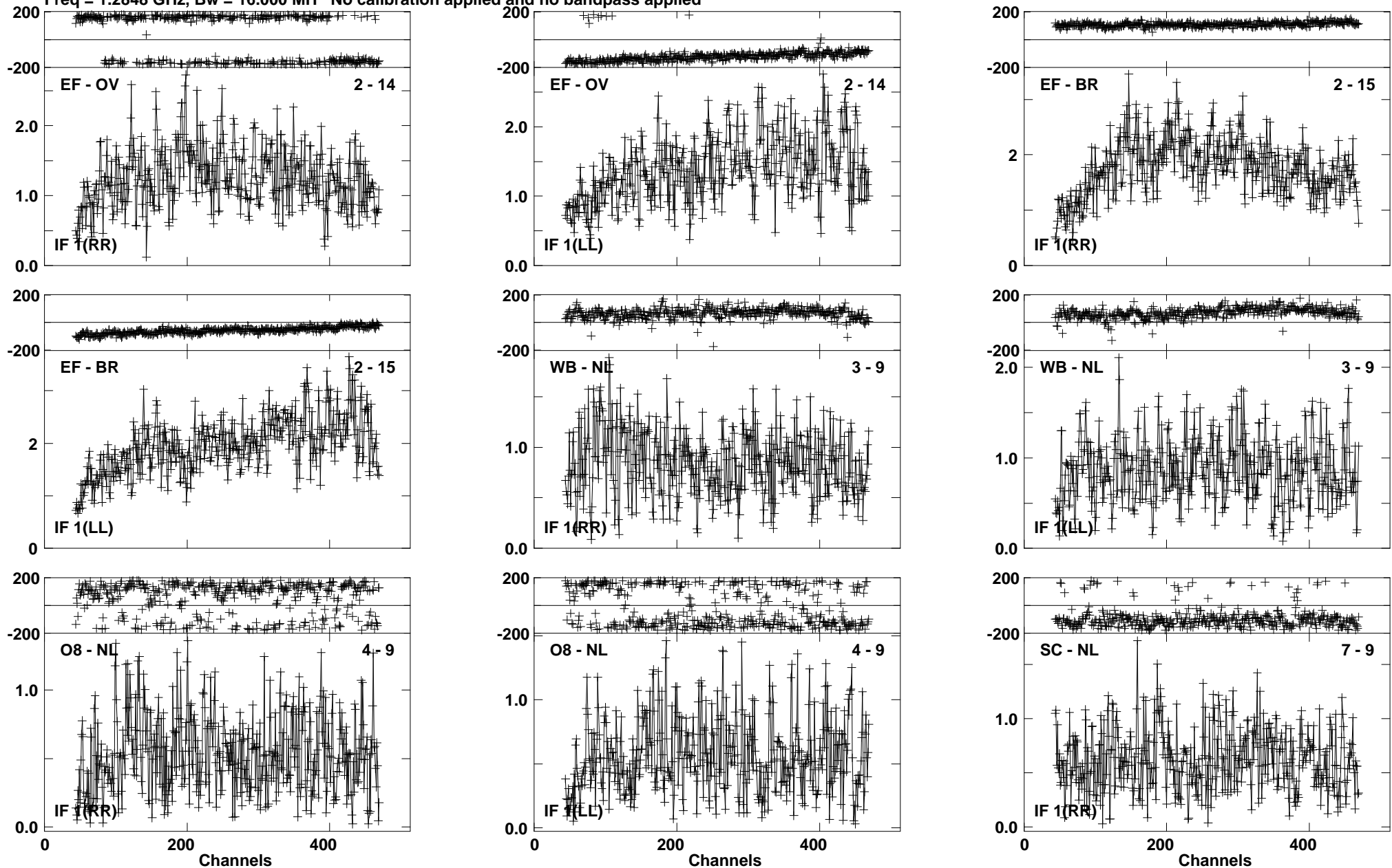
Lower frame: Milli Ampl Jy Top frame: Phas deg Vector averaged cross-power spectrum Baseline: EF (02) - OV (14) Timerange: 00/19:12:00 to 00/19:13:48
