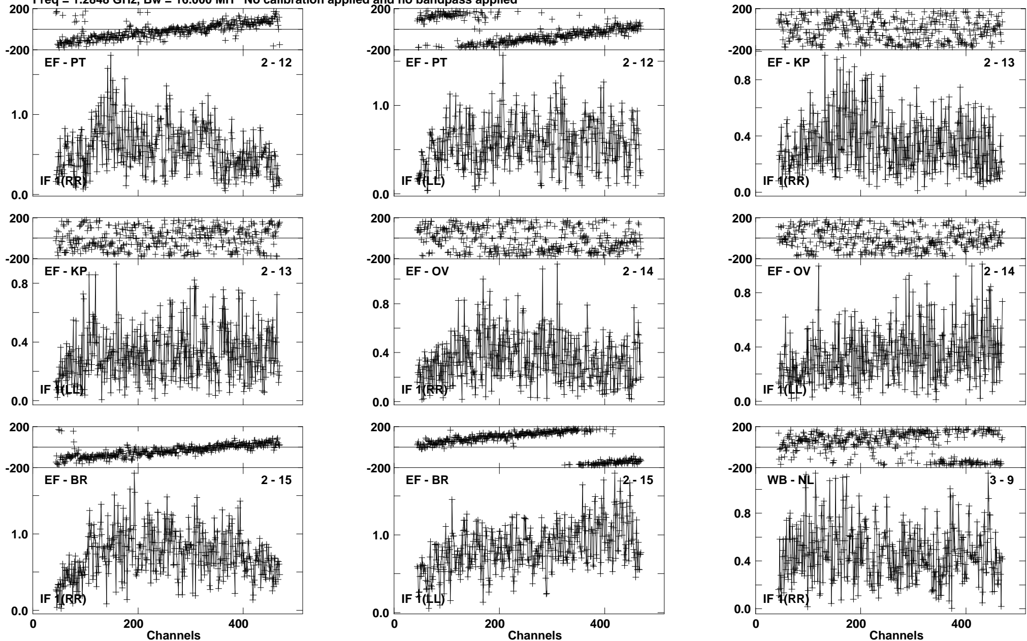
Lower frame: Milli Ampl Jy Top frame: Phas deg Vector averaged cross-power spectrum Baseline: EF (02) - PT (12) Timerange: 00/17:58:29 to 00/18:01:59
