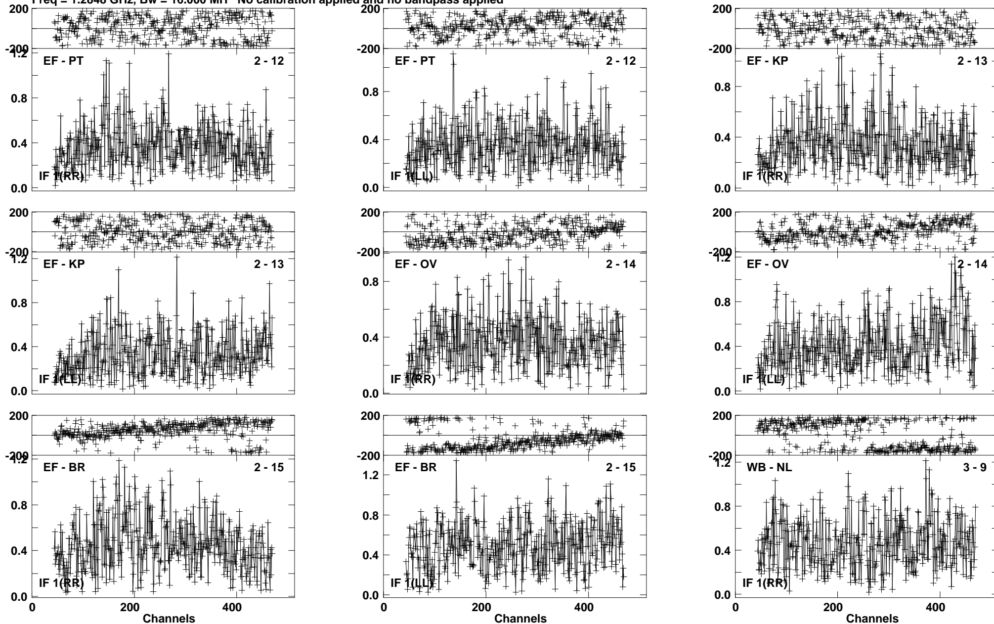
Lower frame: Milli Ampl Jy Top frame: Phas deg Vector averaged cross-power spectrum Baseline: EF (02) - PT (12) Timerange: 00/19:08:30 to 00/19:11:48
