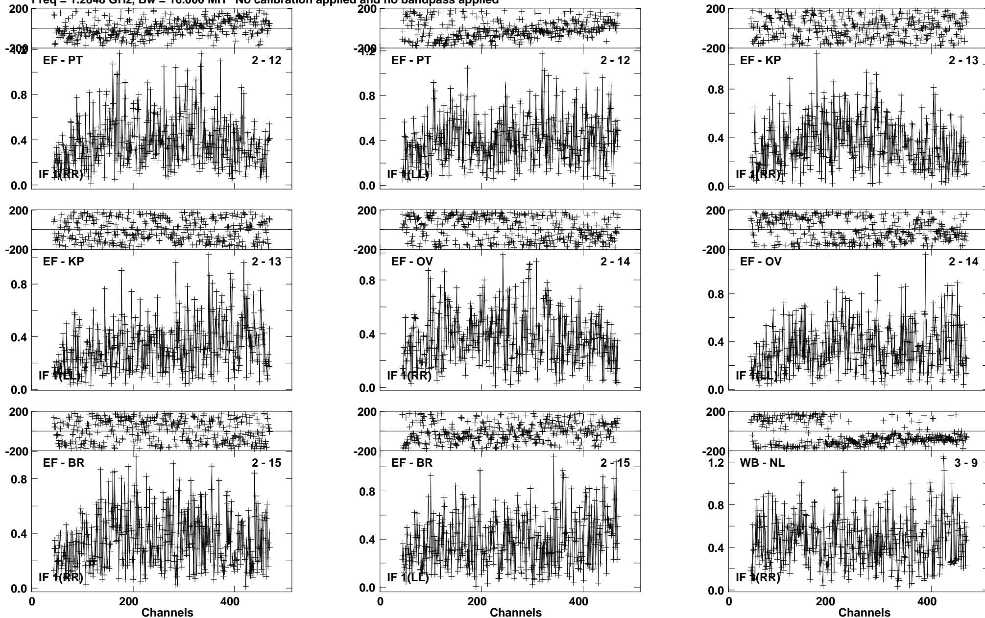
Lower frame: Milli Ampl Jy Top frame: Phas deg Vector averaged cross-power spectrum Baseline: EF (02) - PT (12) Timerange: 00/18:51:54 to 00/18:55:18
