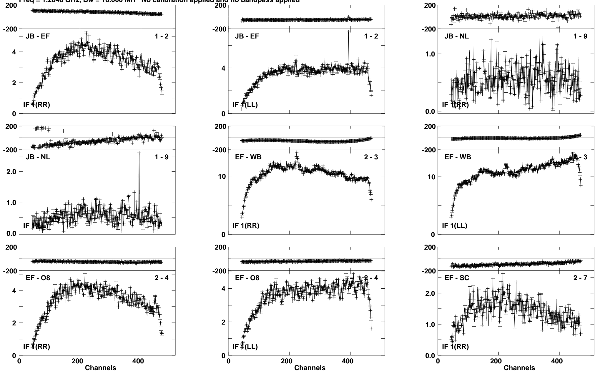
Lower frame: Milli Ampl Jy Top frame: Phas deg Vector averaged cross-power spectrum Baseline: JB (01) - EF (02) Timerange: 00/19:56:30 to 00/19:59:58
