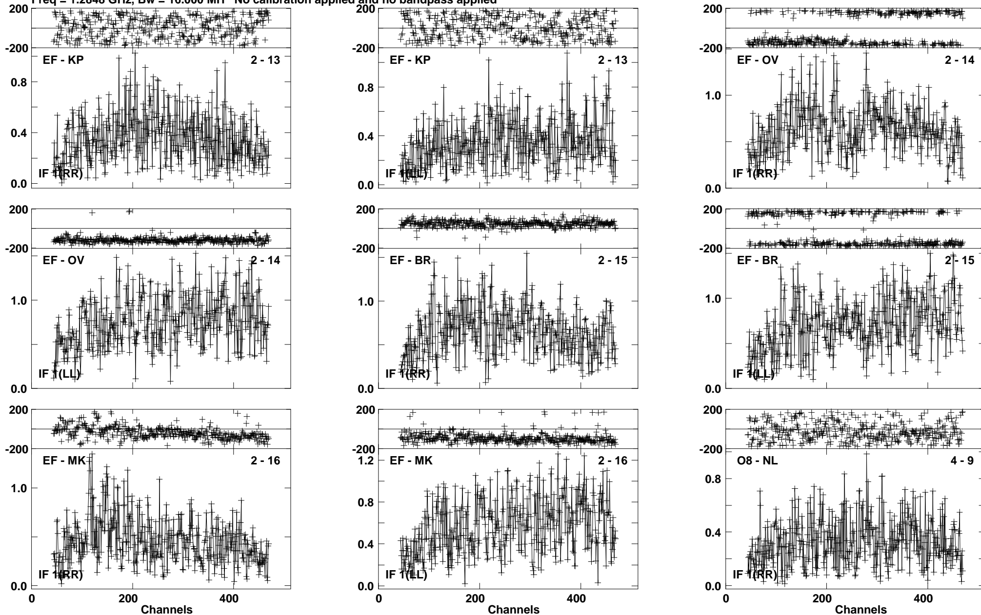
Lower frame: Milli Ampl Jy Top frame: Phas deg Vector averaged cross-power spectrum Baseline: EF (02) - KP (13) Timerange: 00/23:52:34 to 00/23:55:58
