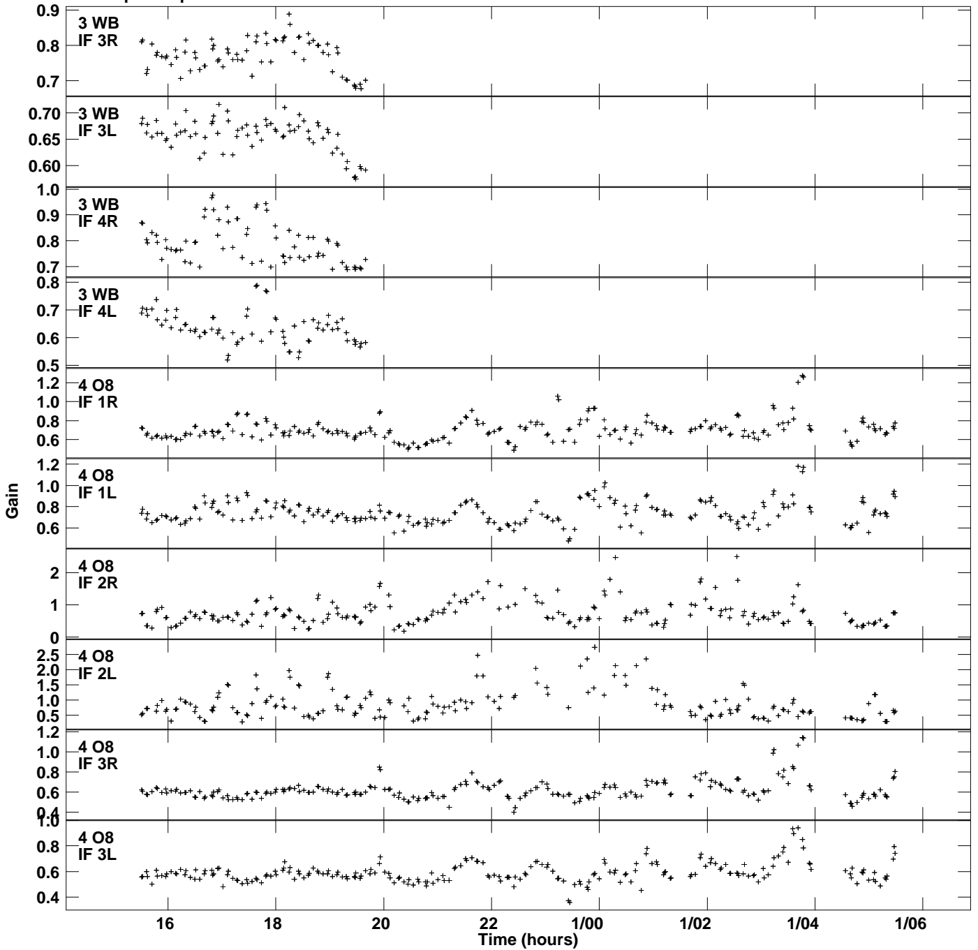
Plot file version 3 created 03-MAR-2016 01:21:30 Gain amp vs UTC time for J1545+5400.MULTI.1 SN 2 Rpol & Lpol IF 1 - 4
