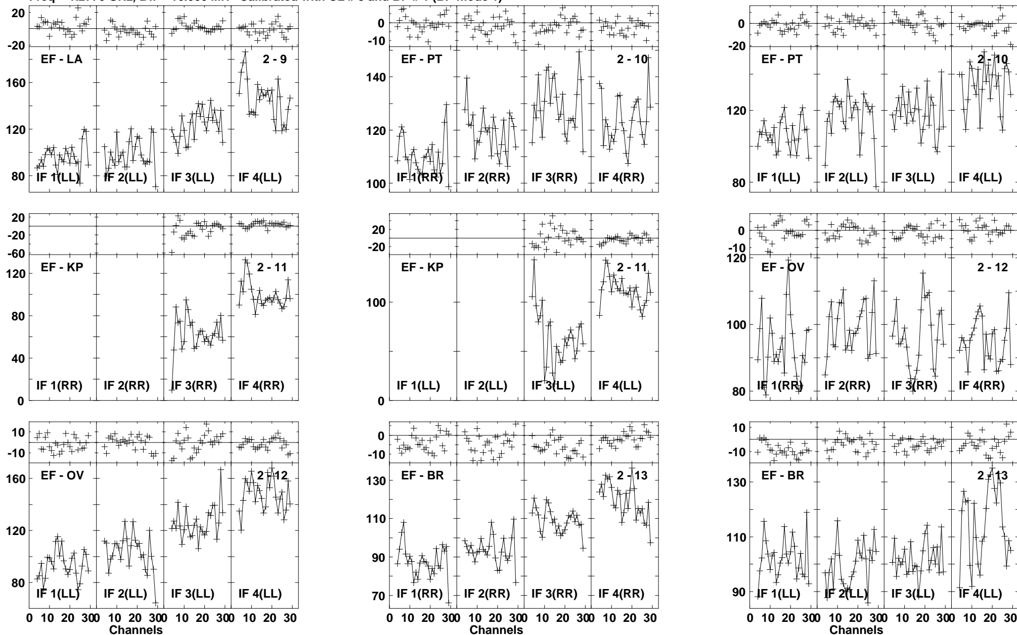
Lower frame: Milli Ampl Jy Top frame: Phas deg Vector averaged cross-power spectrum Baseline: EF (02) - LA (09) Timerange: 01/04:59:05 to 01/05:00:23
