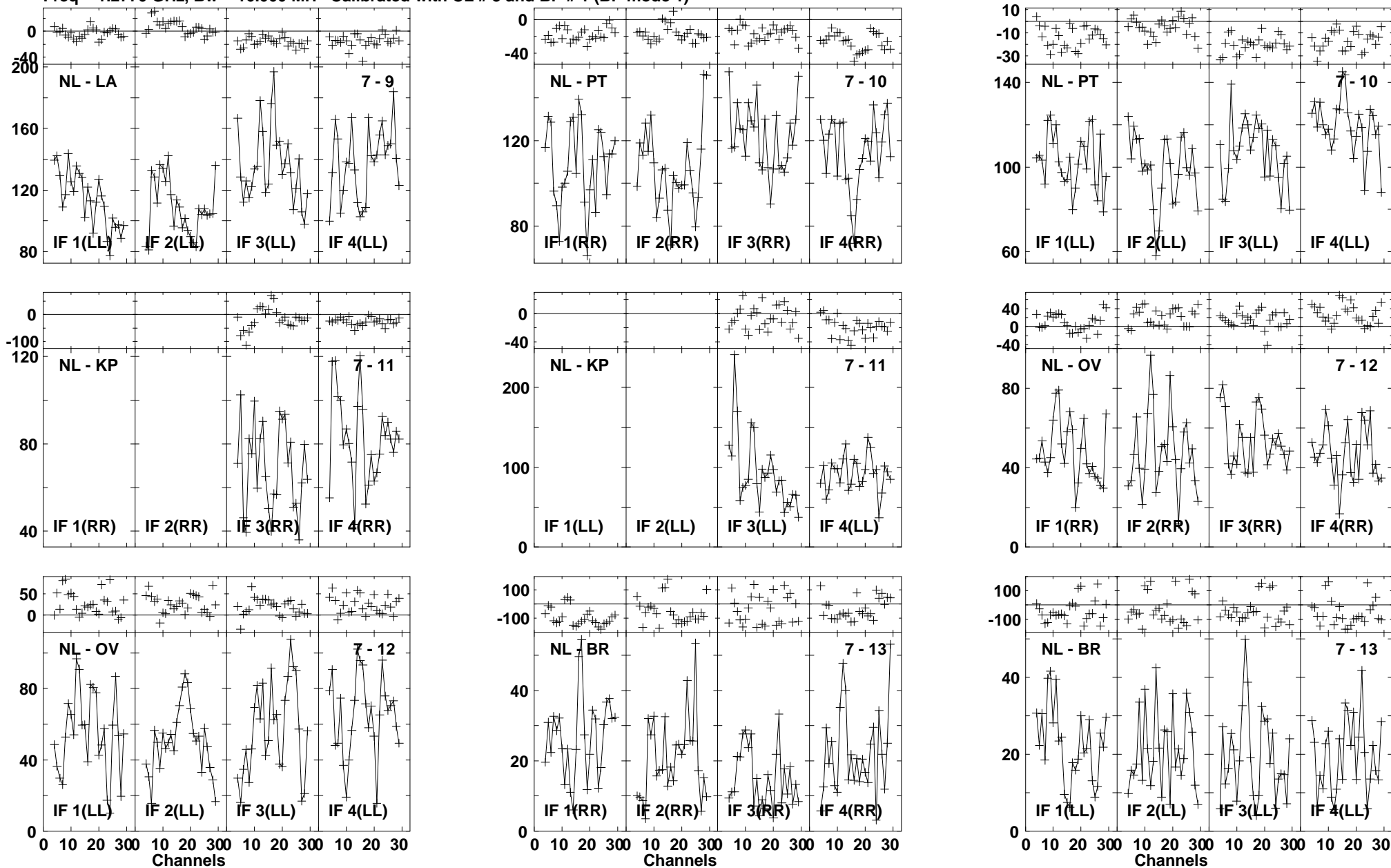
Lower frame: Milli Ampl Jy Top frame: Phas deg Vector averaged cross-power spectrum Baseline: NL (07) - LA (09) Timerange: 01/00:53:43 to 01/00:56:59
