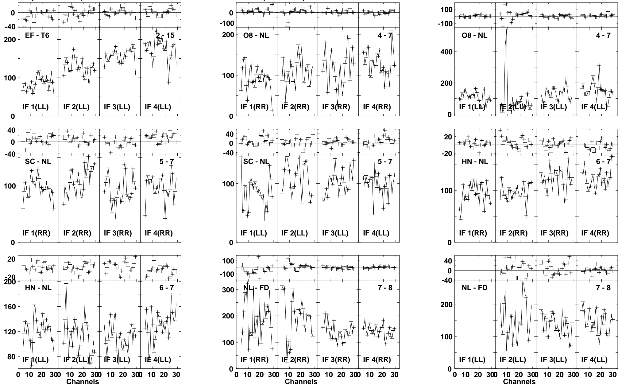
Lower frame: Milli Ampl Jy Top frame: Phas deg Vector averaged cross-power spectrum Baseline: EF (02) - T6 (15) Timerange: 00/23:53:12 to 00/23:55:10
