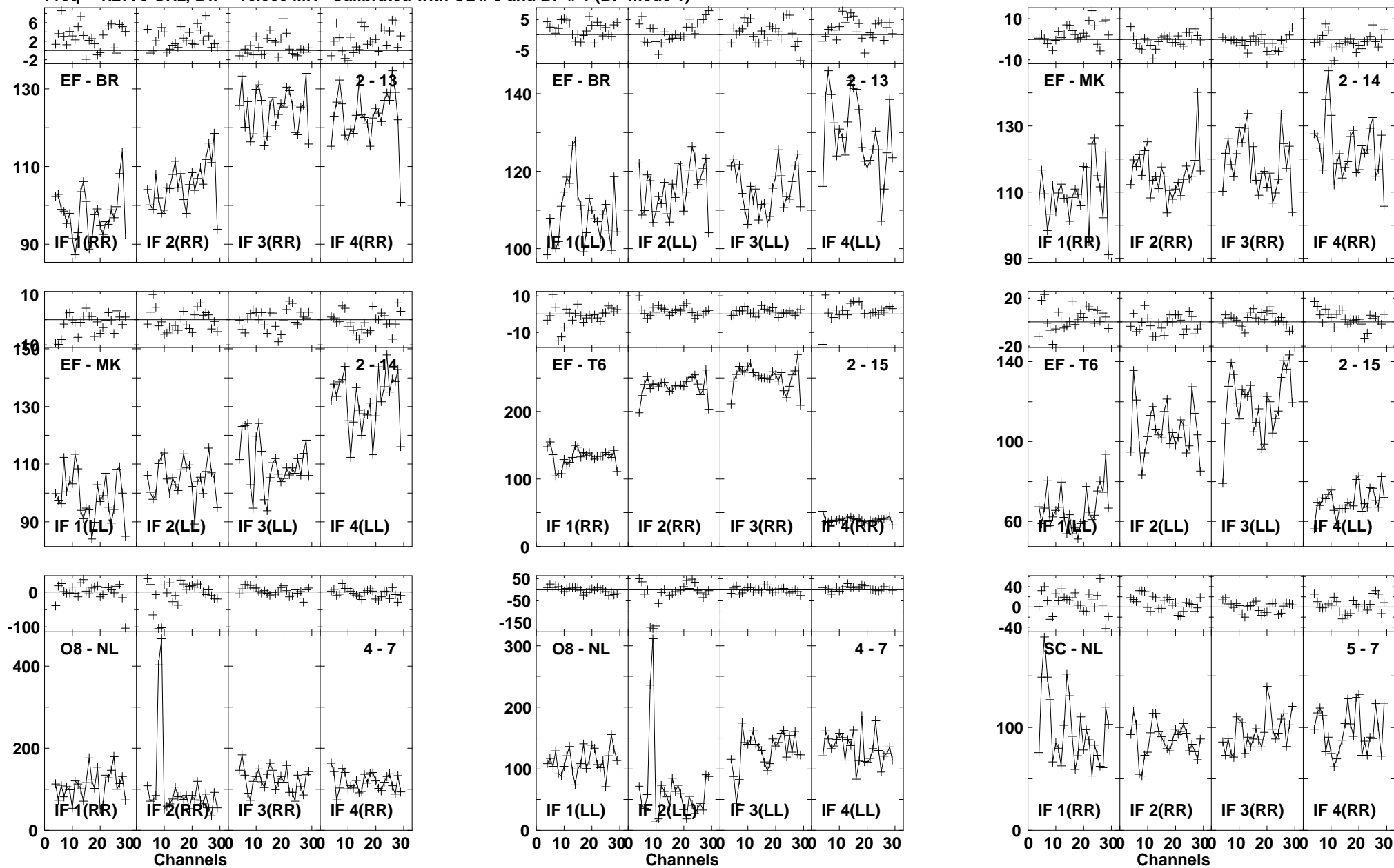
Lower frame: Milli Ampl Jy Top frame: Phas deg Vector averaged cross-power spectrum Baseline: EF (02) - BR (13) Timerange: 00/22:48:42 to 00/22:51:10
