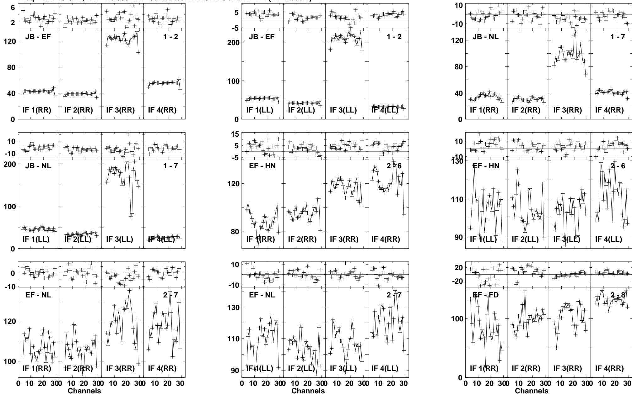
Lower frame: Milli Ampl Jy Top frame: Phas deg Vector averaged cross-power spectrum Baseline: JB (01) - EF (02) Timerange: 01/04:13:25 to 01/04:16:13
