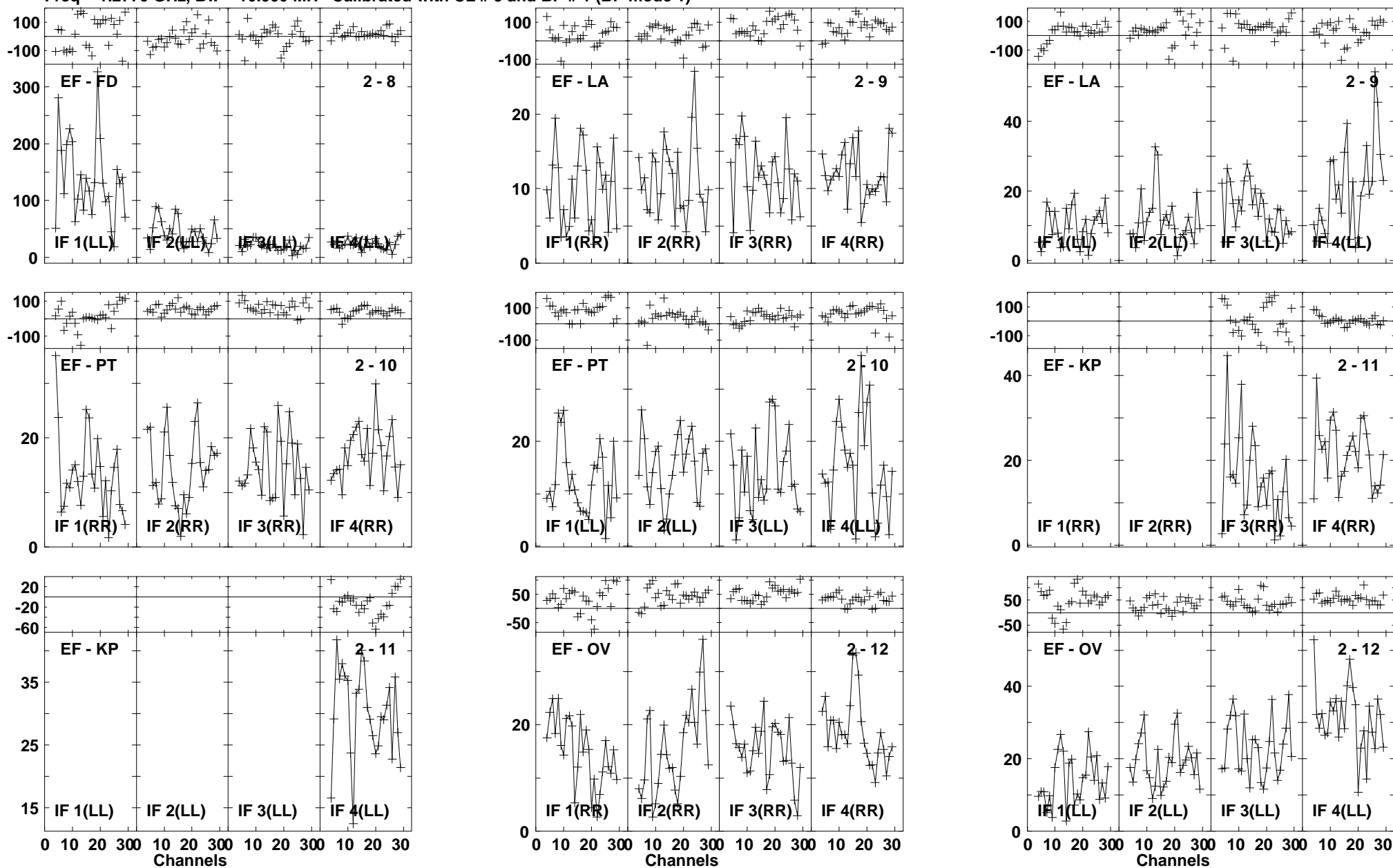
Lower frame: Milli Ampl Jy Top frame: Phas deg Vector averaged cross-power spectrum Baseline: EF (02) - FD (08) Timerange: 01/04:29:15 to 01/04:32:33
