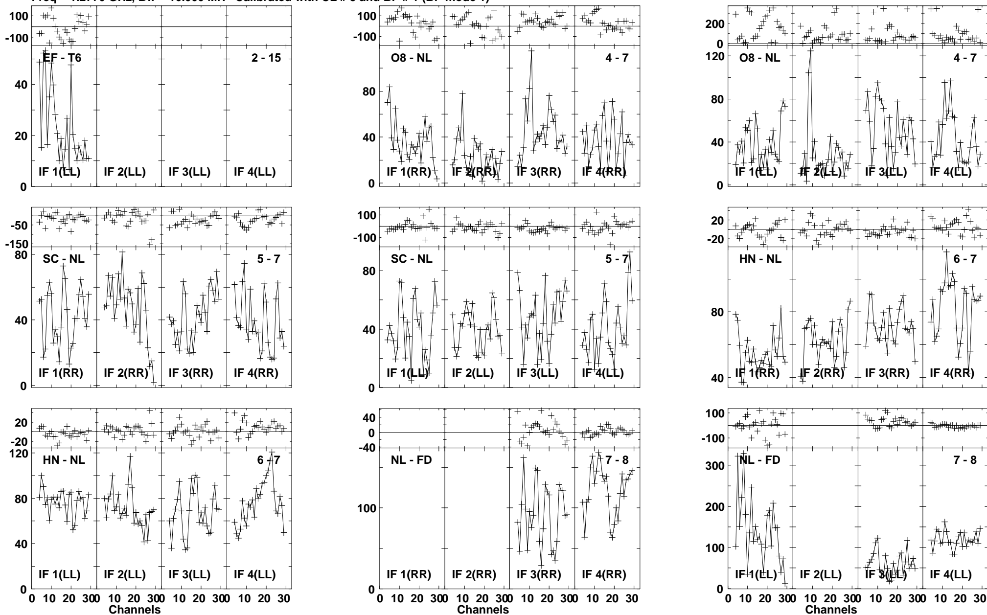
Lower frame: Milli Ampl Jy Top frame: Phas deg Vector averaged cross-power spectrum Baseline: EF (02) - T6 (15) Timerange: 01/00:07:03 to 01/00:10:19
