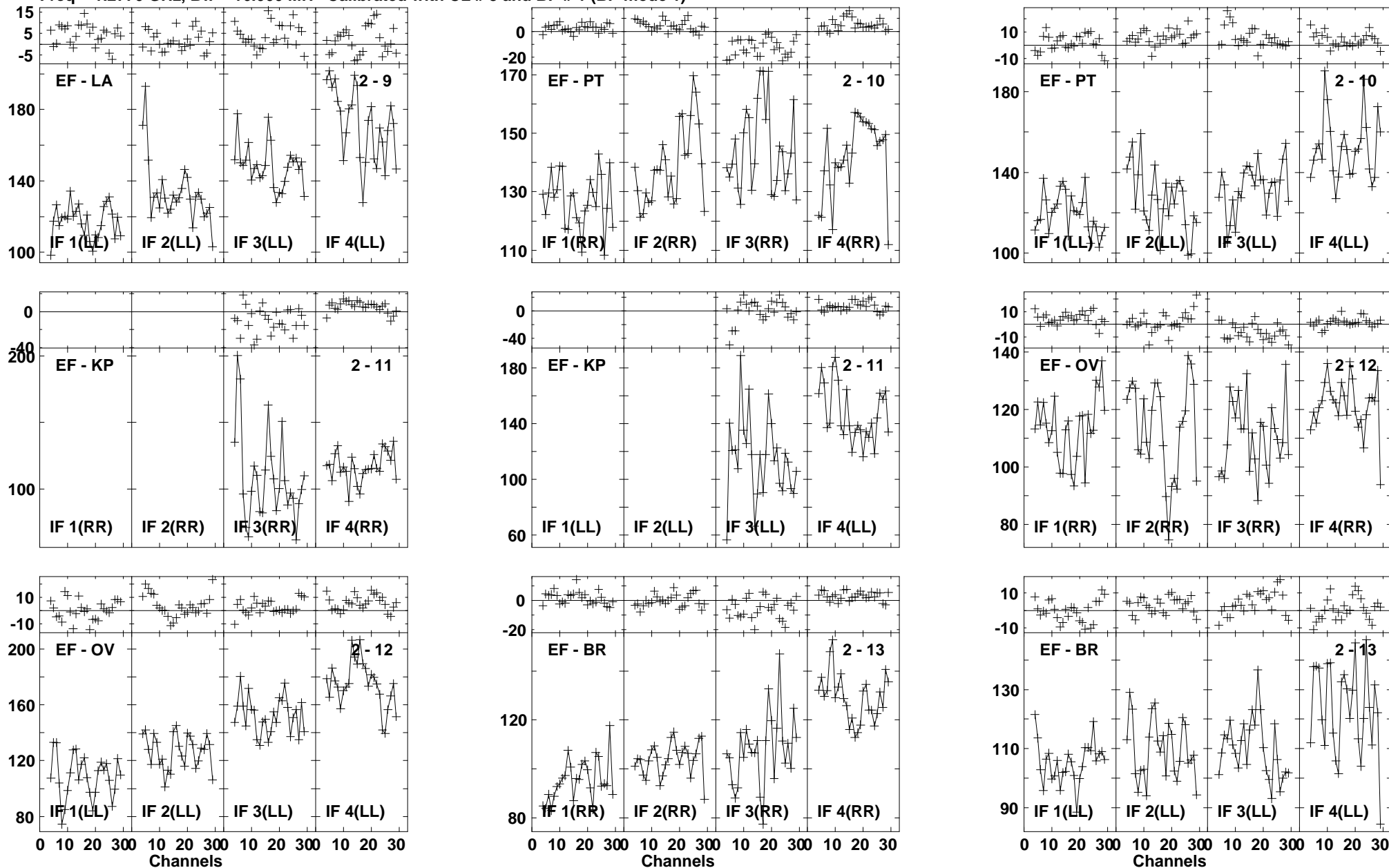
Lower frame: Milli Ampl Jy Top frame: Phas deg Vector averaged cross-power spectrum Baseline: EF (02) - LA (09) Timerange: 01/01:24:10 to 01/01:25:08
