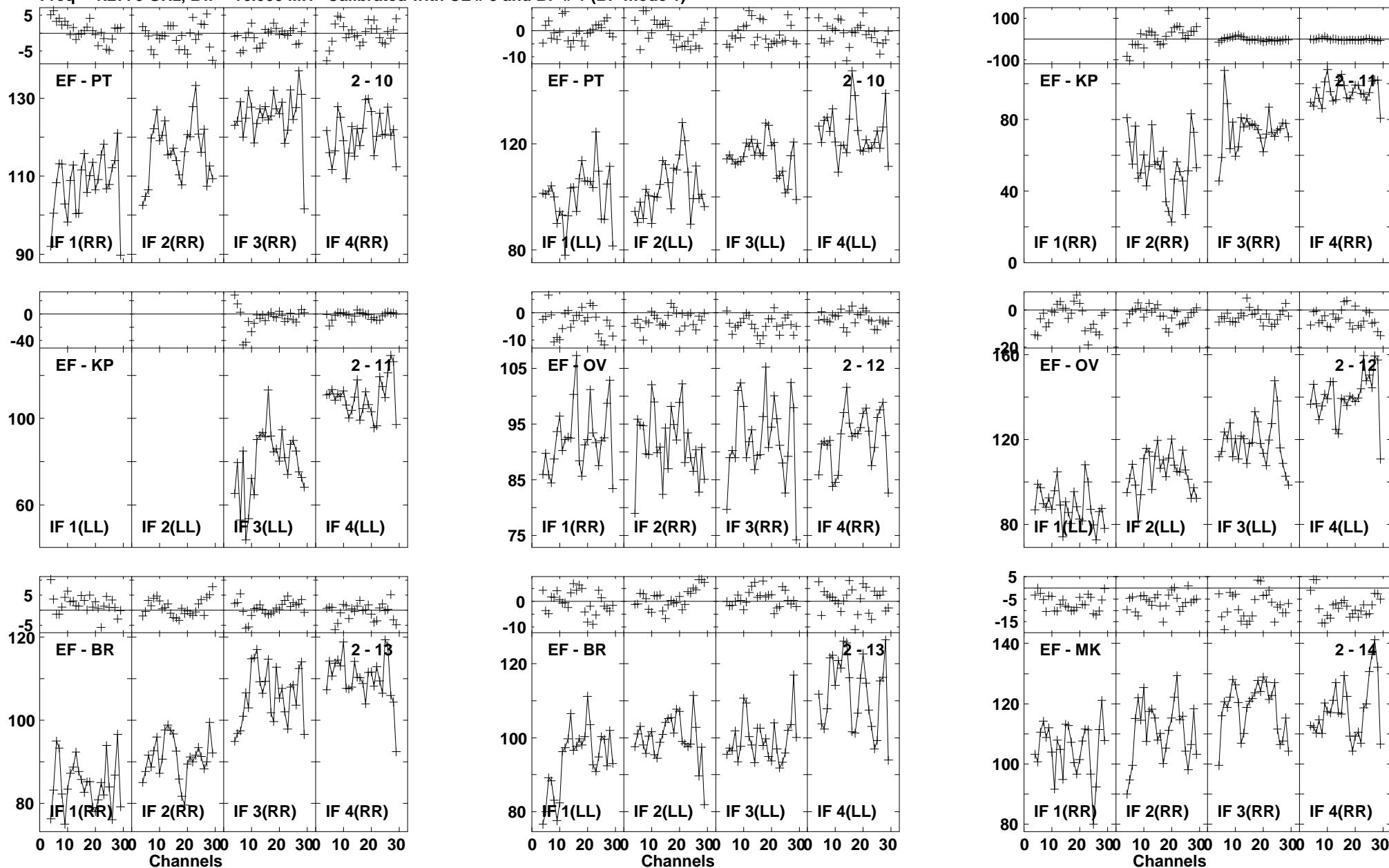
Lower frame: Milli Ampl Jy Top frame: Phas deg Vector averaged cross-power spectrum Baseline: EF (02) - PT (10) Timerange: 00/17:26:58 to 00/17:28:56
