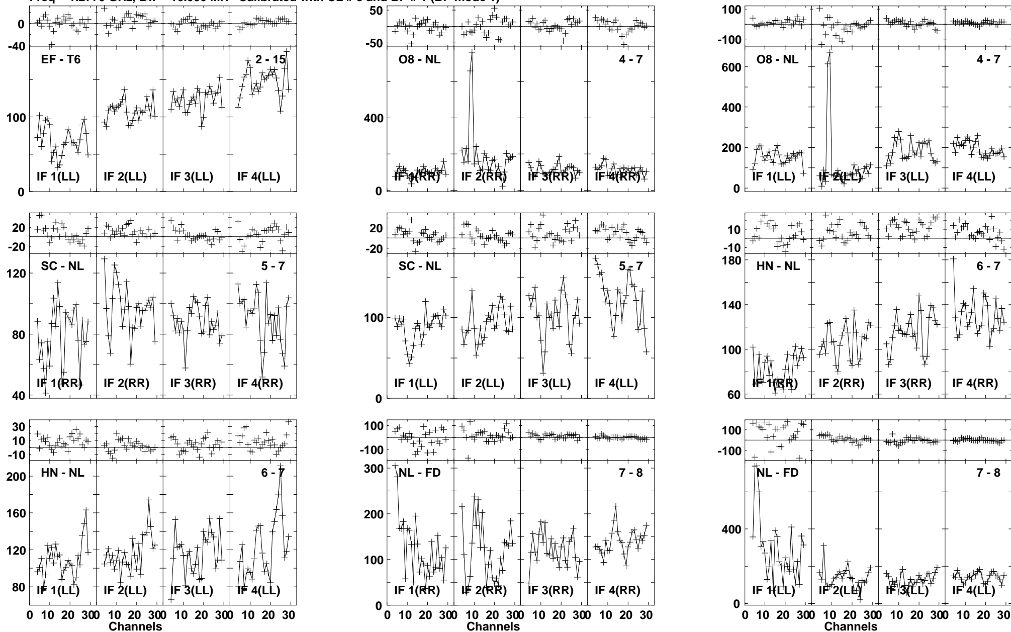
Lower frame: Milli Ampl Jy Top frame: Phas deg Vector averaged cross-power spectrum Baseline: EF (02) - T6 (15) Timerange: 00/23:25:12 to 00/23:27:40
