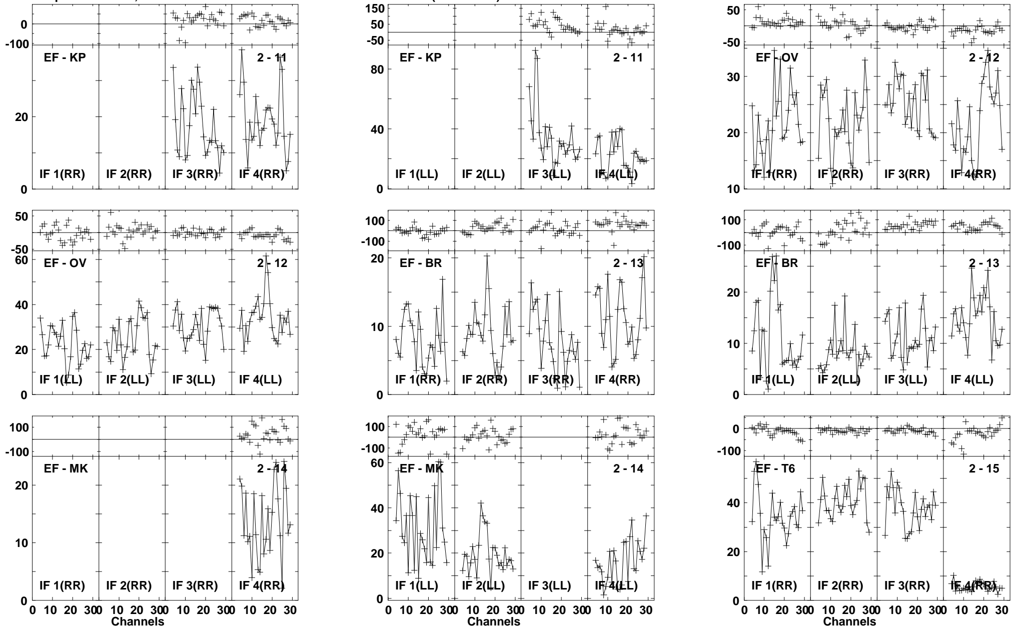
Lower frame: Milli Ampl Jy Top frame: Phas deg Vector averaged cross-power spectrum Baseline: EF (02) - KP (11) Timerange: 01/00:47:15 to 01/00:50:39
