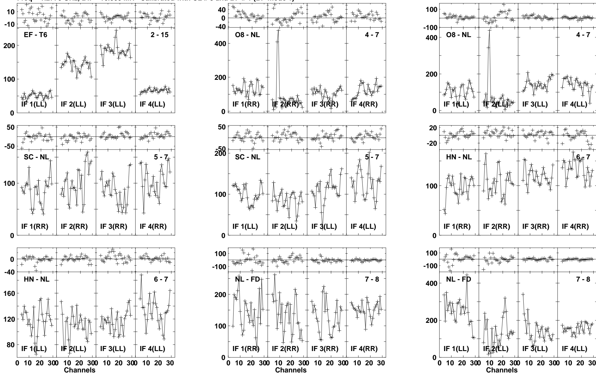
Lower frame: Milli Ampl Jy Top frame: Phas deg Vector averaged cross-power spectrum Baseline: EF (02) - T6 (15) Timerange: 01/00:16:32 to 01/00:18:30
