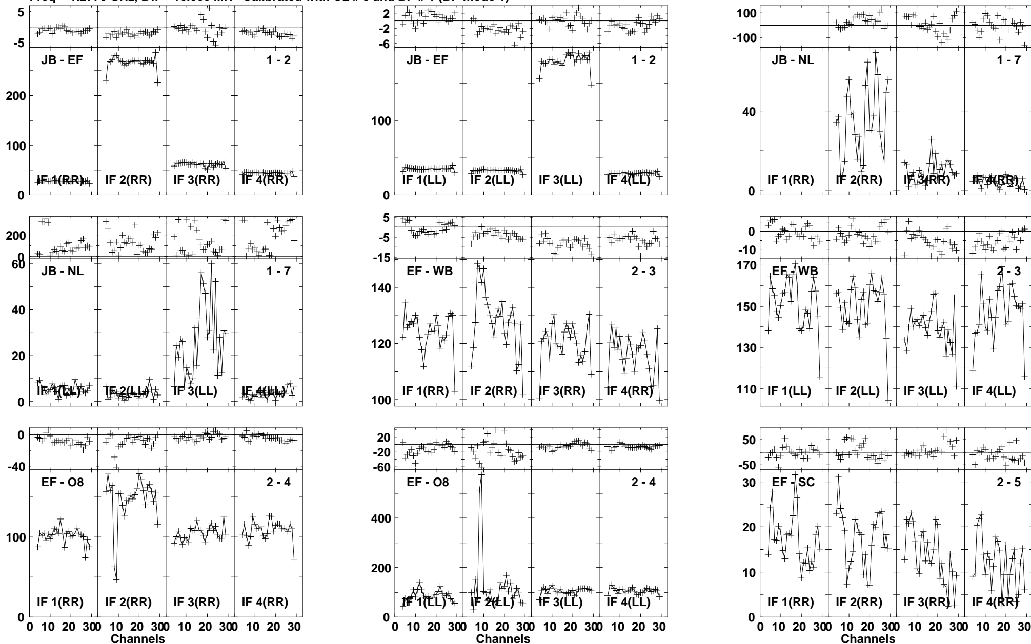
Lower frame: Milli Ampl Jy Top frame: Phas deg Vector averaged cross-power spectrum Baseline: JB (01) - EF (02) Timerange: 00/17:23:11 to 00/17:26:05
