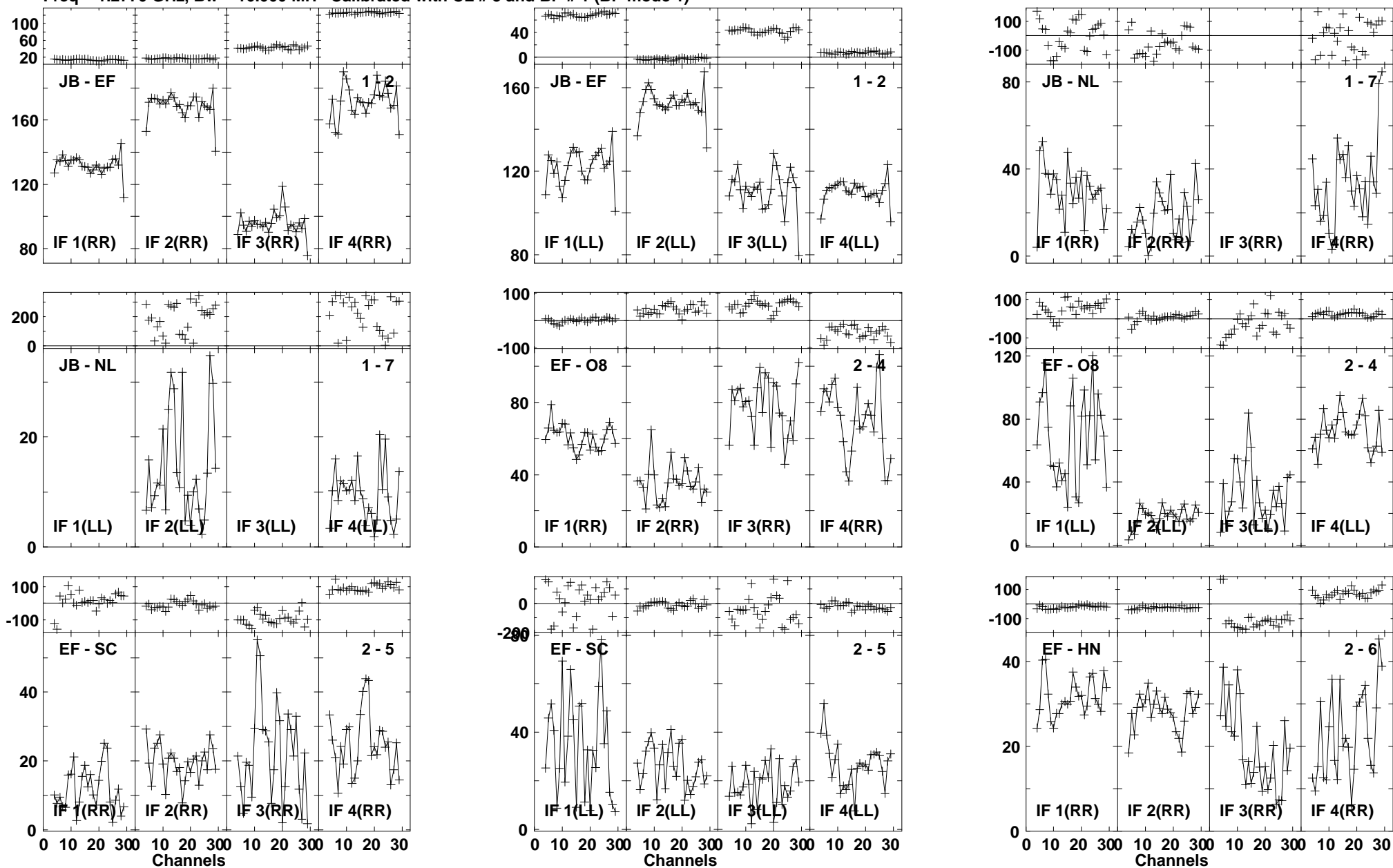
Lower frame: Milli Ampl Jy Top frame: Phas deg Vector averaged cross-power spectrum Baseline: JB (01) - EF (02) Timerange: 00/22:20:02 to 00/22:23:30
