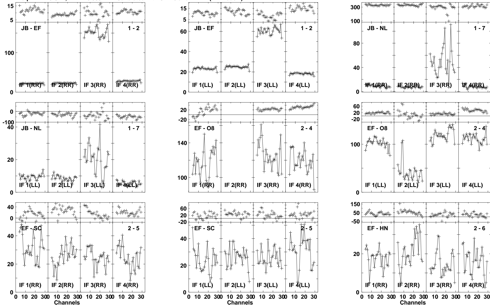
Lower frame: Milli Ampl Jy Top frame: Phas deg Vector averaged cross-power spectrum Baseline: JB (01) - EF (02) Timerange: 00/23:33:05 to 00/23:36:29
