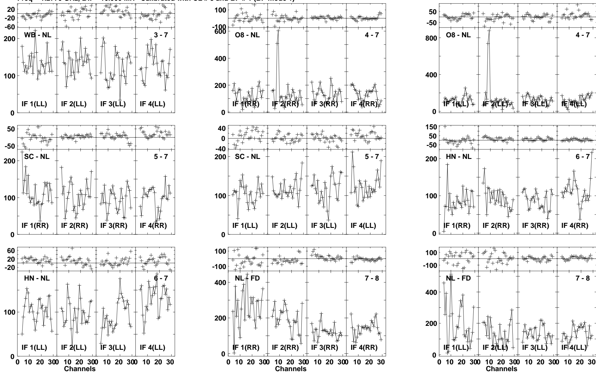
Lower frame: Milli Ampl Jy Top frame: Phas deg Vector averaged cross-power spectrum Baseline: WB (03) - NL (07) Timerange: 00/15:52:21 to 00/15:53:19
