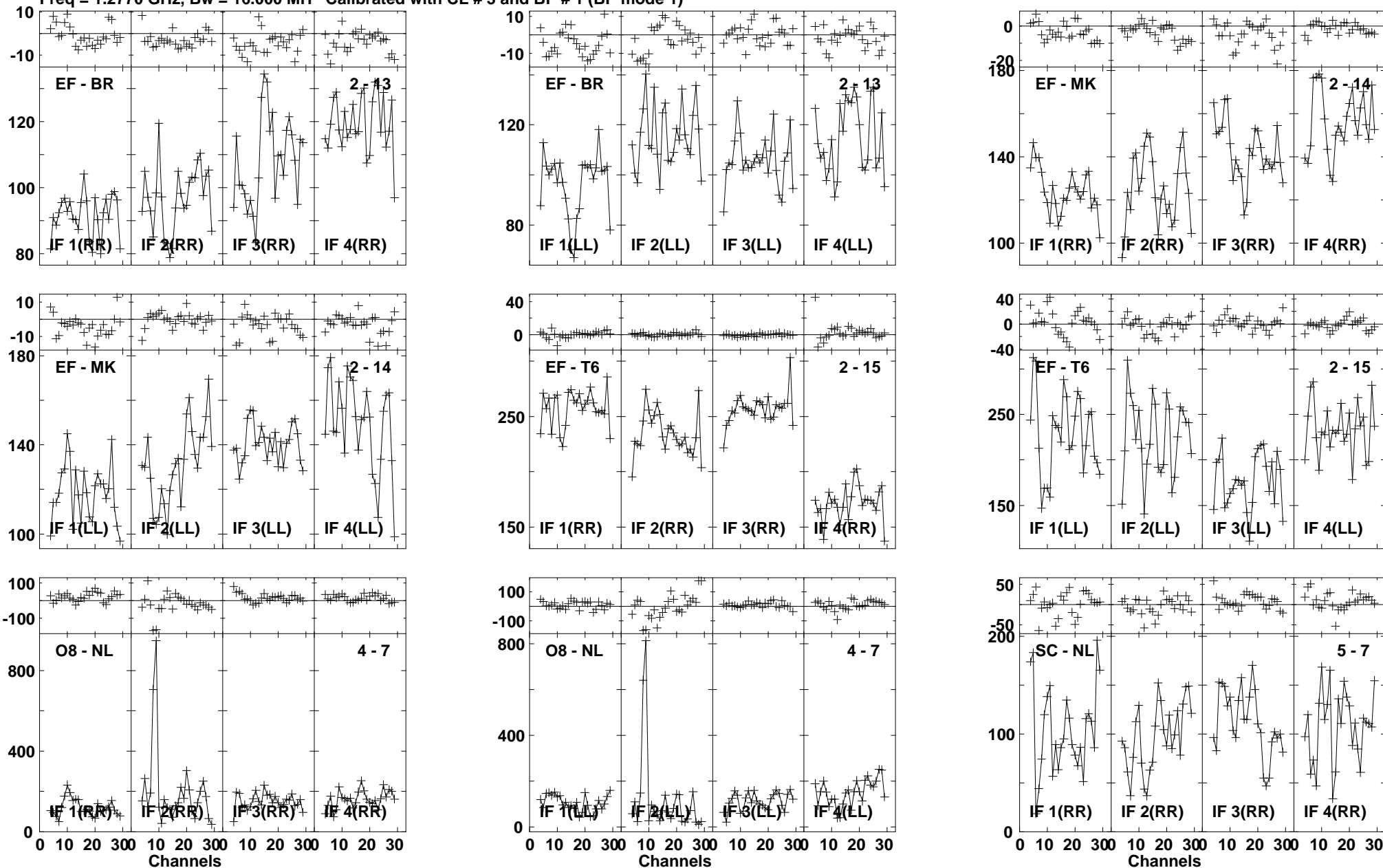
Lower frame: Milli Ampl Jy Top frame: Phas deg Vector averaged cross-power spectrum Baseline: EF (02) - BR (13) Timerange: 01/00:34:32 to 01/00:35:30
