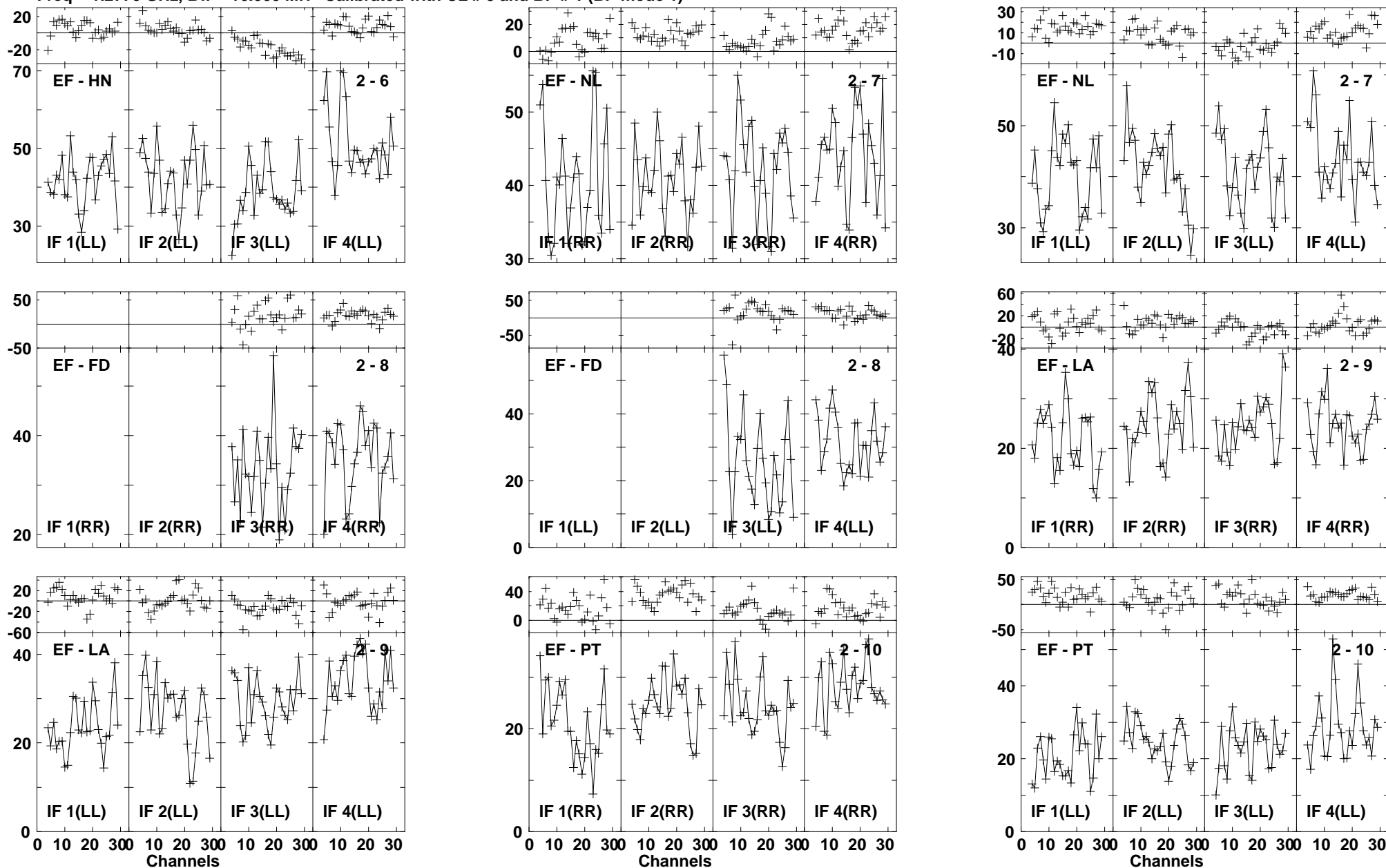
Lower frame: Milli Ampl Jy Top frame: Phas deg Vector averaged cross-power spectrum Baseline: EF (02) - HN (06) Timerange: 00/22:44:25 to 00/22:47:49
