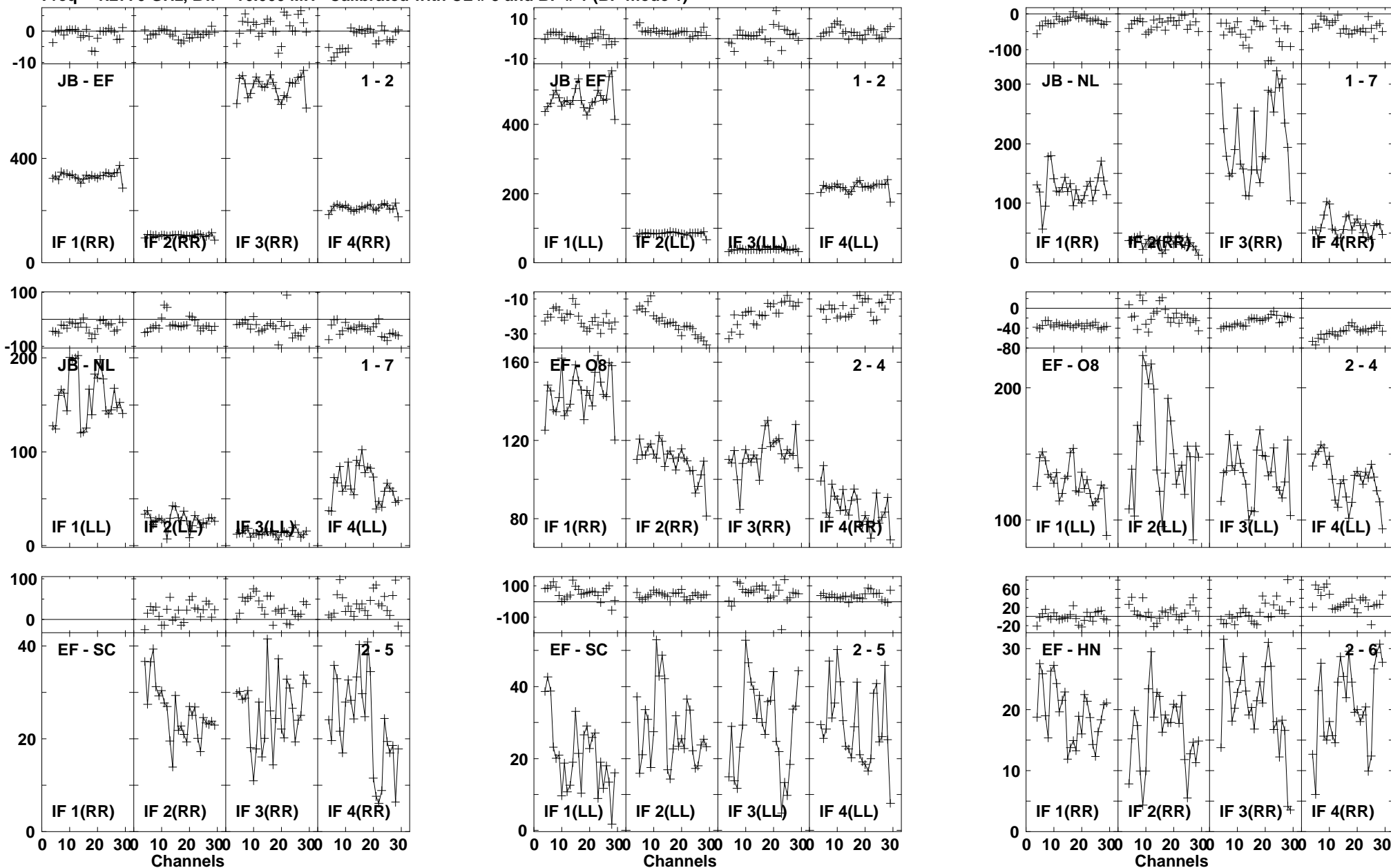
Lower frame: Milli Ampl Jy Top frame: Phas deg Vector averaged cross-power spectrum Baseline: JB (01) - EF (02) Timerange: 01/01:47:33 to 01/01:50:57
