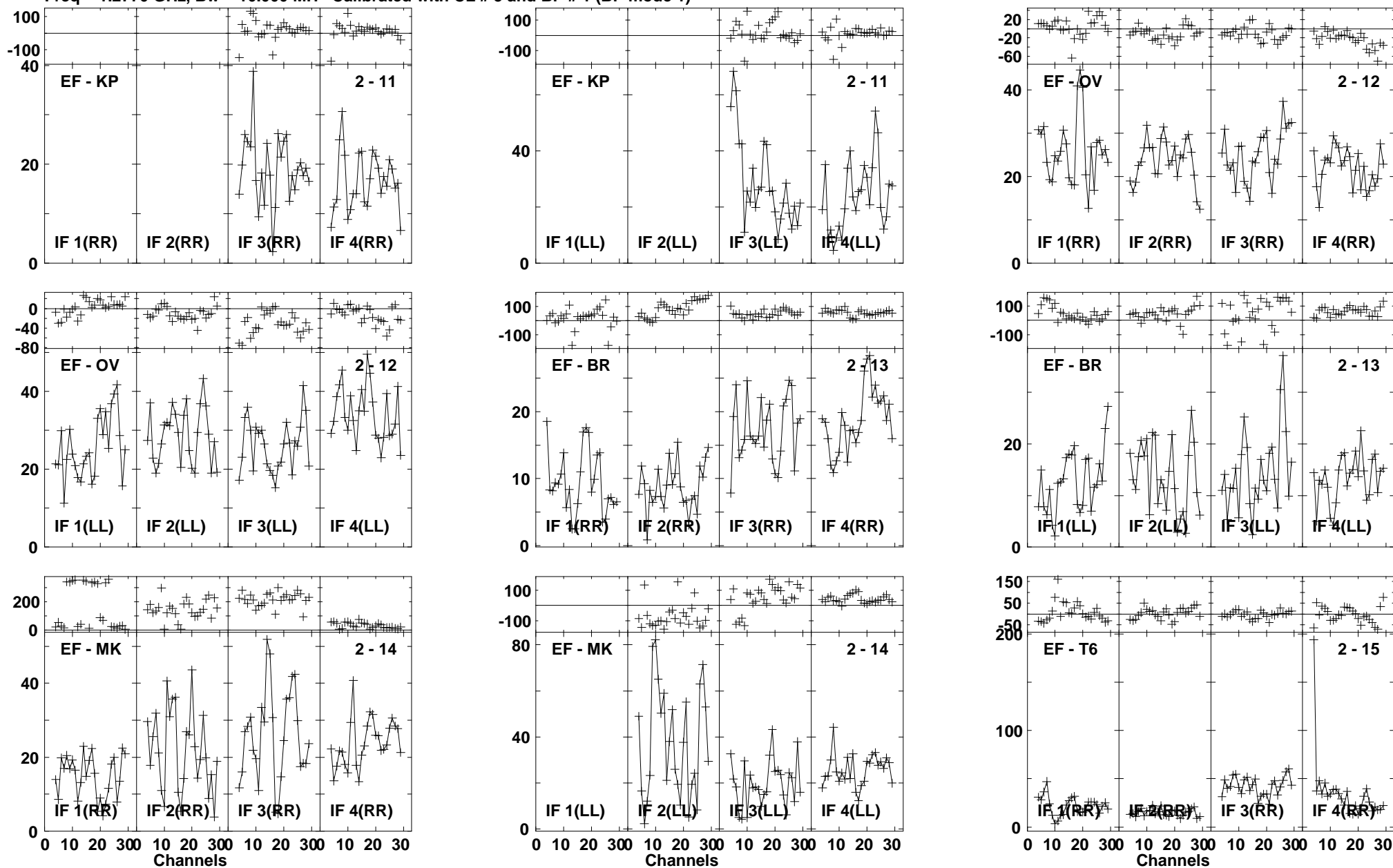
Lower frame: Milli Ampl Jy Top frame: Phas deg Vector averaged cross-power spectrum Baseline: EF (02) - KP (11) Timerange: 01/00:58:55 to 01/01:02:19
