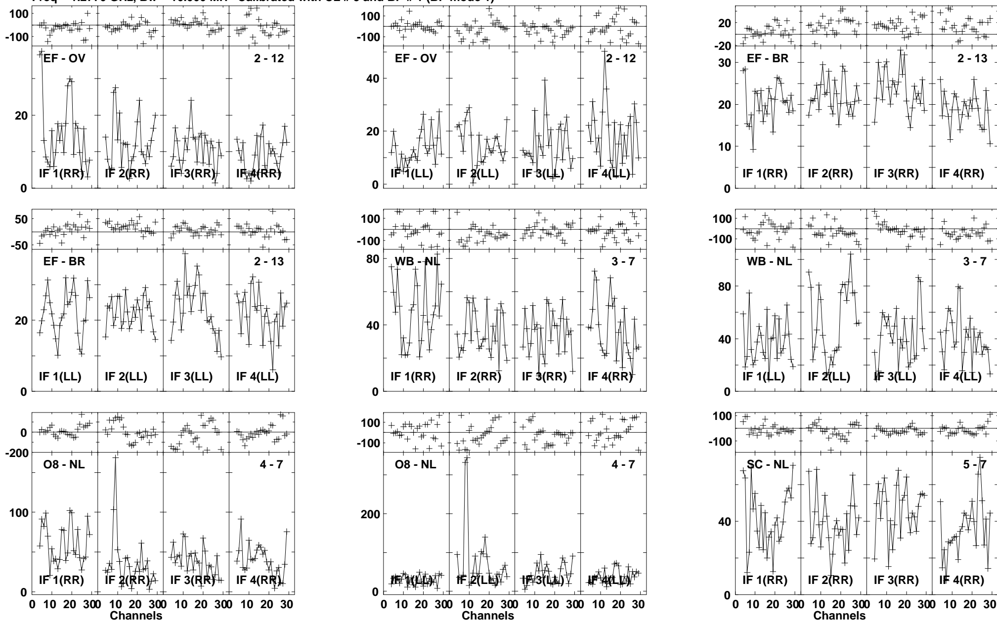
Lower frame: Milli Ampl Jy Top frame: Phas deg Vector averaged cross-power spectrum Baseline: EF (02) - OV (12) Timerange: 00/15:48:42 to 00/15:51:28
