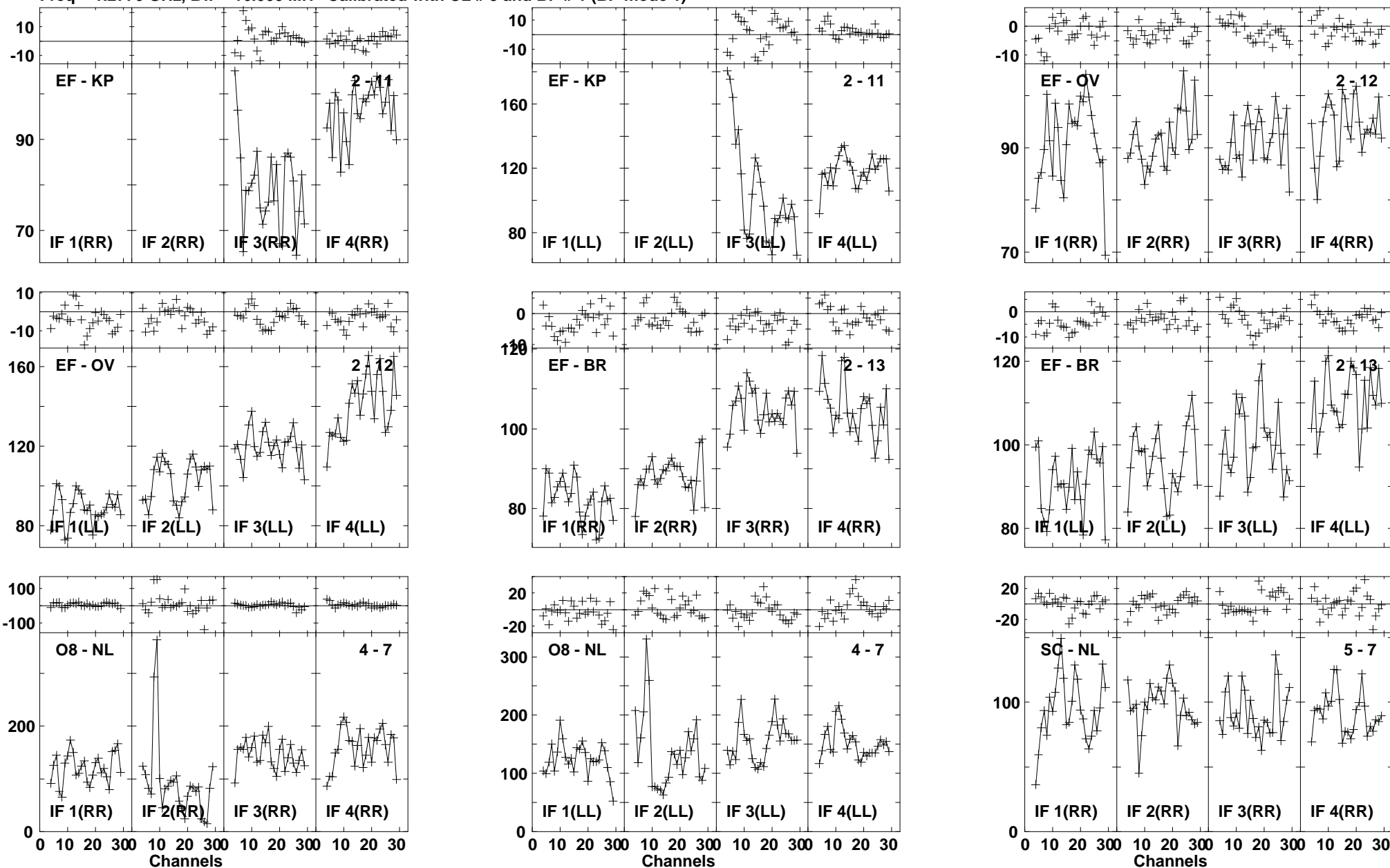
Lower frame: Milli Ampl Jy Top frame: Phas deg Vector averaged cross-power spectrum Baseline: EF (02) - KP (11) Timerange: 00/21:30:28 to 00/21:32:56
