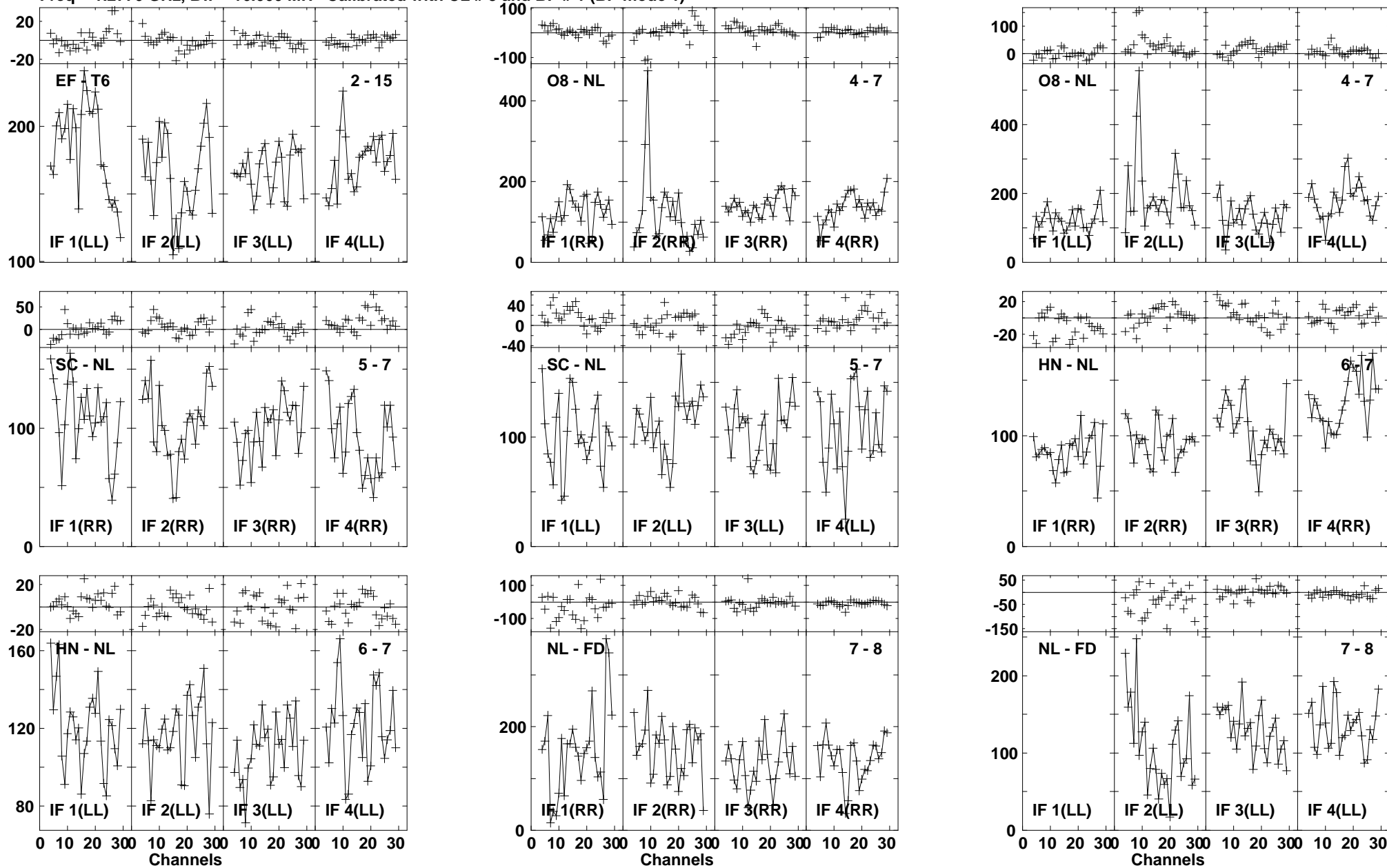
Lower frame: Milli Ampl Jy Top frame: Phas deg Vector averaged cross-power spectrum Baseline: EF (02) - T6 (15) Timerange: 01/01:40:40 to 01/01:42:38
