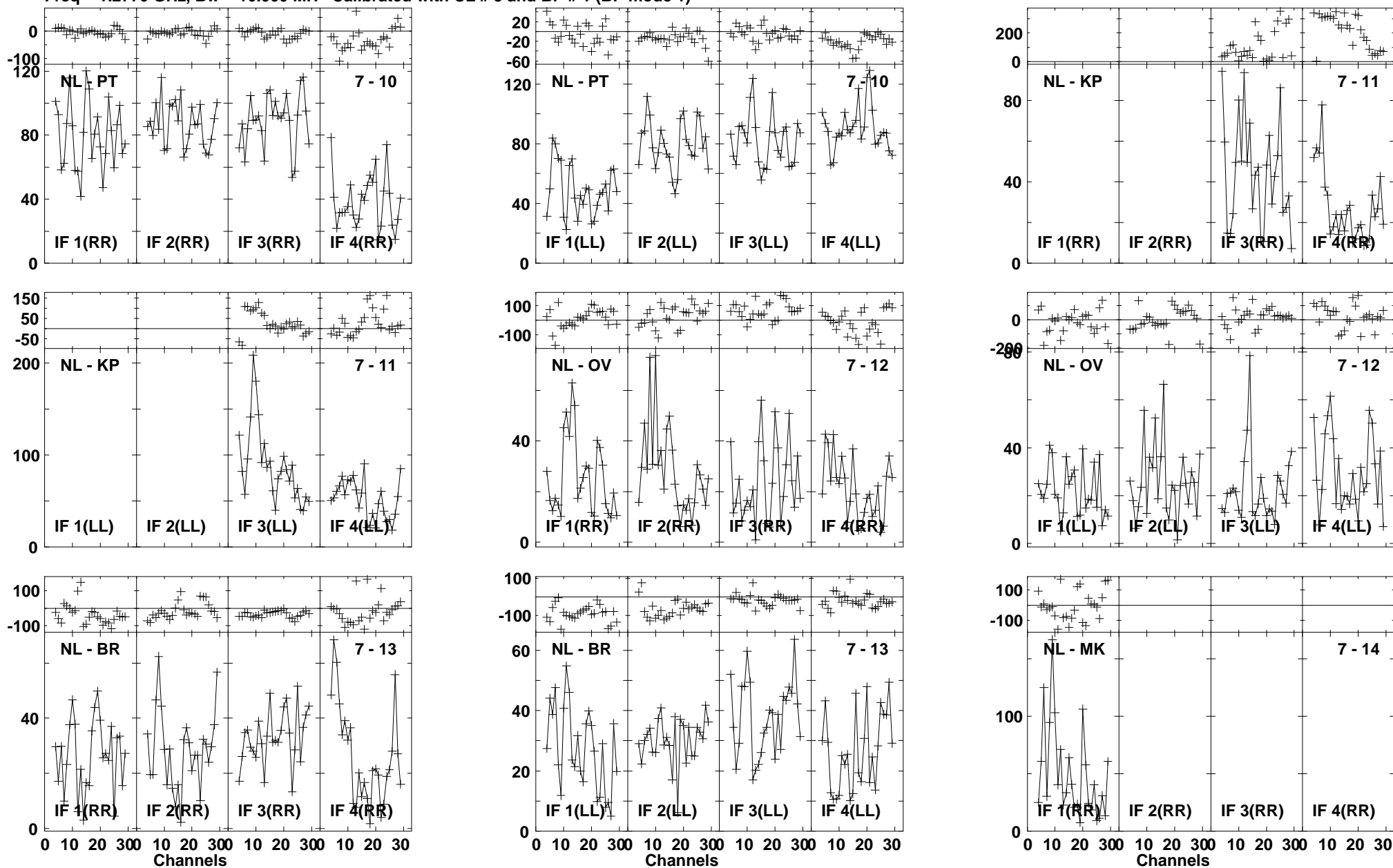
Lower frame: Milli Ampl Jy Top frame: Phas deg Vector averaged cross-power spectrum Baseline: NL (07) - PT (10) Timerange: 00/23:49:03 to 00/23:52:19
