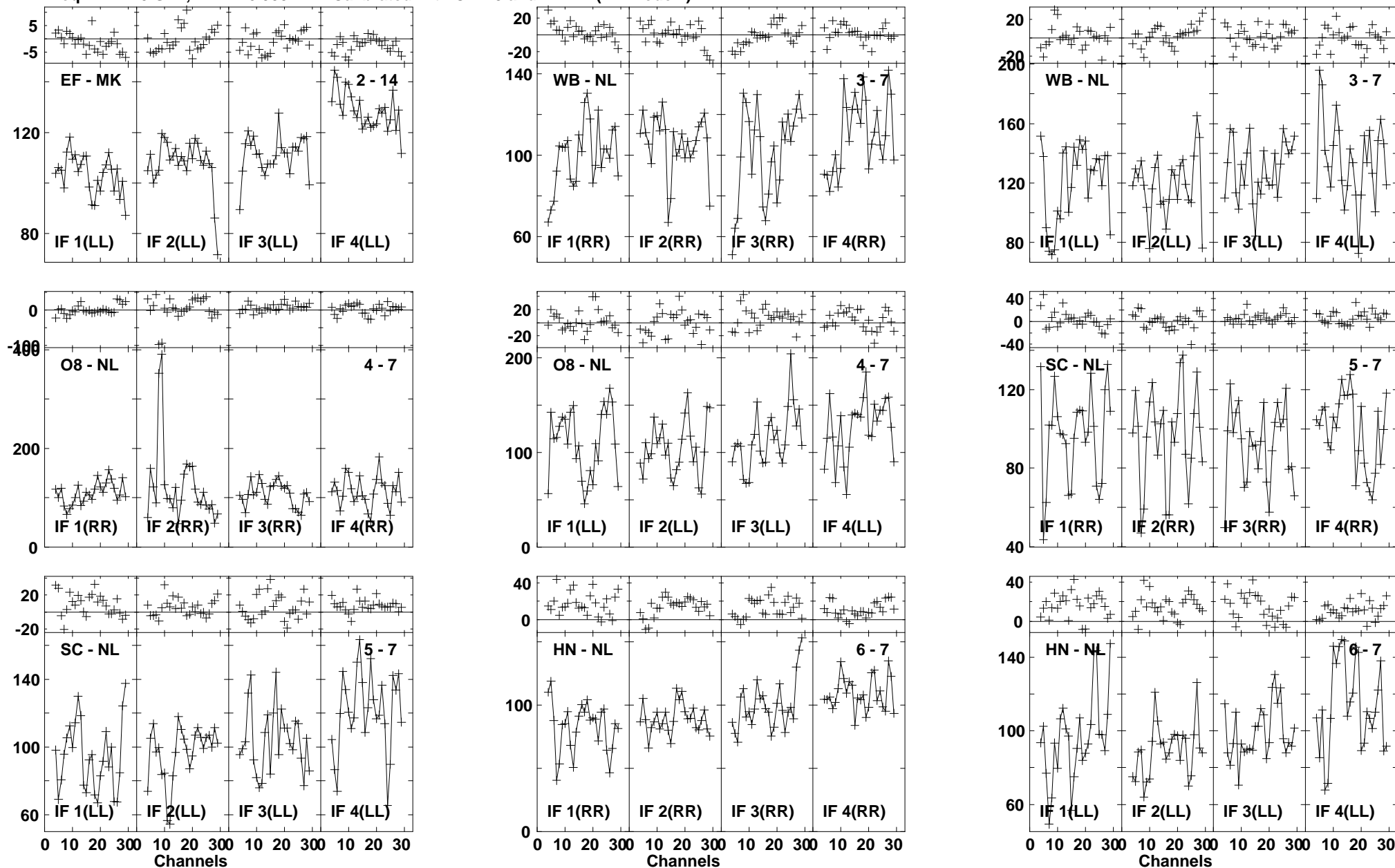
Lower frame: Milli Ampl Jy Top frame: Phas deg Vector averaged cross-power spectrum Baseline: EF (02) - MK (14) Timerange: 00/19:26:46 to 00/19:29:34
