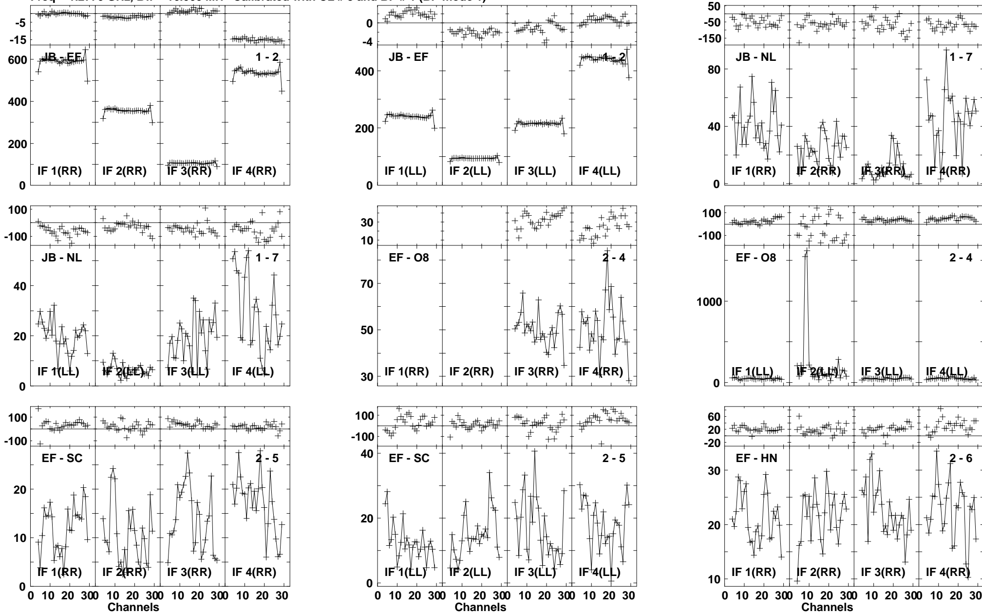
Lower frame: Milli Ampl Jy Top frame: Phas deg Vector averaged cross-power spectrum Baseline: JB (01) - EF (02) Timerange: 00/20:18:18 to 00/20:21:04
