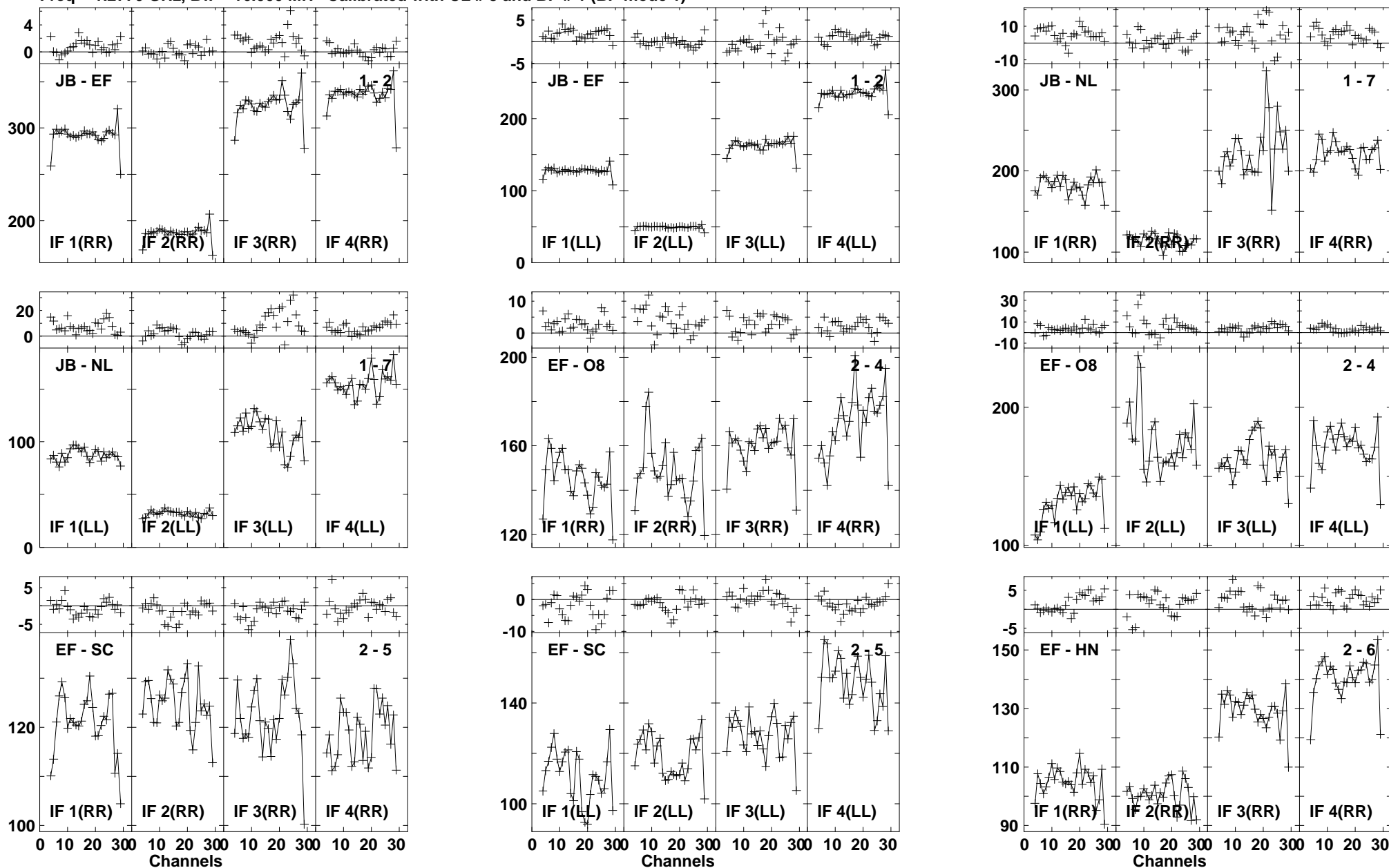
Lower frame: Milli Ampl Jy Top frame: Phas deg Vector averaged cross-power spectrum Baseline: JB (01) - EF (02) Timerange: 00/20:45:58 to 00/20:48:46
