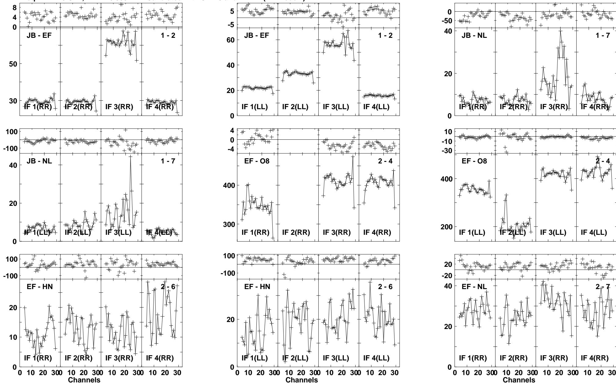
Lower frame: Milli Ampl Jy Top frame: Phas deg Vector averaged cross-power spectrum Baseline: JB (01) - EF (02) Timerange: 01/02:46:40 to 01/02:49:54
