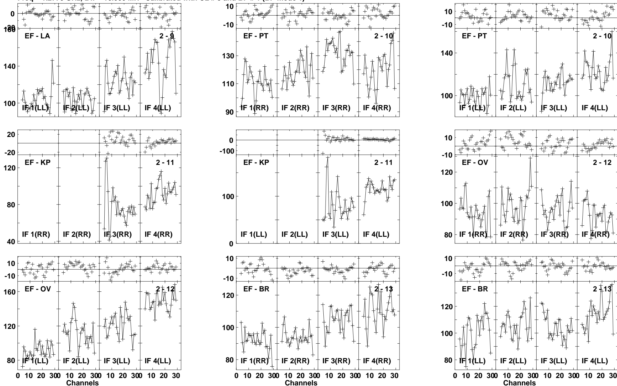
Lower frame: Milli Ampl Jy Top frame: Phas deg Vector averaged cross-power spectrum Baseline: EF (02) - LA (09) Timerange: 01/05:11:55 to 01/05:13:13
