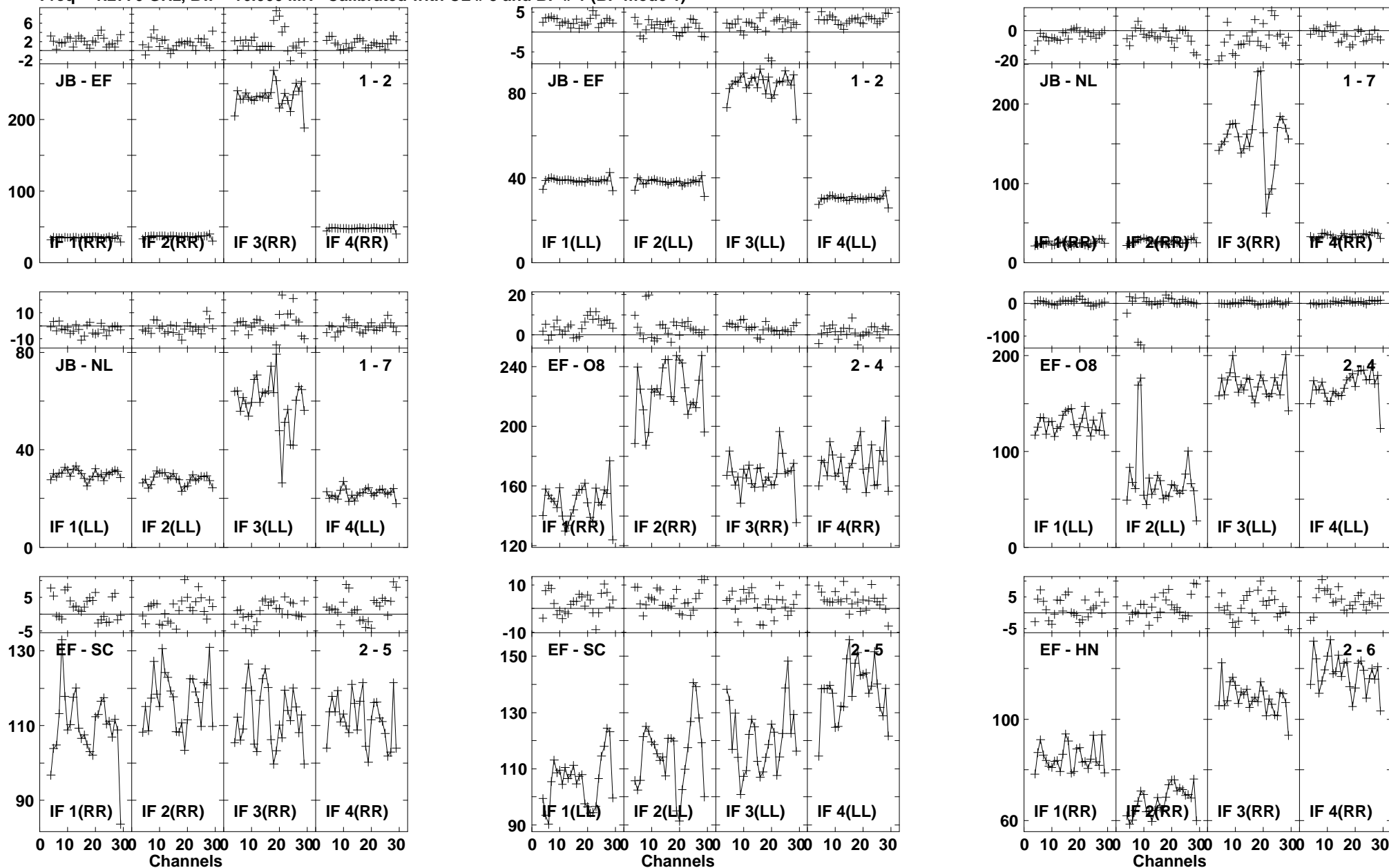
Lower frame: Milli Ampl Jy Top frame: Phas deg Vector averaged cross-power spectrum Baseline: JB (01) - EF (02) Timerange: 00/23:37:22 to 00/23:39:50
