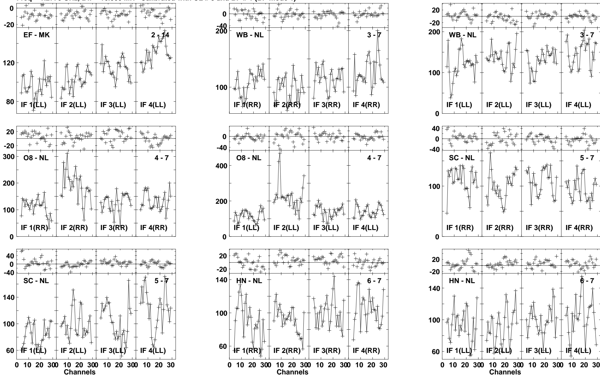
Lower frame: Milli Ampl Jy Top frame: Phas deg Vector averaged cross-power spectrum Baseline: EF (02) - MK (14) Timerange: 00/17:26:58 to 00/17:28:56
