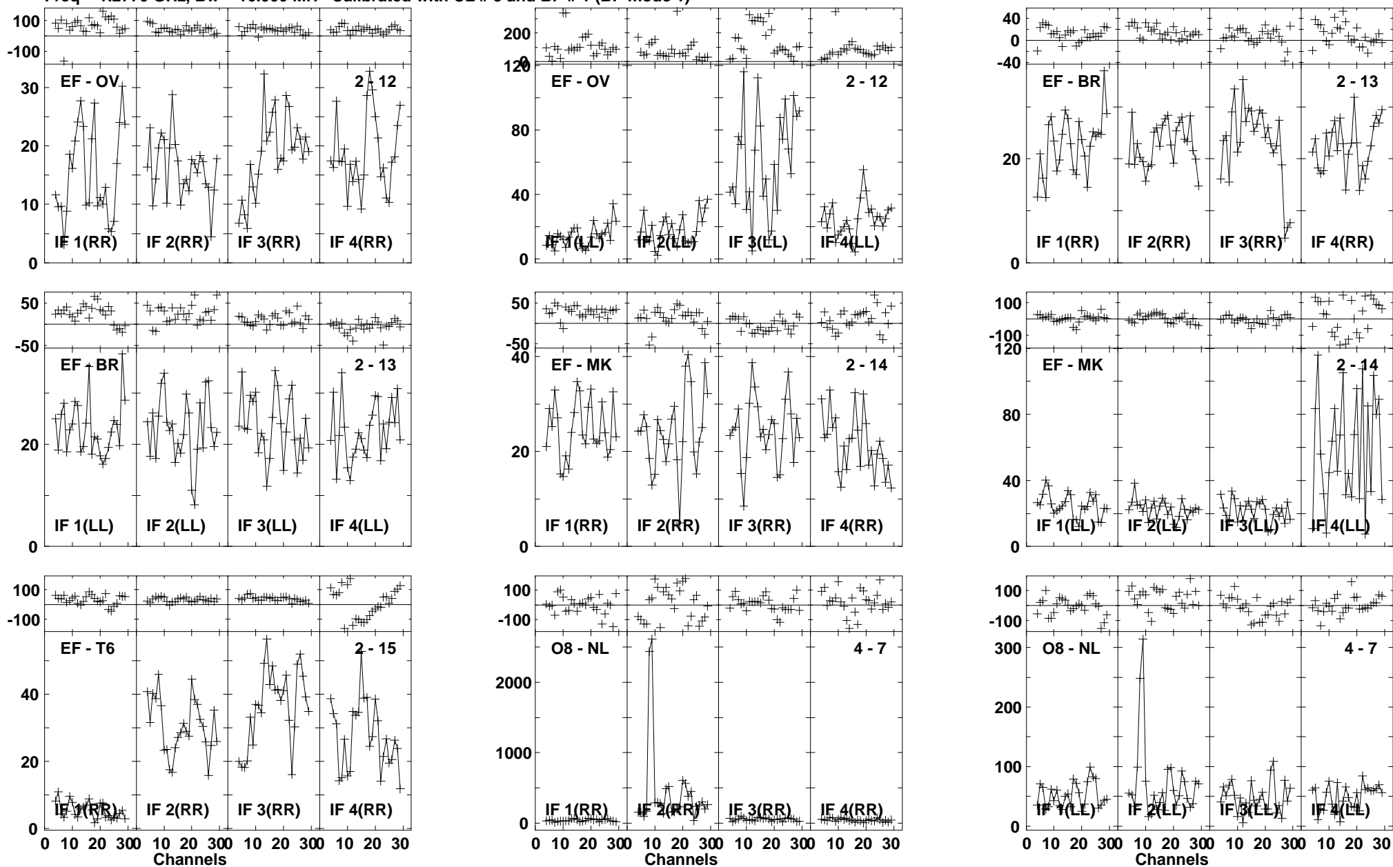
Lower frame: Milli Ampl Jy Top frame: Phas deg Vector averaged cross-power spectrum Baseline: EF (02) - OV (12) Timerange: 01/03:25:57 to 01/03:28:45
