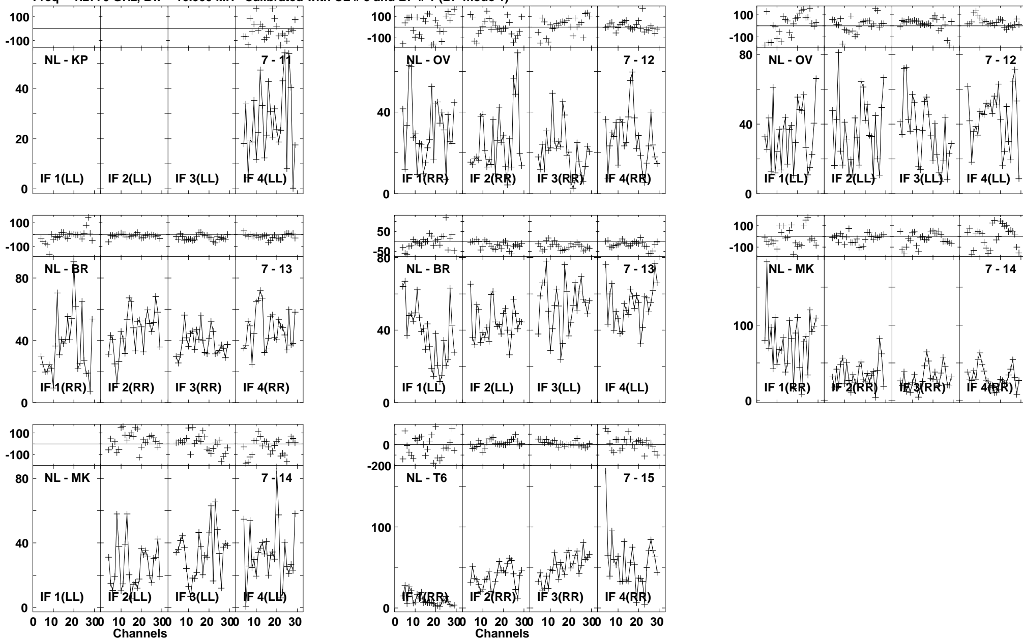
Lower frame: Milli Ampl Jy Top frame: Phas deg Vector averaged cross-power spectrum Baseline: NL (07) - KP (11) Timerange: 00/22:39:13 to 00/22:42:29
