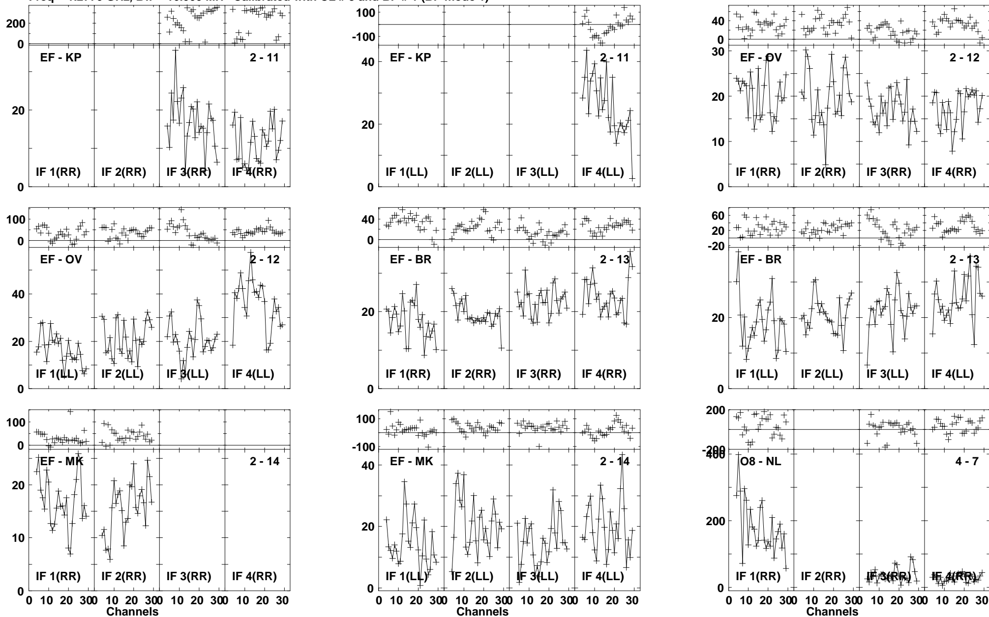
Lower frame: Milli Ampl Jy Top frame: Phas deg Vector averaged cross-power spectrum Baseline: EF (02) - KP (11) Timerange: 00/20:12:19 to 00/20:15:13
