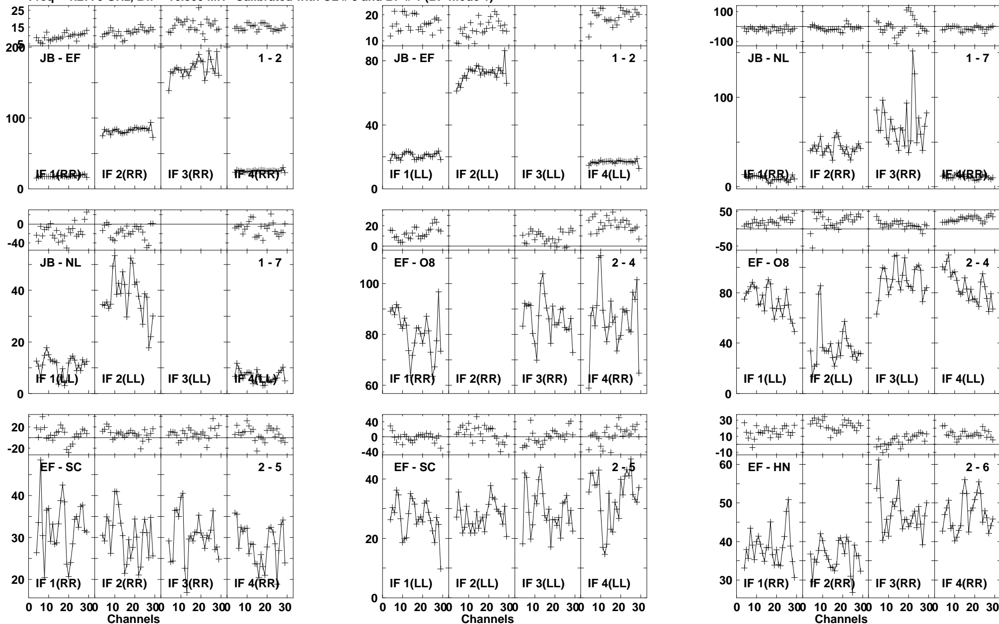
Lower frame: Milli Ampl Jy Top frame: Phas deg Vector averaged cross-power spectrum Baseline: JB (01) - EF (02) Timerange: 00/22:44:25 to 00/22:47:49
