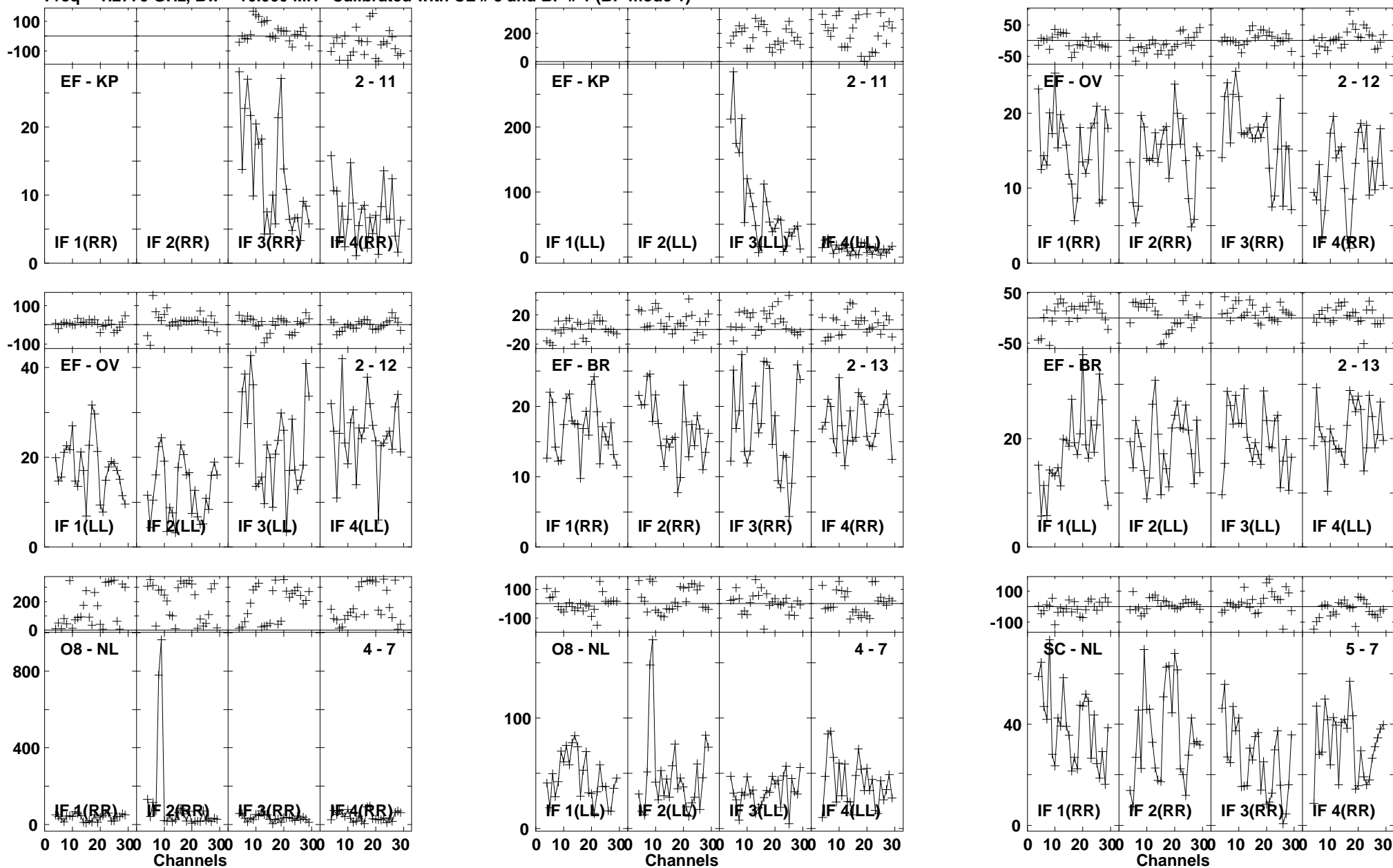
Lower frame: Milli Ampl Jy Top frame: Phas deg Vector averaged cross-power spectrum Baseline: EF (02) - KP (11) Timerange: 00/21:26:21 to 00/21:29:35
