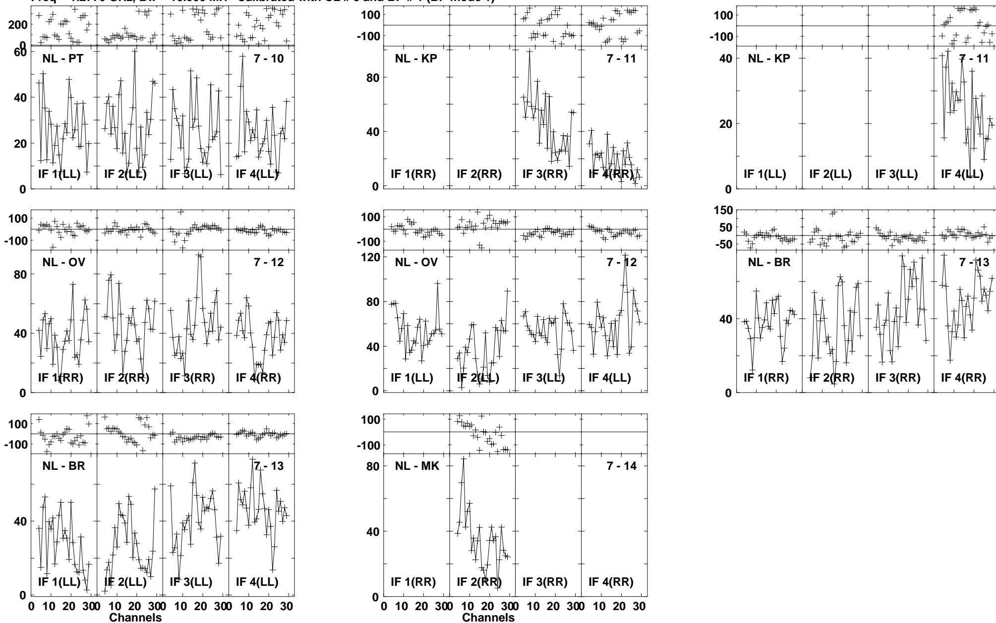
Lower frame: Milli Ampl Jy Top frame: Phas deg Vector averaged cross-power spectrum Baseline: NL (07) - PT (10) Timerange: 00/21:01:21 to 00/21:04:35
