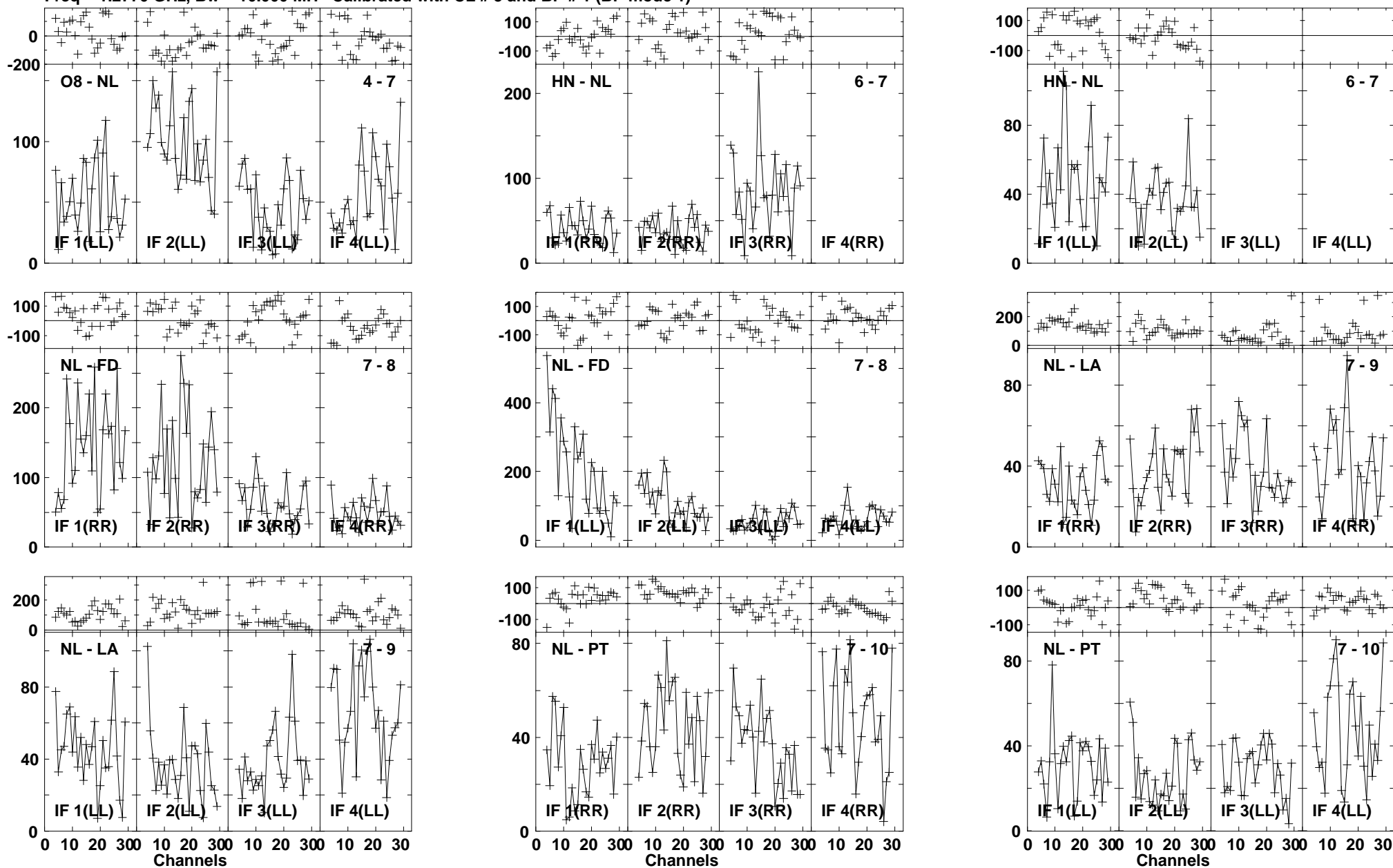
Lower frame: Milli Ampl Jy Top frame: Phas deg Vector averaged cross-power spectrum Baseline: O8 (04) - NL (07) Timerange: 01/04:54:55 to 01/04:58:13
