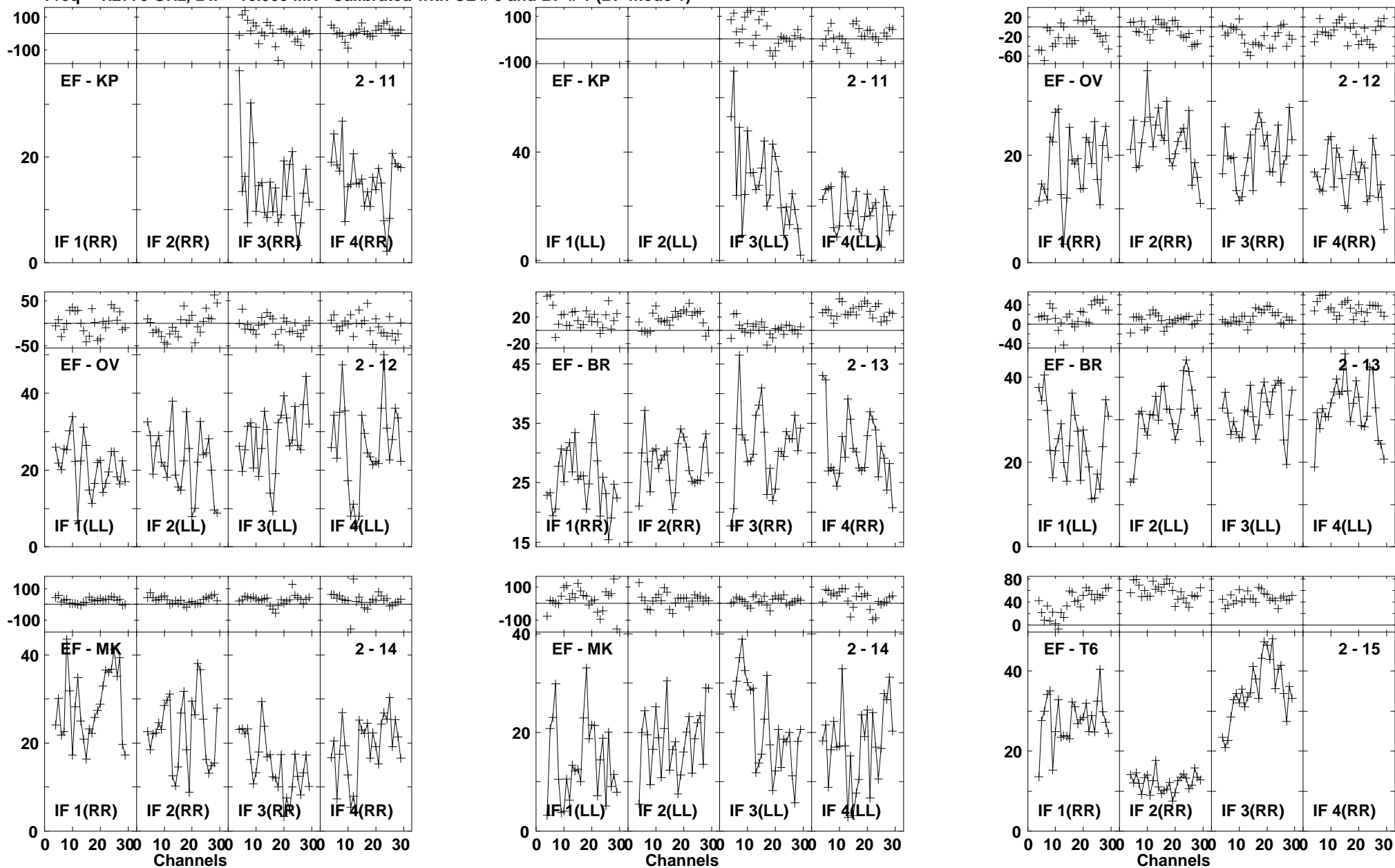
Lower frame: Milli Ampl Jy Top frame: Phas deg Vector averaged cross-power spectrum Baseline: EF (02) - KP (11) Timerange: 01/01:31:32 to 01/01:34:28
