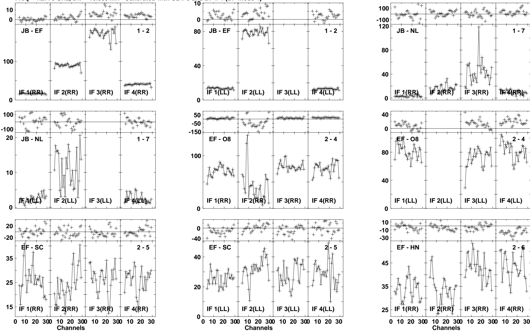
Lower frame: Milli Ampl Jy Top frame: Phas deg Vector averaged cross-power spectrum Baseline: JB (01) - EF (02) Timerange: 00/22:32:15 to 00/22:35:39
