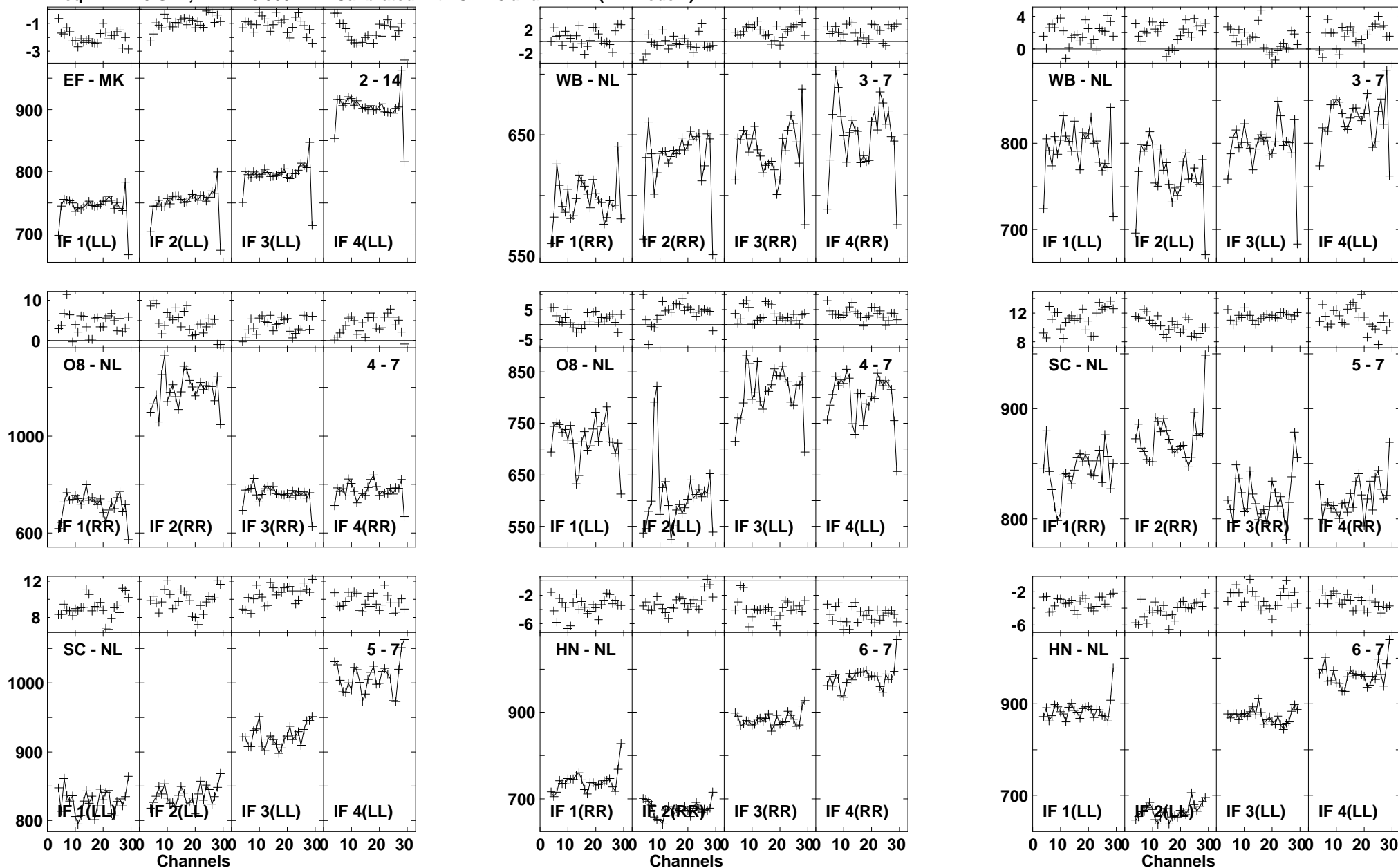
Lower frame: Milli Ampl Jy Top frame: Phas deg Vector averaged cross-power spectrum Baseline: EF (02) - MK (14) Timerange: 00/19:21:33 to 00/19:25:21
