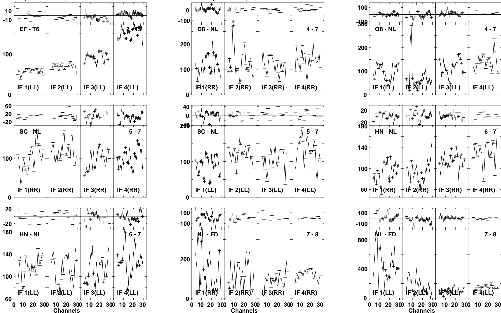
Lower frame: Milli Ampl Jy Top frame: Phas deg Vector averaged cross-power spectrum Baseline: EF (02) - T6 (15) Timerange: 01/00:51:32 to 01/00:53:30
