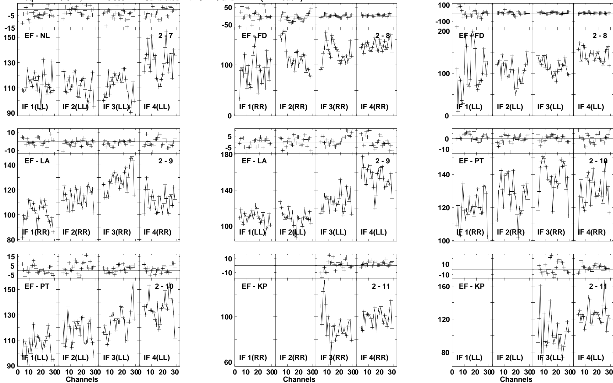
Lower frame: Milli Ampl Jy Top frame: Phas deg Vector averaged cross-power spectrum Baseline: EF (02) - NL (07) Timerange: 01/02:39:47 to 01/02:41:45
