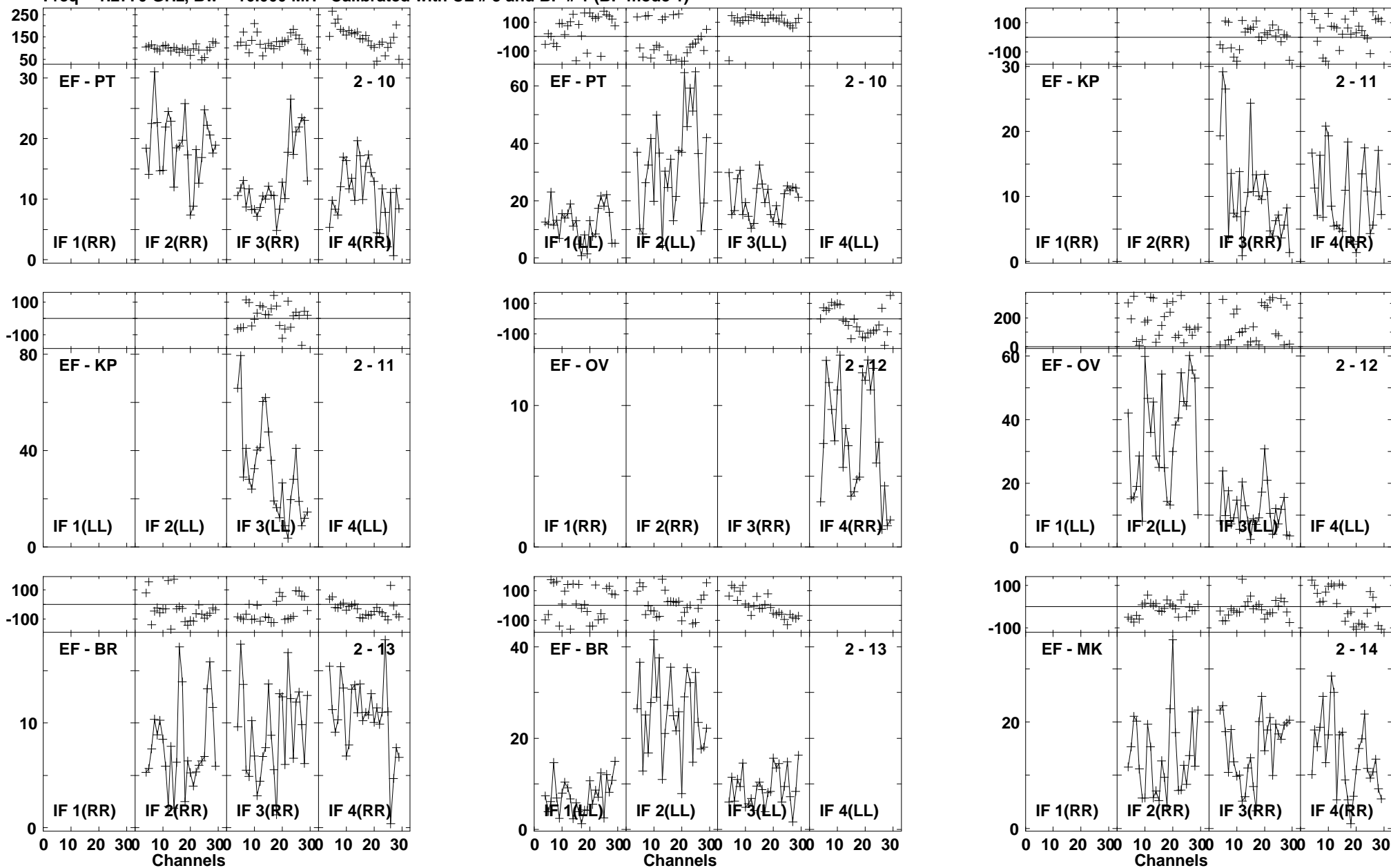
Lower frame: Milli Ampl Jy Top frame: Phas deg Vector averaged cross-power spectrum Baseline: EF (02) - PT (10) Timerange: 00/19:14:24 to 00/19:17:18
