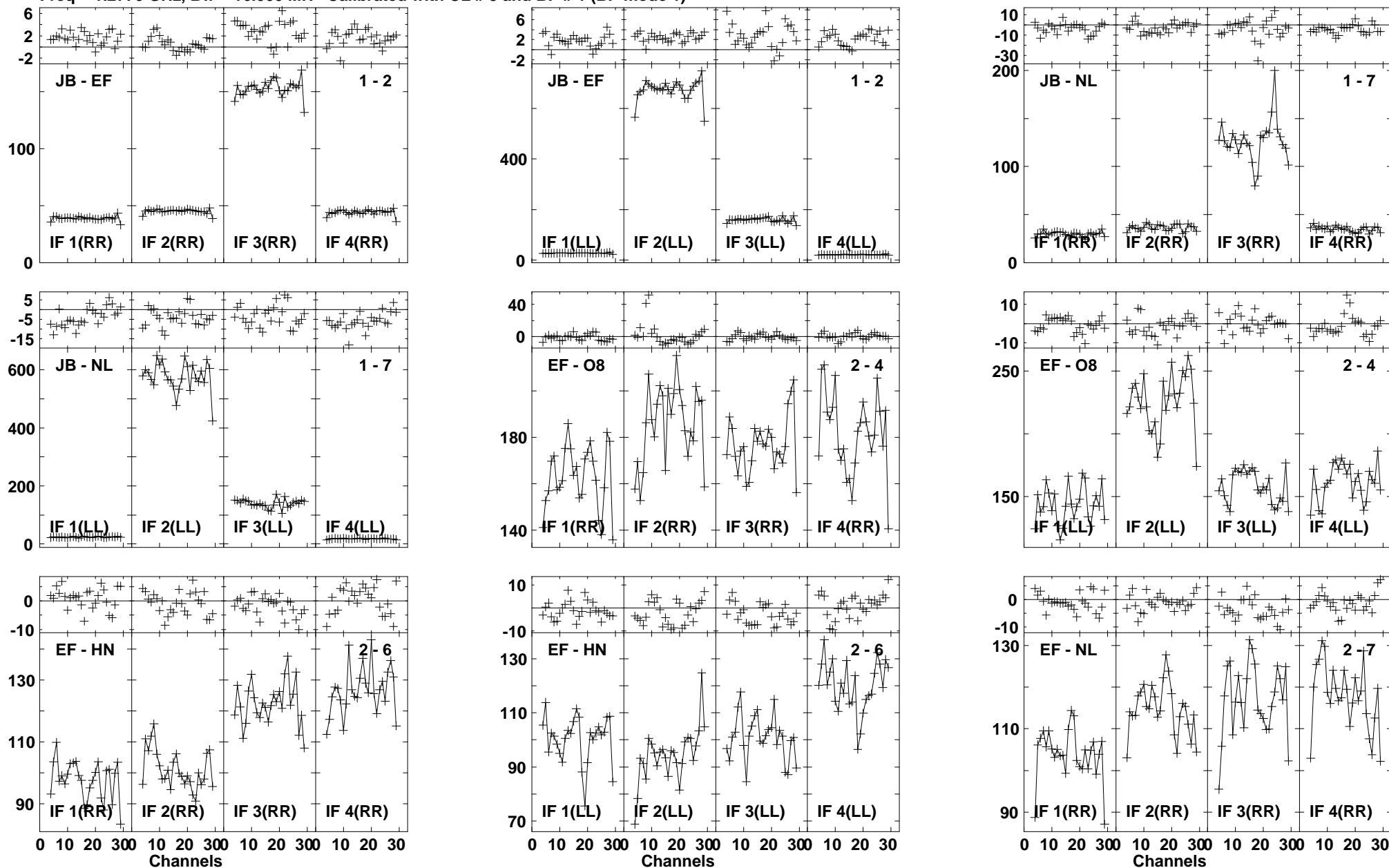
Lower frame: Milli Ampl Jy Top frame: Phas deg Vector averaged cross-power spectrum Baseline: JB (01) - EF (02) Timerange: 01/03:01:47 to 01/03:03:45
