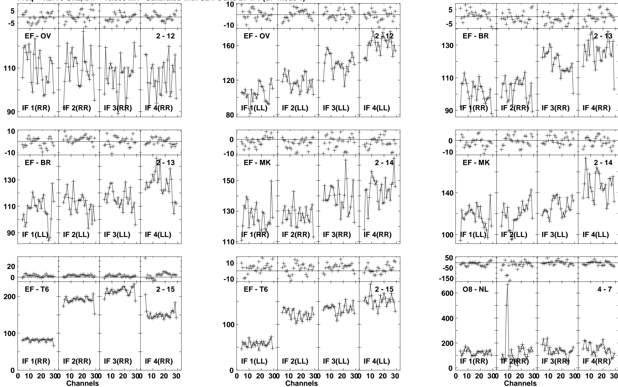
Lower frame: Milli Ampl Jy Top frame: Phas deg Vector averaged cross-power spectrum Baseline: EF (02) - OV (12) Timerange: 01/02:14:10 to 01/02:16:08
