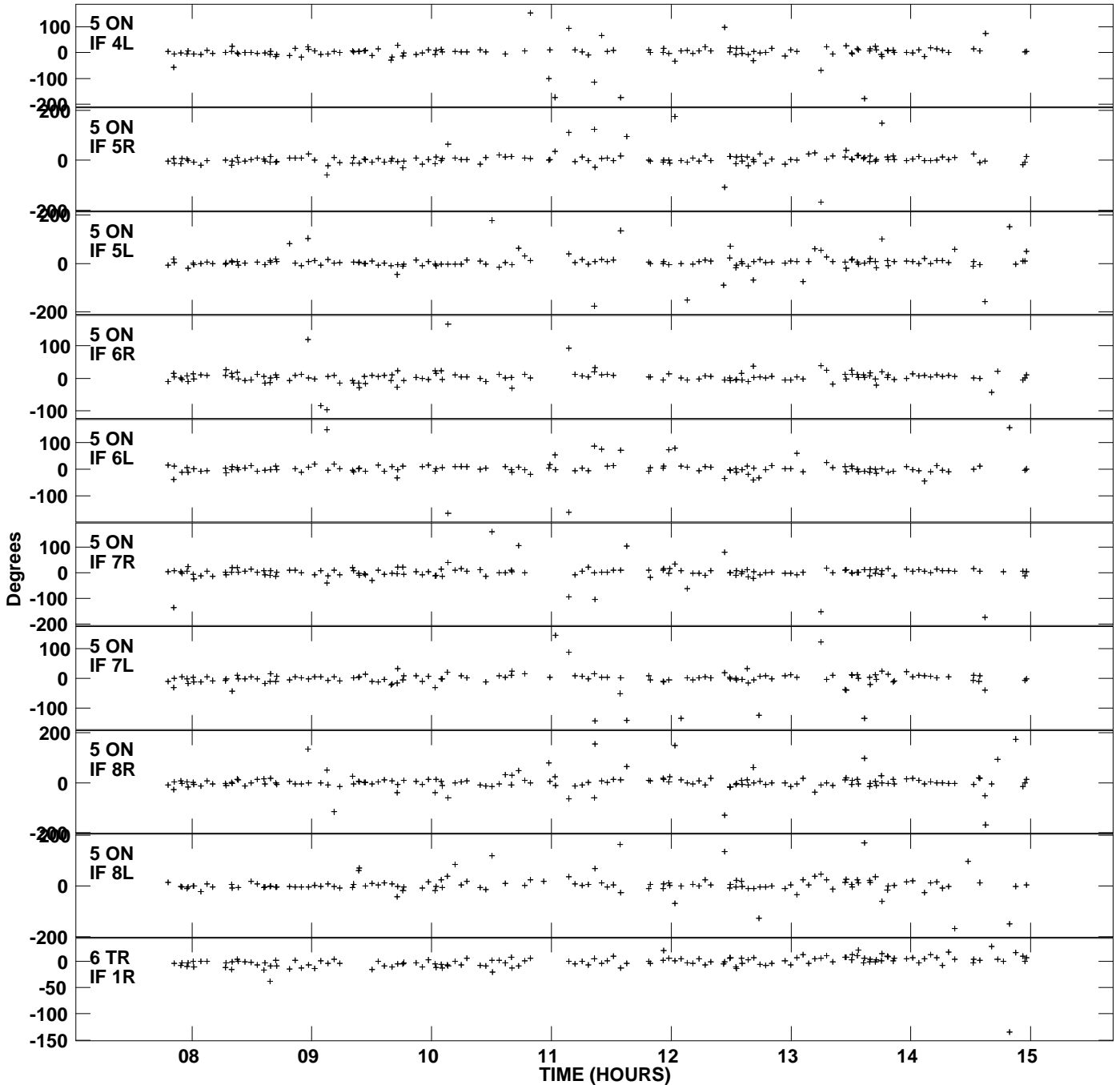
Plot file version 8 created 13-FEB-2009 12:49:31 Gain phs vs UTC time for J1048+2115.MULTI.1 SN 1 Rpol & Lpol IF 1 - 8
