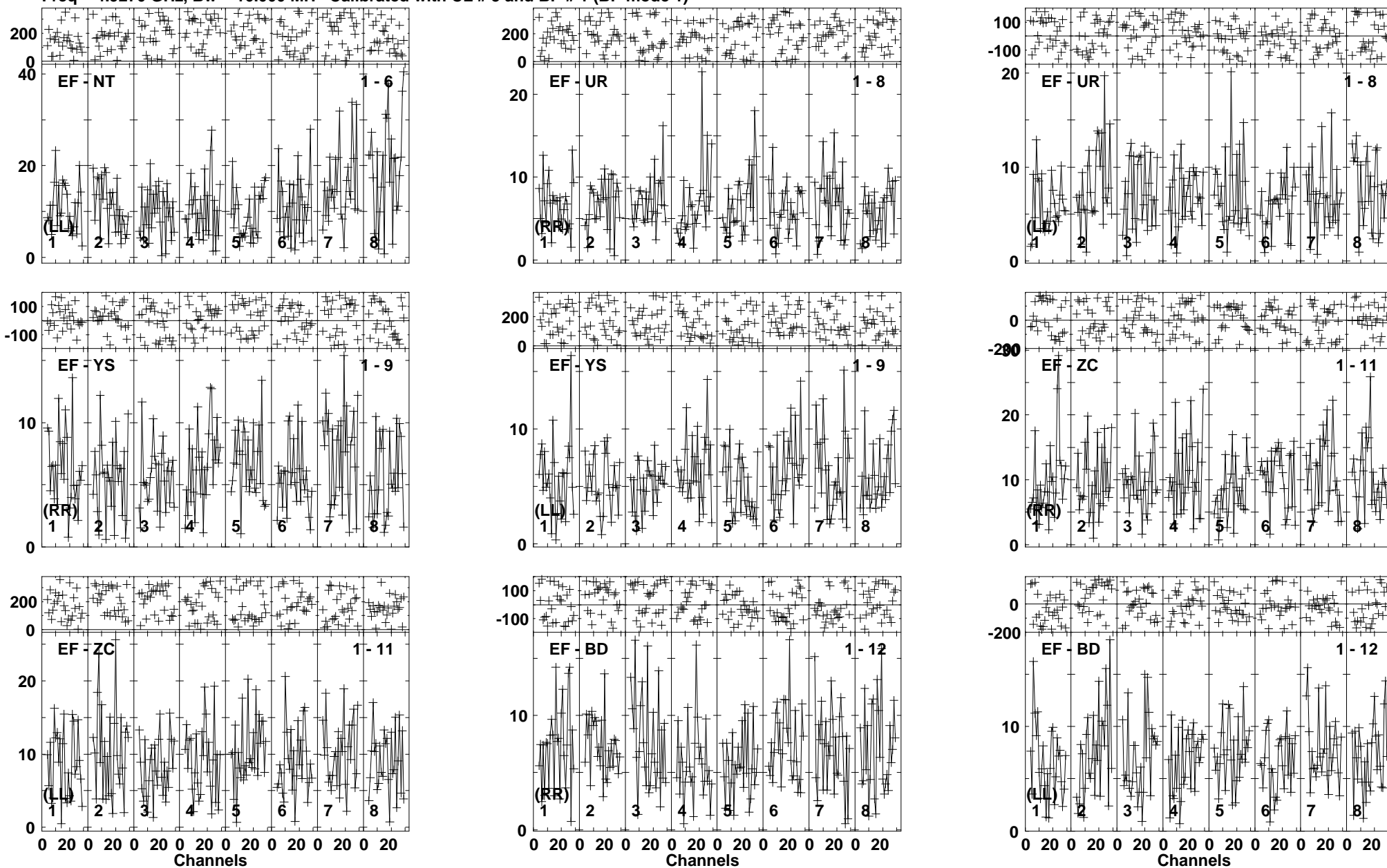
Lower frame: Milli Ampl Jy Top frame: Phas deg Vector averaged cross-power spectrum Baseline: EF (01) - NT (06) Timerange: 00:22:20:21 to 00:22:24:19
