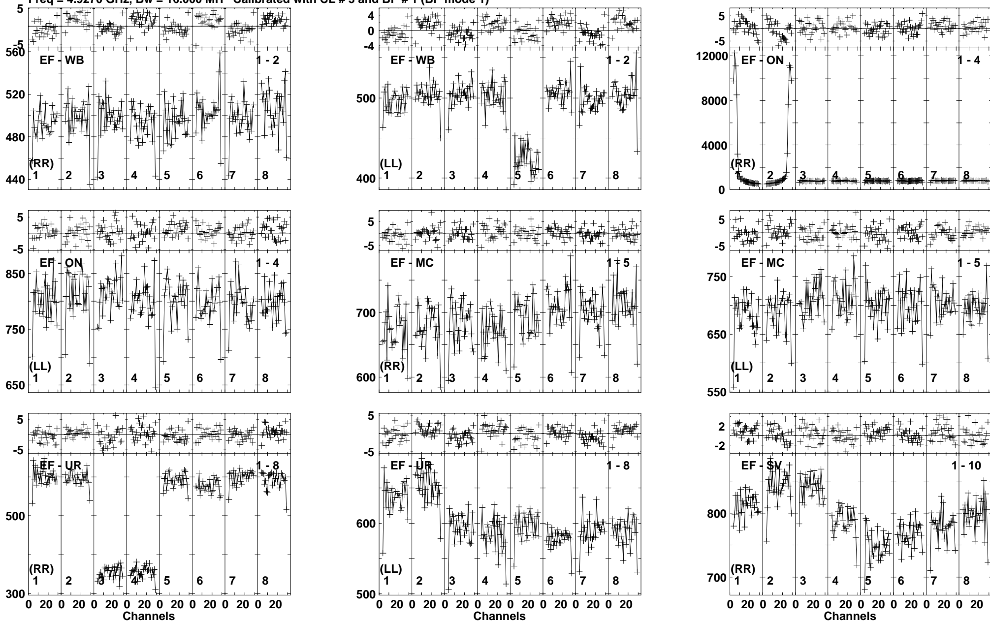
Lower frame: Milli Ampl Jy Top frame: Phas deg Vector averaged cross-power spectrum Baseline: EF (01) - WB (02) Timerange: 00/19:38:11 to 00/19:38:39
