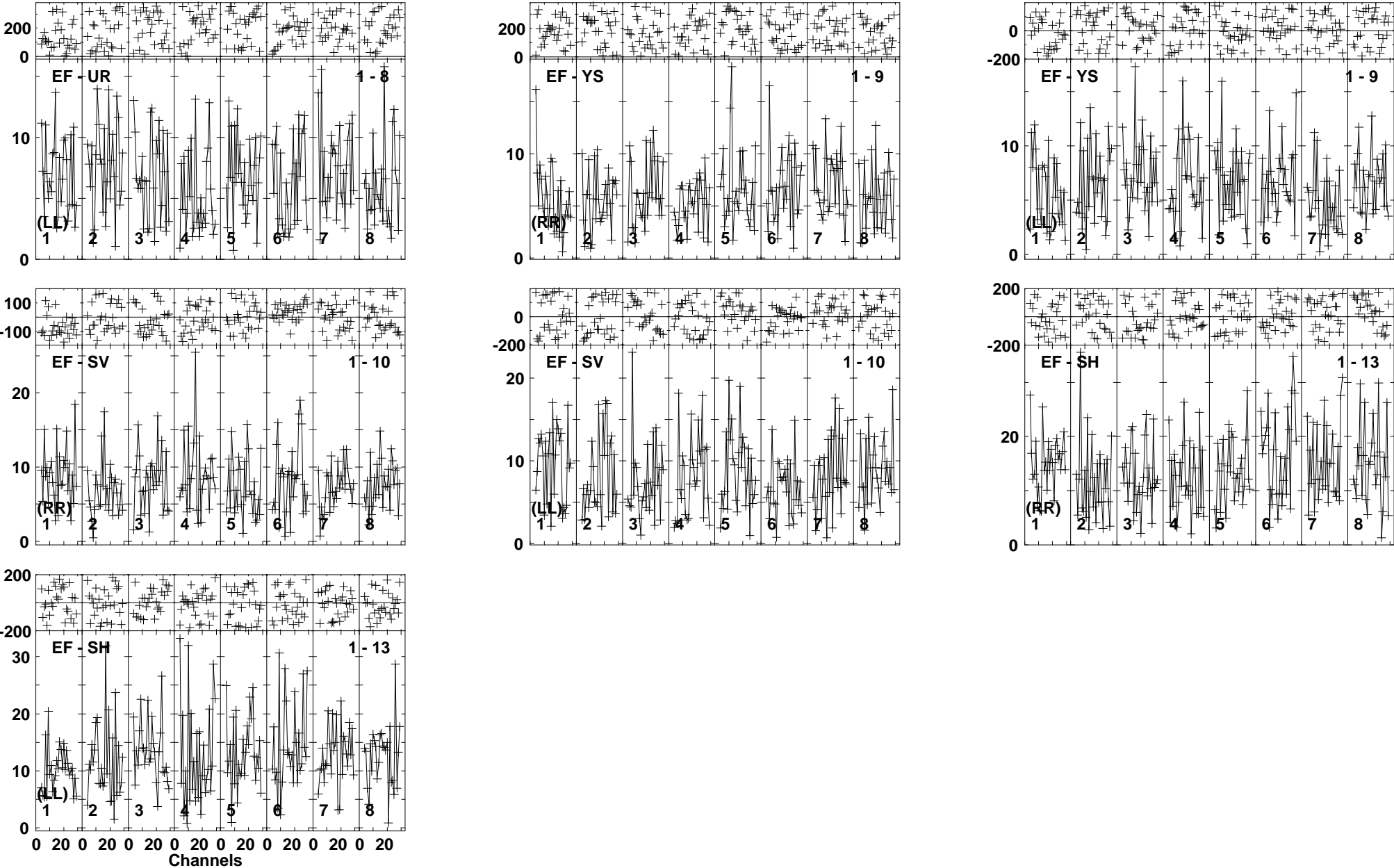
Lower frame: Milli Ampl Jy Top frame: Phas deg Vector averaged cross-power spectrum Baseline: EF (01) - UR (08) Timerange: 00:19:13:36 to 00:19:17:18
