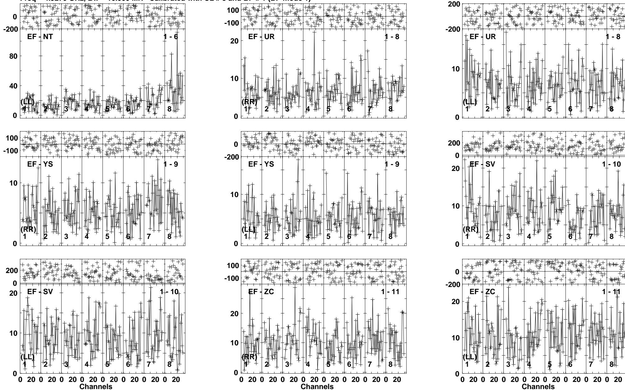
Lower frame: Milli Ampl Jy Top frame: Phas deg Vector averaged cross-power spectrum Baseline: EF (01) - NT (06) Timerange: 00/21:04:35 to 00/21:08:29
