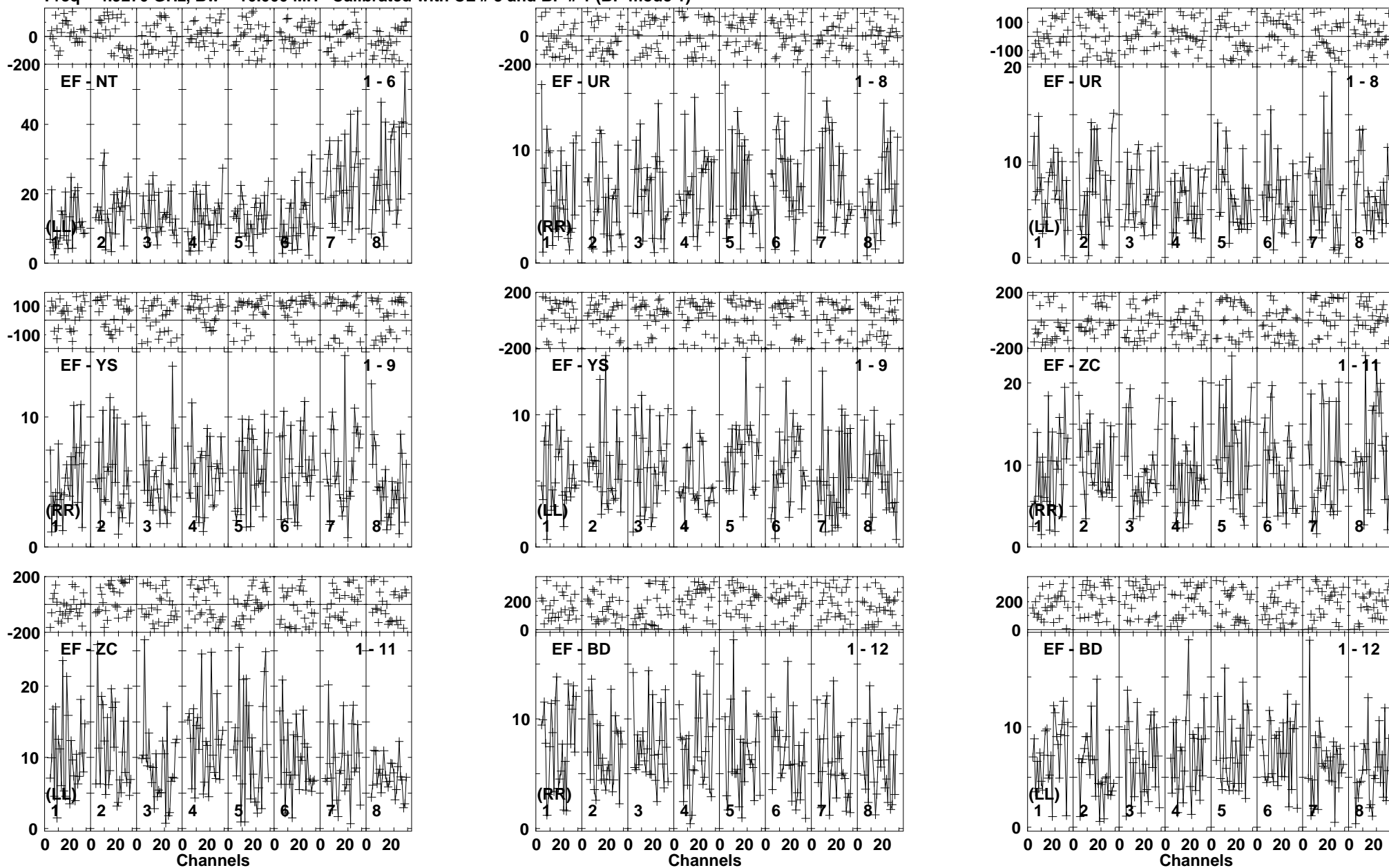
Lower frame: Milli Ampl Jy Top frame: Phas deg Vector averaged cross-power spectrum Baseline: EF (01) - NT (06) Timerange: 00:22:35:35 to 00:22:39:29
