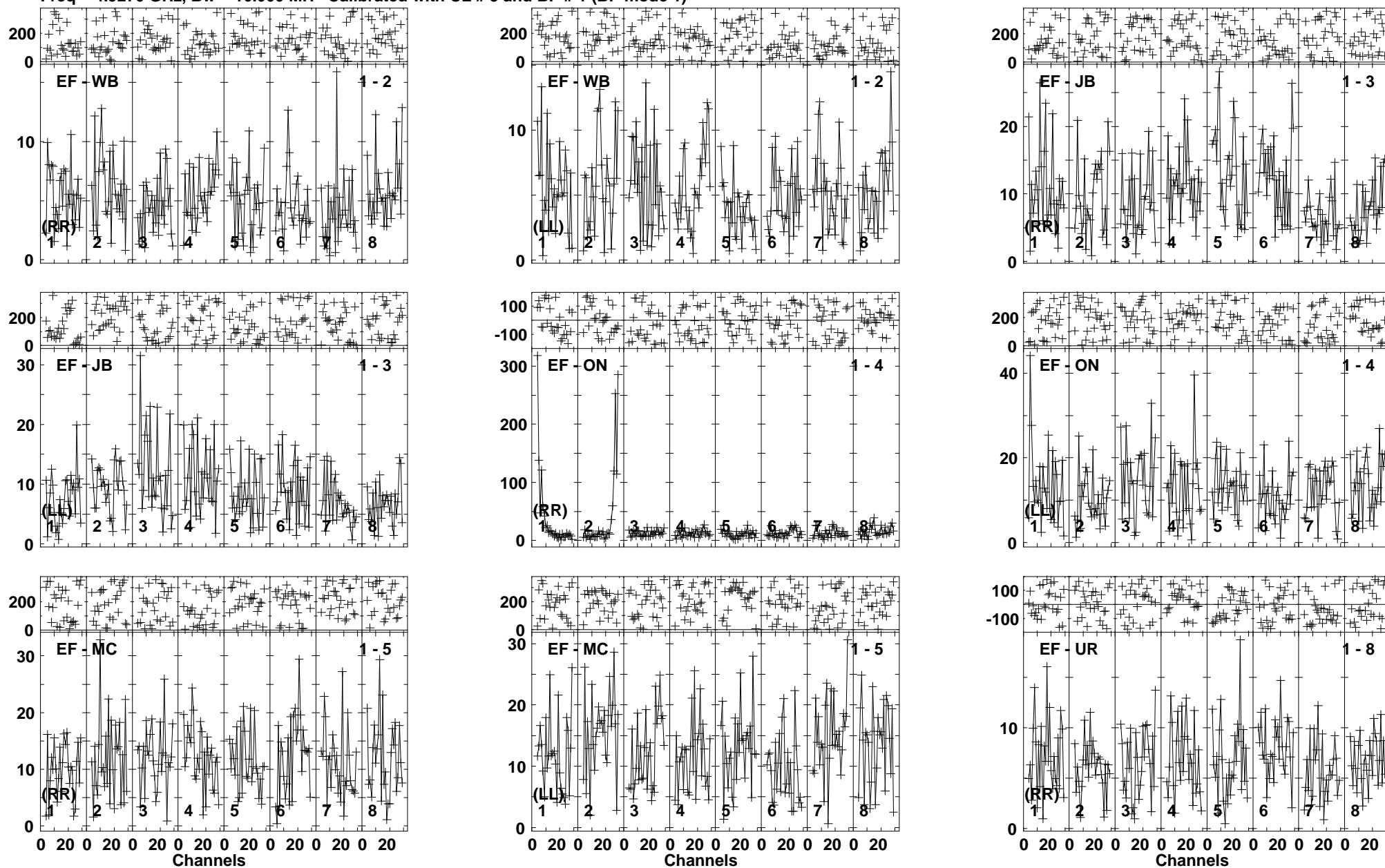
Lower frame: Milli Ampl Jy Top frame: Phas deg Vector averaged cross-power spectrum Baseline: EF (01) - WB (02) Timerange: 00/20:14:05 to 00/20:17:59
