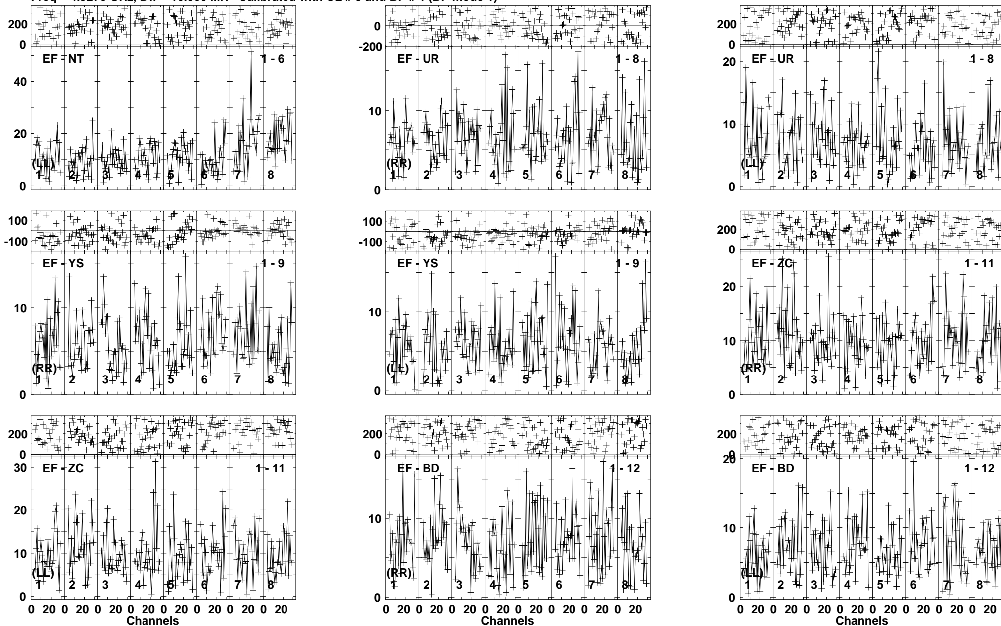
Lower frame: Milli Ampl Jy Top frame: Phas deg Vector averaged cross-power spectrum Baseline: EF (01) - NT (06) Timerange: 00:22:10:21 to 00:22:14:19
