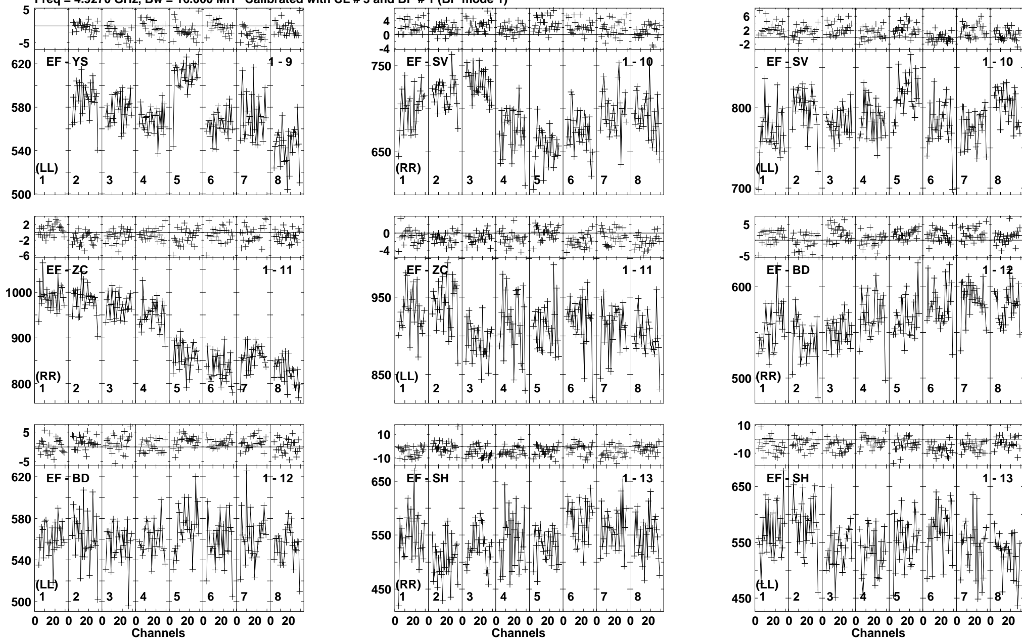
Lower frame: Milli Ampl Jy Top frame: Phas deg Vector averaged cross-power spectrum Baseline: EF (01) - YS (09) Timerange: 01/00:30:56 to 01/00:31:48
