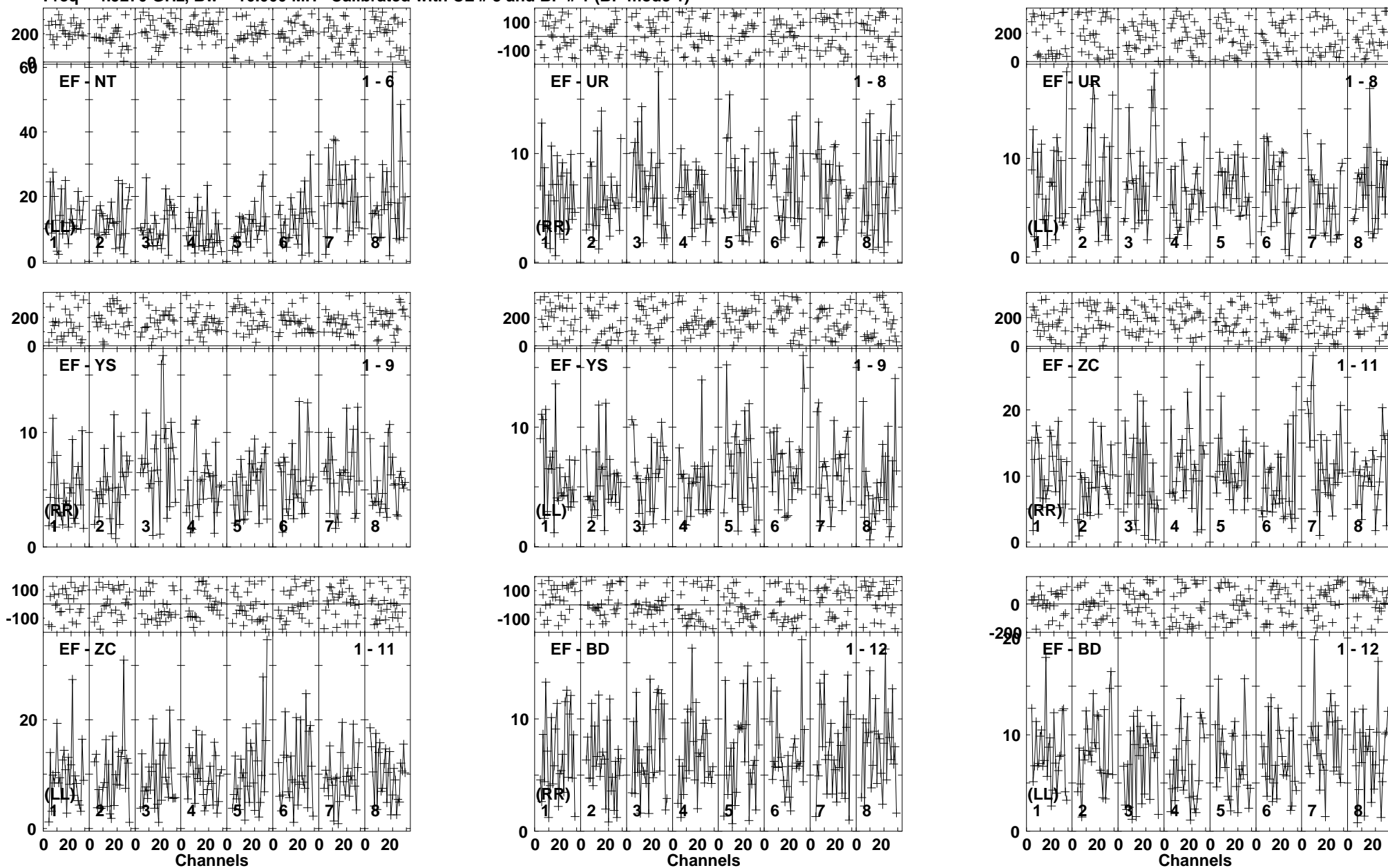
Lower frame: Milli Ampl Jy Top frame: Phas deg Vector averaged cross-power spectrum Baseline: EF (01) - NT (06) Timerange: 00/21:55:15 to 00/21:59:09
