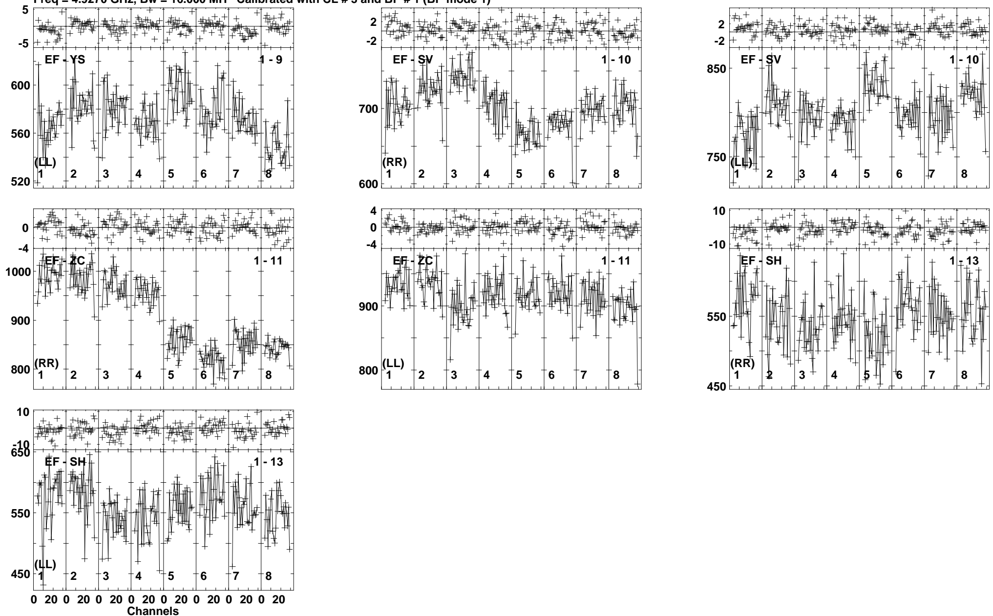
Lower frame: Milli Ampl Jy Top frame: Phas deg Vector averaged cross-power spectrum Baseline: EF (01) - YS (09) Timerange: 01/00:41:31 to 01/00:41:59
