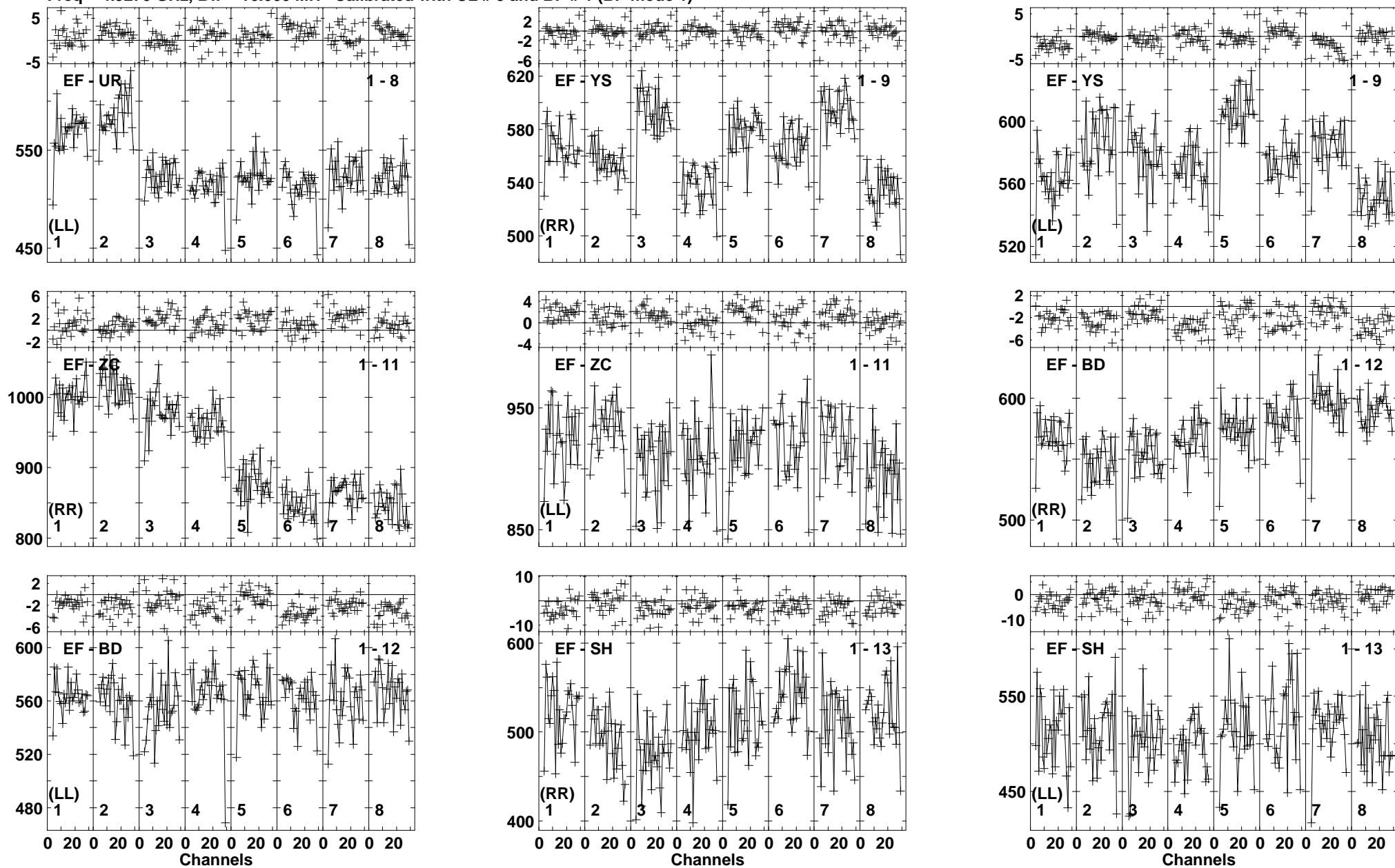
Lower frame: Milli Ampl Jy Top frame: Phas deg Vector averaged cross-power spectrum Baseline: EF (01) - UR (08) Timerange: 00/22:19:25 to 00/22:20:19
