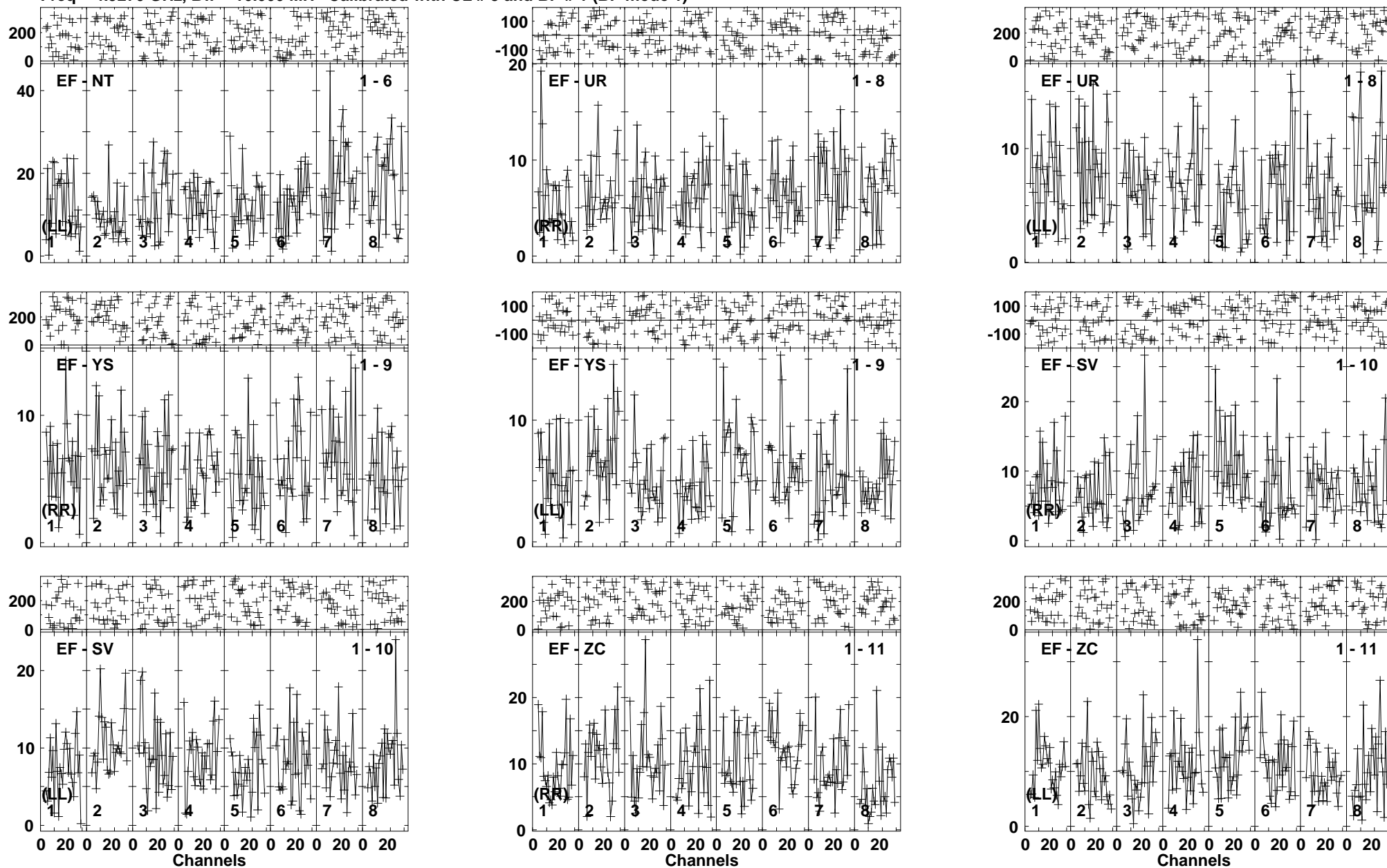
Lower frame: Milli Ampl Jy Top frame: Phas deg Vector averaged cross-power spectrum Baseline: EF (01) - NT (06) Timerange: 00/20:54:35 to 00/20:58:29
