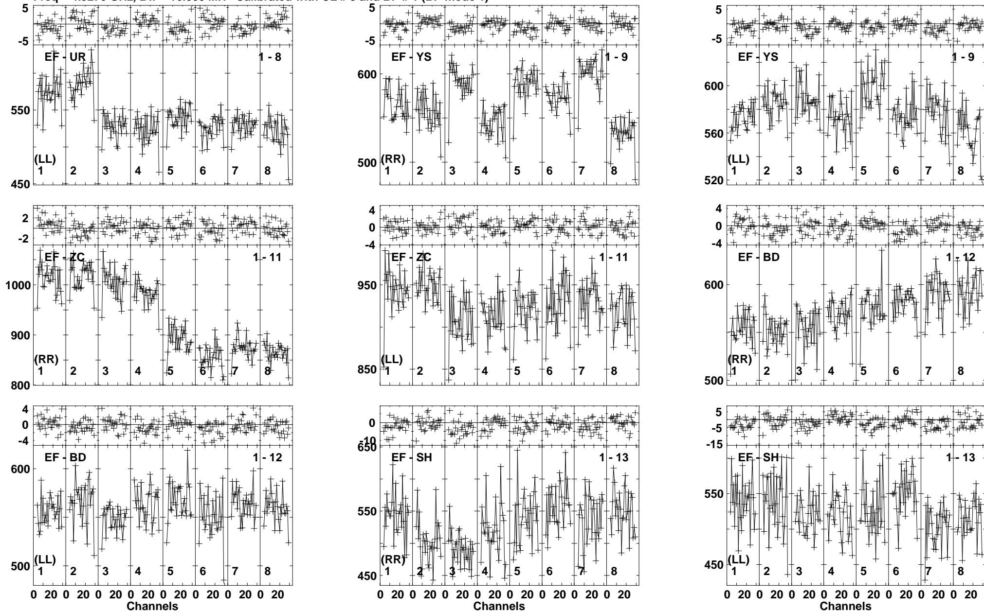
Lower frame: Milli Ampl Jy Top frame: Phas deg Vector averaged cross-power spectrum Baseline: EF (01) - UR (08) Timerange: 00/22:09:51 to 00/22:10:19
