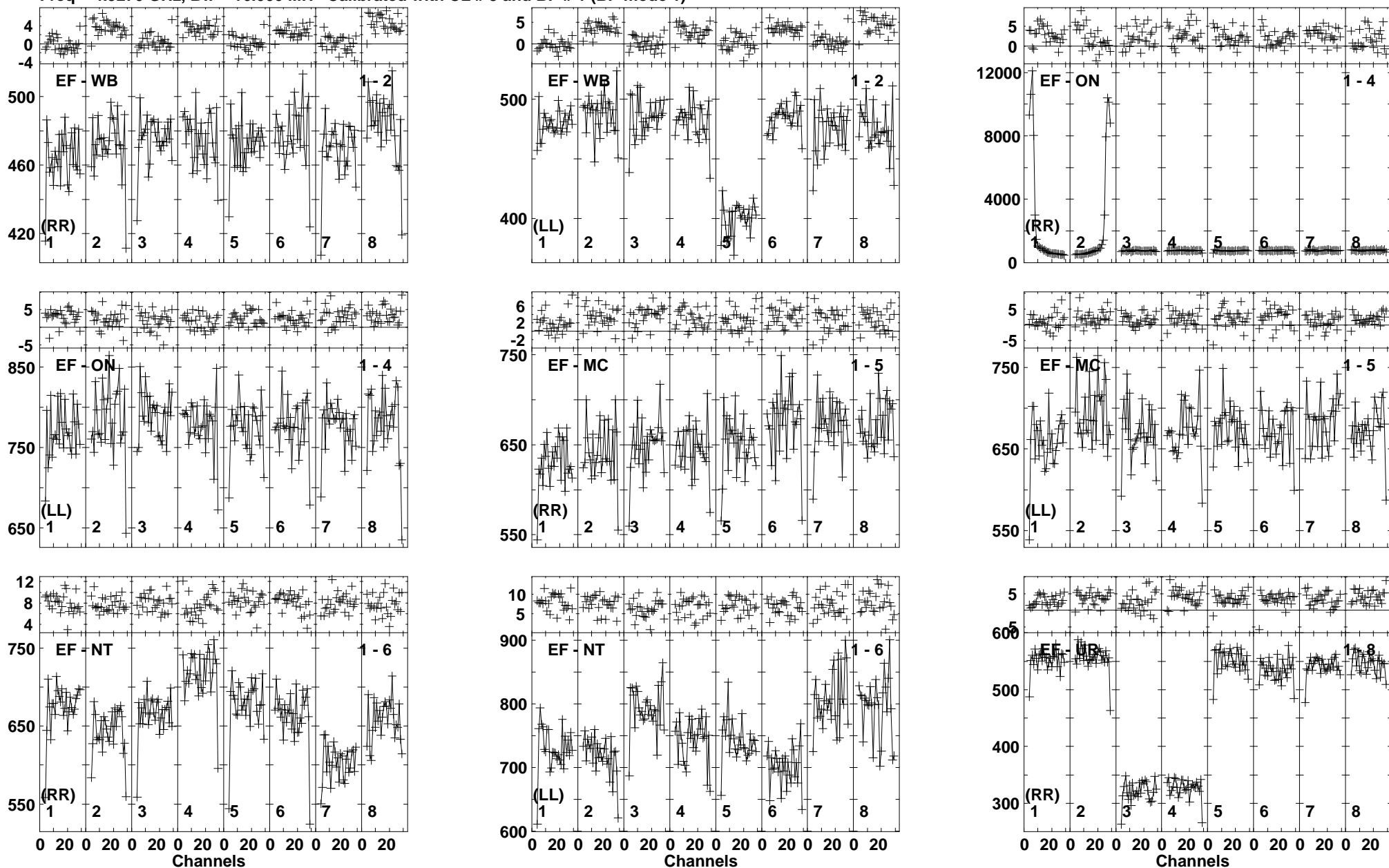
Lower frame: Milli Ampl Jy Top frame: Phas deg Vector averaged cross-power spectrum Baseline: EF (01) - WB (02) Timerange: 00/20:58:35 to 00/20:59:29
