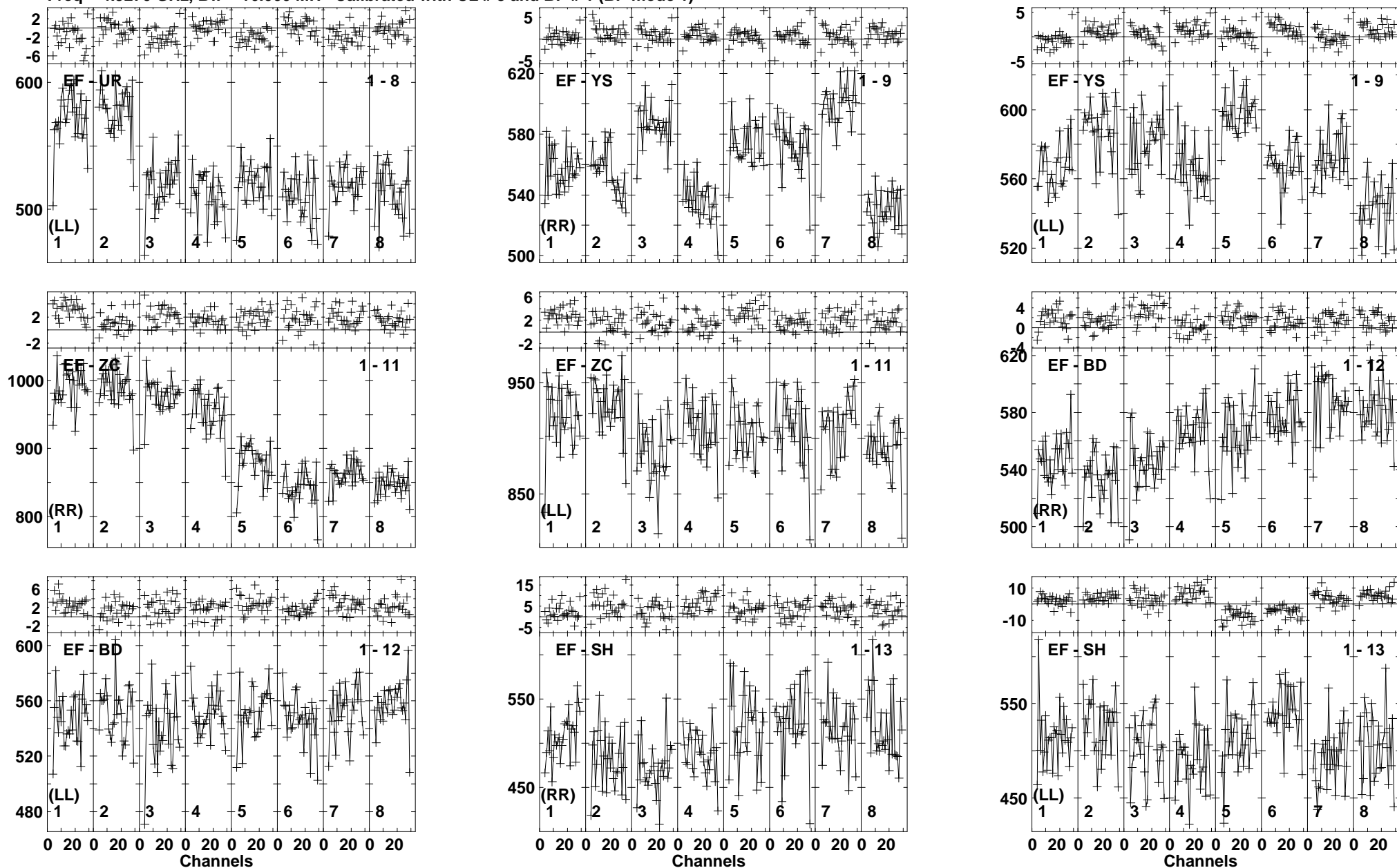
Lower frame: Milli Ampl Jy Top frame: Phas deg Vector averaged cross-power spectrum Baseline: EF (01) - UR (08) Timerange: 00/22:29:35 to 00/22:30:29
