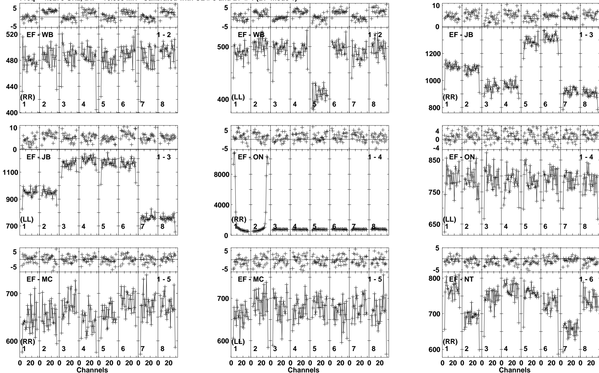
Lower frame: Milli Ampl Jy Top frame: Phas deg Vector averaged cross-power spectrum Baseline: EF (01) - WB (02) Timerange: 00/20:43:25 to 00/20:44:19
