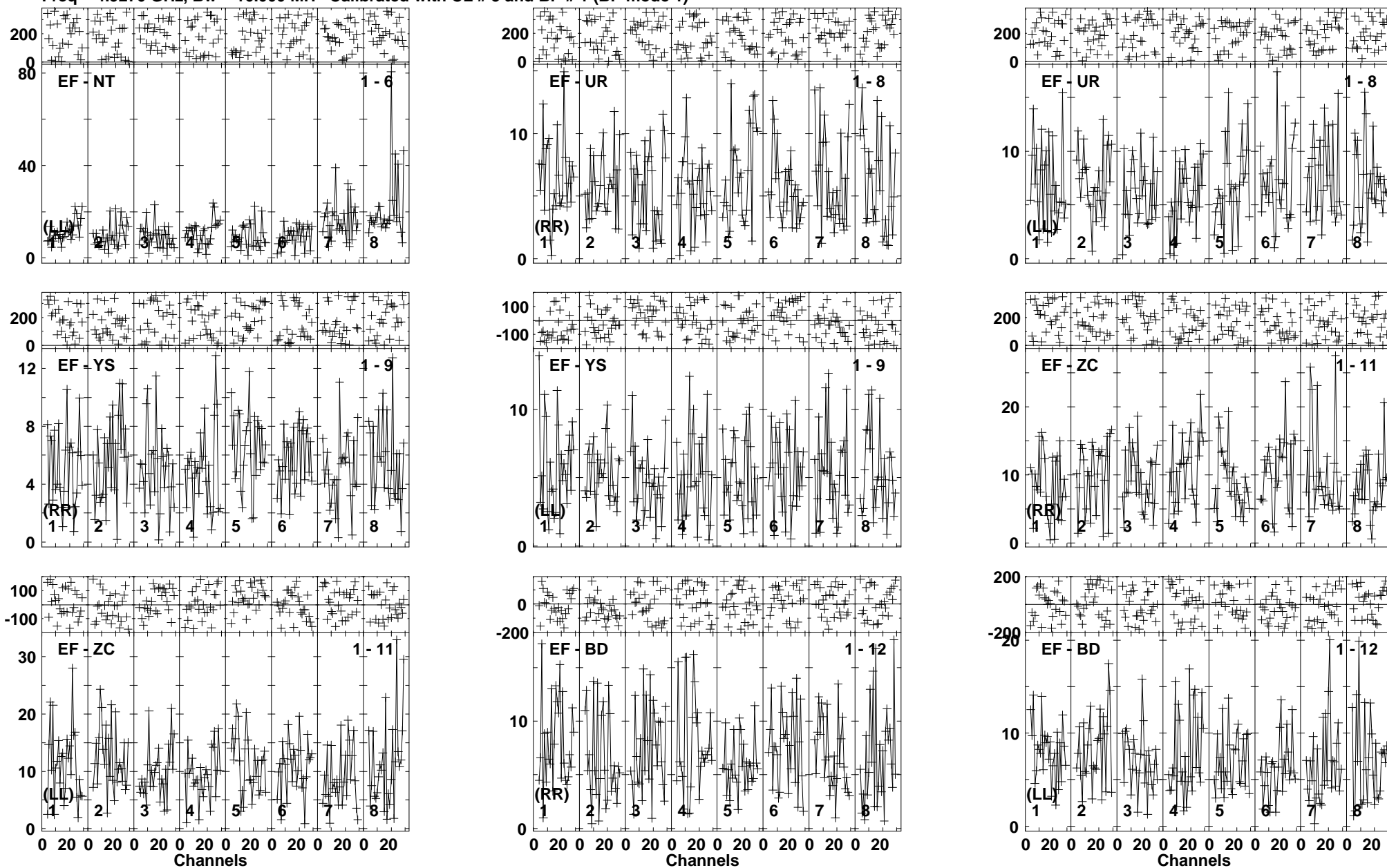
Lower frame: Milli Ampl Jy Top frame: Phas deg Vector averaged cross-power spectrum Baseline: EF (01) - NT (06) Timerange: 00/21:45:05 to 00/21:48:59
