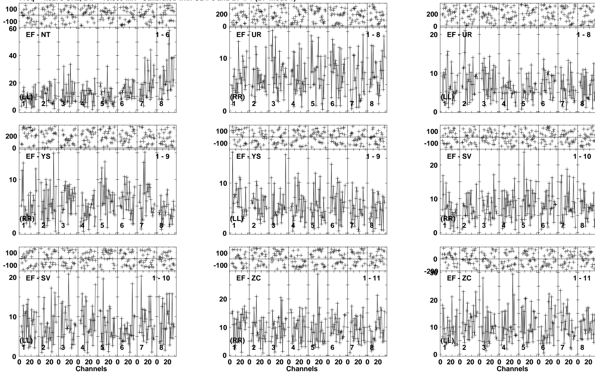
Lower frame: Milli Ampl Jy Top frame: Phas deg Vector averaged cross-power spectrum Baseline: EF (01) - NT (06) Timerange: 00/21:19:41 to 00/21:23:39
