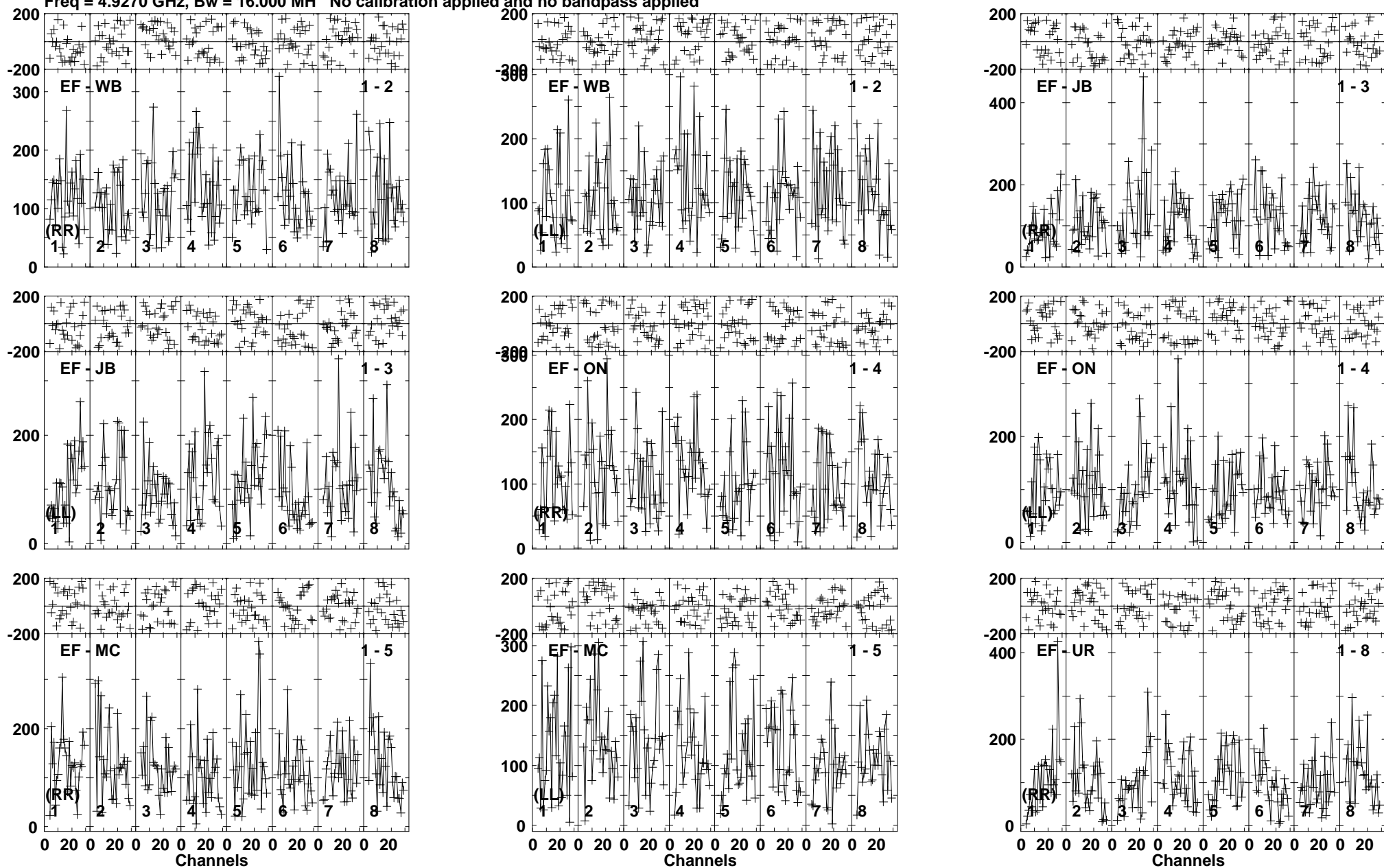
Lower frame: Micro Ampl Jy Top frame: Phas deg Vector averaged cross-power spectrum Baseline: EF (01) - WB (02) Timerange: 00/19:18:21 to 00/19:22:19
