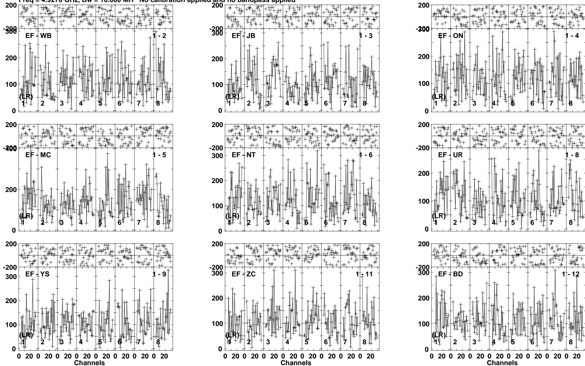
Lower frame: Micro Ampl Jy Top frame: Phas deg Vector averaged cross-power spectrum Baseline: EF (01) - WB (02) Timerange: 00/23:00:51 to 00/23:04:49
