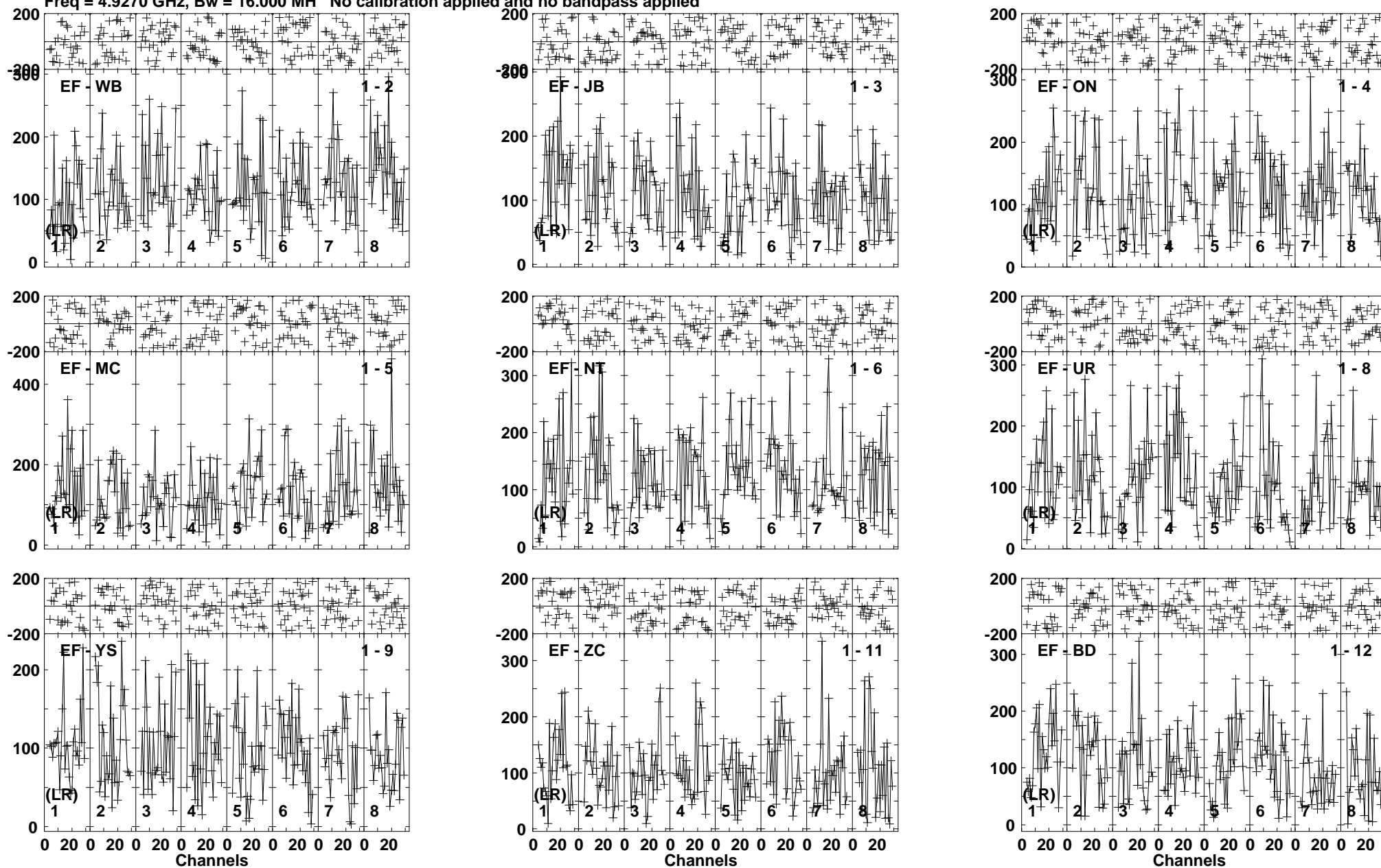
Lower frame: Micro Ampl Jy Top frame: Phas deg Vector averaged cross-power spectrum Baseline: EF (01) - WB (02) Timerange: 00/21:29:51 to 00/21:33:49
