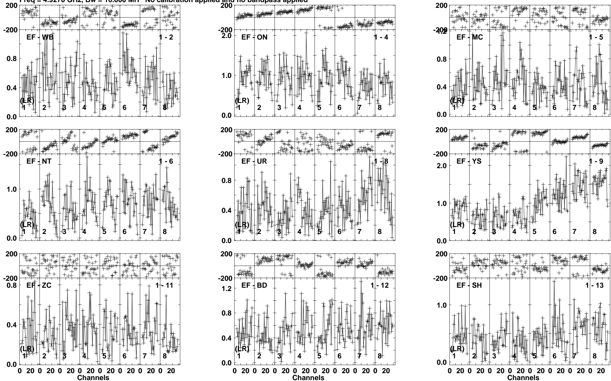
Lower frame: Milli Ampl Jy Top frame: Phas deg Vector averaged cross-power spectrum Baseline: EF (01) - WB (02) Timerange: 00/21:39:31 to 00/21:39:59
