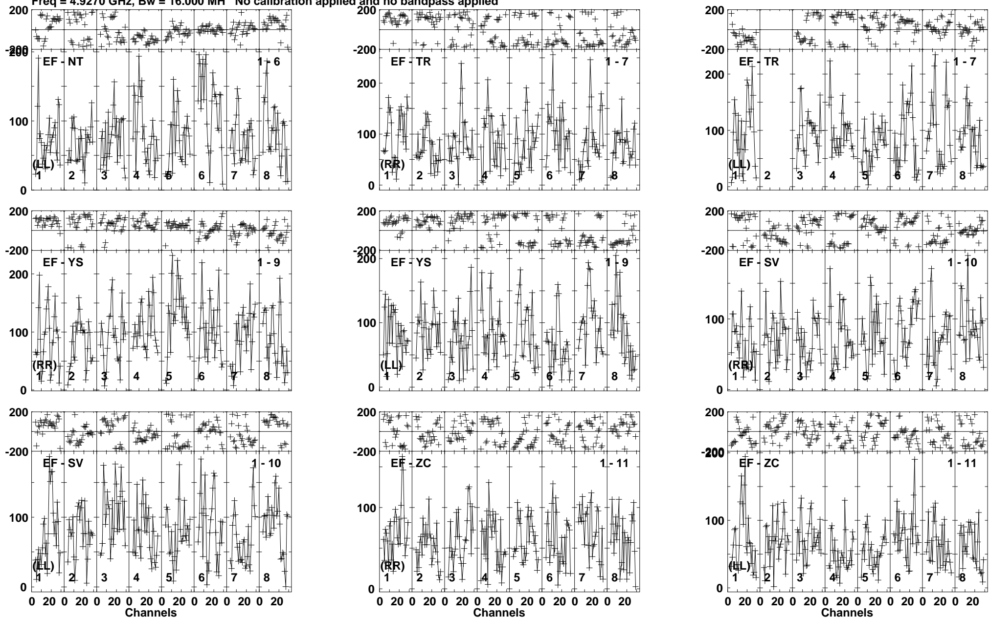
Lower frame: Micro Ampl Jy Top frame: Phas deg Vector averaged cross-power spectrum Baseline: EF (01) - NT (06) Timerange: 00/20:34:05 to 00/20:37:59
