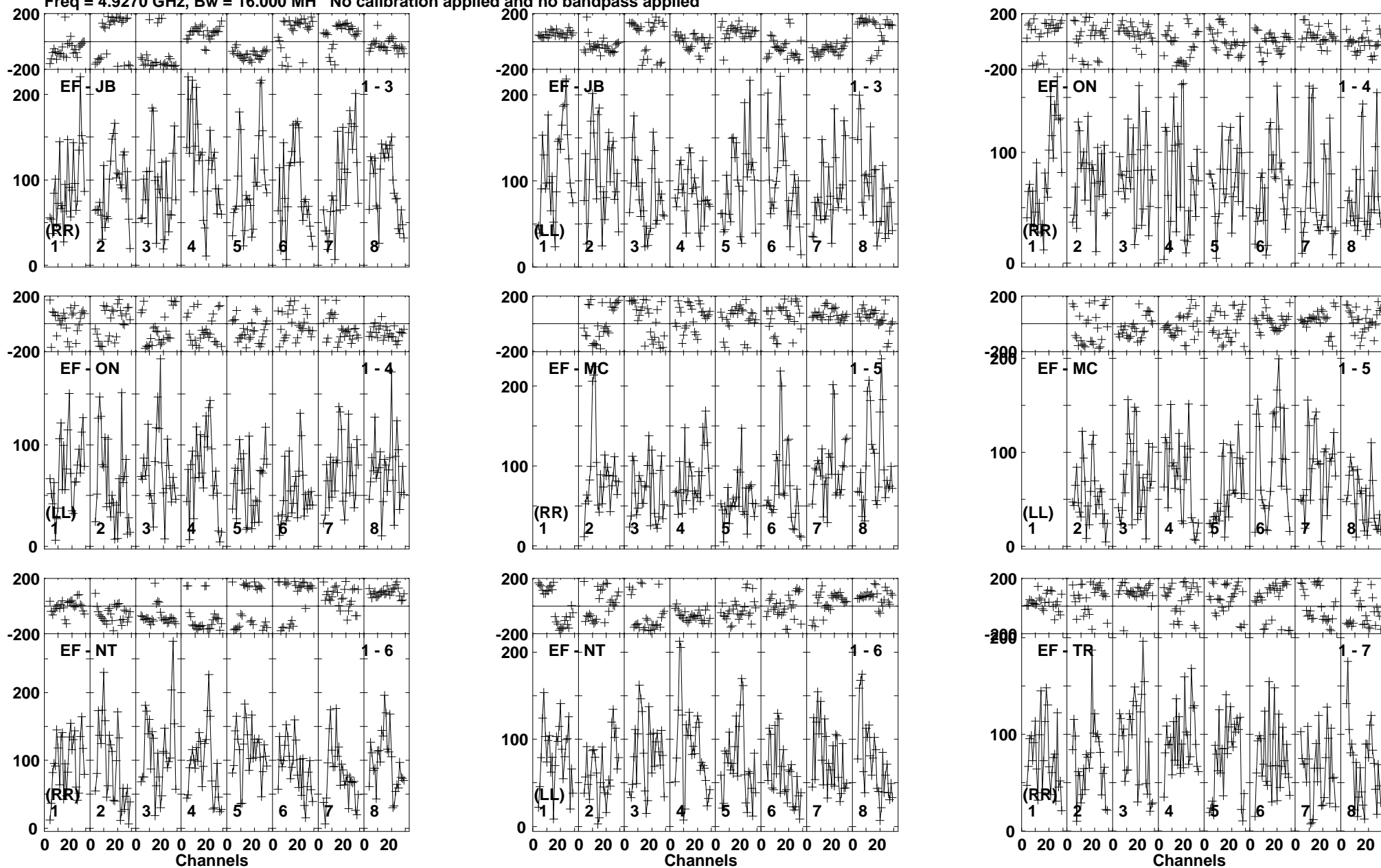
Lower frame: Micro Ampl Jy Top frame: Phas deg Vector averaged cross-power spectrum Baseline: EF (01) - JB (03) Timerange: 00/18:07:23 to 00/18:11:19
