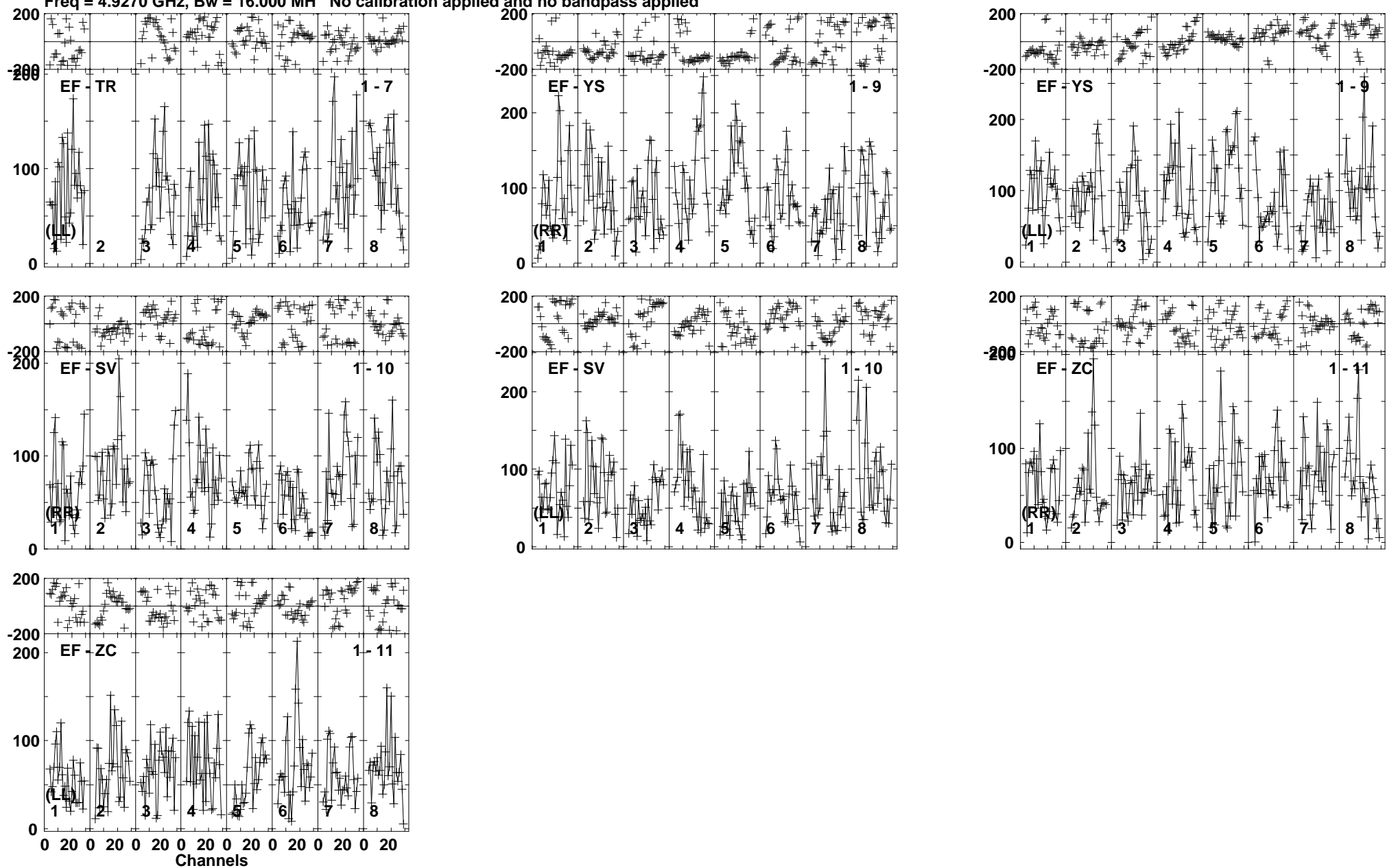
Lower frame: Micro Ampl Jy Top frame: Phas deg Vector averaged cross-power spectrum Baseline: EF (01) - TR (07) Timerange: 00:18:02:24 to 00:18:06:18
