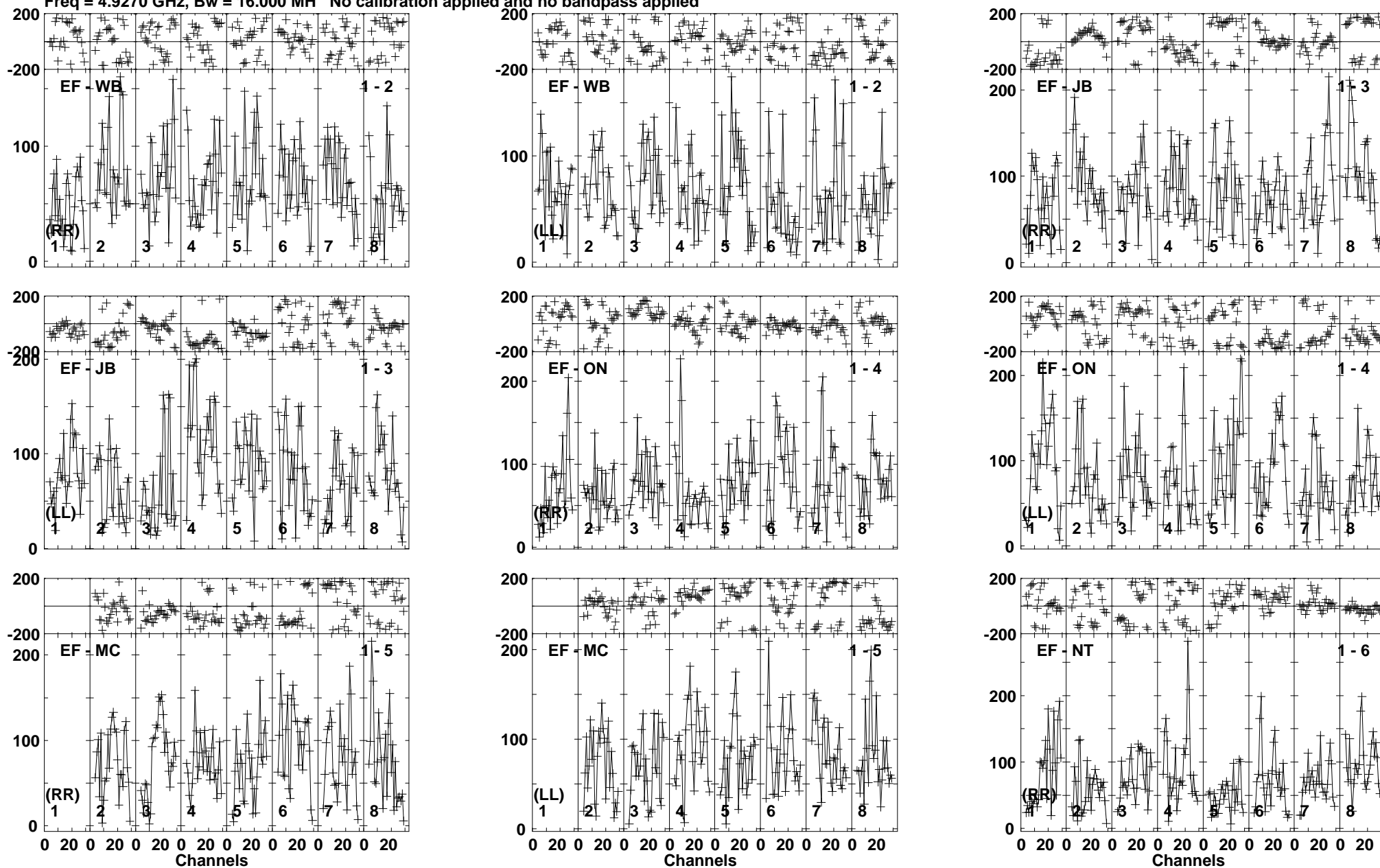
Lower frame: Micro Ampl Jy Top frame: Phas deg Vector averaged cross-power spectrum Baseline: EF (01) - WB (02) Timerange: 00/21:29:43 to 00/21:33:39
