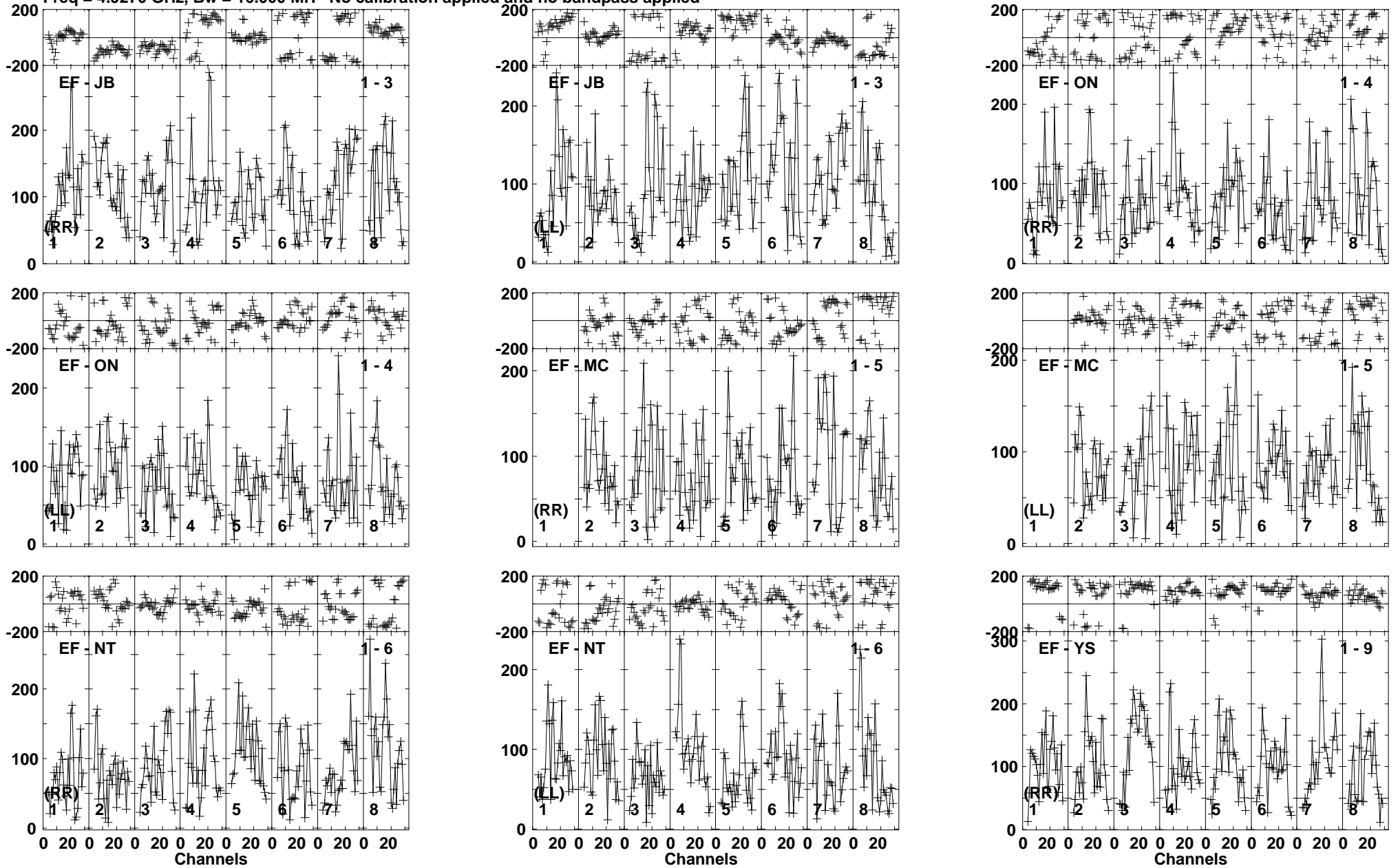
Lower frame: Micro Ampl Jy Top frame: Phas deg Vector averaged cross-power spectrum Baseline: EF (01) - JB (03) Timerange: 00/16:36:23 to 00/16:40:19
