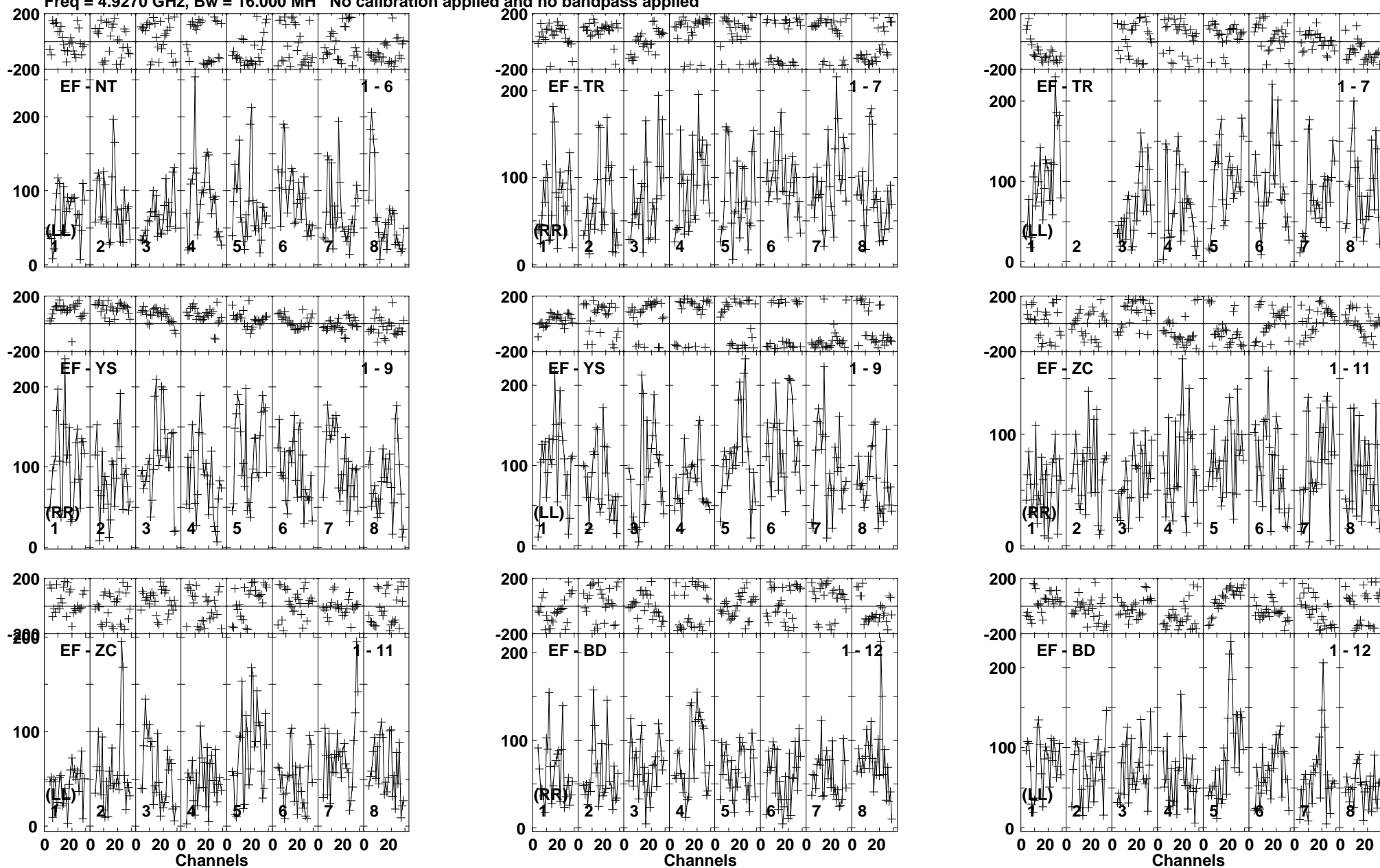
Lower frame: Micro Ampl Jy Top frame: Phas deg Vector averaged cross-power spectrum Baseline: EF (01) - NT (06) Timerange: 00/21:49:53 to 00/21:53:49
