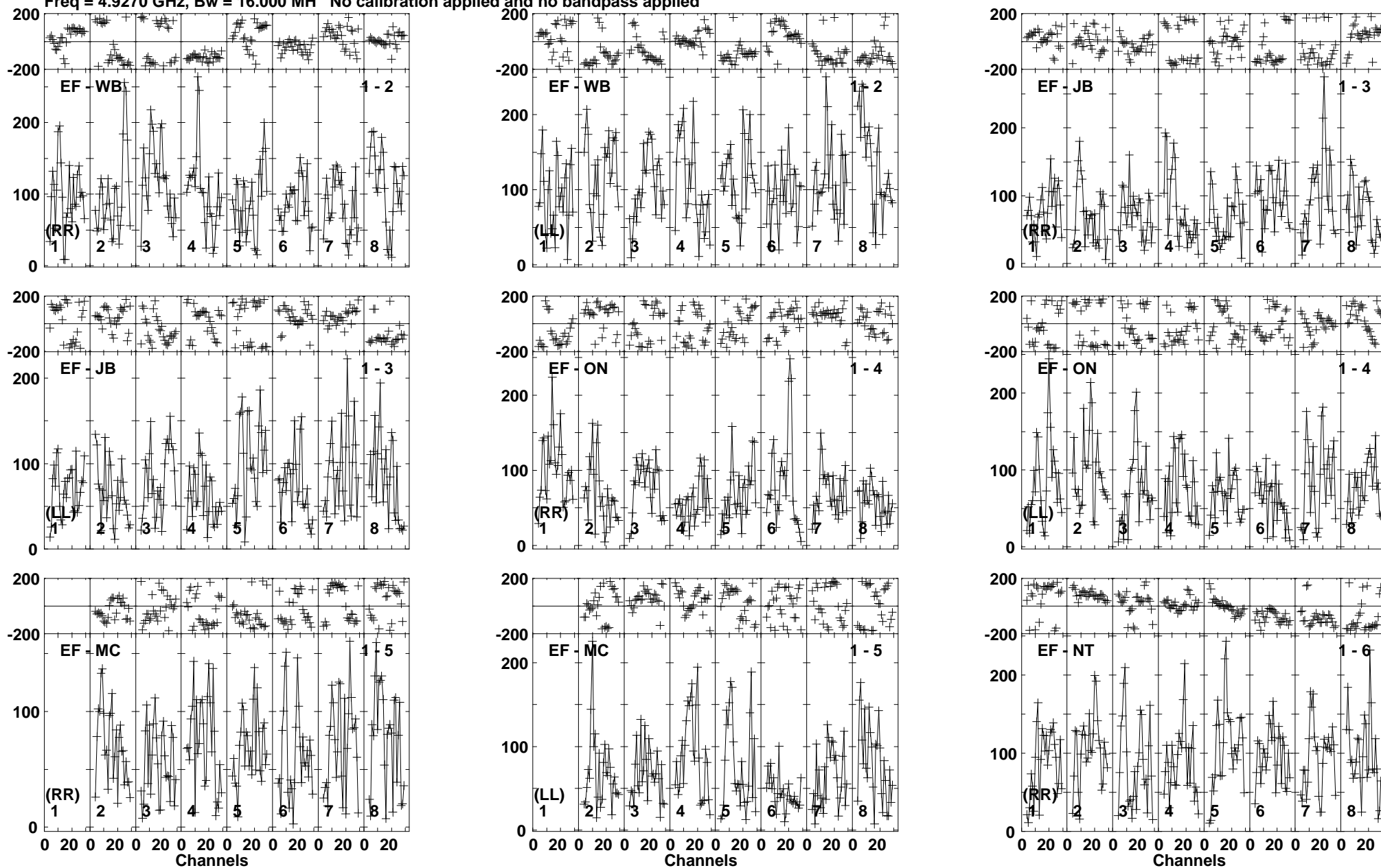
Lower frame: Micro Ampl Jy Top frame: Phas deg Vector averaged cross-power spectrum Baseline: EF (01) - WB (02) Timerange: 00/18:52:55 to 00/18:56:49
