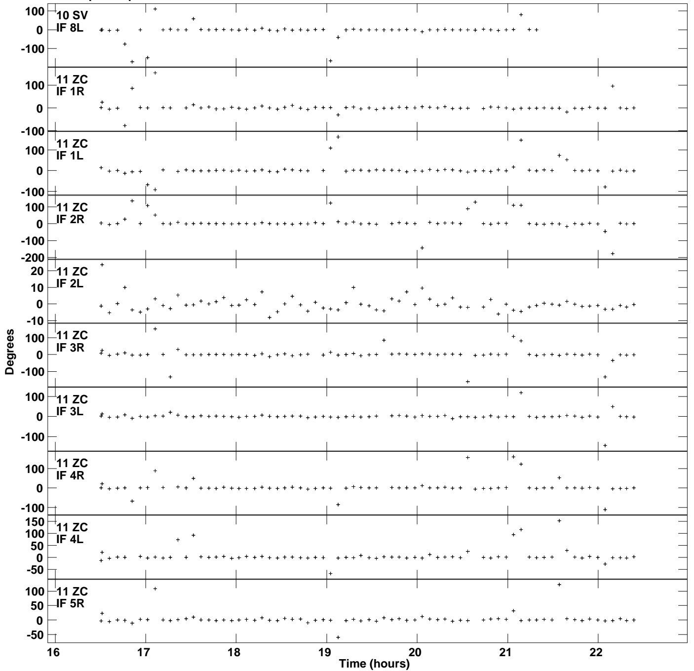
Plot file version 15 created 29-DEC-2015 17:46:54 Gain phs vs UTC time for J1128+5925.MULTI.1 SN 1 Rpol & Lpol IF 1 - 8
