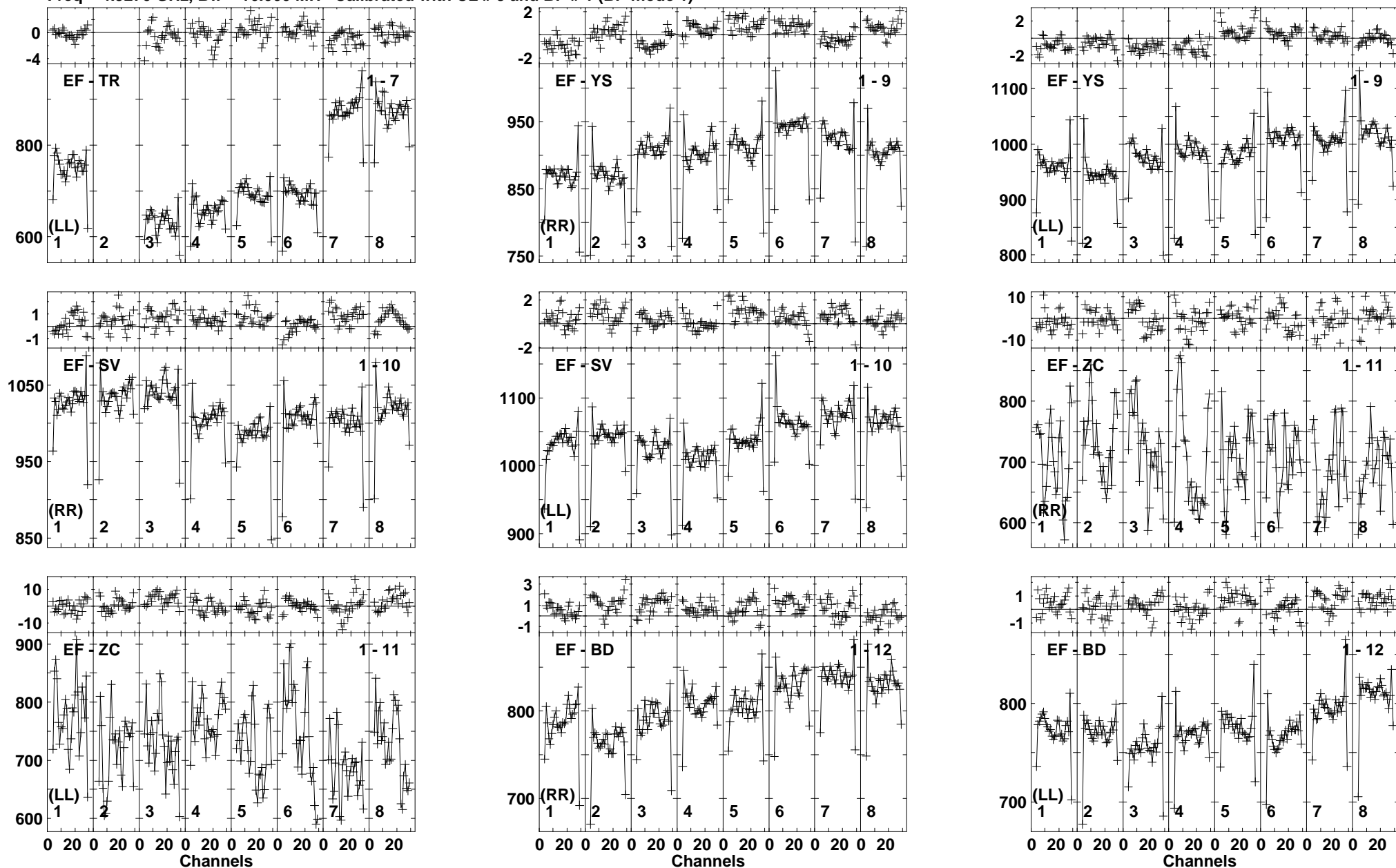
Lower frame: Milli Ampl Jy Top frame: Phas deg Vector averaged cross-power spectrum Baseline: EF (01) - TR (07) Timerange: 00/19:58:11 to 00/19:58:39
