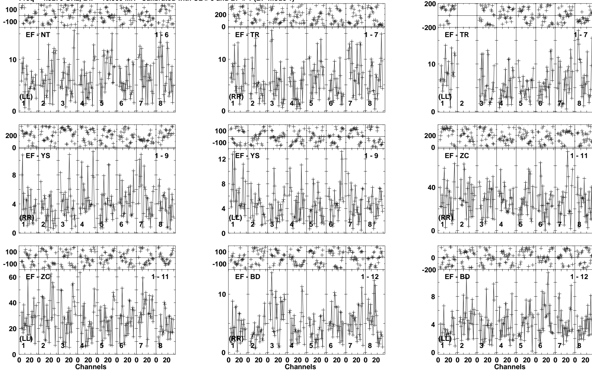
Lower frame: Milli Ampl Jy Top frame: Phas deg Vector averaged cross-power spectrum Baseline: EF (01) - NT (06) Timerange: 00/22:19:23 to 00/22:22:49
