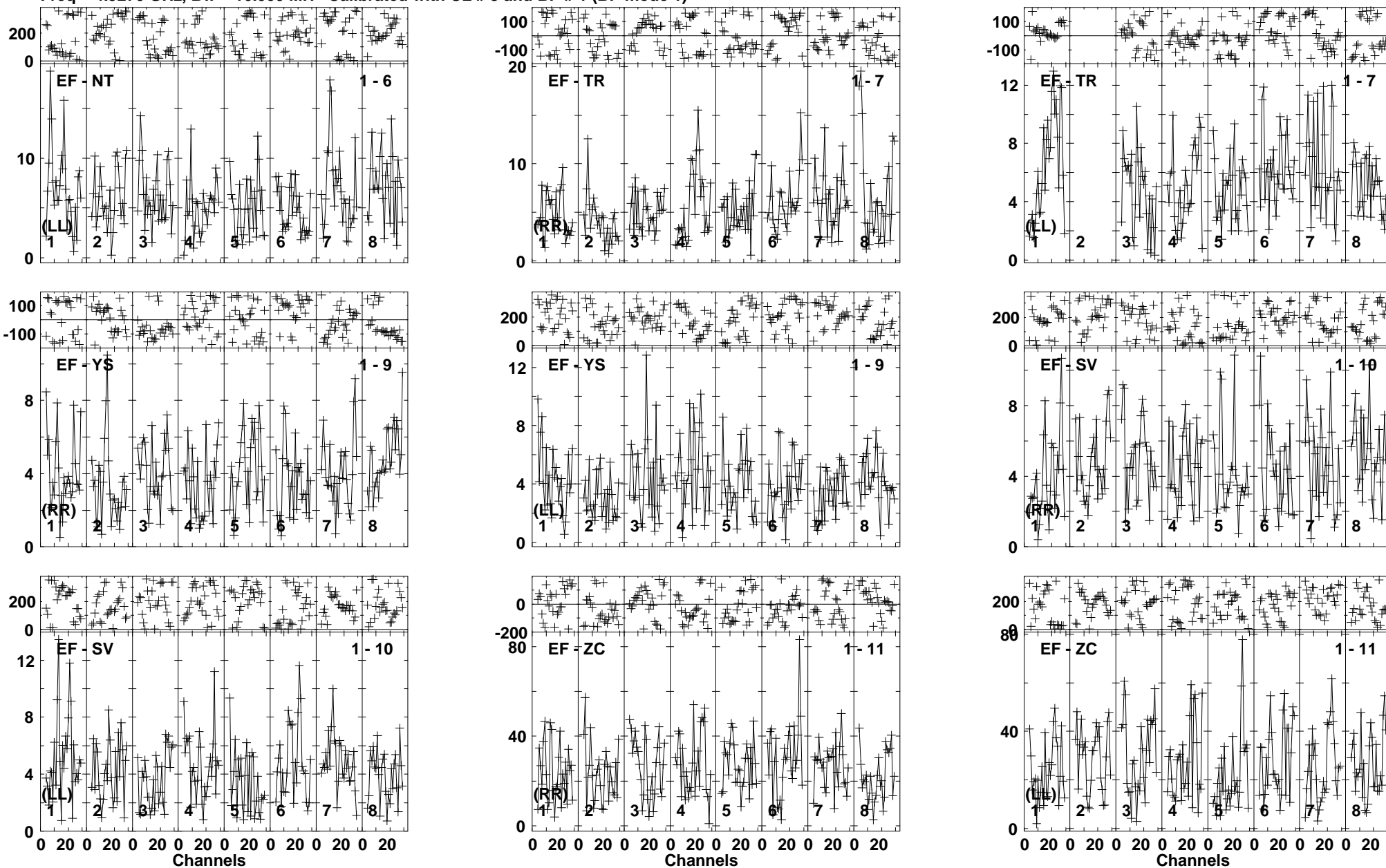
Lower frame: Milli Ampl Jy Top frame: Phas deg Vector averaged cross-power spectrum Baseline: EF (01) - NT (06) Timerange: 00/20:23:55 to 00/20:27:49
