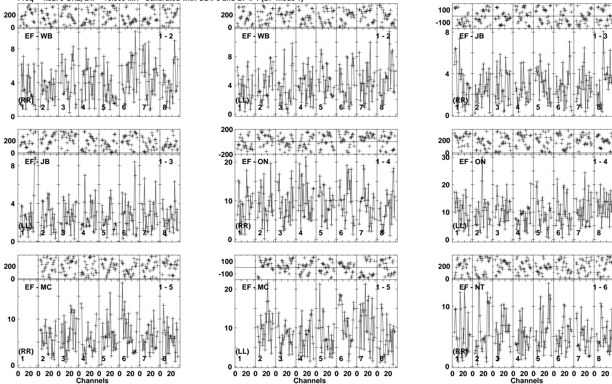
Lower frame: Milli Ampl Jy Top frame: Phas deg Vector averaged cross-power spectrum Baseline: EF (01) - WB (02) Timerange: 00/19:33:25 to 00/19:37:19
