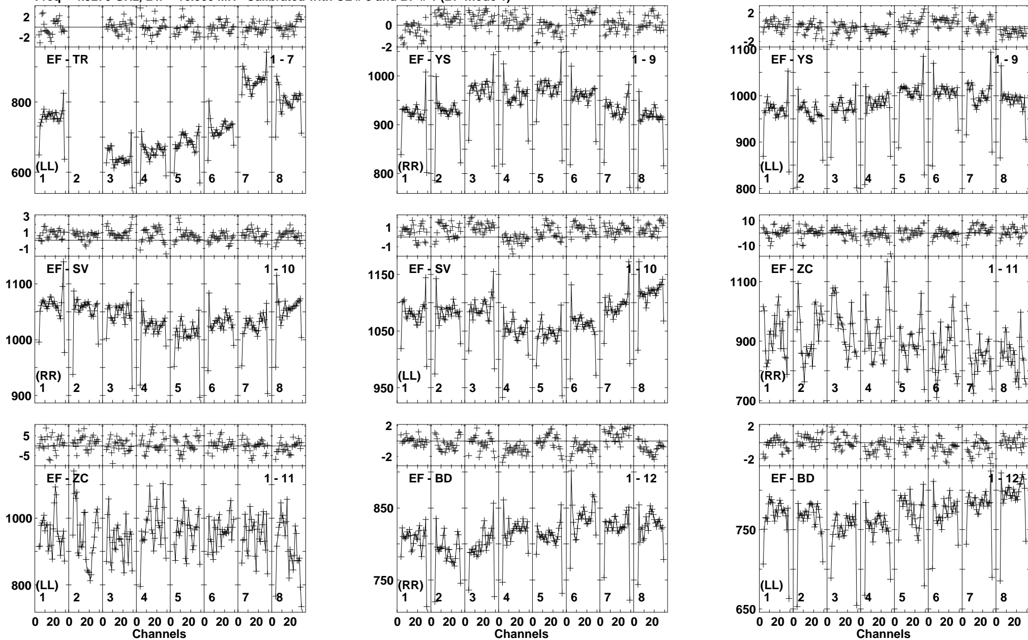
Lower frame: Milli Ampl Jy Top frame: Phas deg Vector averaged cross-power spectrum Baseline: EF (01) - TR (07) Timerange: 00/20:28:33 to 00/20:28:59
