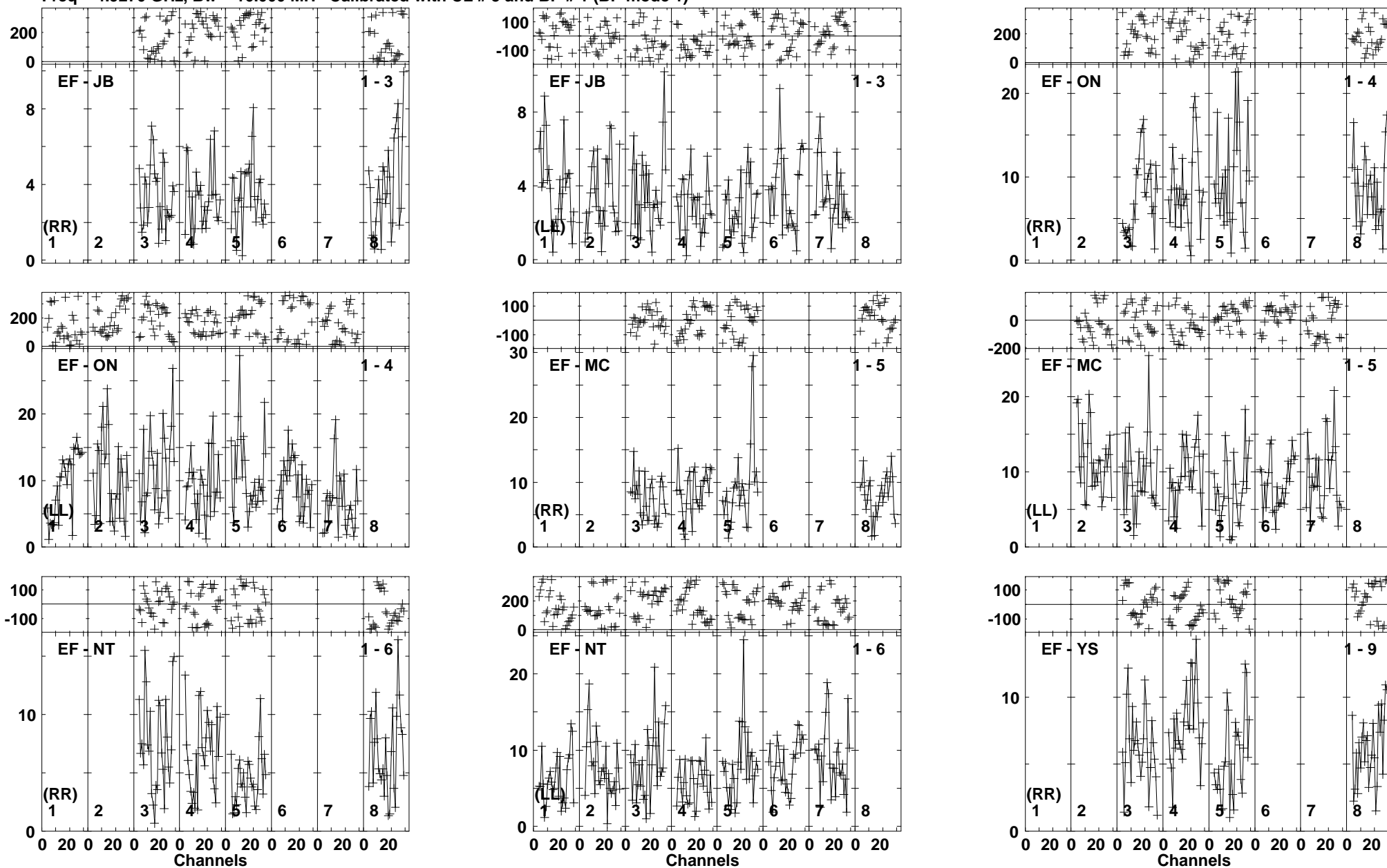
Lower frame: Milli Ampl Jy Top frame: Phas deg Vector averaged cross-power spectrum Baseline: EF (01) - JB (03) Timerange: 00/16:46:33 to 00/16:50:29
