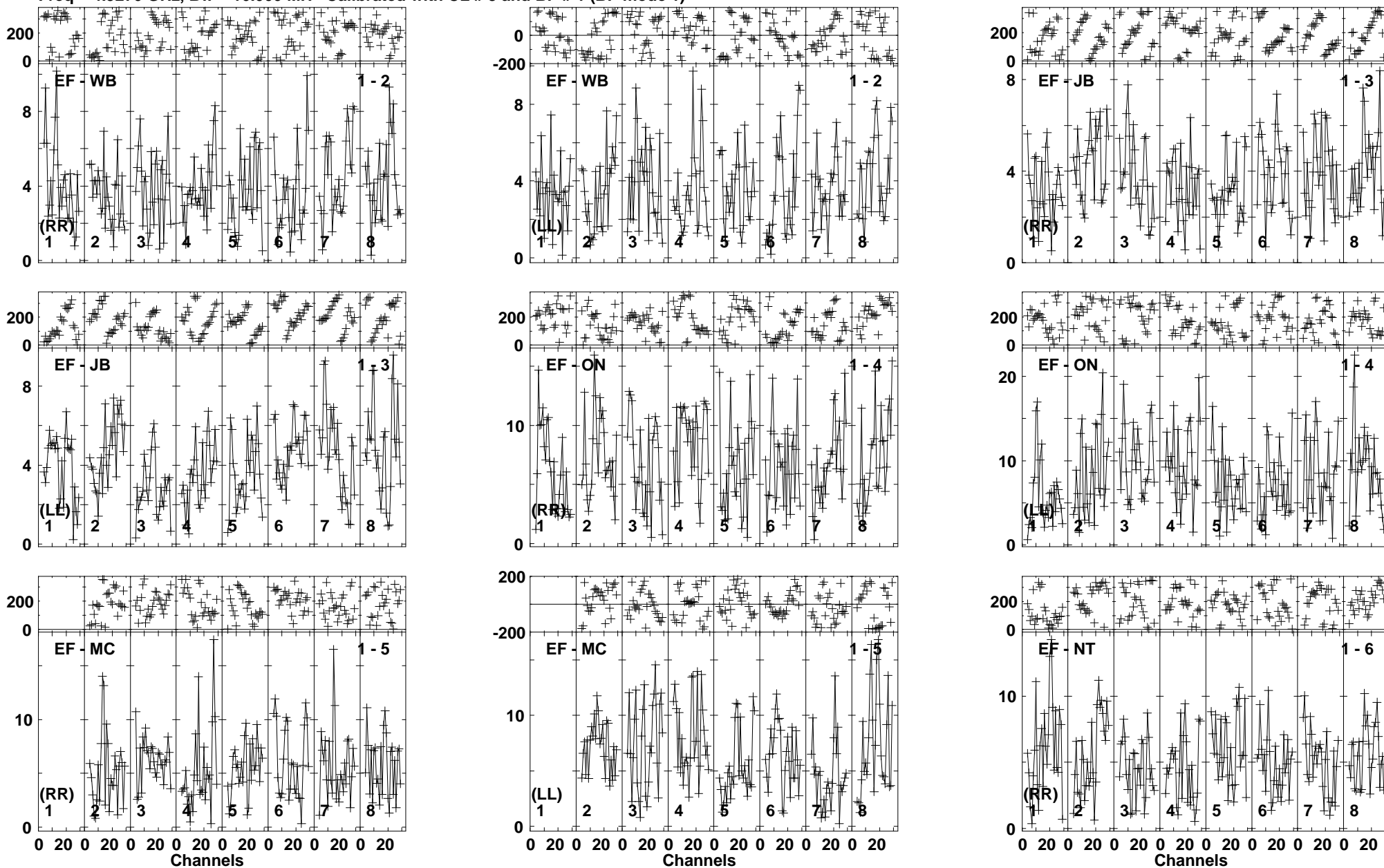
Lower frame: Milli Ampl Jy Top frame: Phas deg Vector averaged cross-power spectrum Baseline: EF (01) - WB (02) Timerange: 00/21:09:23 to 00/21:13:19
