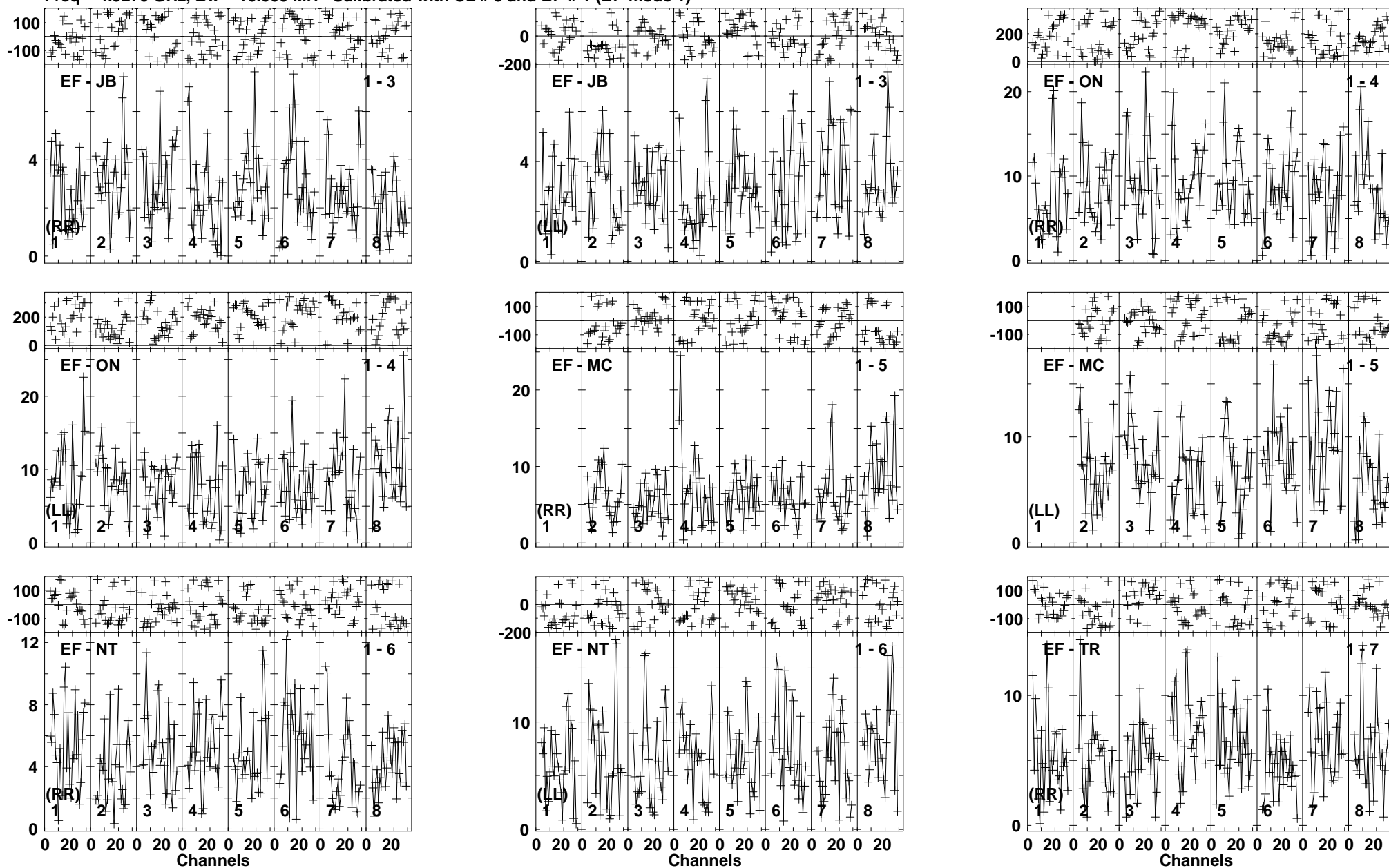
Lower frame: Milli Ampl Jy Top frame: Phas deg Vector averaged cross-power spectrum Baseline: EF (01) - JB (03) Timerange: 00/18:22:34 to 00/18:26:28
