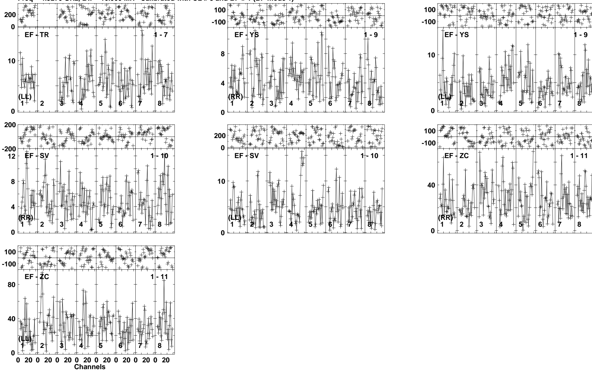
Lower frame: Milli Ampl Jy Top frame: Phas deg Vector averaged cross-power spectrum Baseline: EF (01) - TR (07) Timerange: 00/18:02:24 to 00/18:06:18
