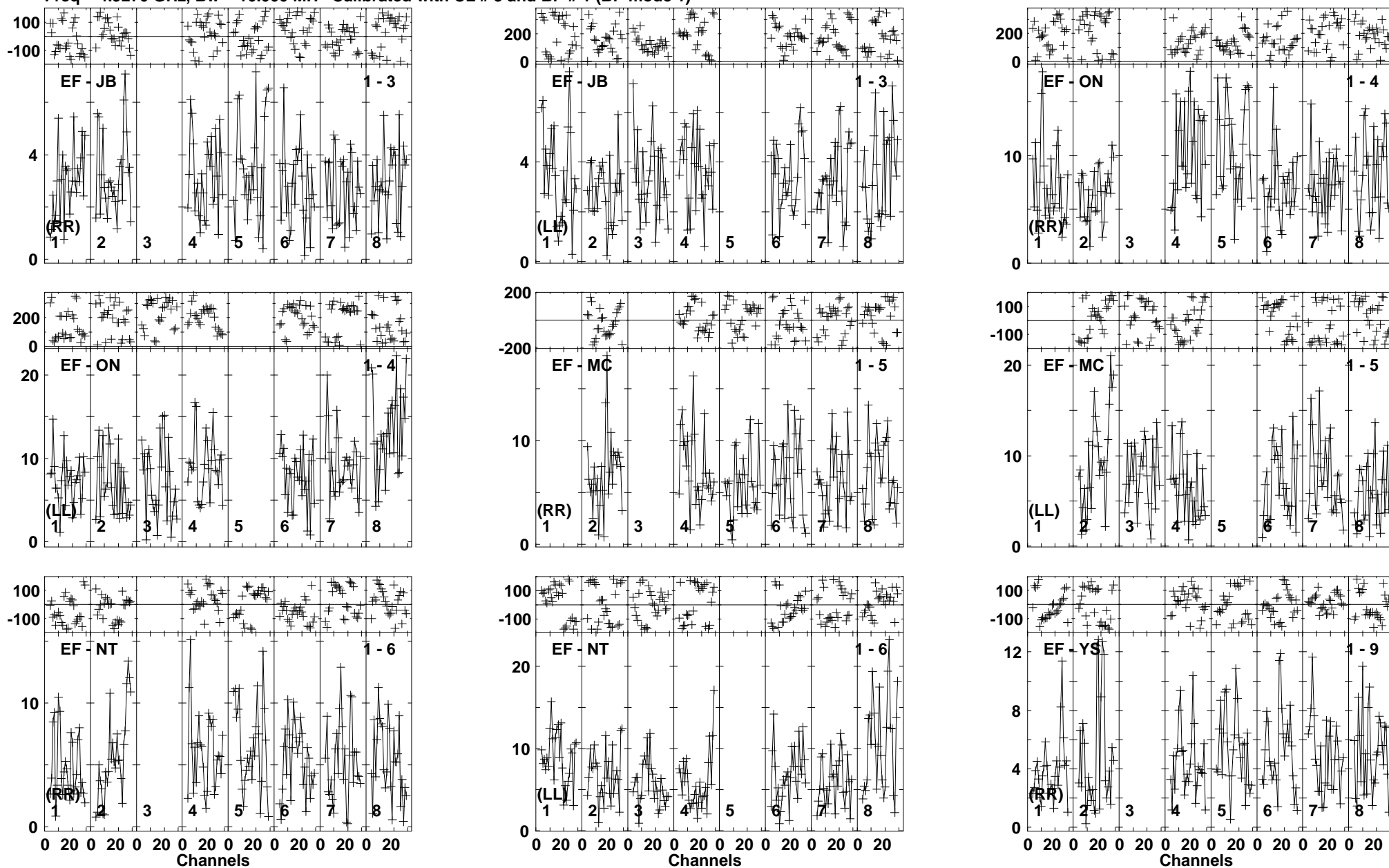
Lower frame: Milli Ampl Jy Top frame: Phas deg Vector averaged cross-power spectrum Baseline: EF (01) - JB (03) Timerange: 00/17:16:53 to 00/17:20:49
