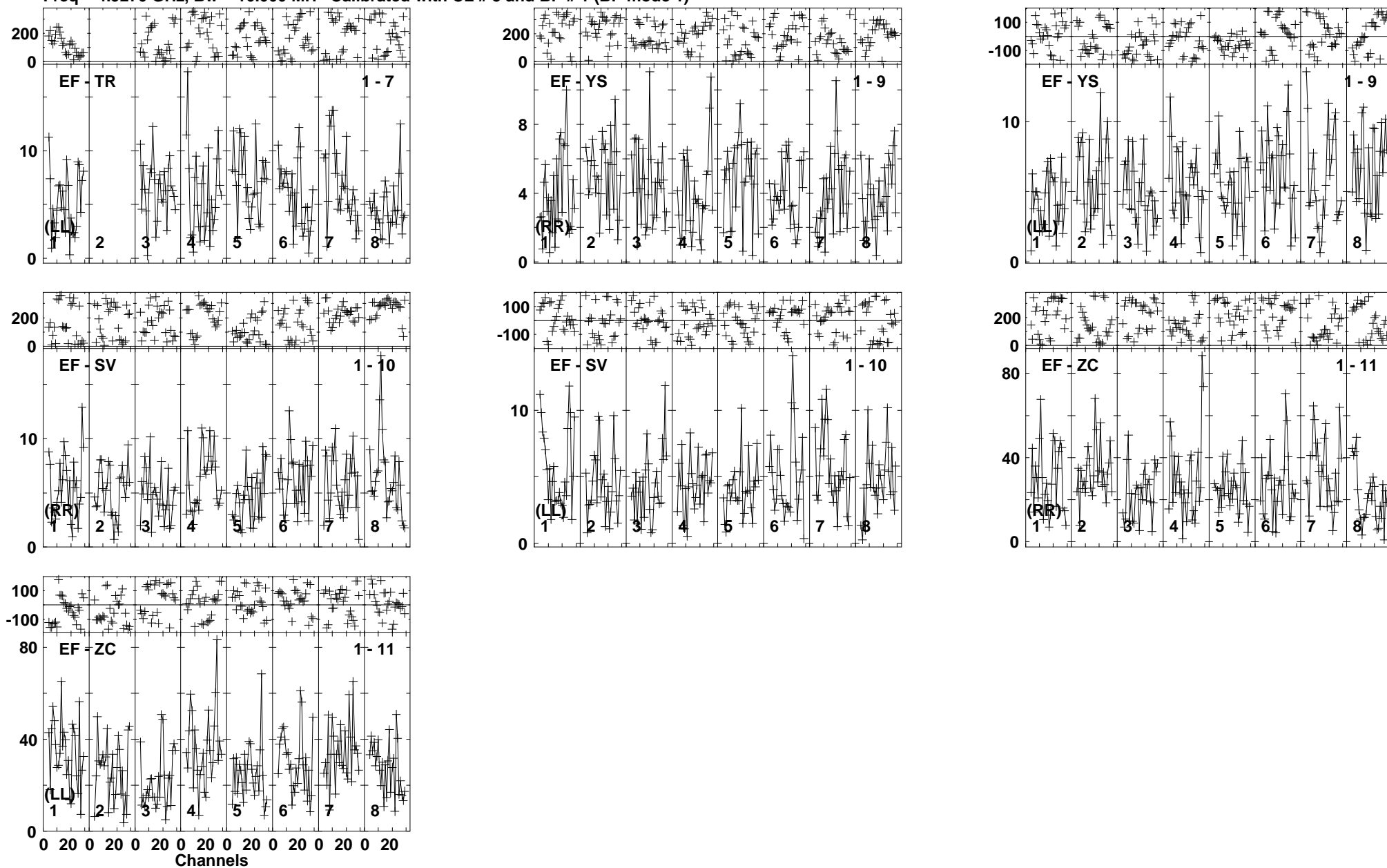
Lower frame: Milli Ampl Jy Top frame: Phas deg Vector averaged cross-power spectrum Baseline: EF (01) - TR (07) Timerange: 00/18:07:23 to 00/18:11:19
