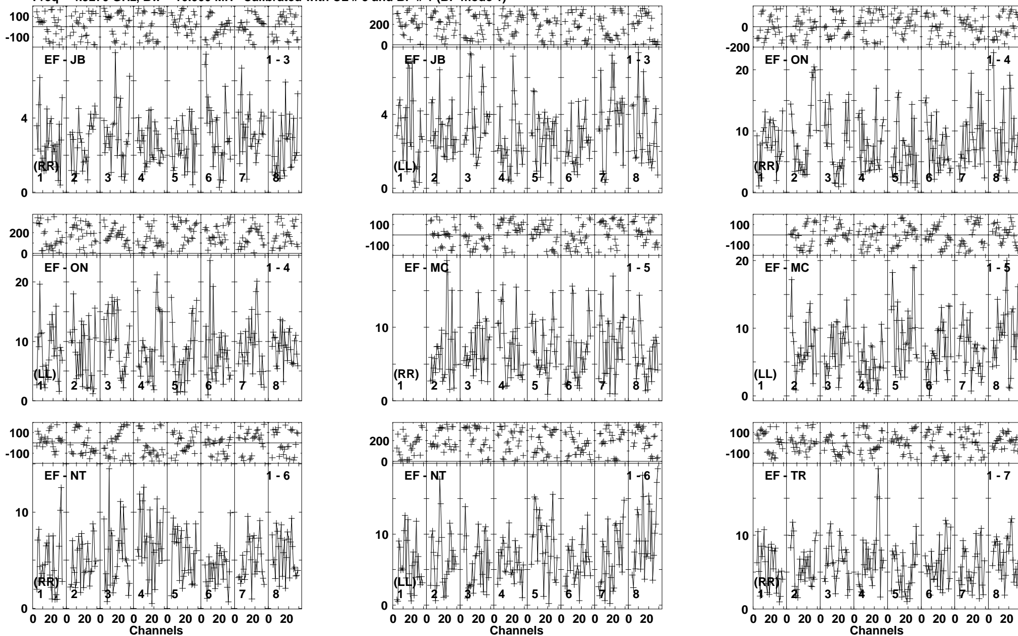
Lower frame: Milli Ampl Jy Top frame: Phas deg Vector averaged cross-power spectrum Baseline: EF (01) - JB (03) Timerange: 00/17:37:03 to 00/17:40:59
