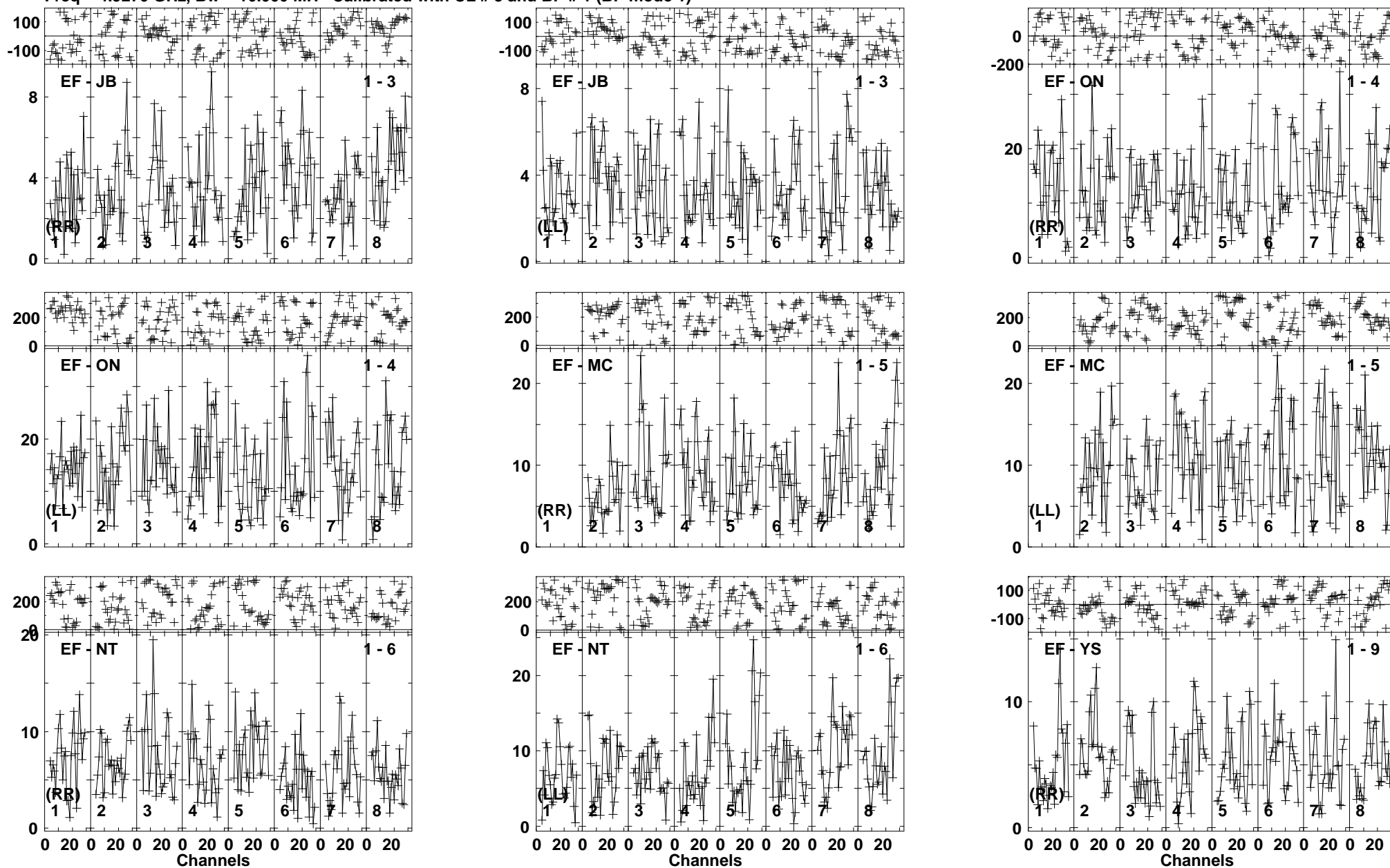
Lower frame: Milli Ampl Jy Top frame: Phas deg Vector averaged cross-power spectrum Baseline: EF (01) - JB (03) Timerange: 00/16:41:34 to 00/16:45:28
