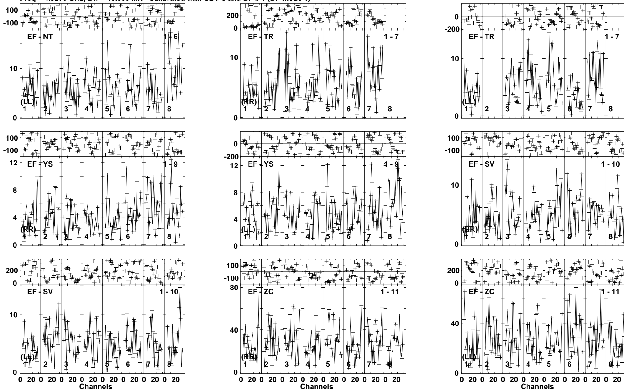
Lower frame: Milli Ampl Jy Top frame: Phas deg Vector averaged cross-power spectrum Baseline: EF (01) - NT (06) Timerange: 00/18:37:43 to 00/18:41:39
