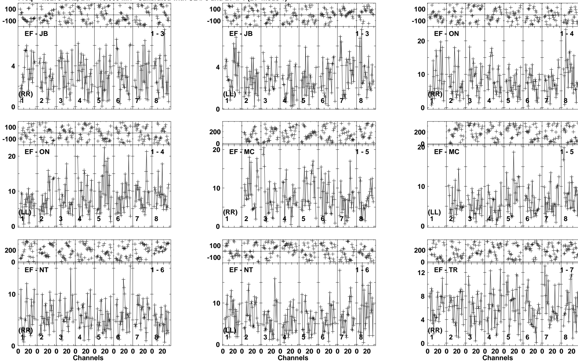
Lower frame: Milli Ampl Jy Top frame: Phas deg Vector averaged cross-power spectrum Baseline: EF (01) - JB (03) Timerange: 00/17:32:04 to 00/17:35:58
