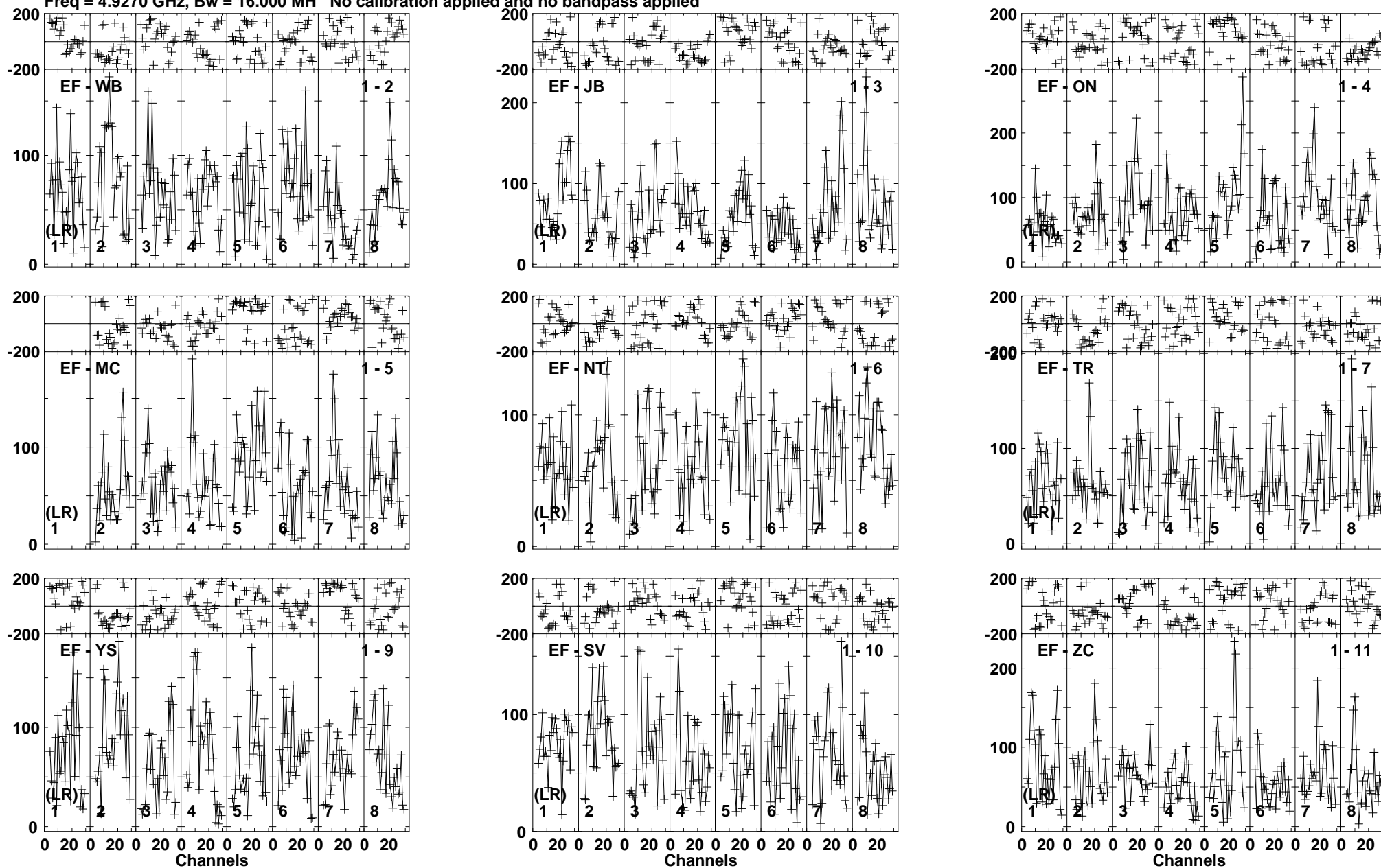
Lower frame: Micro Ampl Jy Top frame: Phas deg Vector averaged cross-power spectrum Baseline: EF (01) - WB (02) Timerange: 00/19:53:35 to 00/19:57:29
