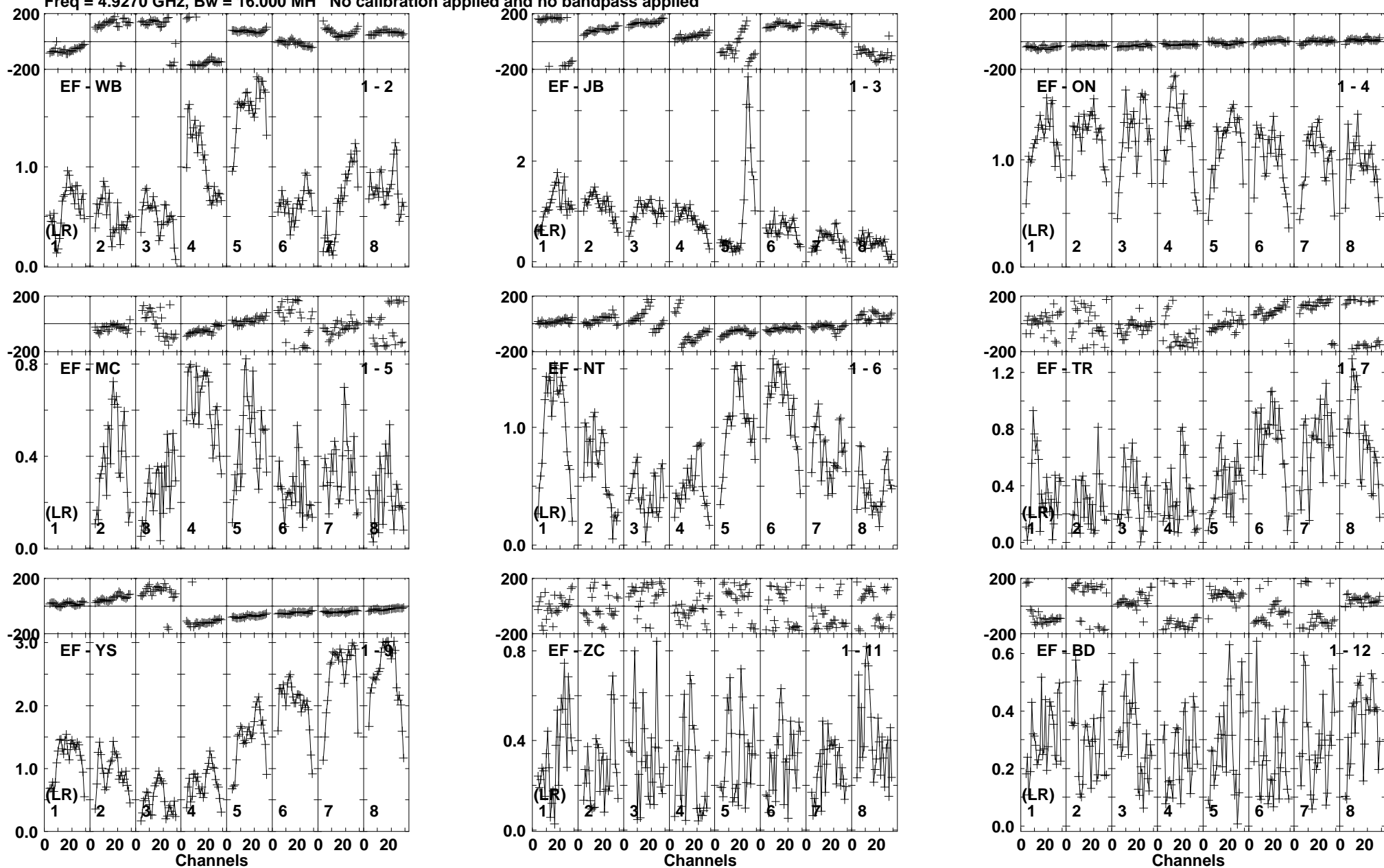
Lower frame: Milli Ampl Jy Top frame: Phas deg Vector averaged cross-power spectrum Baseline: EF (01) - WB (02) Timerange: 00/22:14:23 to 00/22:14:49
