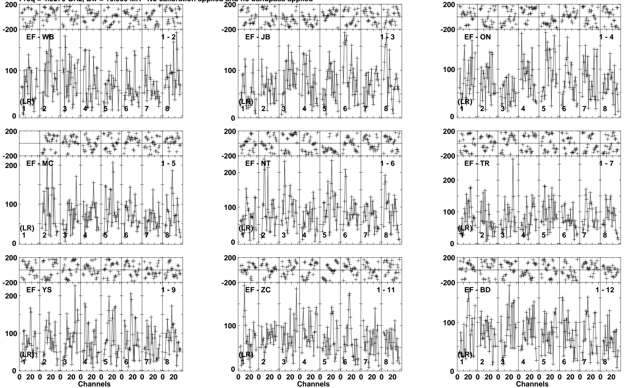
Lower frame: Micro Ampl Jy Top frame: Phas deg Vector averaged cross-power spectrum Baseline: EF (01) - WB (02) Timerange: 00/22:14:55 to 00/22:18:19
