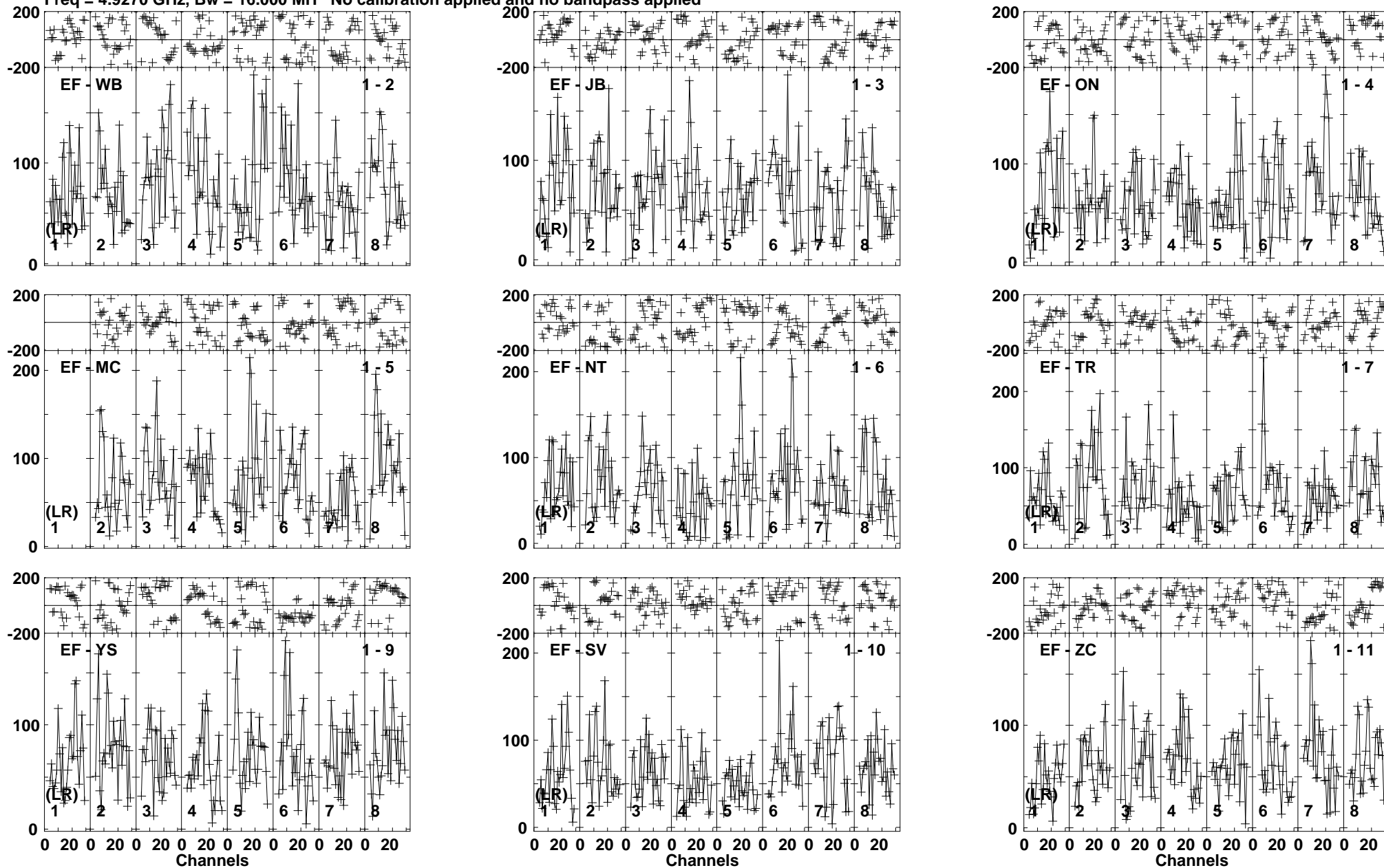
Lower frame: Micro Ampl Jy Top frame: Phas deg Vector averaged cross-power spectrum Baseline: EF (01) - WB (02) Timerange: 00/18:12:33 to 00/18:16:29
