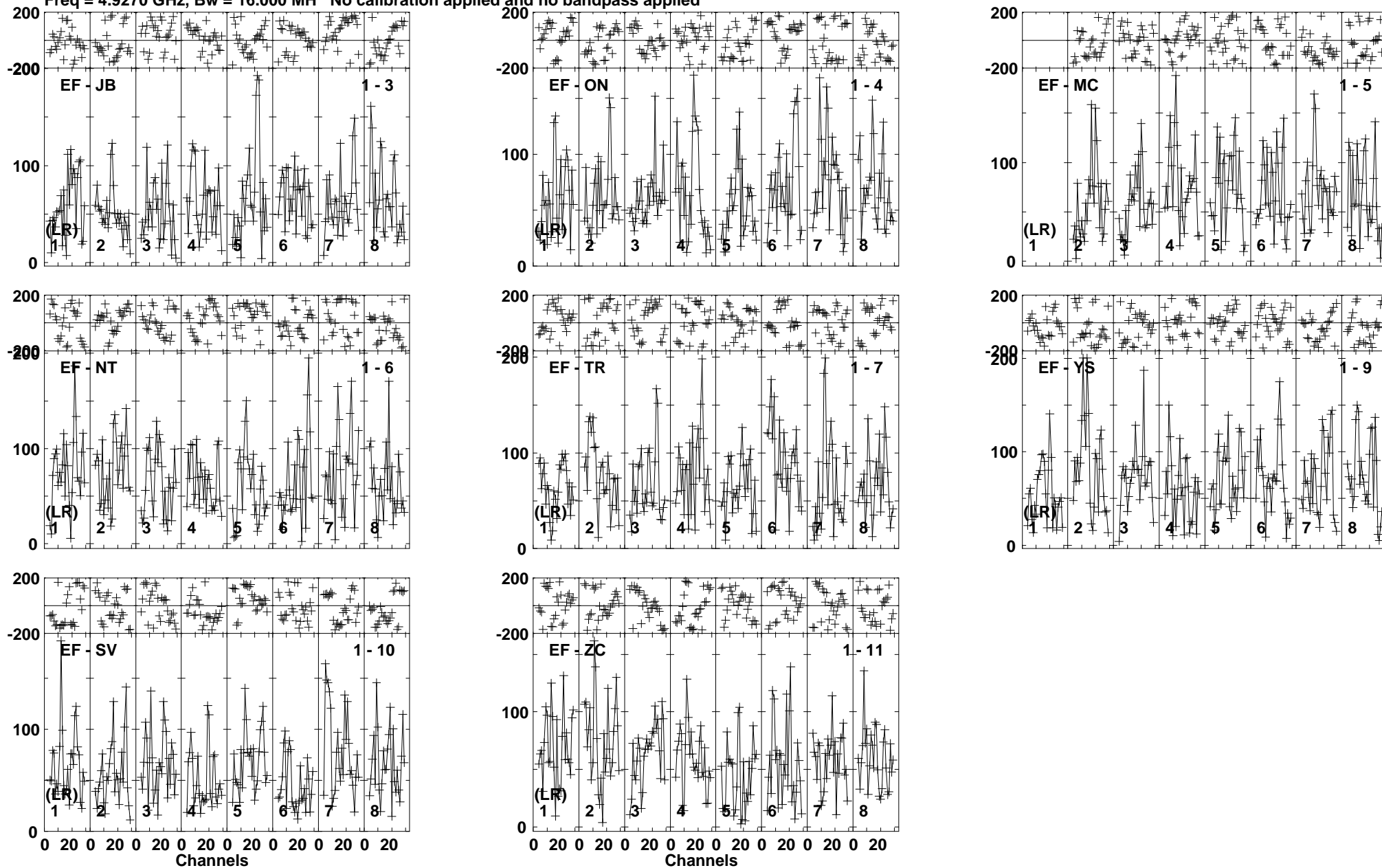
Lower frame: Micro Ampl Jy Top frame: Phas deg Vector averaged cross-power spectrum Baseline: EF (01) - JB (03) Timerange: 00/18:17:33 to 00/18:21:29
