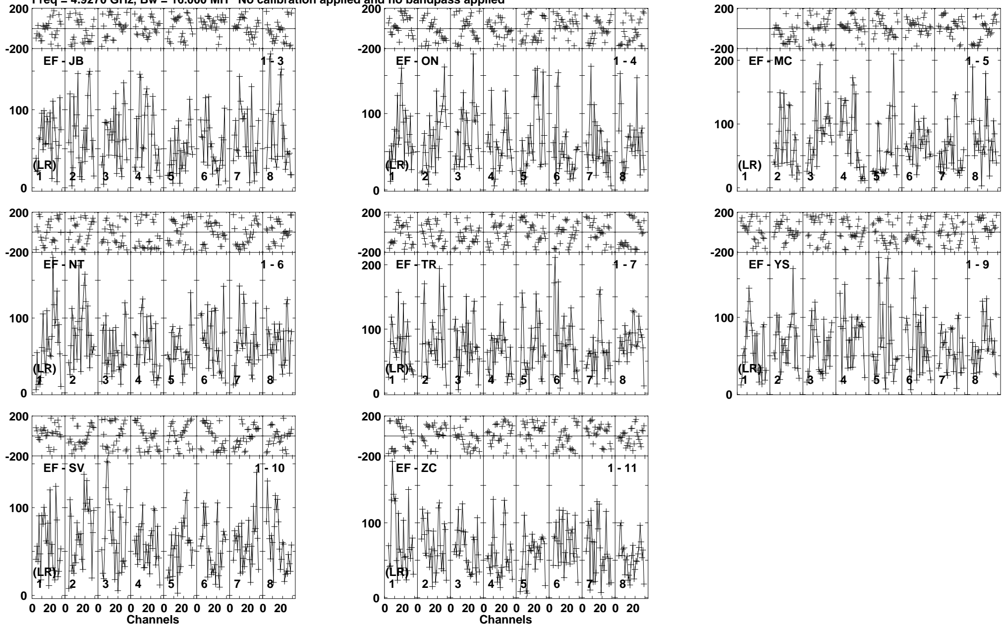
Lower frame: Micro Ampl Jy Top frame: Phas deg Vector averaged cross-power spectrum Baseline: EF (01) - JB (03) Timerange: 00/17:21:54 to 00/17:25:48
