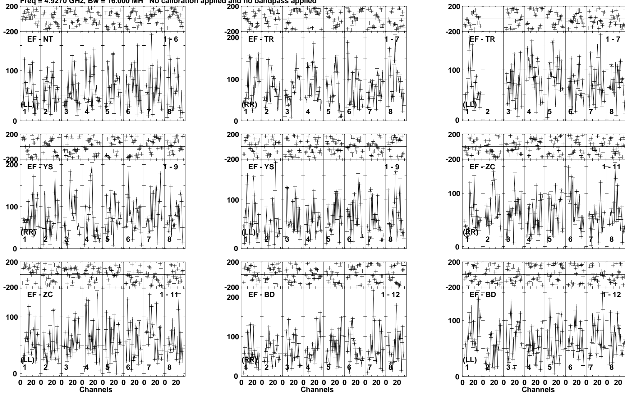
Lower frame: Micro Ampl Jy Top frame: Phas deg Vector average cross-power spectrum Baseline: EF (01) - NT (06) Timerange: 00/22:05:05 to 00/22:08:59
