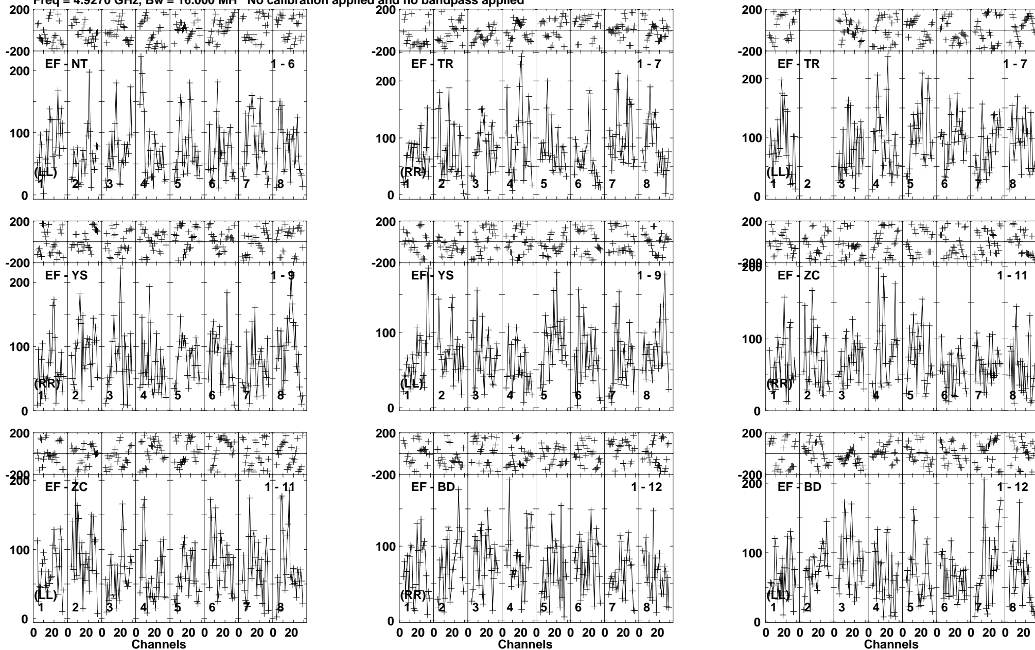
Lower frame: Micro Ampl Jy Top frame: Phas deg Vector averaged cross-power spectrum Baseline: EF (01) - NT (06) Timerange: 00/22:10:03 to 00/22:13:39
