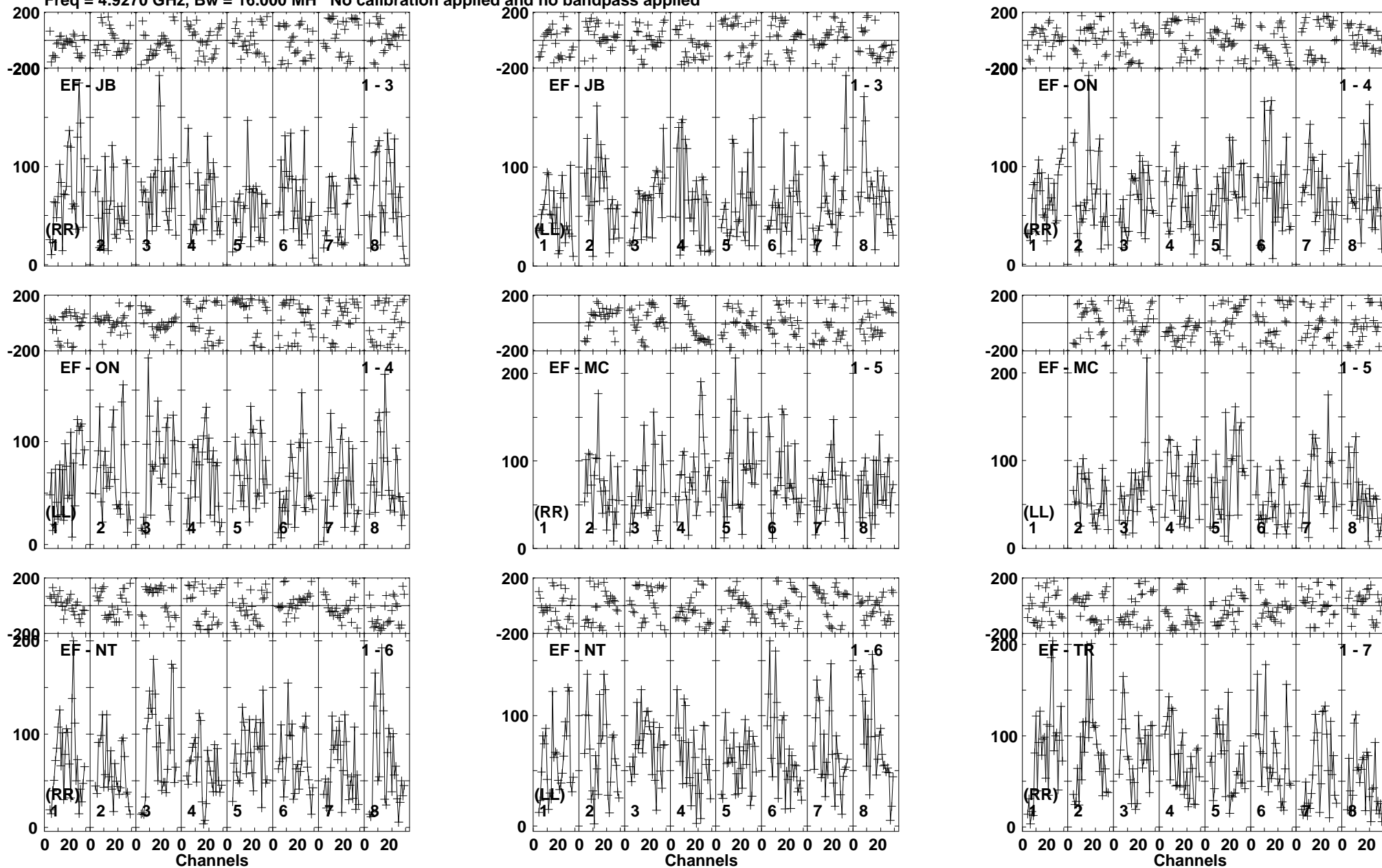
Lower frame: Micro Ampl Jy Top frame: Phas deg Vector averaged cross-power spectrum Baseline: EF (01) - JB (03) Timerange: 00/17:32:04 to 00/17:35:58
