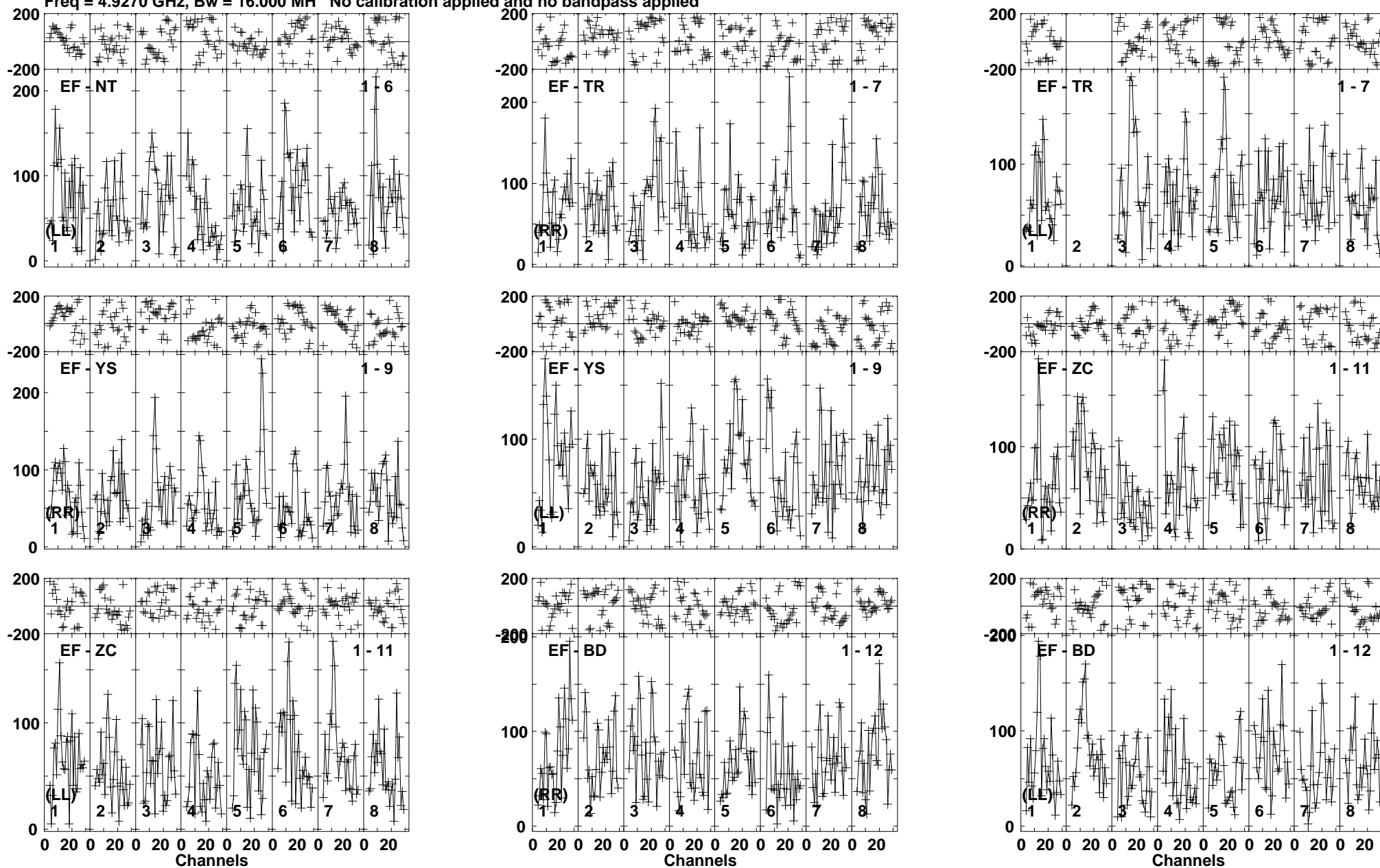
Lower frame: Micro Ampl Jy Top frame: Phas deg Vector averaged cross-power spectrum Baseline: EF (01) - NT (06) Timerange: 00/21:39:43 to 00/21:43:39
