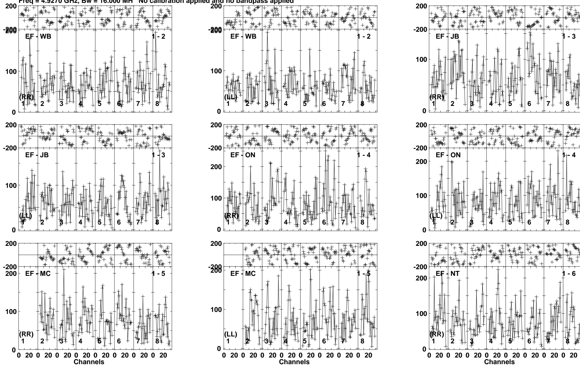
Lower frame: Micro Ampl Jy Top frame: Phas deg Vector averaged cross-power spectrum Baseline: EF (01) - WB (02) Timerange: 00/20:08:43 to 00/20:12:39
