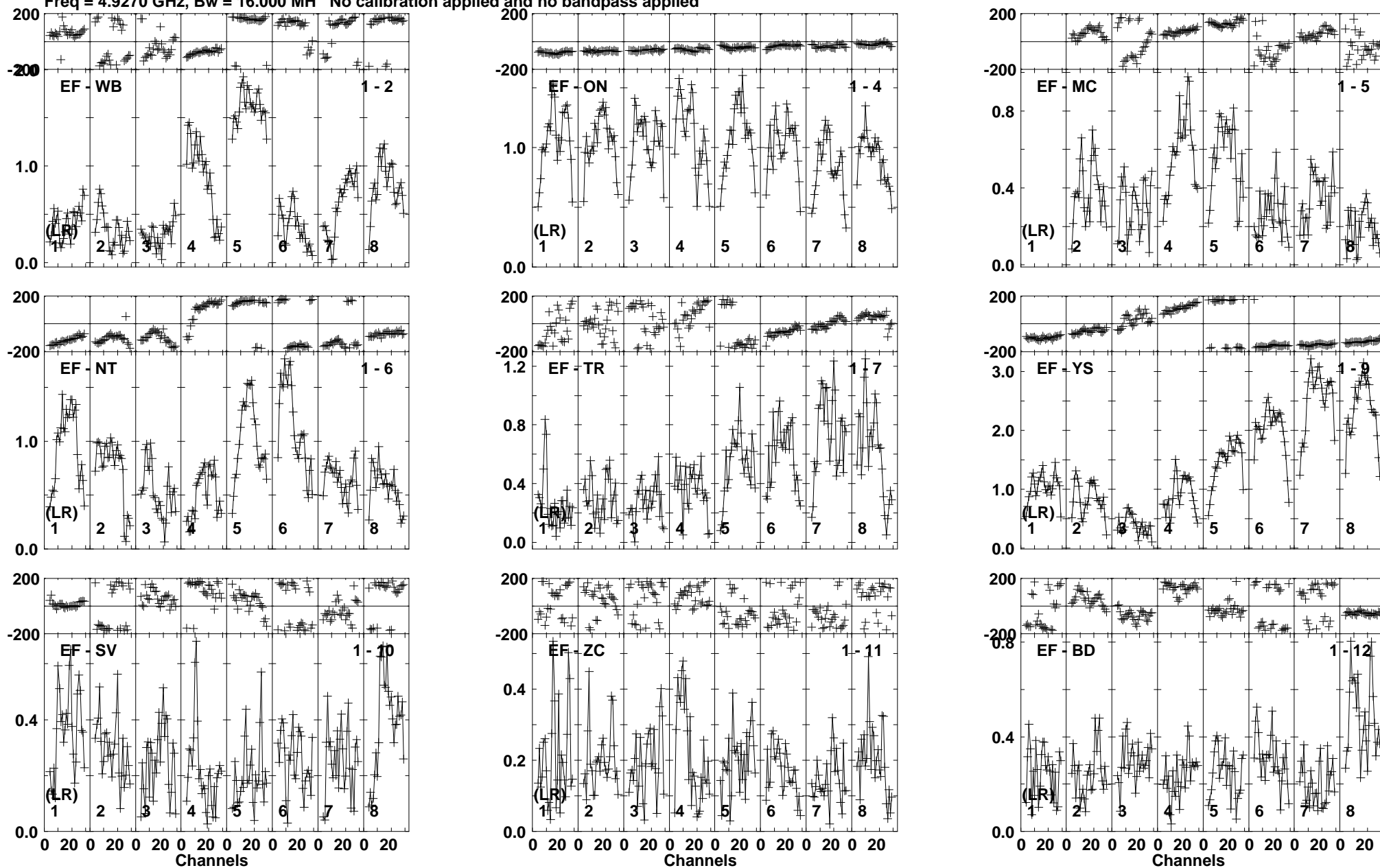
Lower frame: Milli Ampl Jy Top frame: Phas deg Vector averaged cross-power spectrum Baseline: EF (01) - WB (02) Timerange: 00/20:58:53 to 00/20:59:19
