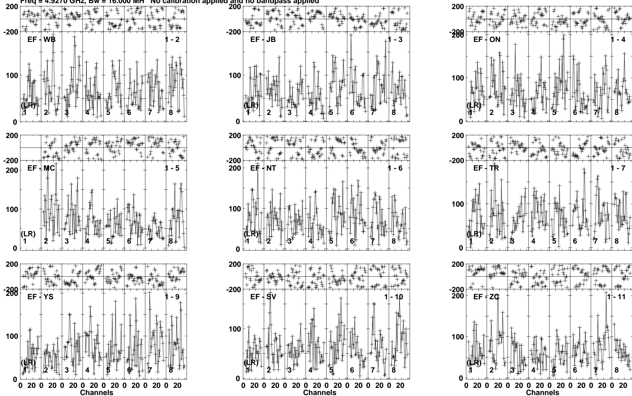
Lower frame: Micro Ampl Jy Top frame: Phas deg Vector averaged cross-power spectrum Baseline: EF (01) - WB (02) Timerange: 00/20:59:23 to 00/21:03:19
