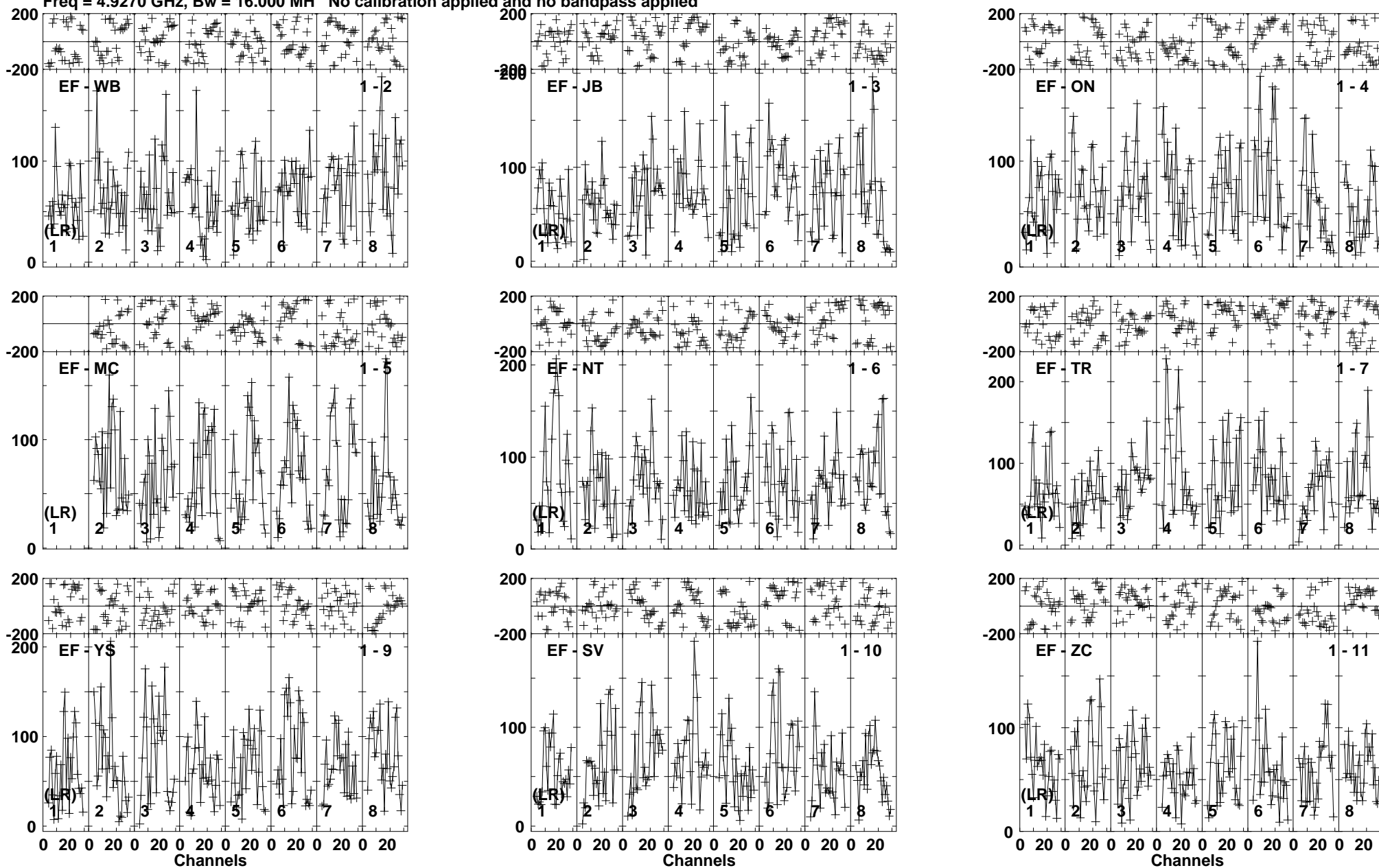
Lower frame: Micro Ampl Jy Top frame: Phas deg Vector averaged cross-power spectrum Baseline: EF (01) - WB (02) Timerange: 00/21:14:35 to 00/21:18:29
