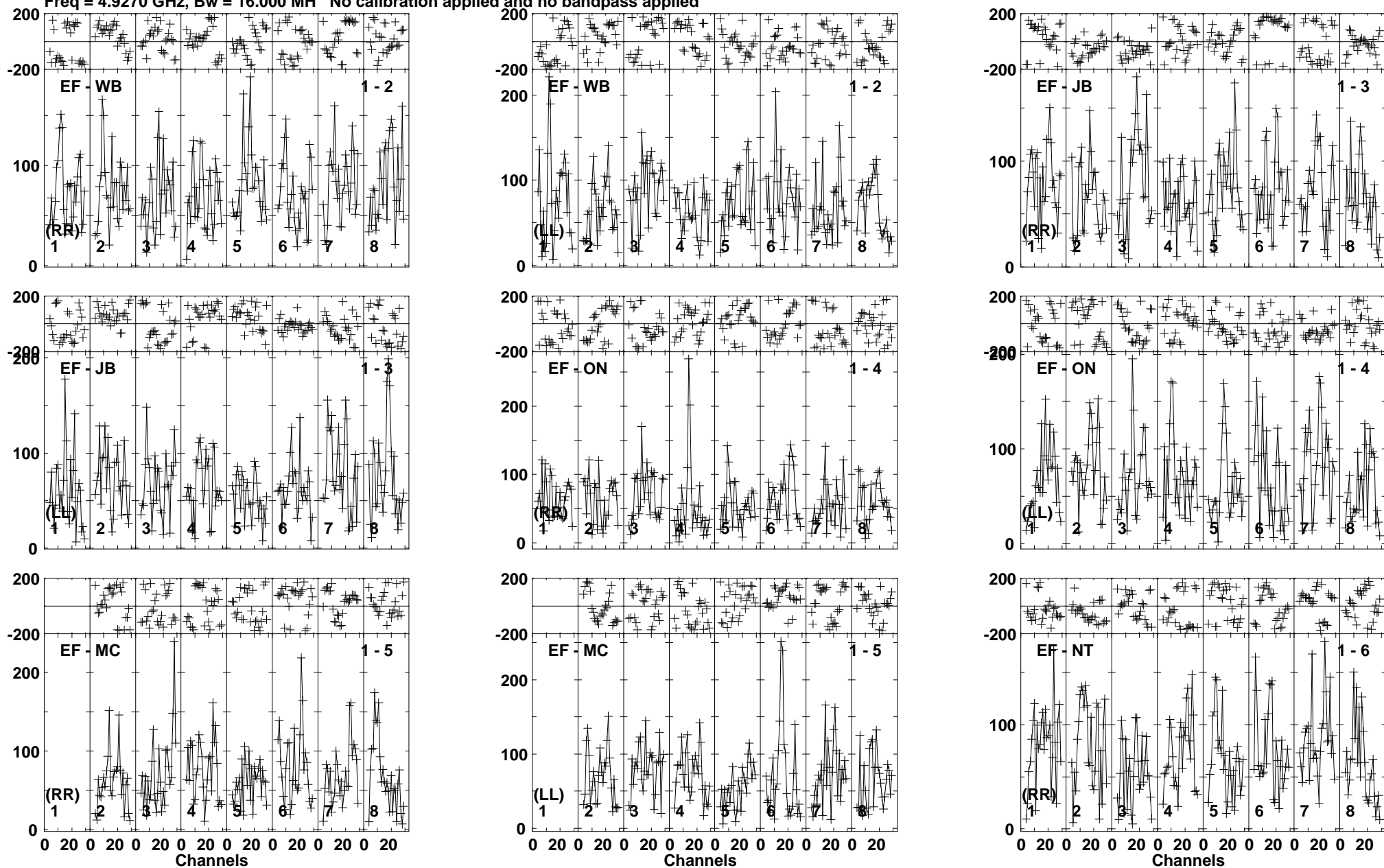
Lower frame: Micro Ampl Jy Top frame: Phas deg Vector averaged cross-power spectrum Baseline: EF (01) - WB (02) Timerange: 00/21:04:25 to 00/21:08:19
