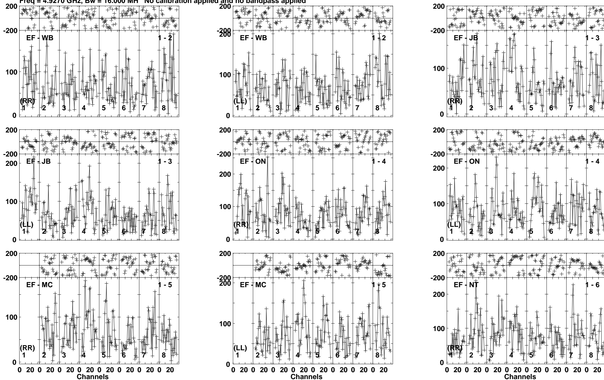
Lower frame: Micro Ampl Jy Top frame: Phas deg Vector averaged cross-power spectrum Baseline: EF (01) - WB (02) Timerange: 00/20:34:05 to 00/20:37:59
