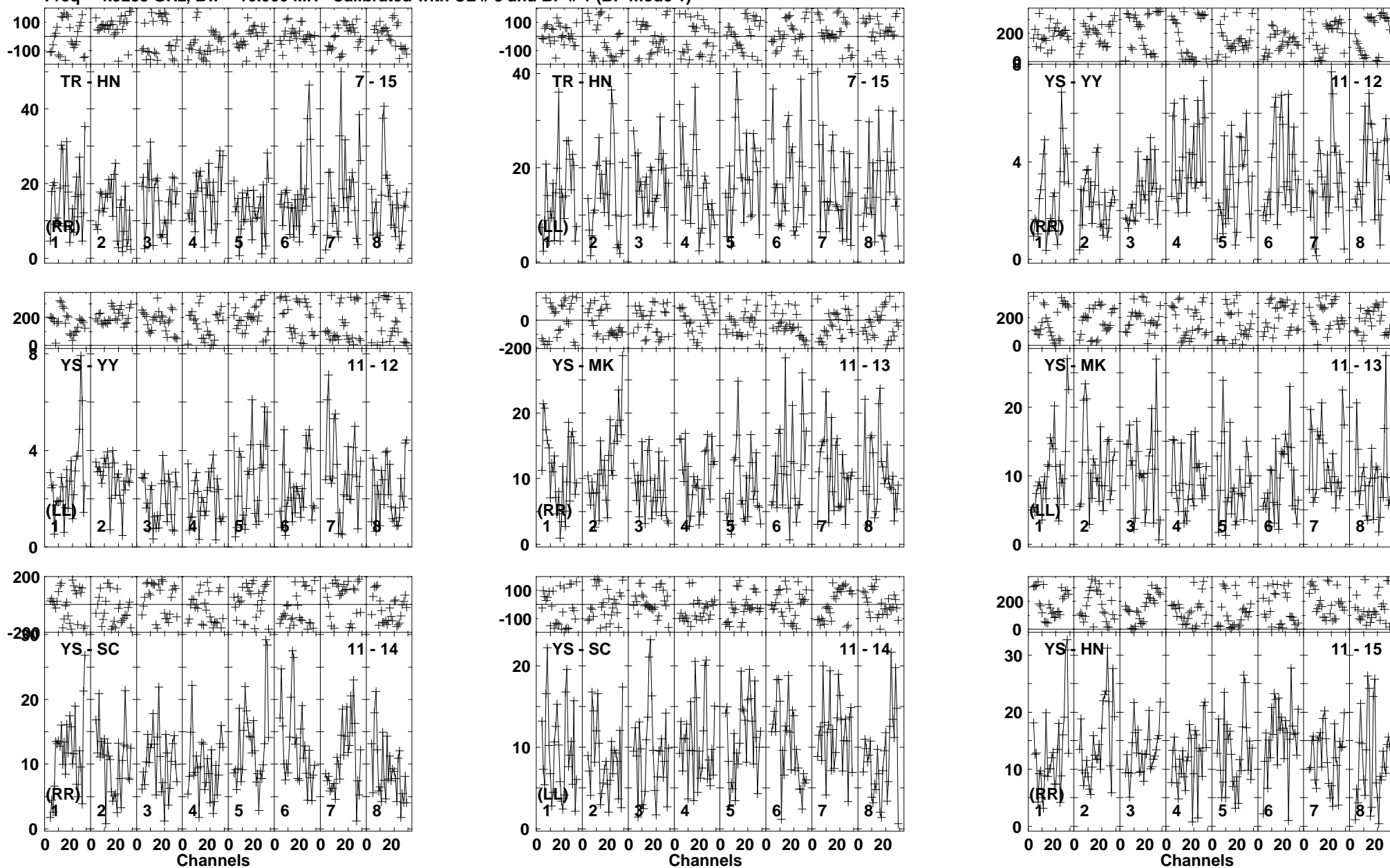
Lower frame: Milli Ampl Jy Top frame: Phas deg Vector averaged cross-power spectrum Baseline: TR (07) - HN (15) Timerange: 01/00:44:23 to 01/00:49:35
