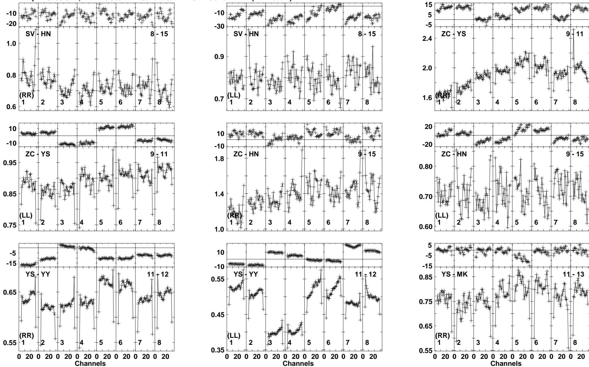
Lower frame: Ampl Jy Top frame: Phas deg Vector averaged cross-power spectrum Baseline: SV (08) - HN (15) Timerange: 00/23:23:11 to 00/23:25:03
