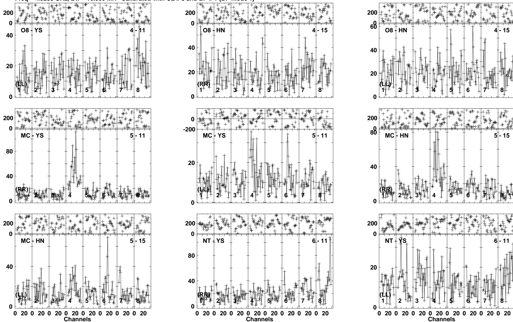
Lower frame: Milli Ampl Jy Top frame: Phas deg Vector averaged cross-spectrum Baseline: O8 (04) - YS (11) Timerange: 00/21:00:58 to 00/21:06:12
