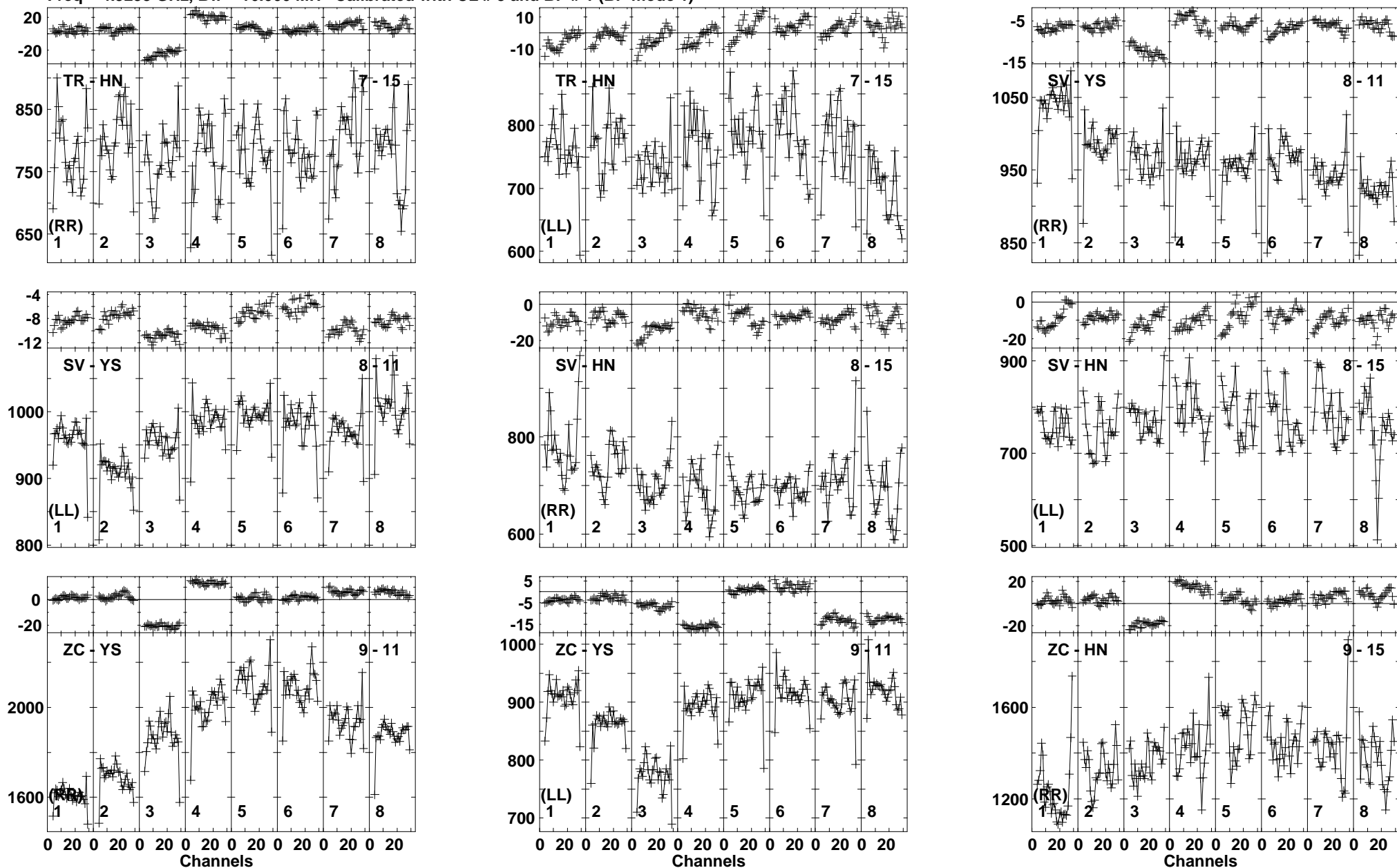
Lower frame: Milli Ampl Jy Top frame: Phas deg Vector averaged cross-power spectrum Baseline: TR (07) - HN (15) Timerange: 00/22:32:49 to 00/22:34:32
