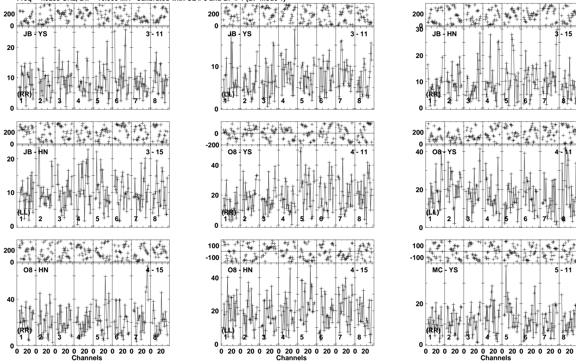
Lower frame: Milli Ampl Jy Top frame: Phas deg Vector averaged cross-power spectrum Baseline: JB (03) - YS (11) Timerange: 01/00:01:08 to 01/00:06:20
