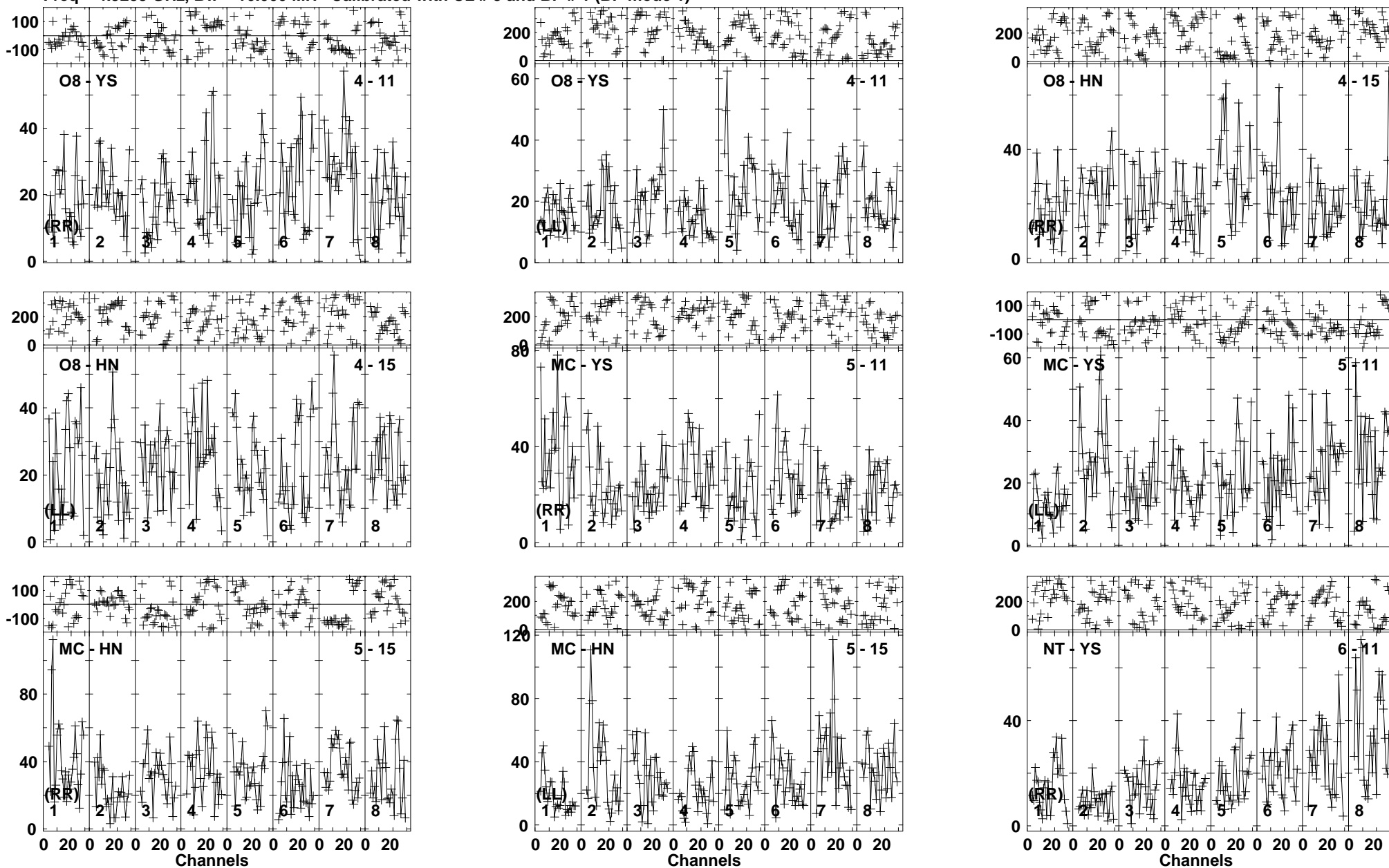
Lower frame: Milli Ampl Jy Top frame: Phas deg Vector averaged cross-power spectrum Baseline: O8 (04) - YS (11) Timerange: 01/02:18:08 to 01/02:23:22
