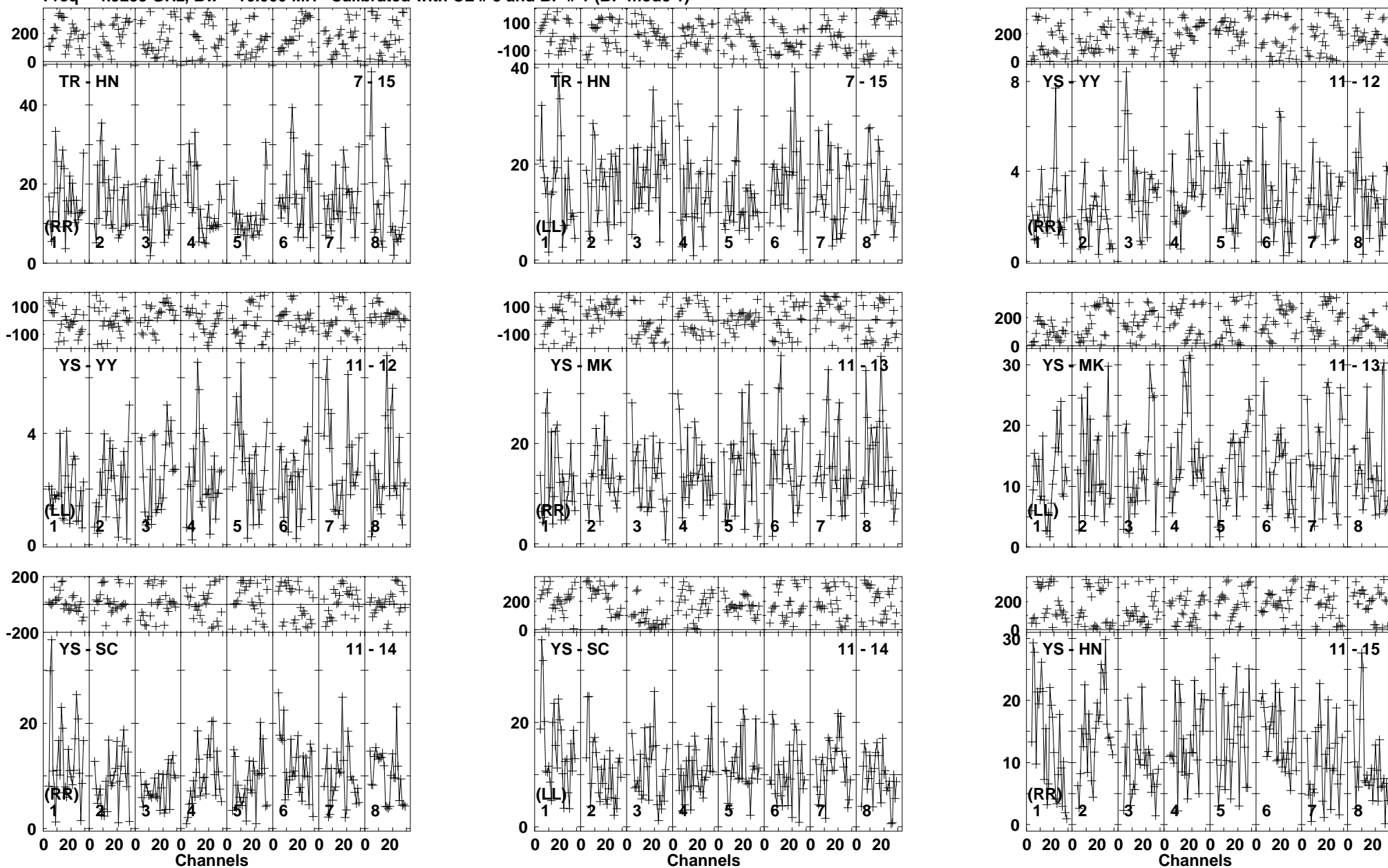
Lower frame: Milli Ampl Jy Top frame: Phas deg Vector averaged cross-power spectrum Baseline: TR (07) - HN (15) Timerange: 00/21:29:48 to 00/21:35:02
