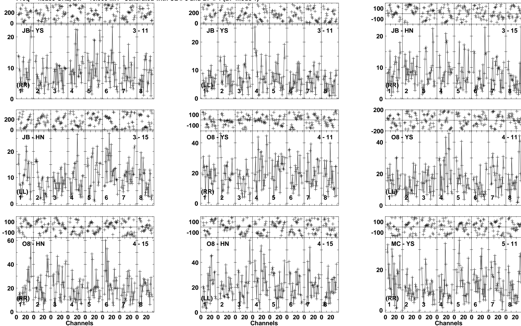
Lower frame: Milli Ampl Jy Top frame: Phas deg Vector averaged cross-power spectrum Baseline: JB (03) - YS (11) Timerange: 01/00:51:38 to 01/00:56:52
