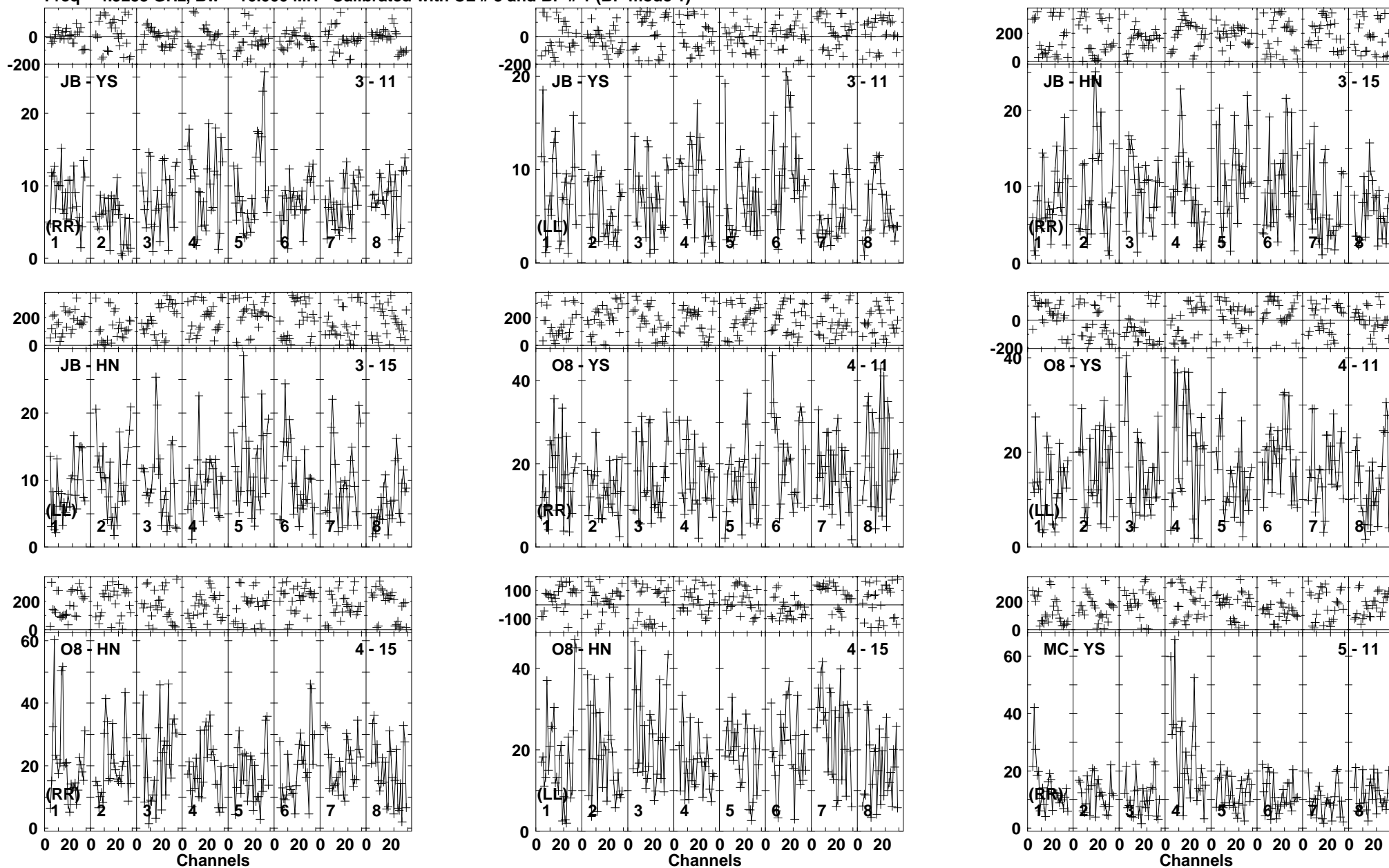
Lower frame: Milli Ampl Jy Top frame: Phas deg Vector averaged cross-power spectrum Baseline: JB (03) - YS (11) Timerange: 00/22:49:03 to 00/22:54:15
