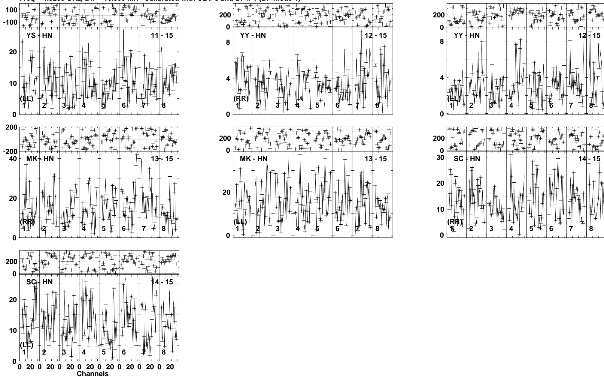
Lower frame: Milli Ampl Jy Top frame: Phas deg Vector averaged cross-power spectrum Baseline: YS (11) - HN (15) Timerange: 00:22:27:28 to 00:22:32:42
