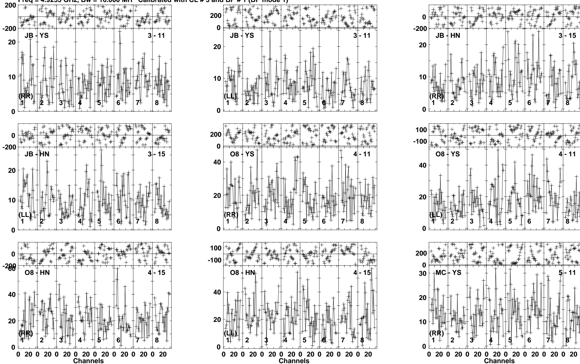
Lower frame: Milli Ampl Jy Top frame: Phas deg Vector averaged cross-power spectrum Baseline: JB (03) - YS (11) Timerange: 01/00:29:58 to 01/00:35:10
