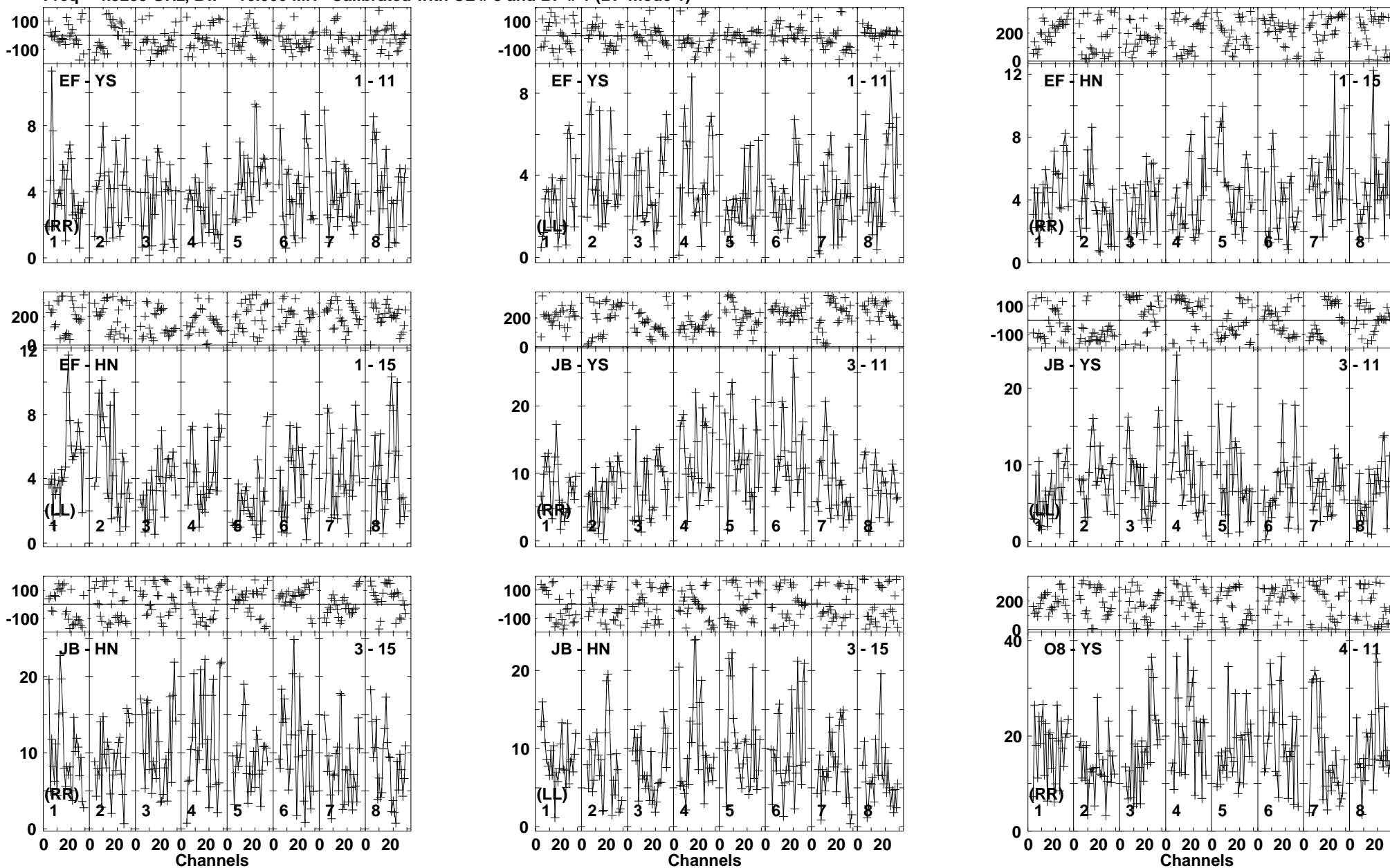
Lower frame: Milli Ampl Jy Top frame: Phas deg Vector averaged cross-power spectrum Baseline: EF (01) - YS (11) Timerange: 00/20:46:33 to 00/20:51:47
