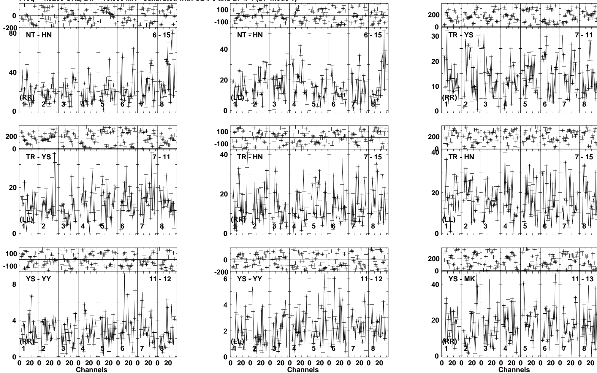
Lower frame: Milli Ampl Jy Top frame: Phas deg Vector averaged cross-power spectrum Baseline: NT (06) - HN (15) Timerange: 00/21:00:58 to 00/21:06:12
