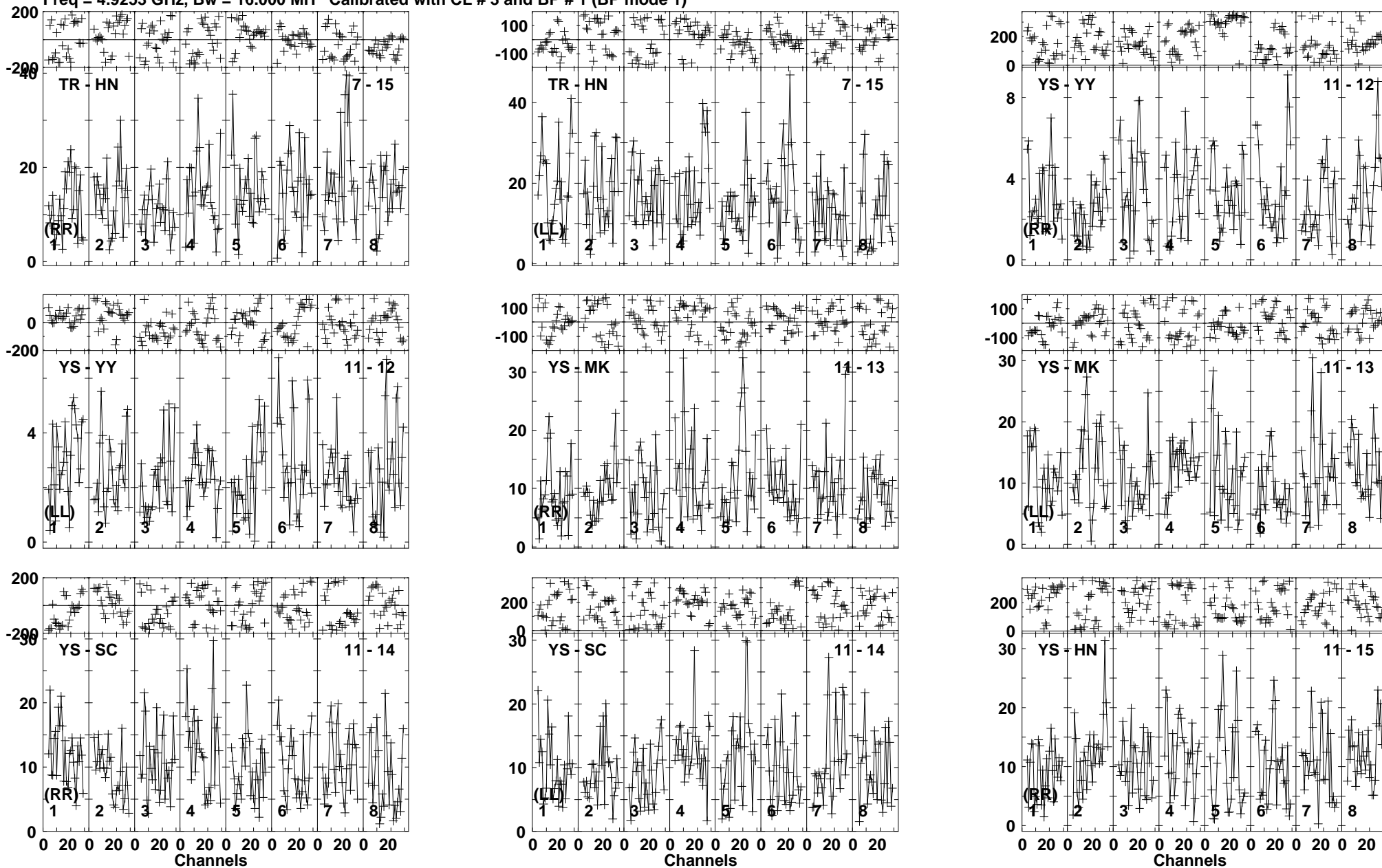
Lower frame: Milli Ampl Jy Top frame: Phas deg Vector averaged cross-power spectrum Baseline: TR (07) - HN (15) Timerange: 00/23:32:18 to 00/23:37:30
