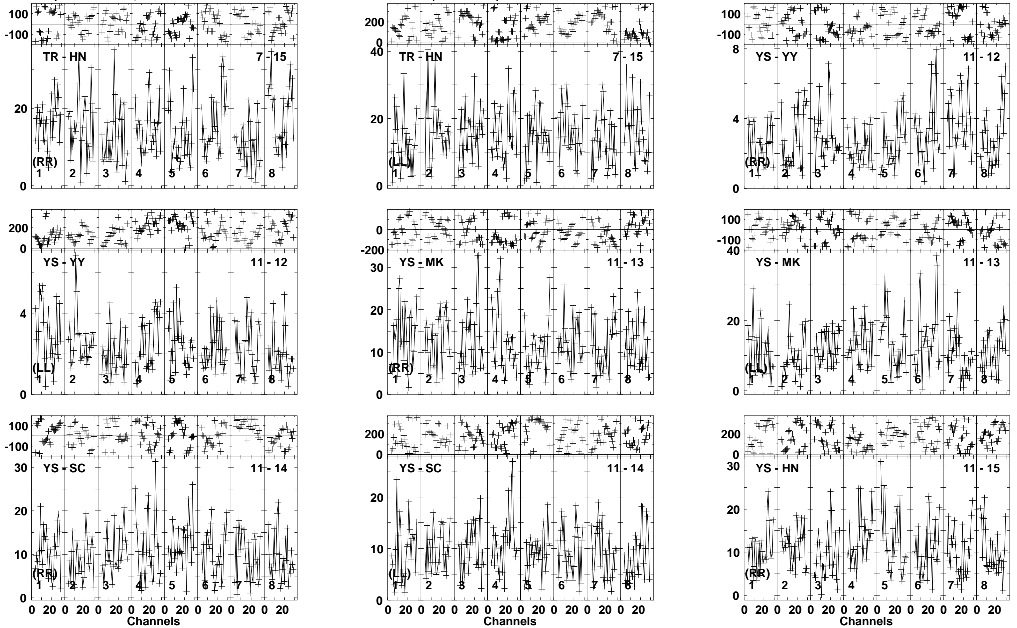
Lower frame: Milli Ampl Jy Top frame: Phas deg Vector averaged cross-power spectrum Baseline: TR (07) - HN (15) Timerange: 00/23:10:43 to 00/23:15:57
