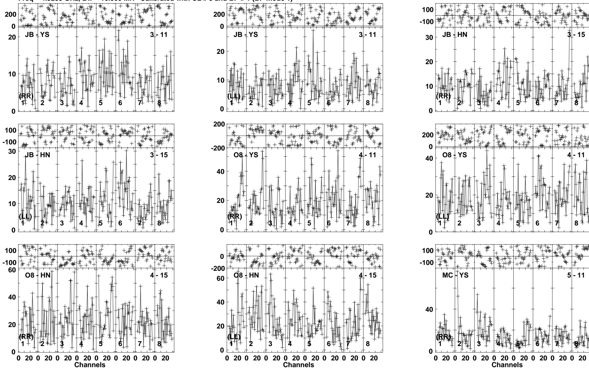
Lower frame: Milli Ampl Jy Top frame: Phas deg Vector averaged cross-power spectrum Baseline: JB (03) - YS (11) Timerange: 01/02:03:43 to 01/02:08:57
