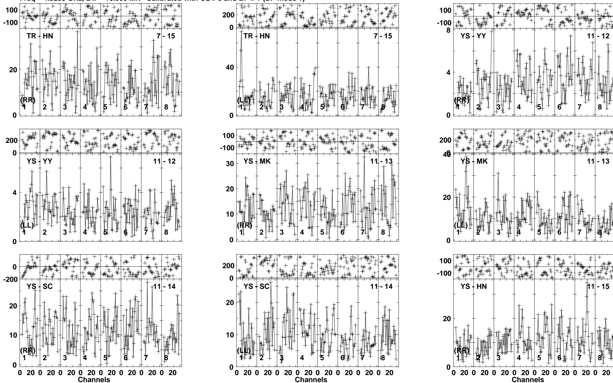
Lower frame: Milli Ampl Jy Top frame: Phas deg Vector averaged cross-power spectrum Baseline: TR (07) - HN (15) Timerange: 00/23:17:53 to 00/23:23:05
