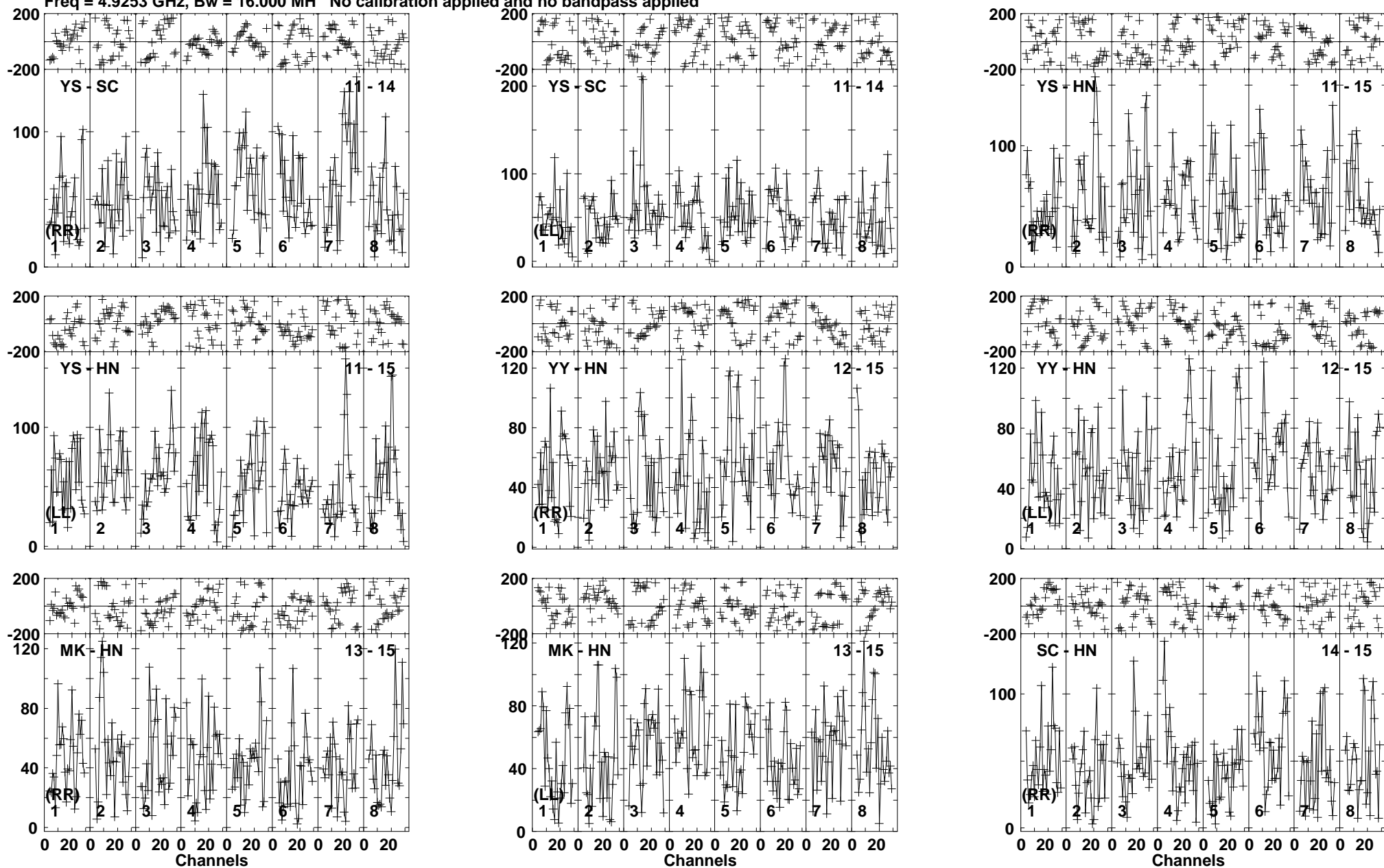
Lower frame: Micro Ampl Jy Top frame: Phas deg Vector averaged cross-power spectrum Baseline: YS (11) - SC (14) Timerange: 01/00:22:48 to 01/00:28:02
