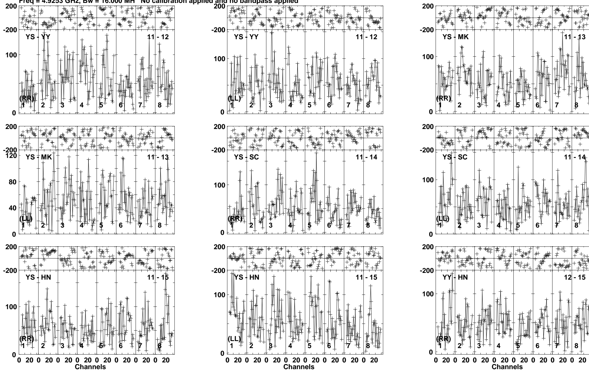
Lower frame: Micro Ampl Jy Top frame: Phas deg Vector averaged cross-power spectrum Baseline: YS (11) - YY (12) Timerange: 00/22:56:18 to 00/23:01:32
