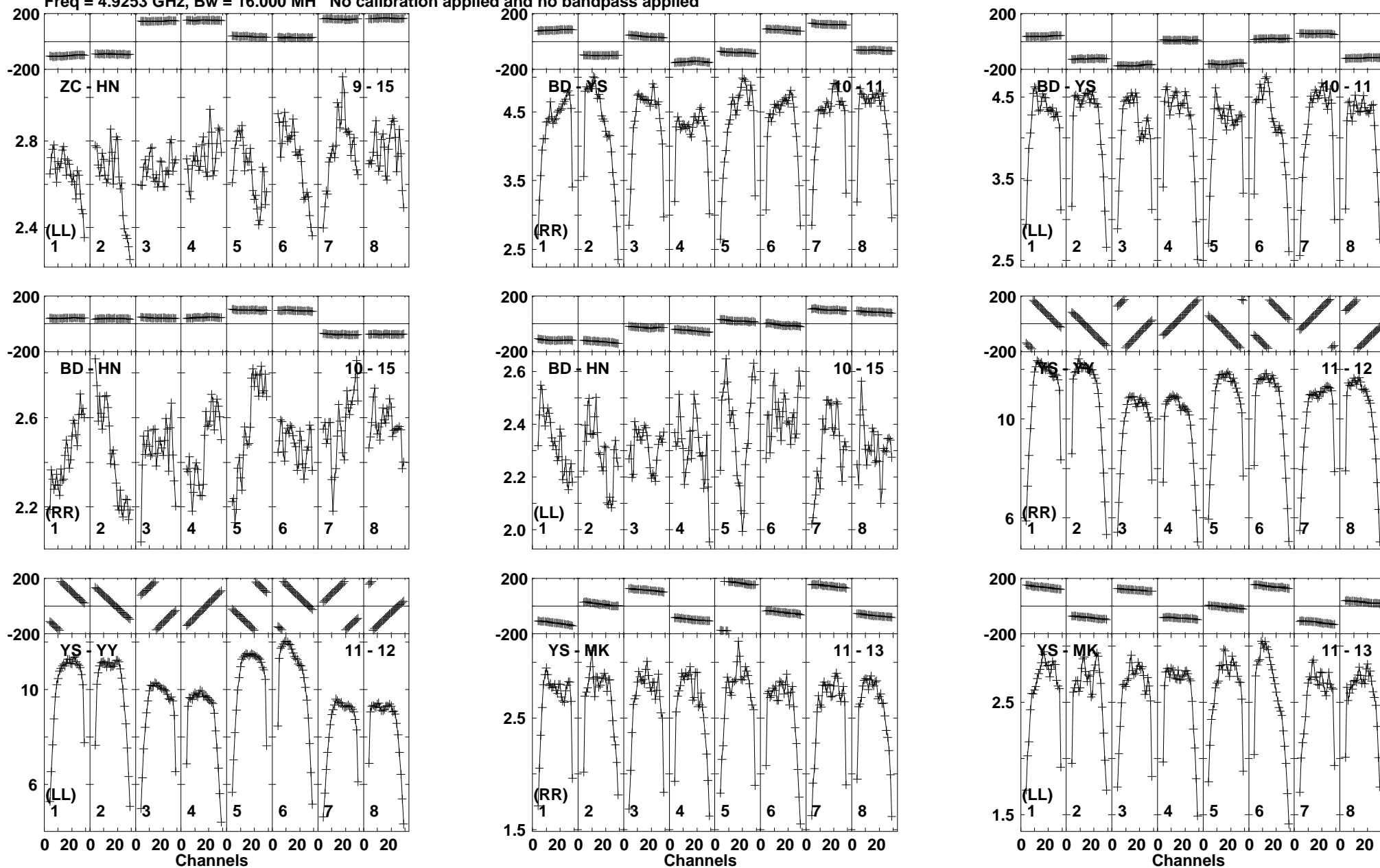
Lower frame: Milli Ampl Jy Top frame: Phas deg Vector averaged cross-power spectrum Baseline: ZC (09) - HN (15) Timerange: 00/21:13:27 to 00/21:15:18
