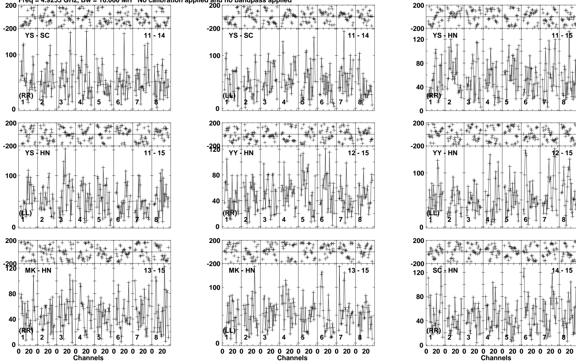
Lower frame: Micro Ampl Jy Top frame: Phas deg Vector averaged cross-power spectrum Baseline: YS (11) - SC (14) Timerange: 01/01:13:13 to 01/01:18:25
