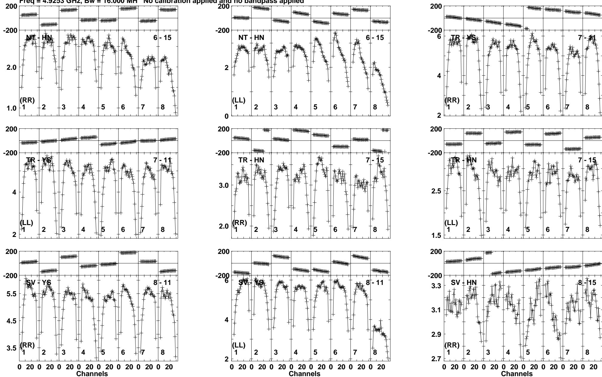
Lower frame: Milli Ampl Jy Top frame: Phas deg Vector averaged cross-power spectrum Baseline: NT (06) - HN (15) Timerange: 00/23:59:18 to 01/00:01:02
