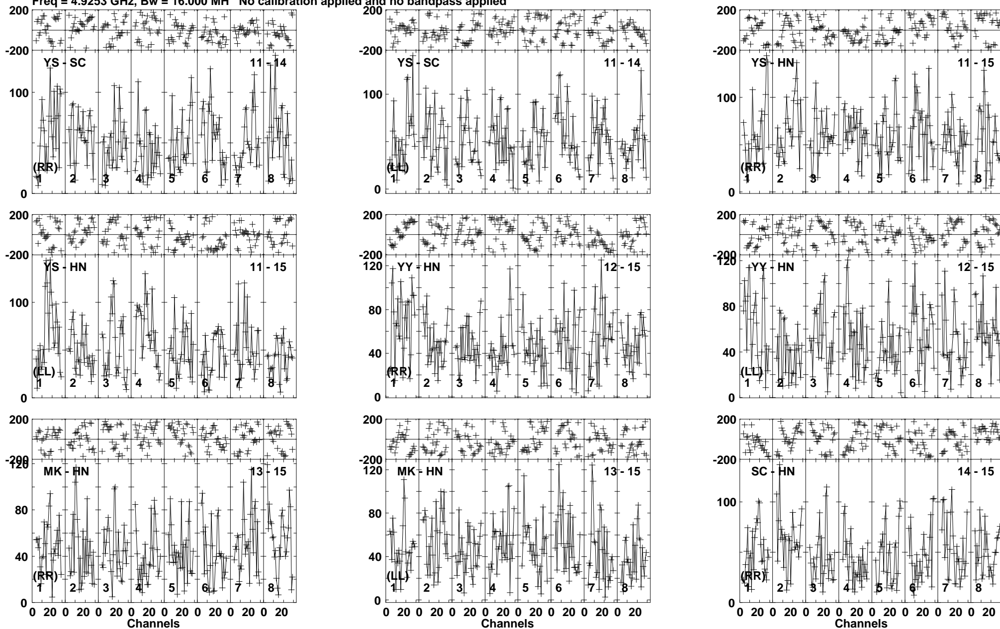
Lower frame: Micro Ampl Jy Top frame: Phas deg Vector averaged cross-power spectrum Baseline: YS (11) - SC (14) Timerange: 01/00:44:23 to 01/00:49:35
