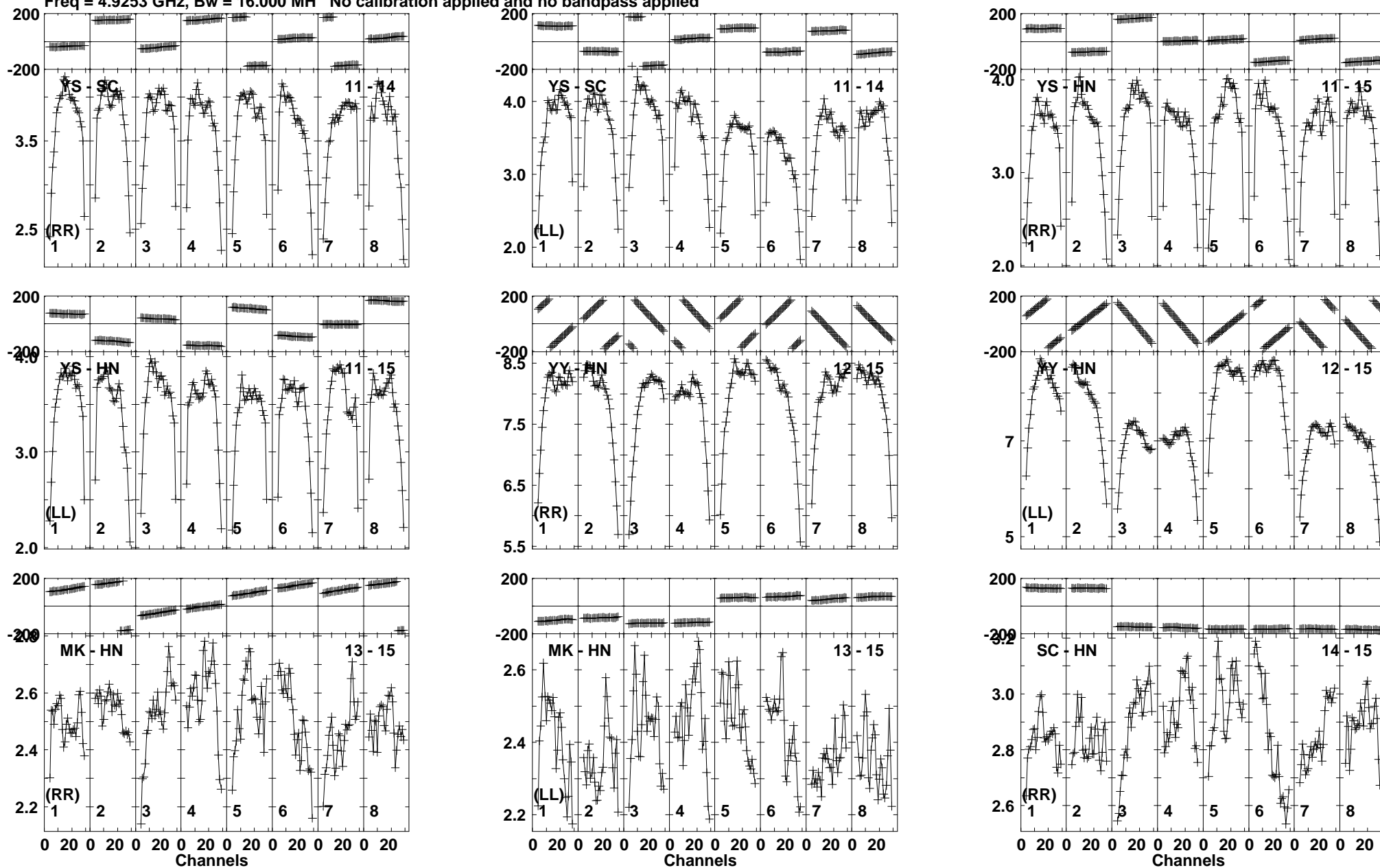
Lower frame: Milli Ampl Jy Top frame: Phas deg Vector averaged cross-power spectrum Baseline: YS (11) - SC (14) Timerange: 01/01:40:13 to 01/01:41:57
