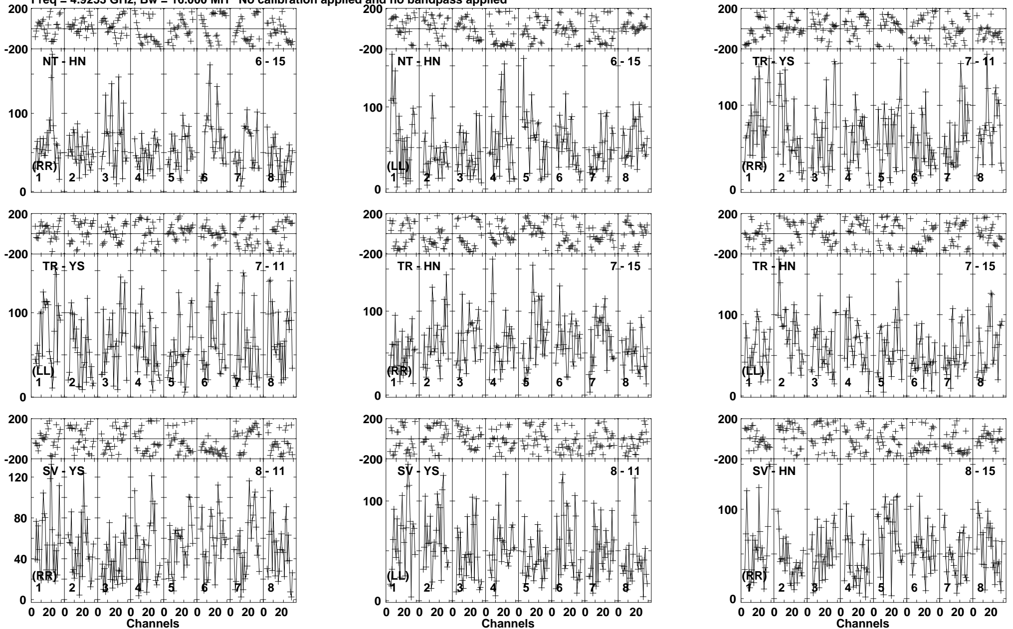
Lower frame: Micro Ampl Jy Top frame: Phas deg Vector averaged cross-power spectrum Baseline: NT (06) - HN (15) Timerange: 00/22:20:14 to 00/22:25:26
