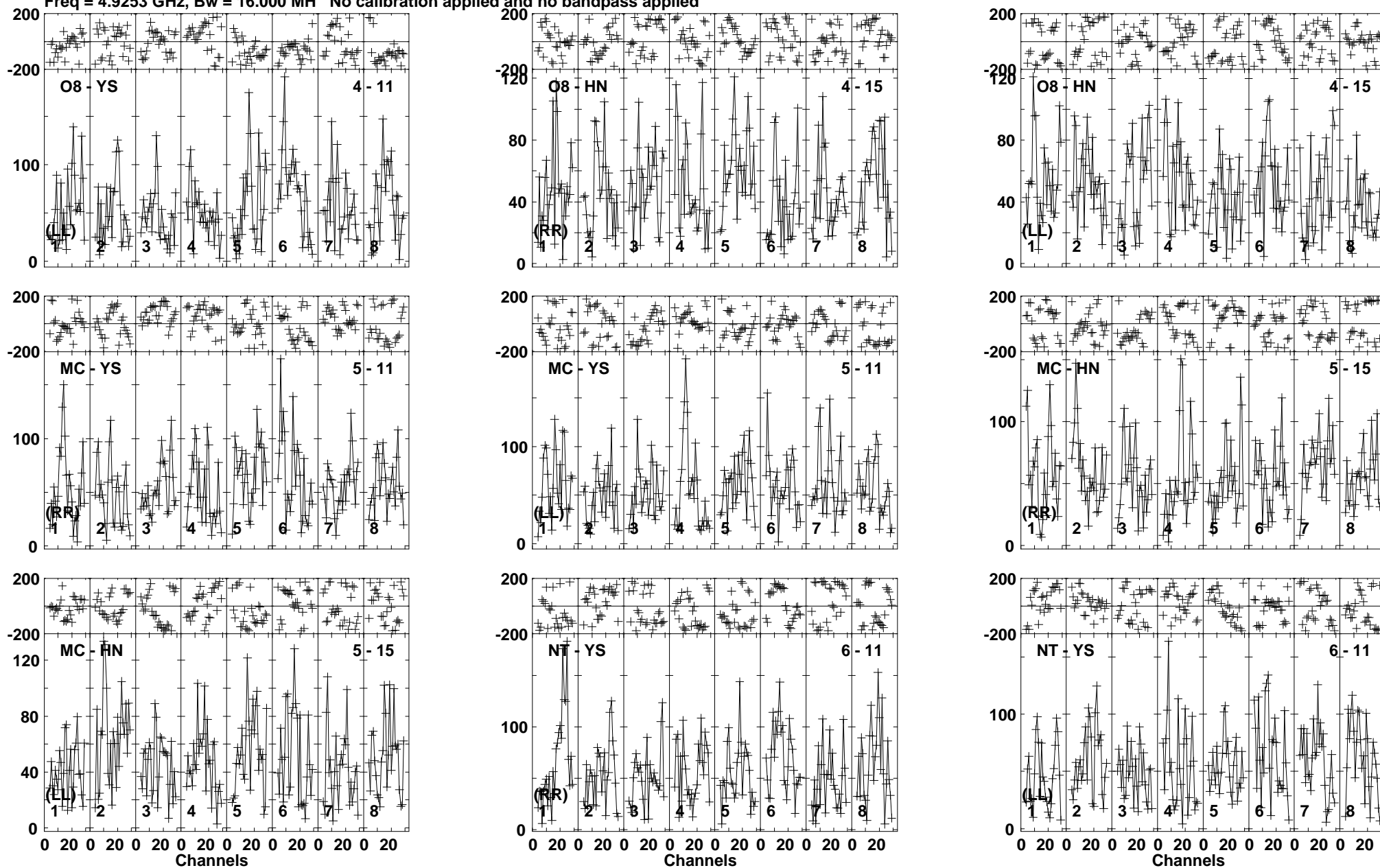
Lower frame: Micro Ampl Jy Top frame: Phas deg Vector averaged cross-power spectrum Baseline: O8 (04) - YS (11) Timerange: 00/23:53:58 to 00/23:59:12
