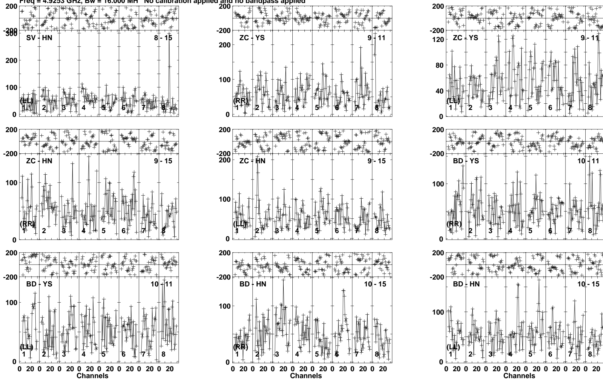
Lower frame: Micro Ampl Jy Top frame: Phas deg Vector averaged cross-power spectrum Baseline: SV (08) - HN (15) Timerange: 00/22:27:28 to 00/22:32:42
