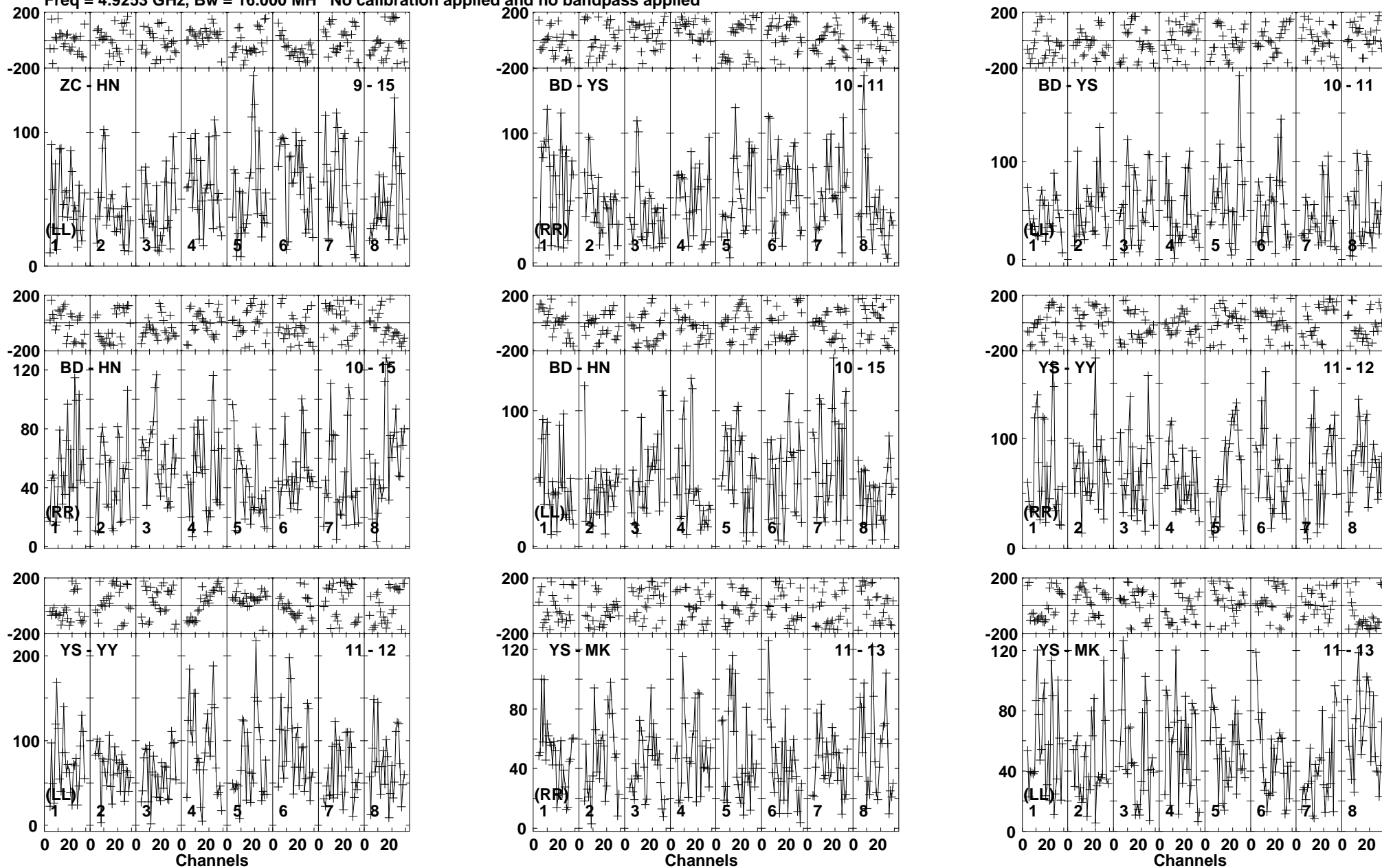
Lower frame: Micro Ampl Jy Top frame: Phas deg Vector averaged cross-power spectrum Baseline: ZC (09) - HN (15) Timerange: 01/00:29:58 to 01/00:35:10
