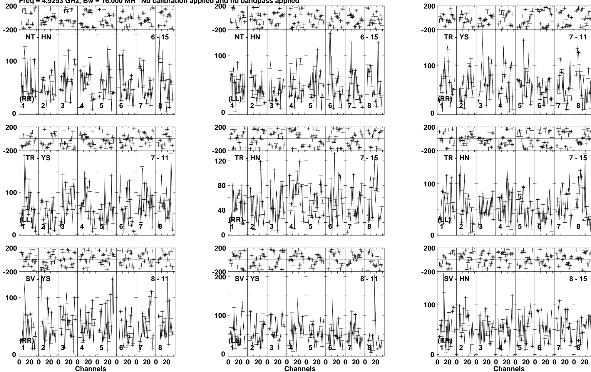
Lower frame: Micro Ampl Jy Top frame: Phas deg Vector averaged cross-power spectrum Baseline: NT (06) - HN (15) Timerange: 00/21:36:59 to 00/21:42:11
