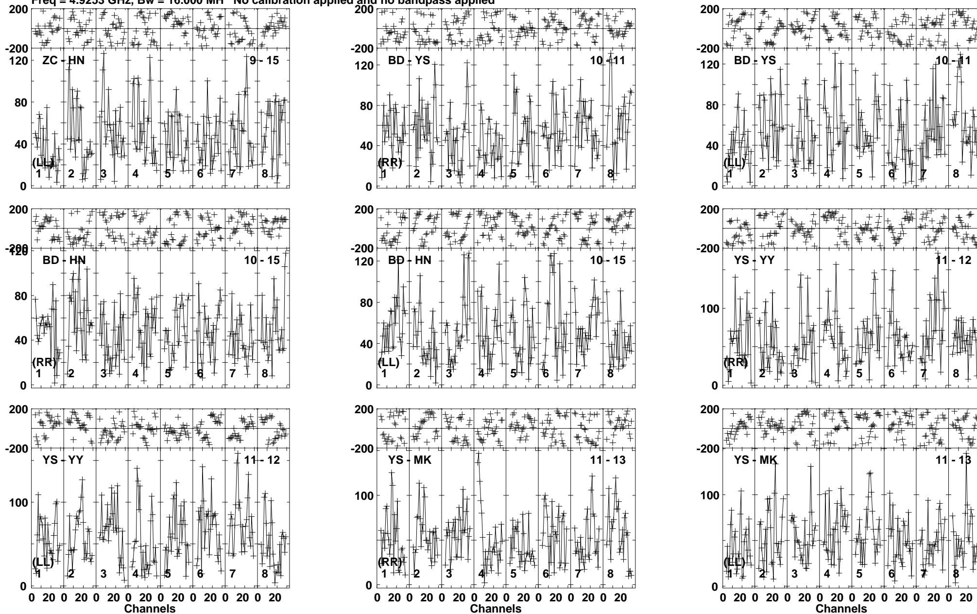
Lower frame: Micro Ampl Jy Top frame: Phas deg Vector averaged cross-power spectrum Baseline: ZC (09) - HN (15) Timerange: 01/02:03:43 to 01/02:08:57
