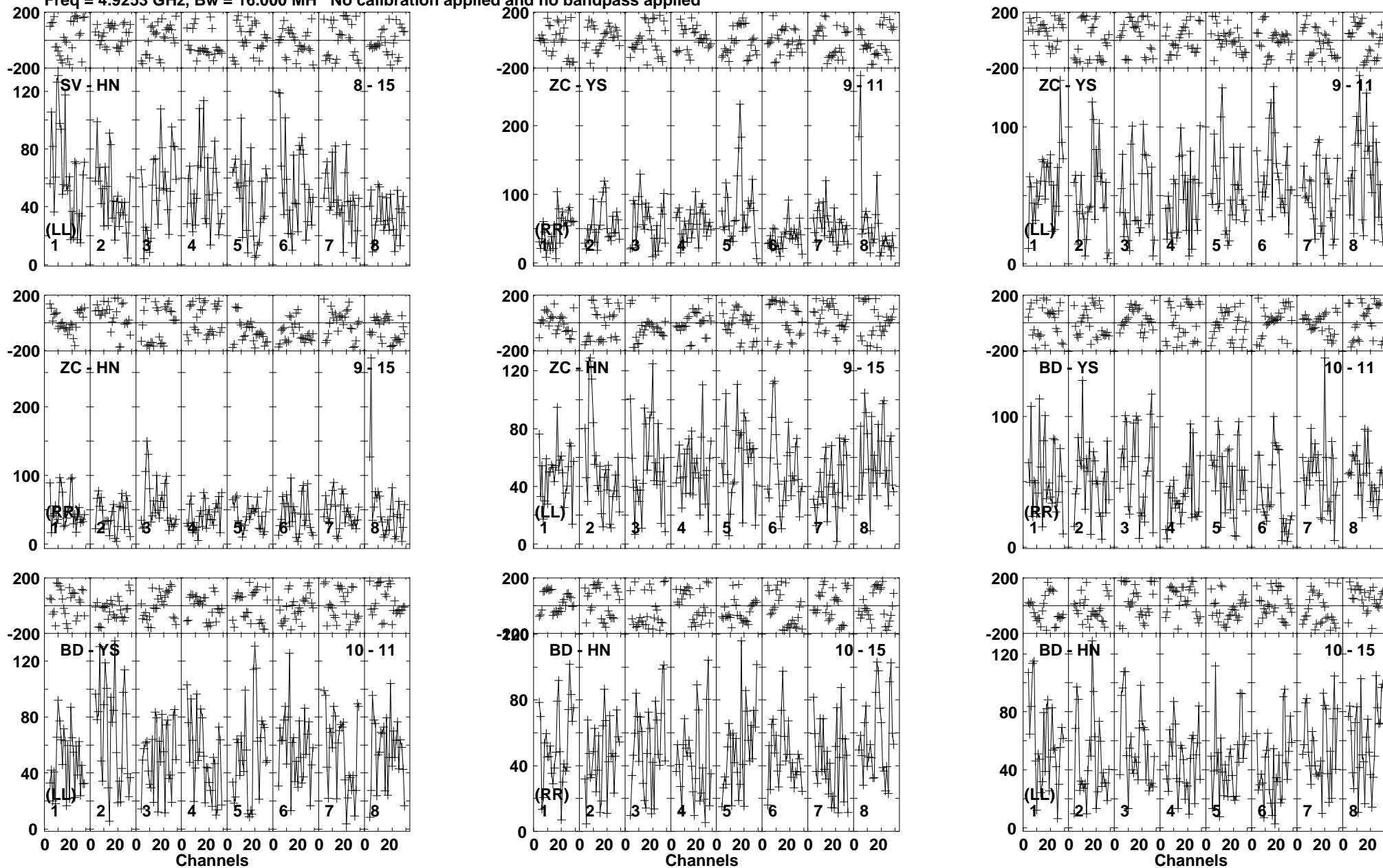
Lower frame: Micro Ampl Jy Top frame: Phas deg Vector averaged cross-power spectrum Baseline: SV (08) - HN (15) Timerange: 00/22:56:18 to 00/23:01:32
