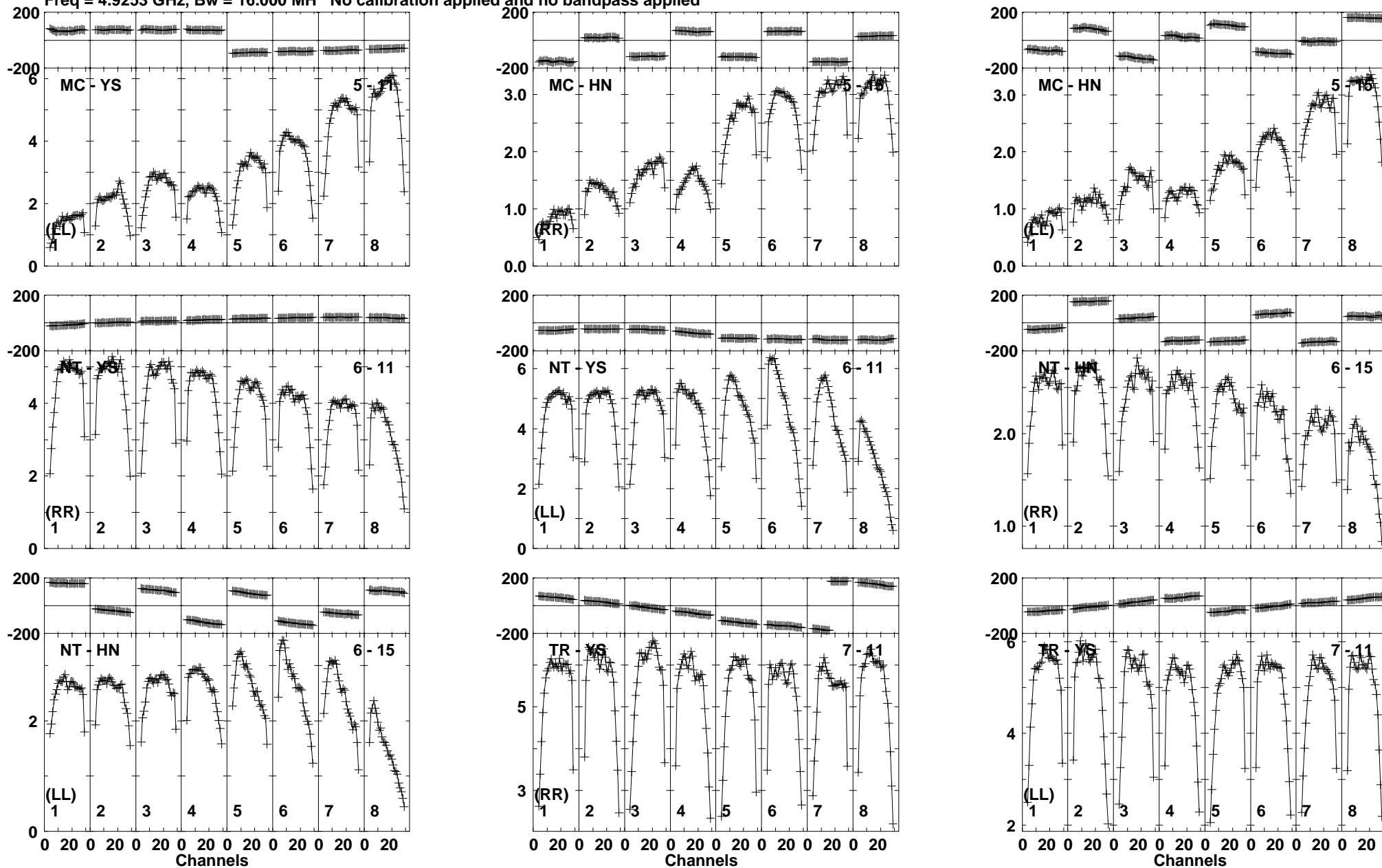
Lower frame: Milli Ampl Jy Top frame: Phas deg Vector averaged cross-power spectrum Baseline: MC (05) - YS (11) Timerange: 00/21:42:17 to 00/21:44:08
