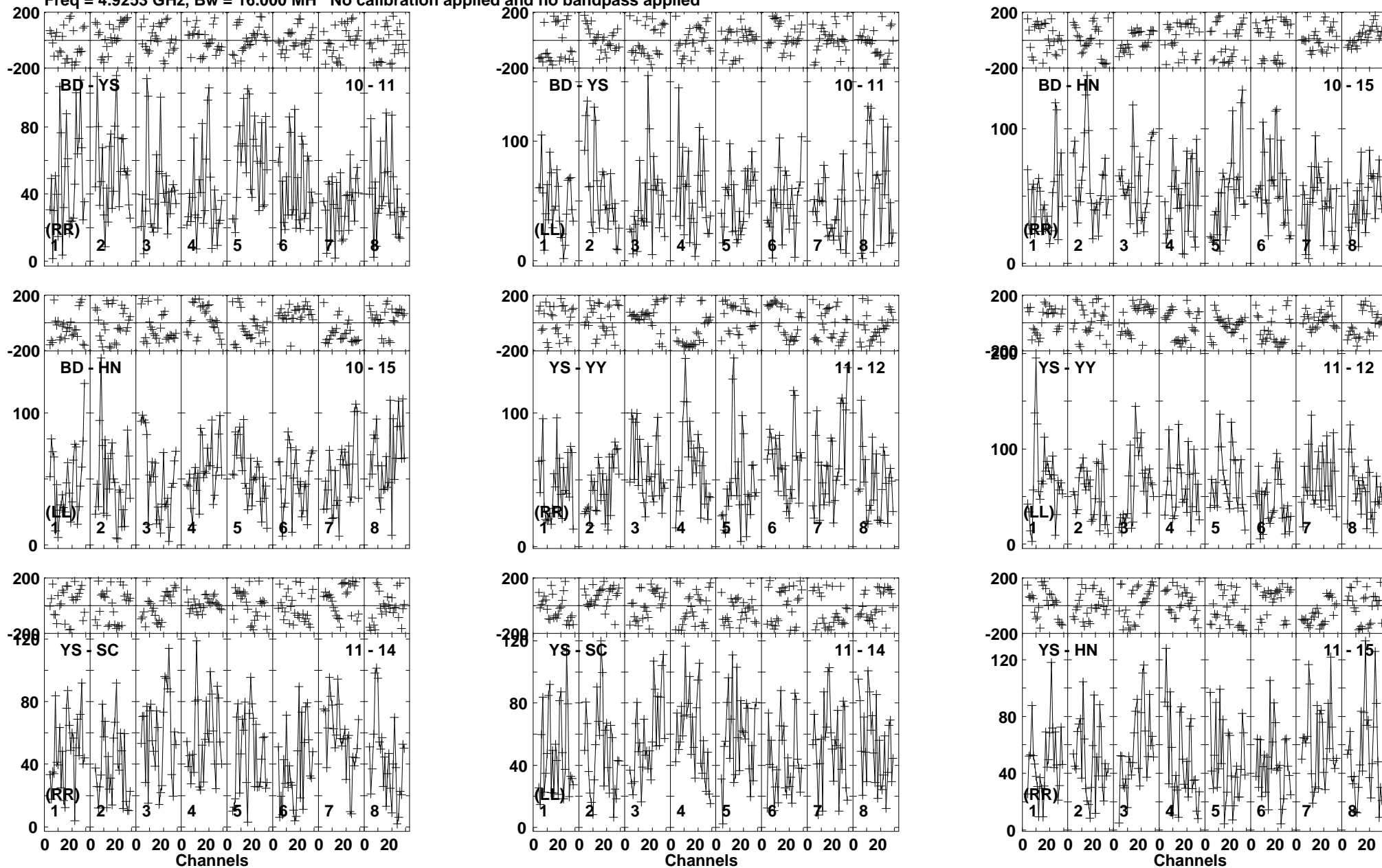
Lower frame: Micro Ampl Jy Top frame: Phas deg Vector averaged cross-power spectrum Baseline: BD (10) - YS (11) Timerange: 00/20:39:19 to 00/20:44:31
