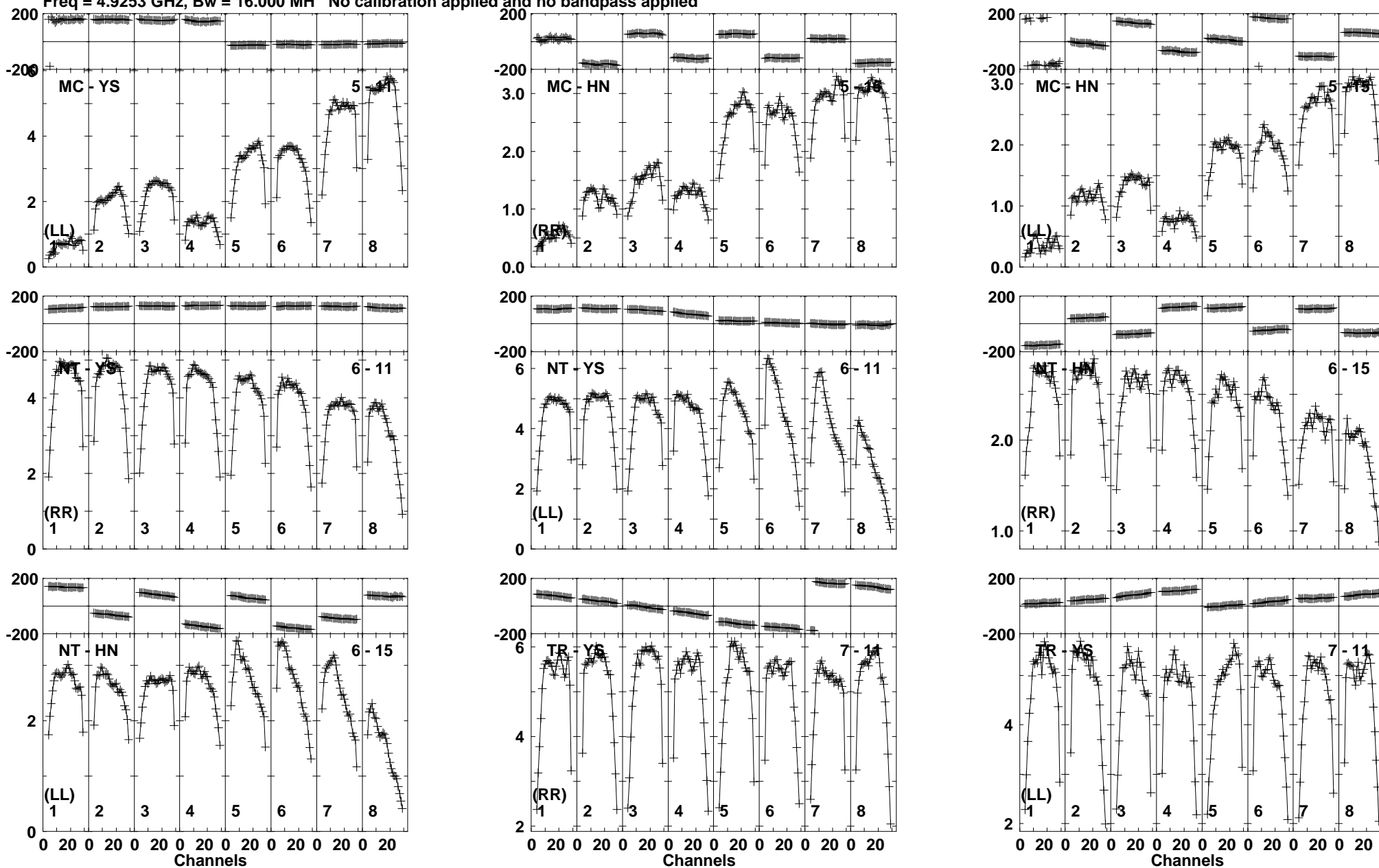
Lower frame: Milli Ampl Jy Top frame: Phas deg Vector averaged cross-power spectrum Baseline: MC (05) - YS (11) Timerange: 00/23:37:36 to 00/23:39:28
