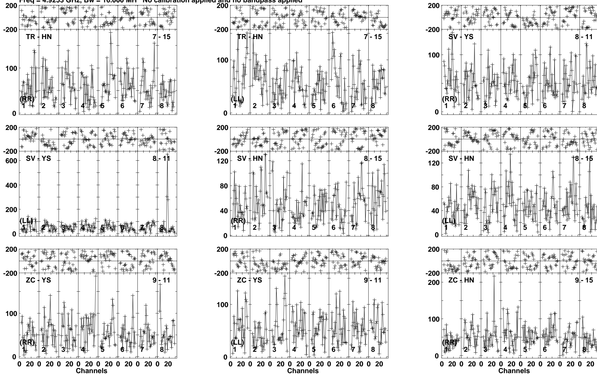
Lower frame: Micro Ampl Jy Top frame: Phas deg Vector averaged cross-power spectrum Baseline: TR (07) - HN (15) Timerange: 01/01:42:03 to 01/01:47:15
