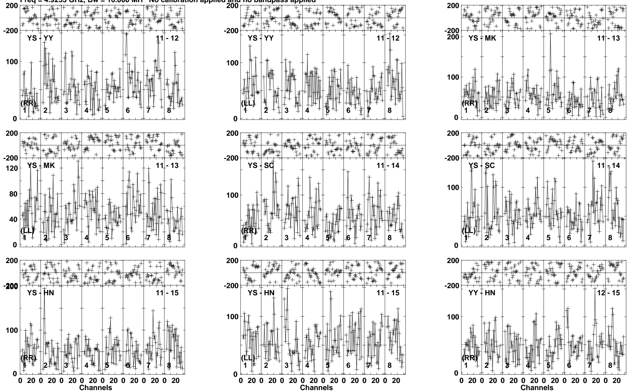
Lower frame: Micro Ampl Jy Top frame: Phas deg Vector averaged cross-power spectrum Baseline: YS (11) - YY (12) Timerange: 00/21:51:24 to 00/21:56:36
