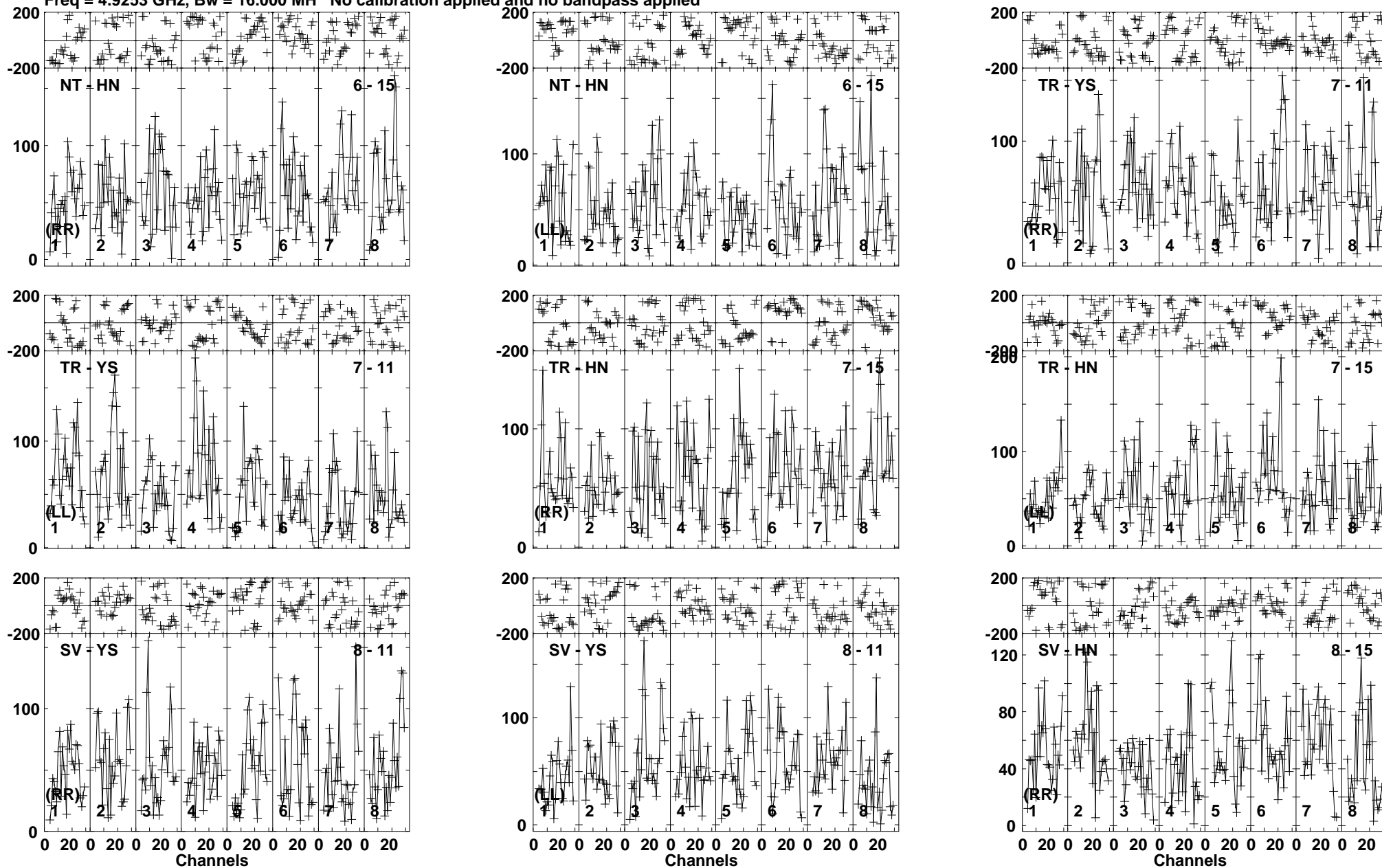
Lower frame: Micro Ampl Jy Top frame: Phas deg Vector averaged cross-power spectrum Baseline: NT (06) - HN (15) Timerange: 00/22:34:39 to 00/22:39:51
