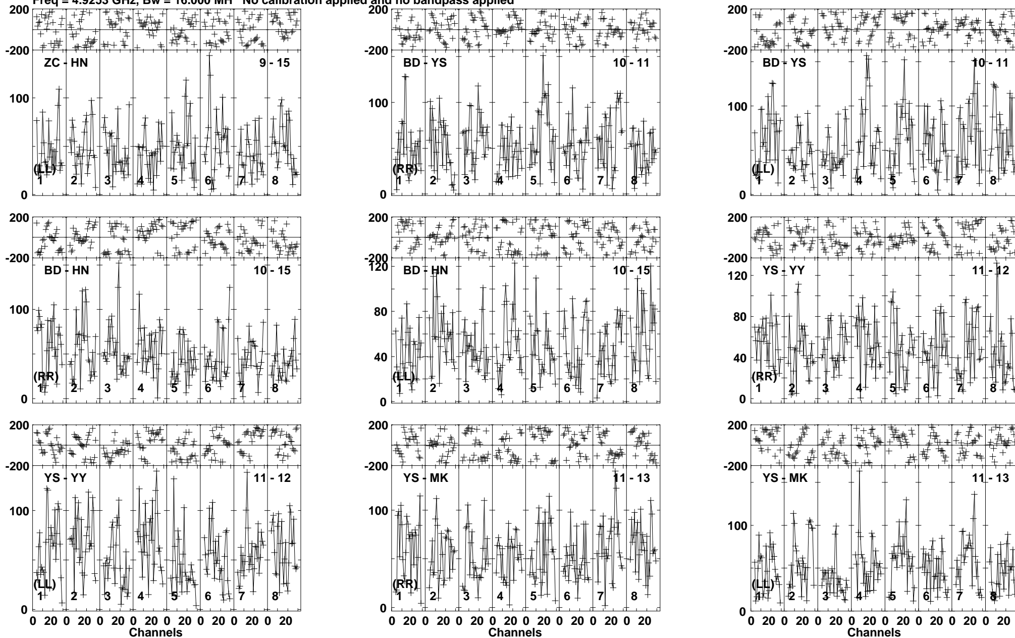
Lower frame: Micro Ampl Jy Top frame: Phas deg Vector averaged cross-power spectrum Baseline: ZC (09) - HN (15) Timerange: 01/01:06:03 to 01/01:11:17
