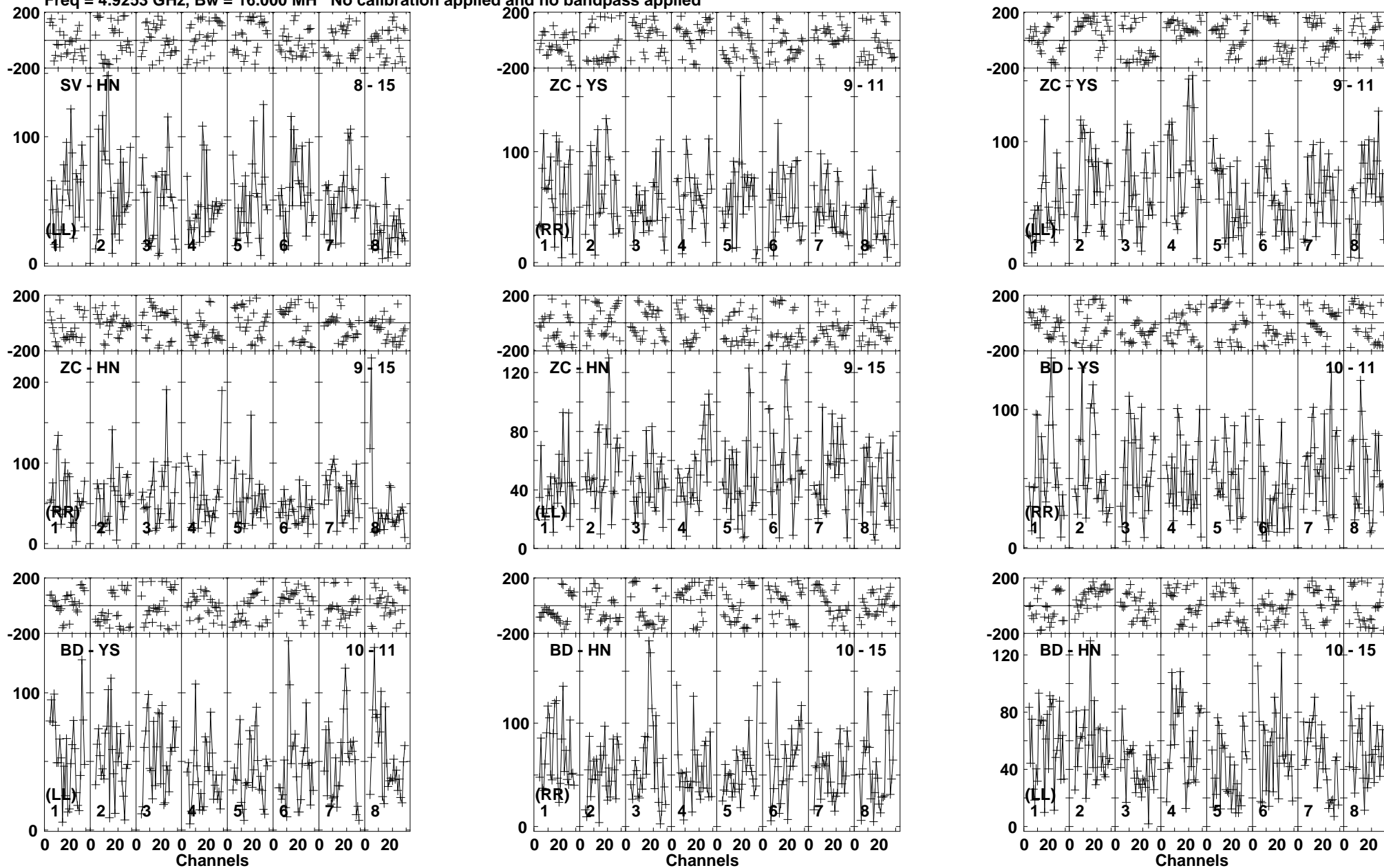
Lower frame: Micro Ampl Jy Top frame: Phas deg Vector averaged cross-power spectrum Baseline: SV (08) - HN (15) Timerange: 00/21:22:34 to 00/21:27:46
