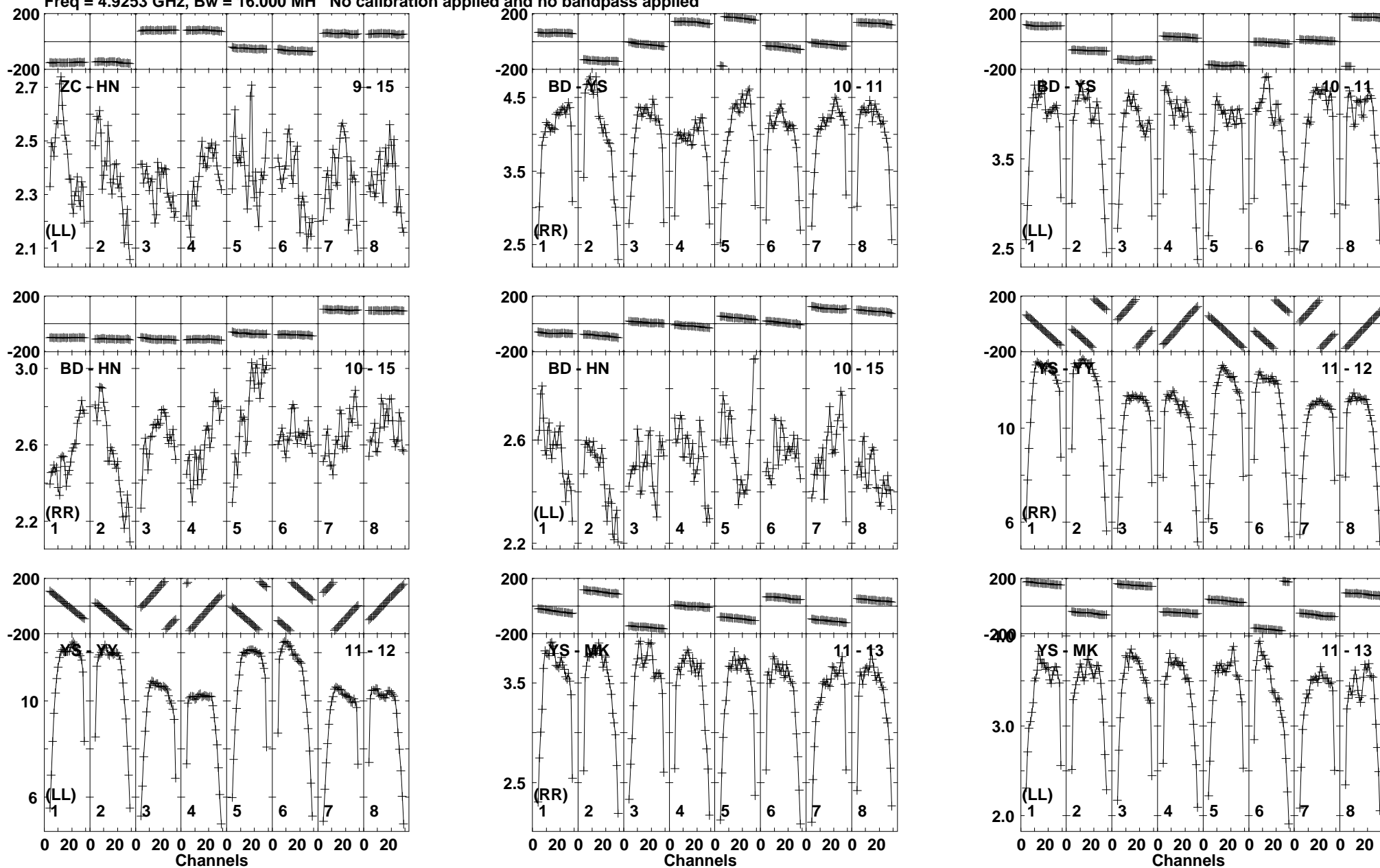
Lower frame: Milli Ampl Jy Top frame: Phas deg Vector averaged cross-power spectrum Baseline: ZC (09) - HN (15) Timerange: 01/02:09:03 to 01/02:10:47
