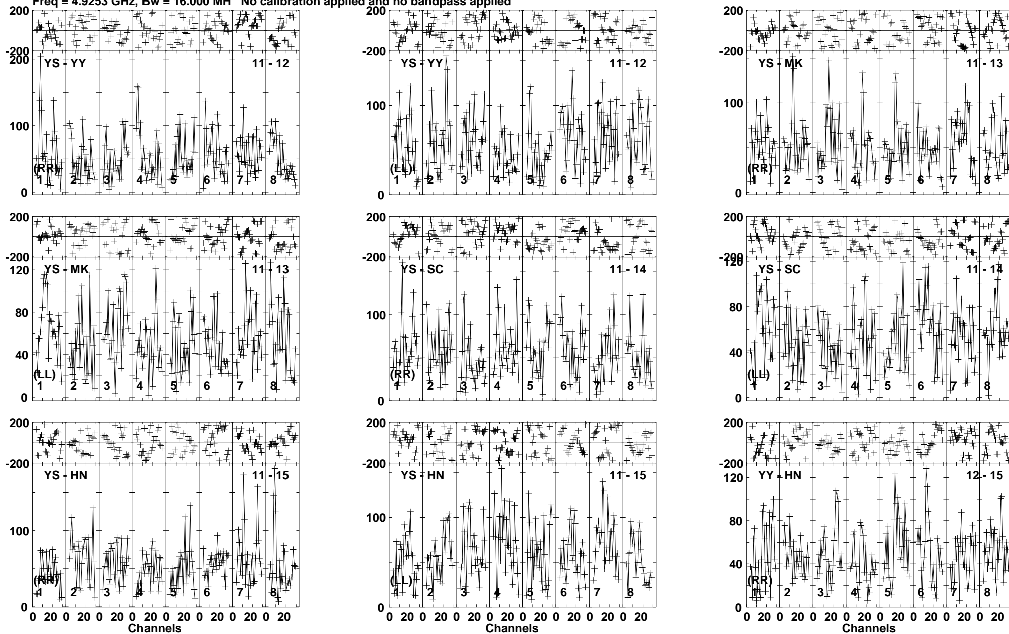
Lower frame: Micro Ampl Jy Top frame: Phas deg Vector averaged cross-power spectrum Baseline: YS (11) - YY (12) Timerange: 00/21:22:34 to 00/21:27:46
