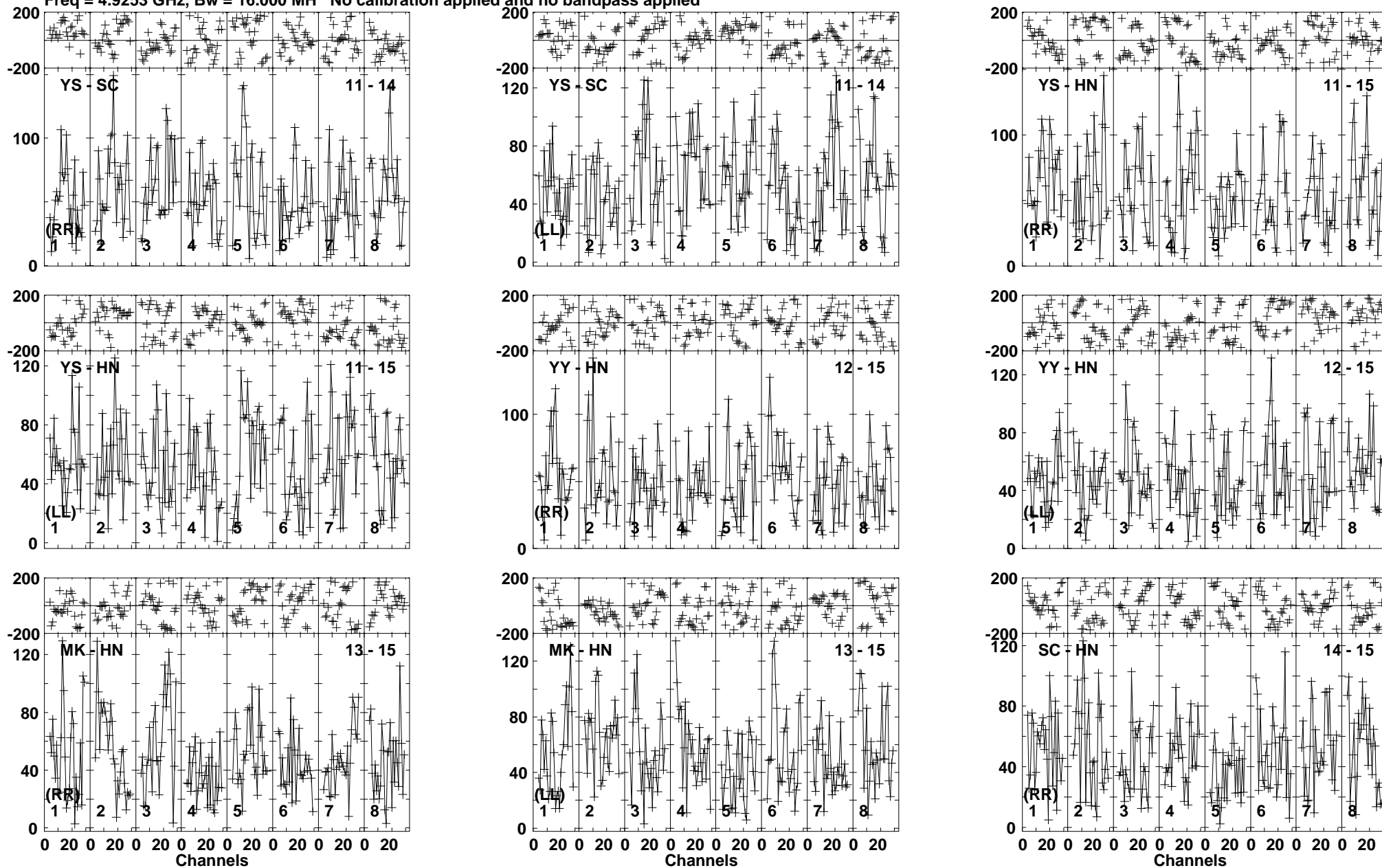
Lower frame: Micro Ampl Jy Top frame: Phas deg Vector averaged cross-power spectrum Baseline: YS (11) - SC (14) Timerange: 01/00:51:38 to 01/00:56:52
