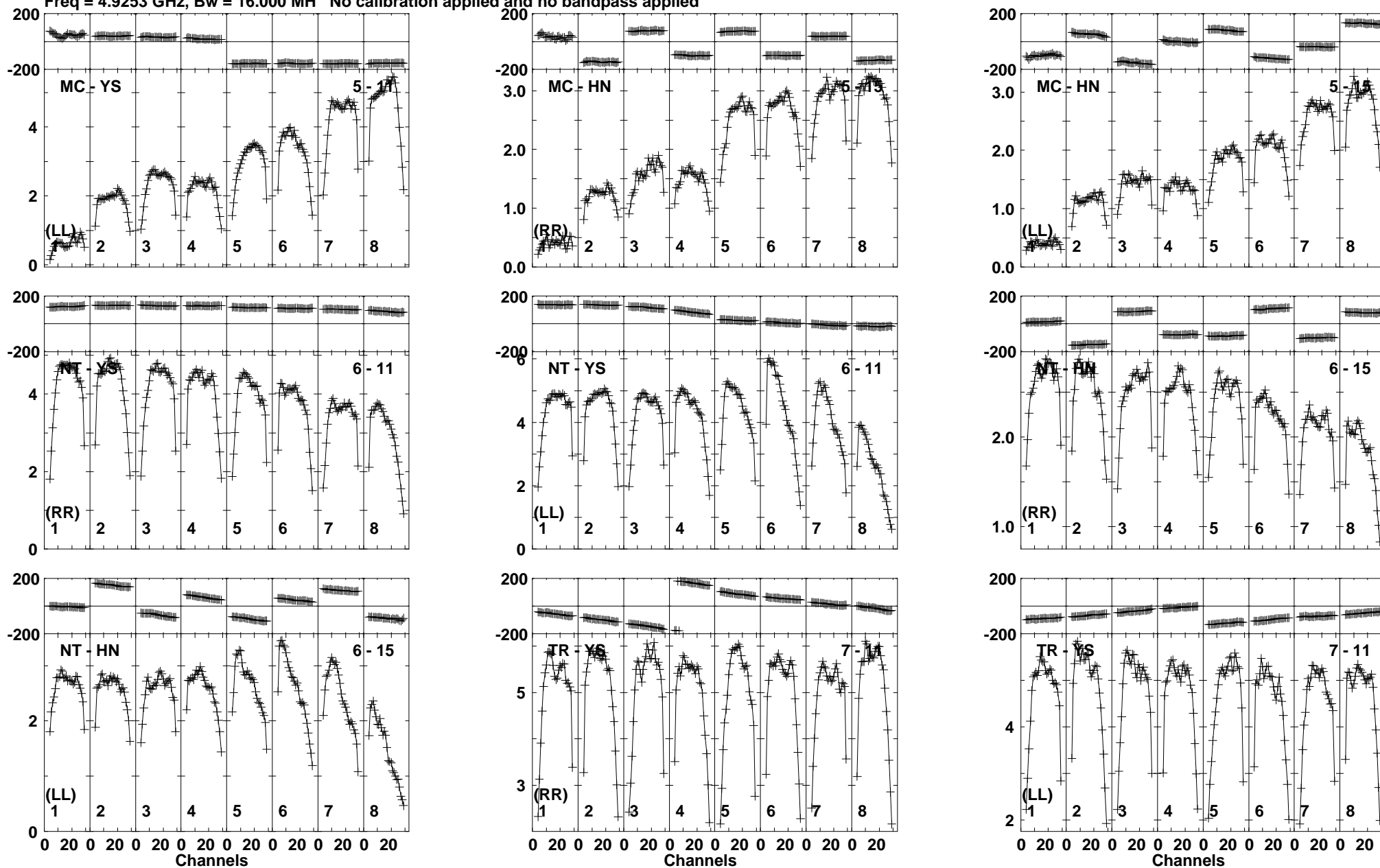
Lower frame: Milli Ampl Jy Top frame: Phas deg Vector averaged cross-power spectrum Baseline: MC (05) - YS (11) Timerange: 01/00:42:33 to 01/00:44:17
