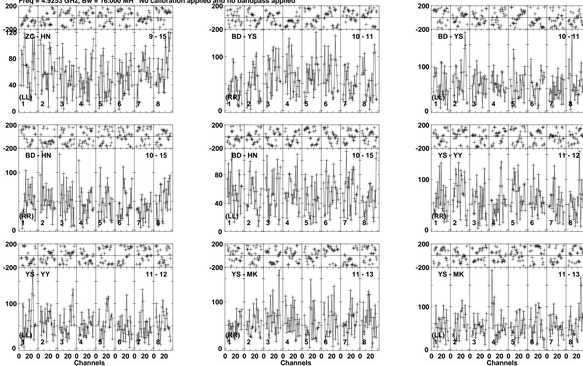
Lower frame: Micro Ampl Jy Top frame: Phas deg Vector average cross-power spectrum Baseline: ZC (09) - HN (15) Timerange: 01/00:08:23 to 01/00:13:37
