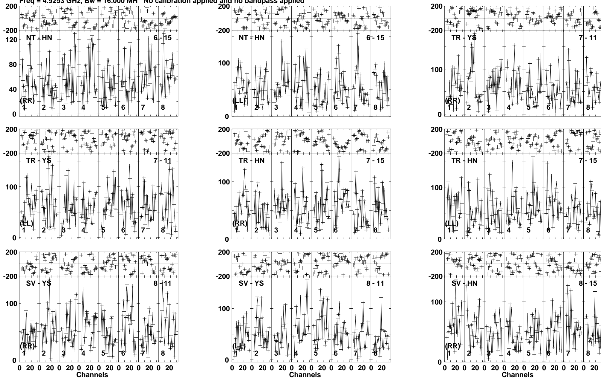
Lower frame: Micro Ampl Jy Top frame: Phas deg Vector averaged cross-power spectrum Baseline: NT (06) - HN (15) Timerange: 00/22:56:18 to 00/23:01:32
