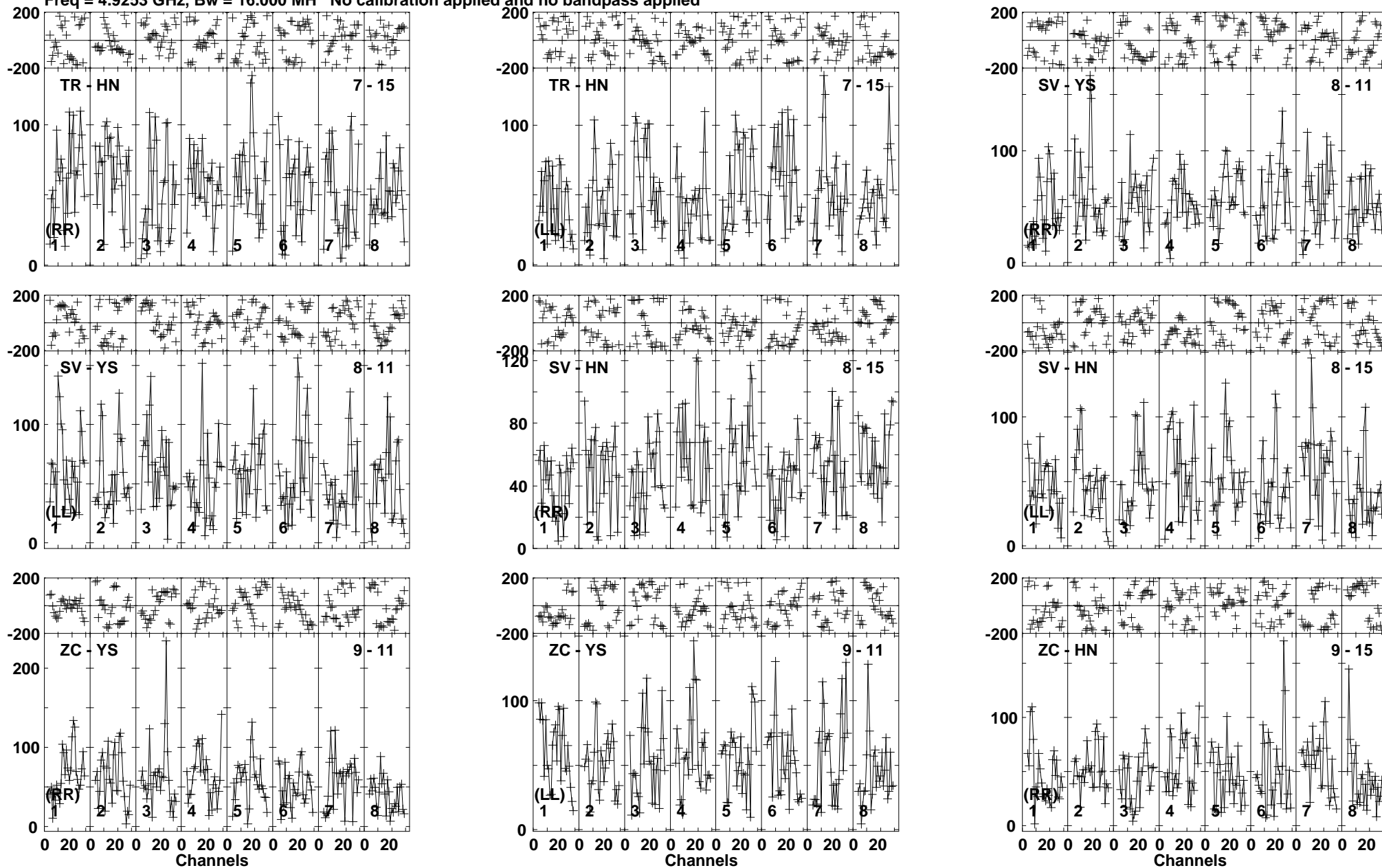
Lower frame: Micro Ampl Jy Top frame: Phas deg Vector averaged cross-power spectrum Baseline: TR (07) - HN (15) Timerange: 01/01:34:53 to 01/01:40:07
