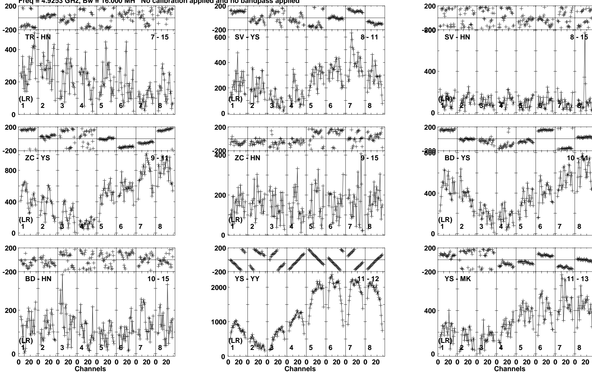
Lower frame: Micro Ampl Jy Top frame: Phas deg Vector averaged cross-power spectrum Baseline: TR (07) - HN (15) Timerange: 01/00:13:43 to 01/00:15:27
