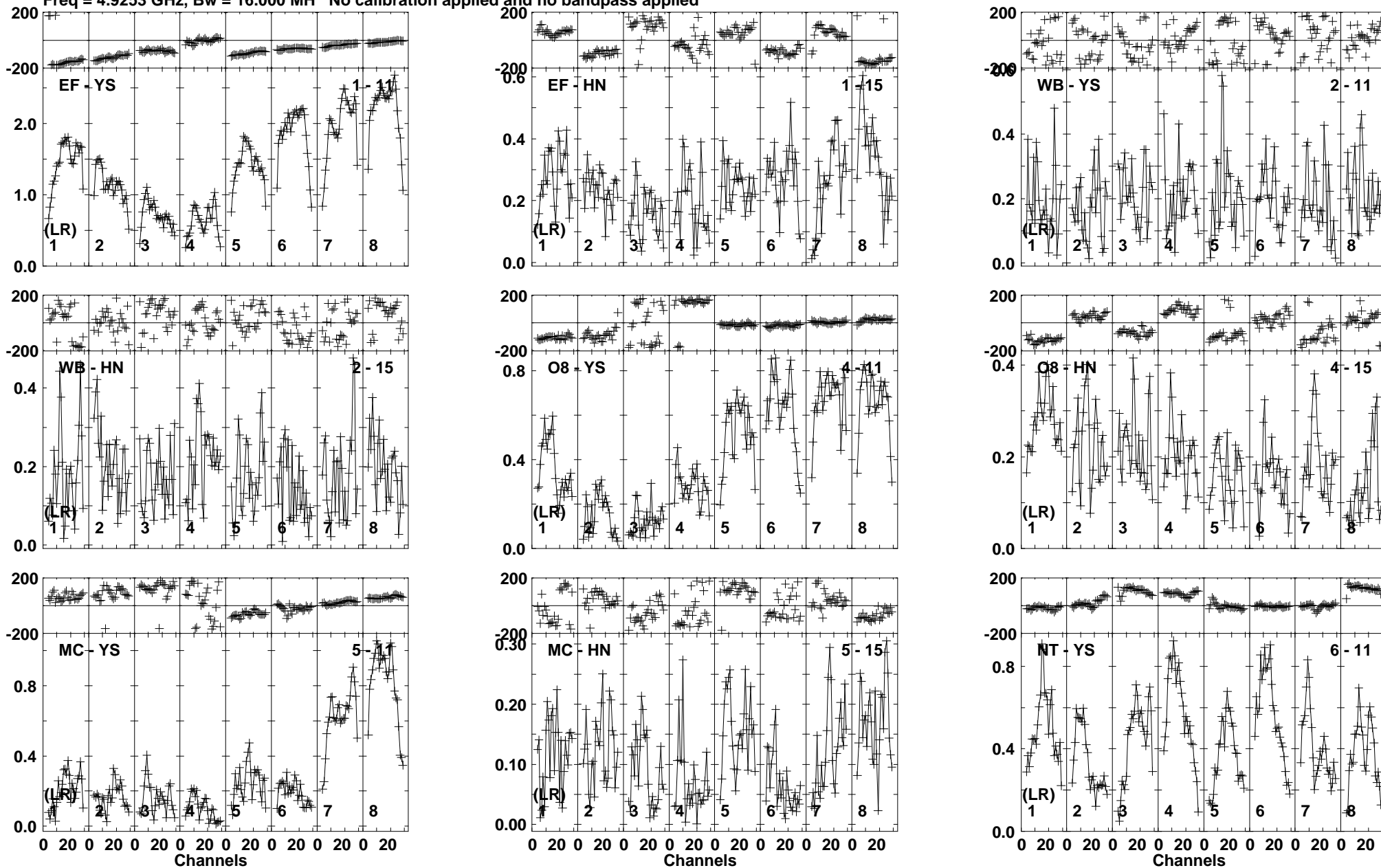
Lower frame: Milli Ampl Jy Top frame: Phas deg Vector averaged cross-power spectrum Baseline: EF (01) - YS (11) Timerange: 00/20:59:02 to 00/21:00:53
