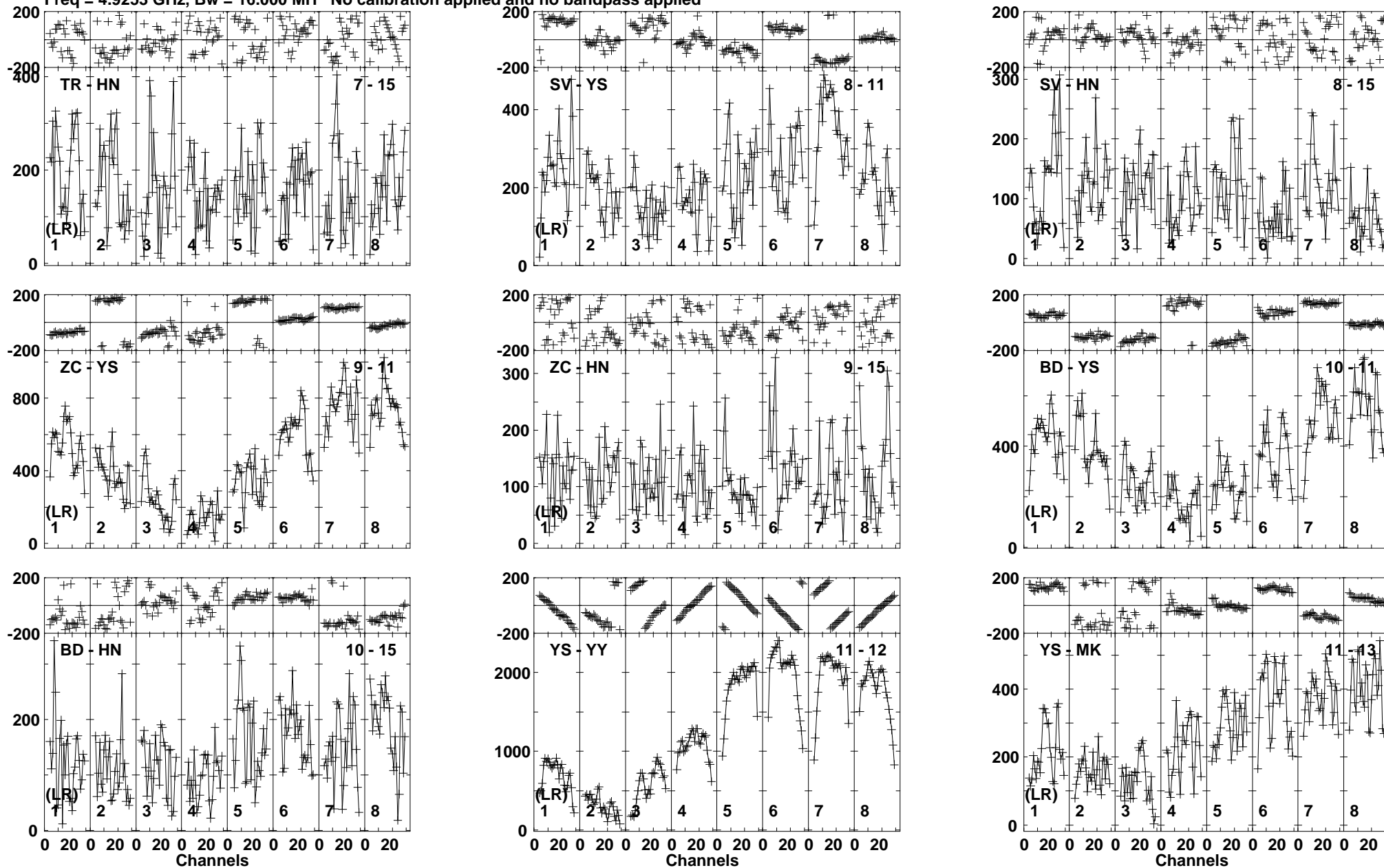
Lower frame: Micro Ampl Jy Top frame: Phas deg Vector averaged cross-power spectrum Baseline: TR (07) - HN (15) Timerange: 00:22:25:32 to 00:22:27:23
