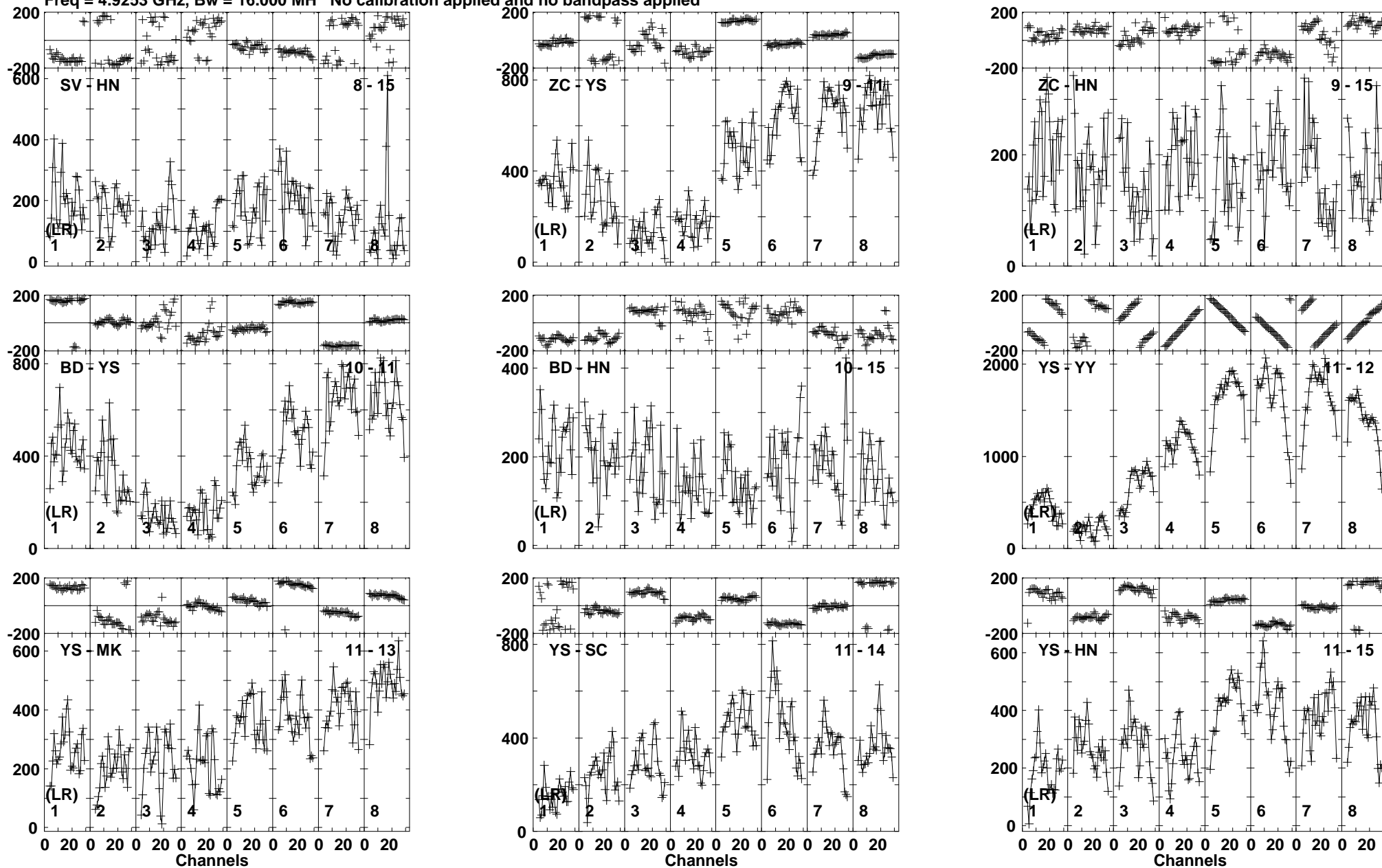
Lower frame: Micro Ampl Jy Top frame: Phas deg Vector averaged cross-power spectrum Baseline: SV (08) - HN (15) Timerange: 01/02:01:46 to 01/02:03:38
