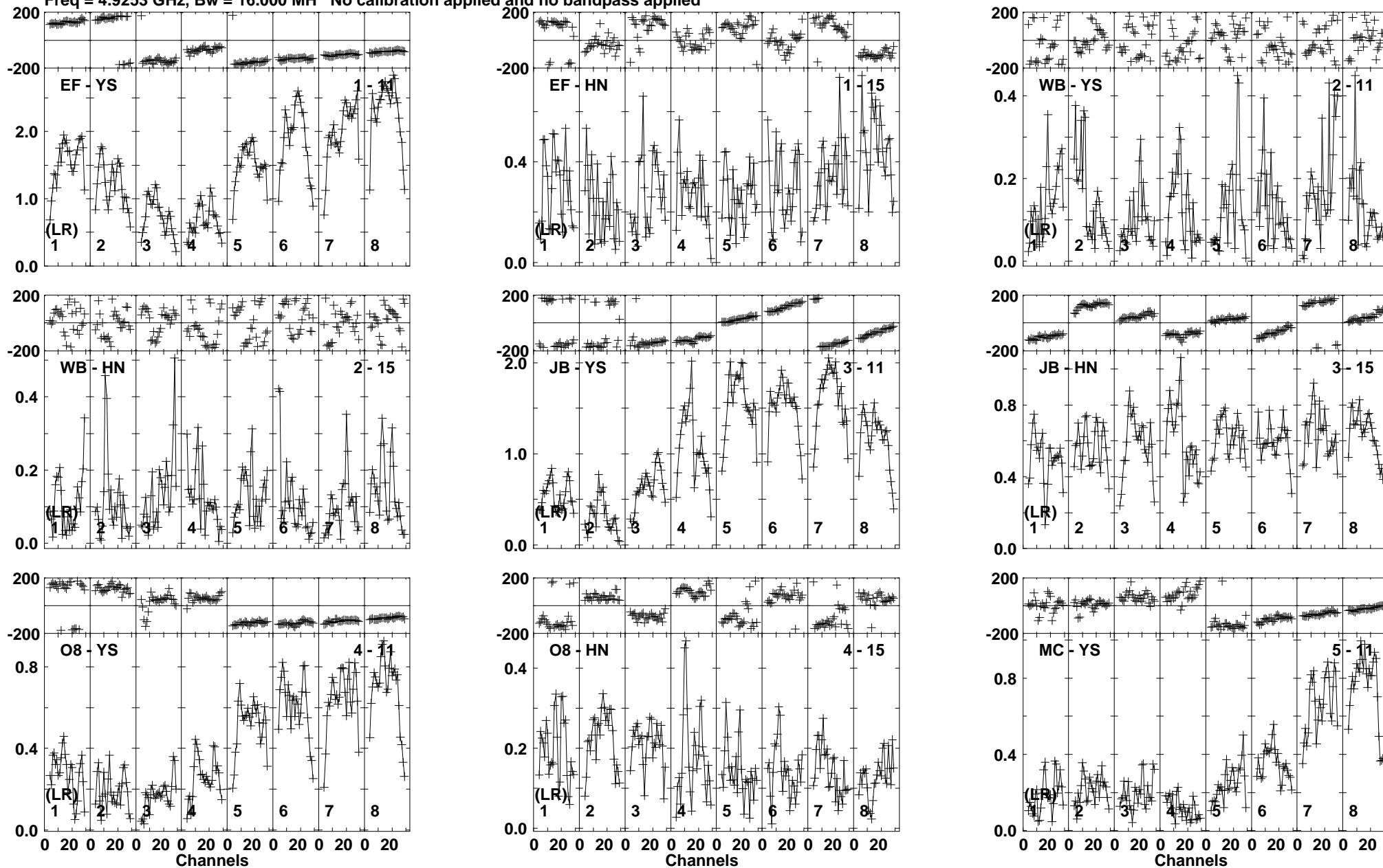
Lower frame: Milli Ampl Jy Top frame: Phas deg Vector averaged cross-power spectrum Baseline: EF (01) - YS (11) Timerange: 00/21:06:19 to 00/21:08:02
