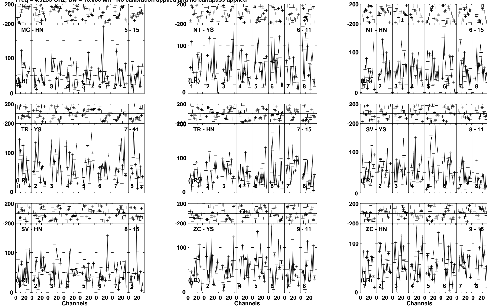
Lower frame: Micro Ampl Jy Top frame: Phas deg Vector averaged cross-power spectrum Baseline: MC (05) - HN (15) Timerange: 00/21:00:58 to 00/21:06:12
