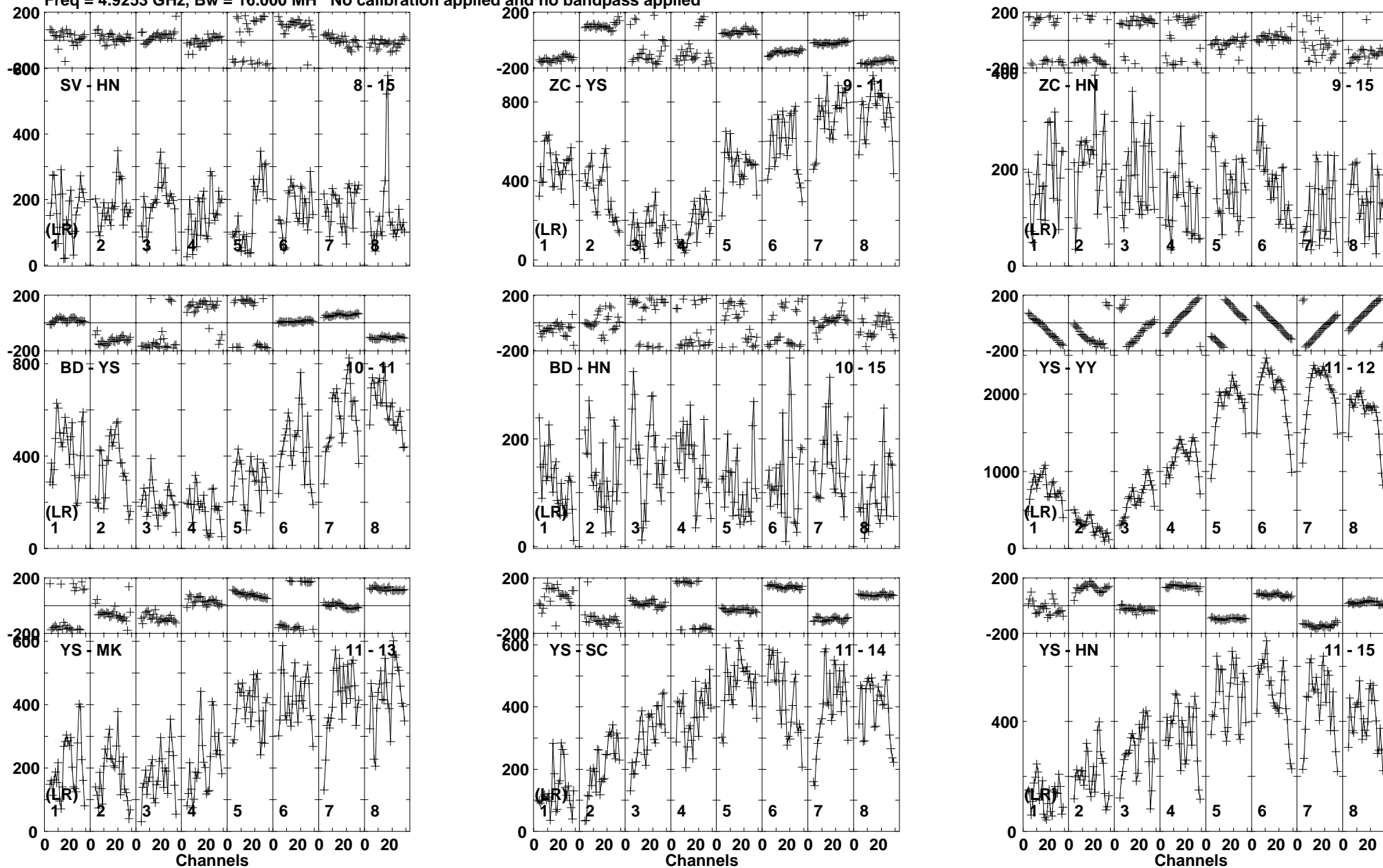
Lower frame: Micro Ampl Jy Top frame: Phas deg Vector averaged cross-power spectrum Baseline: SV (08) - HN (15) Timerange: 01/00:49:41 to 01/00:51:33
