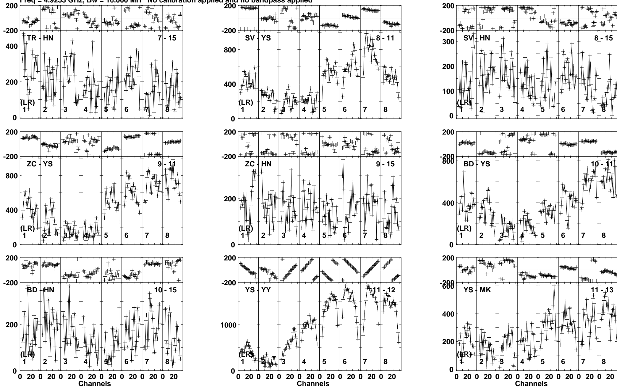
Lower frame: Micro Ampl Jy Top frame: Phas deg Vector averaged cross-power spectrum Baseline: TR (07) - HN (15) Timerange: 01/01:40:13 to 01/01:41:57
