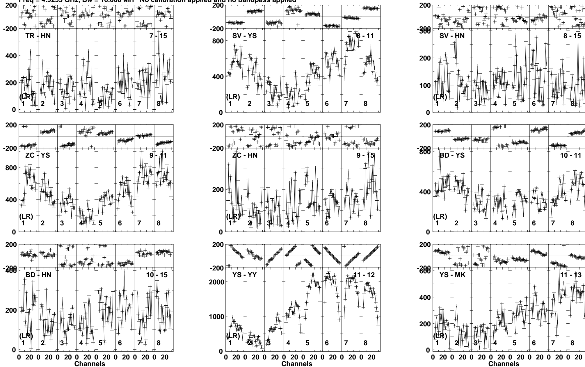
Lower frame: Micro Ampl Jy Top frame: Phas deg Vector averaged cross-power spectrum Baseline: TR (07) - HN (15) Timerange: 00/21:27:52 to 00/21:29:43
