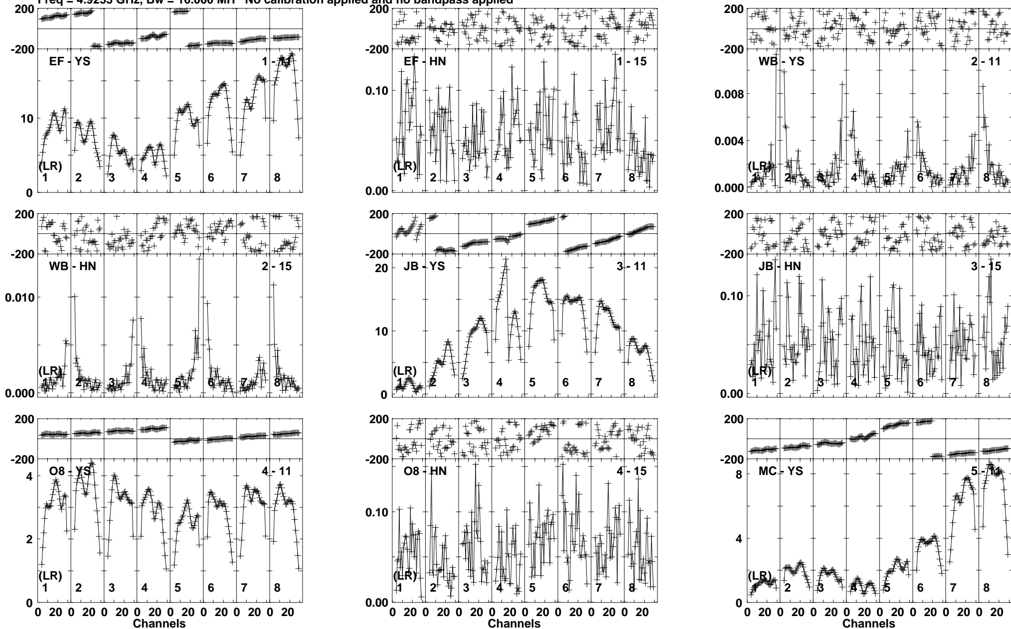
Lower frame: Milli Ampl Jy Top frame: Phas deg Vector averaged cross-power spectrum Baseline: EF (01) - YS (11) Timerange: 00/20:30:01 to 00/20:34:56
