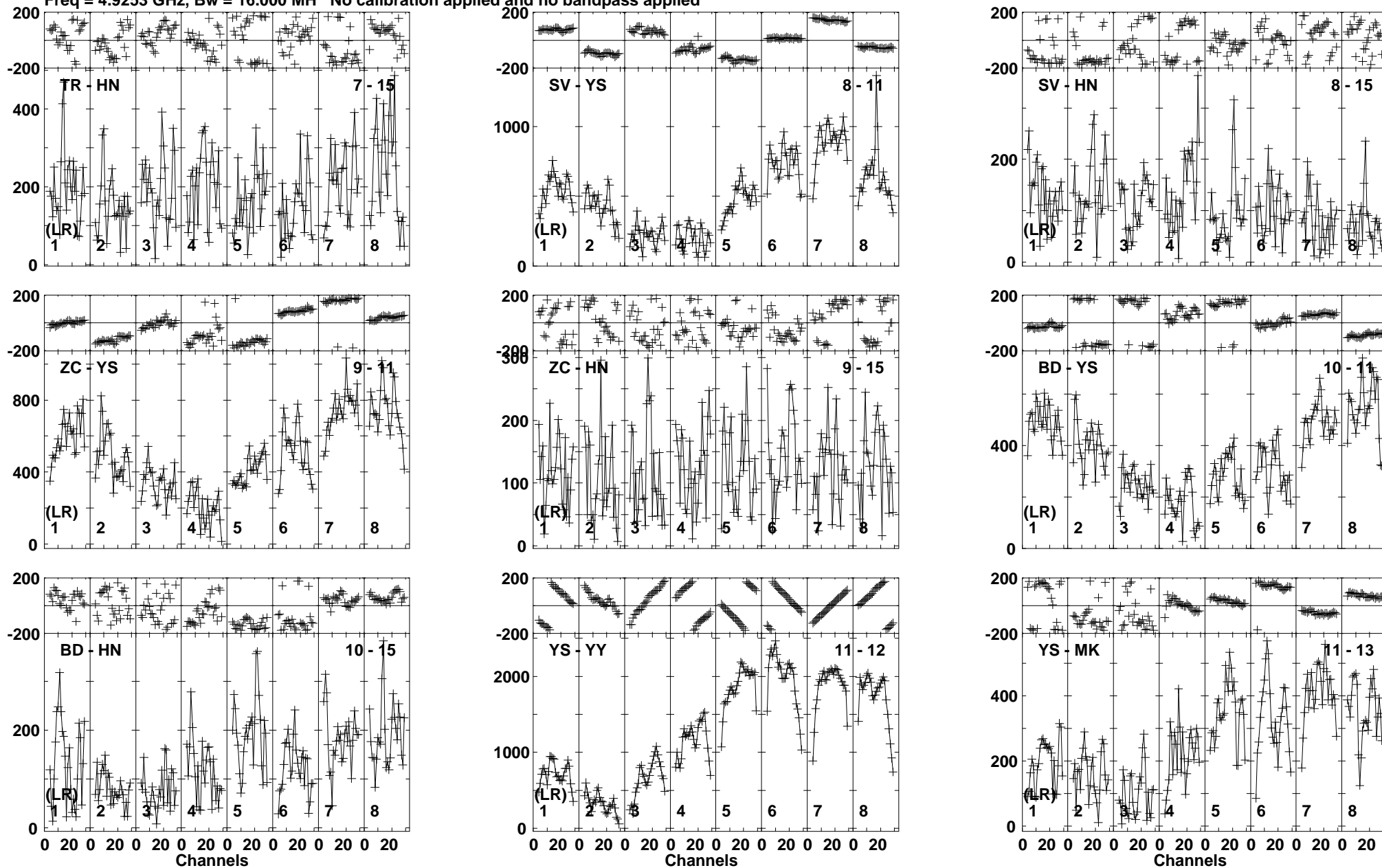
Lower frame: Micro Ampl Jy Top frame: Phas deg Vector averaged cross-power spectrum Baseline: TR (07) - HN (15) Timerange: 00:22:11:07 to 00:22:12:58
