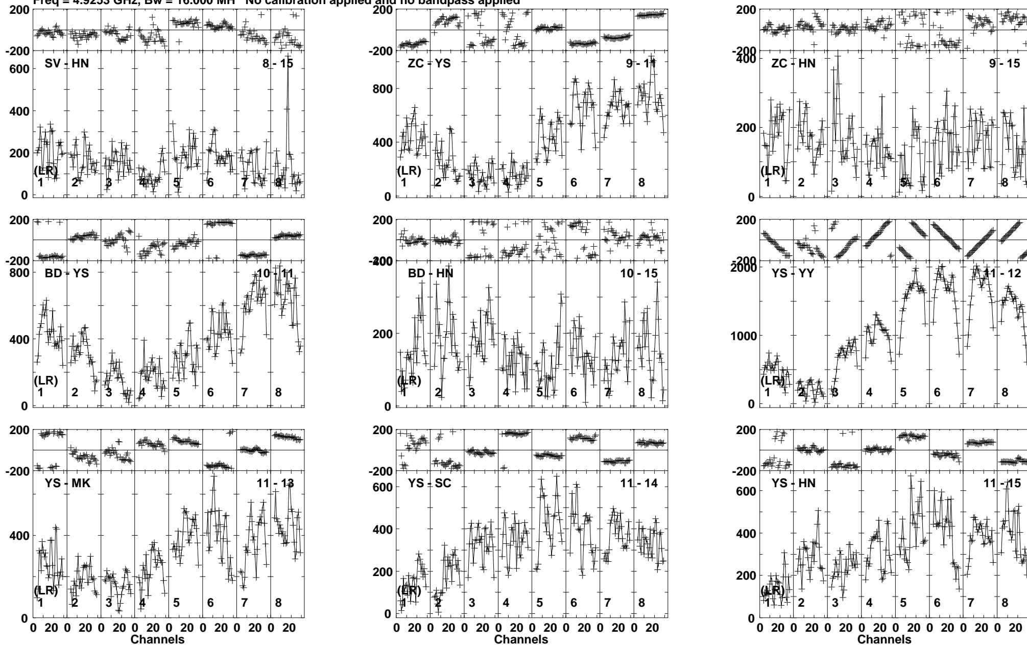
Lower frame: Micro Ampl Jy Top frame: Phas deg Vector averaged cross-power spectrum Baseline: SV (08) - HN (15) Timerange: 01/01:47:21 to 01/01:49:13
