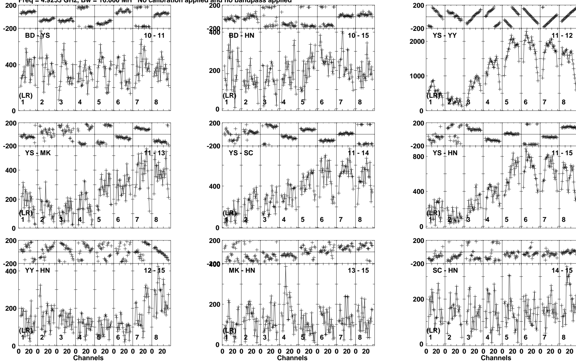
Lower frame: Micro Ampl Jy Top frame: Phas deg Vector averaged cross-power spectrum Baseline: BD (10) - YS (11) Timerange: 00/21:06:19 to 00/21:08:02
