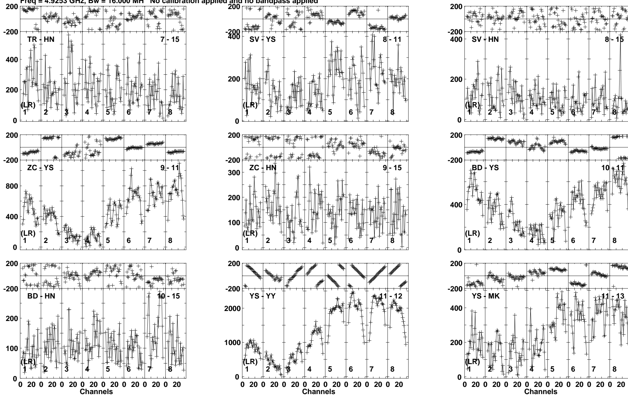
Lower frame: Micro Ampl Jy Top frame: Phas deg Vector averaged cross-power spectrum Baseline: TR (07) - HN (15) Timerange: 00/23:52:01 to 00/23:53:53
