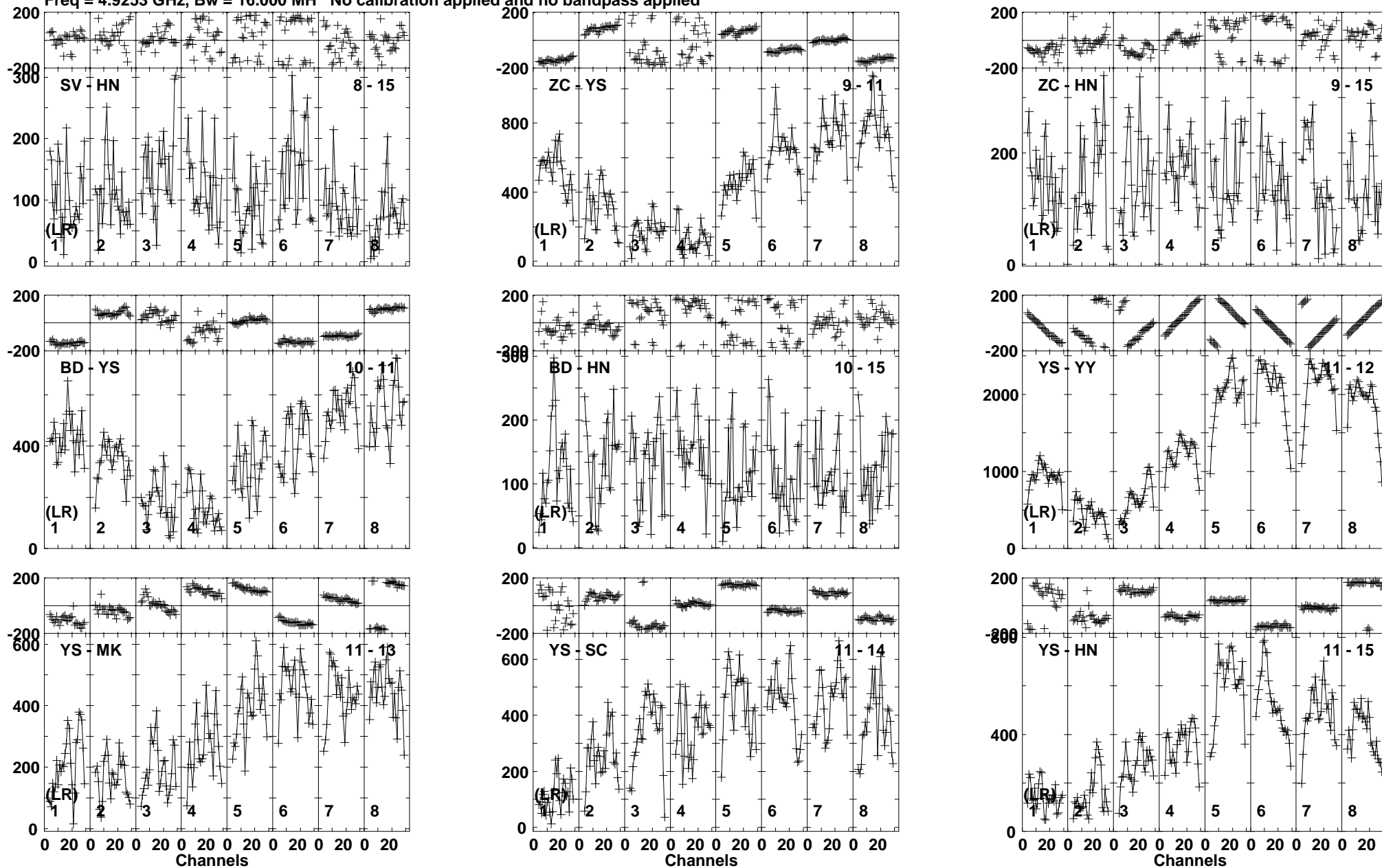
Lower frame: Micro Ampl Jy Top frame: Phas deg Vector averaged cross-power spectrum Baseline: SV (08) - HN (15) Timerange: 01/00:06:26 to 01/00:08:18
