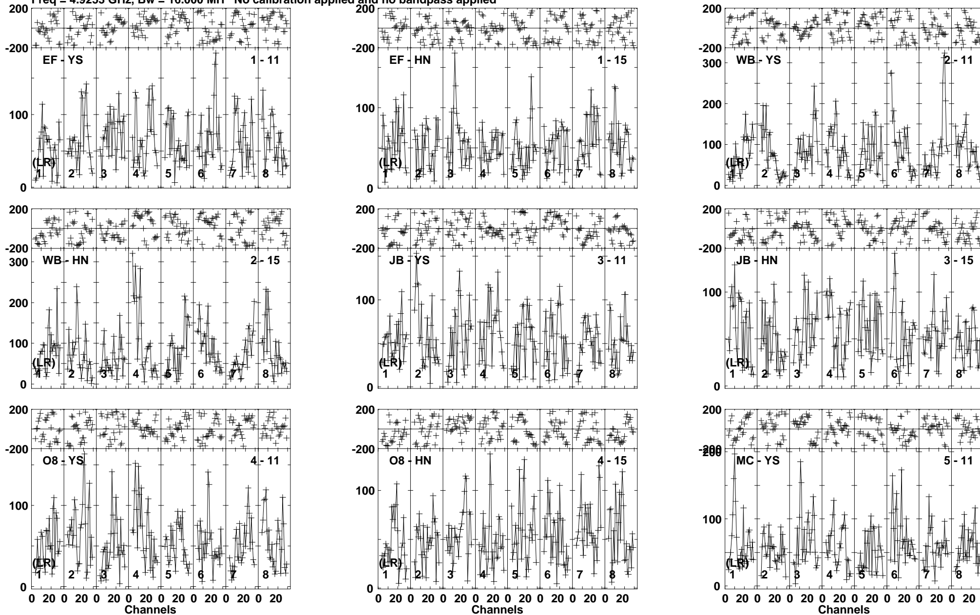
Lower frame: Micro Ampl Jy Top frame: Phas deg Vector averaged cross-power spectrum Baseline: EF (01) - YS (11) Timerange: 00/20:46:33 to 00/20:51:47
