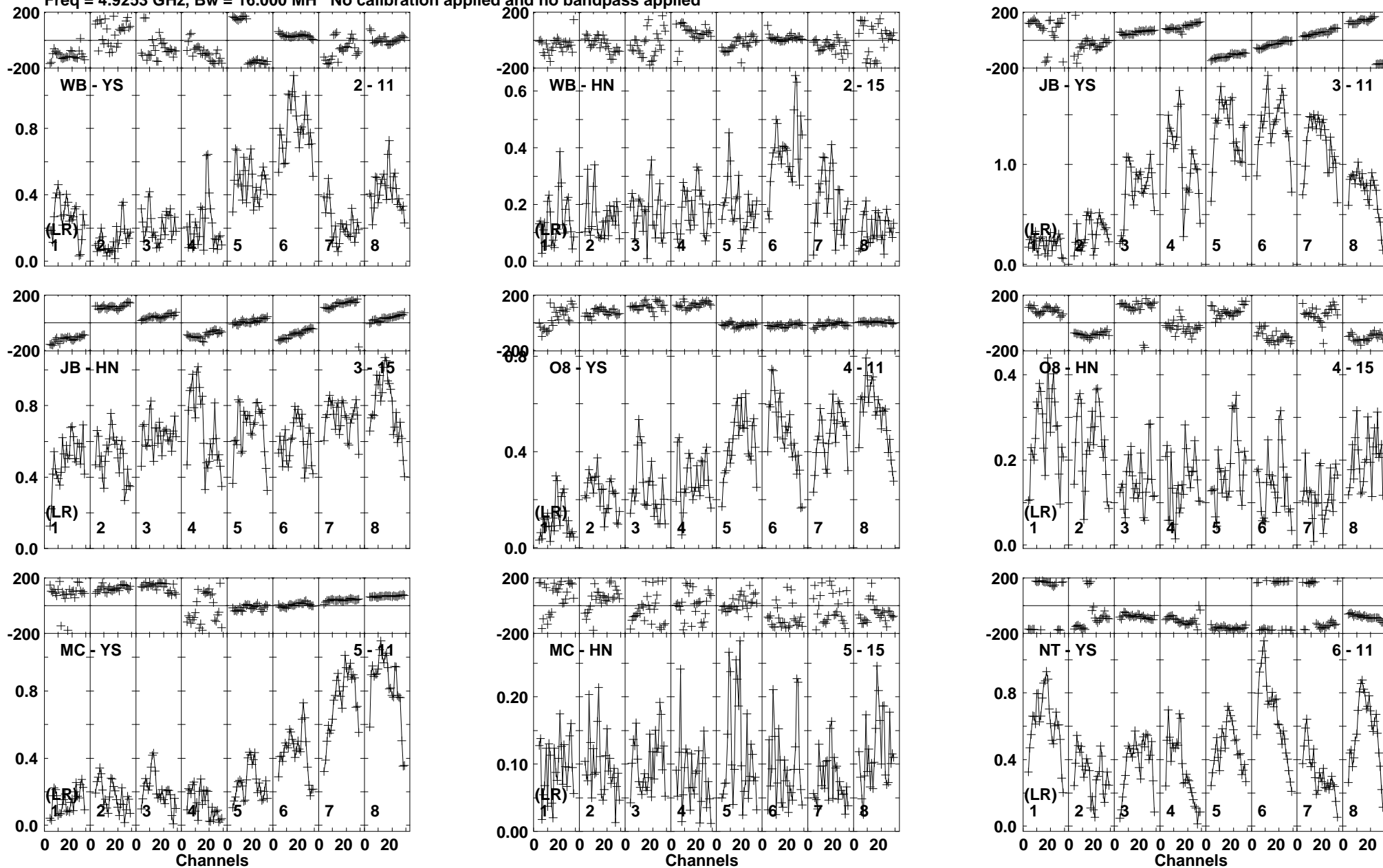
Lower frame: Milli Ampl Jy Top frame: Phas deg Vector averaged cross-power spectrum Baseline: WB (02) - YS (11) Timerange: 00/22:47:13 to 00/22:48:57
