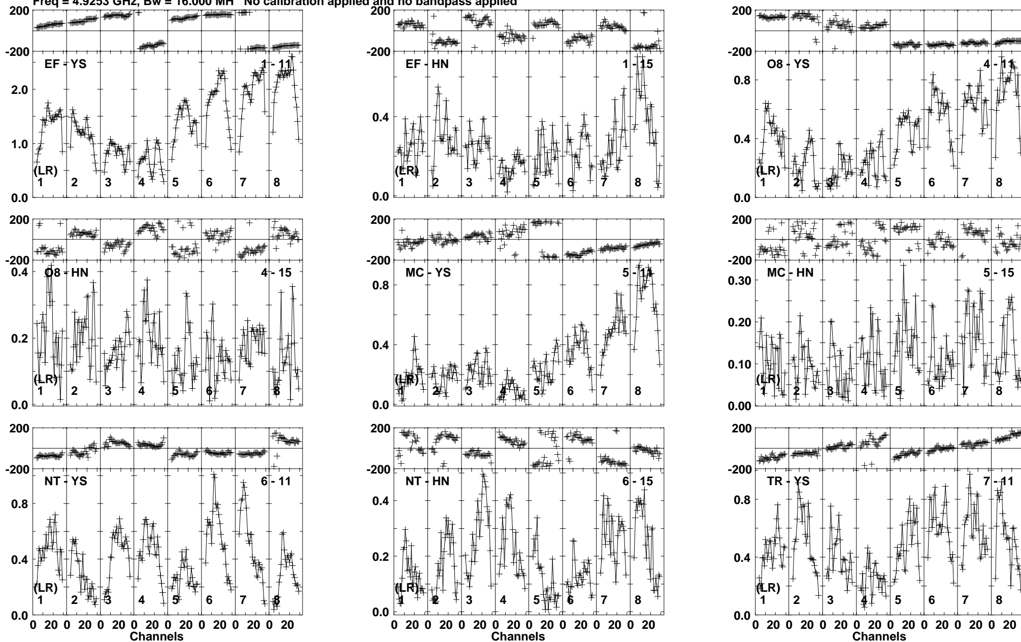
Lower frame: Milli Ampl Jy Top frame: Phas deg Vector averaged cross-power spectrum Baseline: EF (01) - YS (11) Timerange: 00/20:44:37 to 00/20:46:28
