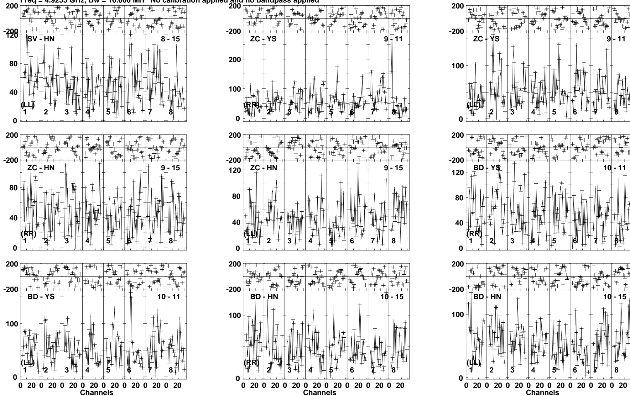
Lower frame: Micro Ampl Jy Top frame: Phas deg Vector averaged cross-power spectrum Baseline: SV (08) - HN (15) Timerange: 00:22:05:49 to 00:22:11:01
