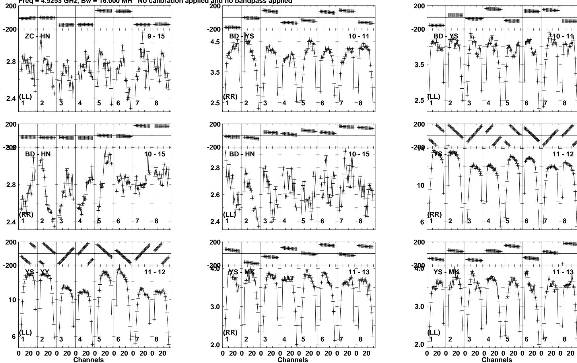
Lower frame: Milli Ampl Jy Top frame: Phas deg Vector averaged cross-power spectrum Baseline: ZC (09) - HN (15) Timerange: 01/00:56:58 to 01/00:58:42
