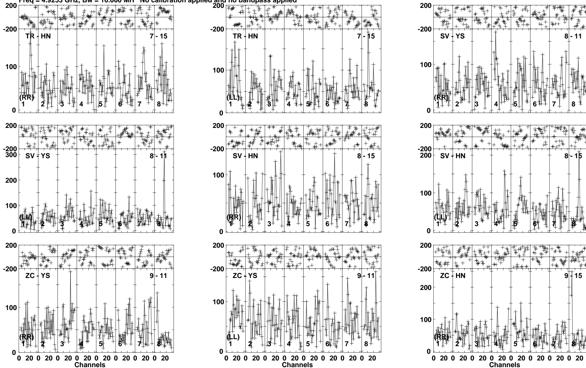
Lower frame: Micro Ampl Jy Top frame: Phas deg Vector averaged cross-power spectrum Baseline: TR (07) - HN (15) Timerange: 01/02:10:53 to 01/02:16:05
