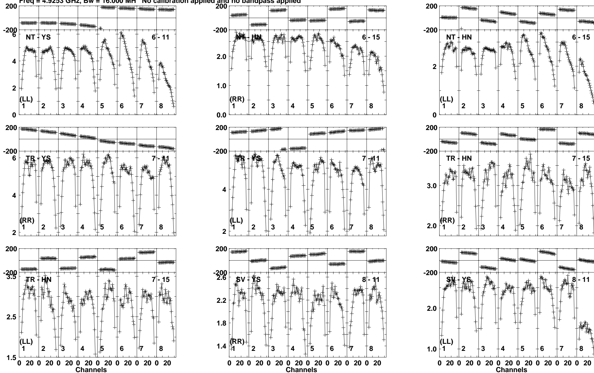
Lower frame: Milli Ampl Jy Top frame: Phas deg Vector averaged cross-power spectrum Baseline: NT (06) - YS (11) Timerange: 01/00:06:26 to 01/00:08:18
