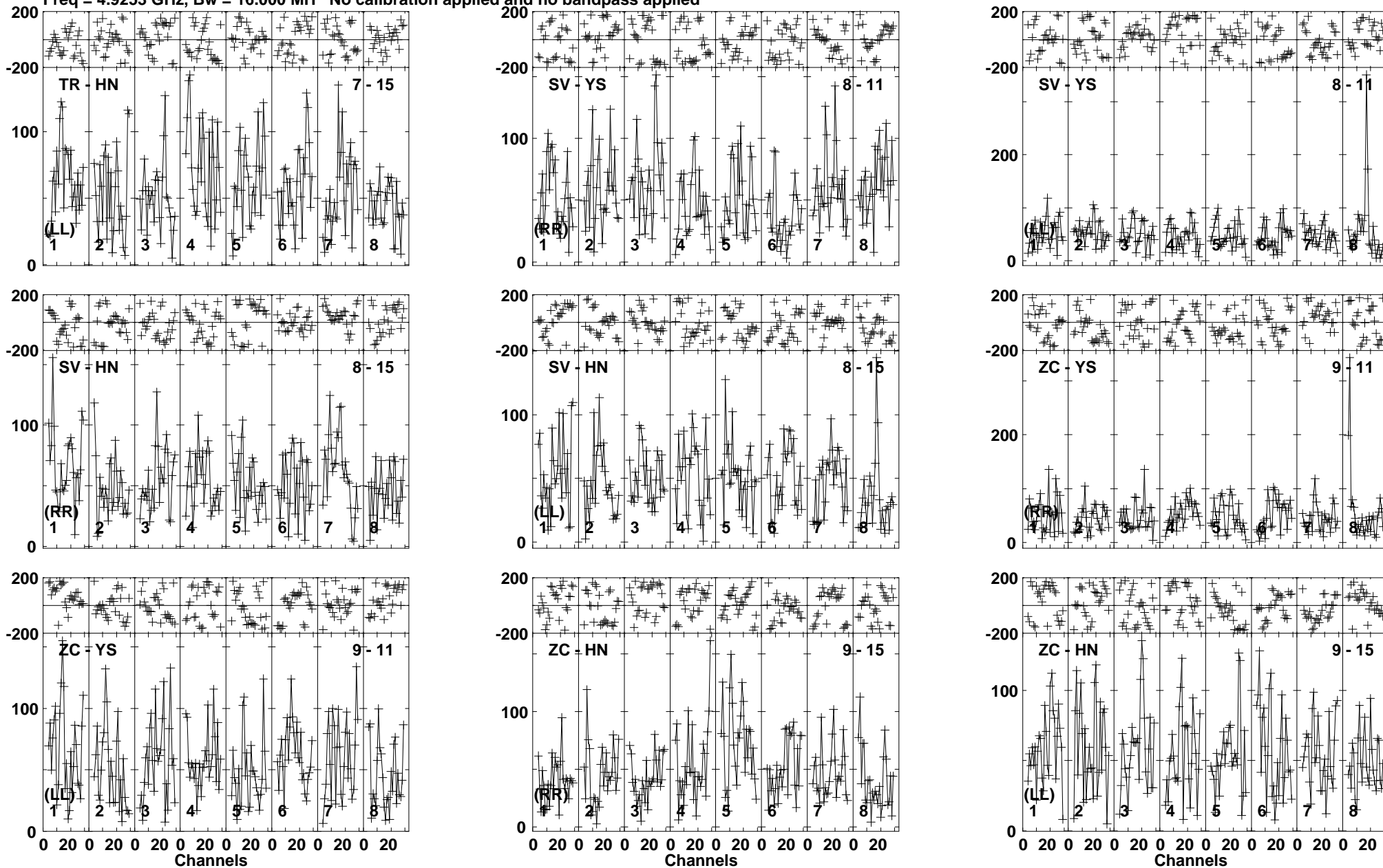
Lower frame: Micro Ampl Jy Top frame: Phas deg Vector averaged cross-power spectrum Baseline: TR (07) - HN (15) Timerange: 00/20:39:19 to 00/20:44:31
