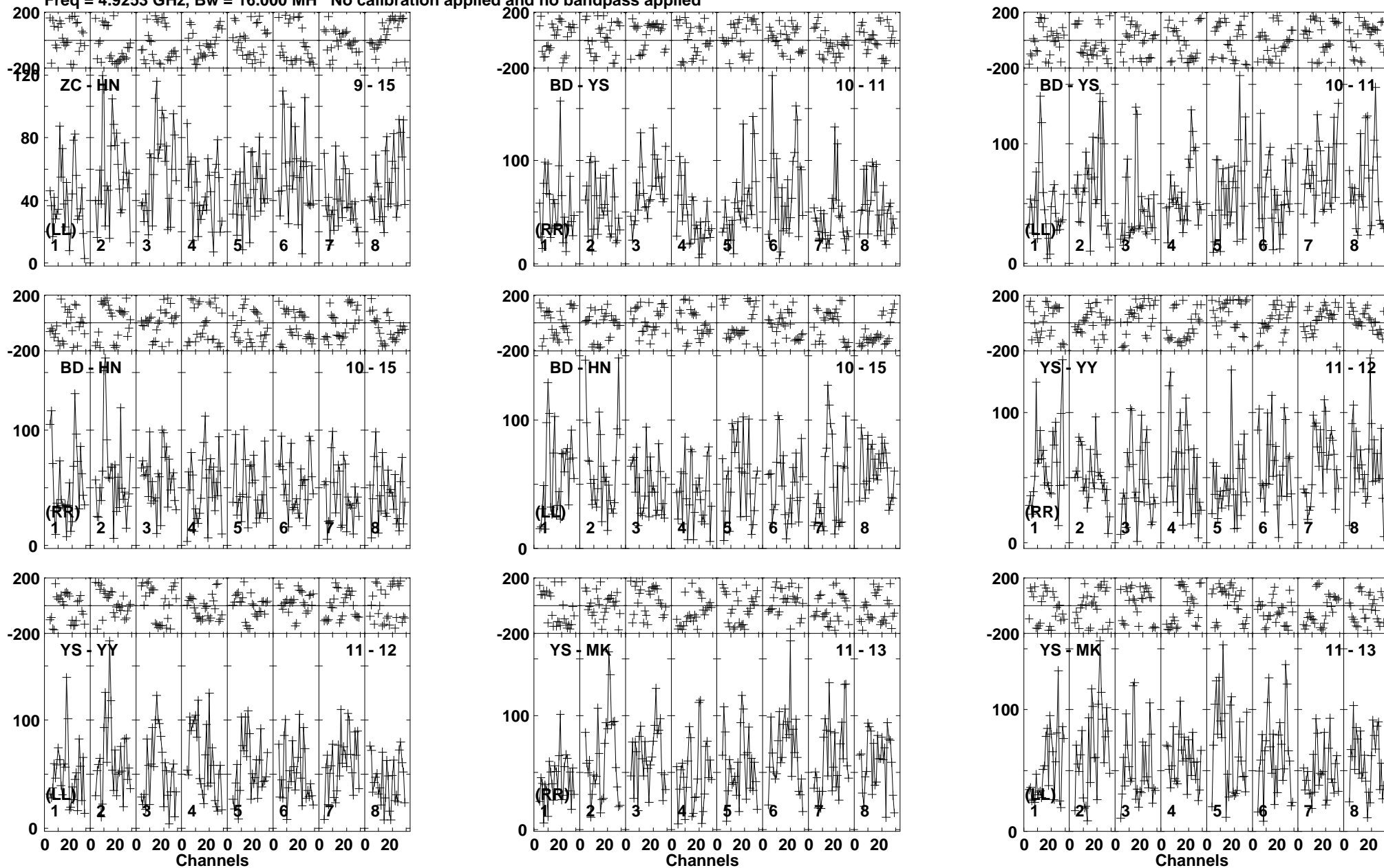
Lower frame: Micro Ampl Jy Top frame: Phas deg Vector averaged cross-power spectrum Baseline: ZC (09) - HN (15) Timerange: 01/00:15:33 to 01/00:20:45
