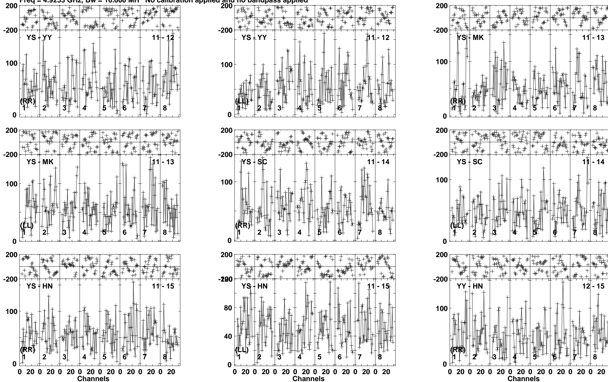
Lower frame: Micro Ampl Jy Top frame: Phas deg Vector averaged cross-power spectrum Baseline: YS (11) - YY (12) Timerange: 00/22:41:53 to 00/22:47:07
