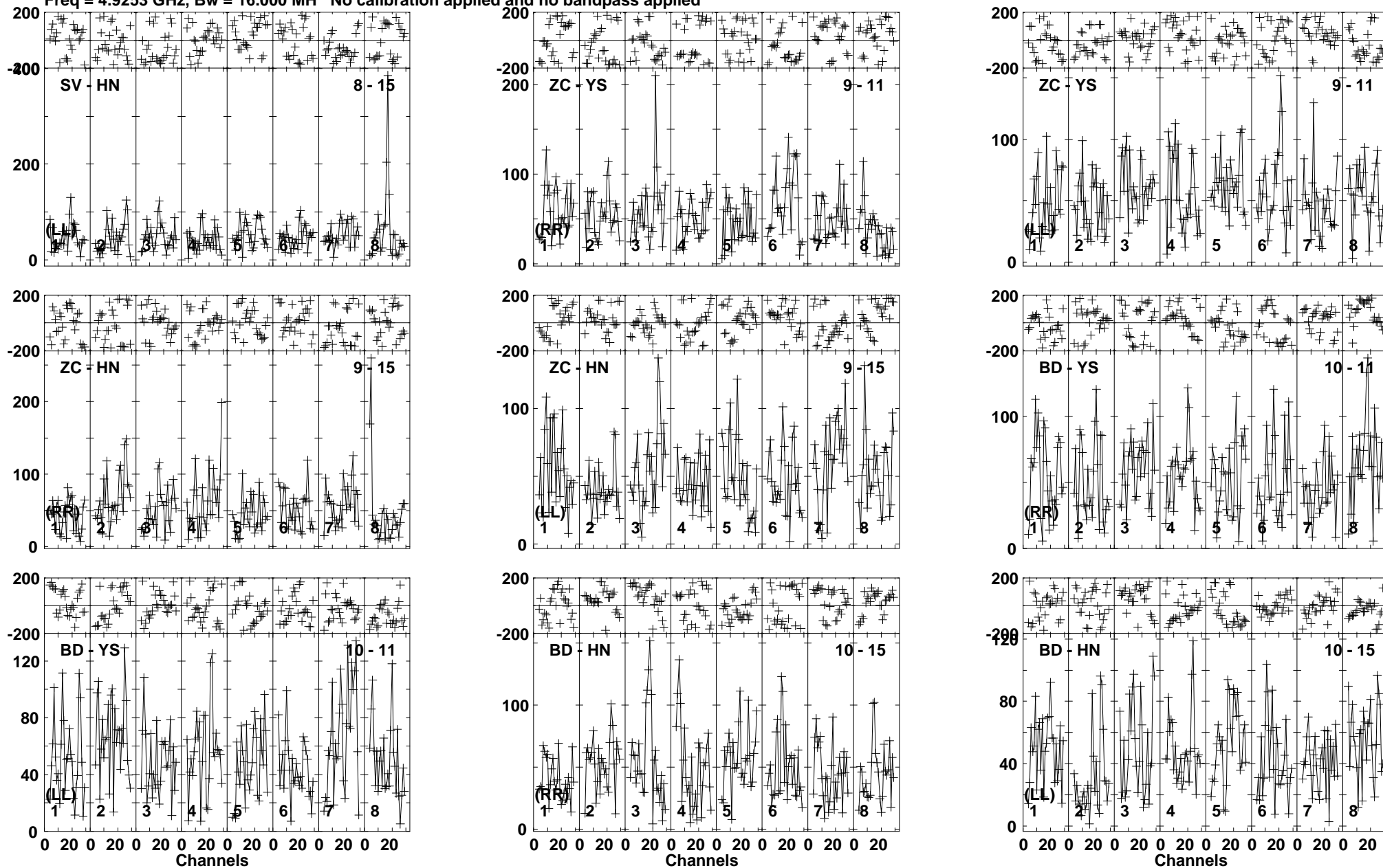
Lower frame: Micro Ampl Jy Top frame: Phas deg Vector averaged cross-power spectrum Baseline: SV (08) - HN (15) Timerange: 00/23:32:18 to 00/23:37:30
