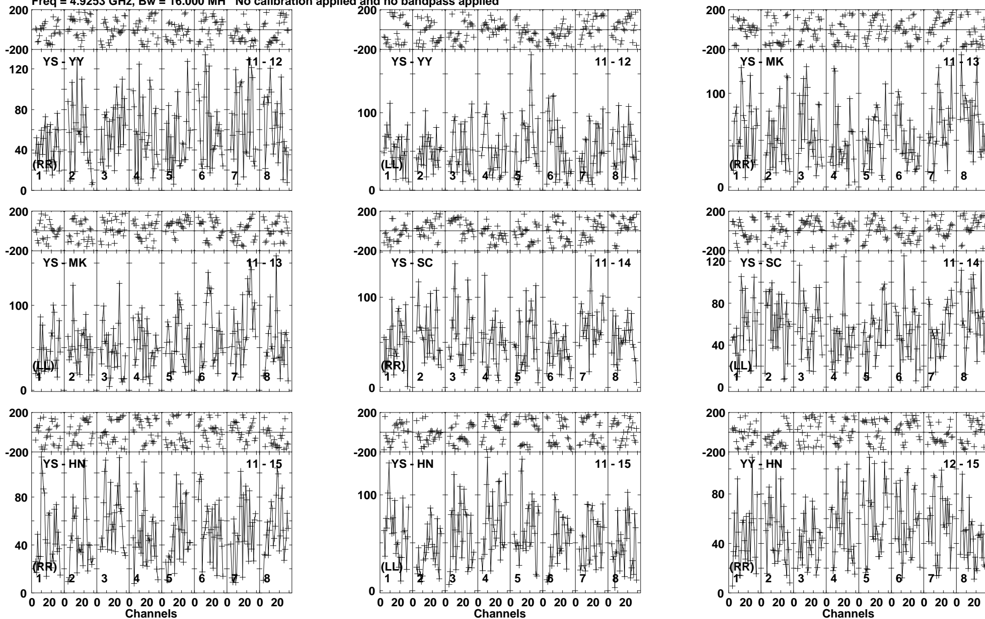
Lower frame: Micro Ampl Jy Top frame: Phas deg Vector average cross-power spectrum Baseline: YS (11) - YY (12) Timerange: 00:22:05:49 to 00:22:11:01
