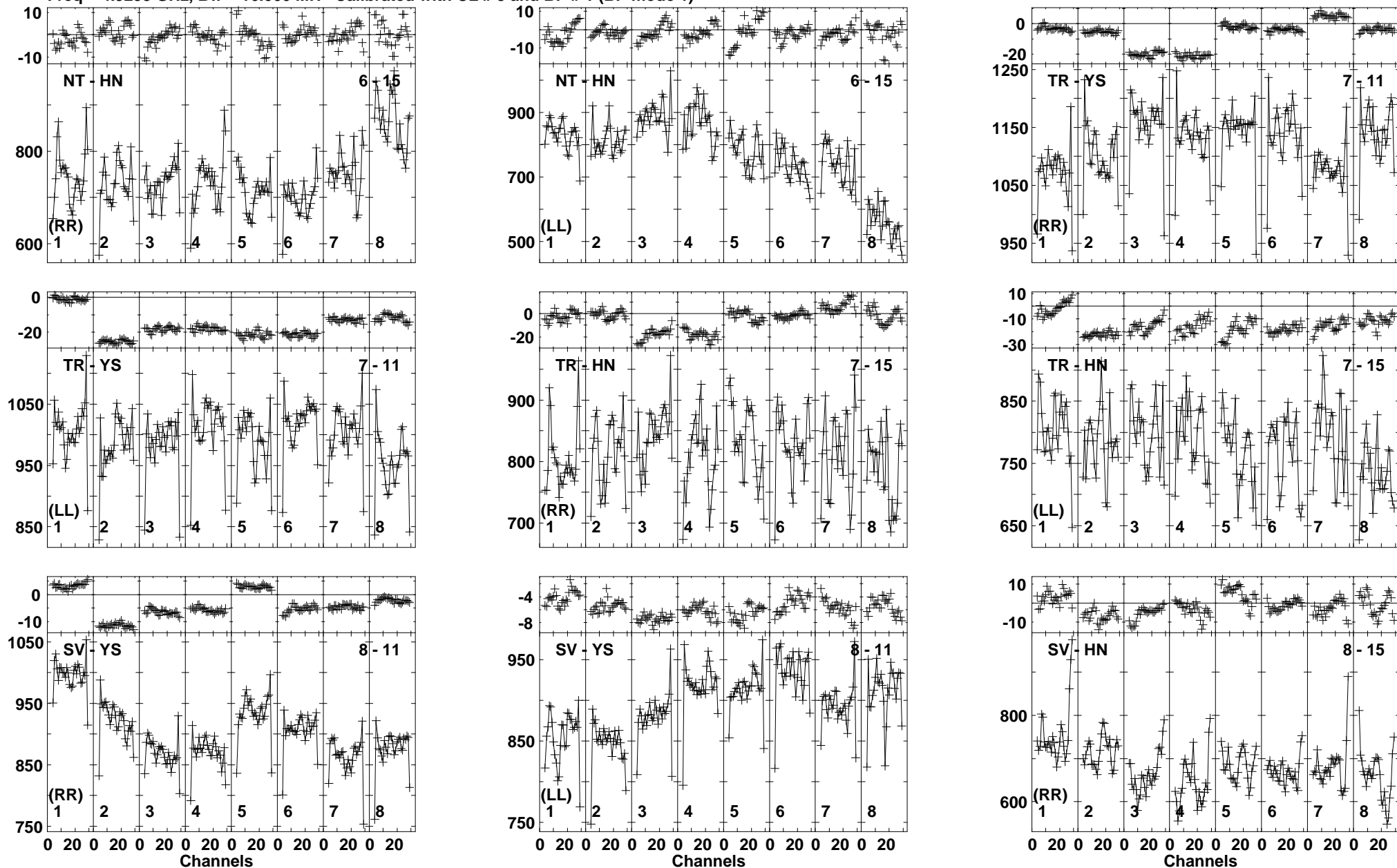
Lower frame: Milli Ampl Jy Top frame: Phas deg Vector averaged cross-power spectrum Baseline: NT (06) - HN (15) Timerange: 00/20:51:50 to 00/20:53:37
