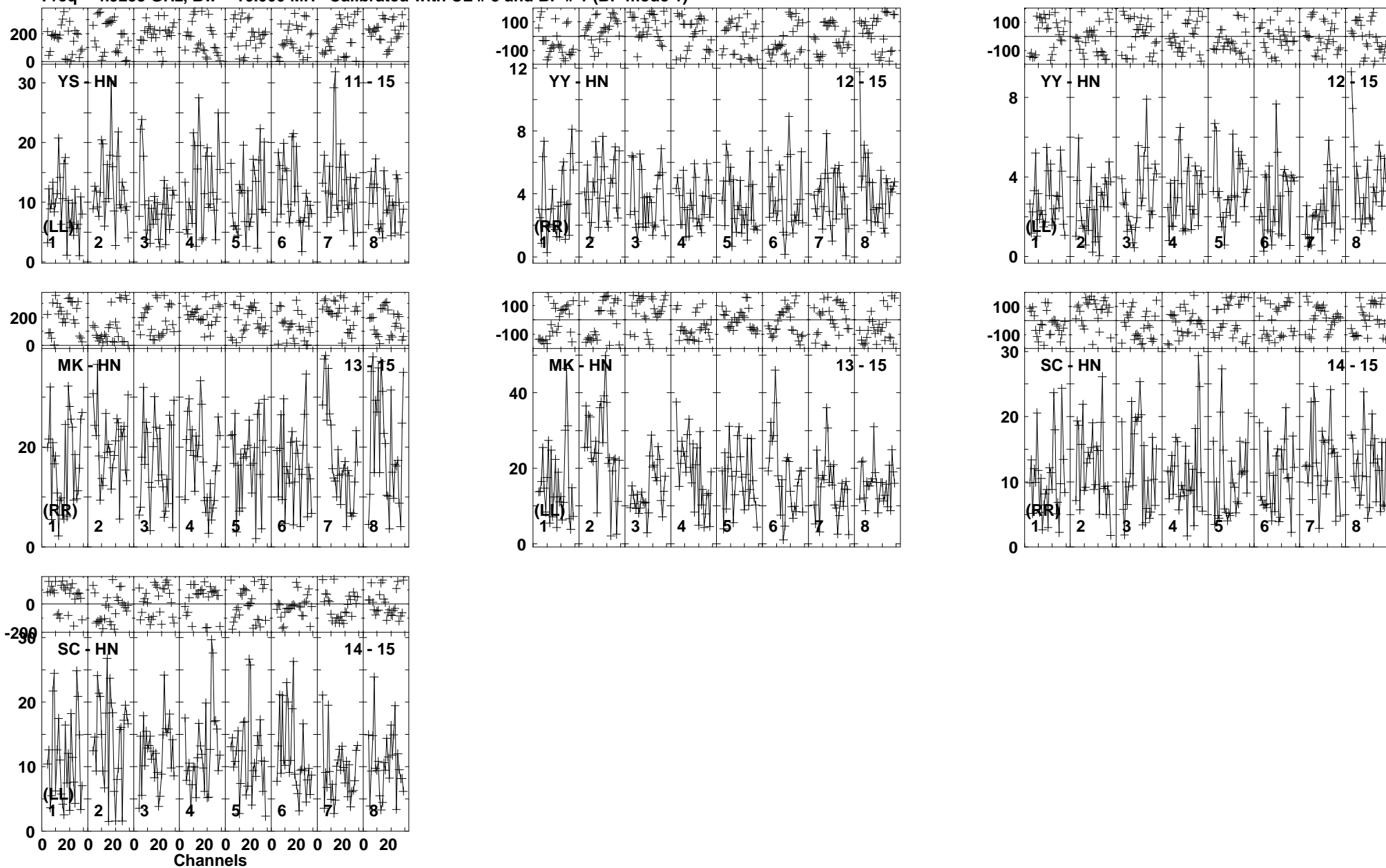
Lower frame: Milli Ampl Jy Top frame: Phas deg Vector averaged cross-power spectrum Baseline: YS (11) - HN (15) Timerange: 00/21:22:34 to 00/21:27:46
