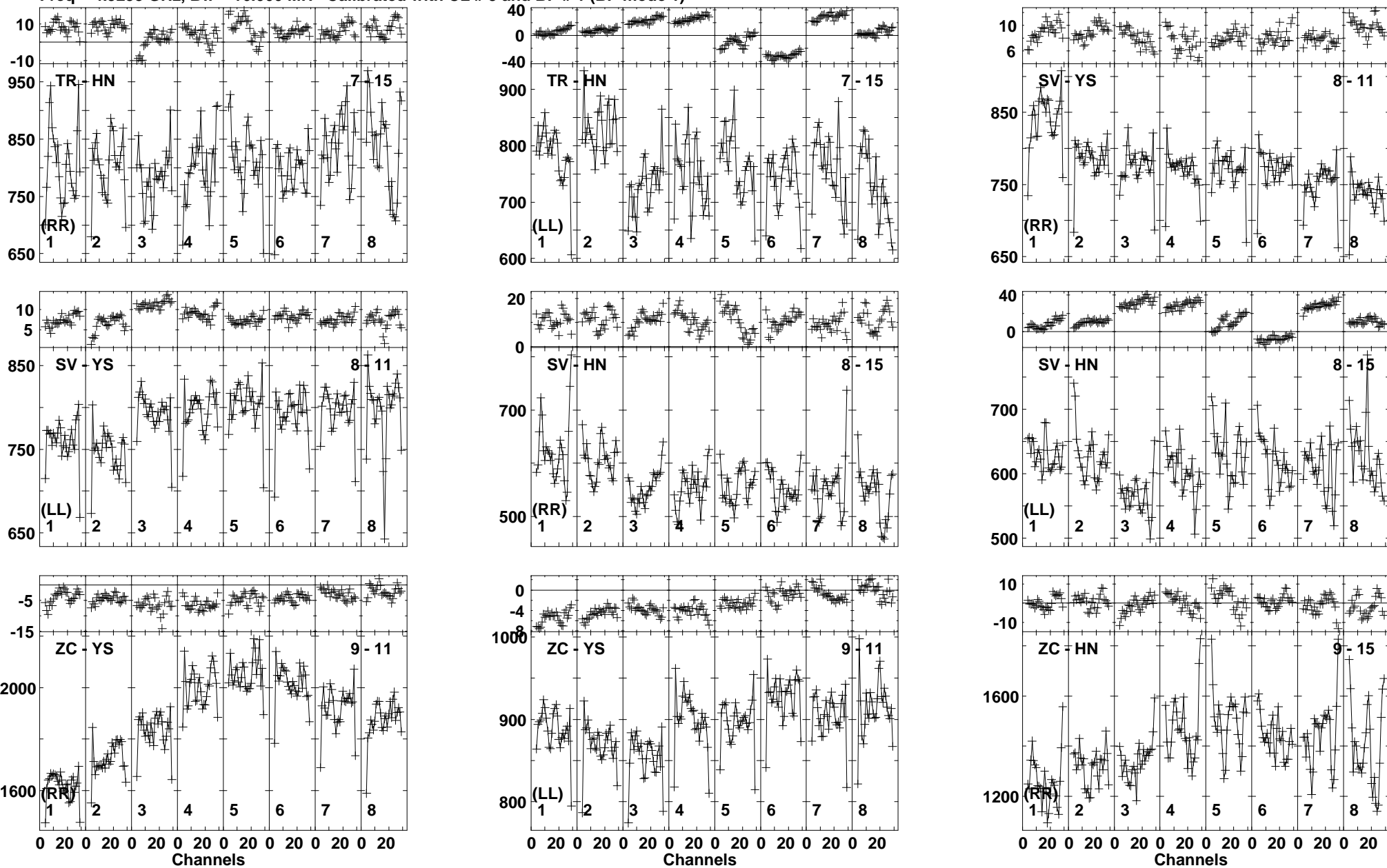
Lower frame: Milli Ampl Jy Top frame: Phas deg Vector averaged cross-power spectrum Baseline: TR (07) - HN (15) Timerange: 00/23:30:28 to 00/23:32:12
