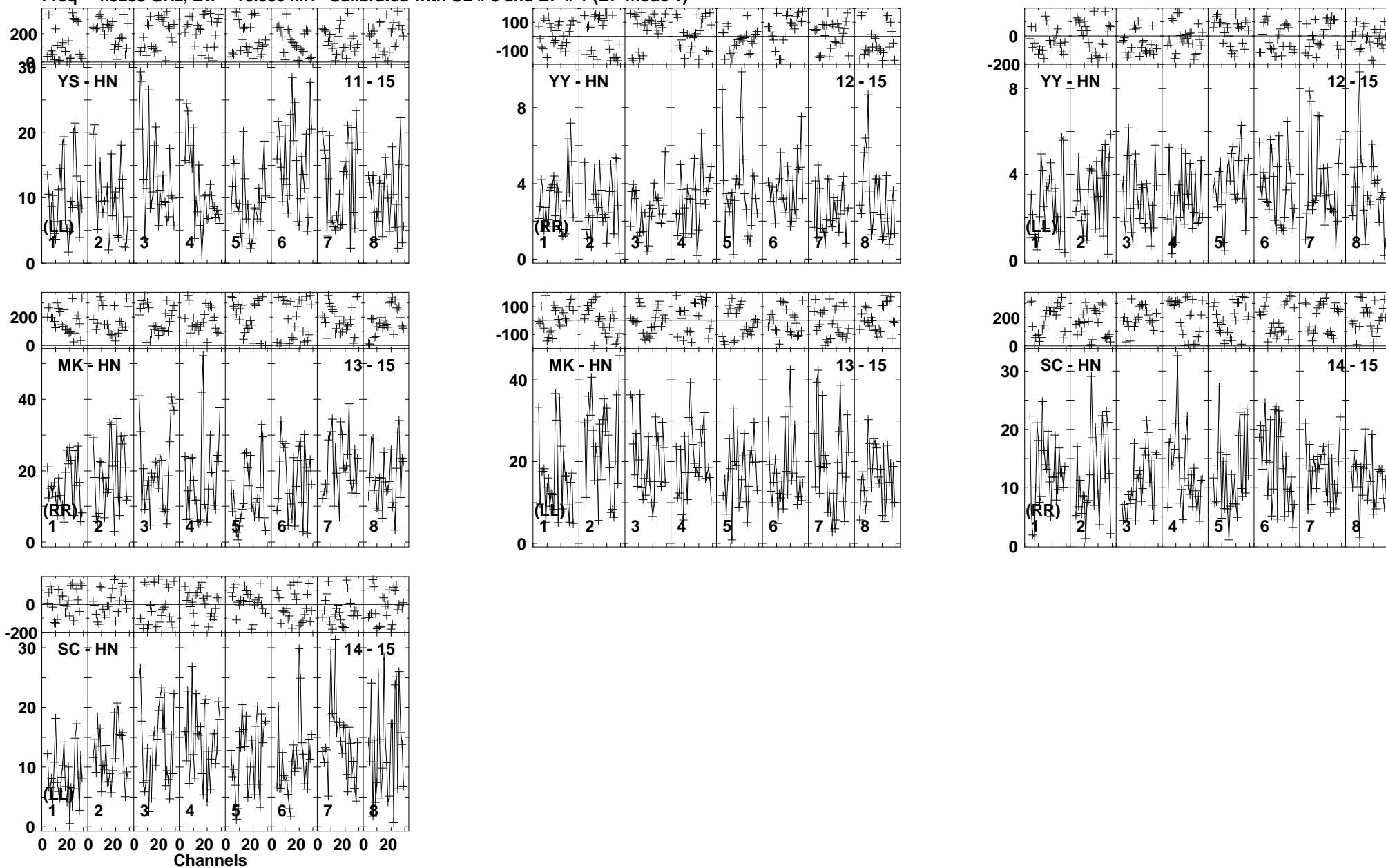
Lower frame: Milli Ampl Jy Top frame: Phas deg Vector averaged cross-power spectrum Baseline: YS (11) - HN (15) Timerange: 00/21:08:09 to 00/21:13:21
