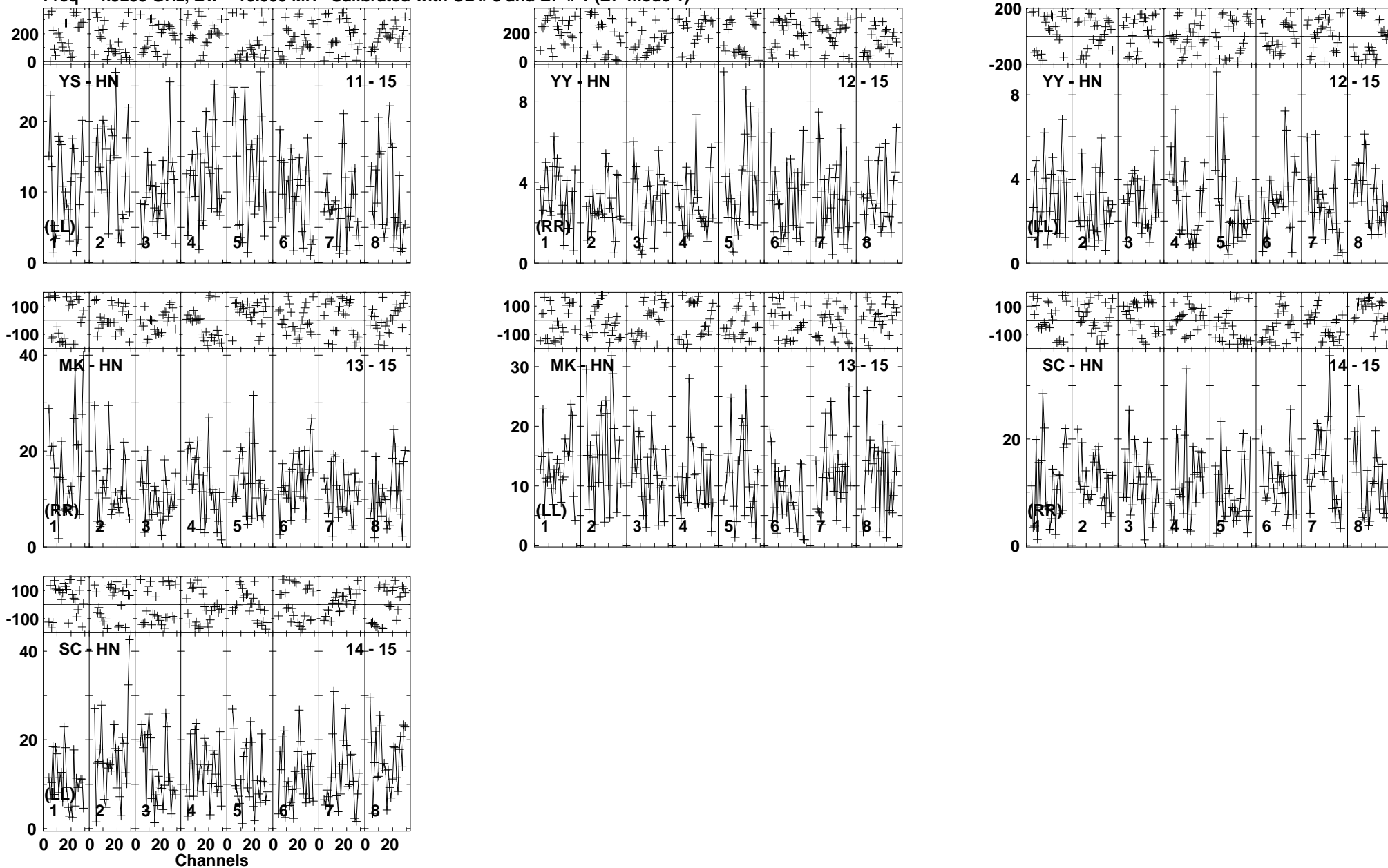
Lower frame: Milli Ampl Jy Top frame: Phas deg Vector averaged cross-power spectrum Baseline: YS (11) - HN (15) Timerange: 01/00:15:33 to 01/00:20:45
