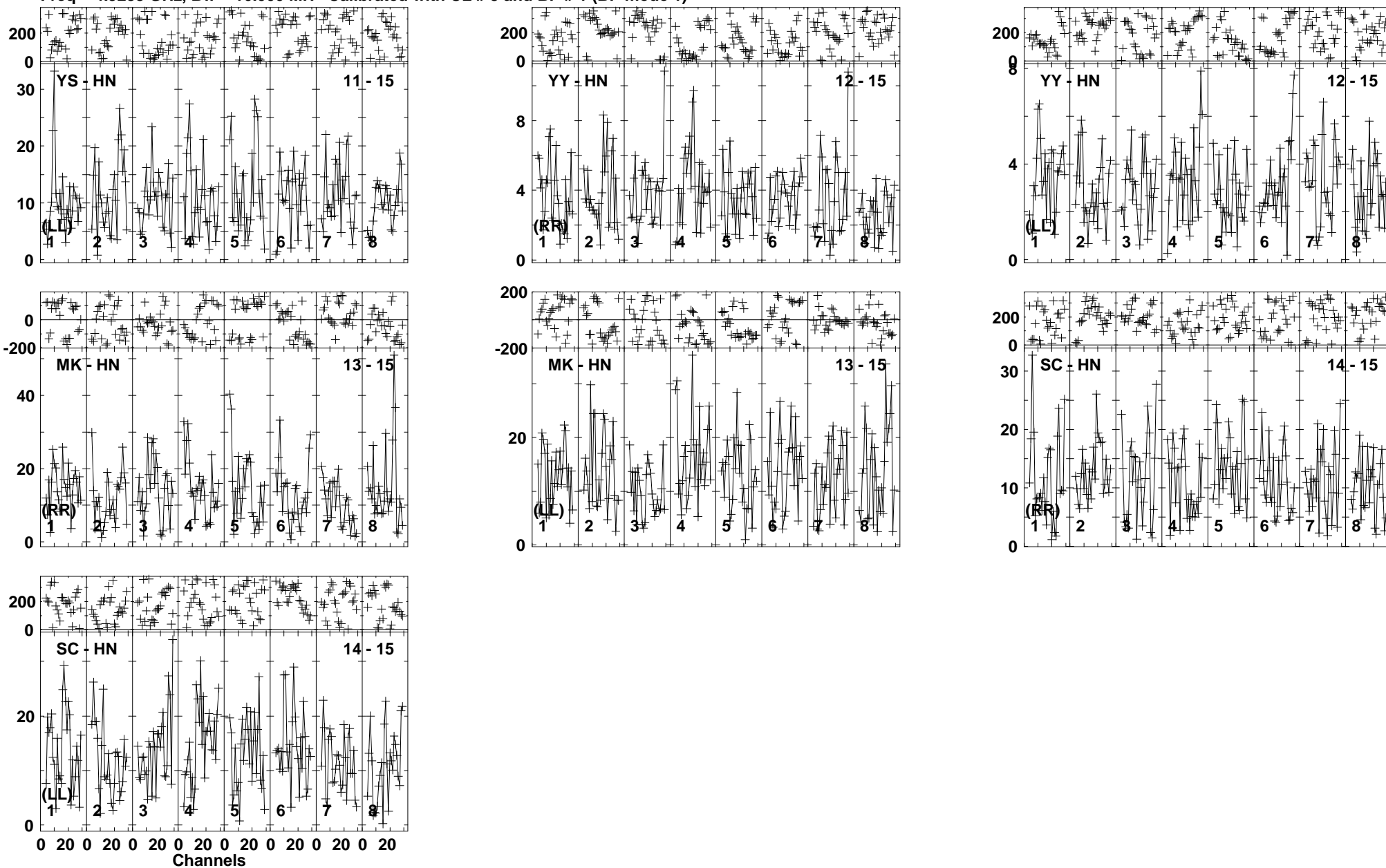
Lower frame: Milli Ampl Jy Top frame: Phas deg Vector averaged cross-power spectrum Baseline: YS (11) - HN (15) Timerange: 00/23:46:43 to 00/23:51:55
