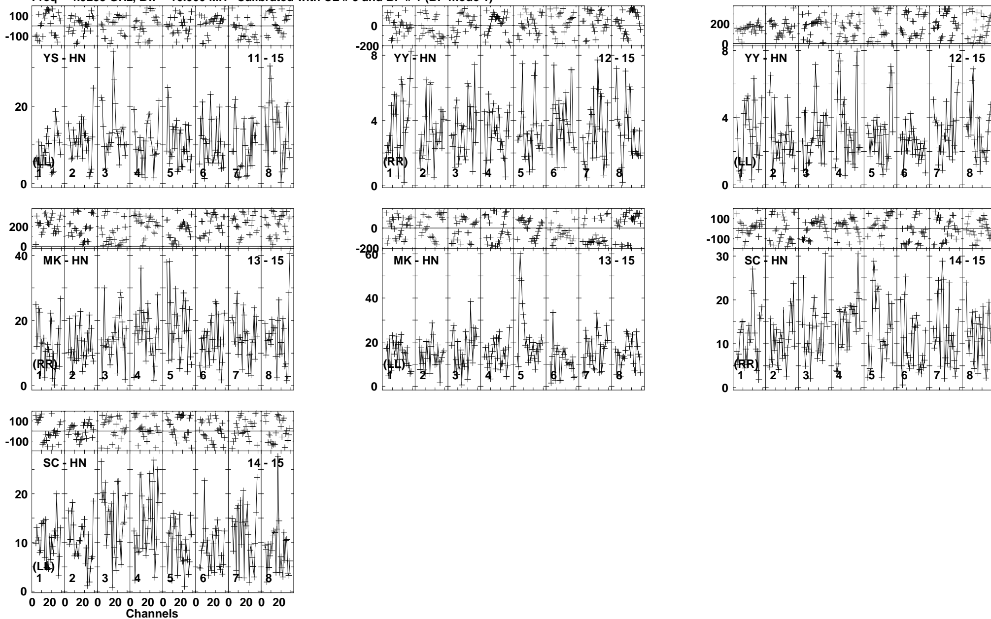
Lower frame: Milli Ampl Jy Top frame: Phas deg Vector averaged cross-power spectrum Baseline: YS (11) - HN (15) Timerange: 00/22:49:03 to 00/22:54:15
