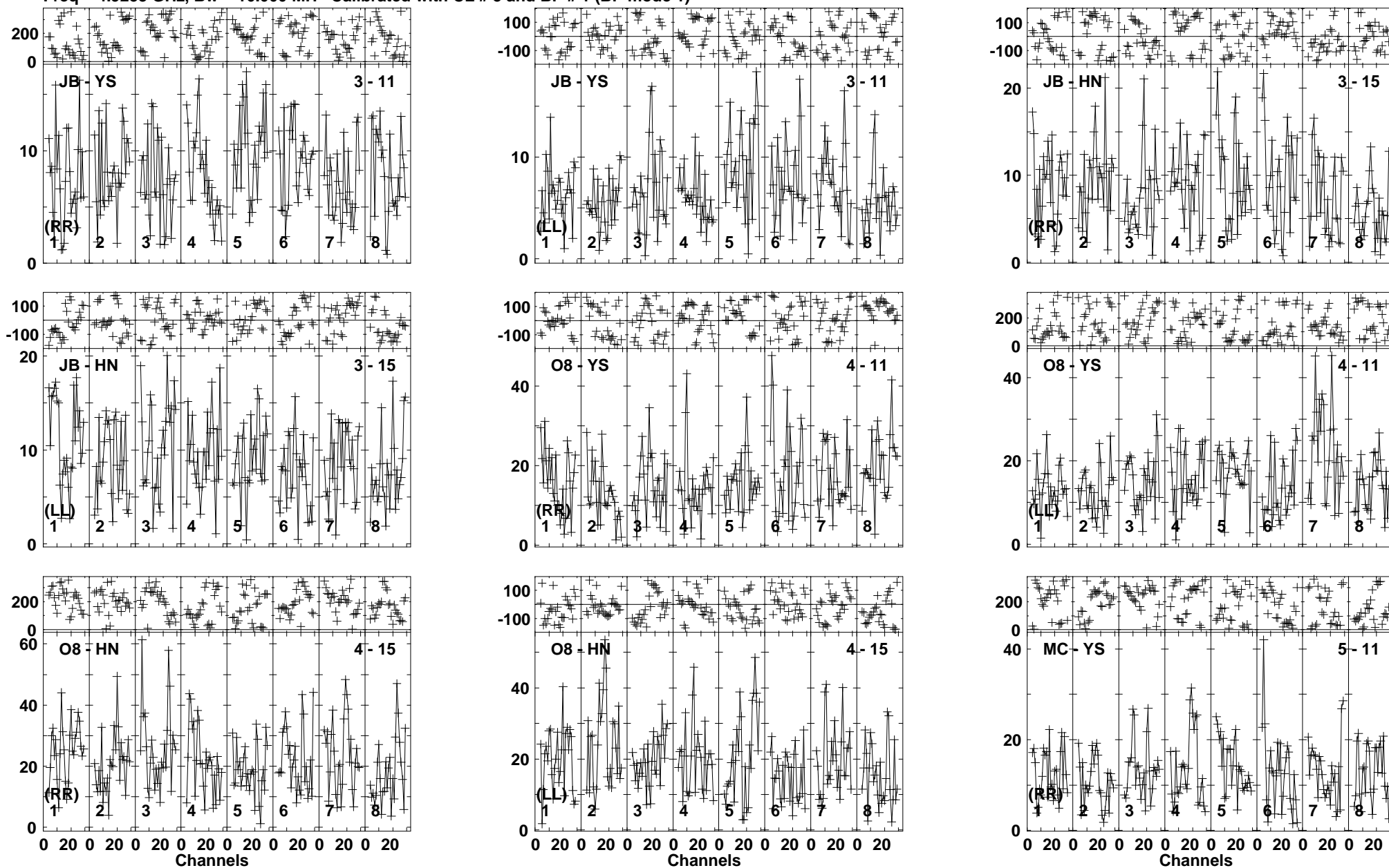
Lower frame: Milli Ampl Jy Top frame: Phas deg Vector averaged cross-power spectrum Baseline: JB (03) - YS (11) Timerange: 00/22:05:49 to 00/22:11:01
