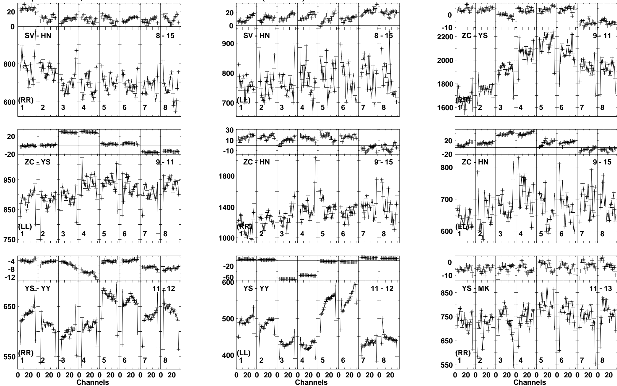
Lower frame: Milli Ampl Jy Top frame: Phas deg Vector averaged cross-power spectrum Baseline: SV (08) - HN (15) Timerange: 00/21:13:27 to 00/21:15:18
