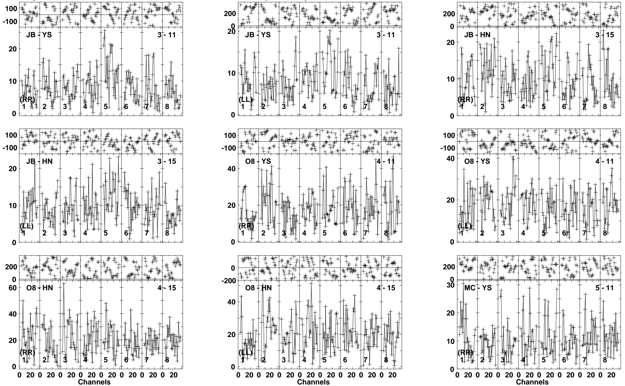
Lower frame: Milli Ampl Jy Top frame: Phas deg Vector averaged cross-power spectrum Baseline: JB (03) - YS (11) Timerange: 00/23:03:28 to 00/23:08:40
