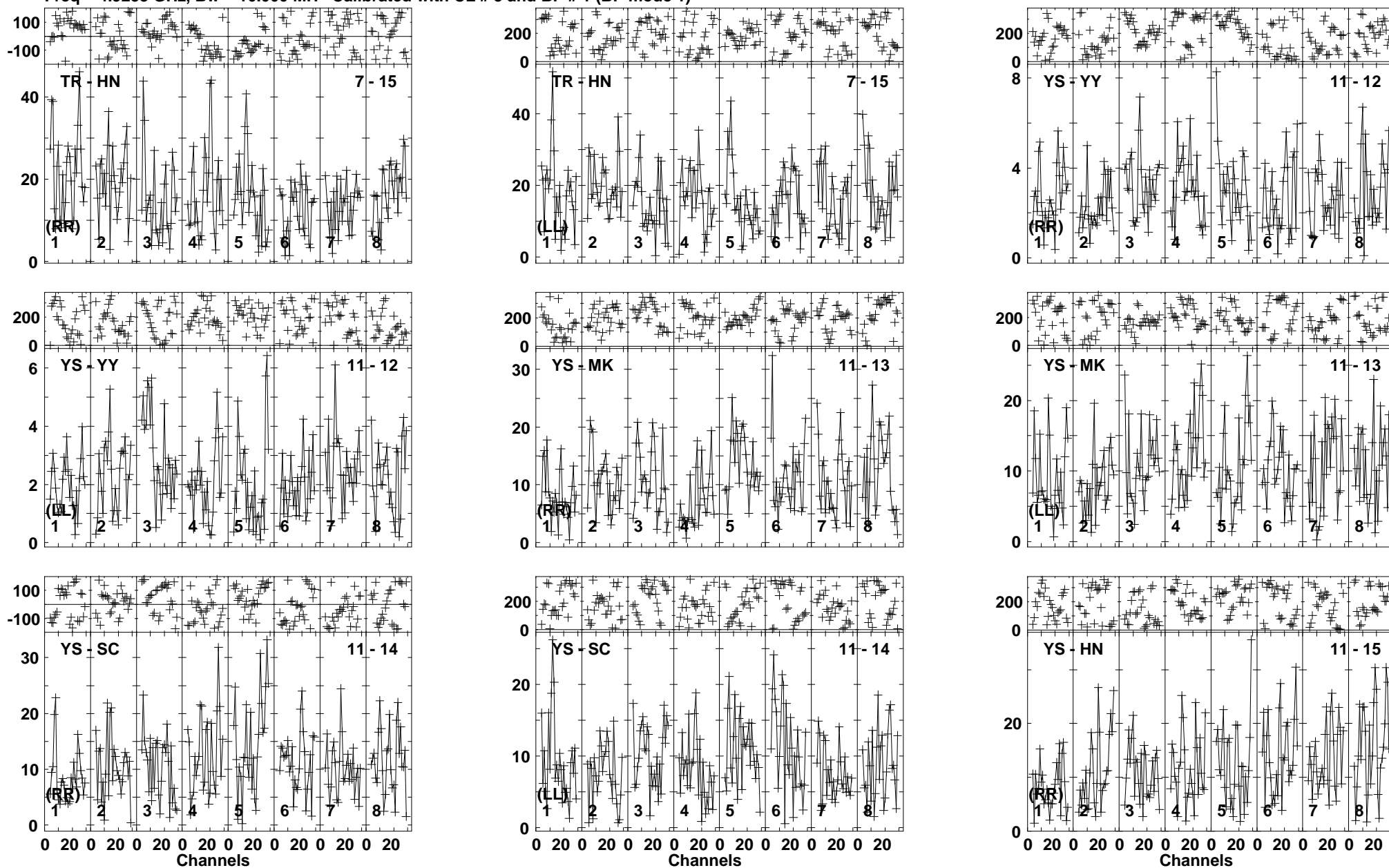
Lower frame: Milli Ampl Jy Top frame: Phas deg Vector averaged cross-power spectrum Baseline: TR (07) - HN (15) Timerange: 01/01:49:18 to 01/01:54:32
