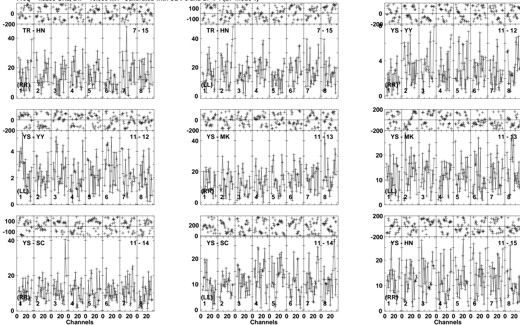
Lower frame: Milli Ampl Jy Top frame: Phas deg Vector averaged cross-power spectrum Baseline: TR (07) - HN (15) Timerange: 00/22:27:28 to 00/22:32:42
