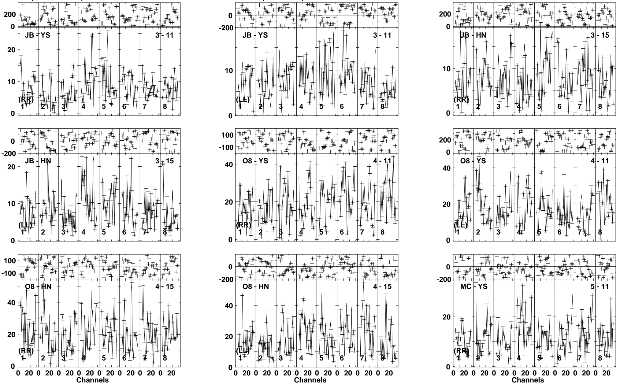
Lower frame: Milli Ampl Jy Top frame: Phas deg Vector averaged cross-power spectrum Baseline: JB (03) - YS (11) Timerange: 00/23:39:33 to 00/23:44:47
