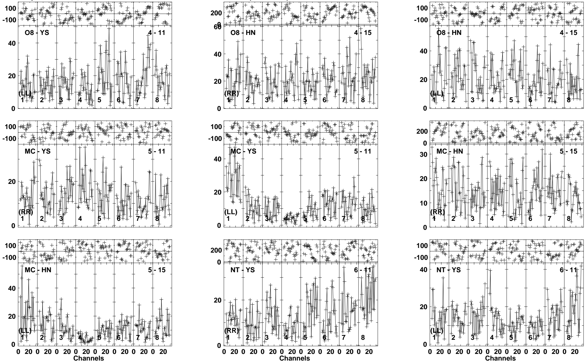
Lower frame: Milli Ampl Jy Top frame: Phas deg Vector averaged cross-power spectrum Baseline: O8 (04) - YS (11) Timerange: 00/20:39:19 to 00/20:44:31
