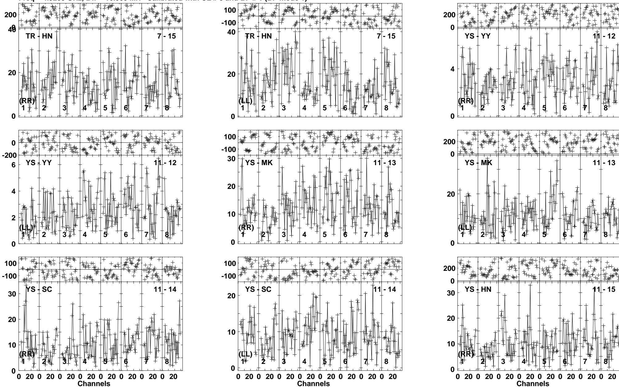
Lower frame: Milli Ampl Jy Top frame: Phas deg Vector averaged cross-power spectrum Baseline: TR (07) - HN (15) Timerange: 00/23:46:43 to 00/23:51:55
