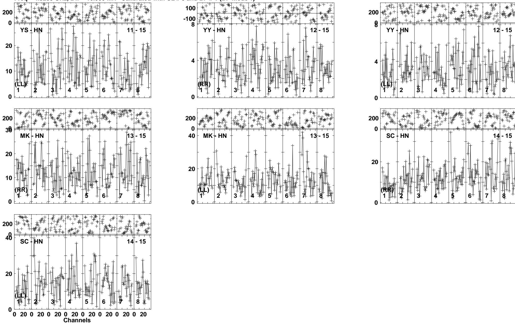
Lower frame: Milli Ampl Jy Top frame: Phas deg Vector averaged cross-power spectrum Baseline: YS (11) - HN (15) Timerange: 01/01:49:18 to 01/01:54:32
