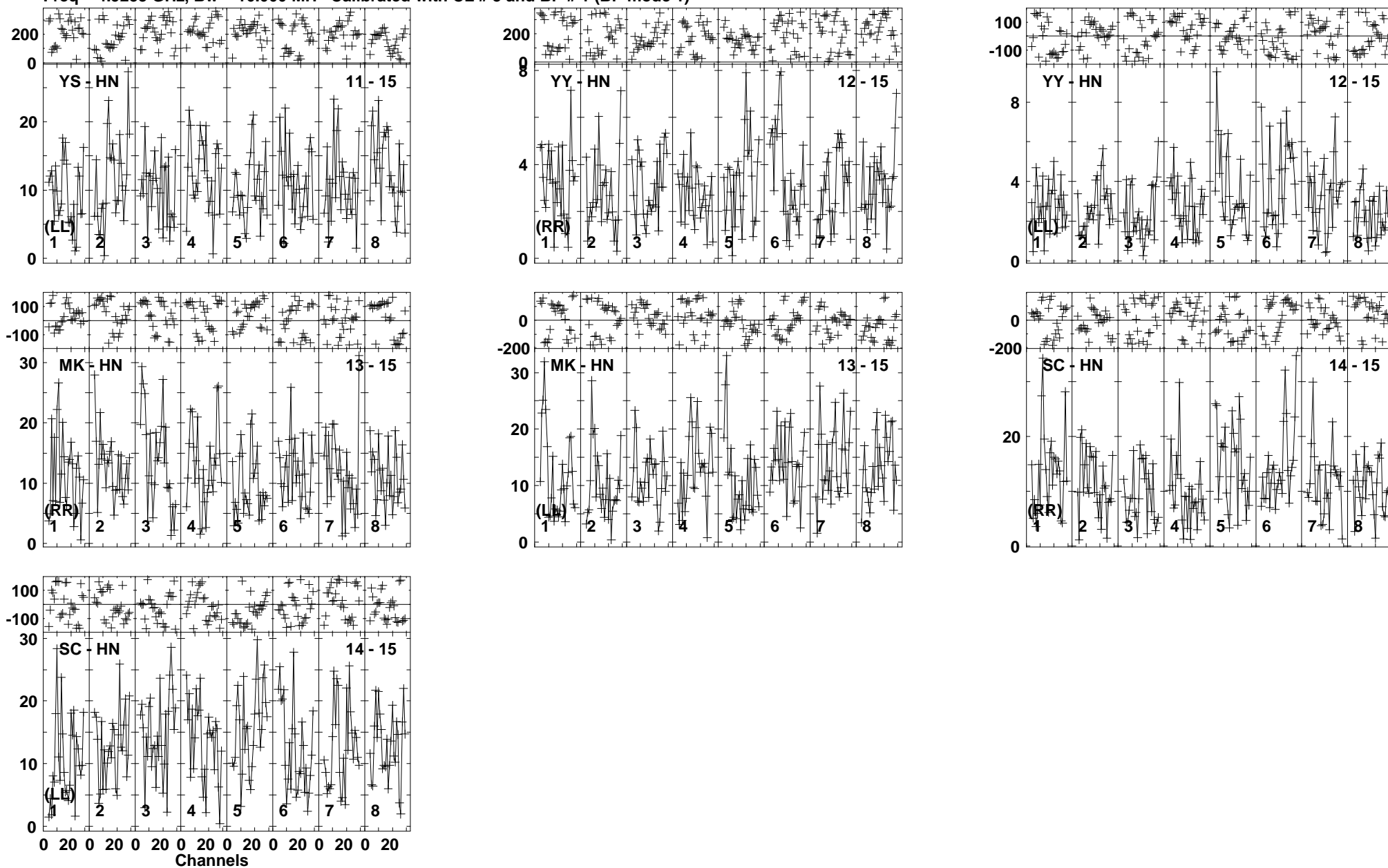
Lower frame: Milli Ampl Jy Top frame: Phas deg Vector averaged cross-power spectrum Baseline: YS (11) - HN (15) Timerange: 01/01:06:03 to 01/01:11:17
