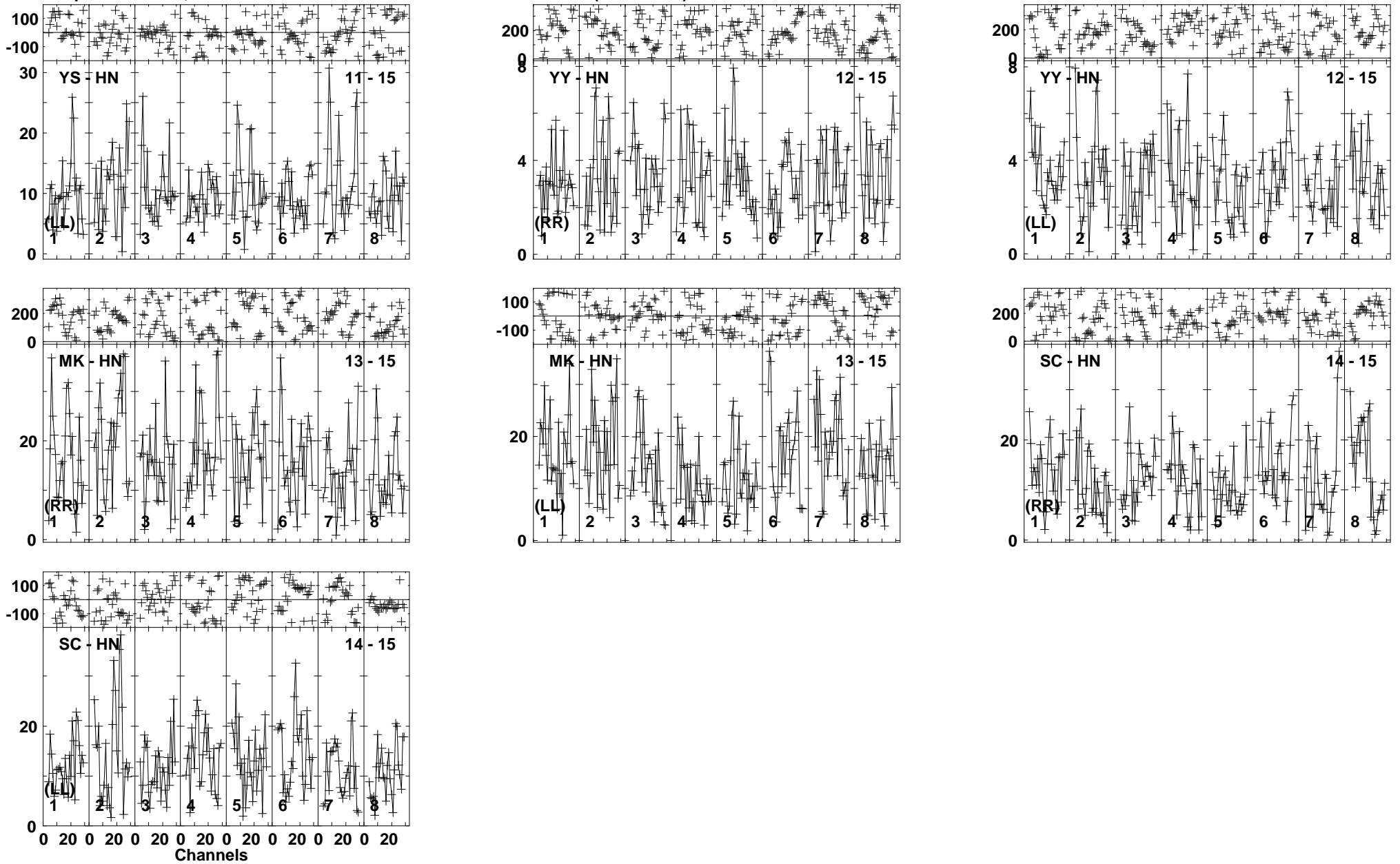
Lower frame: Milli Ampl Jy Top frame: Phas deg Vector averaged cross-power spectrum Baseline: YS (11) - HN (15) Timerange: 00:22:13:03 to 00:22:18:17
