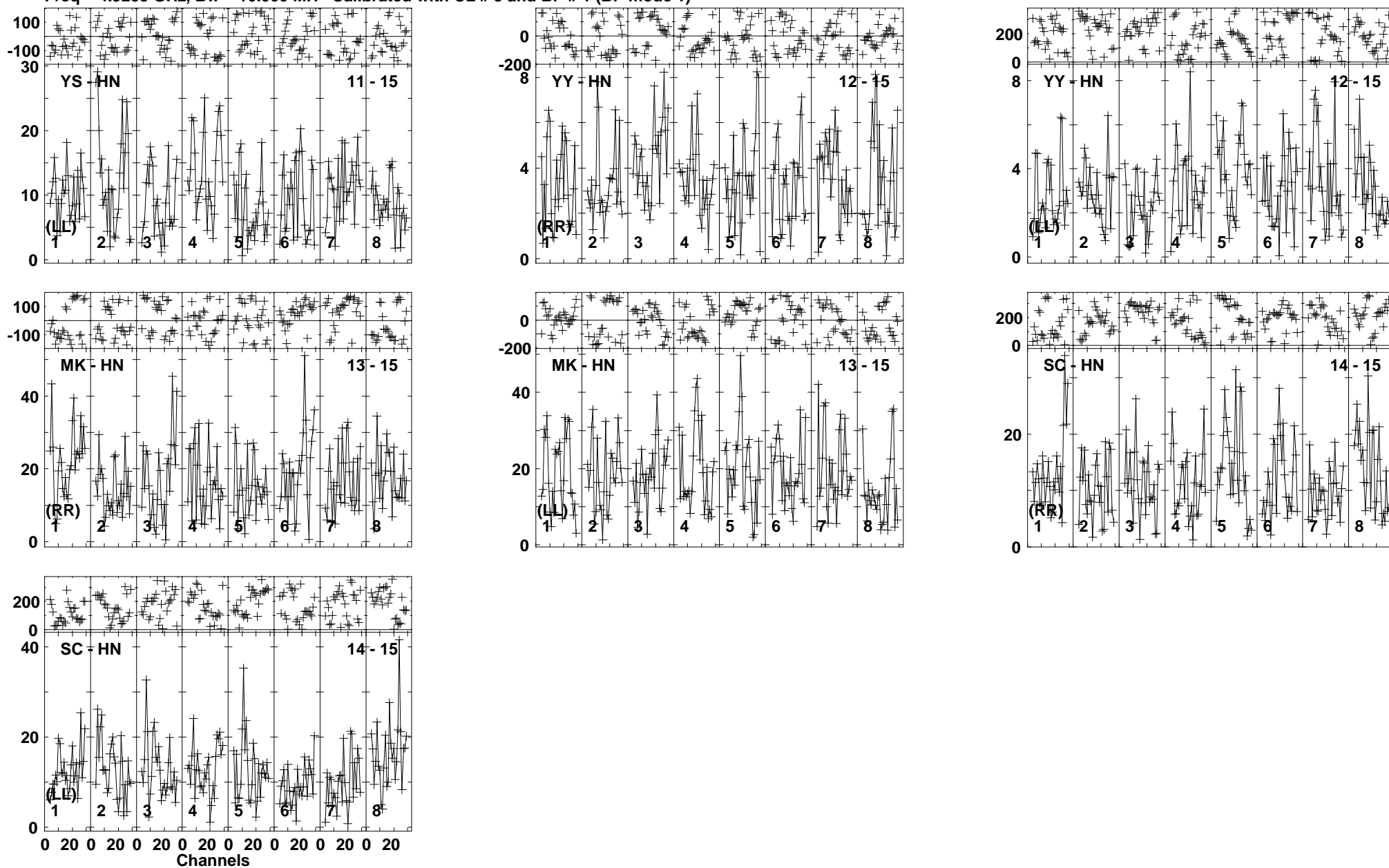
Lower frame: Milli Ampl Jy Top frame: Phas deg Vector averaged cross-power spectrum Baseline: YS (11) - HN (15) Timerange: 00/21:36:59 to 00/21:42:11
