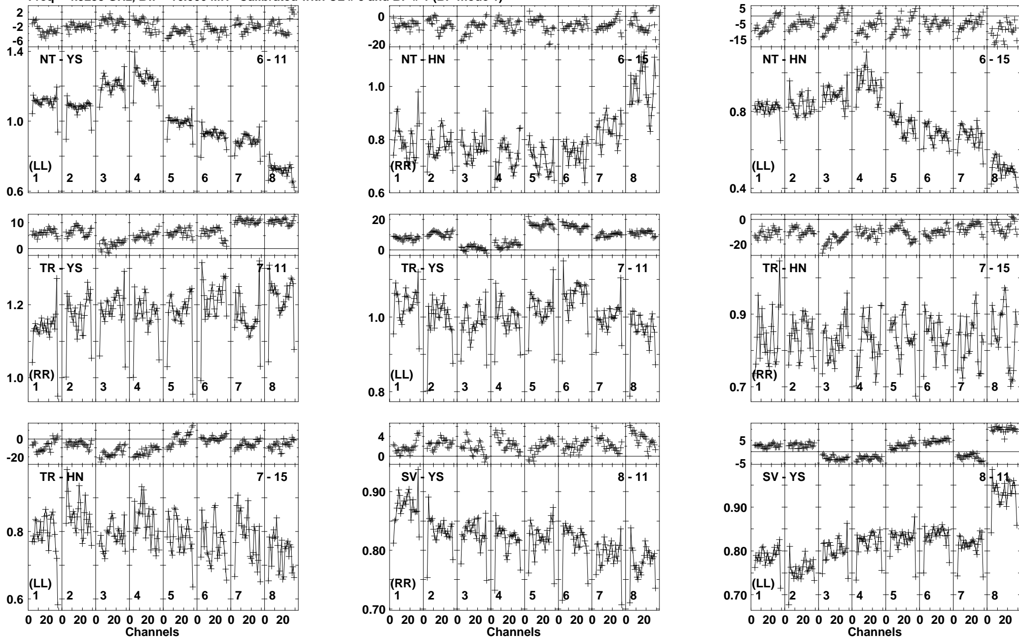
Lower frame: Ampl Jy Top frame: Phas deg Vector averaged cross-power spectrum Baseline: NT (06) - YS (11) Timerange: 00/21:42:17 to 00/21:44:08
