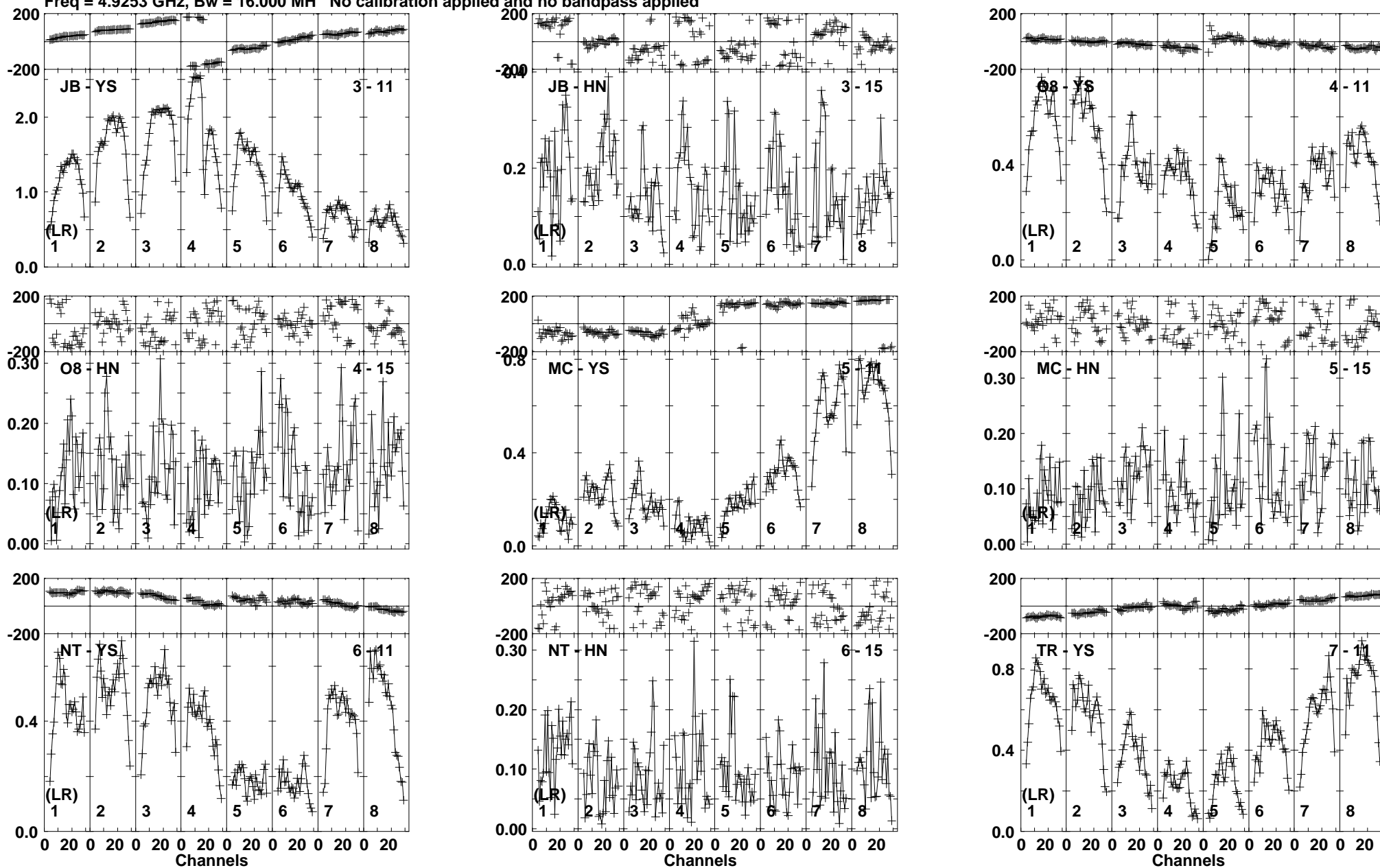
Lower frame: Milli Ampl Jy Top frame: Phas deg Vector averaged cross-power spectrum Baseline: JB (03) - YS (11) Timerange: 01/02:25:52 to 01/02:29:58
