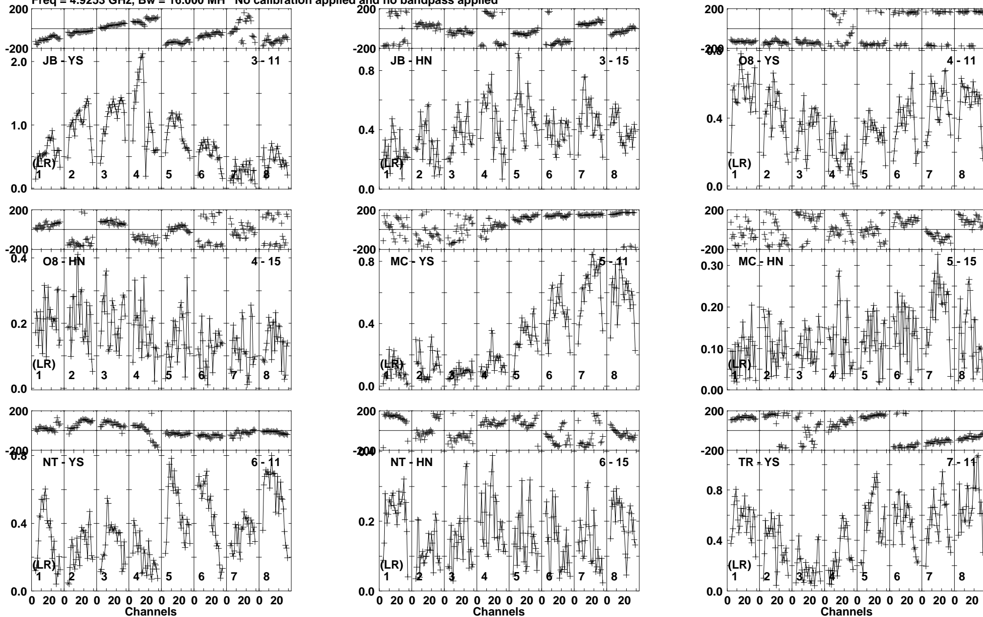
Lower frame: Milli Ampl Jy Top frame: Phas deg Vector averaged cross-power spectrum Baseline: JB (03) - YS (11) Timerange: 01/02:09:03 to 01/02:10:47
