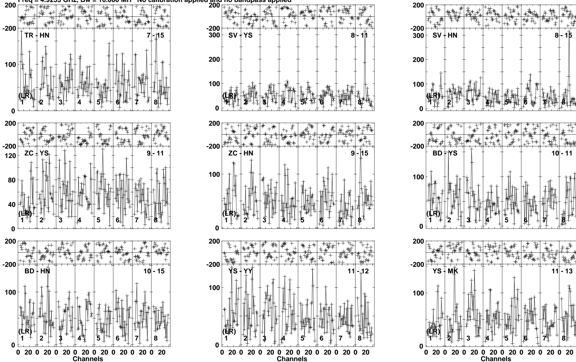
Lower frame: Micro Ampl Jy Top frame: Phas deg Vector averaged cross-power spectrum Baseline: TR (07) - HN (15) Timerange: 01/01:56:28 to 01/02:01:40
