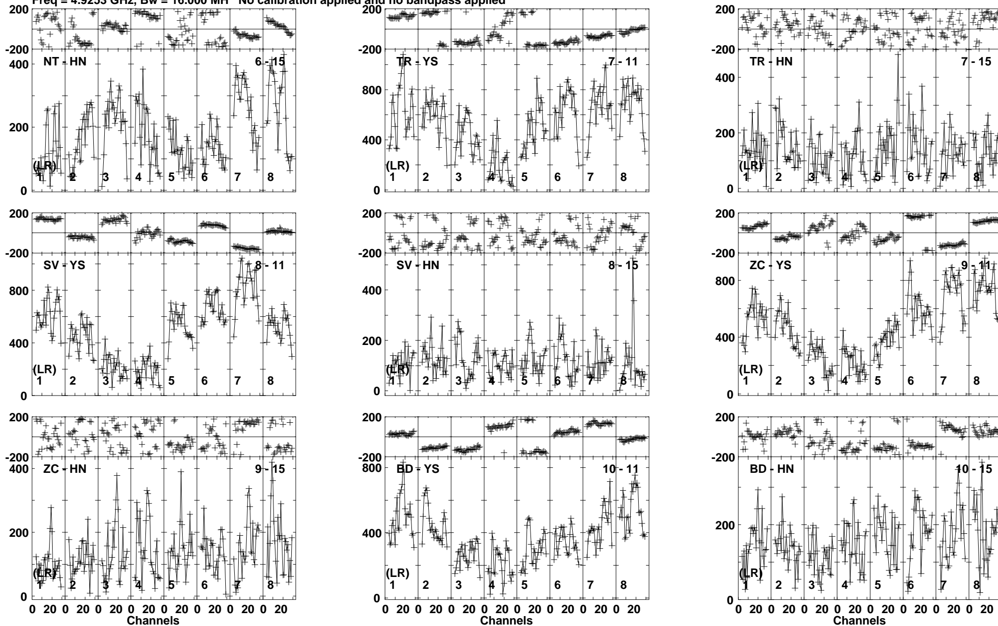
Lower frame: Micro Ampl Jy Top frame: Phas deg Vector averaged cross-power spectrum Baseline: NT (06) - HN (15) Timerange: 00/22:03:59 to 00/22:05:42
