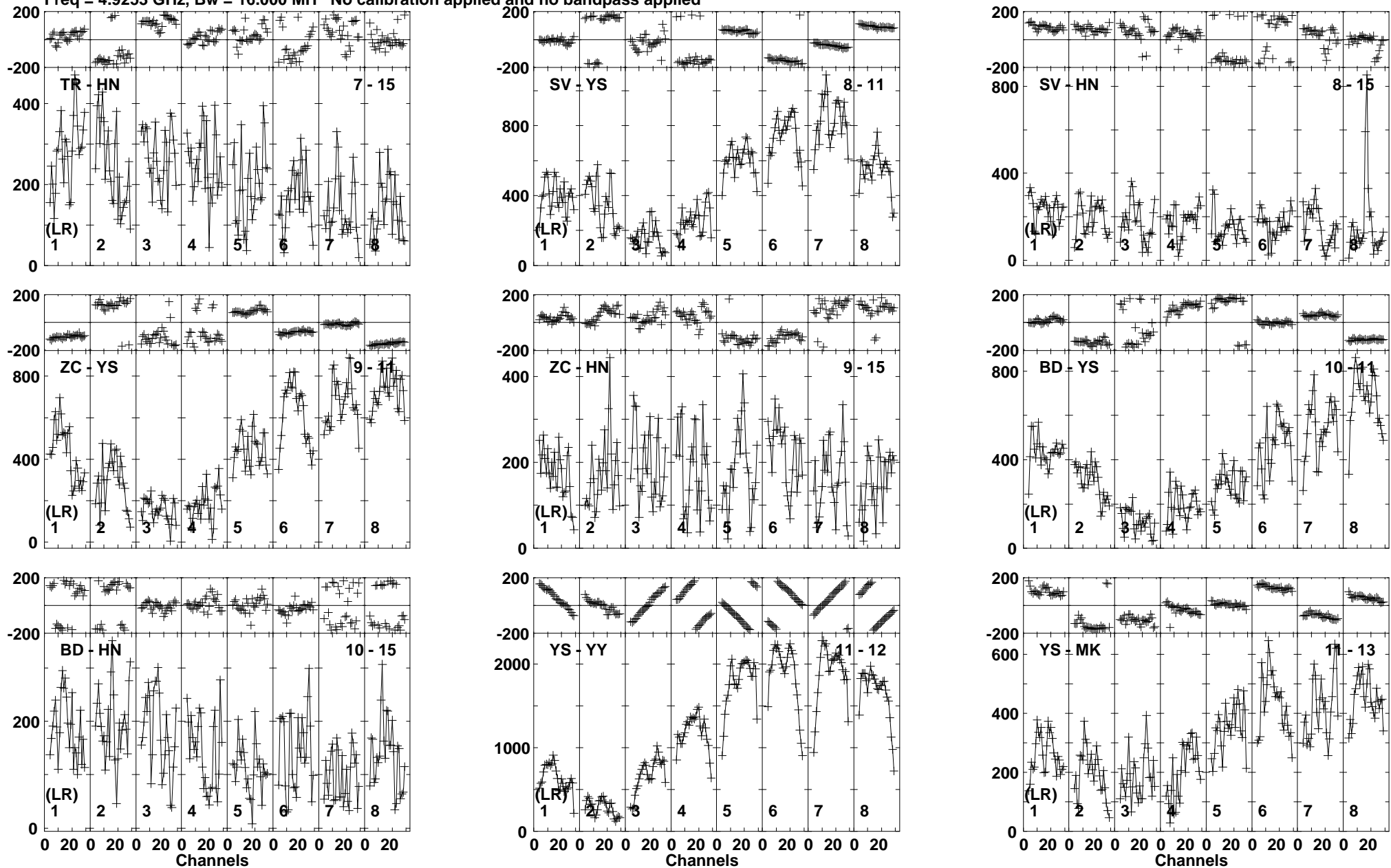
Lower frame: Micro Ampl Jy Top frame: Phas deg Vector averaged cross-power spectrum Baseline: TR (07) - HN (15) Timerange: 01/01:25:48 to 01/01:27:32
