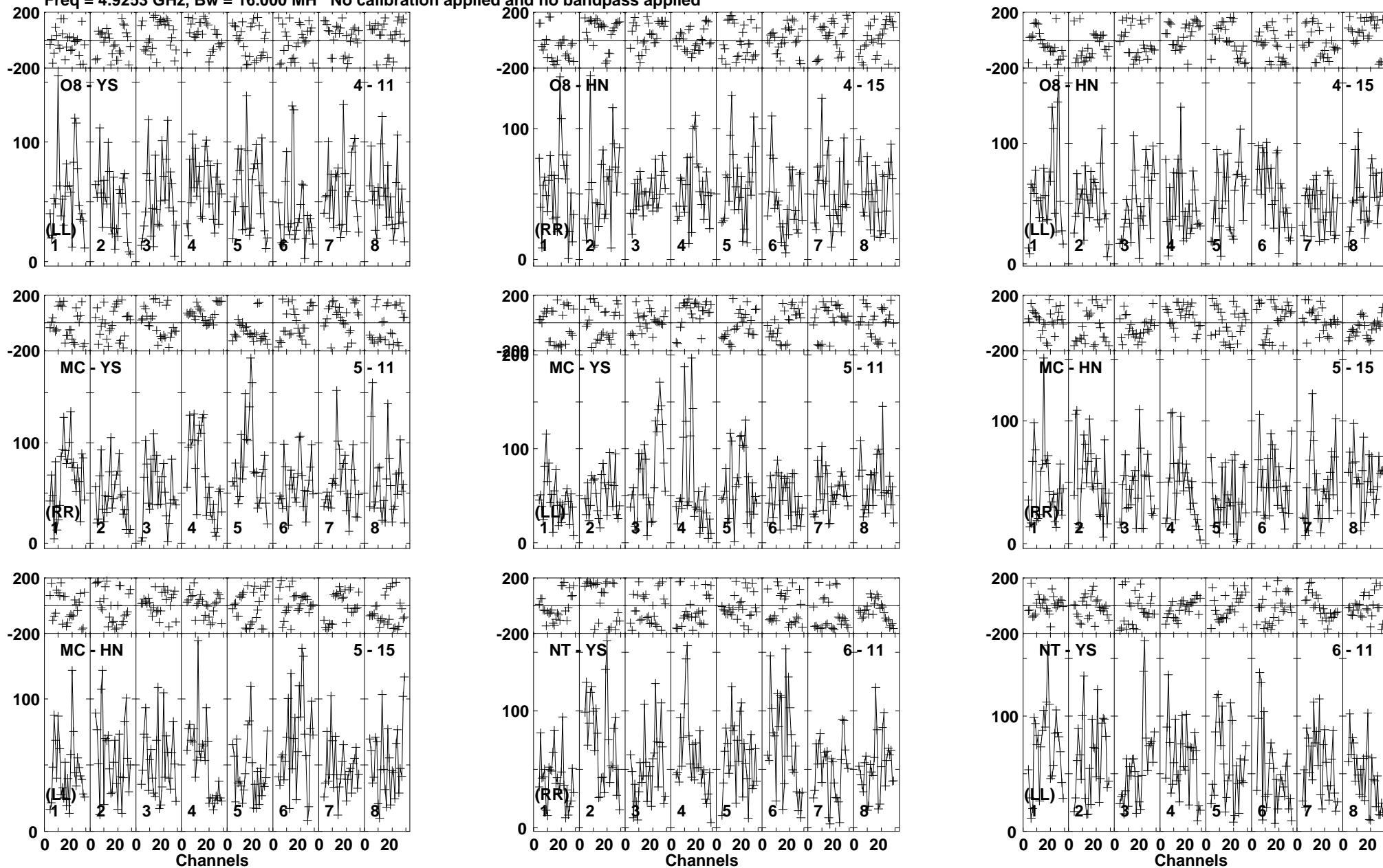
Lower frame: Micro Ampl Jy Top frame: Phas deg Vector averaged cross-power spectrum Baseline: O8 (04) - YS (11) Timerange: 00/21:08:09 to 00/21:13:21
