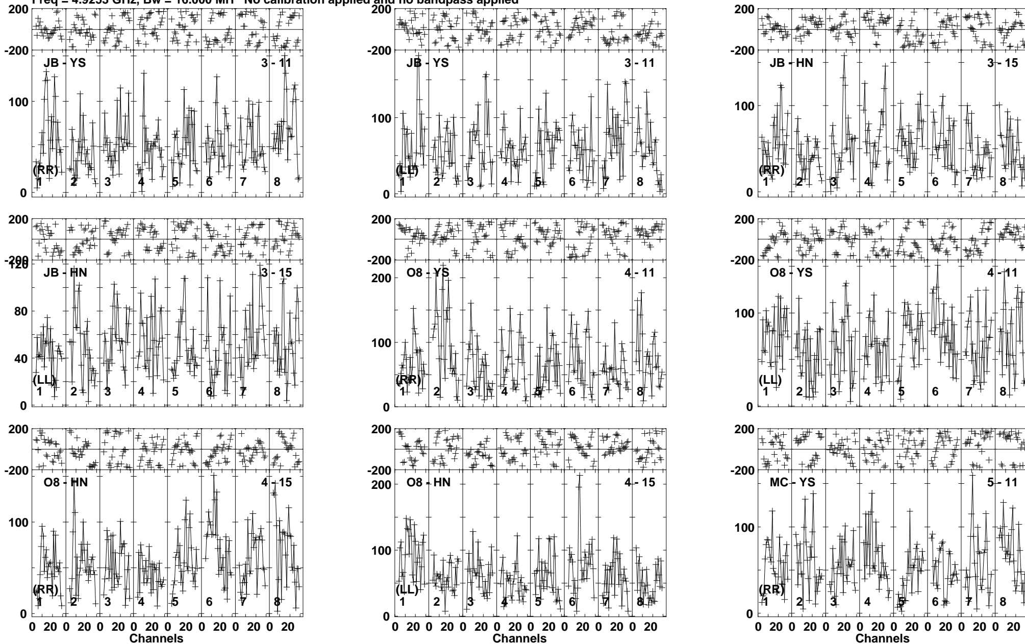
Lower frame: Micro Ampl Jy Top frame: Phas deg Vector averaged cross-power spectrum Baseline: JB (03) - YS (11) Timerange: 01/01:34:53 to 01/01:40:07
