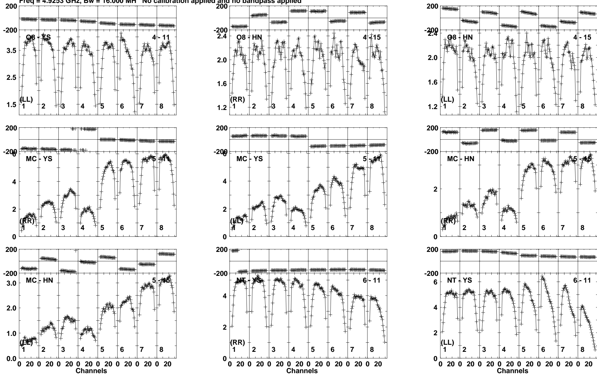
Lower frame: Milli Ampl Jy Top frame: Phas deg Vector averaged cross-power spectrum Baseline: O8 (04) - YS (11) Timerange: 00/22:47:13 to 00/22:48:57
