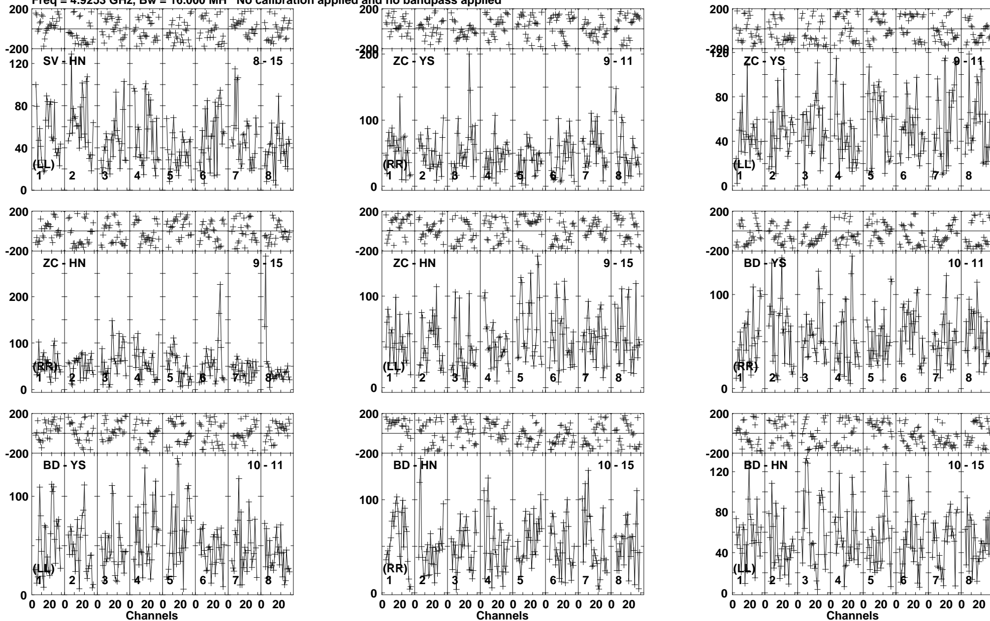
Lower frame: Micro Ampl Jy Top frame: Phas deg Vector averaged cross-power spectrum Baseline: SV (08) - HN (15) Timerange: 00/22:49:03 to 00/22:54:15
