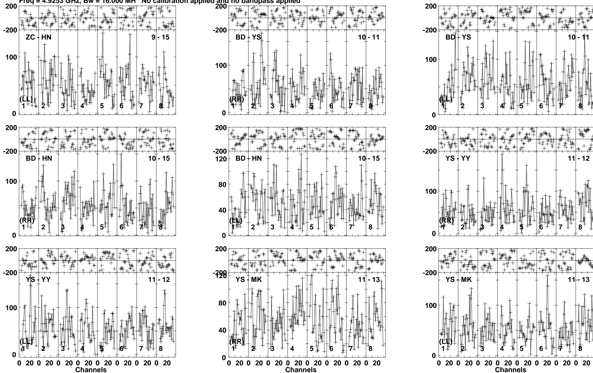
Lower frame: Micro Ampl Jy Top frame: Phas deg Vector averaged cross-power spectrum Baseline: ZC (09) - HN (15) Timerange: 01/01:27:38 to 01/01:32:50
