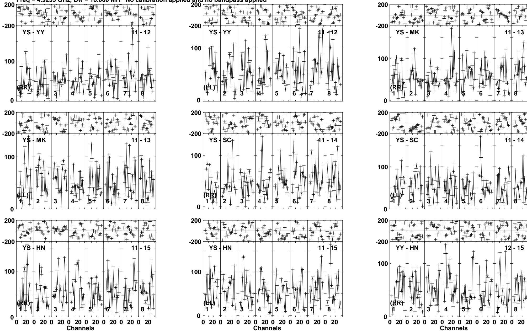
Lower frame: Micro Ampl Jy Top frame: Phas deg Vector averaged cross-power spectrum Baseline: YS (11) - YY (12) Timerange: 00/21:58:38 to 00/22:03:52
