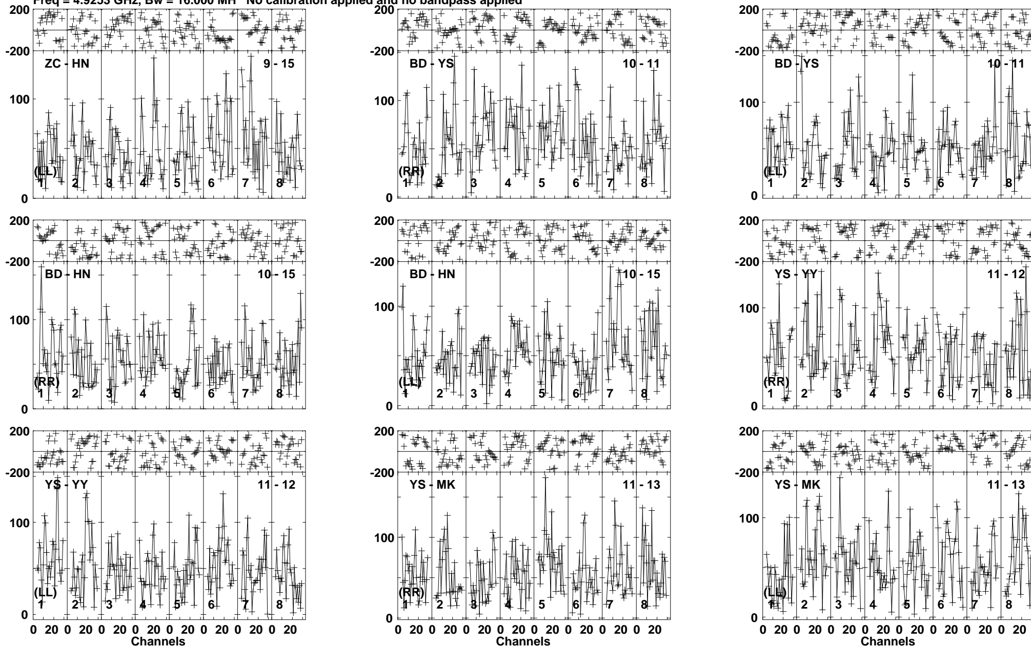
Lower frame: Micro Ampl Jy Top frame: Phas deg Vector averaged cross-power spectrum Baseline: ZC (09) - HN (15) Timerange: 01/01:42:03 to 01/01:47:15
