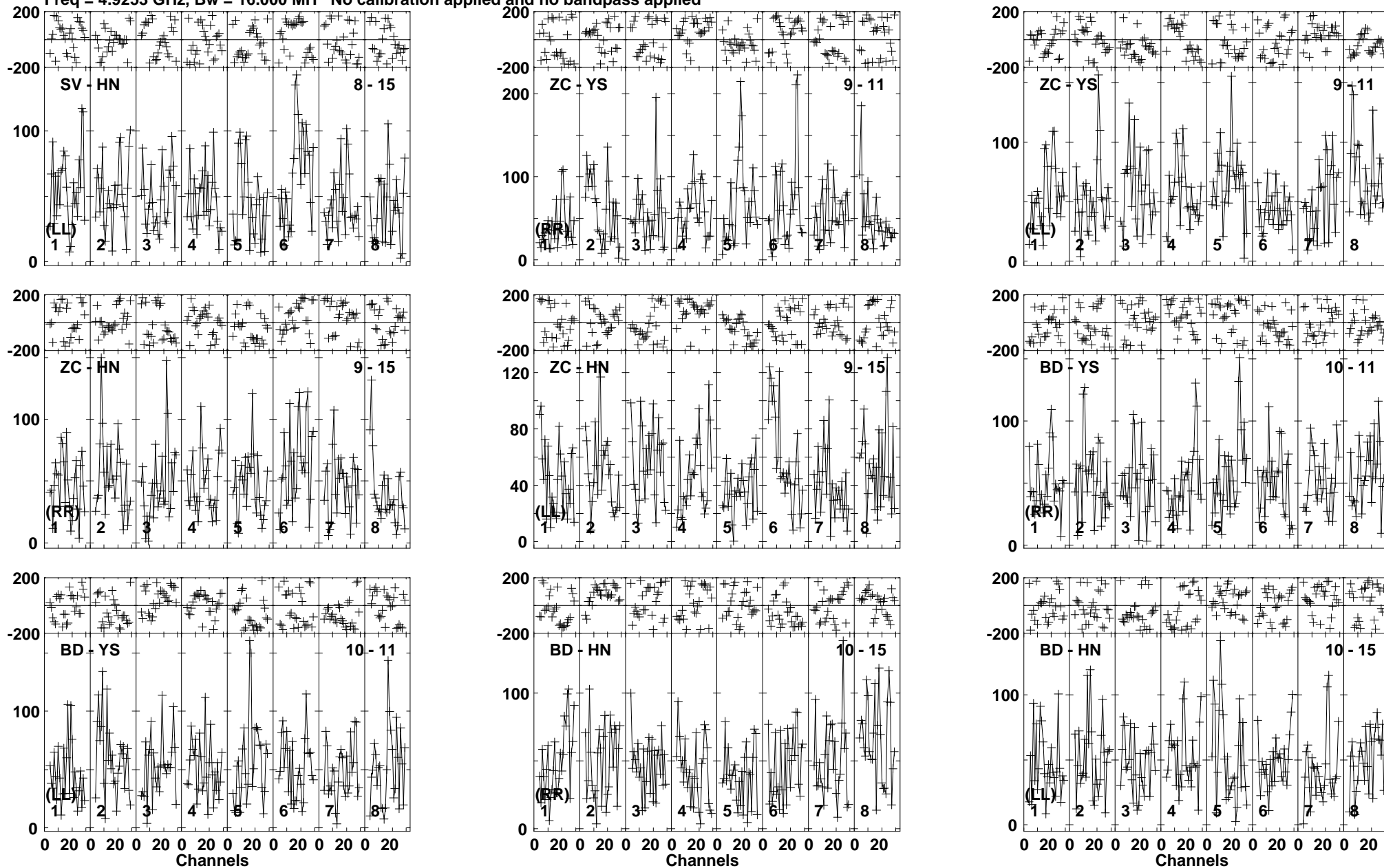
Lower frame: Micro Ampl Jy Top frame: Phas deg Vector averaged cross-power spectrum Baseline: SV (08) - HN (15) Timerange: 00/21:15:23 to 00/21:20:37
