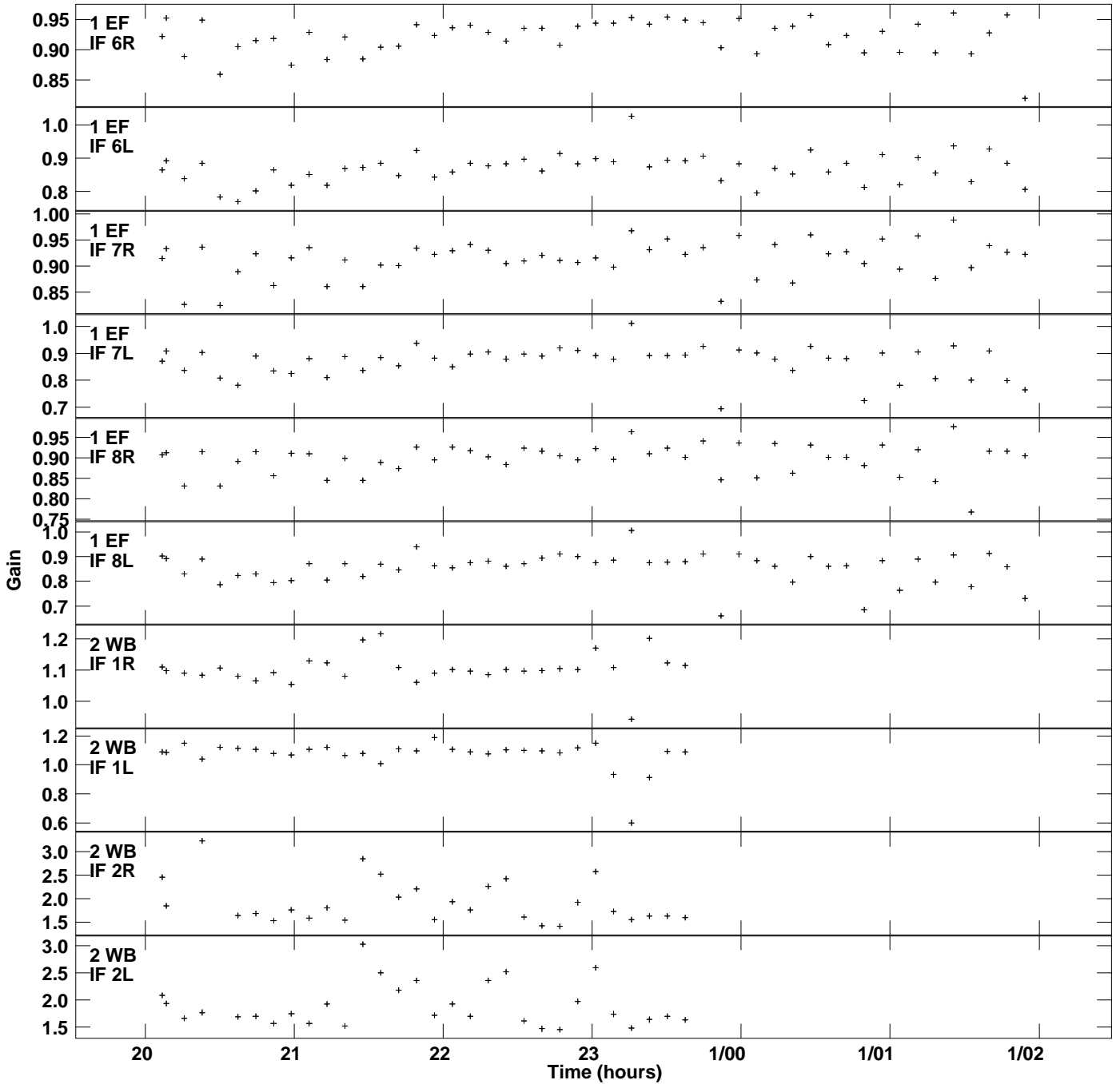
Plot file version 2 created 14-APR-2016 21:03:28 Gain amp vs UTC time for J1128+5925.MULTI.1 SN 2 Rpol & Lpol IF 1 - 8
