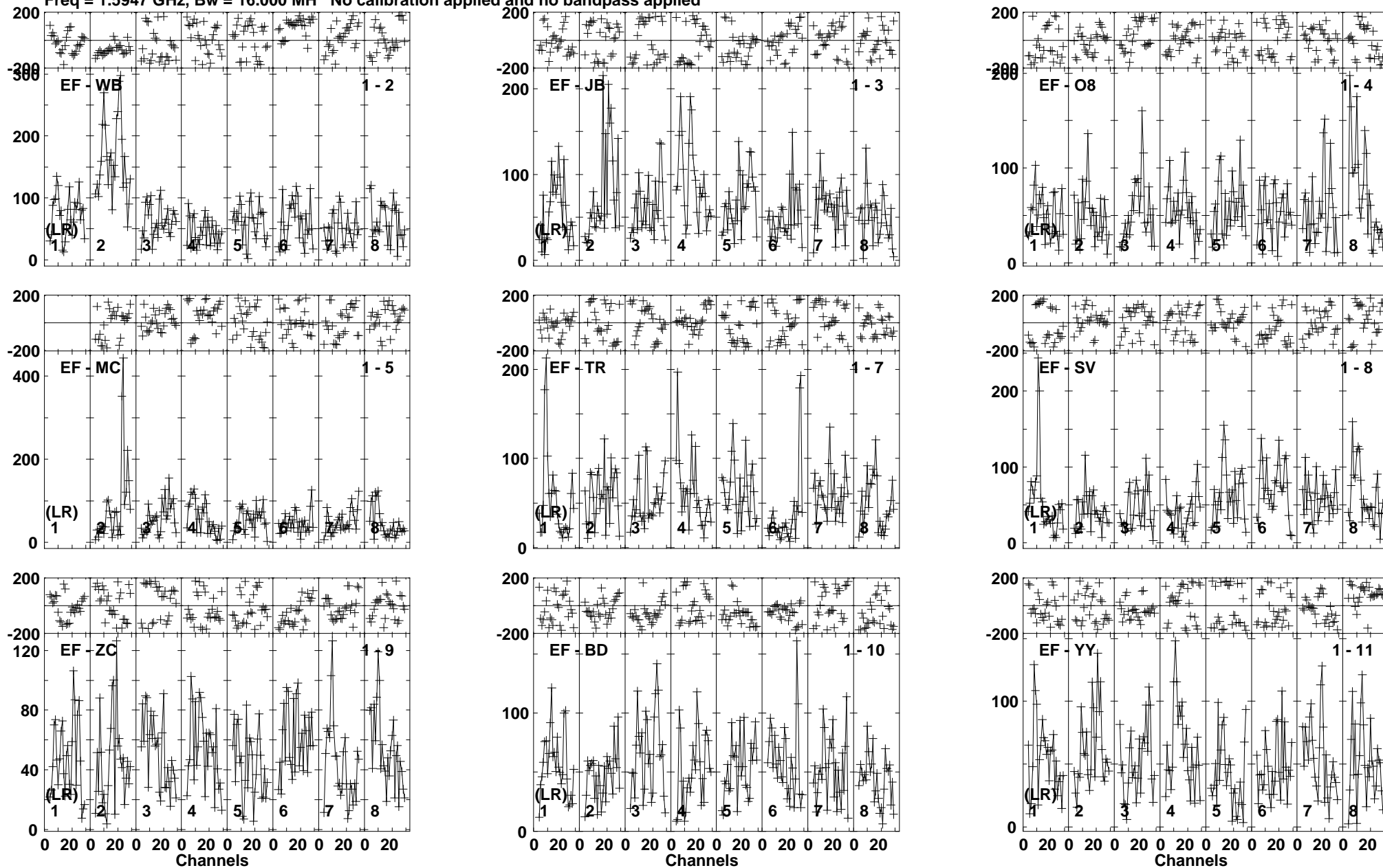
Lower frame: Micro Ampl Jy Top frame: Phas deg Vector averaged cross-power spectrum Baseline: EF (01) - WB (02) Timerange: 00/21:14:13 to 00/21:19:27
