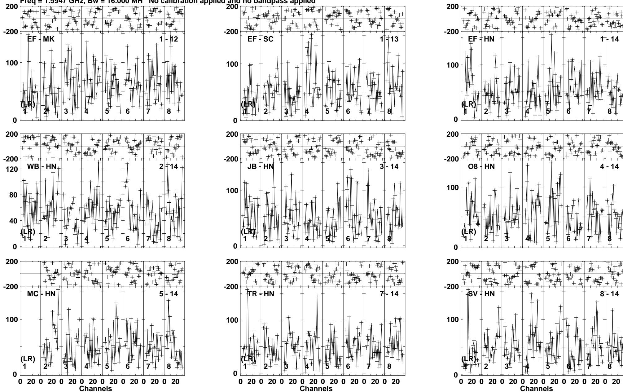
Lower frame: Micro Ampl Jy Top frame: Phas deg Vector averaged cross-power spectrum Baseline: EF (01) - MK (12) Timerange: 00/23:31:10 to 00/23:36:20
