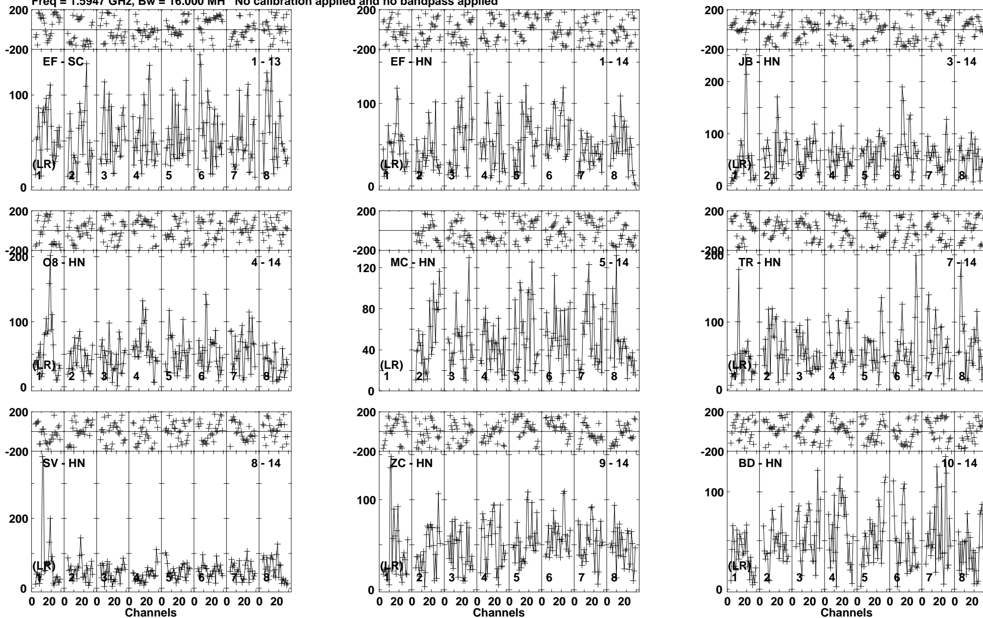
Lower frame: Micro Ampl Jy Top frame: Phas deg Vector averaged cross-power spectrum Baseline: EF (01) - SC (13) Timerange: 01/00:50:28 to 01/00:55:42
