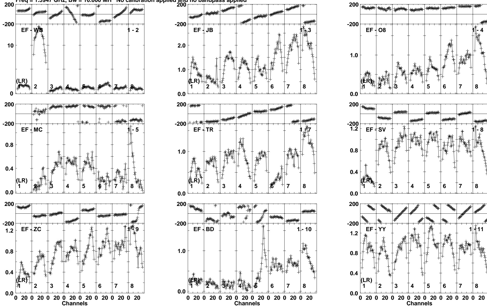
Lower frame: Milli Ampl Jy Top frame: Phas deg Vector averaged cross-power spectrum Baseline: EF (01) - WB (02) Timerange: 00/20:05:17 to 00/20:09:12
