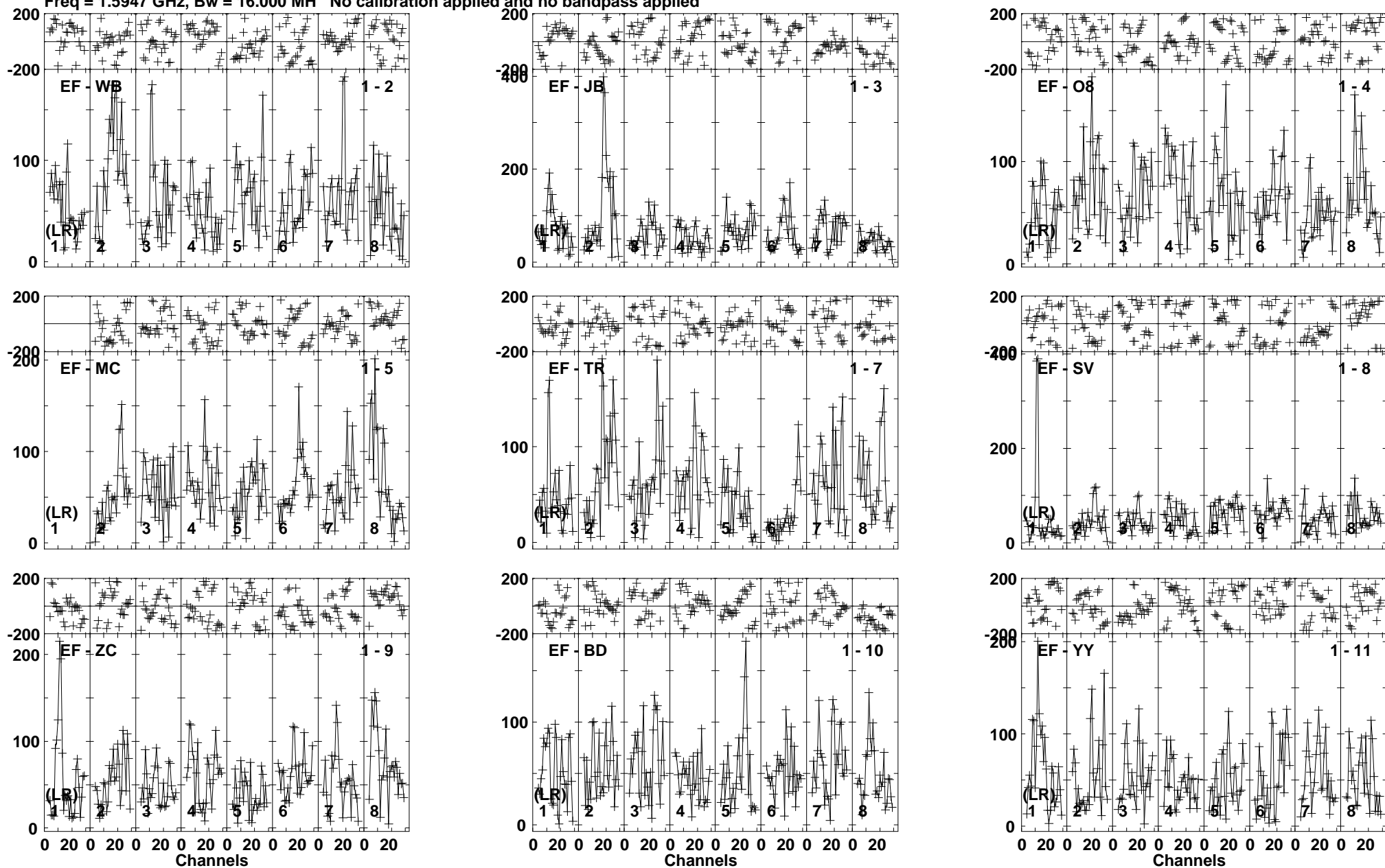
Lower frame: Micro Ampl Jy Top frame: Phas deg Vector averaged cross-power spectrum Baseline: EF (01) - WB (02) Timerange: 00/22:11:53 to 00/22:17:07
