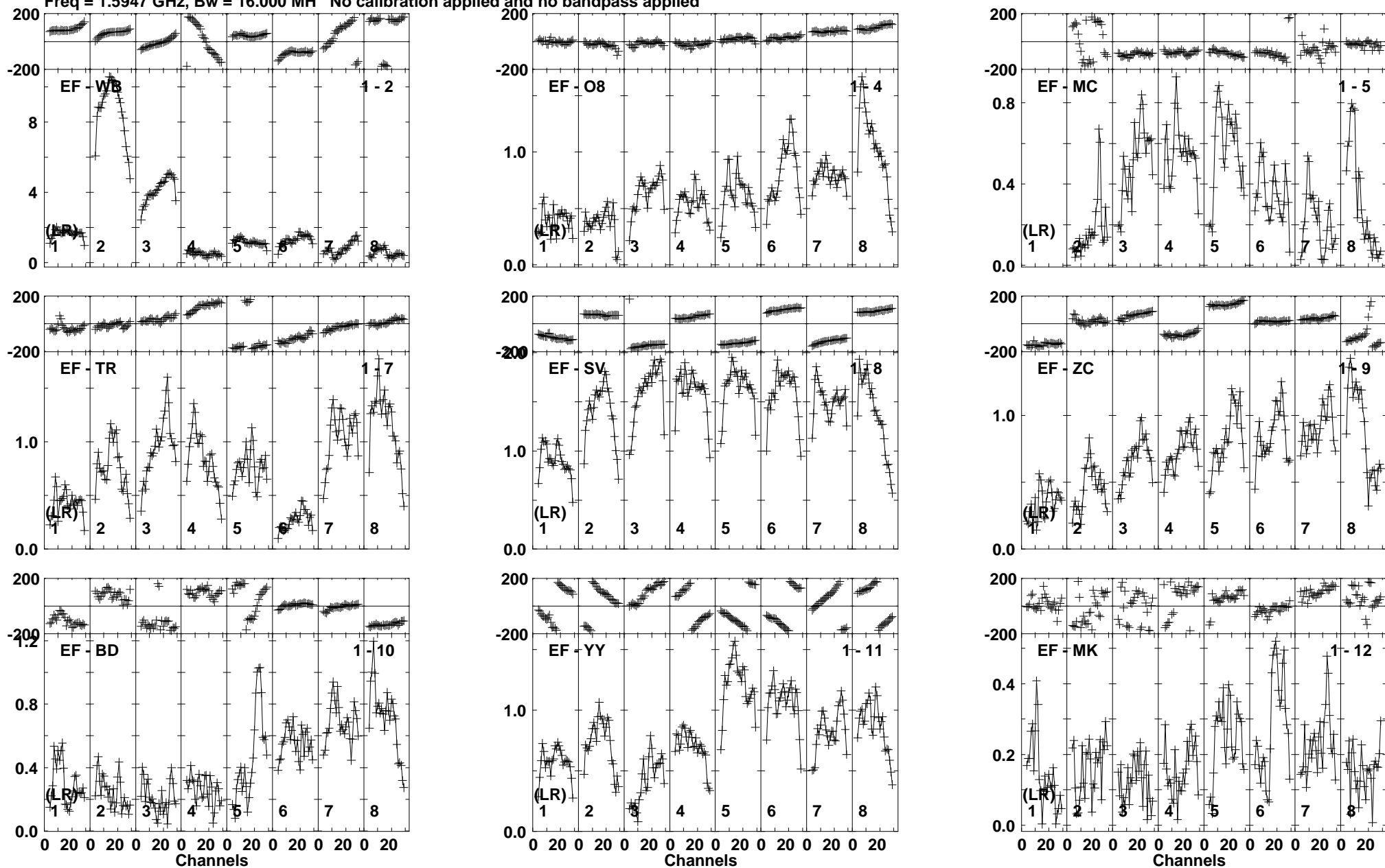
Lower frame: Milli Ampl Jy Top frame: Phas deg Vector averaged cross-power spectrum Baseline: EF (01) - WB (02) Timerange: 00/22:24:23 to 00/22:26:13
