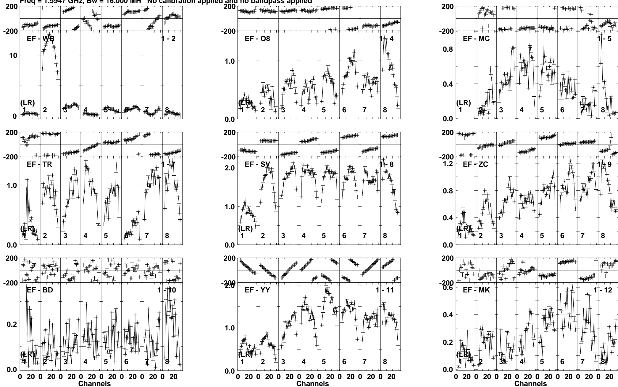
Lower frame: Milli Ampl Jy Top frame: Phas deg Vector averaged cross-power spectrum Baseline: EF (01) - WB (02) Timerange: 00/23:22:03 to 00/23:23:53
