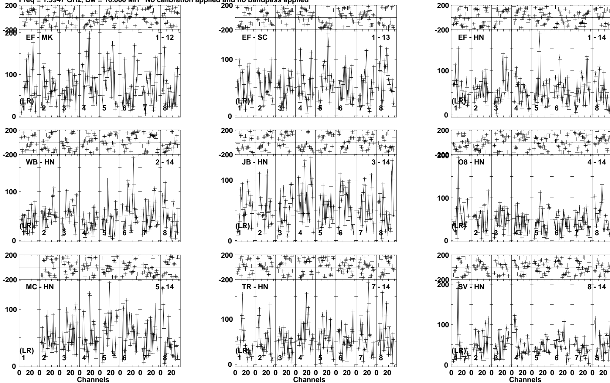
Lower frame: Micro Ampl Jy Top frame: Phas deg Vector averaged cross-power spectrum Baseline: EF (01) - MK (12) Timerange: 00/23:23:58 to 00/23:29:12
