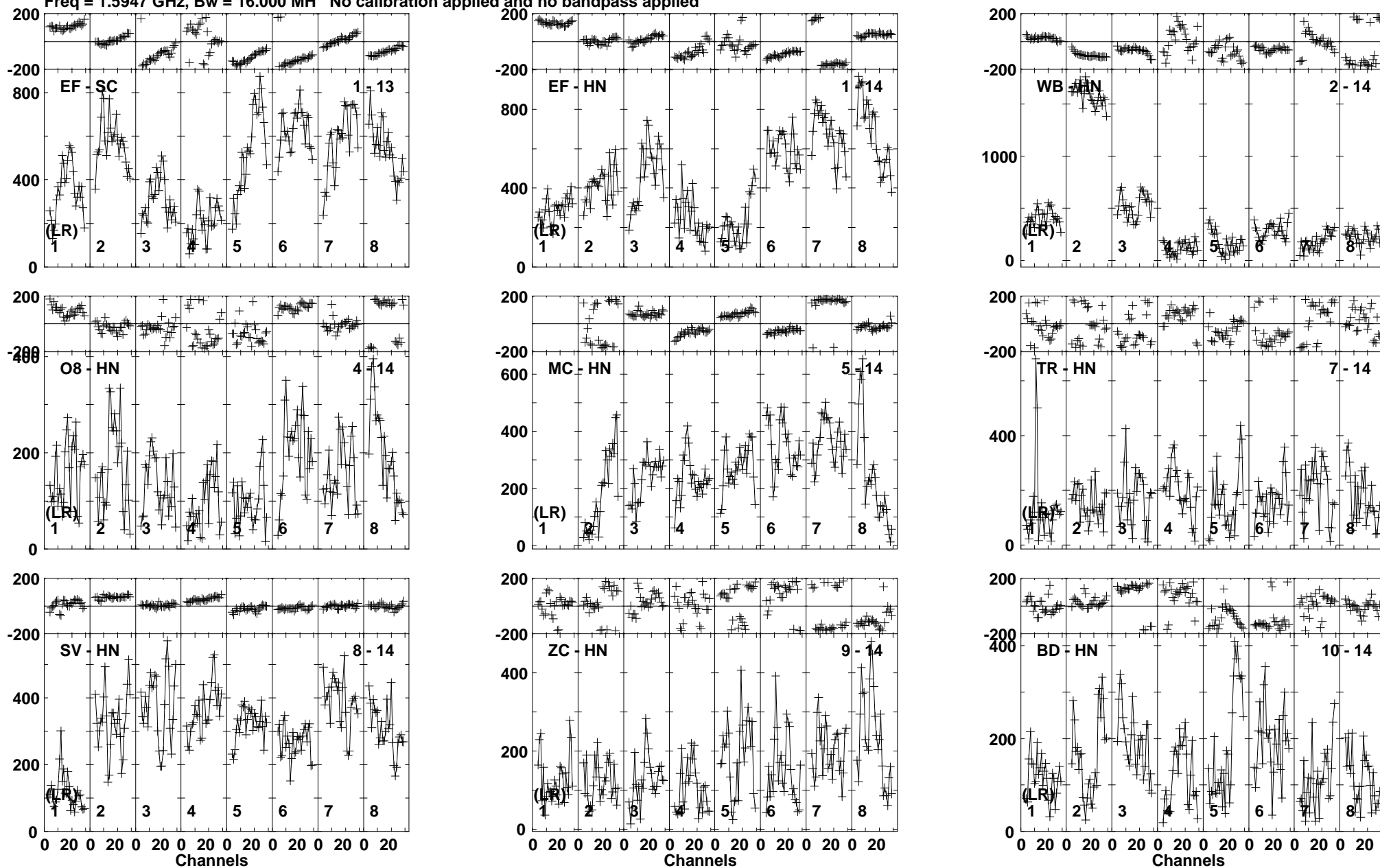
Lower frame: Micro Ampl Jy Top frame: Phas deg Vector averaged cross-power spectrum Baseline: EF (01) - SC (13) Timerange: 00/21:41:09 to 00/21:42:58
