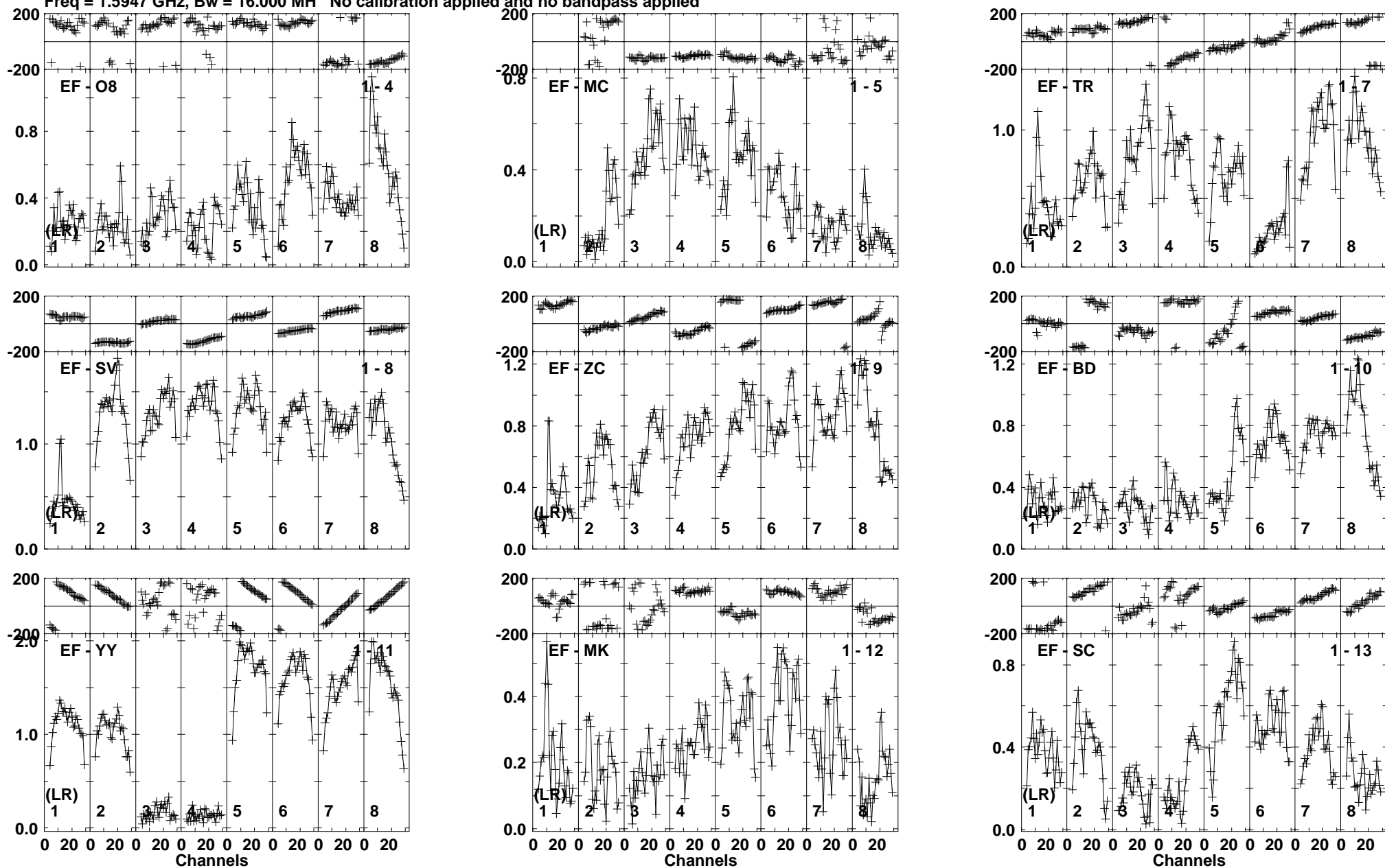
Lower frame: Milli Ampl Jy Top frame: Phas deg Vector averaged cross-power spectrum Baseline: EF (01) - O8 (04) Timerange: 01/01:46:14 to 01/01:48:03
