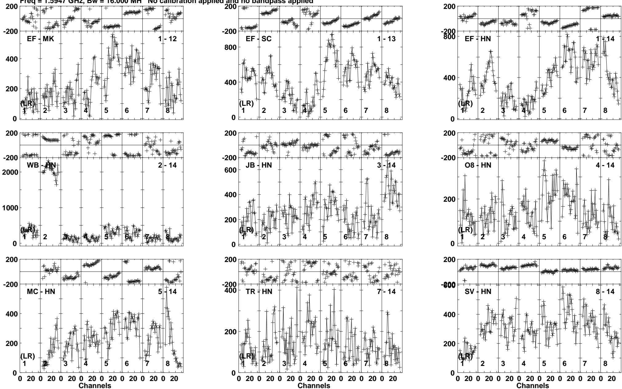
Lower frame: Micro Ampl Jy Top frame: Phas deg Vector averaged cross-power spectrum Baseline: EF (01) - MK (12) Timerange: 00/23:29:20 to 00/23:31:02
