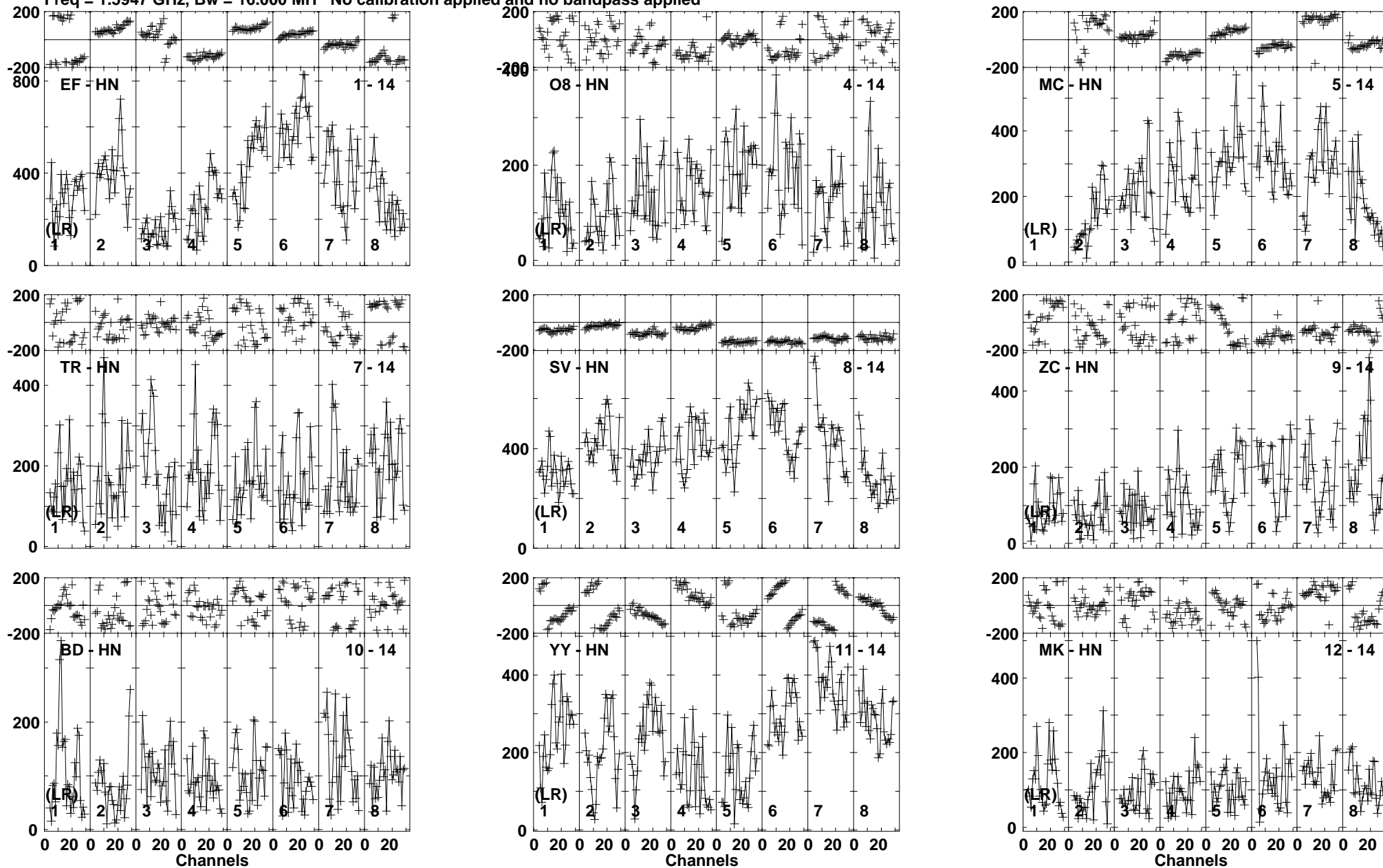
Lower frame: Micro Ampl Jy Top frame: Phas deg Vector averaged cross-power spectrum Baseline: EF (01) - HN (14) Timerange: 01/00:19:43 to 01/00:21:33
