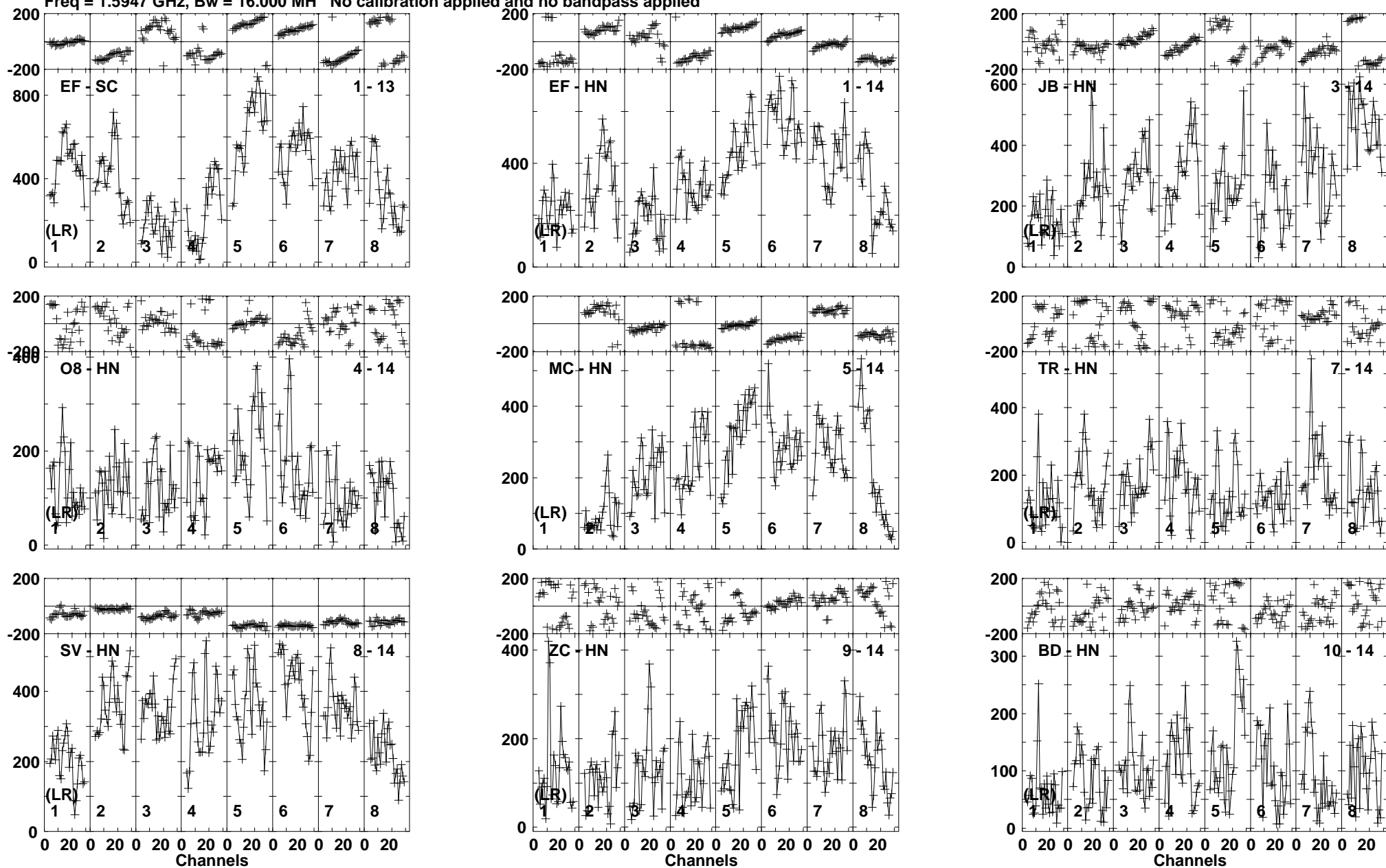
Lower frame: Micro Ampl Jy Top frame: Phas deg Vector averaged cross-power spectrum Baseline: EF (01) - SC (13) Timerange: 01/00:27:01 to 01/00:28:42
