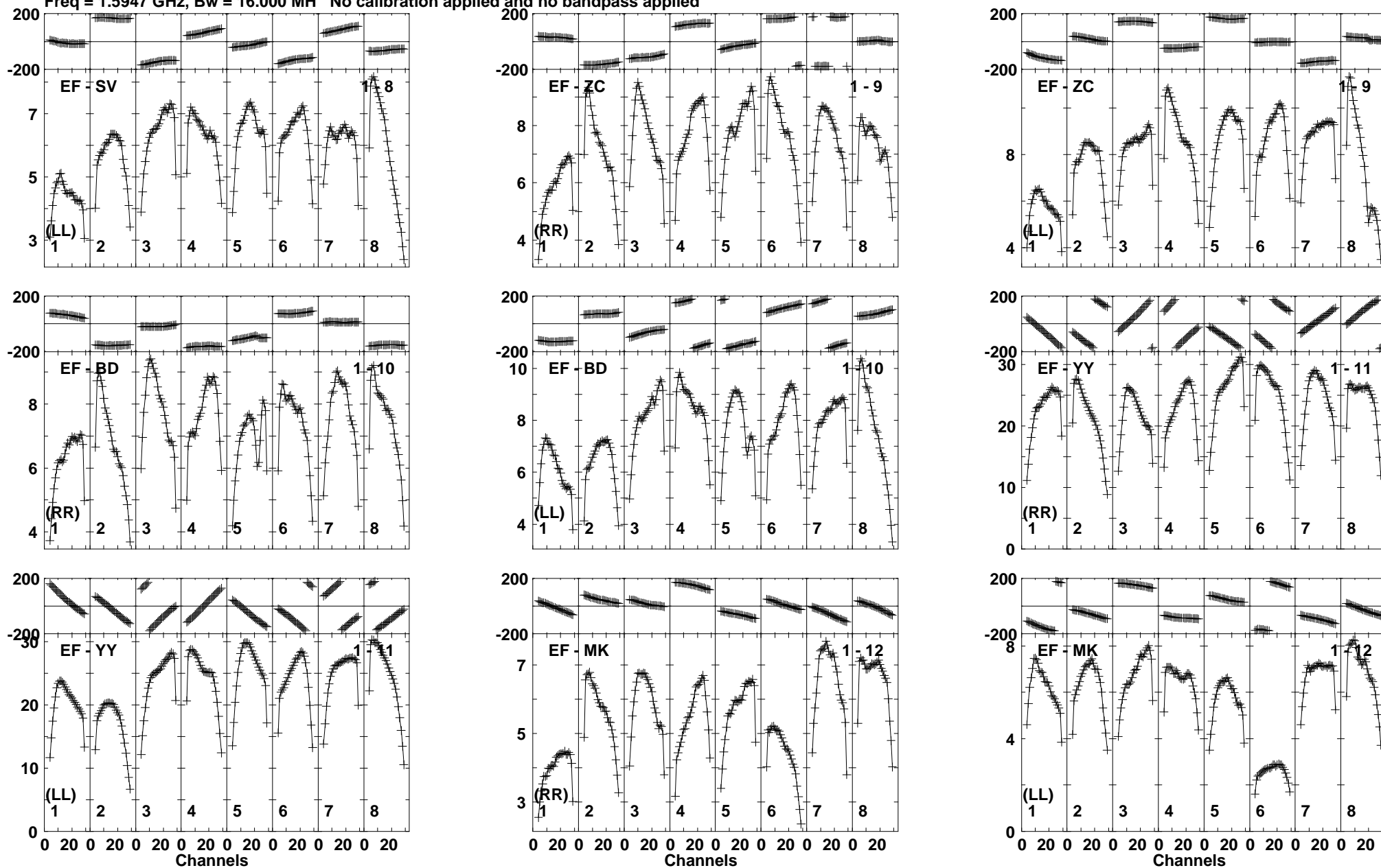
Lower frame: Milli Ampl Jy Top frame: Phas deg Vector averaged cross-power spectrum Baseline: EF (01) - SV (08) Timerange: 01/01:10:16 to 01/01:11:57
