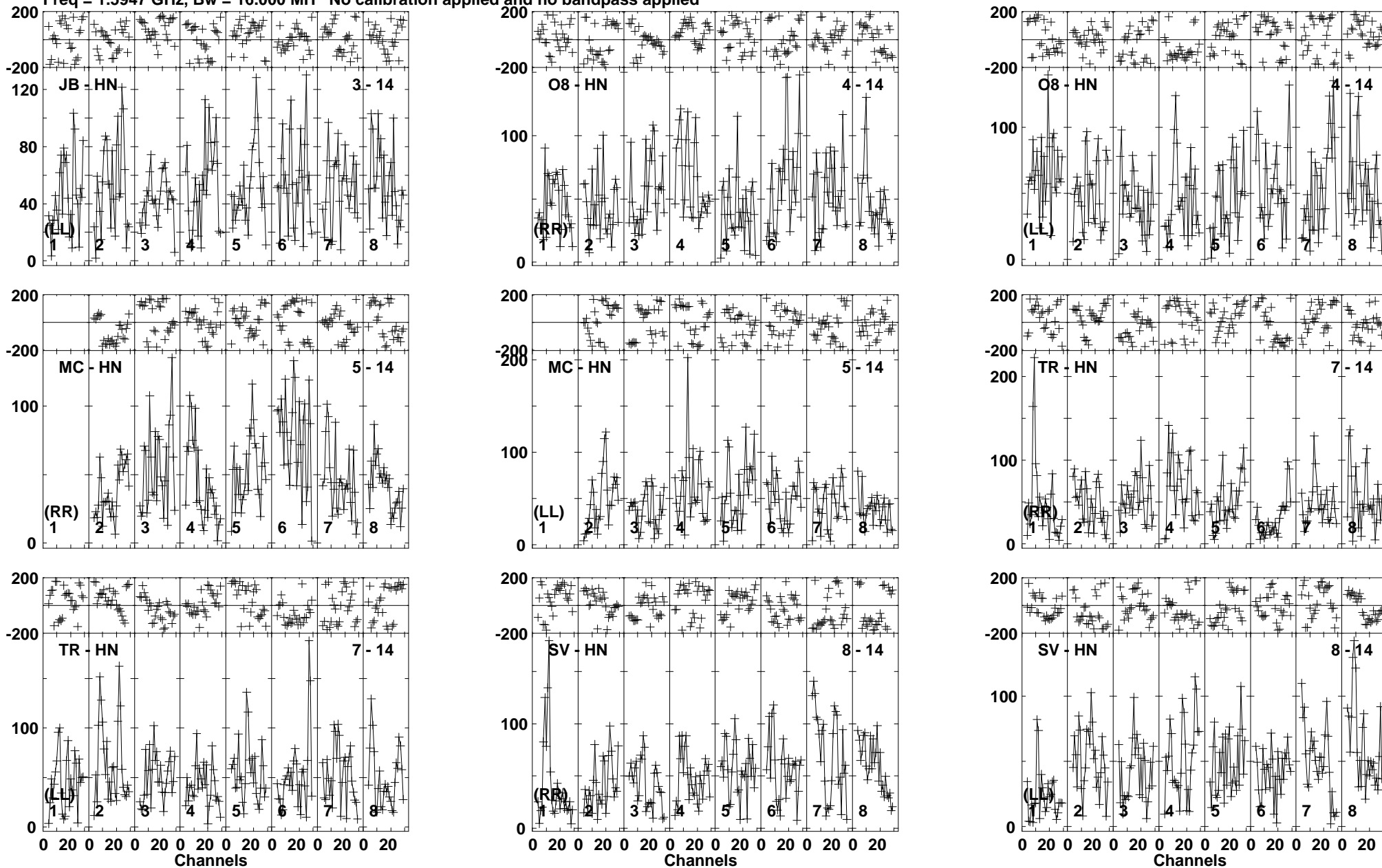
Lower frame: Micro Ampl Jy Top frame: Phas deg Vector averaged cross-power spectrum Baseline: JB (03) - HN (14) Timerange: 00/21:14:13 to 00/21:19:27
