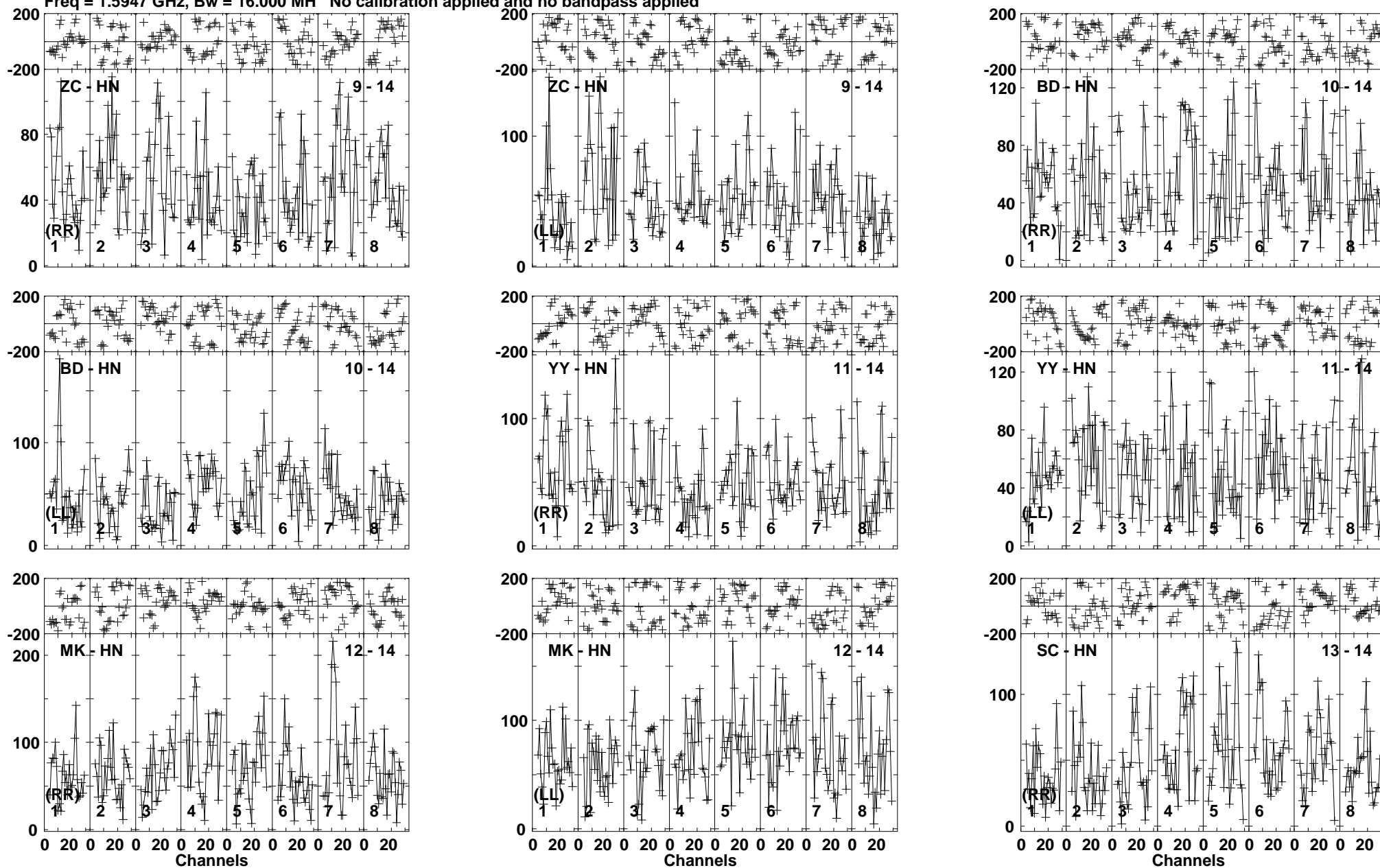
Lower frame: Micro Ampl Jy Top frame: Phas deg Vector averaged cross-power spectrum Baseline: ZC (09) - HN (14) Timerange: 00/23:23:58 to 00/23:29:12
