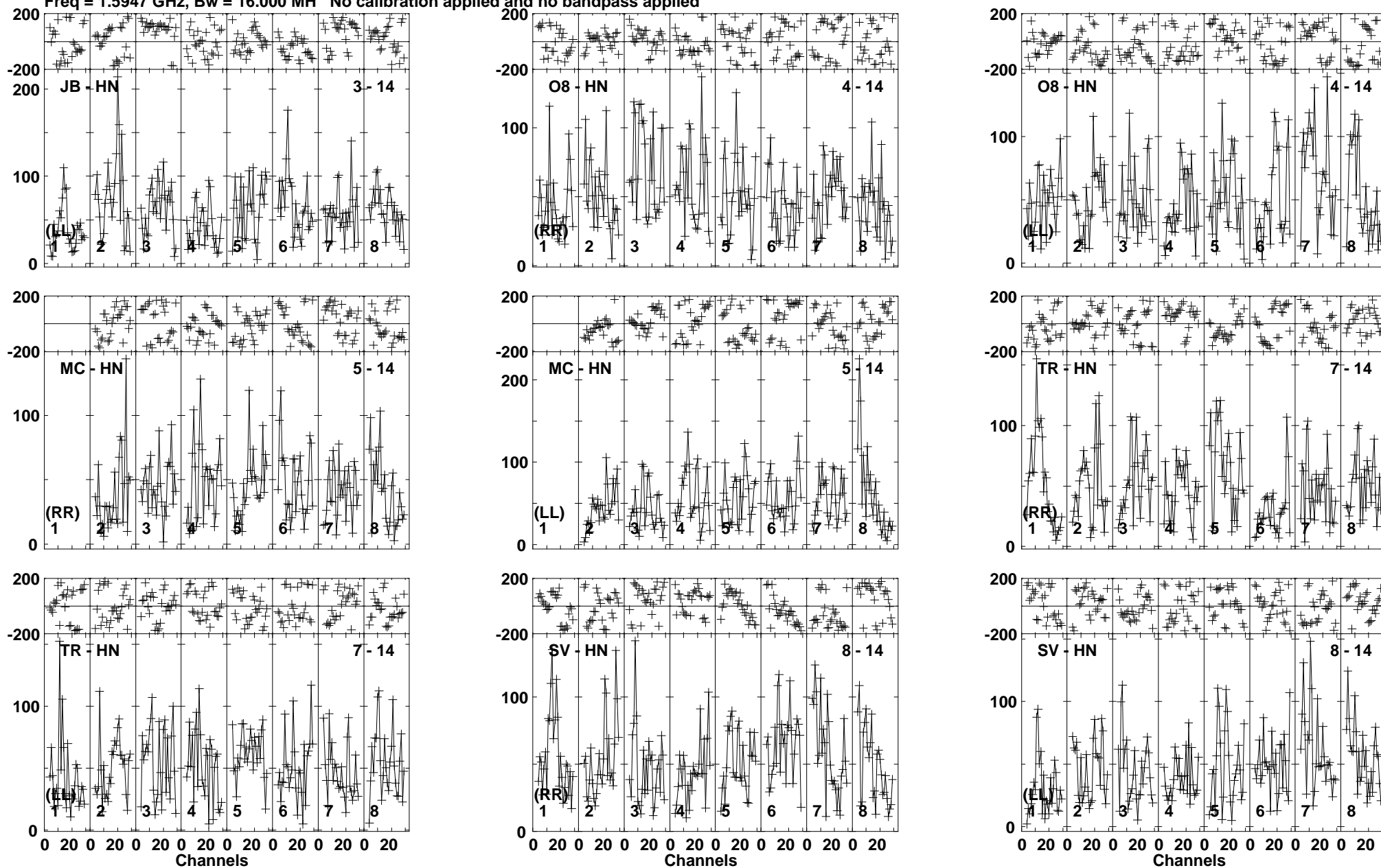
Lower frame: Micro Ampl Jy Top frame: Phas deg Vector averaged cross-power spectrum Baseline: JB (03) - HN (14) Timerange: 00/23:16:45 to 00/23:21:55
