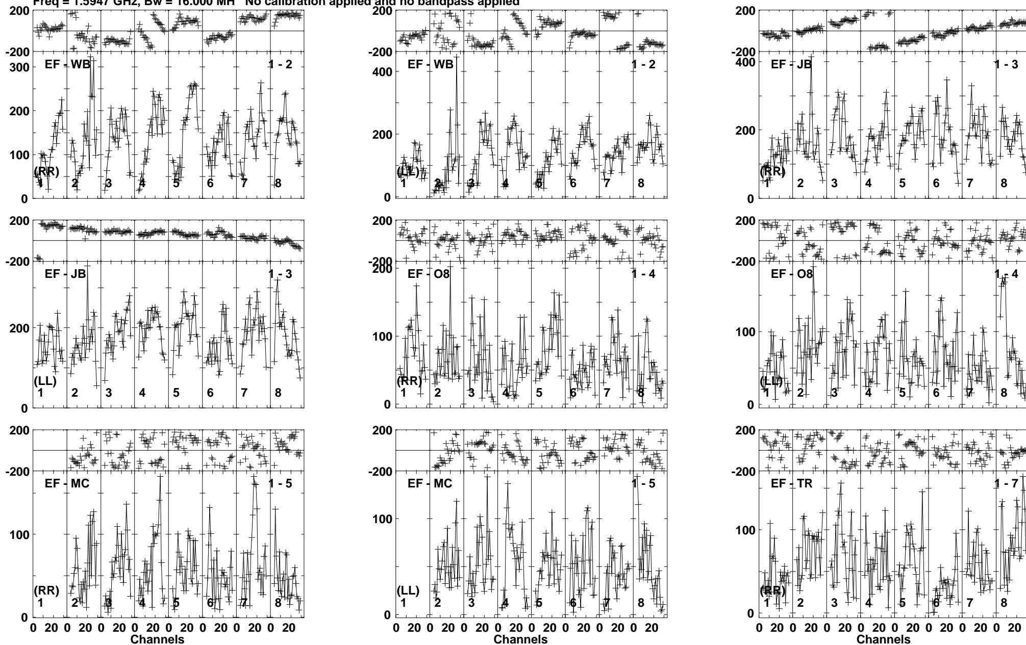
Lower frame: Micro Ampl Jy Top frame: Phas deg Vector averaged cross-power spectrum Baseline: EF (01) - WB (02) Timerange: 00/22:47:55 to 00/22:53:05
