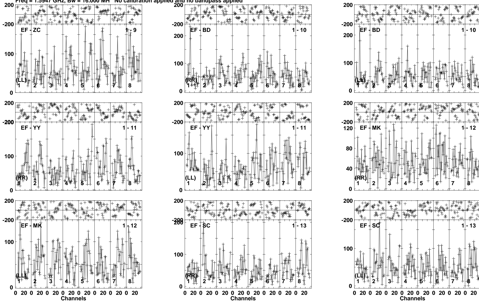
Lower frame: Micro Ampl Jy Top frame: Phas deg Vector averaged cross-power spectrum Baseline: EF (01) - ZC (09) Timerange: 01/01:48:11 to 01/01:53:23
