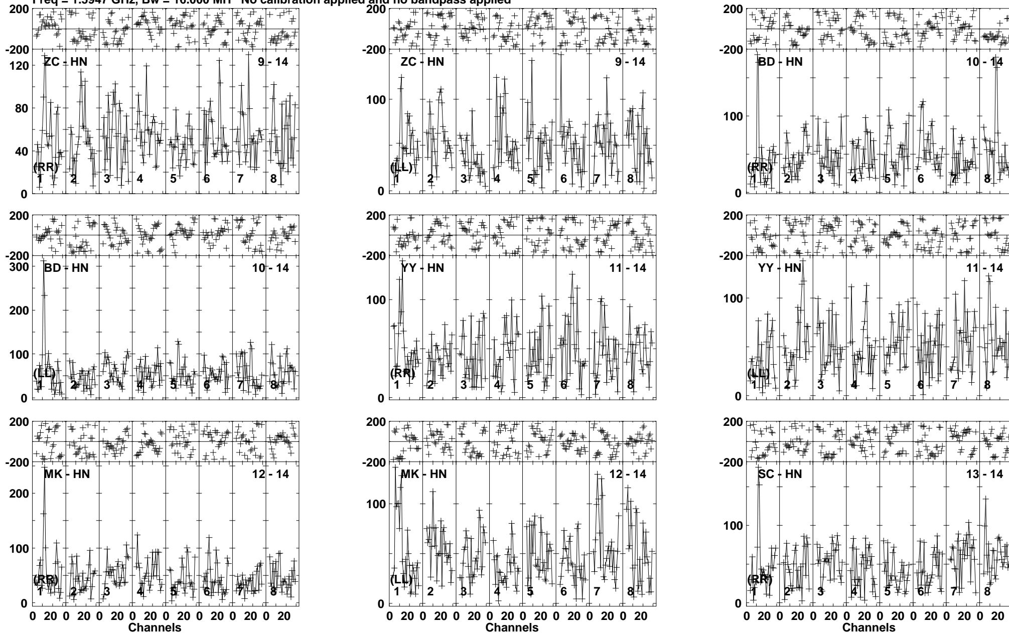
Lower frame: Micro Ampl Jy Top frame: Phas deg Vector averaged cross-power spectrum Baseline: ZC (09) - HN (14) Timerange: 00/22:55:08 to 00/23:00:22
