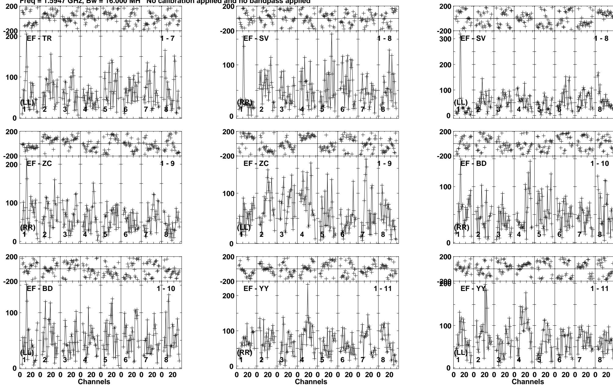
Lower frame: Micro Ampl Jy Top frame: Phas deg Vector averaged cross-power spectrum Baseline: EF (01) - TR (07) Timerange: 00/20:09:21 to 00/20:14:31
