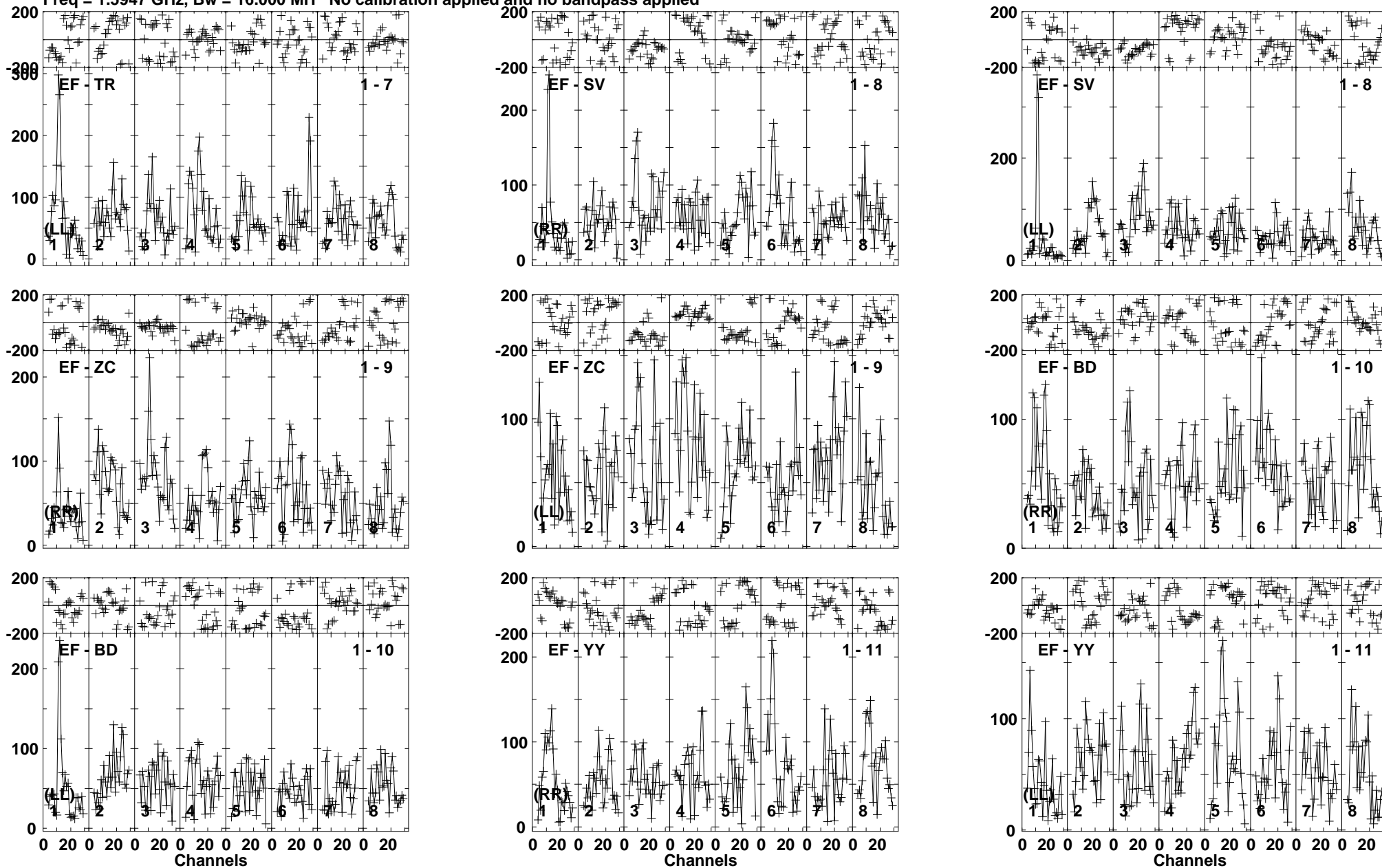
Lower frame: Micro Ampl Jy Top frame: Phas deg Vector averaged cross-power spectrum Baseline: EF (01) - TR (07) Timerange: 00/20:52:36 to 00/20:57:46
