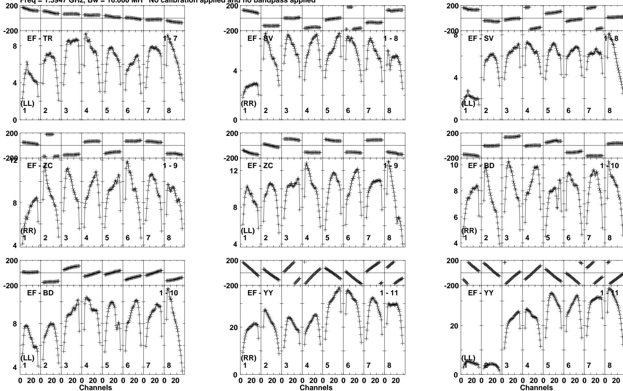
Lower frame: Milli Ampl Jy Top frame: Phas deg Vector averaged cross-power spectrum Baseline: EF (01) - TR (07) Timerange: 00:22:17:15 to 00:22:18:57
