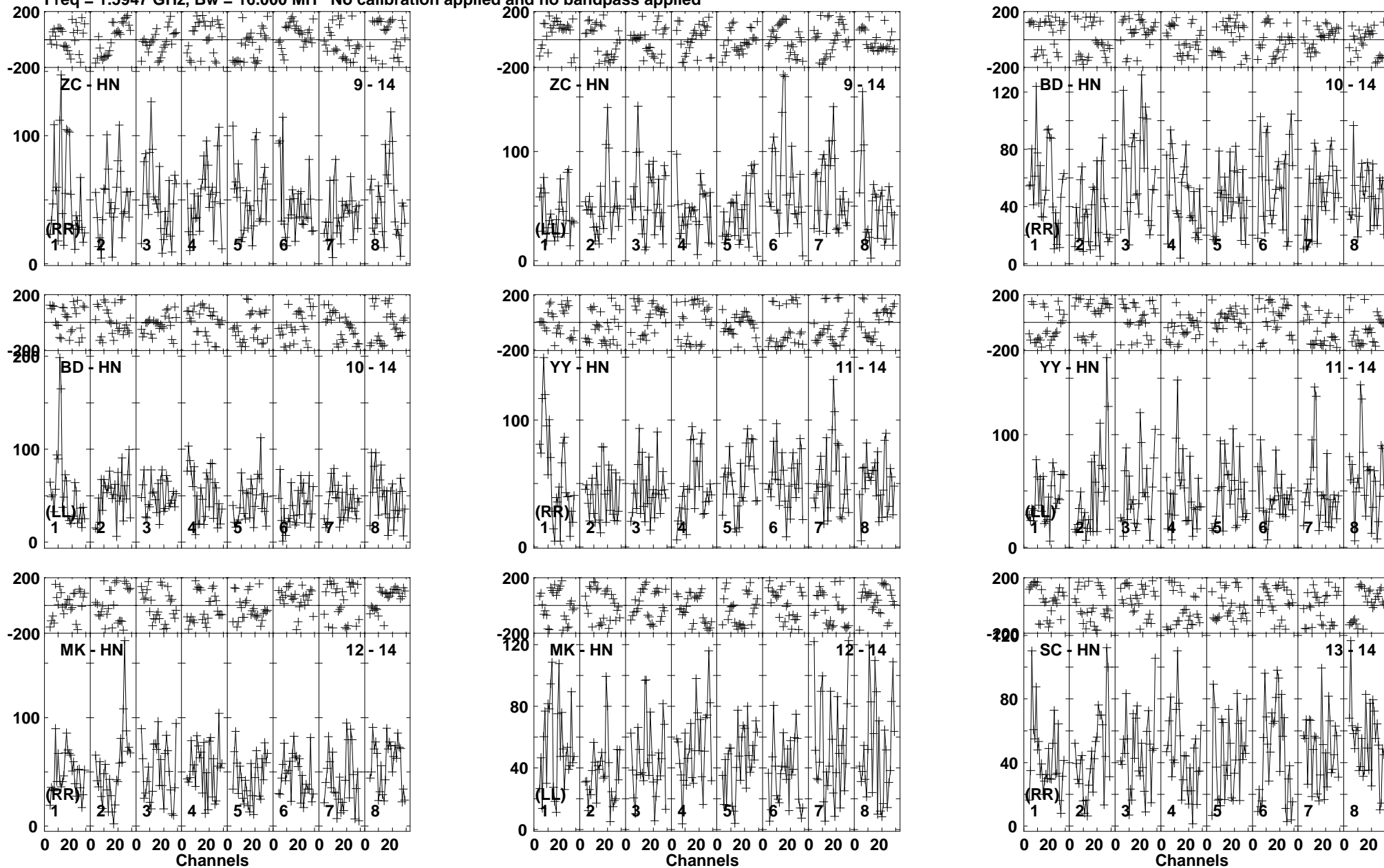
Lower frame: Micro Ampl Jy Top frame: Phas deg Vector averaged cross-power spectrum Baseline: ZC (09) - HN (14) Timerange: 00/20:30:58 to 00/20:36:12
