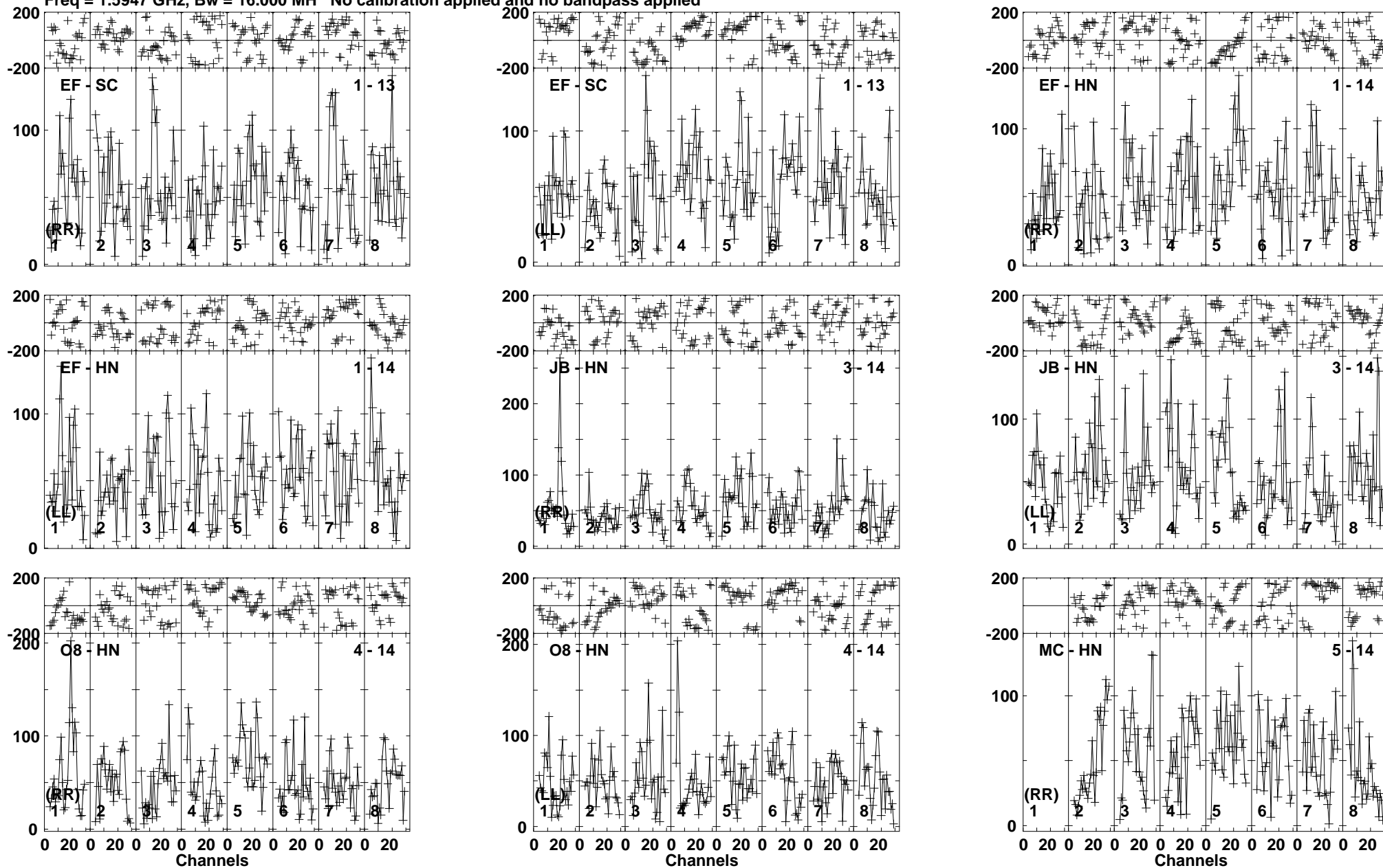
Lower frame: Micro Ampl Jy Top frame: Phas deg Vector averaged cross-power spectrum Baseline: EF (01) - SC (13) Timerange: 01/00:28:51 to 01/00:34:01
