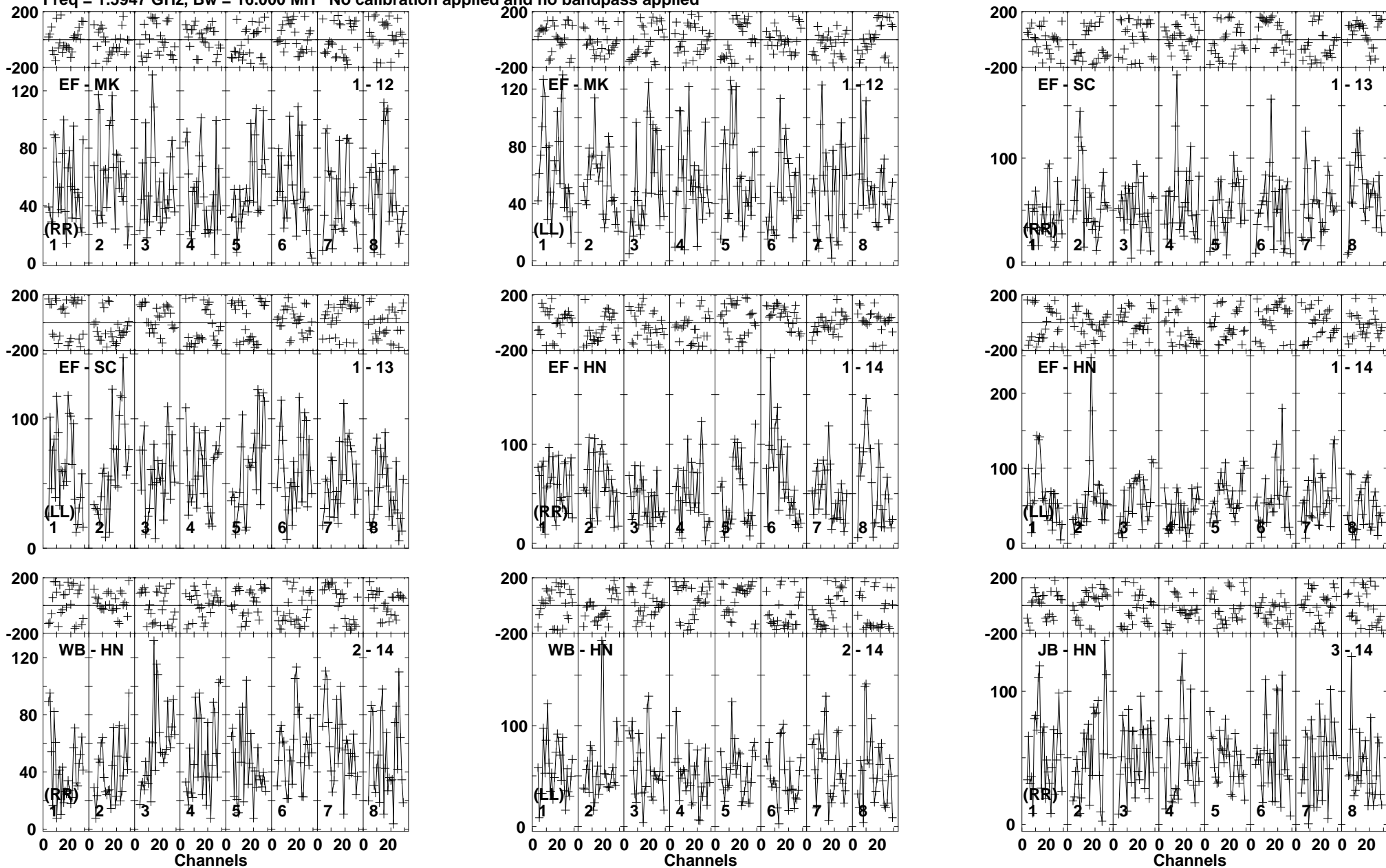
Lower frame: Micro Ampl Jy Top frame: Phas deg Vector averaged cross-power spectrum Baseline: EF (01) - MK (12) Timerange: 00/21:21:26 to 00/21:26:36
