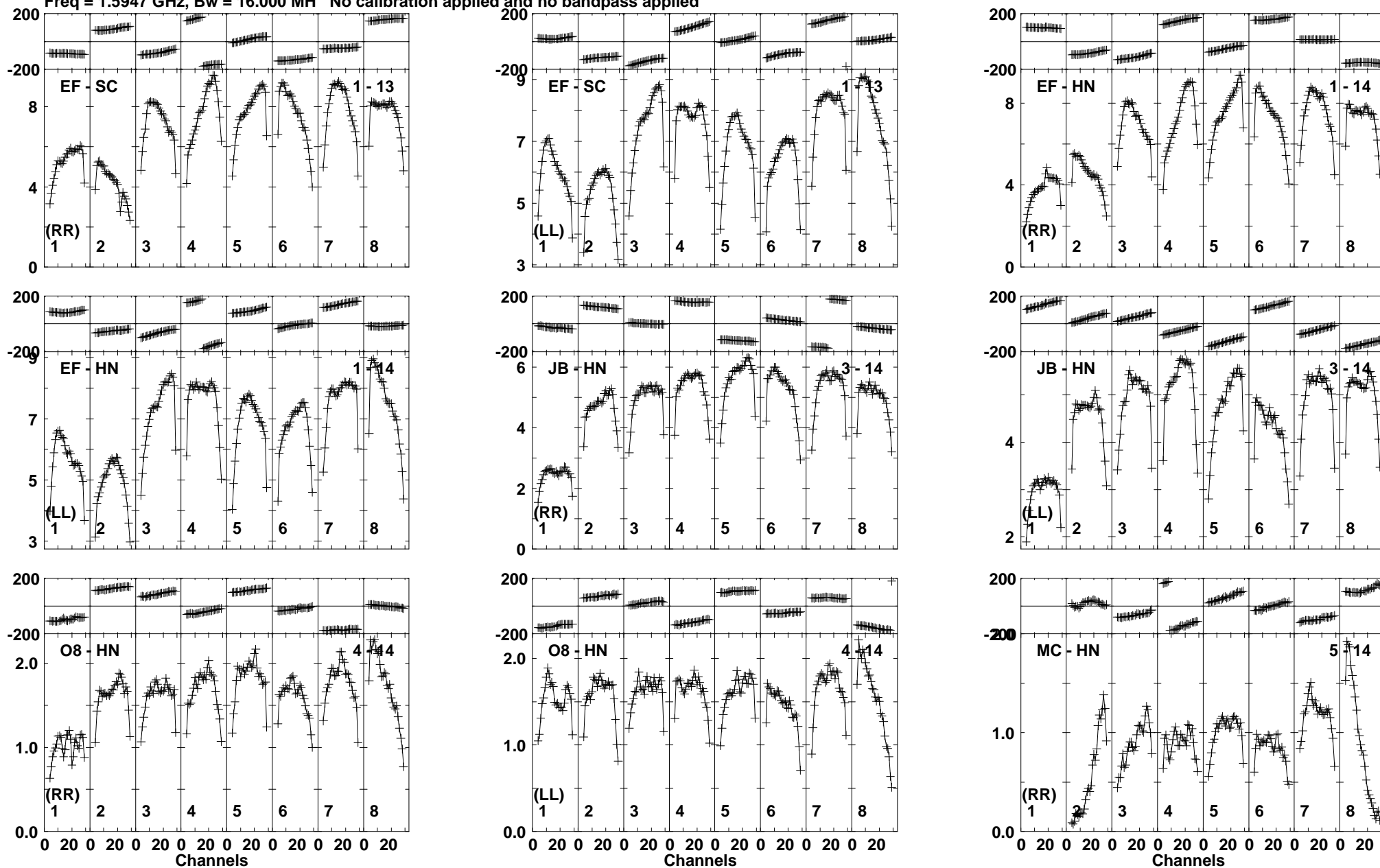
Lower frame: Milli Ampl Jy Top frame: Phas deg Vector averaged cross-power spectrum Baseline: EF (01) - SC (13) Timerange: 01/00:55:51 to 01/00:57:32
