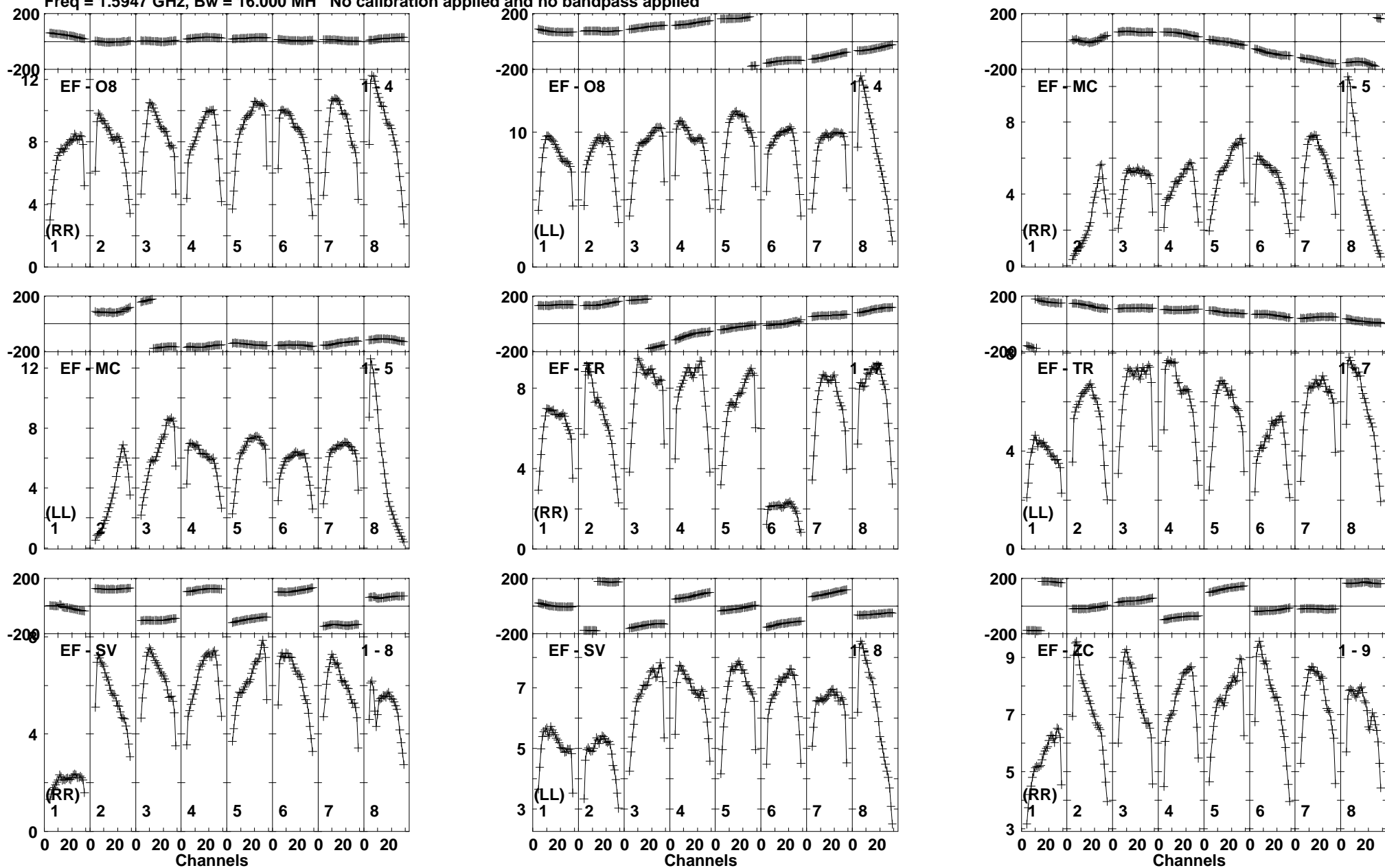
Lower frame: Milli Ampl Jy Top frame: Phas deg Vector averaged cross-power spectrum Baseline: EF (01) - O8 (04) Timerange: 01/01:17:24 to 01/01:19:13
