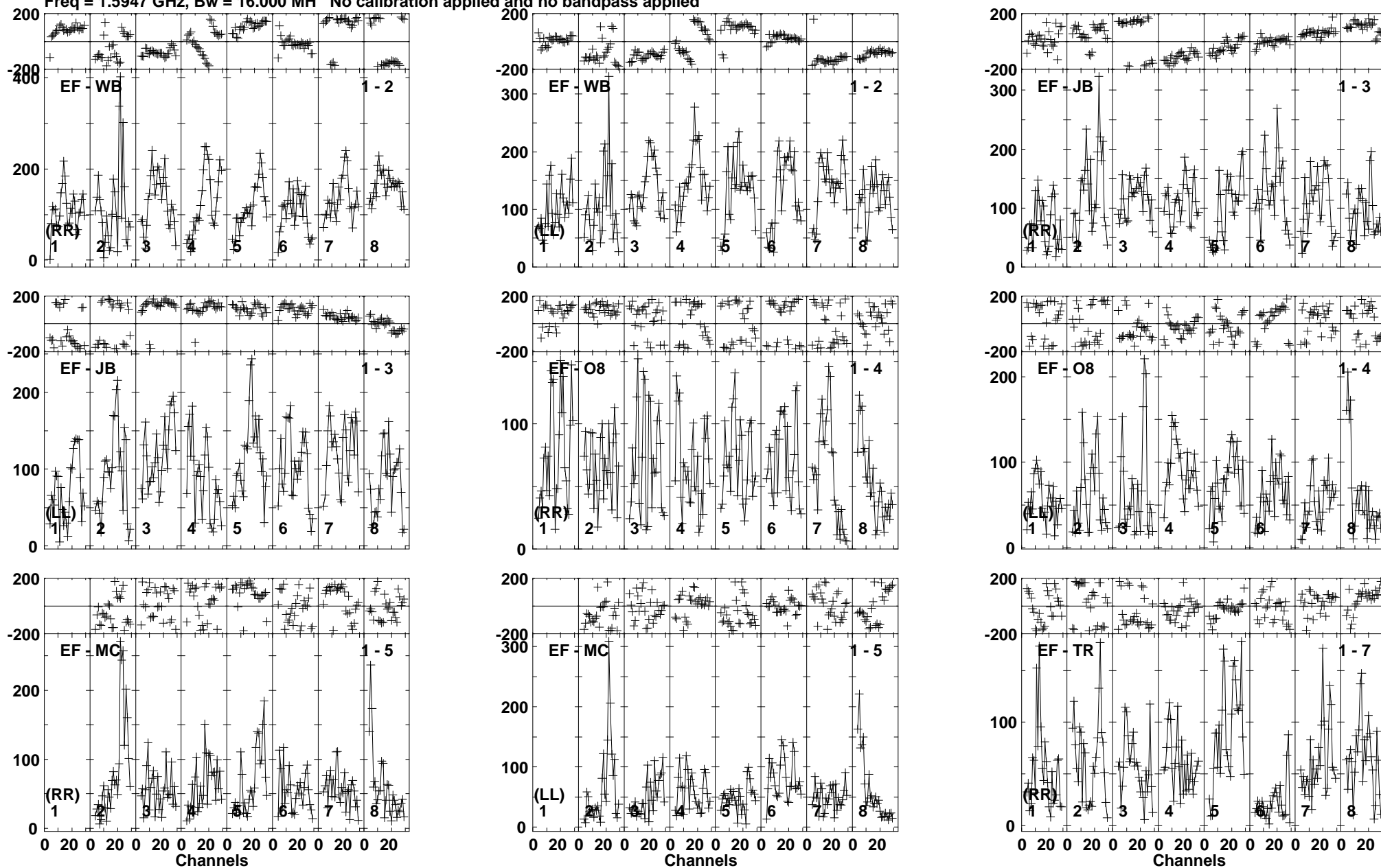
Lower frame: Micro Ampl Jy Top frame: Phas deg Vector averaged cross-power spectrum Baseline: EF (01) - WB (02) Timerange: 00/22:40:43 to 00/22:45:57
