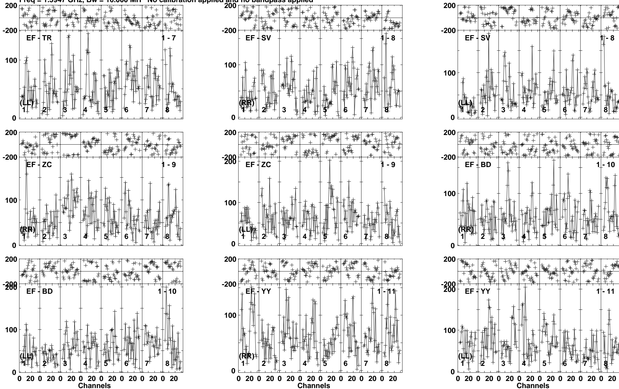
Lower frame: Micro Ampl Jy Top frame: Phas deg Vector averaged cross-power spectrum Baseline: EF (01) - TR (07) Timerange: 00/21:21:26 to 00/21:26:36
