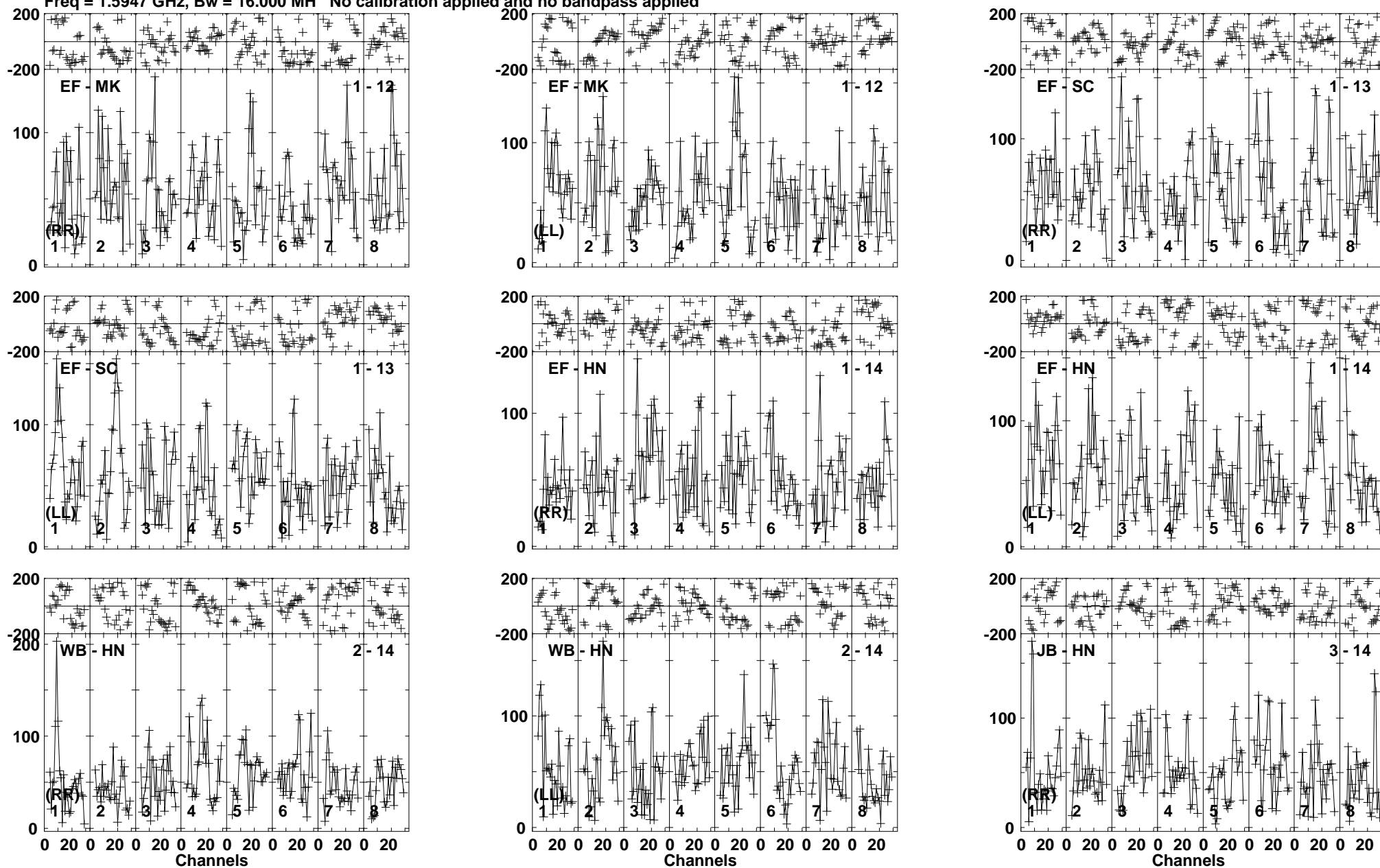
Lower frame: Micro Ampl Jy Top frame: Phas deg Vector averaged cross-power spectrum Baseline: EF (01) - MK (12) Timerange: 00/21:14:13 to 00/21:19:27
