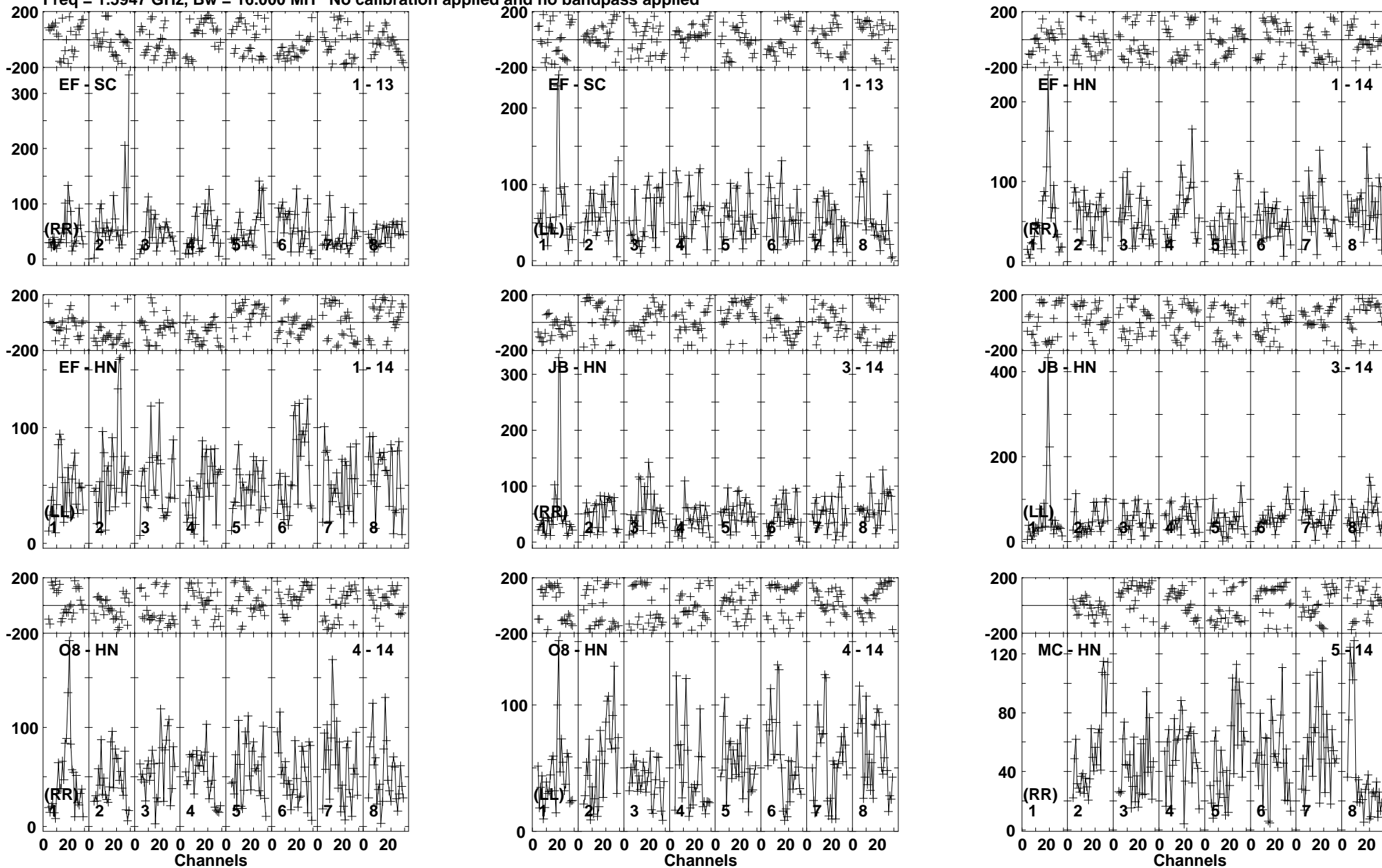
Lower frame: Micro Ampl Jy Top frame: Phas deg Vector averaged cross-power spectrum Baseline: EF (01) - SC (13) Timerange: 01/00:43:16 to 01/00:48:26
