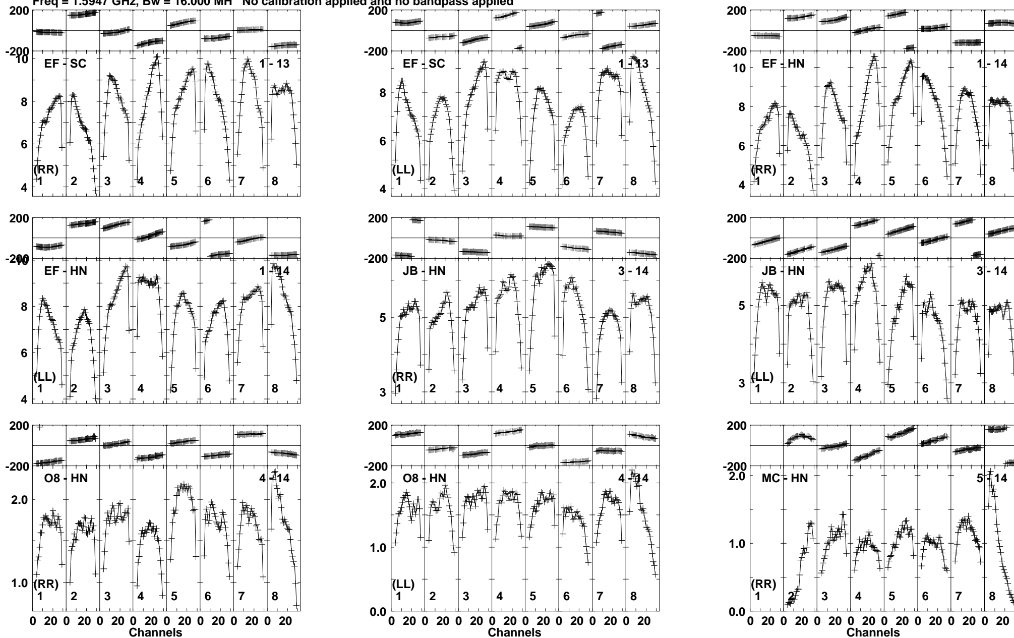
Lower frame: Milli Ampl Jy Top frame: Phas deg Vector averaged cross-power spectrum Baseline: EF (01) - SC (13) Timerange: 01/00:12:35 to 01/00:14:17
