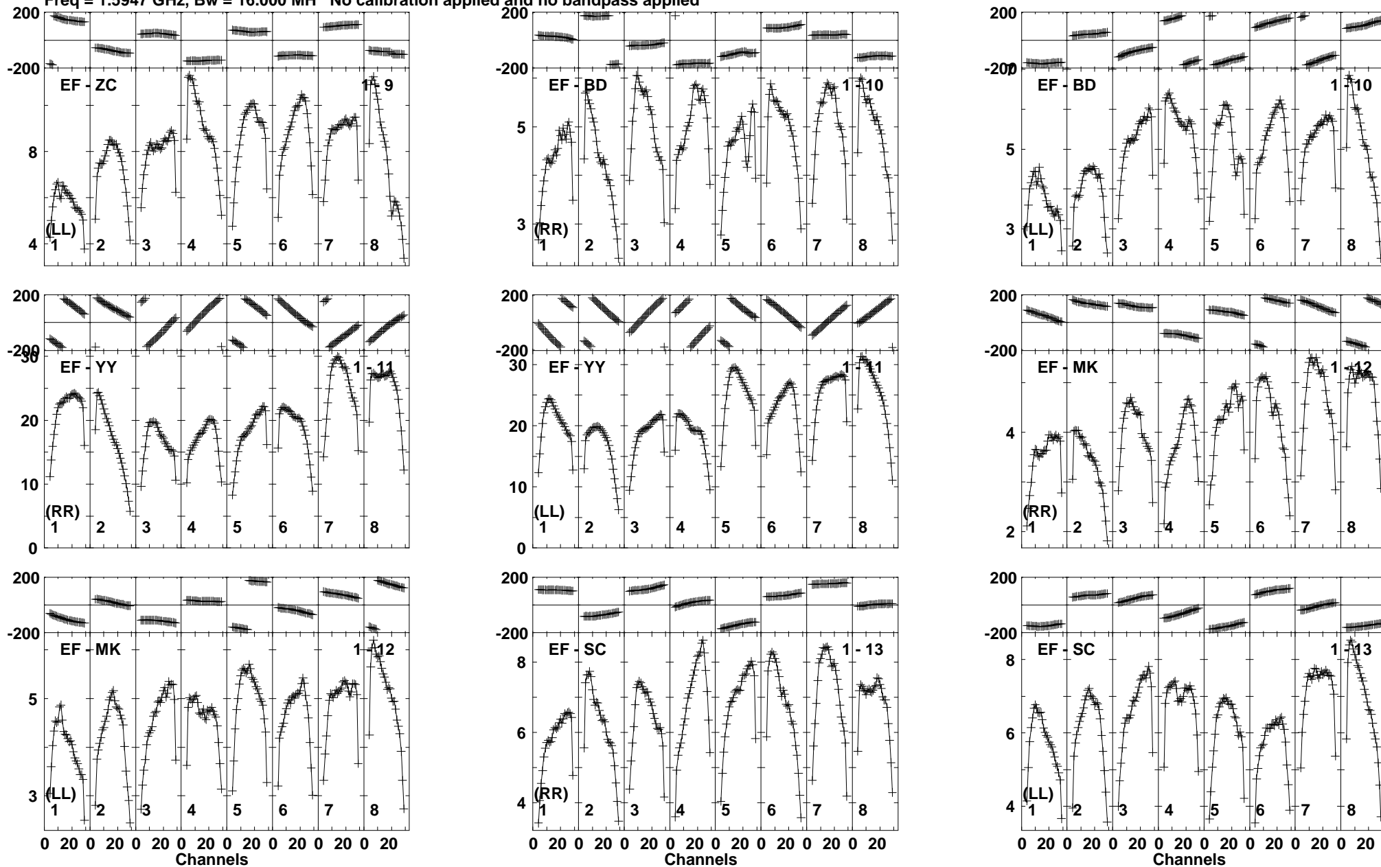
Lower frame: Milli Ampl Jy Top frame: Phas deg Vector averaged cross-power spectrum Baseline: EF (01) - ZC (09) Timerange: 01/00:34:09 to 01/00:35:58
