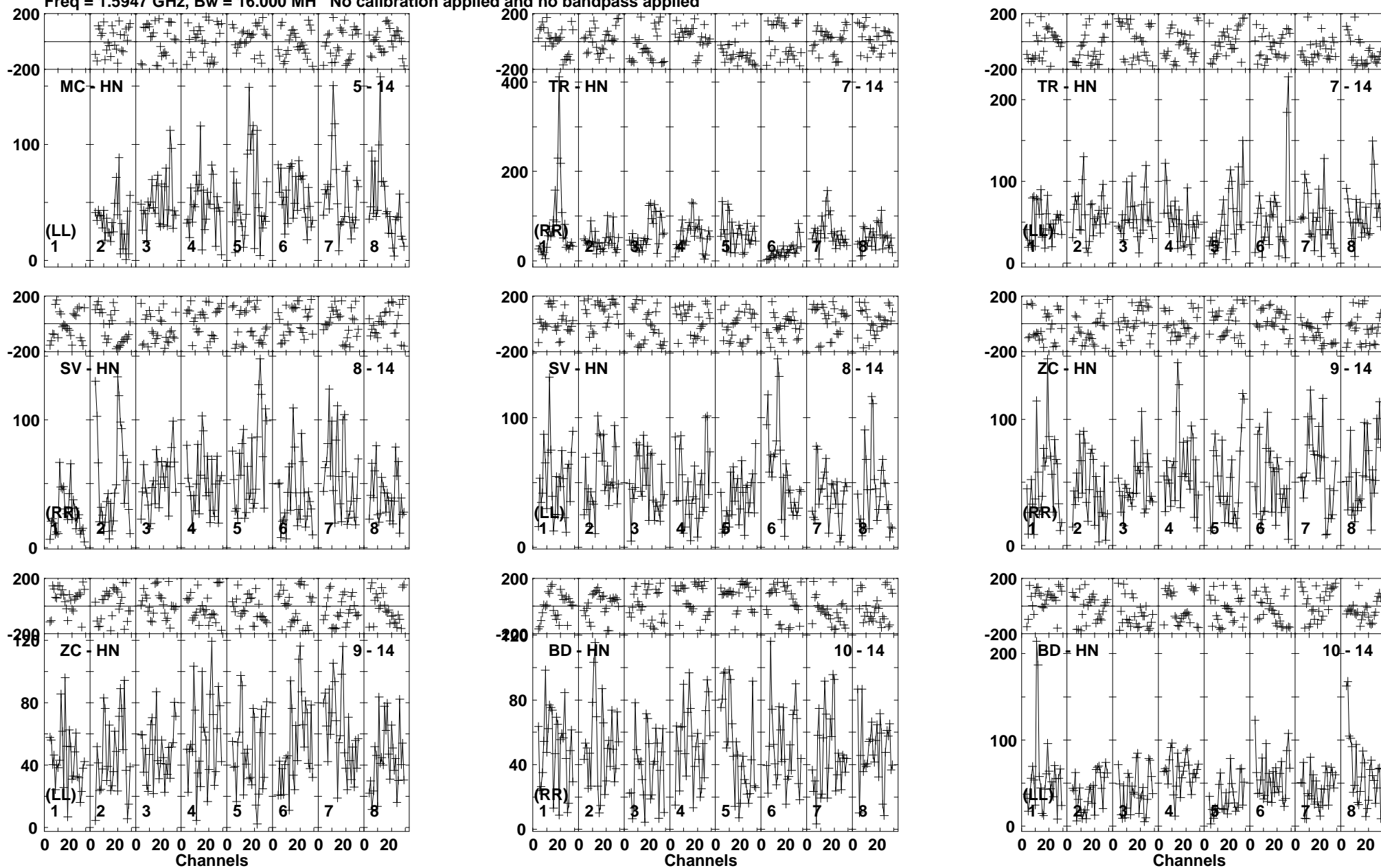
Lower frame: Micro Ampl Jy Top frame: Phas deg Vector average cross-power spectrum Baseline: MC (05) - HN (14) Timerange: 01/00:57:41 to 01/01:02:51
