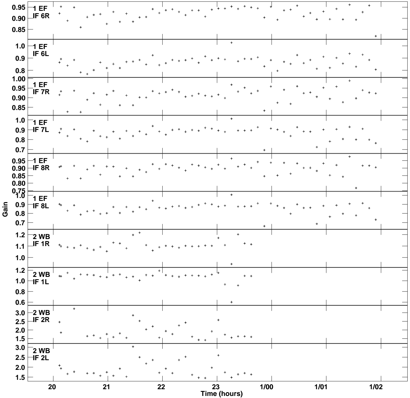
Plot file version 2 created 14-APR-2016 21:29:34 Gain amp vs UTC time for J1128+5925.MULTI.1 SN 2 Rpol & Lpol IF 1 - 8
