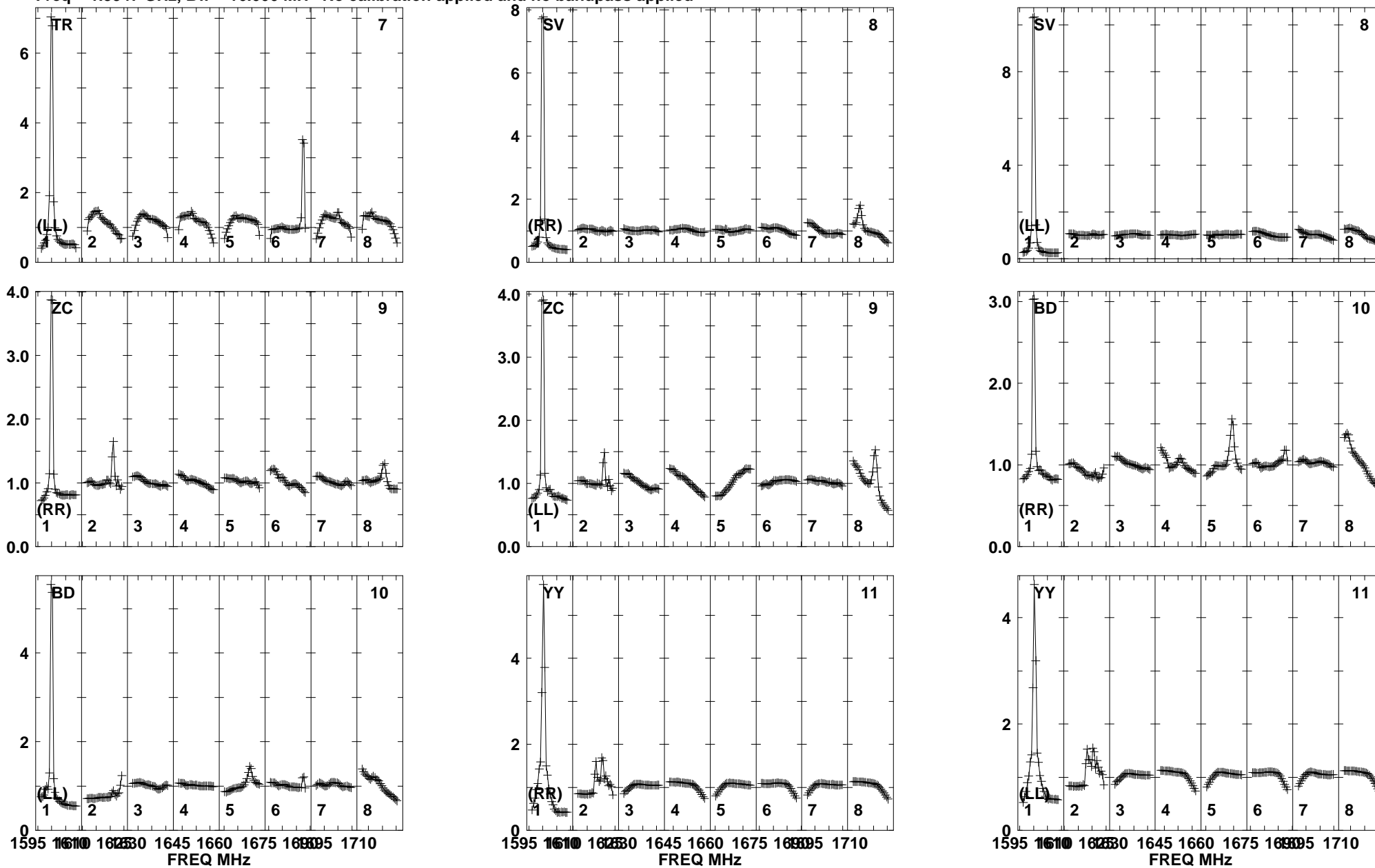
Lower frame: Real Jy Total-power spectrum Antenna: TR (07) Timerange: 00/22:38:48 to 00/22:40:38
