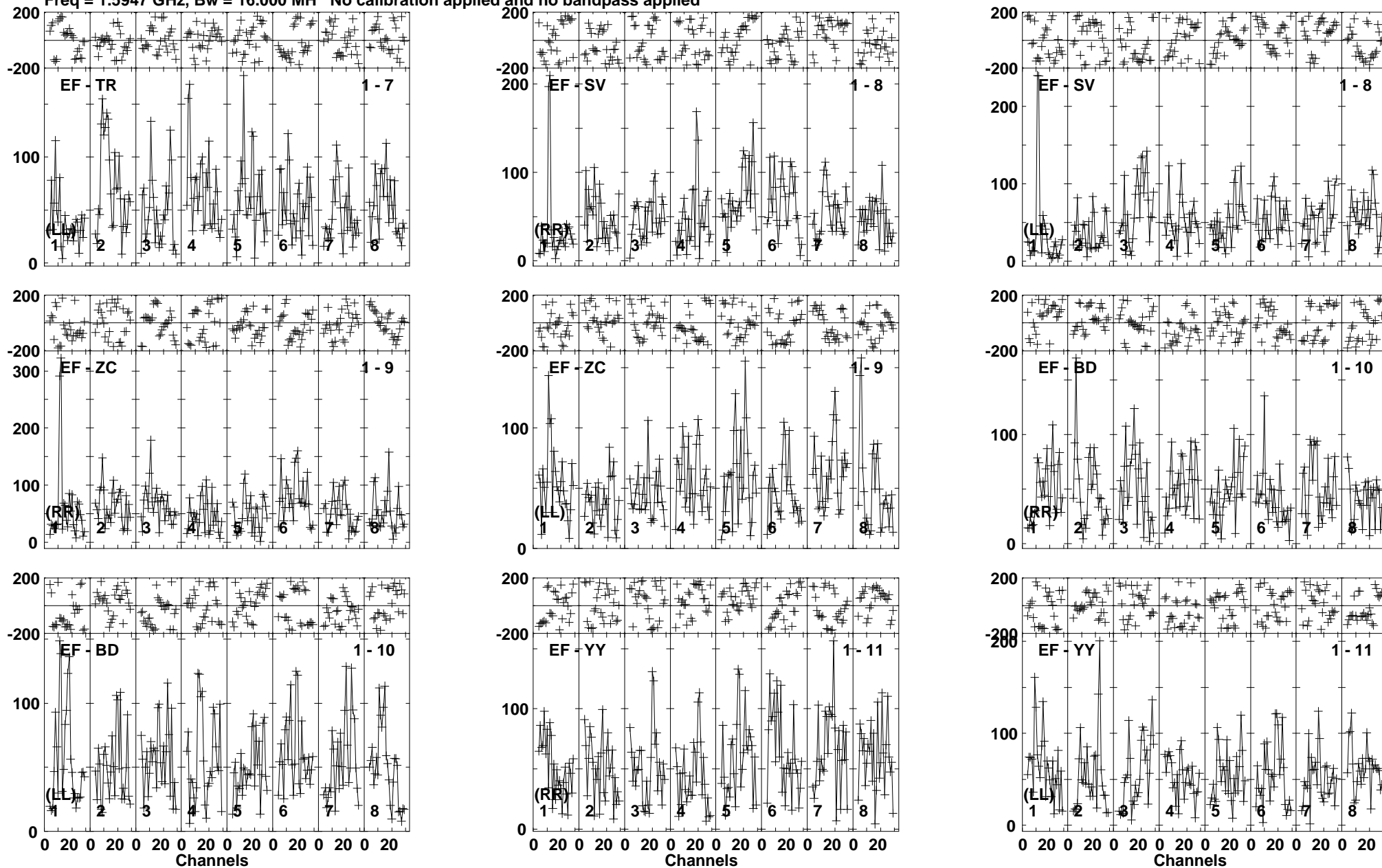
Lower frame: Micro Ampl Jy Top frame: Phas deg Vector averaged cross-power spectrum Baseline: EF (01) - TR (07) Timerange: 00/20:30:58 to 00/20:36:12
