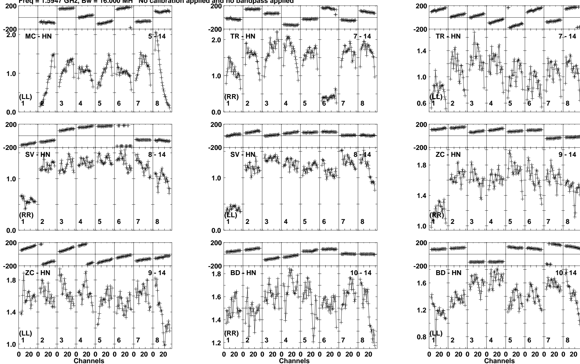
Lower frame: Milli Ampl Jy Top frame: Phas deg Vector averaged cross-power spectrum Baseline: MC (05) - HN (14) Timerange: 00/21:41:09 to 00/21:42:58
