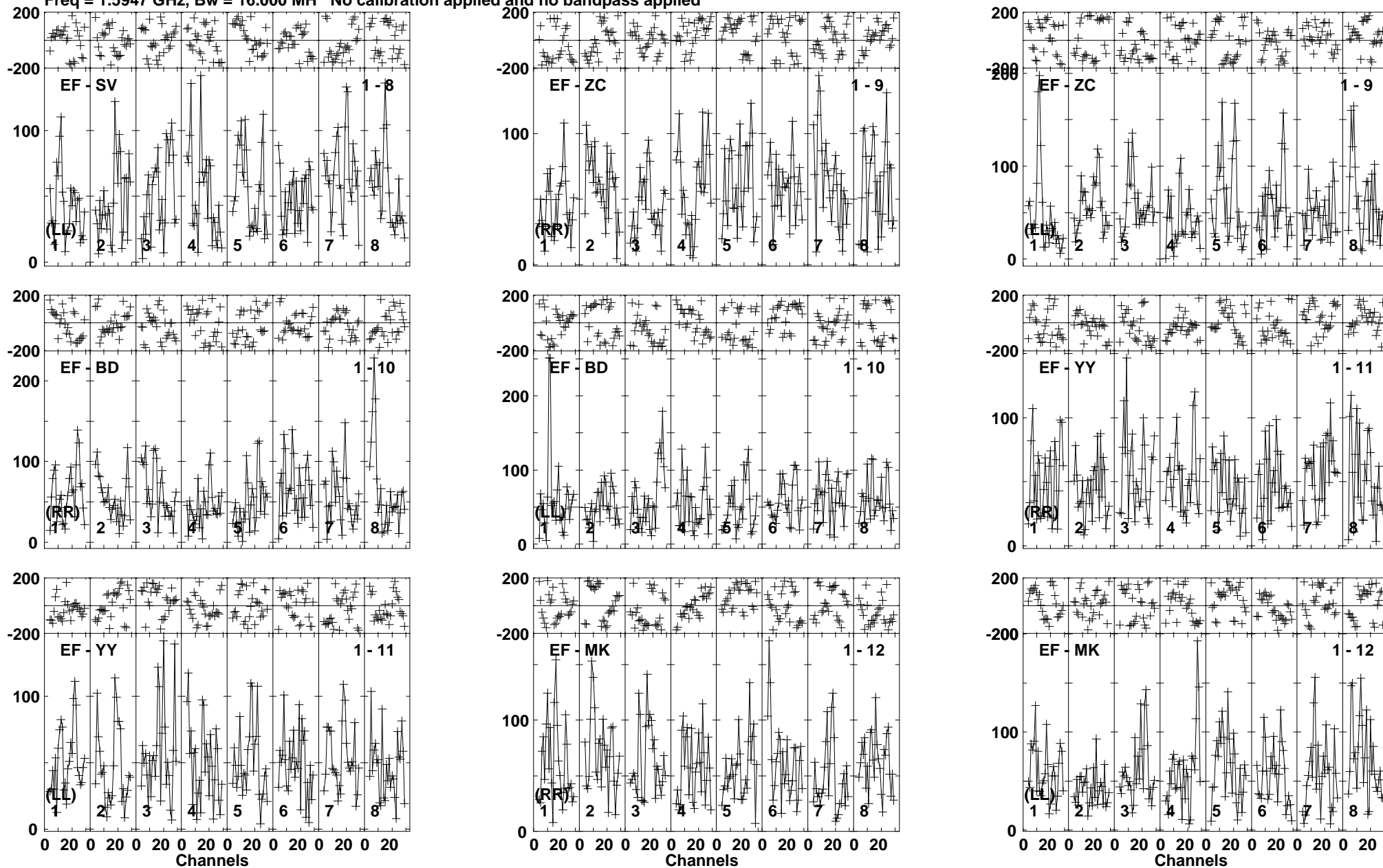
Lower frame: Micro Ampl Jy Top frame: Phas deg Vector averaged cross-power spectrum Baseline: EF (01) - SV (08) Timerange: 01/01:33:43 to 01/01:38:57
