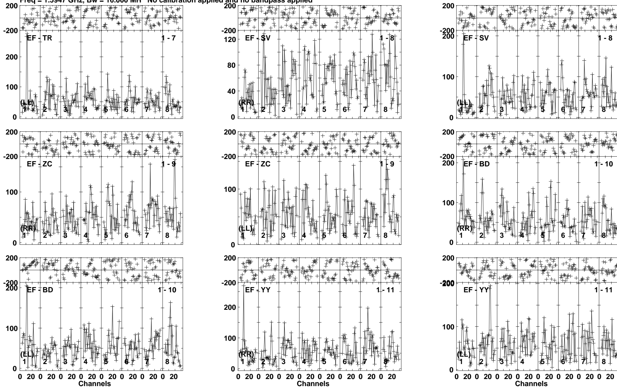
Lower frame: Micro Ampl Jy Top frame: Phas deg Vector average cross-power spectrum Baseline: EF (01) - TR (07) Timerange: 00/20:59:48 to 00/21:05:02
