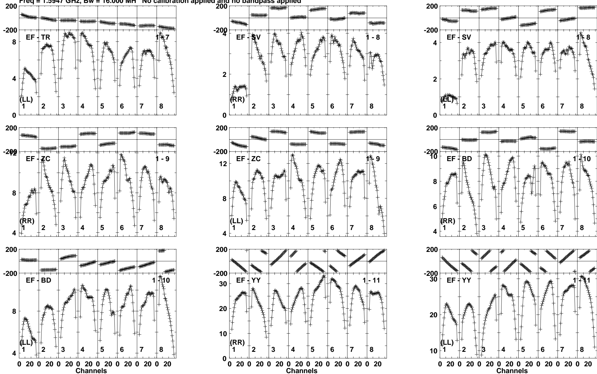
Lower frame: Milli Ampl Jy Top frame: Phas deg Vector averaged cross-power spectrum Baseline: EF (01) - TR (07) Timerange: 00/21:48:26 to 00/21:50:07
