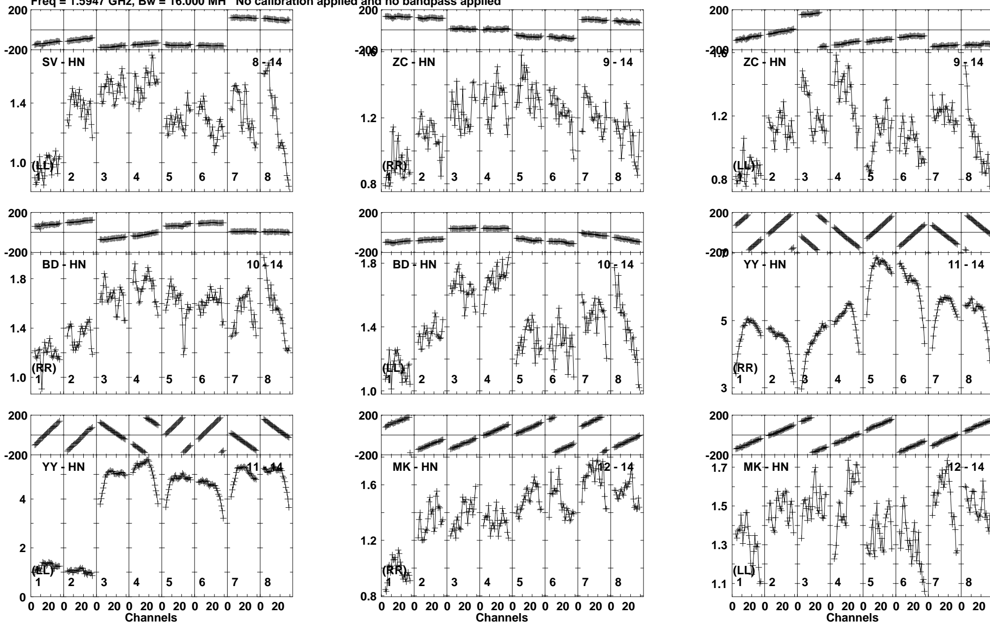
Lower frame: Milli Ampl Jy Top frame: Phas deg Vector averaged cross-power spectrum Baseline: SV (08) - HN (14) Timerange: 01/01:53:31 to 01/01:55:12
