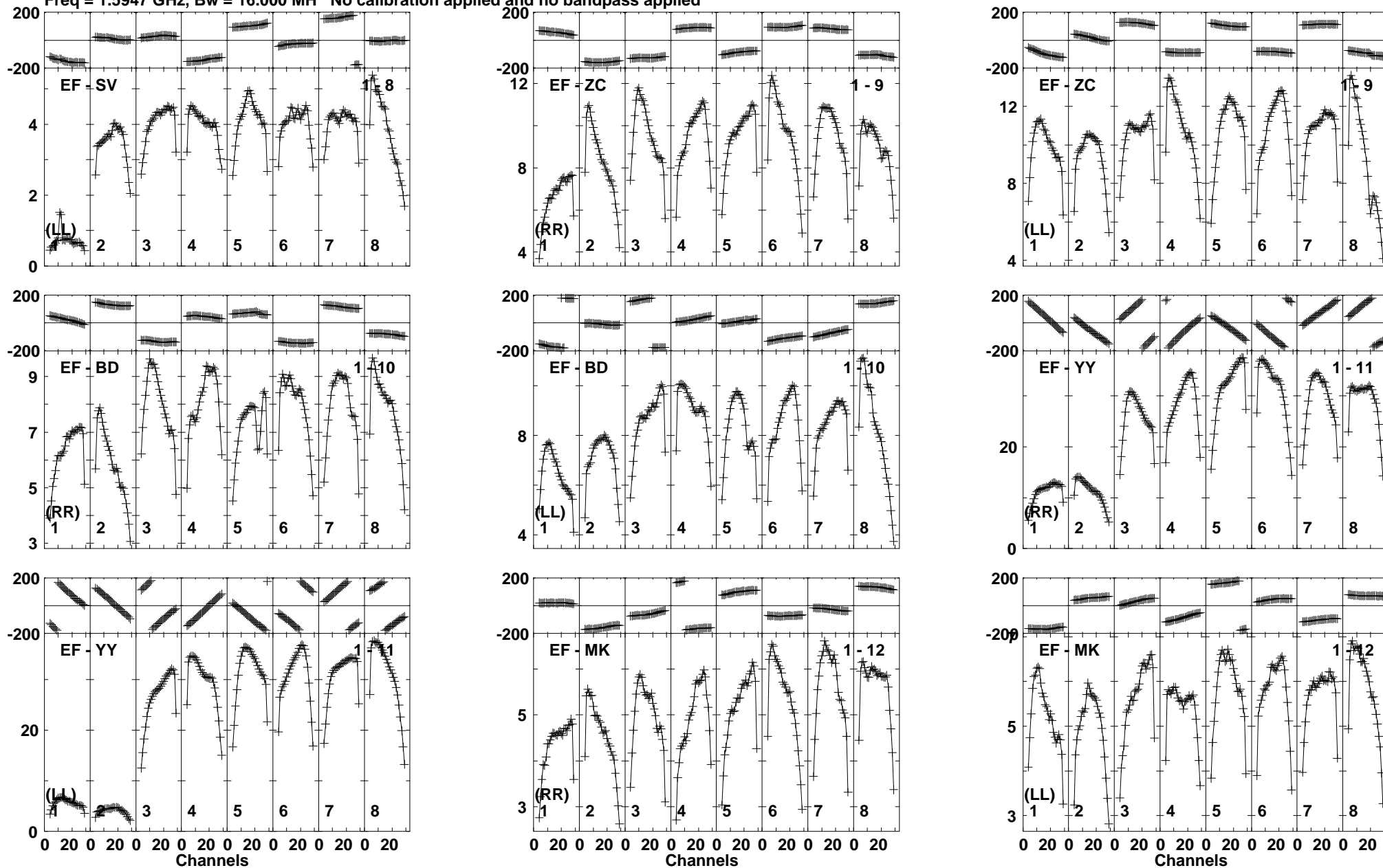
Lower frame: Milli Ampl Jy Top frame: Phas deg Vector averaged cross-power spectrum Baseline: EF (01) - SV (08) Timerange: 00/20:29:04 to 00/20:30:53
