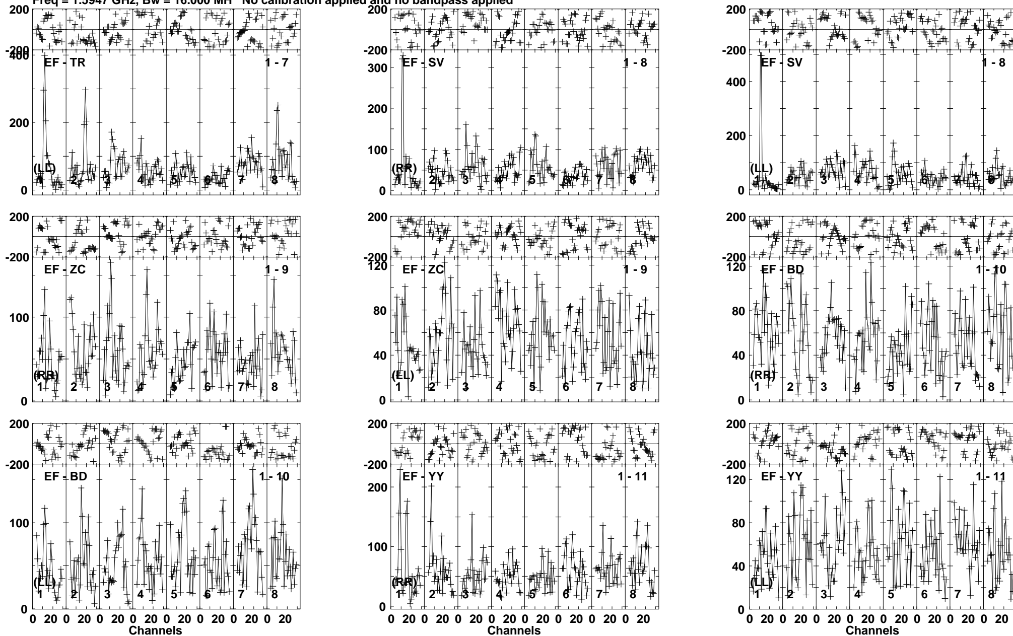
Lower frame: Micro Ampl Jy Top frame: Phas deg Vector average cross-power spectrum Baseline: EF (01) - TR (07) Timerange: 00/20:52:36 to 00/20:57:46
