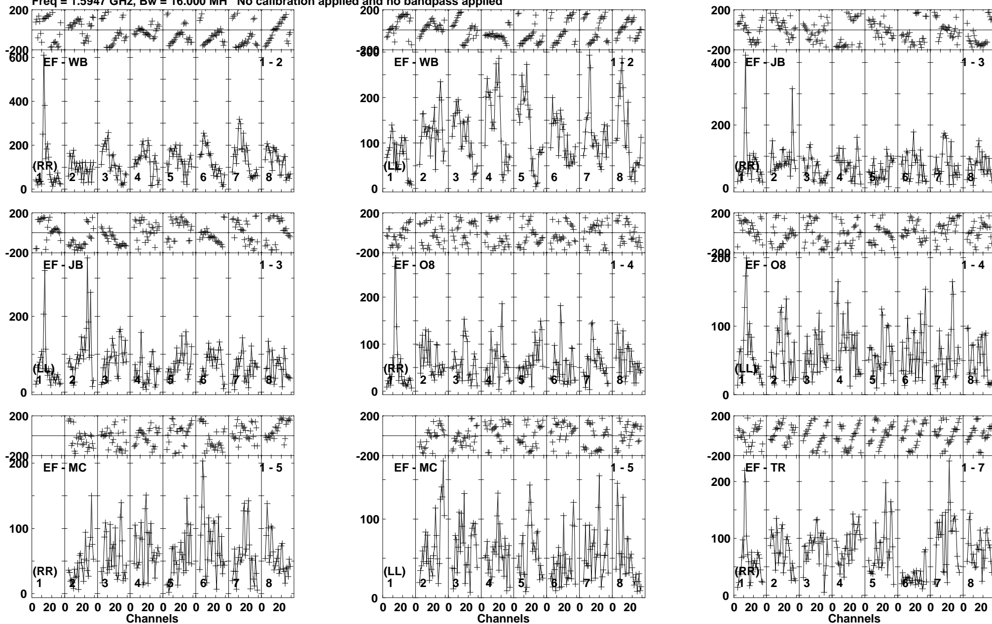
Lower frame: Micro Ampl Jy Top frame: Phas deg Vector averaged cross-power spectrum Baseline: EF (01) - WB (02) Timerange: 00/23:09:33 to 00/23:14:47
