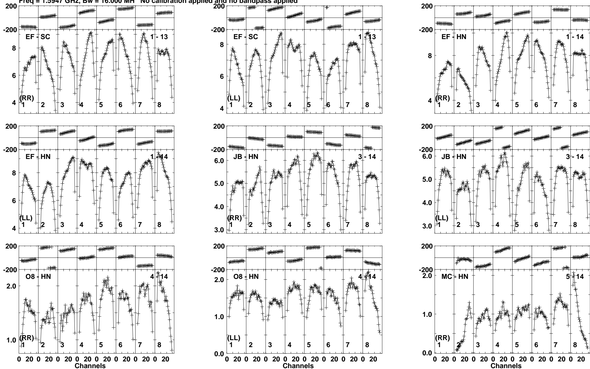
Lower frame: Milli Ampl Jy Top frame: Phas deg Vector averaged cross-power spectrum Baseline: EF (01) - SC (13) Timerange: 01/01:39:06 to 01/01:40:47
