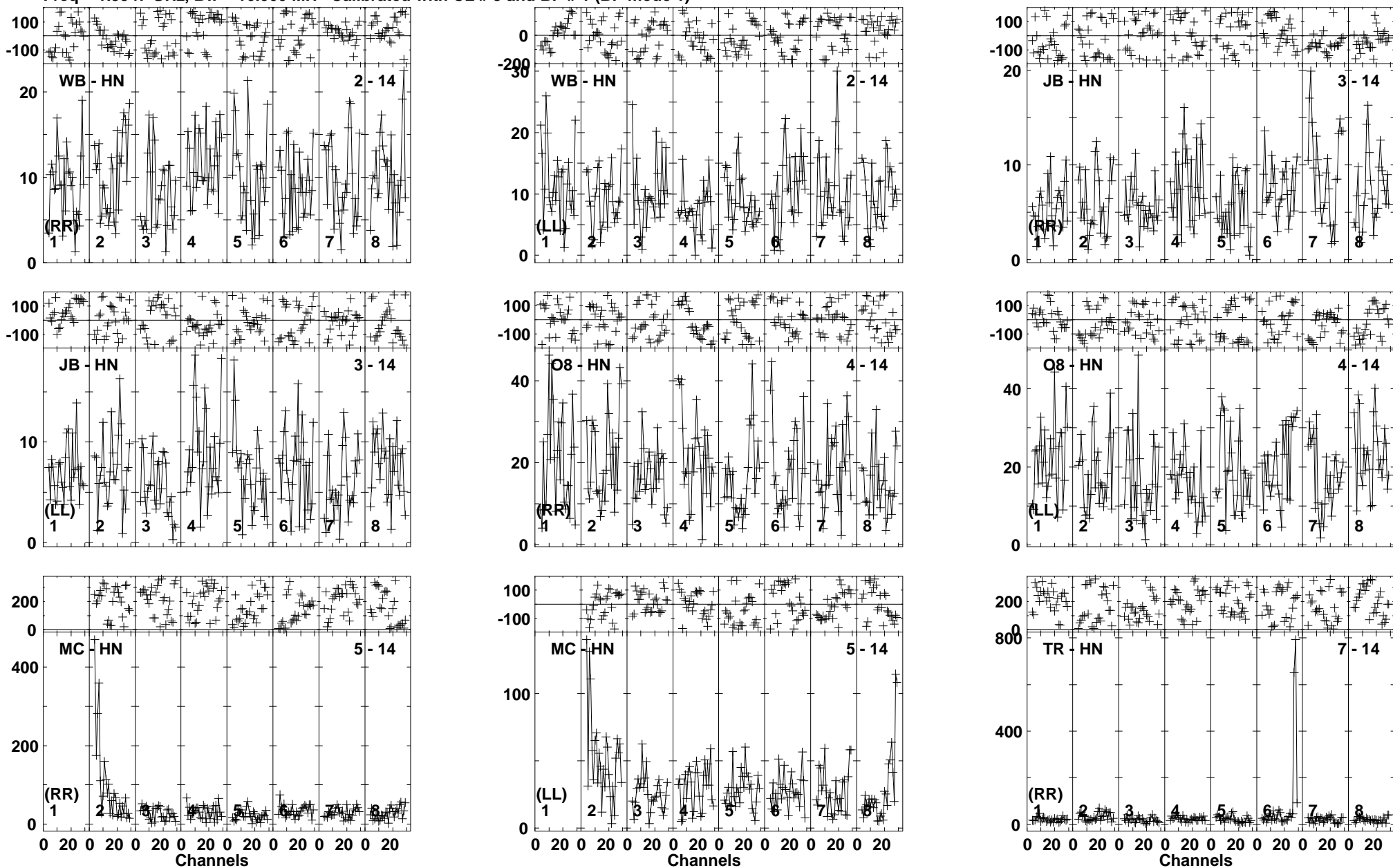
Lower frame: Milli Ampl Jy Top frame: Phas deg Vector averaged cross-power spectrum Baseline: WB (02) - HN (14) Timerange: 00/21:57:28 to 00/22:02:42
