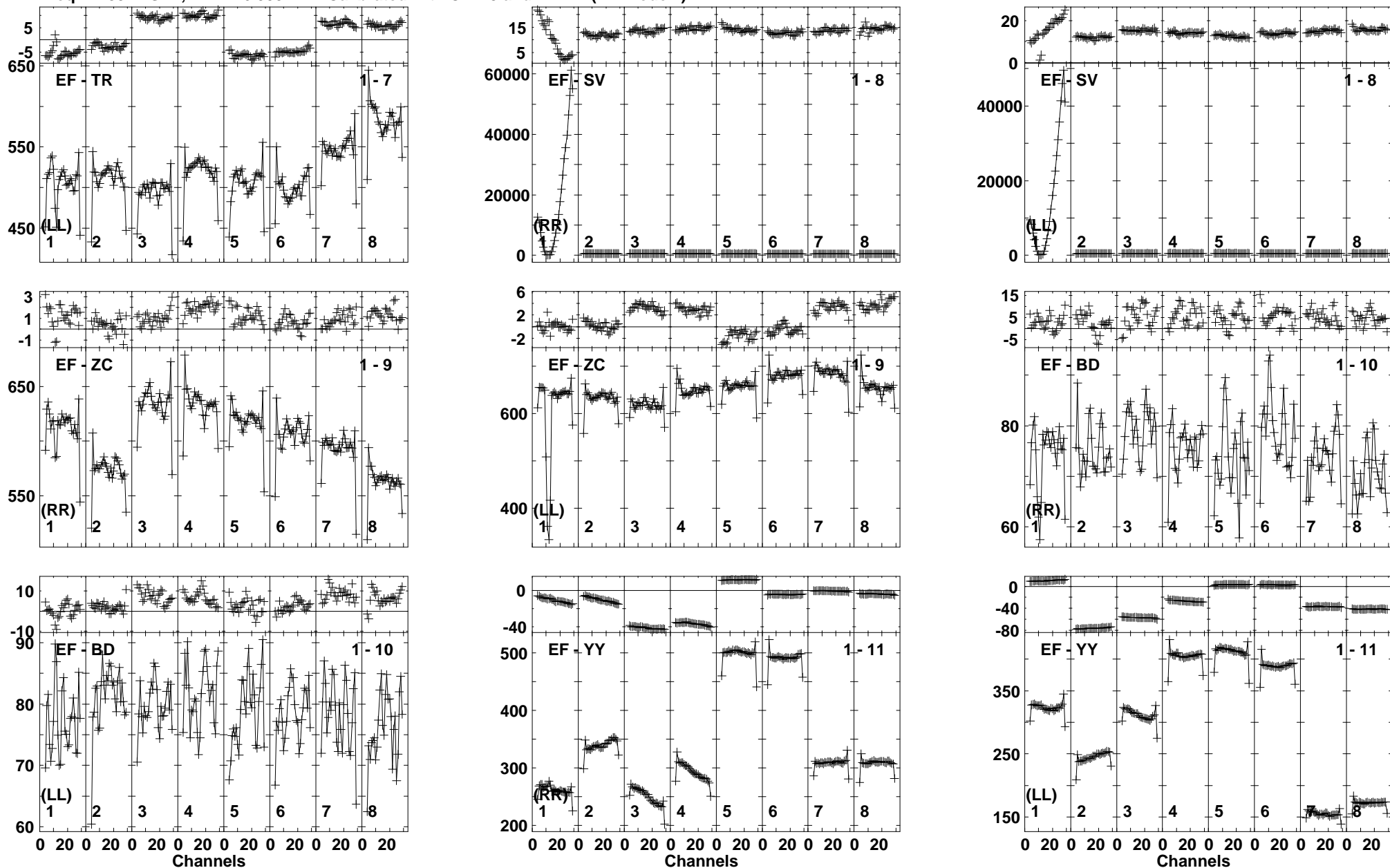
Lower frame: Milli Ampl Jy Top frame: Phas deg Vector averaged cross-power spectrum Baseline: EF (01) - TR (07) Timerange: 00/22:46:05 to 00/22:47:47
