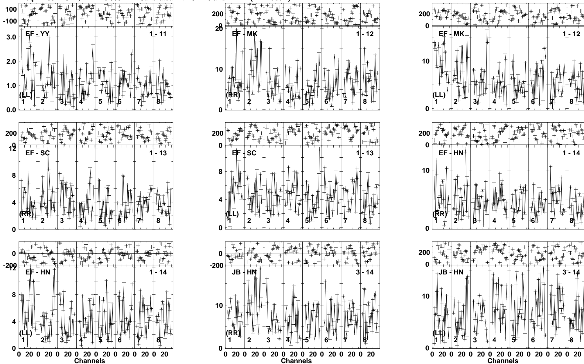
Lower frame: Milli Ampl Jy Top frame: Phas deg Vector averaged cross-power spectrum Baseline: EF (01) - YY (11) Timerange: 01/00:00:00 to 01/00:05:10
