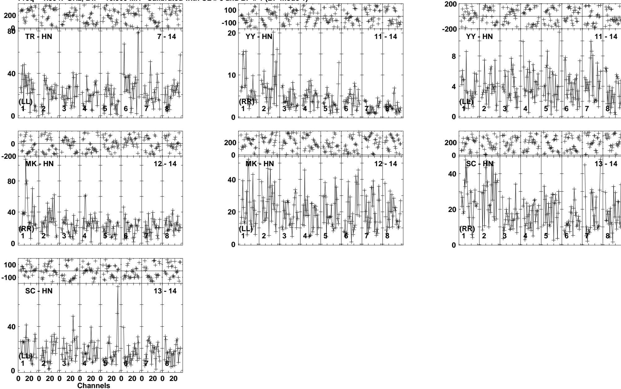
Lower frame: Milli Ampl Jy Top frame: Phas deg Vector averaged cross-power spectrum Baseline: TR (07) - HN (14) Timerange: 00/23:02:20 to 00/23:07:30
