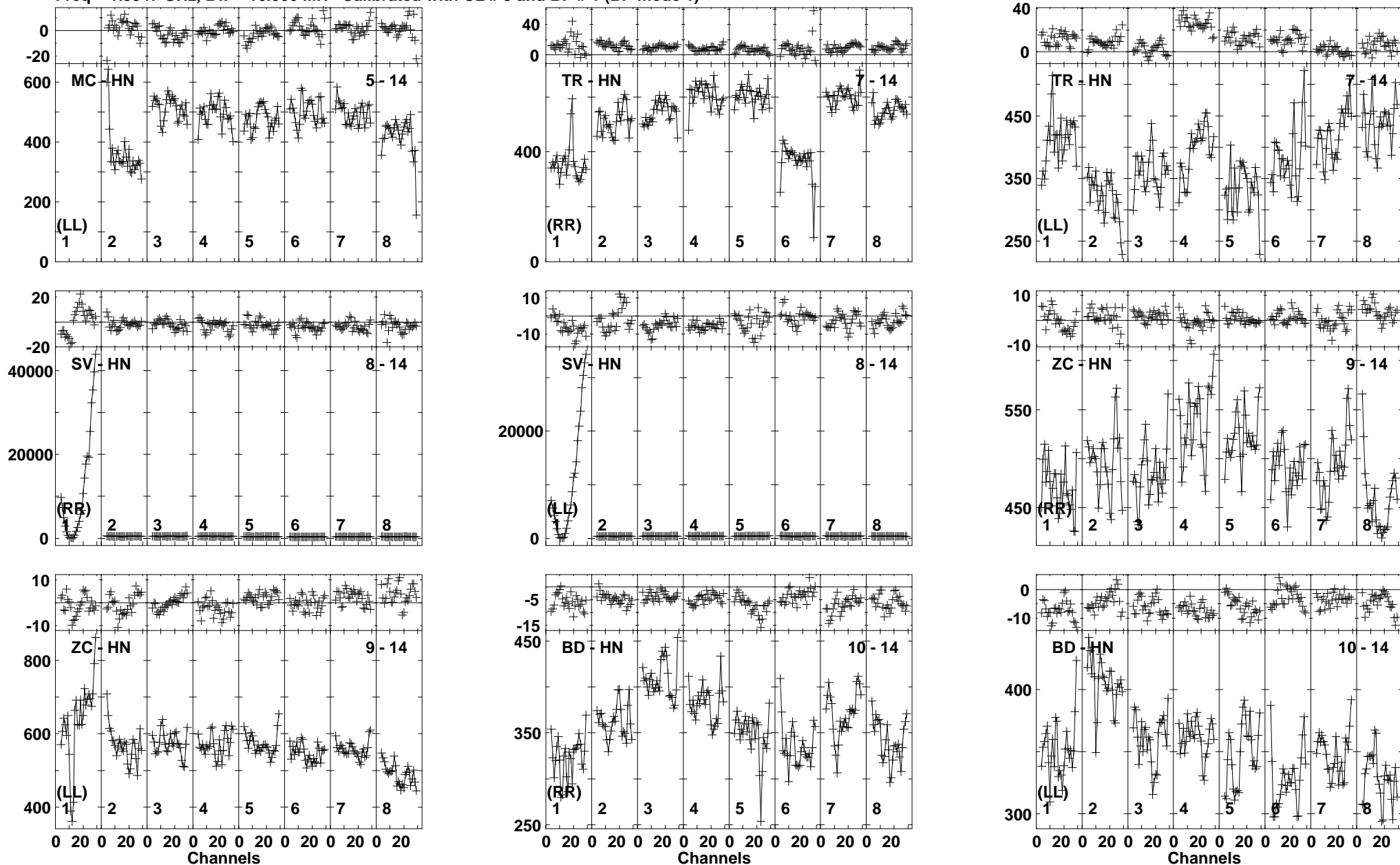
Lower frame: Milli Ampl Jy Top frame: Phas deg Vector averaged cross-power spectrum Baseline: MC (05) - HN (14) Timerange: 01/00:41:26 to 01/00:43:07
