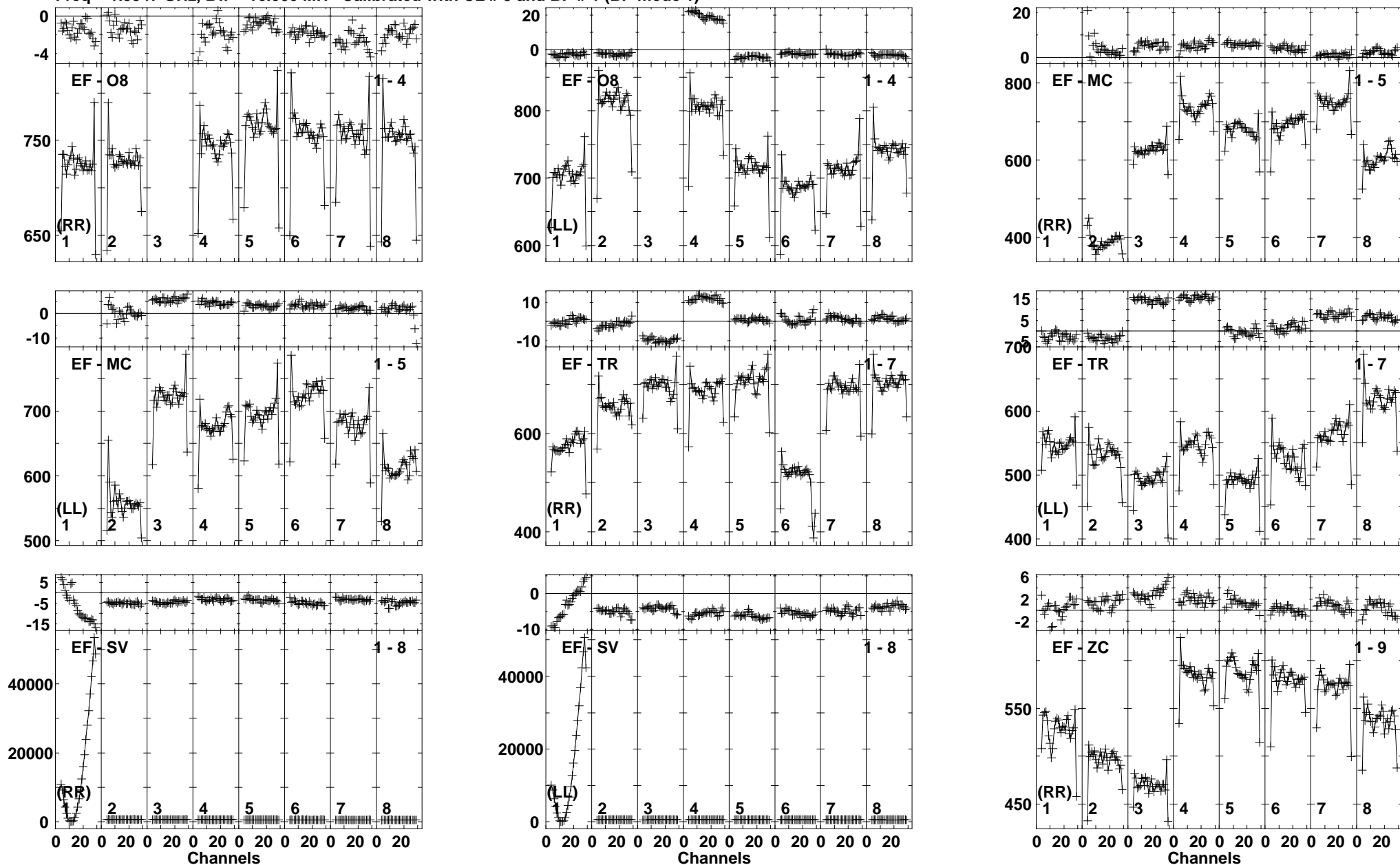
Lower frame: Milli Ampl Jy Top frame: Phas deg Vector averaged cross-power spectrum Baseline: EF (01) - O8 (04) Timerange: 01/00:34:09 to 01/00:35:58
