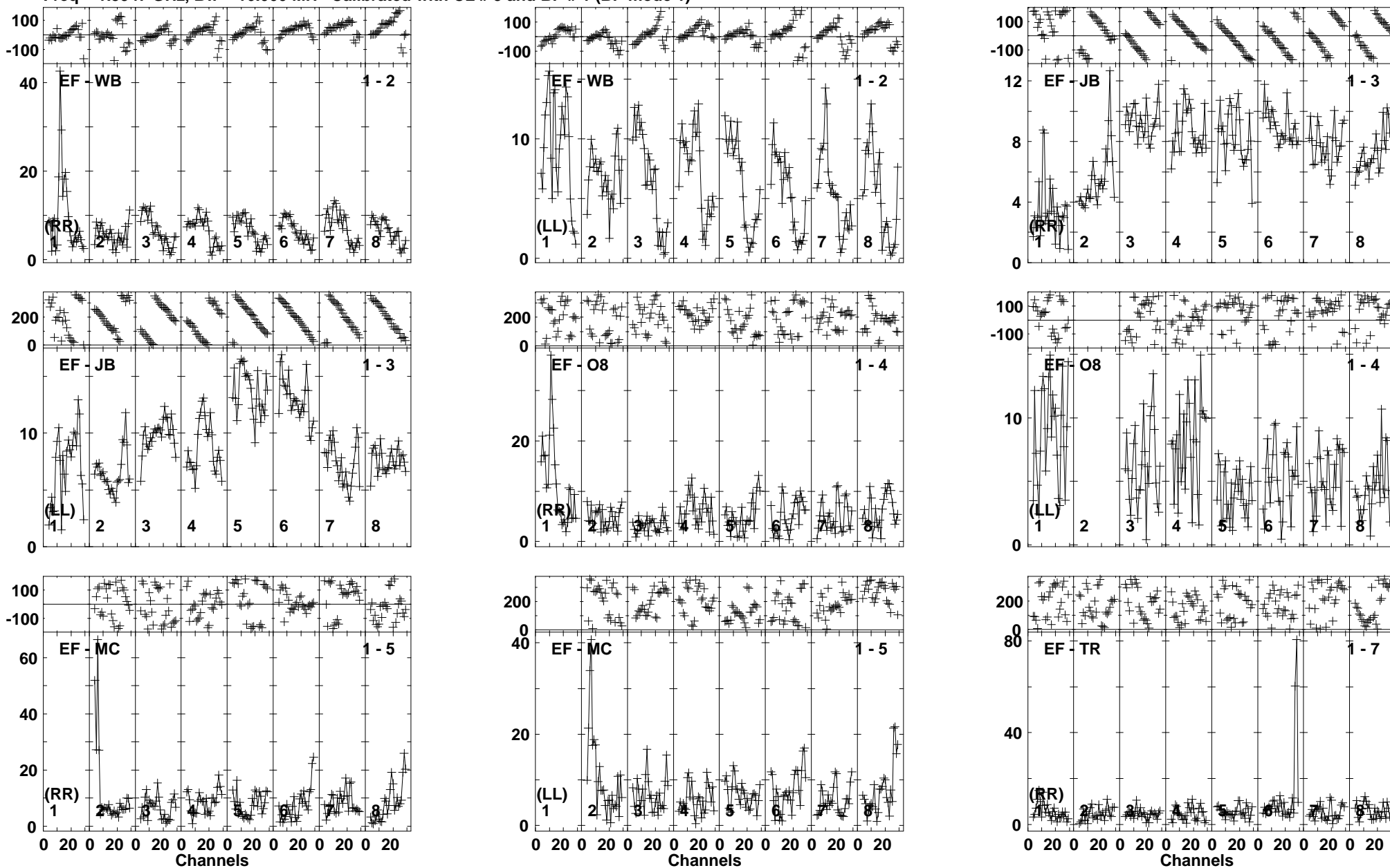
Lower frame: Milli Ampl Jy Top frame: Phas deg Vector averaged cross-power spectrum Baseline: EF (01) - WB (02) Timerange: 00/23:09:33 to 00/23:14:47
