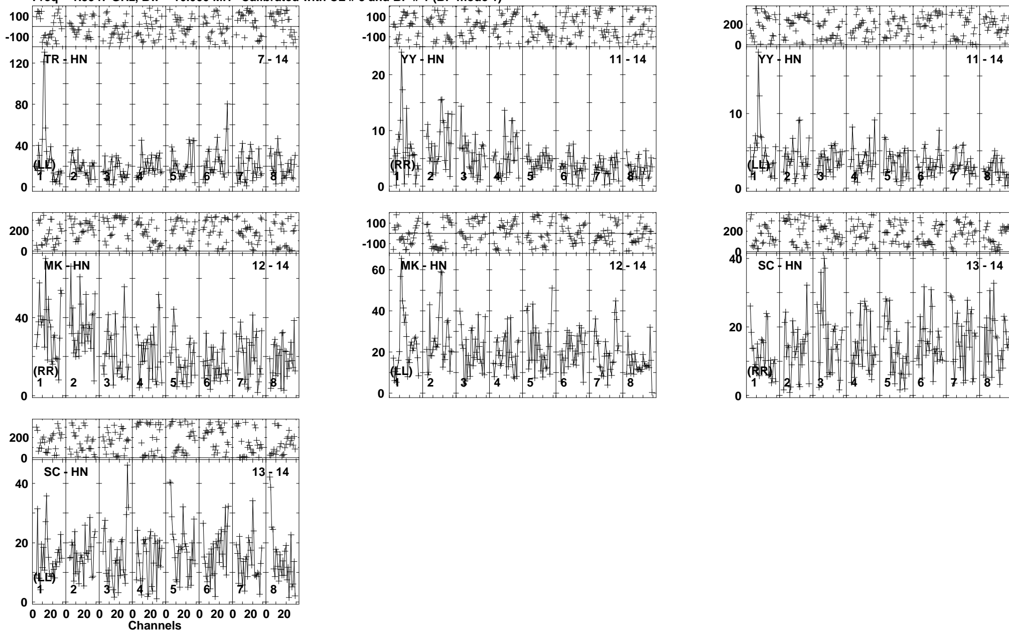
Lower frame: Milli Ampl Jy Top frame: Phas deg Vector averaged cross-power spectrum Baseline: TR (07) - HN (14) Timerange: 00/22:33:30 to 00/22:38:40
