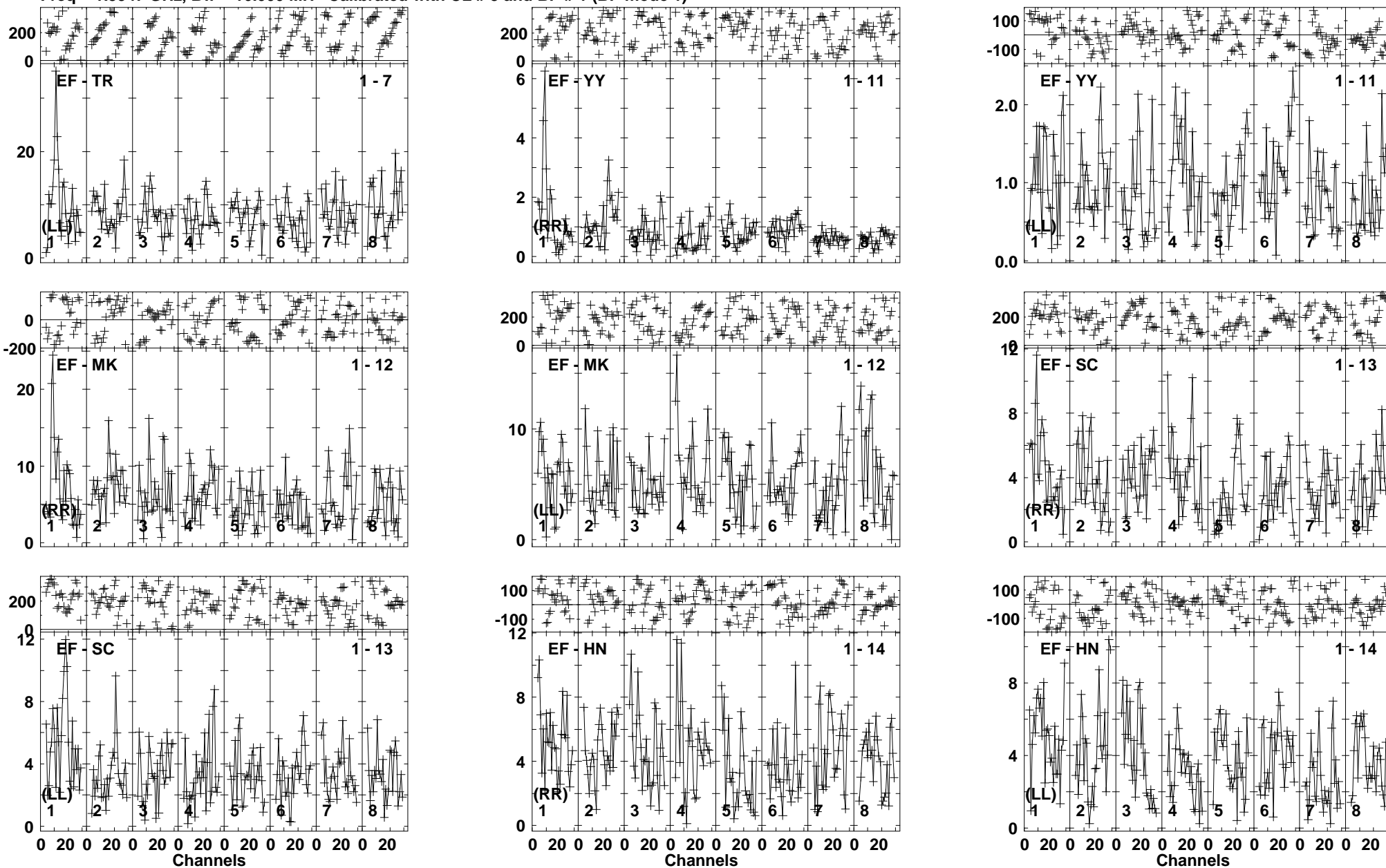
Lower frame: Milli Ampl Jy Top frame: Phas deg Vector averaged cross-power spectrum Baseline: EF (01) - TR (07) Timerange: 00/20:59:48 to 00/21:05:02
