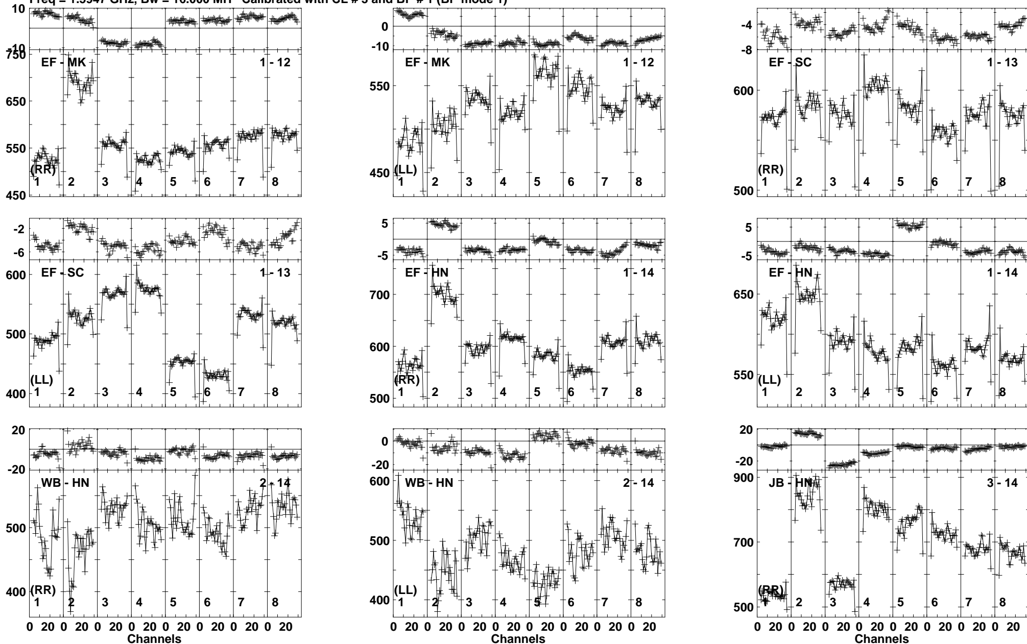
Lower frame: Milli Ampl Jy Top frame: Phas deg Vector averaged cross-power spectrum Baseline: EF (01) - MK (12) Timerange: 00/22:46:05 to 00/22:47:47
