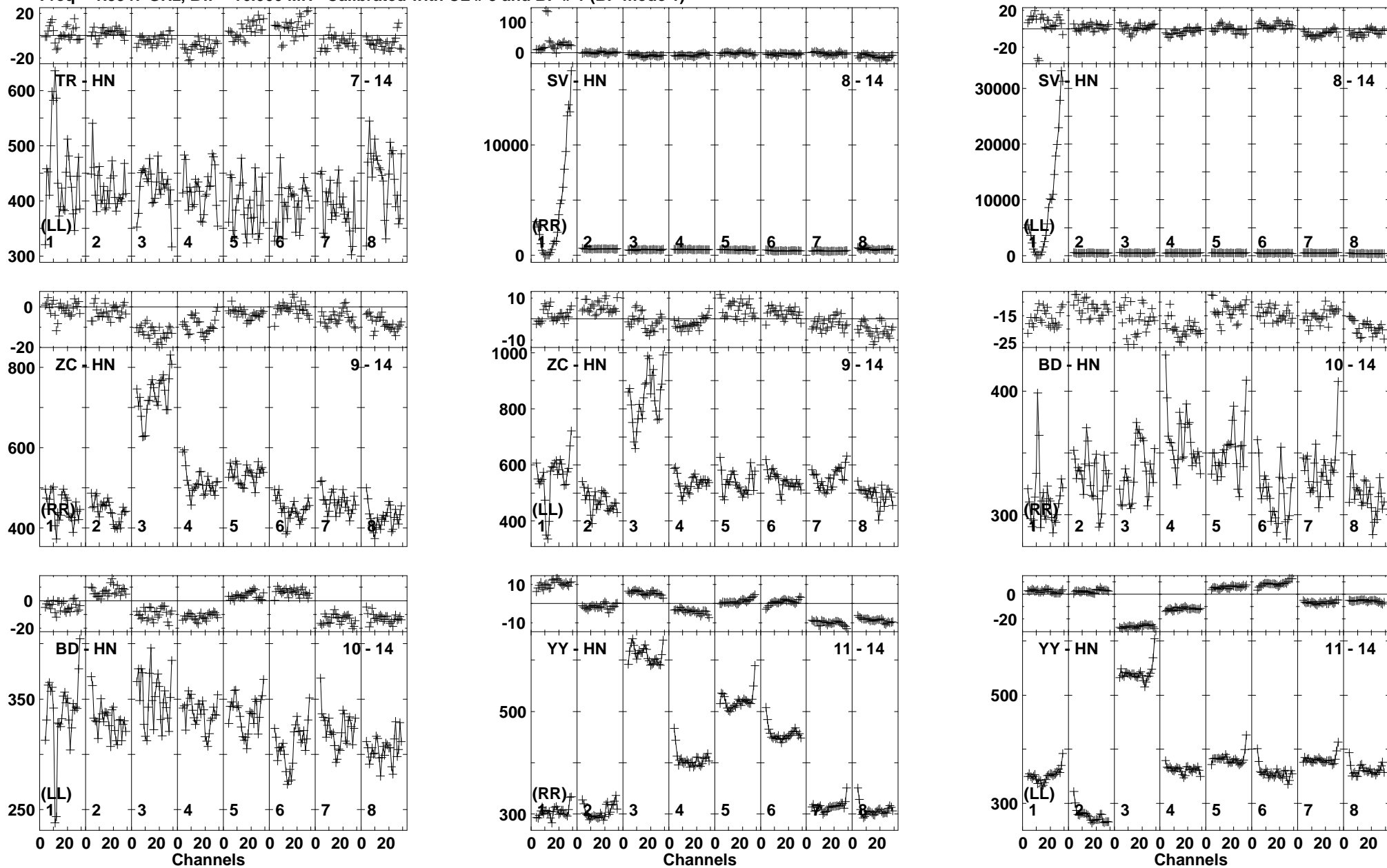
Lower frame: Milli Ampl Jy Top frame: Phas deg Vector averaged cross-power spectrum Baseline: TR (07) - HN (14) Timerange: 00/20:14:39 to 00/20:16:28
