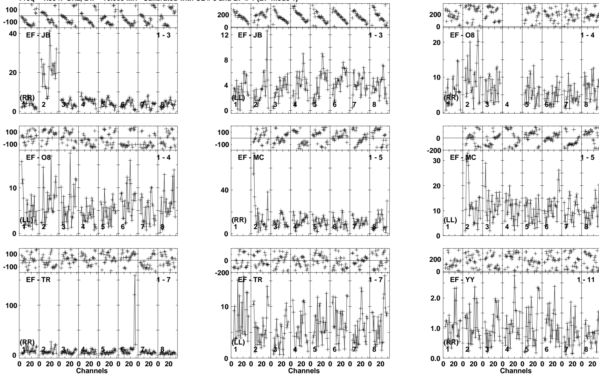
Lower frame: Milli Ampl Jy Top frame: Phas deg Vector averaged cross-power spectrum Baseline: EF (01) - JB (03) Timerange: 01/01:33:43 to 01/01:38:57
