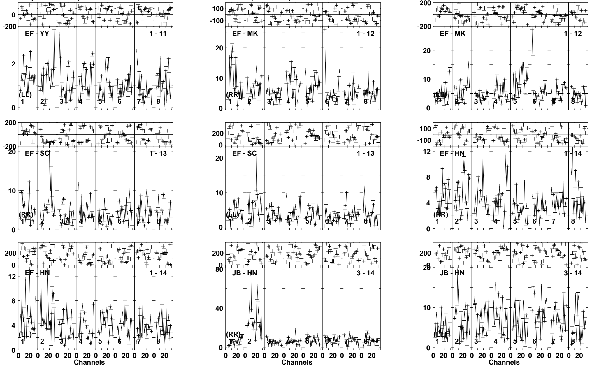
Lower frame: Milli Ampl Jy Top frame: Phas deg Vector averaged cross-power spectrum Baseline: EF (01) - YY (11) Timerange: 01/01:04:53 to 01/01:10:07
