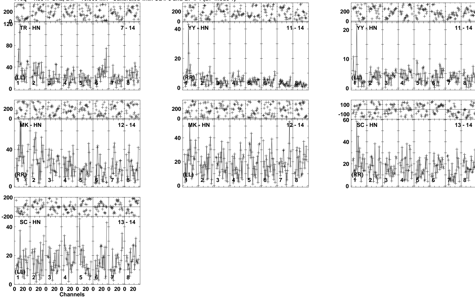
Lower frame: Milli Ampl Jy Top frame: Phas deg Vector averaged cross-power spectrum Baseline: TR (07) - HN (14) Timerange: 00:22:40:43 to 00:22:45:57
