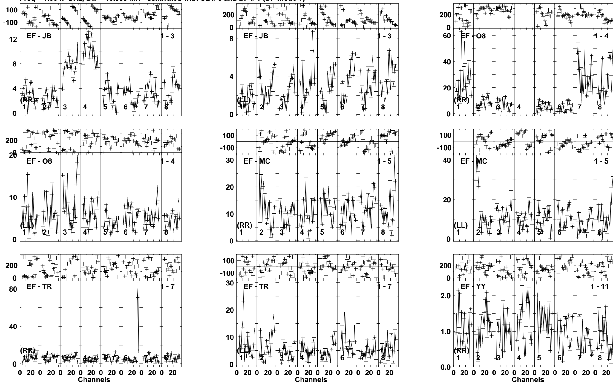
Lower frame: Milli Ampl Jy Top frame: Phas deg Vector averaged cross-power spectrum Baseline: EF (01) - JB (03) Timerange: 01/01:26:31 to 01/01:31:41
