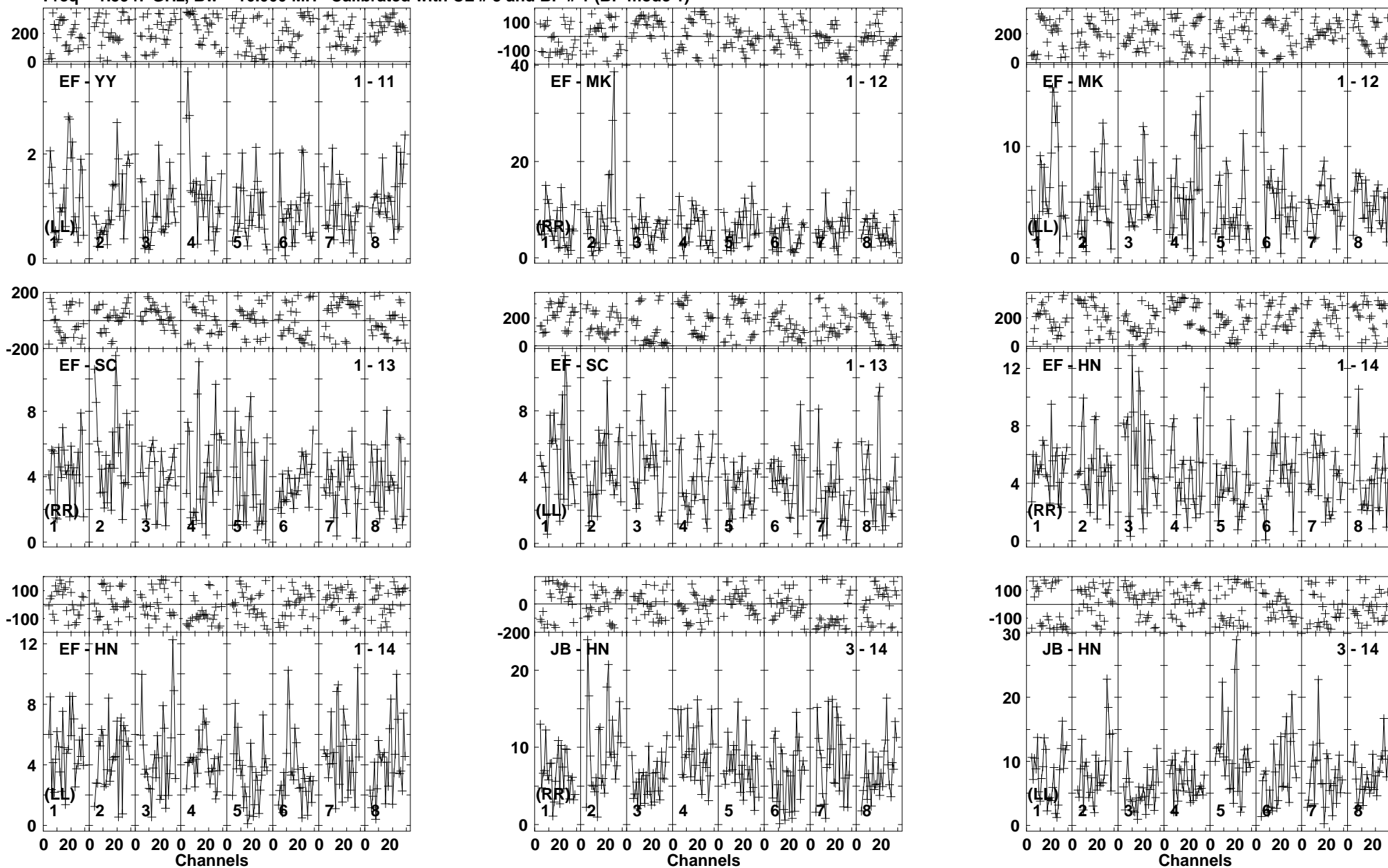
Lower frame: Milli Ampl Jy Top frame: Phas deg Vector averaged cross-power spectrum Baseline: EF (01) - YY (11) Timerange: 01/00:28:51 to 01/00:34:01
