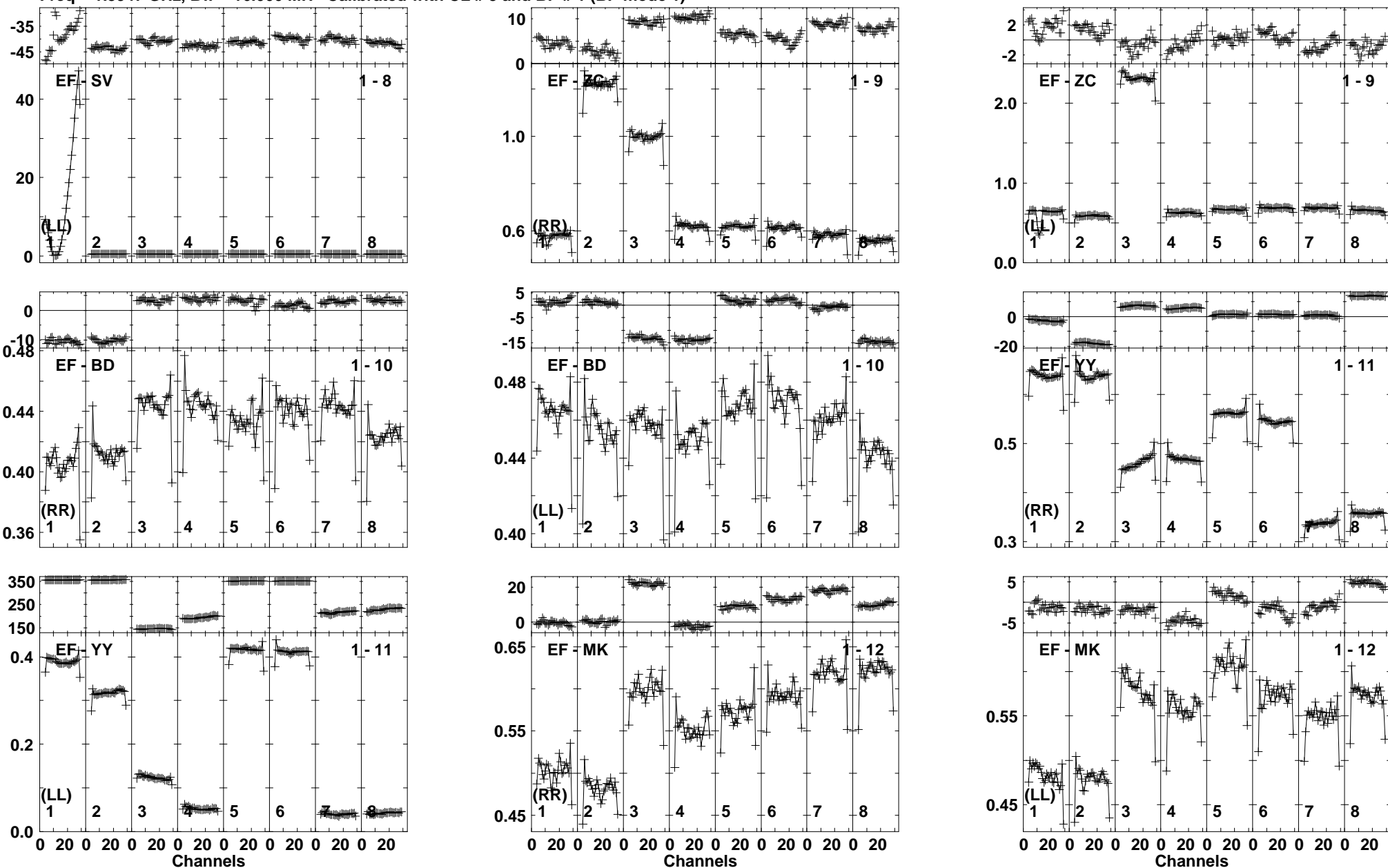
Lower frame: Ampl Jy Top frame: Phas deg Vector averaged cross-power spectrum Baseline: EF (01) - SV (08) Timerange: 00/22:09:59 to 00/22:11:48
