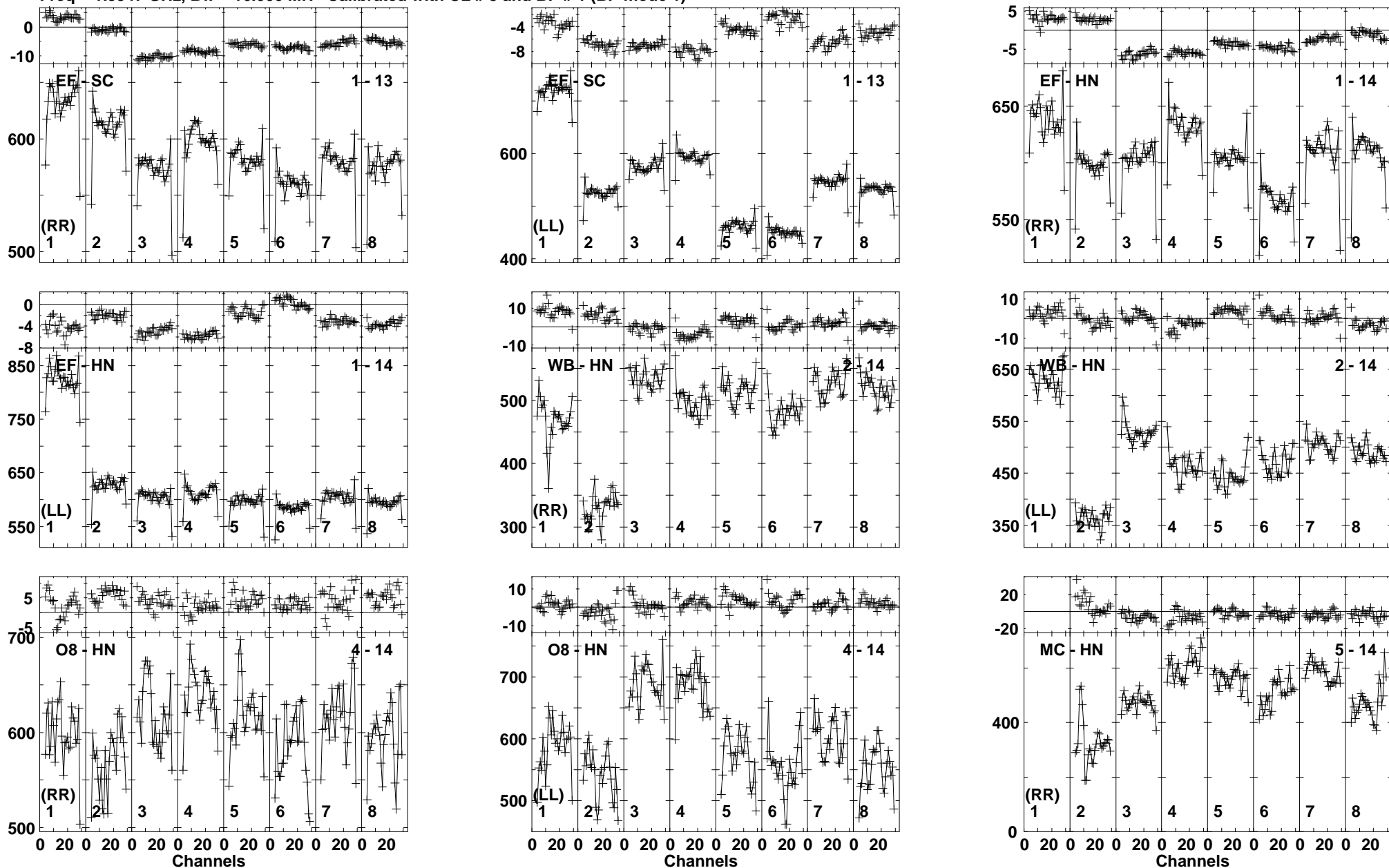
Lower frame: Milli Ampl Jy Top frame: Phas deg Vector averaged cross-power spectrum Baseline: EF (01) - SC (13) Timerange: 00/23:22:03 to 00/23:23:53
