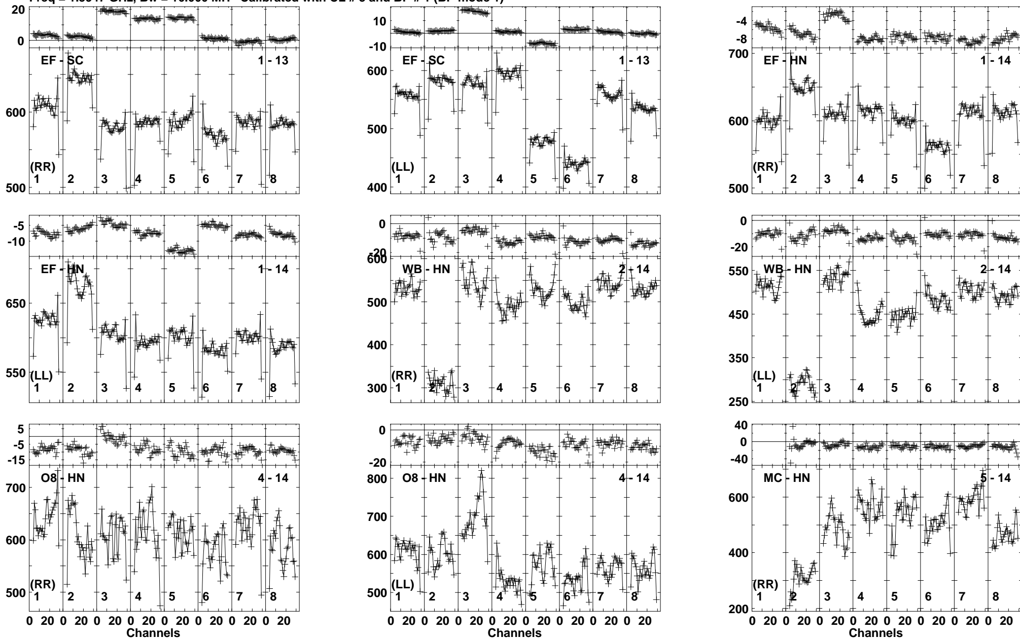
Lower frame: Milli Ampl Jy Top frame: Phas deg Vector averaged cross-power spectrum Baseline: EF (01) - SC (13) Timerange: 00/21:41:09 to 00/21:42:58
