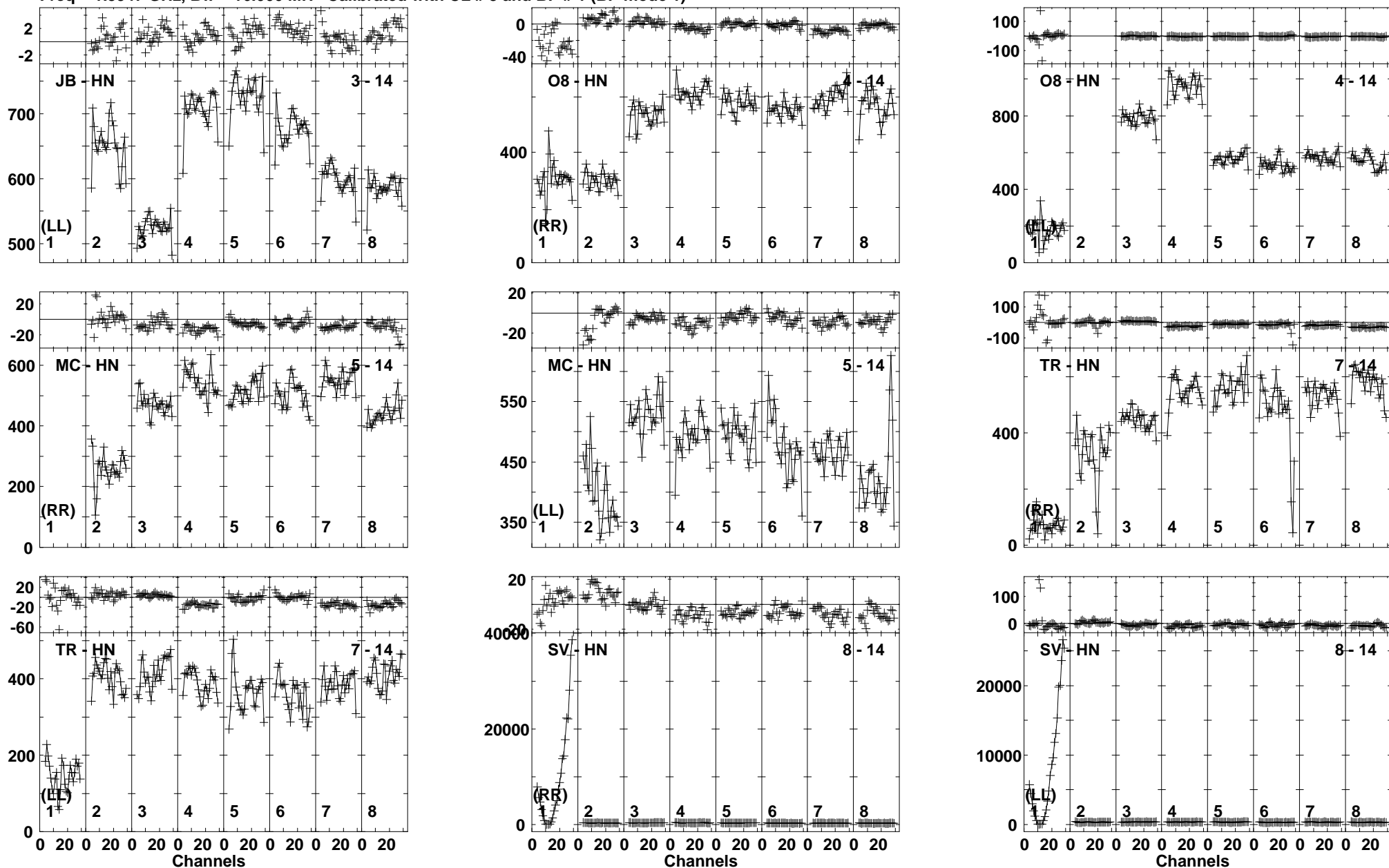
Lower frame: Milli Ampl Jy Top frame: Phas deg Vector averaged cross-power spectrum Baseline: JB (03) - HN (14) Timerange: 00/23:14:55 to 00/23:16:37
