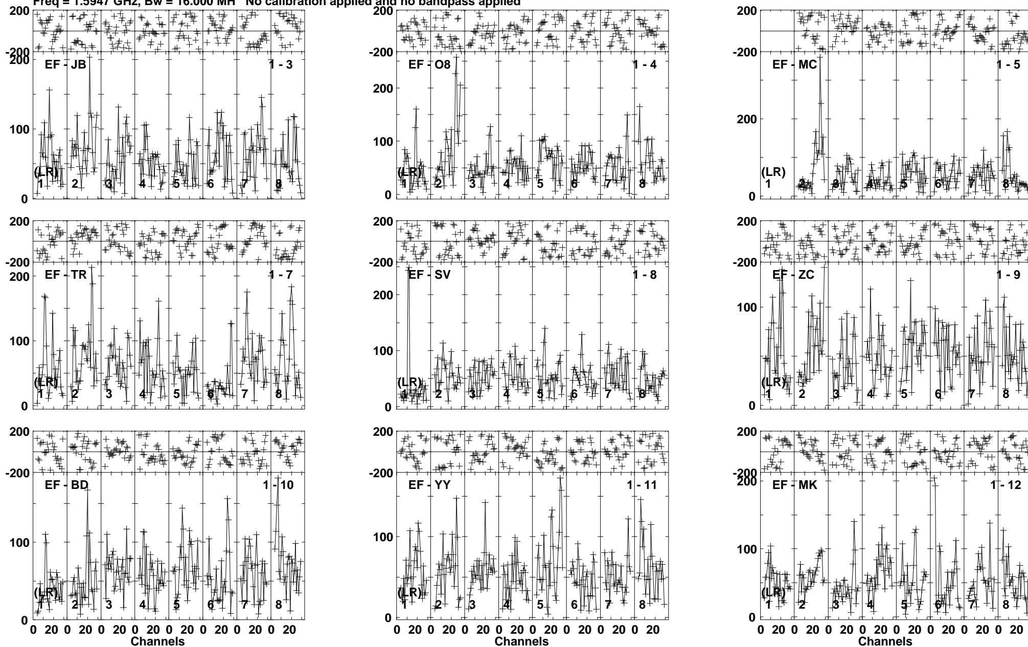
Lower frame: Micro Ampl Jy Top frame: Phas deg Vector averaged cross-power spectrum Baseline: EF (01) - JB (03) Timerange: 01/00:57:41 to 01/01:02:51
