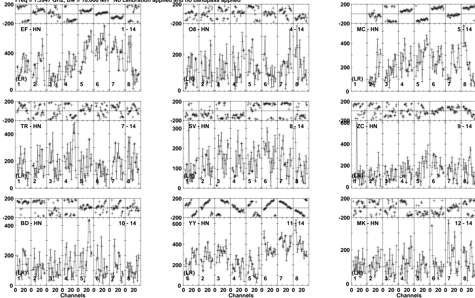
Lower frame: Micro Ampl Jy Top frame: Phas deg Vector averaged cross-power spectrum Baseline: EF (01) - HN (14) Timerange: 01/01:02:59 to 01/01:04:48
