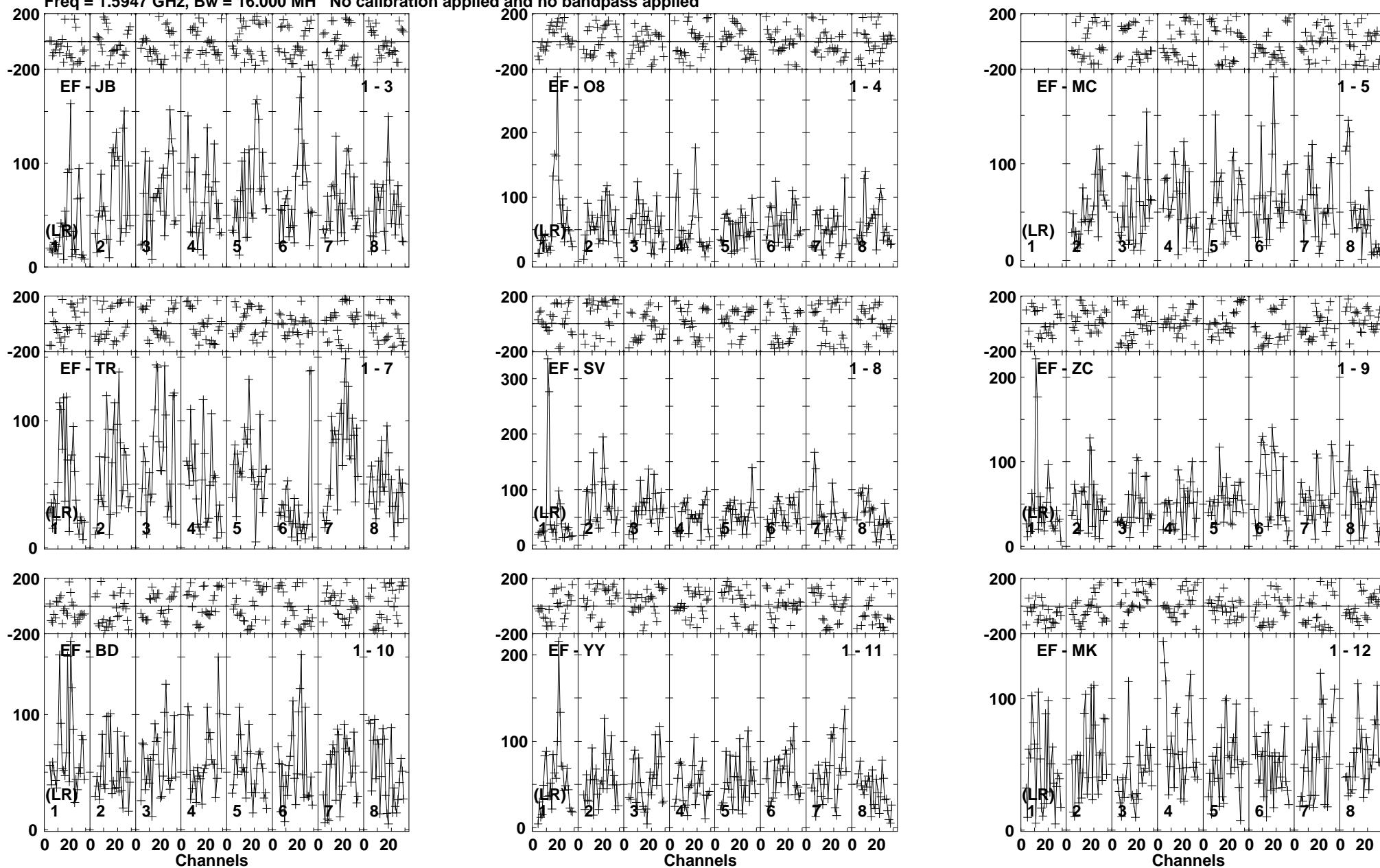
Lower frame: Micro Ampl Jy Top frame: Phas deg Vector averaged cross-power spectrum Baseline: EF (01) - JB (03) Timerange: 01/00:50:28 to 01/00:55:42
