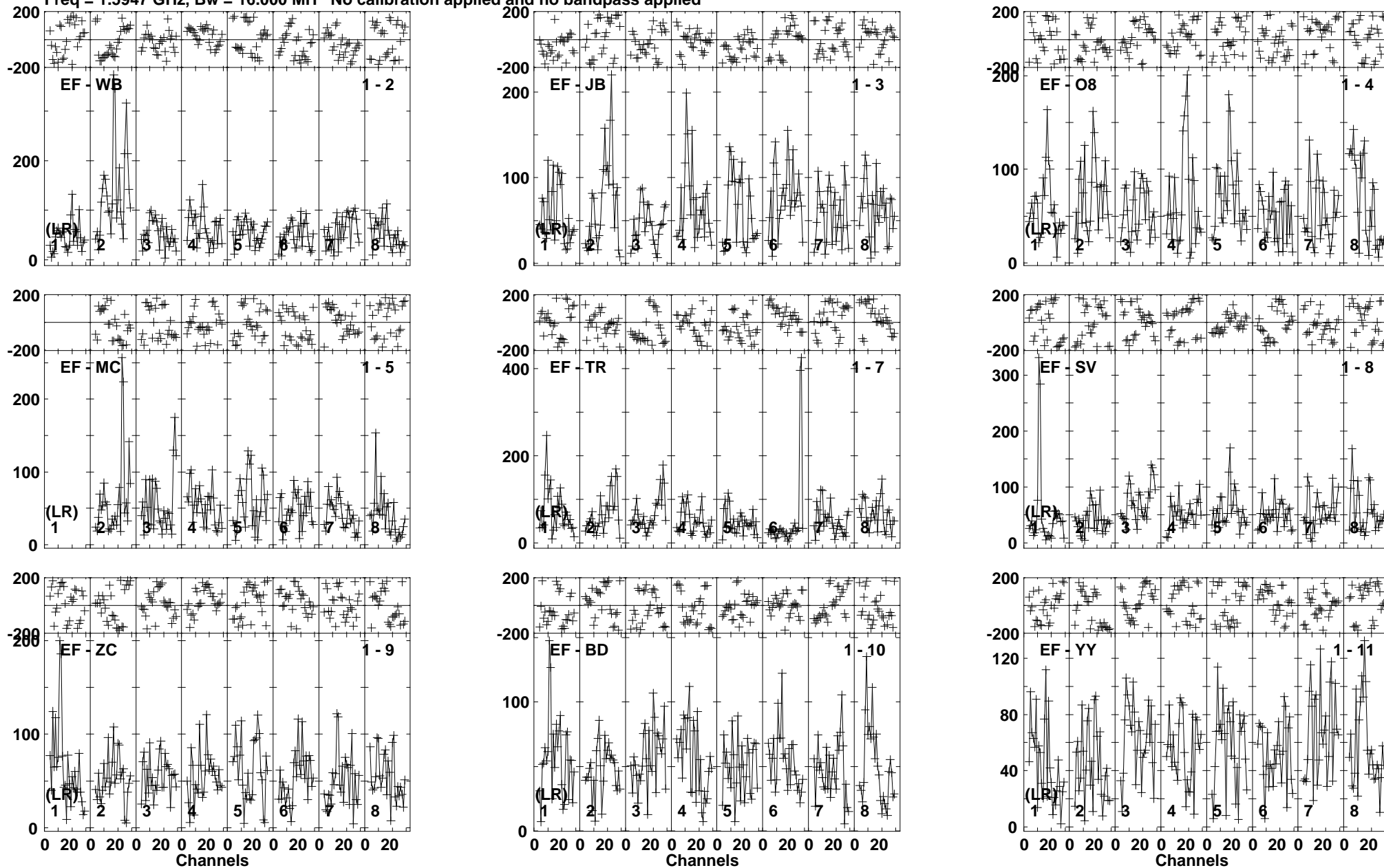
Lower frame: Micro Ampl Jy Top frame: Phas deg Vector averaged cross-power spectrum Baseline: EF (01) - WB (02) Timerange: 00/21:50:16 to 00/21:55:26
