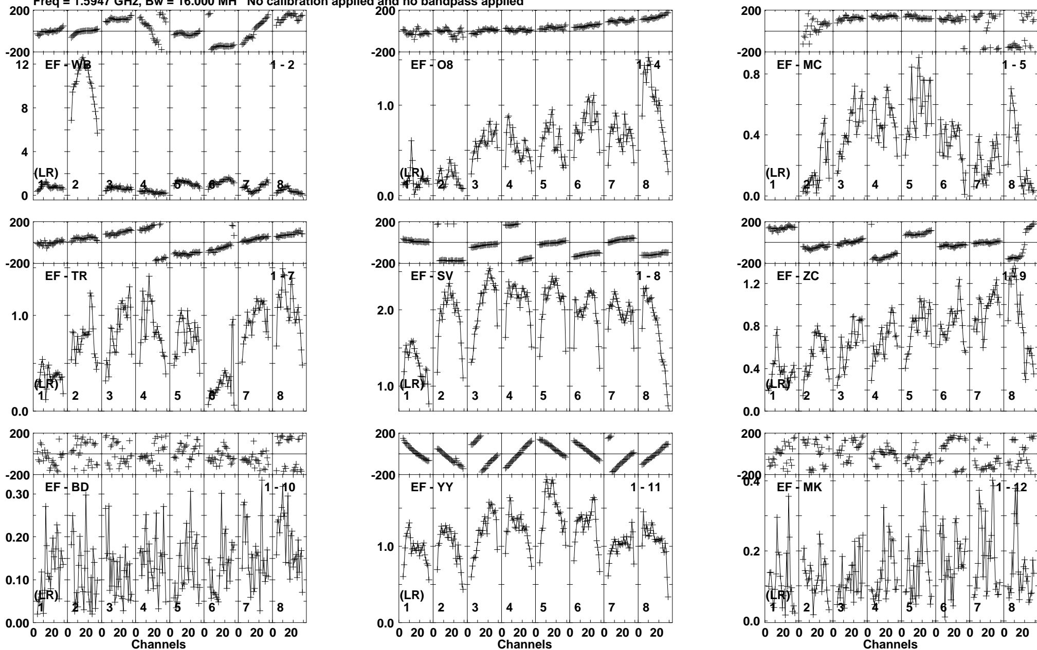
Lower frame: Milli Ampl Jy Top frame: Phas deg Vector averaged cross-power spectrum Baseline: EF (01) - WB (02) Timerange: 00/23:07:38 to 00/23:09:28
