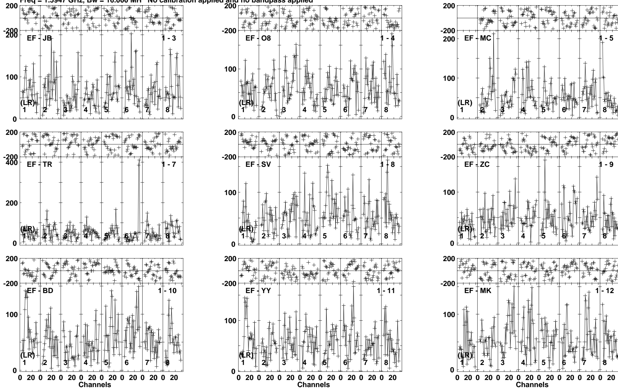
Lower frame: Micro Ampl Jy Top frame: Phas deg Vector averaged cross-power spectrum Baseline: EF (01) - JB (03) Timerange: 00/23:45:35 to 00/23:50:45
