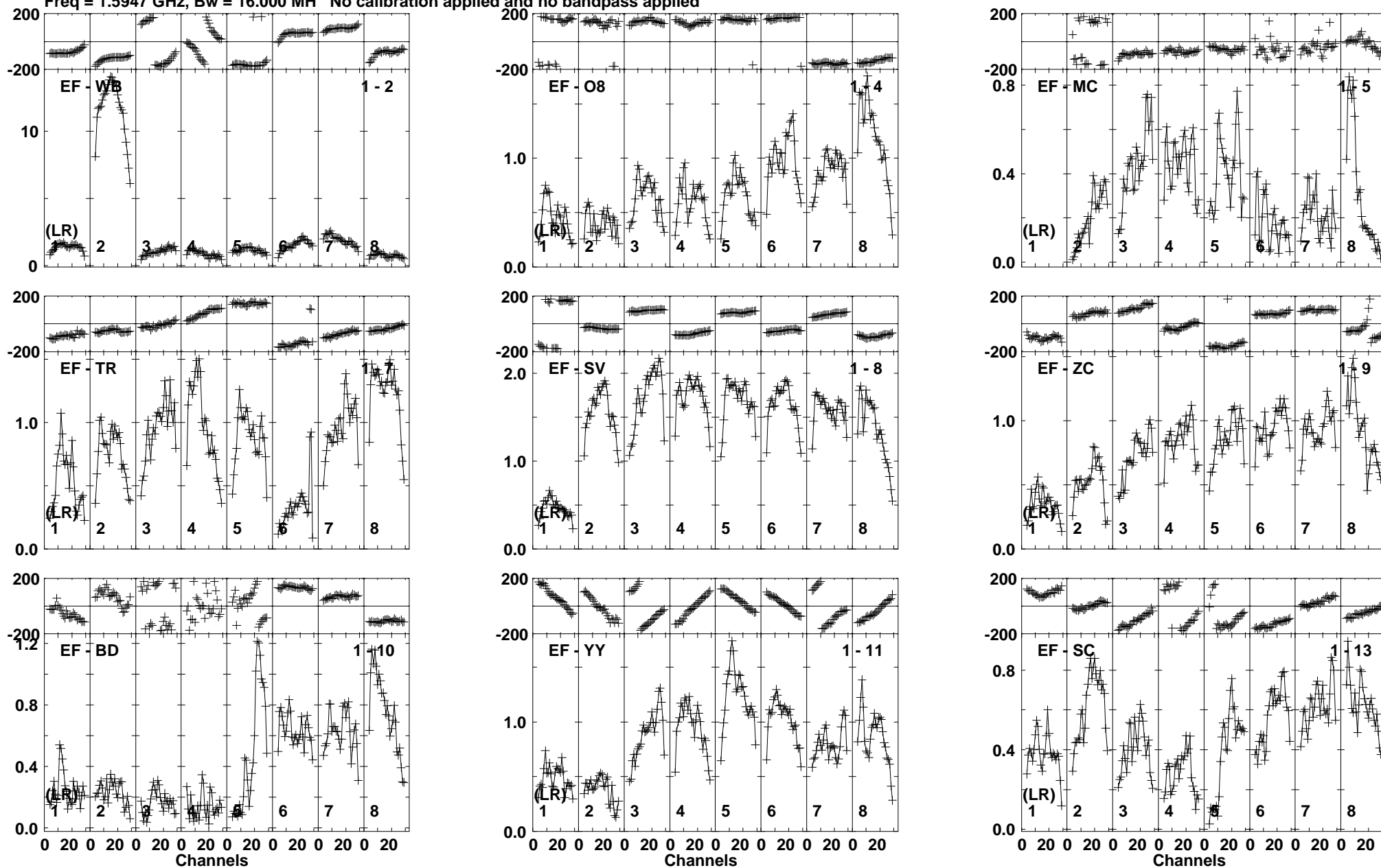
Lower frame: Milli Ampl Jy Top frame: Phas deg Vector averaged cross-power spectrum Baseline: EF (01) - WB (02) Timerange: 00/20:14:39 to 00/20:16:28
