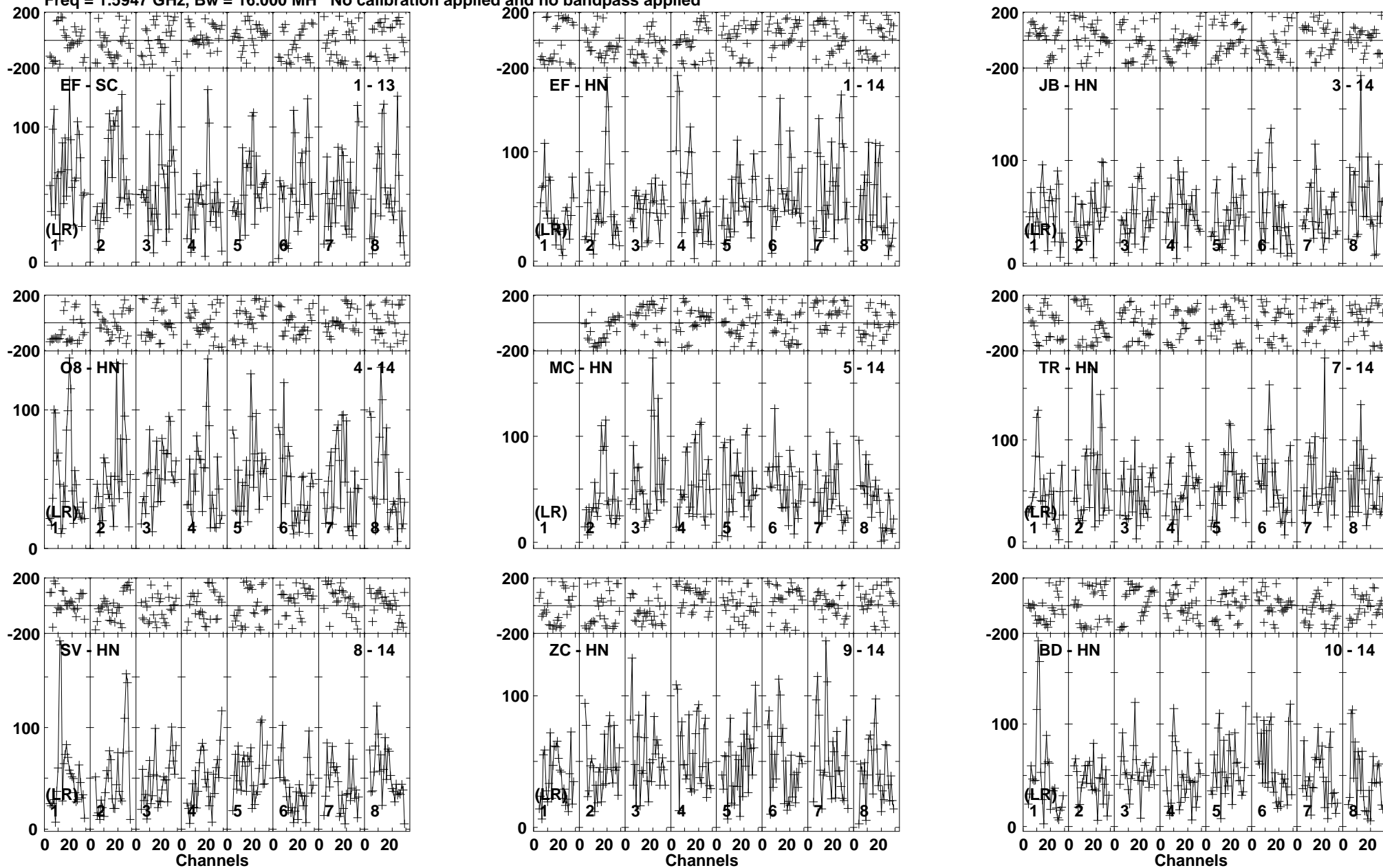
Lower frame: Micro Ampl Jy Top frame: Phas deg Vector averaged cross-power spectrum Baseline: EF (01) - SC (13) Timerange: 01/01:19:18 to 01/01:24:32
