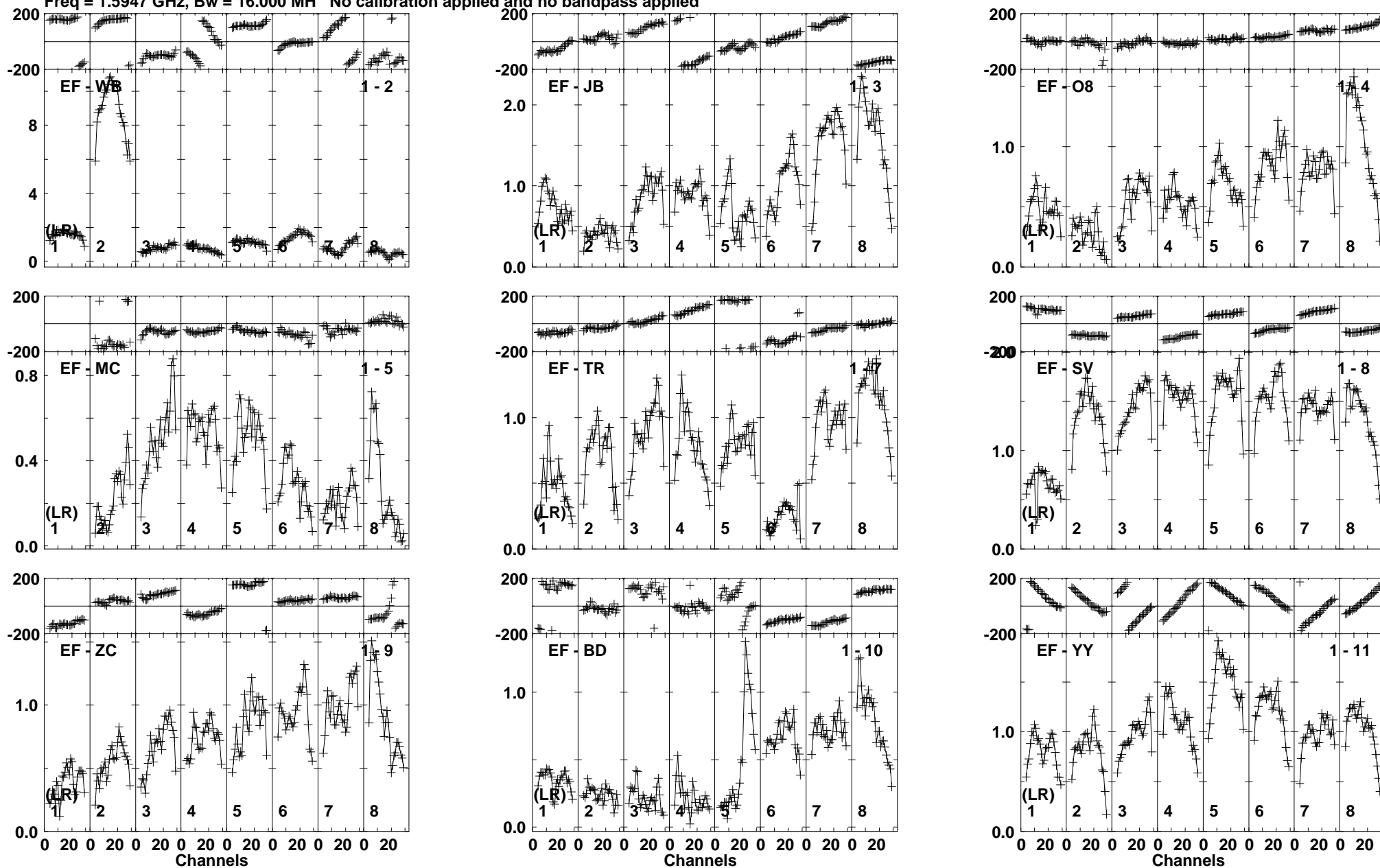
Lower frame: Milli Ampl Jy Top frame: Phas deg Vector averaged cross-power spectrum Baseline: EF (01) - WB (02) Timerange: 00/22:17:15 to 00/22:18:57
