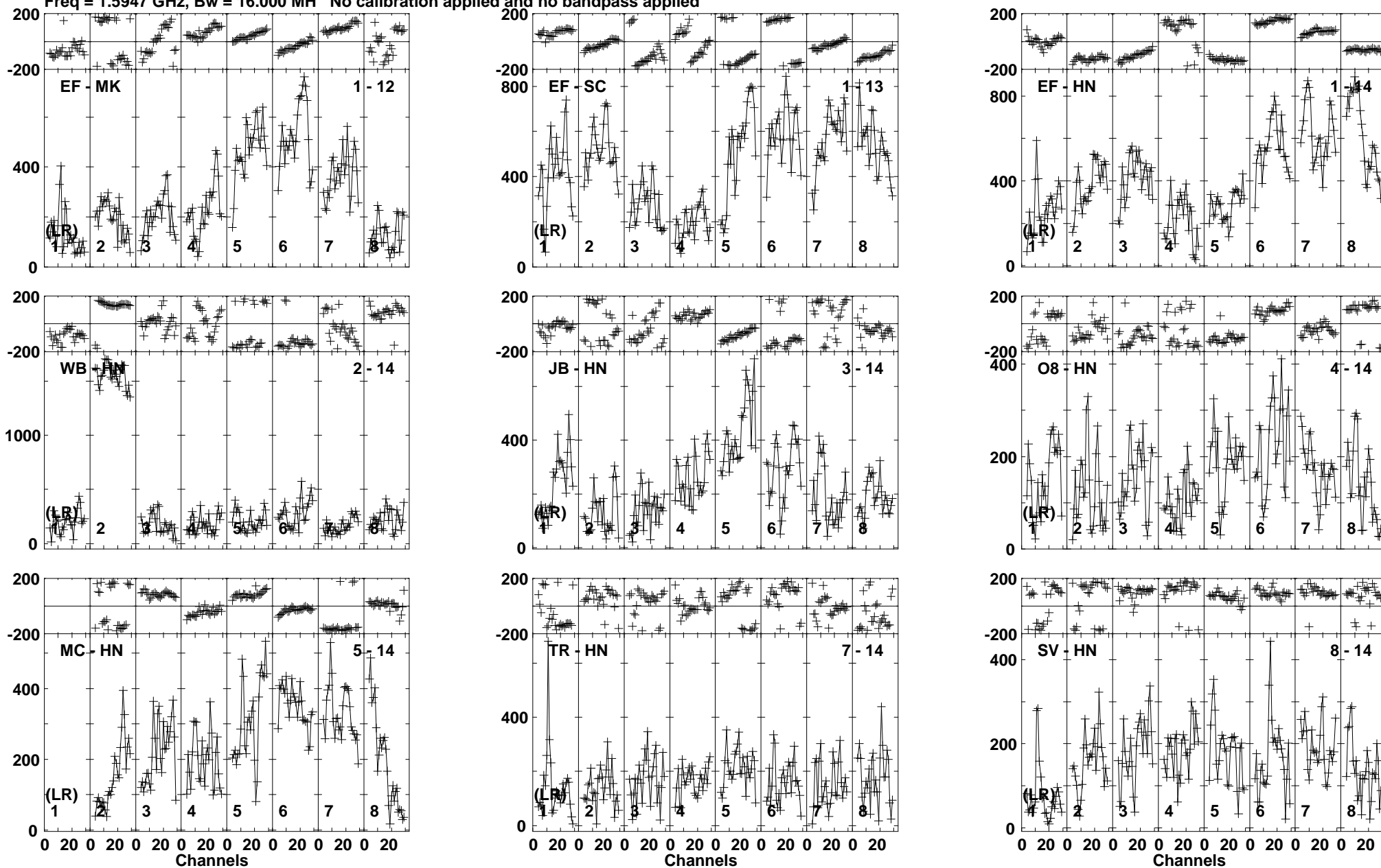
Lower frame: Micro Ampl Jy Top frame: Phas deg Vector averaged cross-power spectrum Baseline: EF (01) - MK (12) Timerange: 00/22:02:51 to 00/22:04:32
