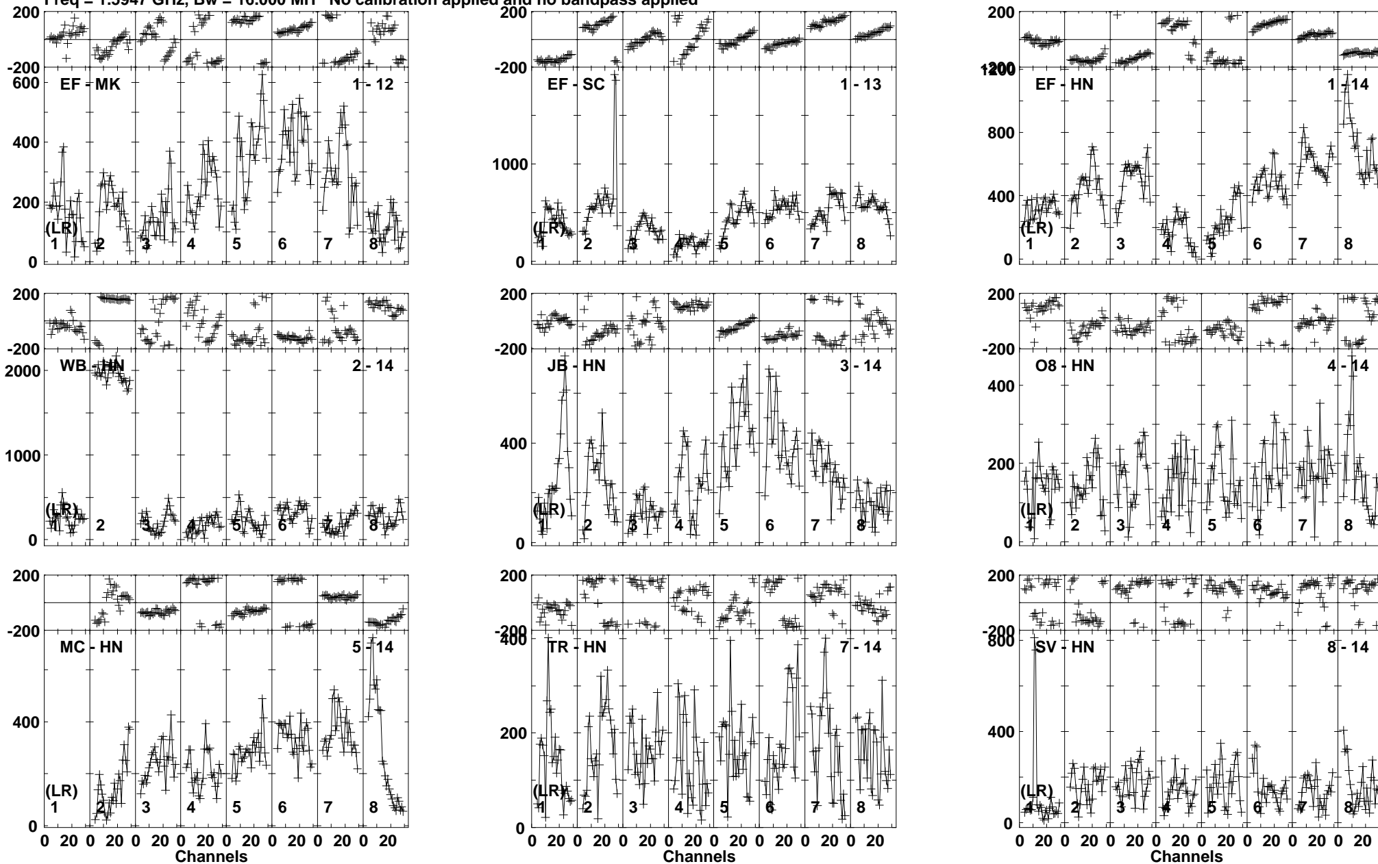
Lower frame: Micro Ampl Jy Top frame: Phas deg Vector averaged cross-power spectrum Baseline: EF (01) - MK (12) Timerange: 00/21:48:26 to 00/21:50:07
