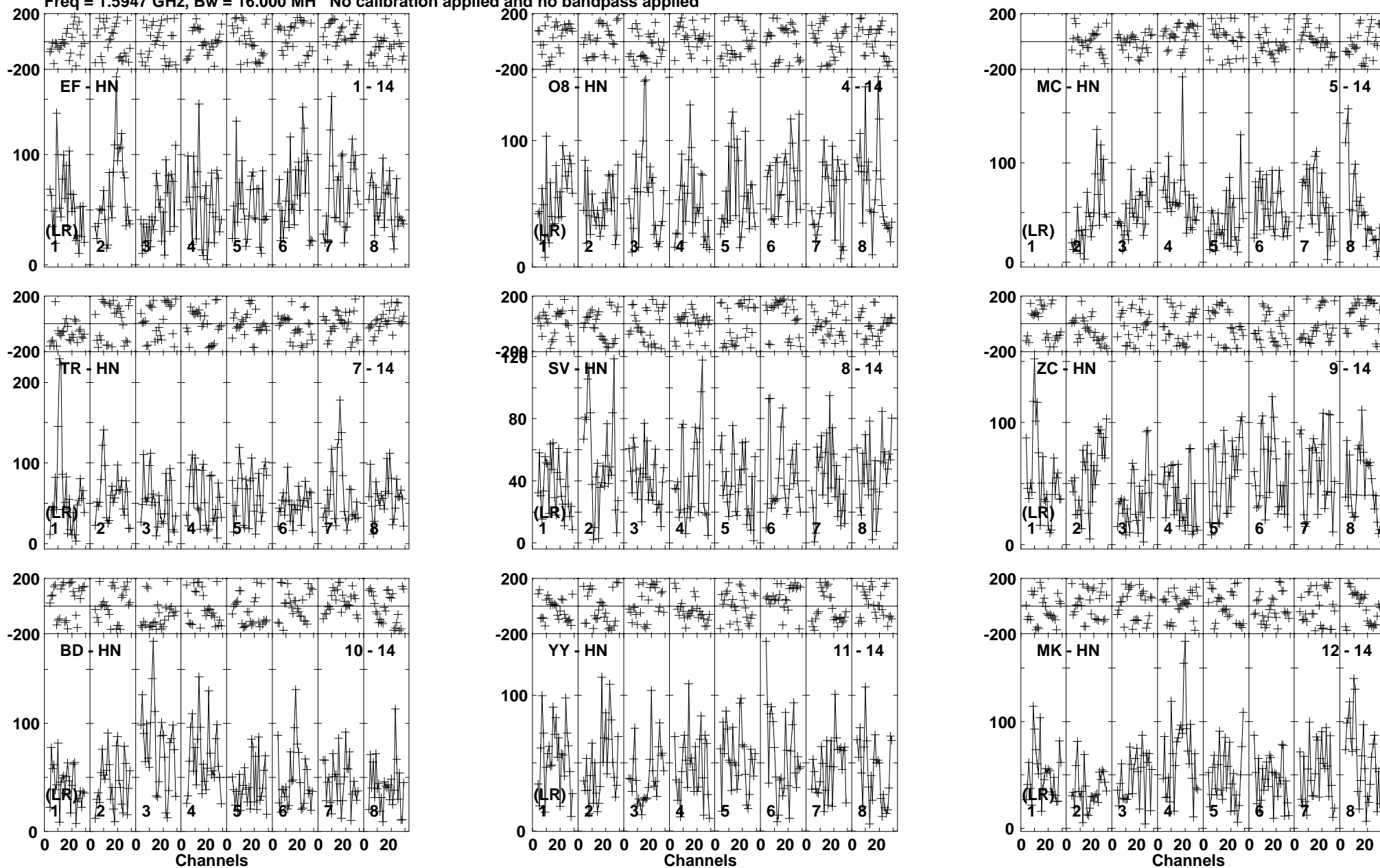
Lower frame: Micro Ampl Jy Top frame: Phas deg Vector averaged cross-power spectrum Baseline: EF (01) - HN (14) Timerange: 01/01:48:11 to 01/01:53:23
