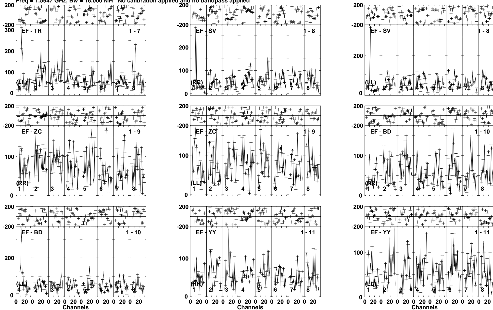
Lower frame: Micro Ampl Jy Top frame: Phas deg Vector averaged cross-power spectrum Baseline: EF (01) - TR (07) Timerange: 00/21:50:16 to 00/21:55:26
