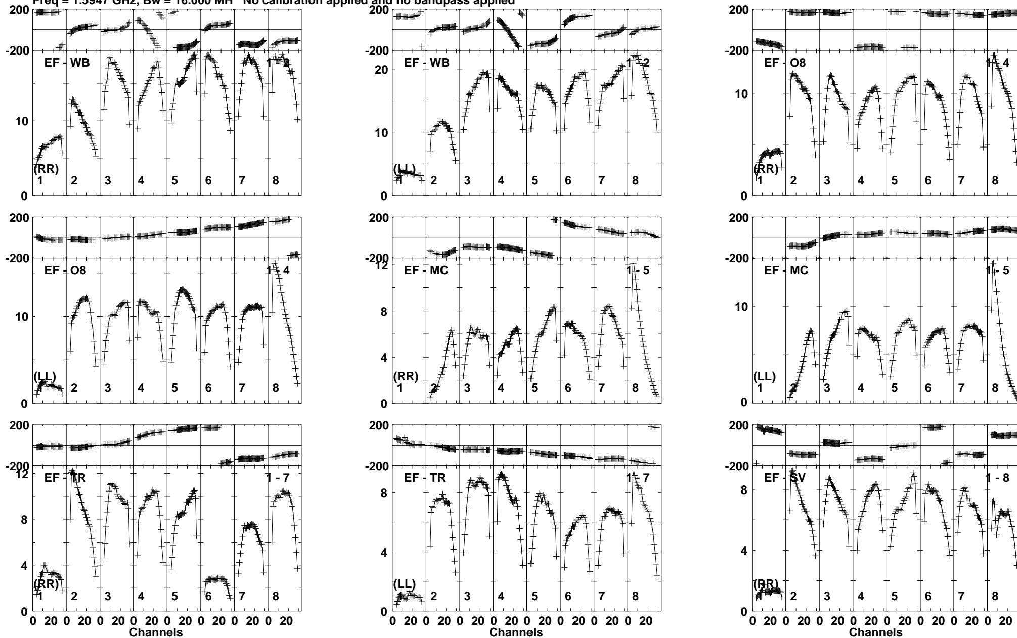
Lower frame: Milli Ampl Jy Top frame: Phas deg Vector averaged cross-power spectrum Baseline: EF (01) - WB (02) Timerange: 00/20:57:54 to 00/20:59:43
