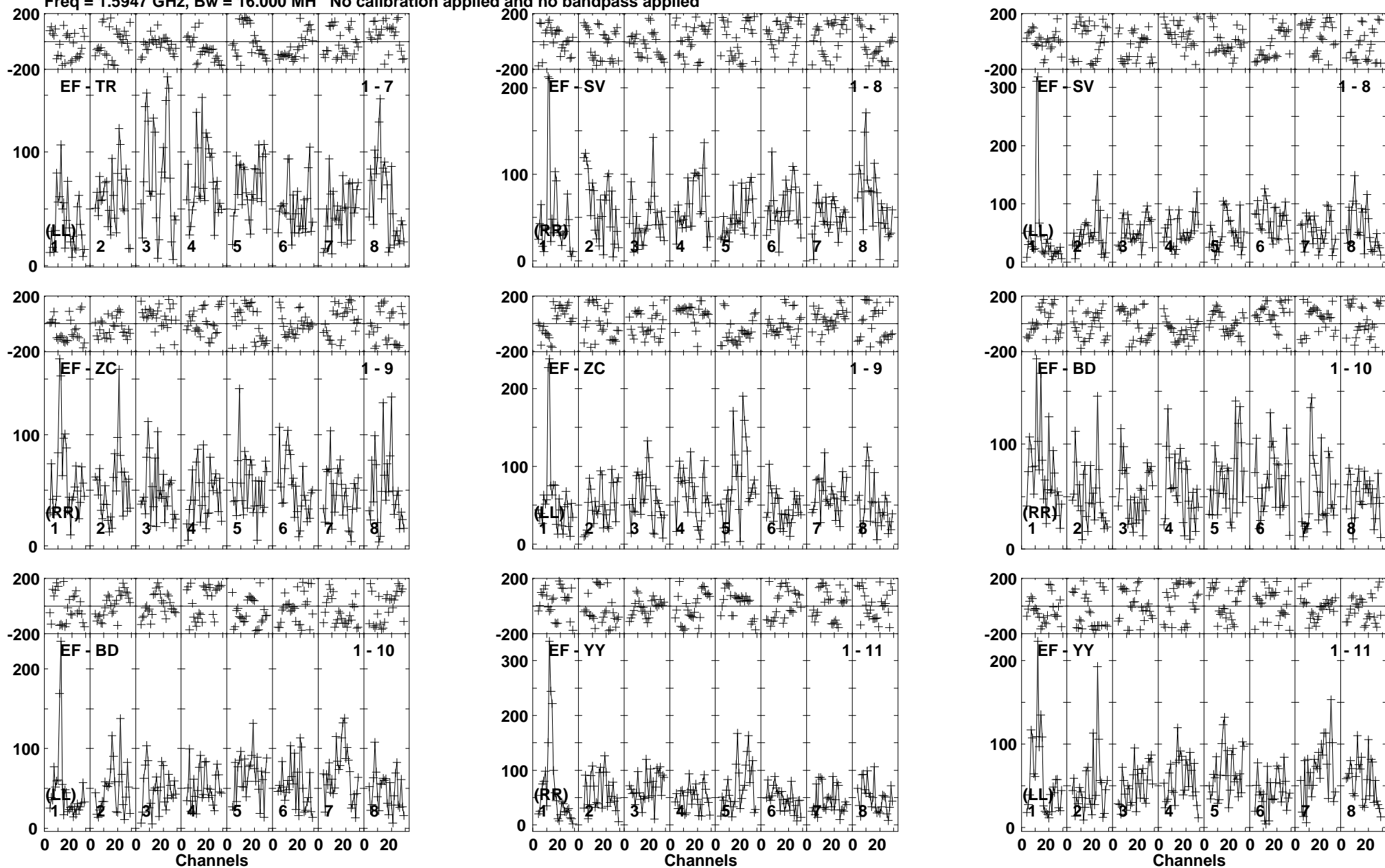
Lower frame: Micro Ampl Jy Top frame: Phas deg Vector averaged cross-power spectrum Baseline: EF (01) - TR (07) Timerange: 00:22:40:43 to 00:22:45:57
