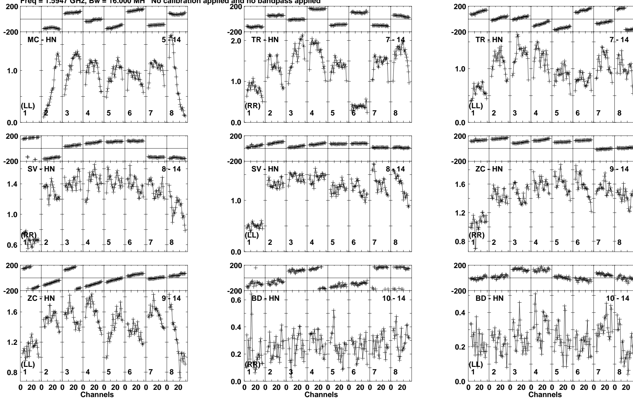
Lower frame: Milli Ampl Jy Top frame: Phas deg Vector averaged cross-power spectrum Baseline: MC (05) - HN (14) Timerange: 00/22:53:13 to 00/22:55:03
