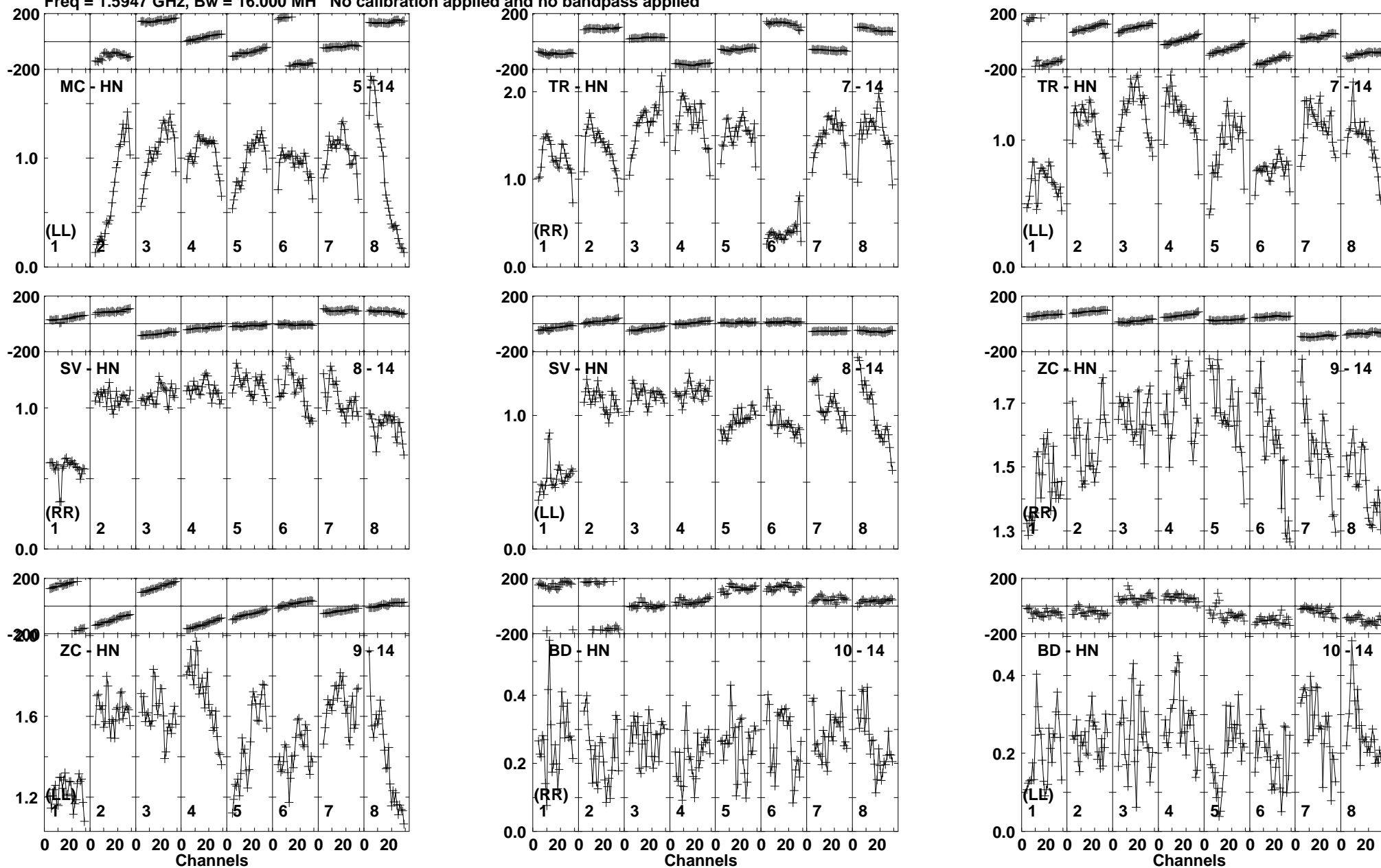
Lower frame: Milli Ampl Jy Top frame: Phas deg Vector averaged cross-power spectrum Baseline: MC (05) - HN (14) Timerange: 00:23:43:45 to 00:23:45:27
