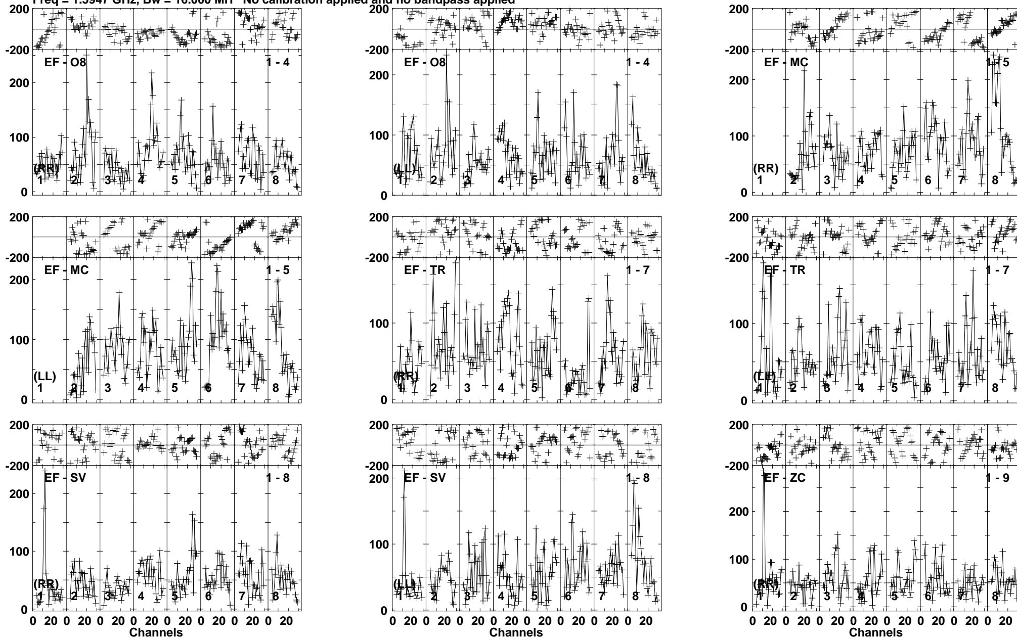
Lower frame: Micro Ampl Jy Top frame: Phas deg Vector averaged cross-power spectrum Baseline: EF (01) - O8 (04) Timerange: 01/01:48:11 to 01/01:53:23
