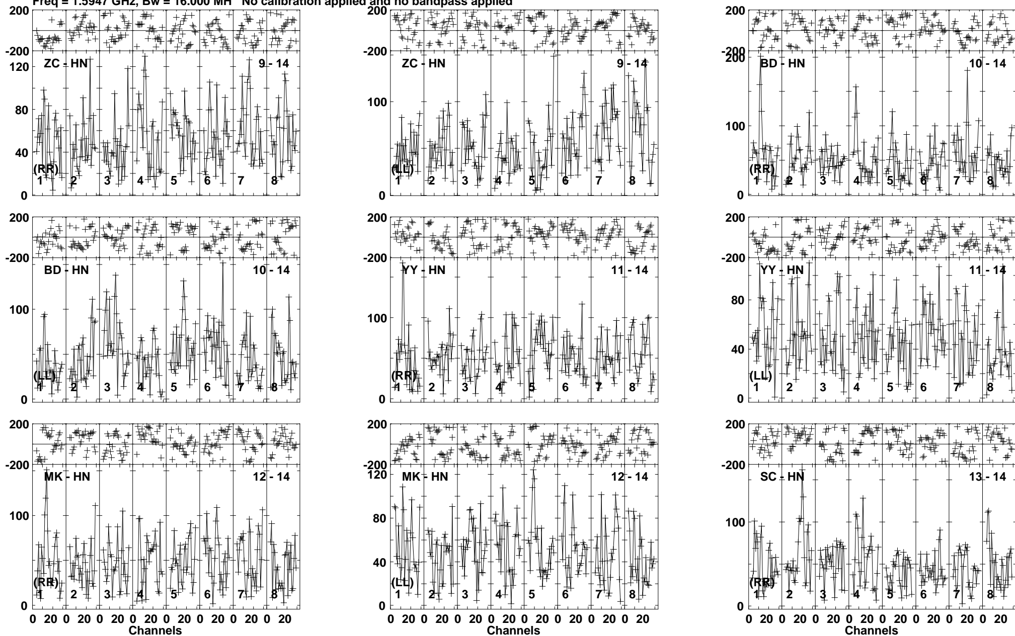
Lower frame: Micro Ampl Jy Top frame: Phas deg Vector averaged cross-power spectrum Baseline: ZC (09) - HN (14) Timerange: 00/22:11:53 to 00/22:17:07
