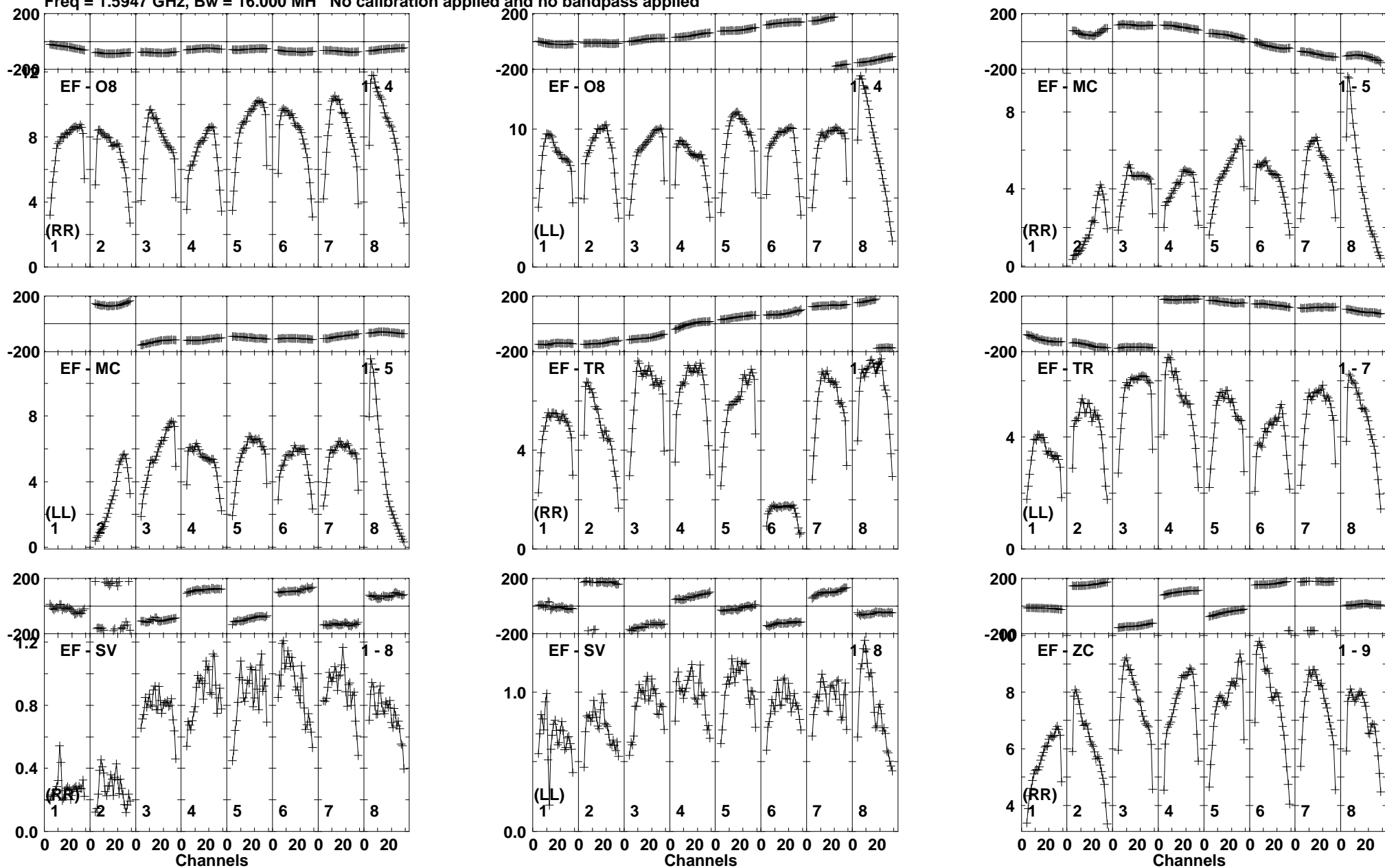
Lower frame: Milli Ampl Jy Top frame: Phas deg Vector averaged cross-power spectrum Baseline: EF (01) - O8 (04) Timerange: 01/01:31:49 to 01/01:33:38
