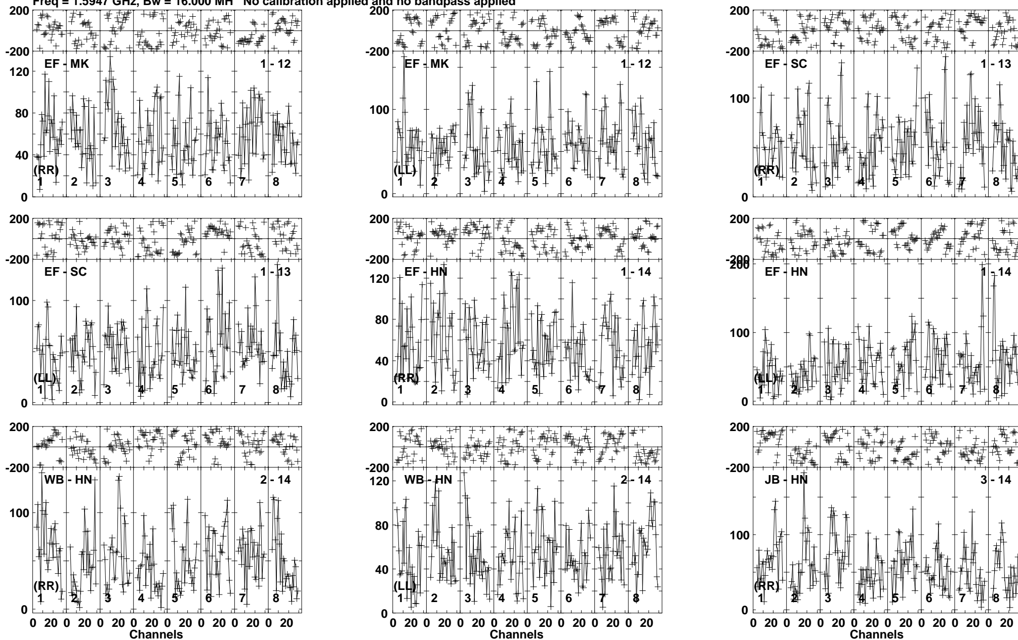
Lower frame: Micro Ampl Jy Top frame: Phas deg Vector averaged cross-power spectrum Baseline: EF (01) - MK (12) Timerange: 00/21:35:51 to 00/21:41:01
