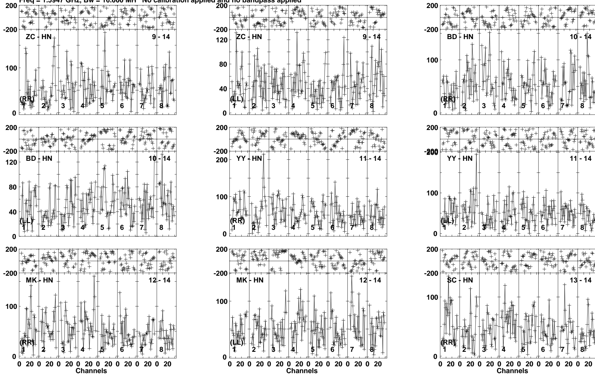
Lower frame: Micro Ampl Jy Top frame: Phas deg Vector averaged cross-power spectrum Baseline: ZC (09) - HN (14) Timerange: 00/23:38:23 to 00/23:43:37
