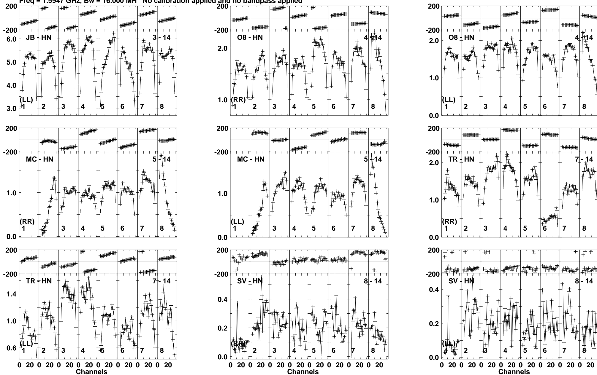
Lower frame: Milli Ampl Jy Top frame: Phas deg Vector averaged cross-power spectrum Baseline: JB (03) - HN (14) Timerange: 00/20:50:46 to 00/20:52:27
