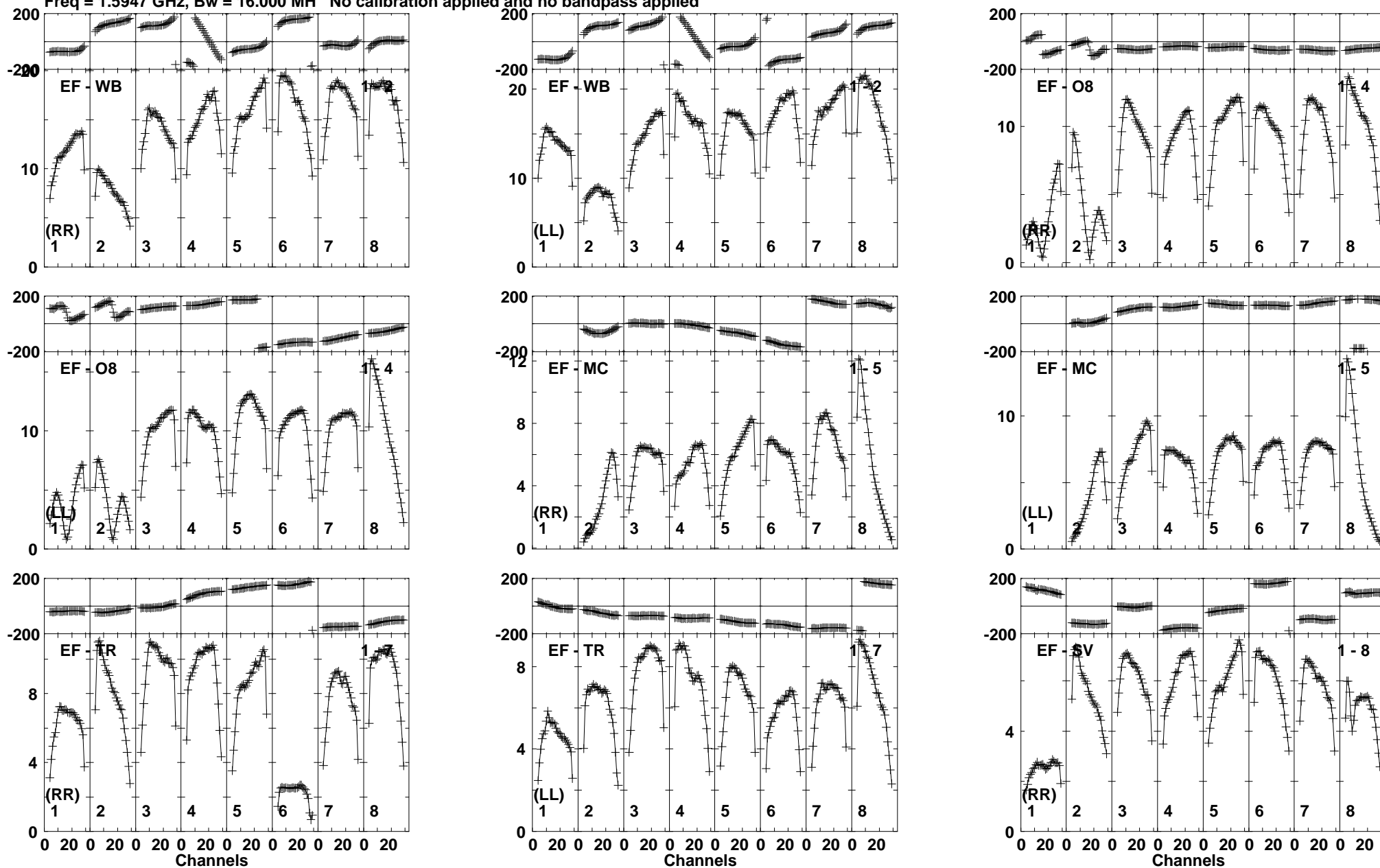
Lower frame: Milli Ampl Jy Top frame: Phas deg Vector averaged cross-power spectrum Baseline: EF (01) - WB (02) Timerange: 00/21:26:44 to 00/21:28:33
