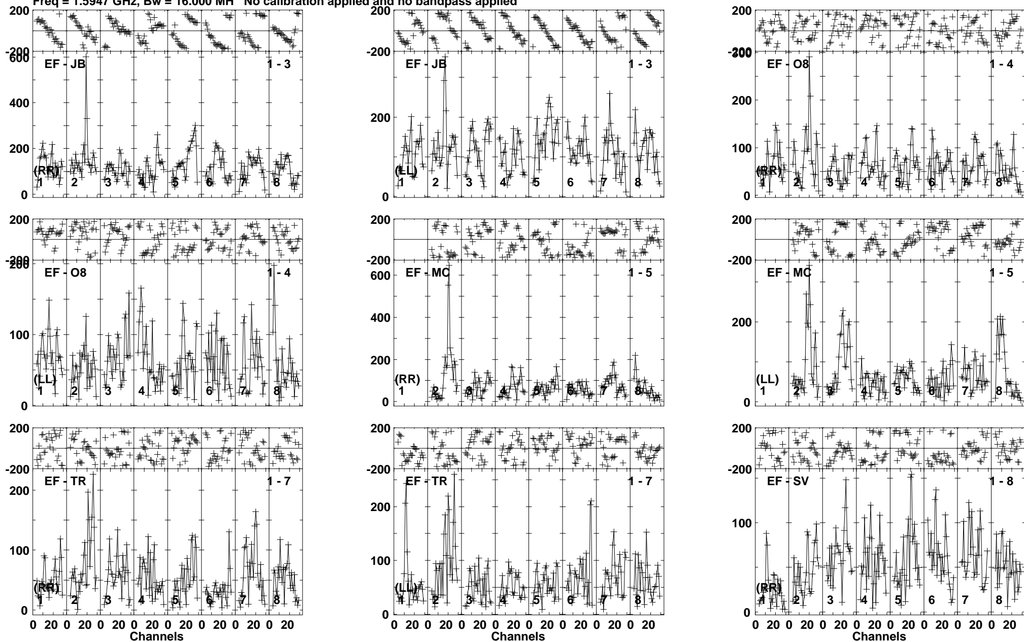
Lower frame: Micro Ampl Jy Top frame: Phas deg Vector averaged cross-power spectrum Baseline: EF (01) - JB (03) Timerange: 01/01:04:53 to 01/01:10:07
