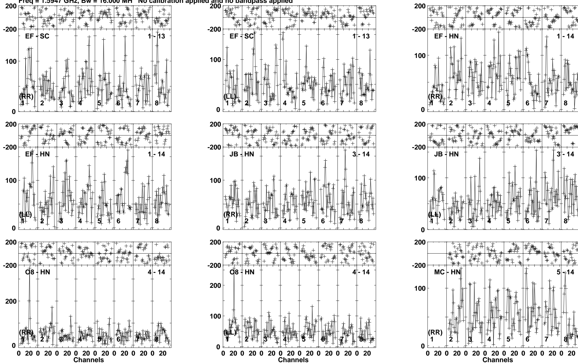
Lower frame: Micro Ampl Jy Top frame: Phas deg Vector averaged cross-power spectrum Baseline: EF (01) - SC (13) Timerange: 01/00:57:41 to 01/01:02:51
