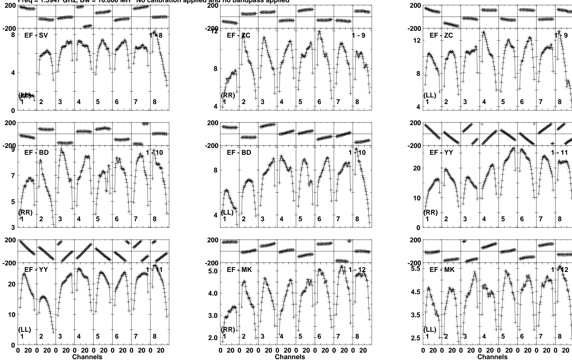
Lower frame: Milli Ampl Jy Top frame: Phas deg Vector averaged cross-power spectrum Baseline: EF (01) - SV (08) Timerange: 00/21:26:44 to 00/21:28:33
