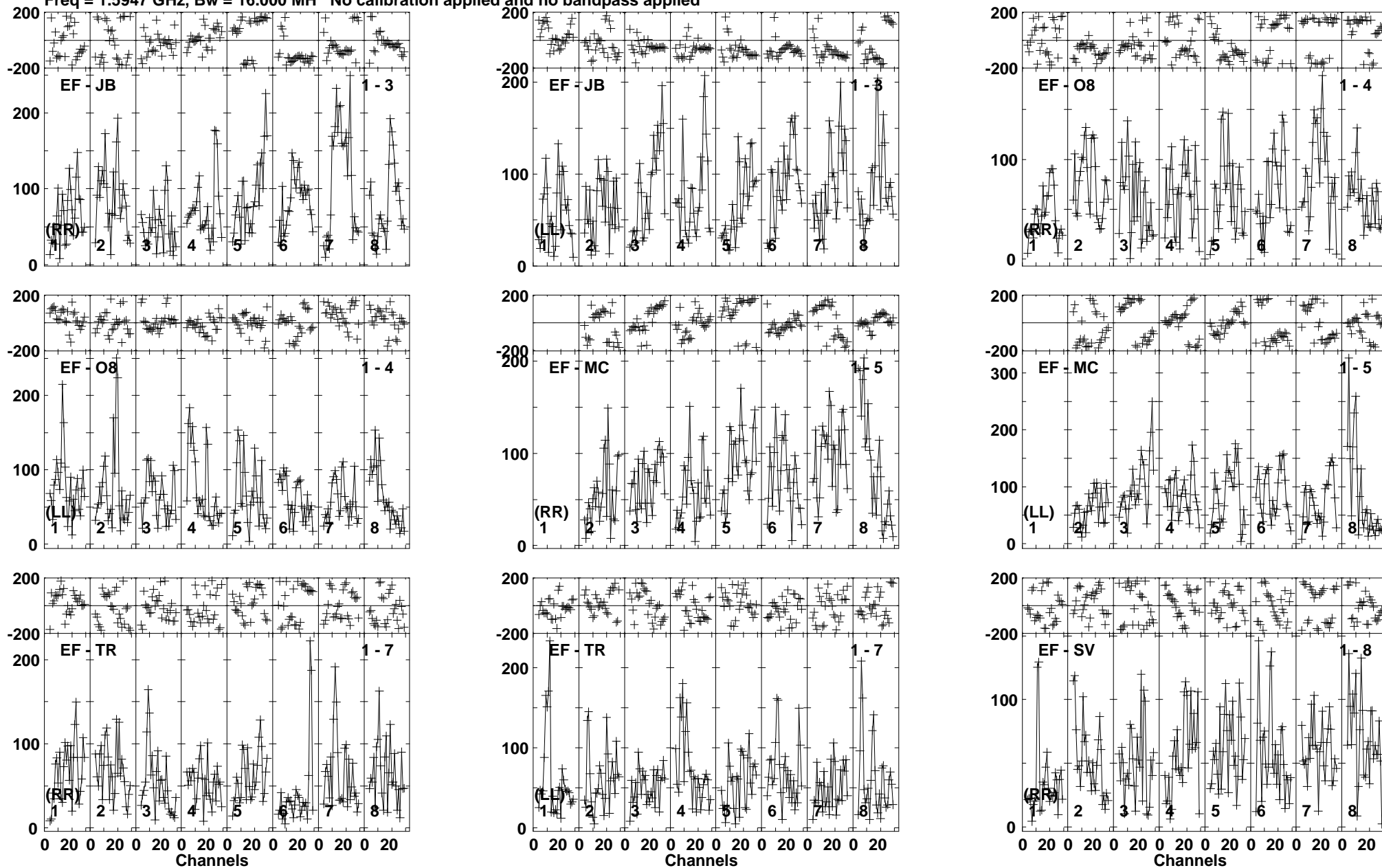
Lower frame: Micro Ampl Jy Top frame: Phas deg Vector averaged cross-power spectrum Baseline: EF (01) - JB (03) Timerange: 01/01:26:31 to 01/01:31:41
