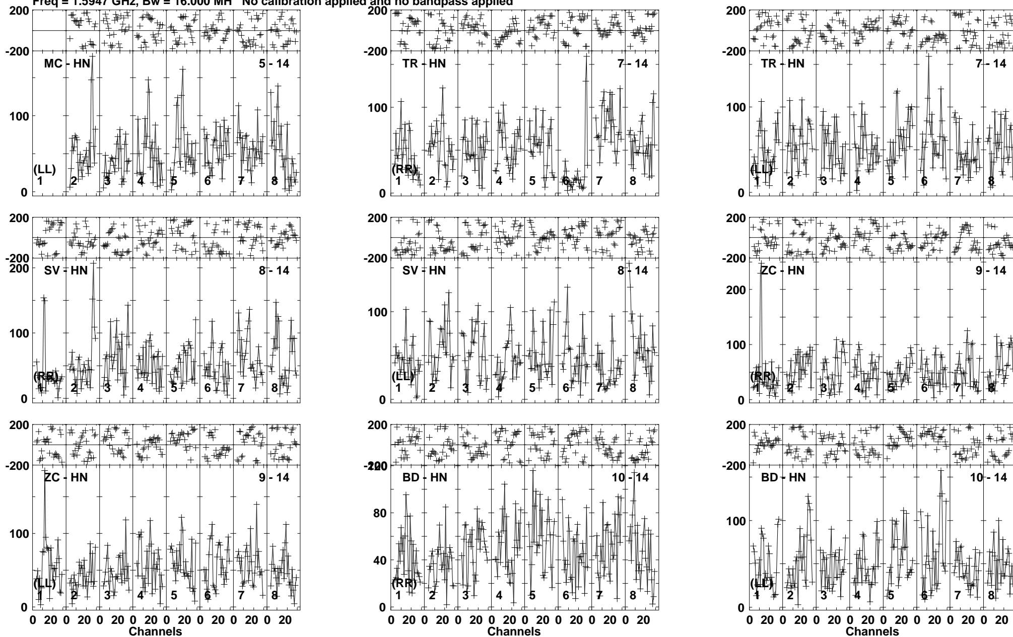
Lower frame: Micro Ampl Jy Top frame: Phas deg Vector averaged cross-power spectrum Baseline: MC (05) - HN (14) Timerange: 01/01:40:56 to 01/01:46:06
