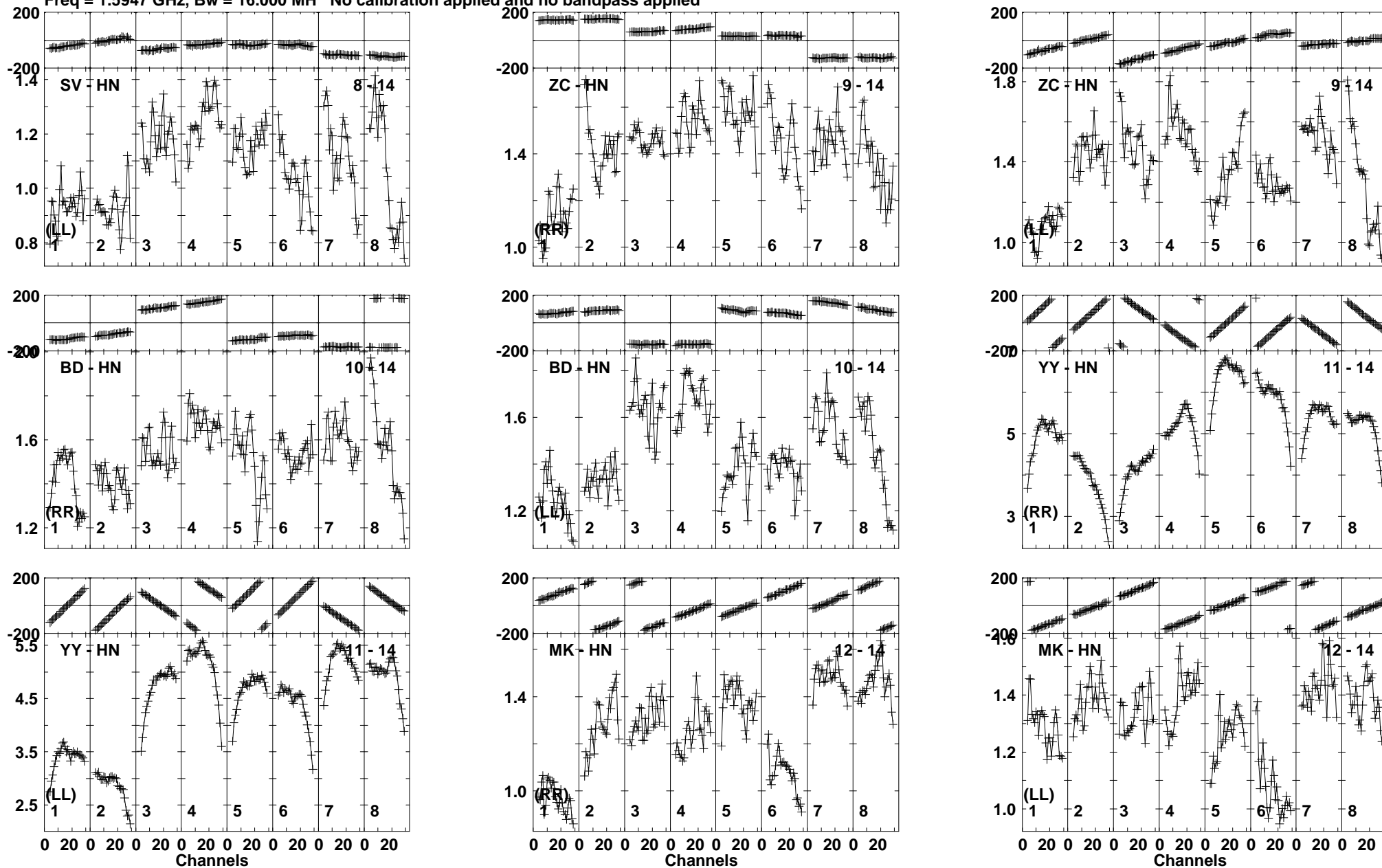
Lower frame: Milli Ampl Jy Top frame: Phas deg Vector averaged cross-power spectrum Baseline: SV (08) - HN (14) Timerange: 01/01:17:24 to 01/01:19:13
