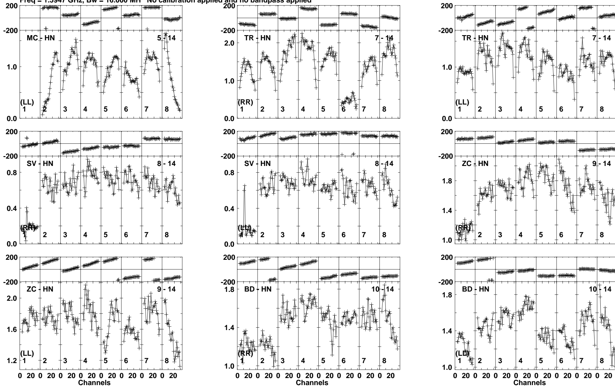
Lower frame: Milli Ampl Jy Top frame: Phas deg Vector averaged cross-power spectrum Baseline: MC (05) - HN (14) Timerange: 00/20:29:04 to 00/20:30:53
