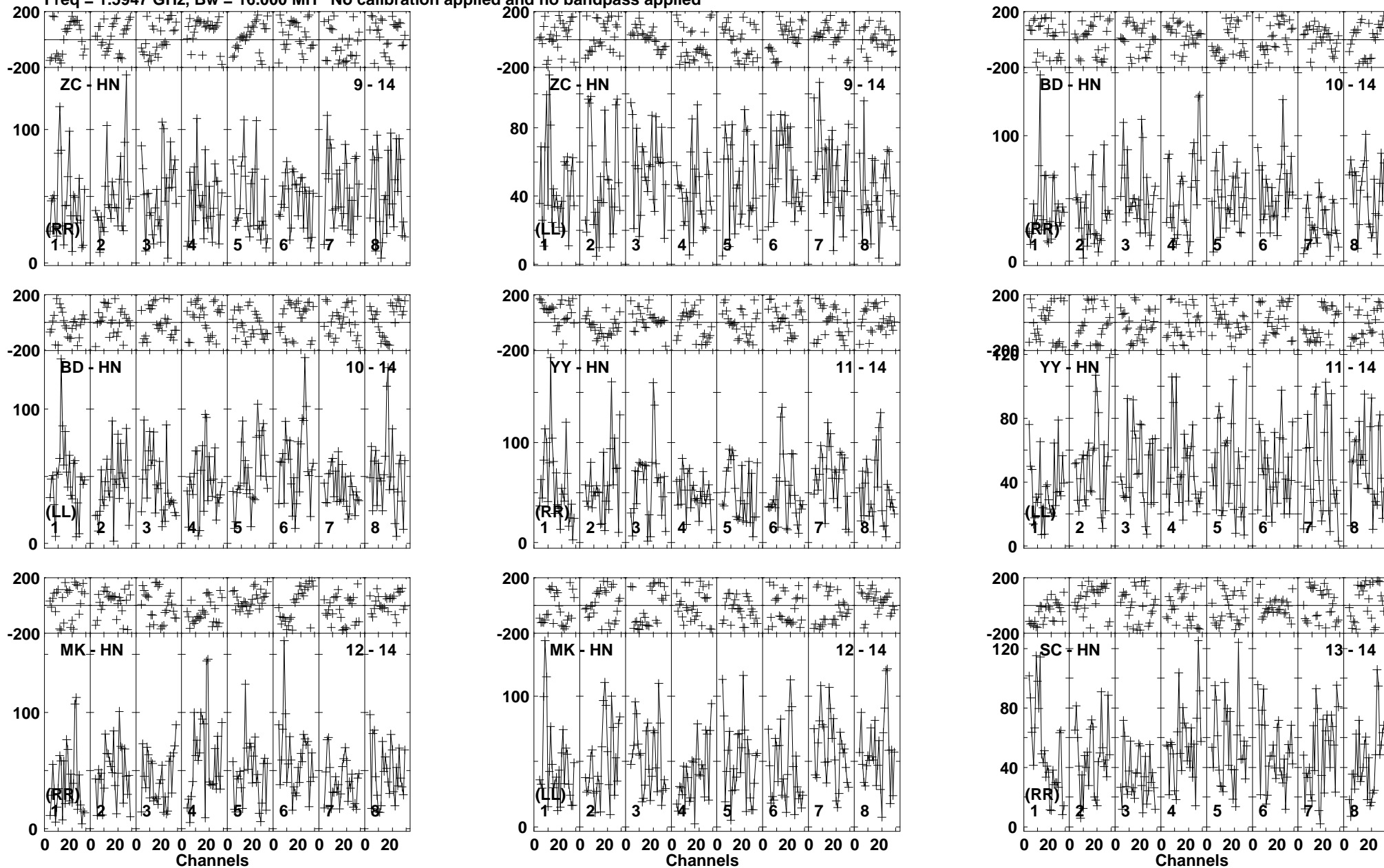
Lower frame: Micro Ampl Jy Top frame: Phas deg Vector averaged cross-power spectrum Baseline: ZC (09) - HN (14) Timerange: 00/23:02:20 to 00/23:07:30
