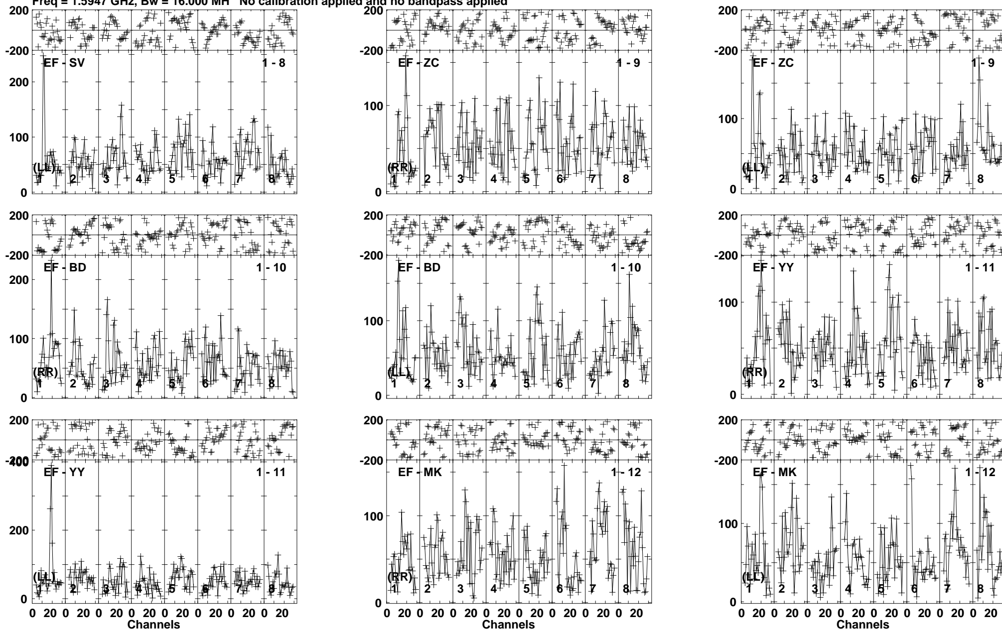
Lower frame: Micro Ampl Jy Top frame: Phas deg Vector averaged cross-power spectrum Baseline: EF (01) - SV (08) Timerange: 01/00:50:28 to 01/00:55:42
