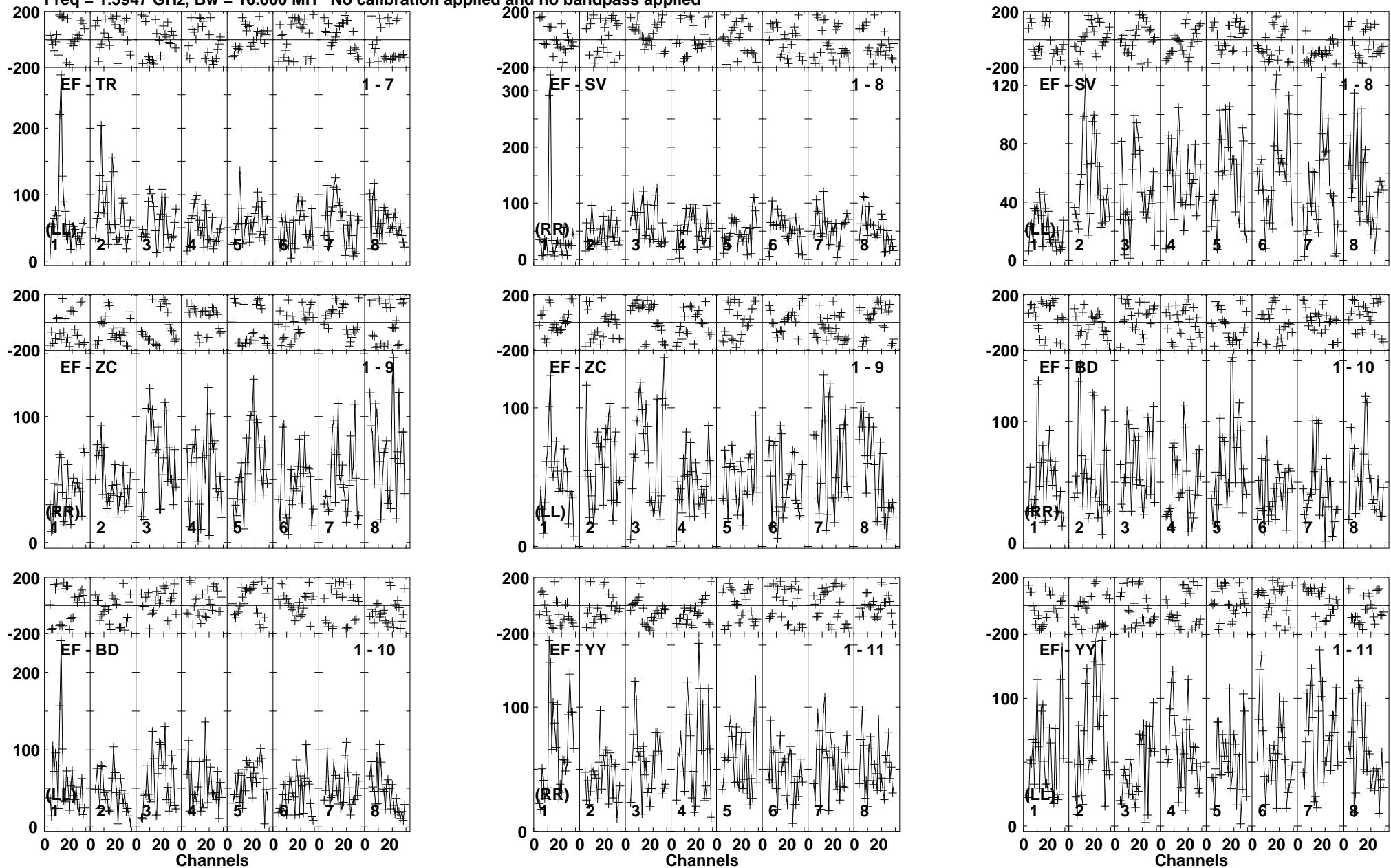
Lower frame: Micro Ampl Jy Top frame: Phas deg Vector averaged cross-power spectrum Baseline: EF (01) - TR (07) Timerange: 00/22:04:41 to 00/22:09:51
