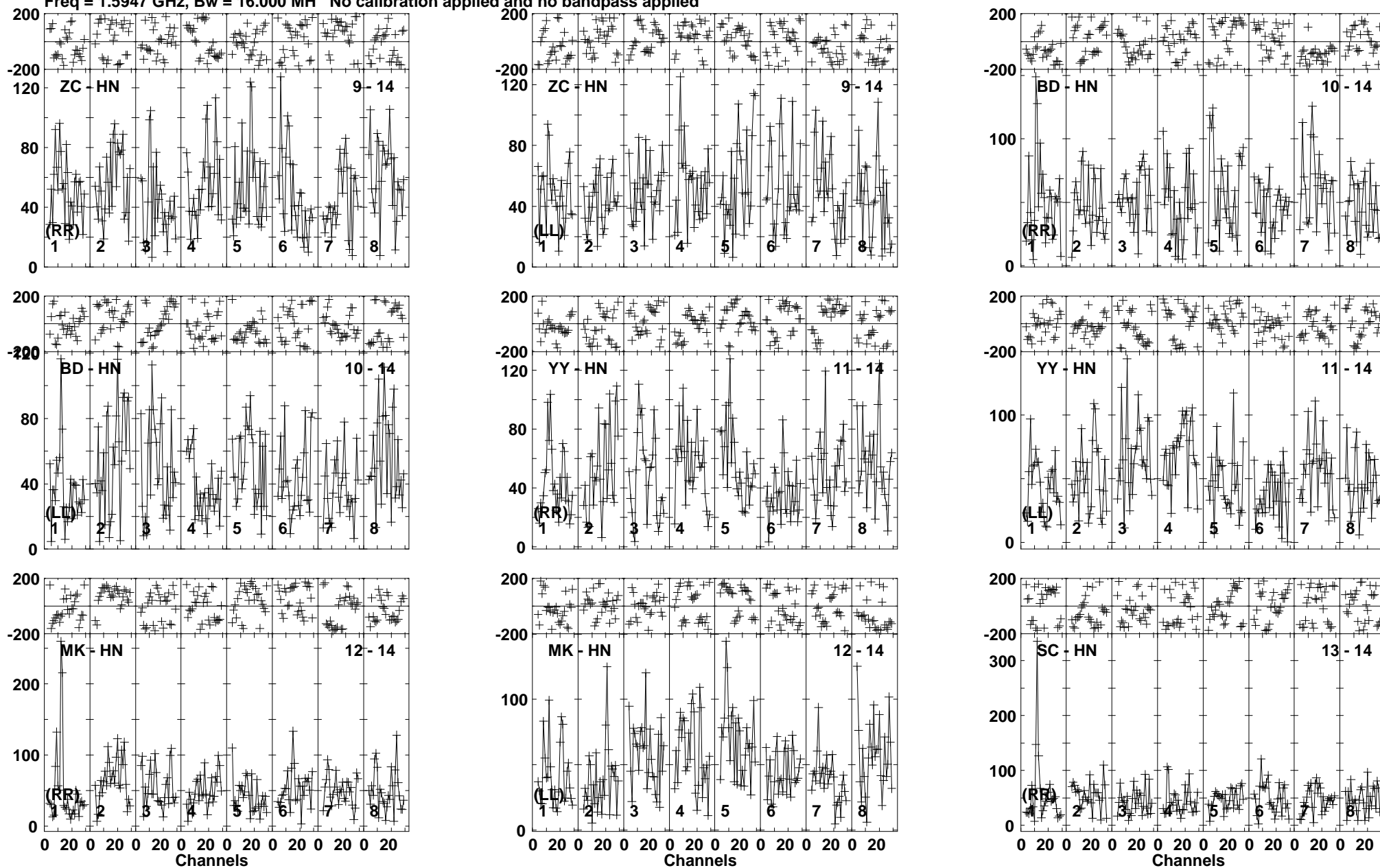
Lower frame: Micro Ampl Jy Top frame: Phas deg Vector averaged cross-power spectrum Baseline: ZC (09) - HN (14) Timerange: 00/22:47:55 to 00/22:53:05
