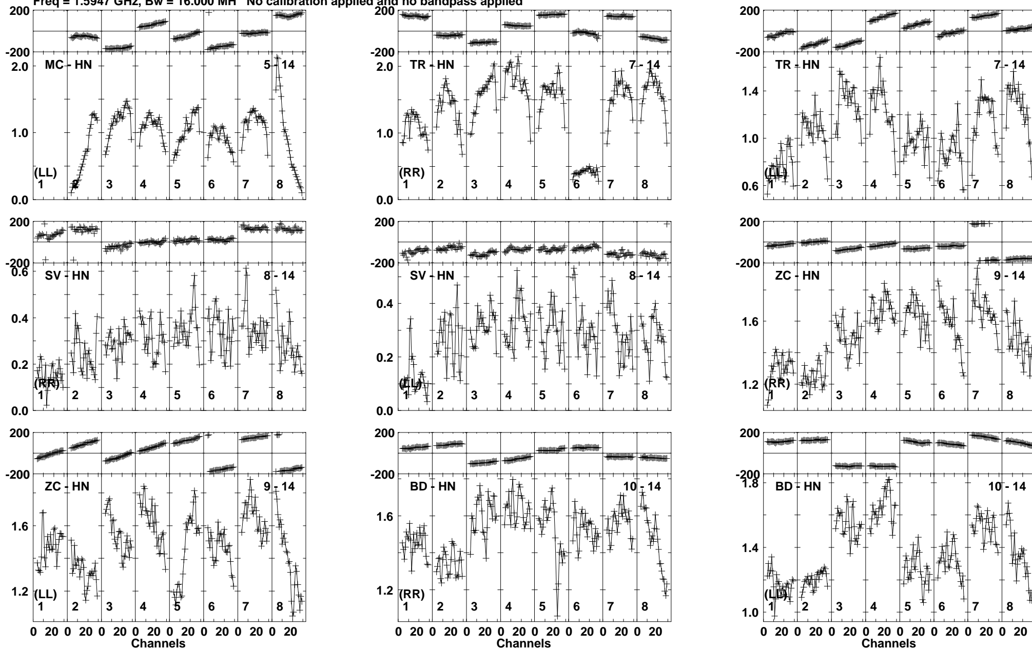
Lower frame: Milli Ampl Jy Top frame: Phas deg Vector averaged cross-power spectrum Baseline: MC (05) - HN (14) Timerange: 00/22:09:59 to 00/22:11:48
