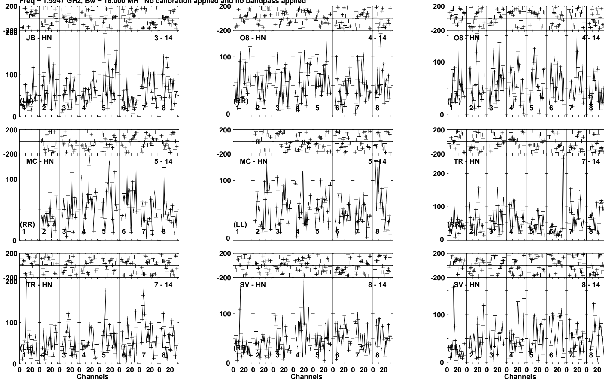
Lower frame: Micro Ampl Jy Top frame: Phas deg Vector averaged cross-power spectrum Baseline: JB (03) - HN (14) Timerange: 00/22:26:18 to 00/22:31:32
