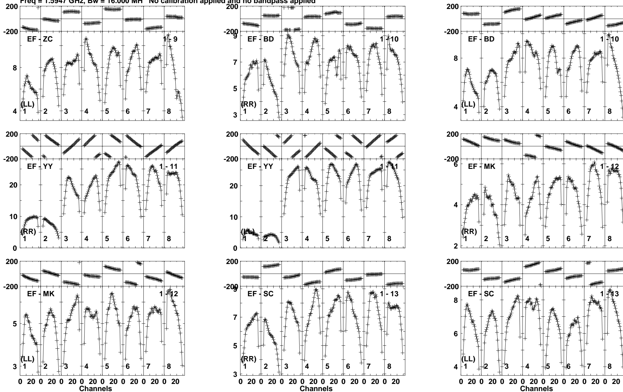
Lower frame: Milli Ampl Jy Top frame: Phas deg Vector averaged cross-power spectrum Baseline: EF (01) - ZC (09) Timerange: 01/01:31:49 to 01/01:33:38
