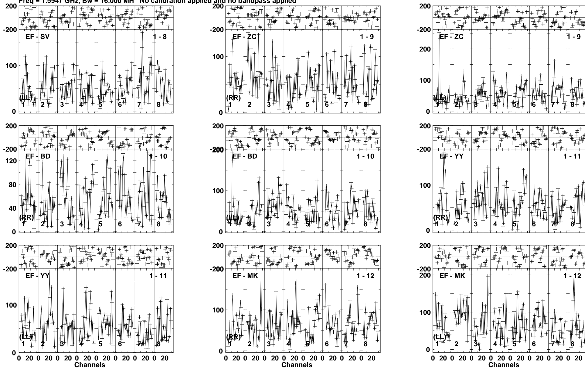
Lower frame: Micro Ampl Jy Top frame: Phas deg Vector averaged cross-power spectrum Baseline: EF (01) - SV (08) Timerange: 01/00:00:00 to 01/00:05:10
