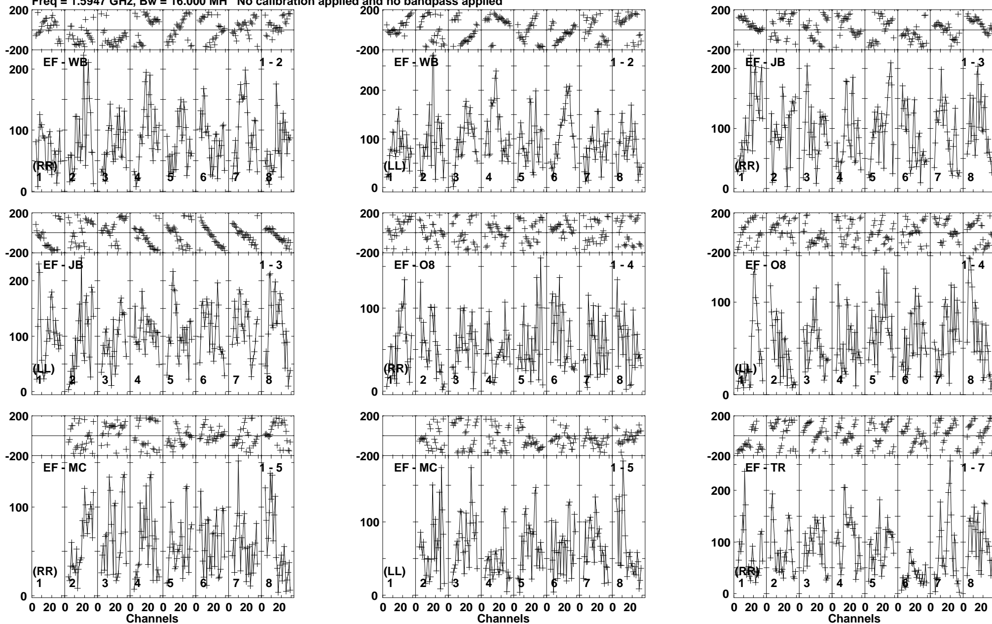
Lower frame: Micro Ampl Jy Top frame: Phas deg Vector averaged cross-power spectrum Baseline: EF (01) - WB (02) Timerange: 00/21:21:26 to 00/21:26:36
