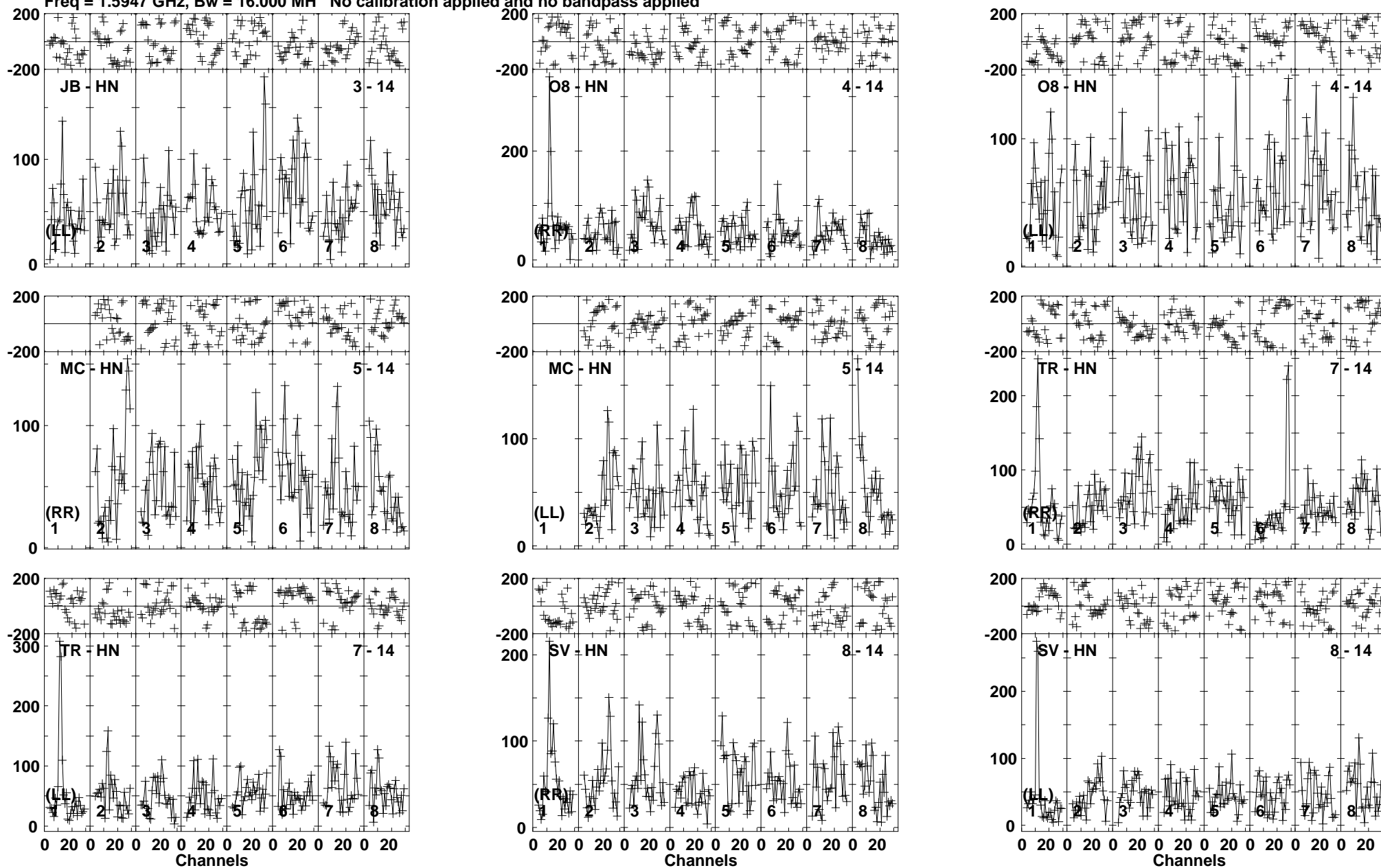
Lower frame: Micro Ampl Jy Top frame: Phas deg Vector averaged cross-power spectrum Baseline: JB (03) - HN (14) Timerange: 00/22:55:08 to 00/23:00:22
