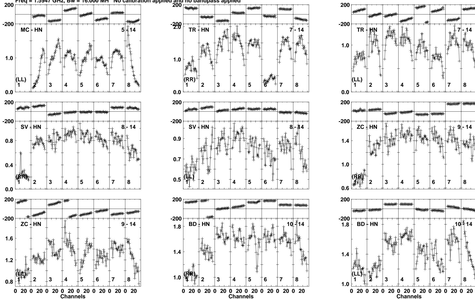
Lower frame: Milli Ampl Jy Top frame: Phas deg Vector averaged cross-power spectrum Baseline: MC (05) - HN (14) Timerange: 01/00:55:51 to 01/00:57:32
