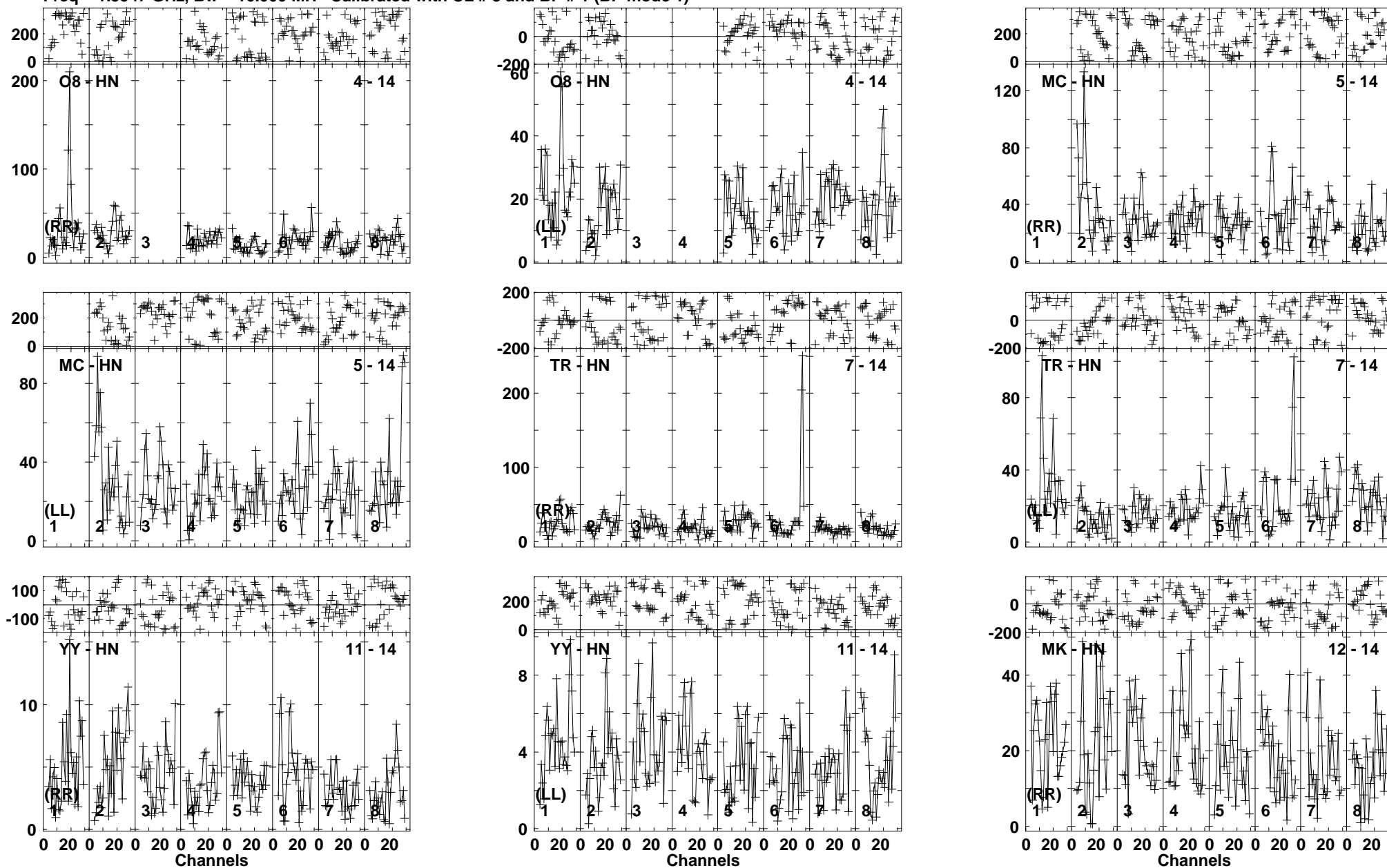
Lower frame: Milli Ampl Jy Top frame: Phas deg Vector averaged cross-power spectrum Baseline: O8 (04) - HN (14) Timerange: 01/00:36:03 to 01/00:41:17
