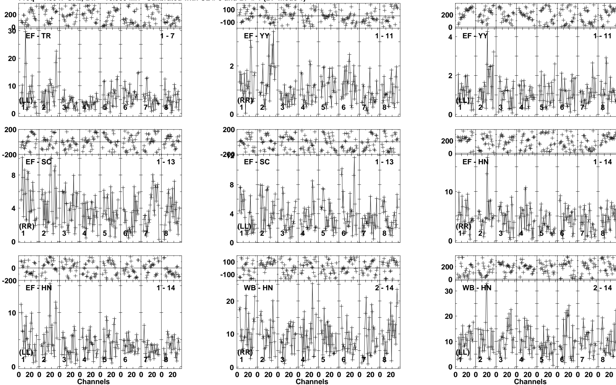
Lower frame: Milli Ampl Jy Top frame: Phas deg Vector averaged cross-power spectrum Baseline: EF (01) - TR (07) Timerange: 00/20:09:21 to 00/20:14:31
