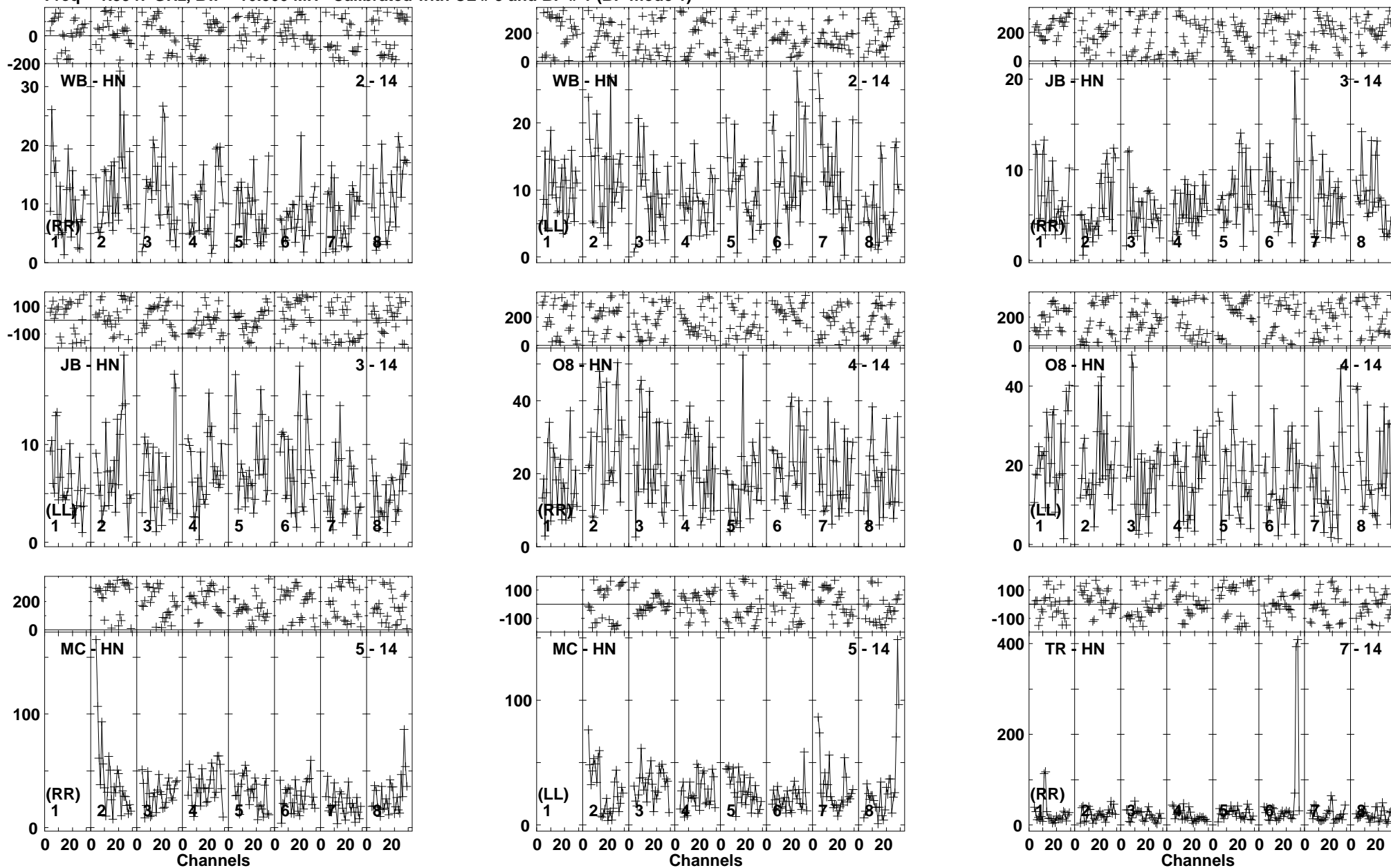
Lower frame: Milli Ampl Jy Top frame: Phas deg Vector averaged cross-power spectrum Baseline: WB (02) - HN (14) Timerange: 00/22:19:05 to 00/22:24:15
