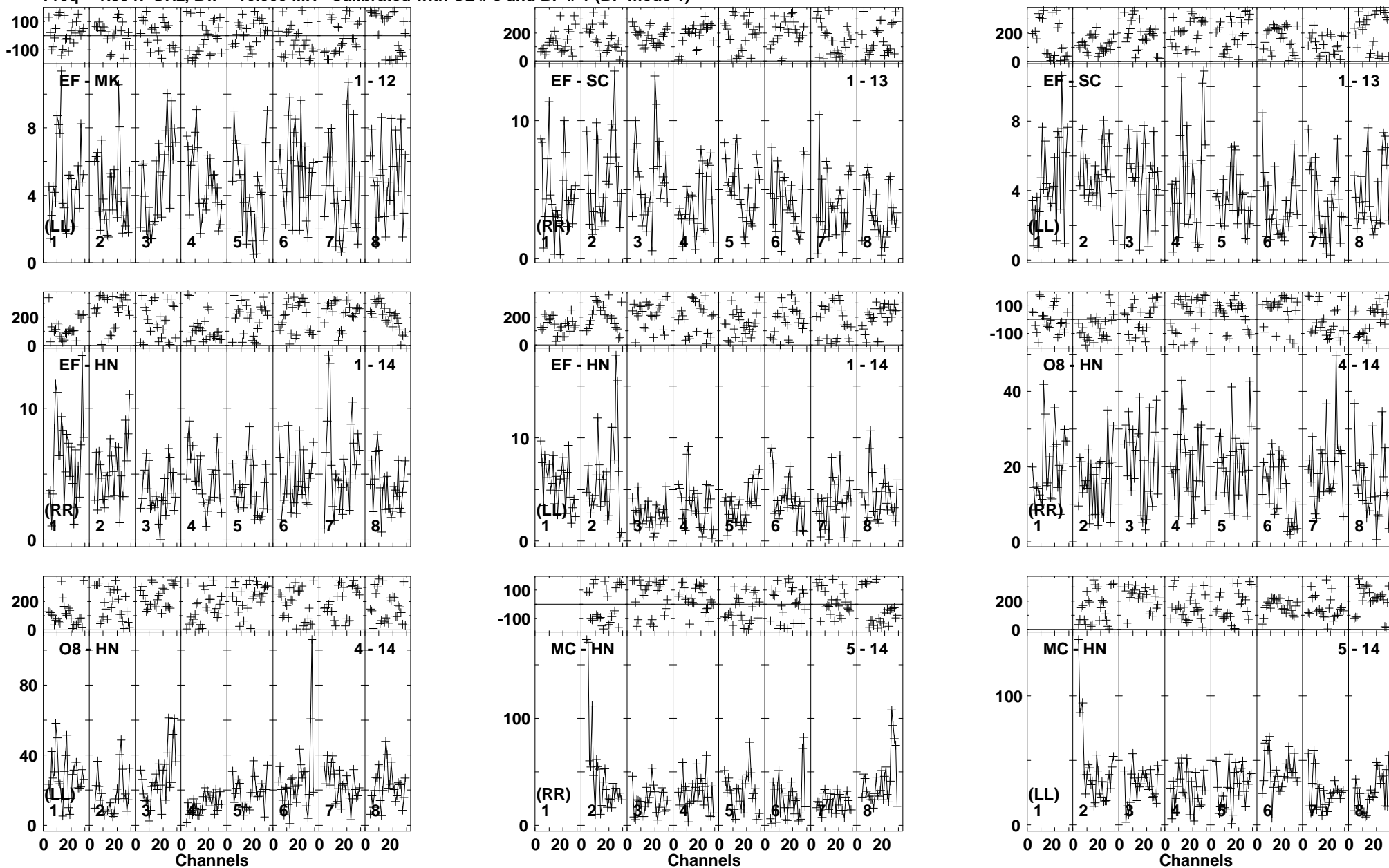
Lower frame: Milli Ampl Jy Top frame: Phas deg Vector averaged cross-power spectrum Baseline: EF (01) - MK (12) Timerange: 01/01:48:11 to 01/01:53:23
