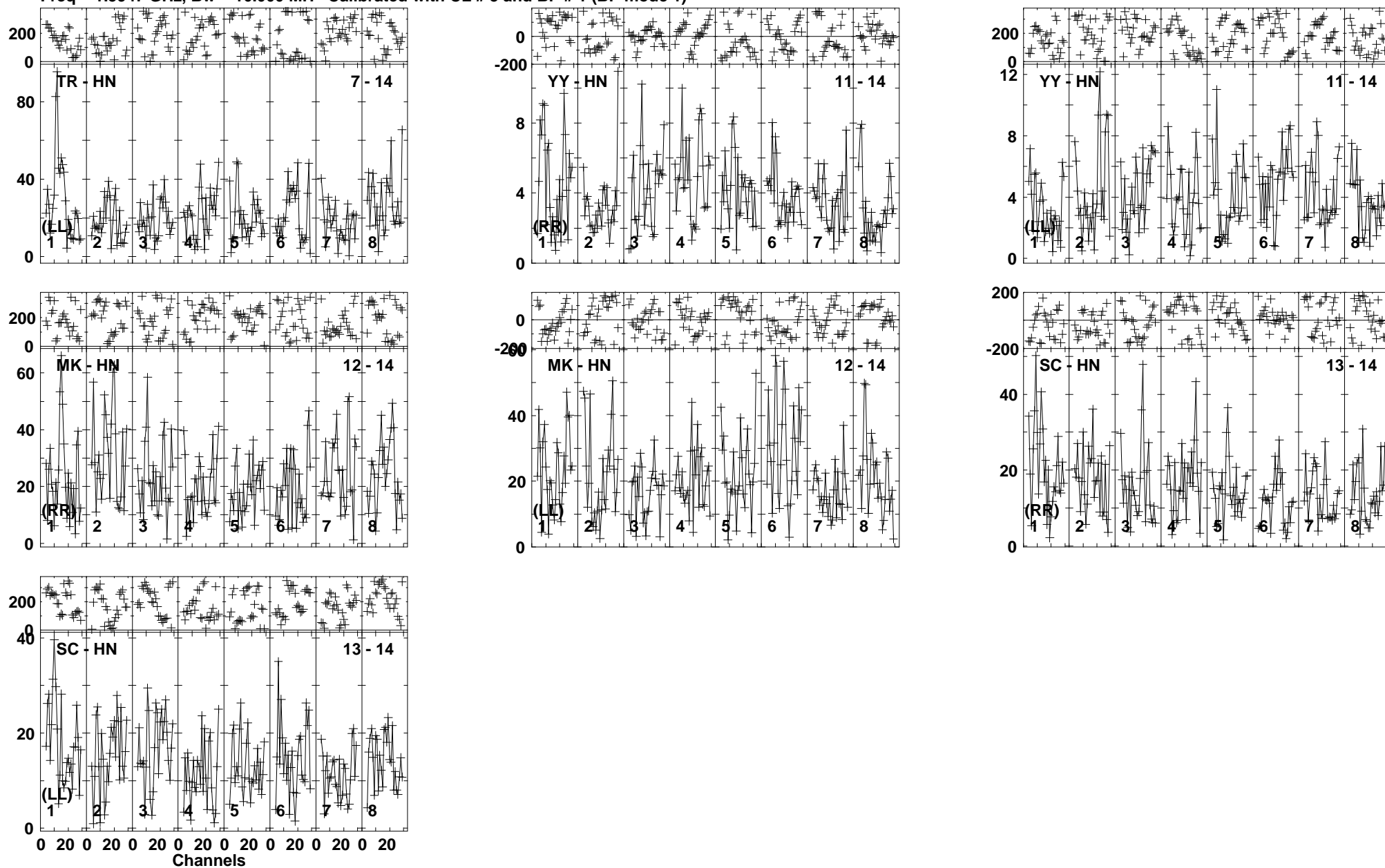
Lower frame: Milli Ampl Jy Top frame: Phas deg Vector averaged cross-power spectrum Baseline: TR (07) - HN (14) Timerange: 00/20:38:11 to 00/20:43:21
