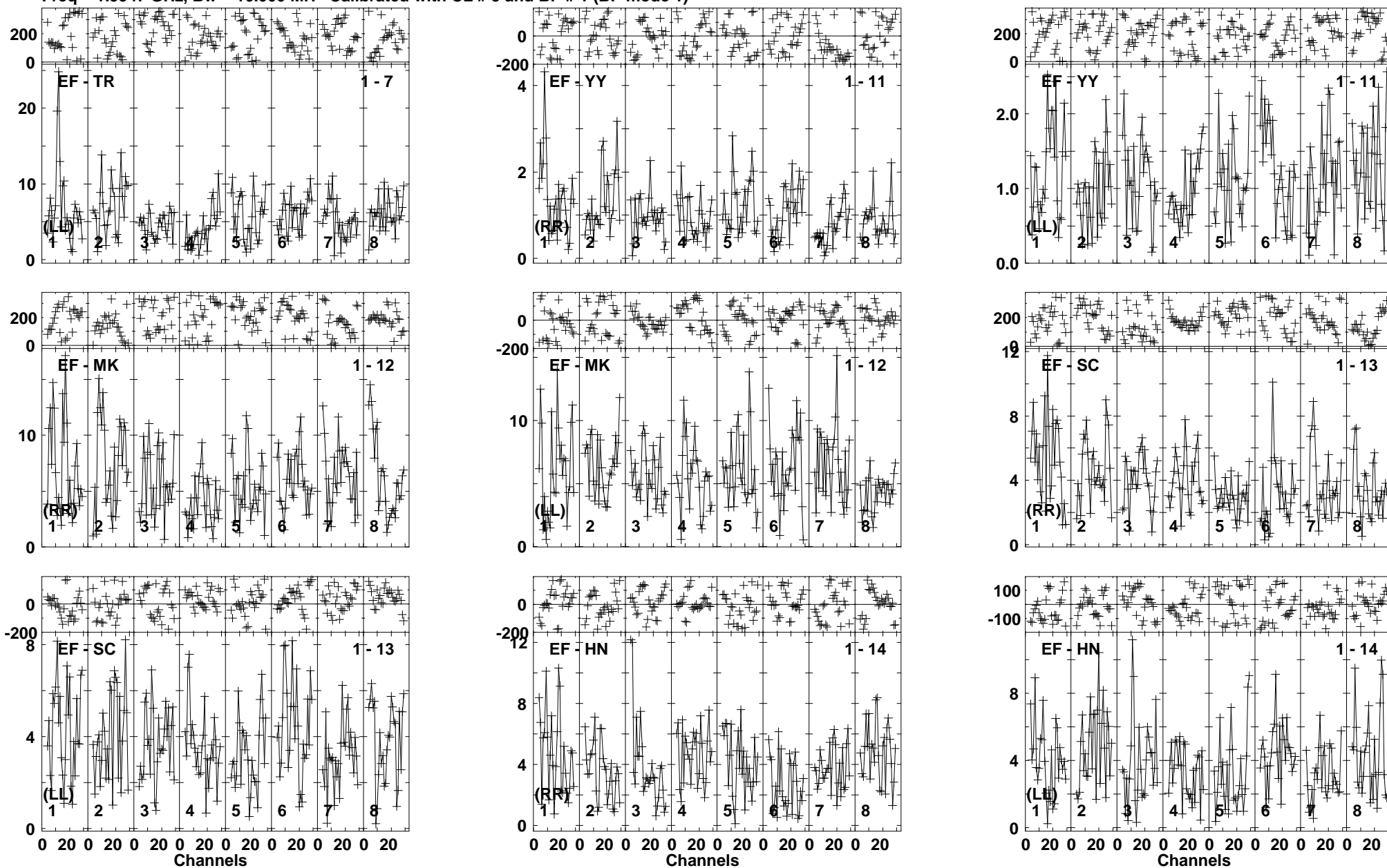
Lower frame: Milli Ampl Jy Top frame: Phas deg Vector averaged cross-power spectrum Baseline: EF (01) - TR (07) Timerange: 00/20:23:46 to 00/20:28:56
