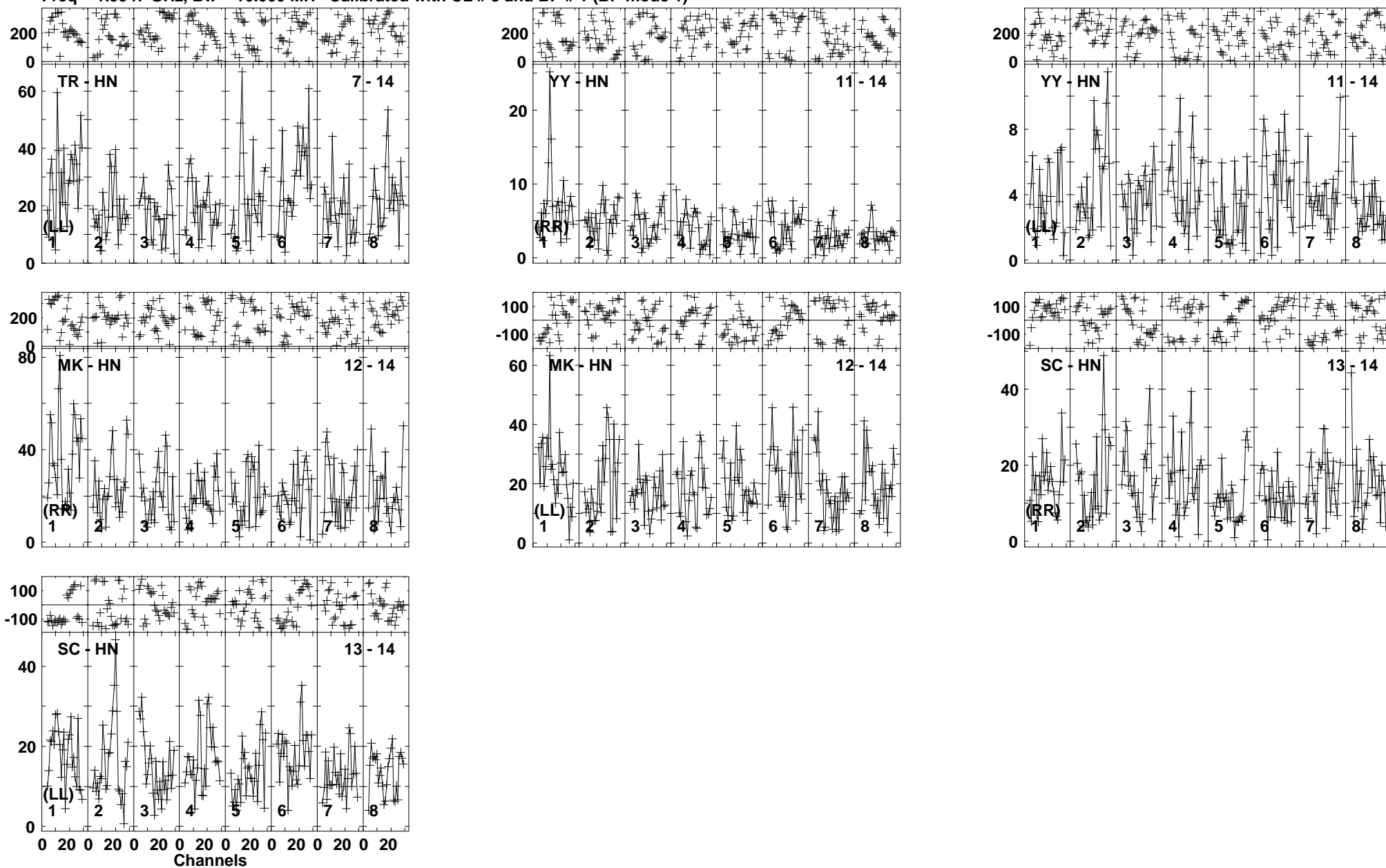
Lower frame: Milli Ampl Jy Top frame: Phas deg Vector averaged cross-power spectrum Baseline: TR (07) - HN (14) Timerange: 00:22:19:05 to 00:22:24:15
