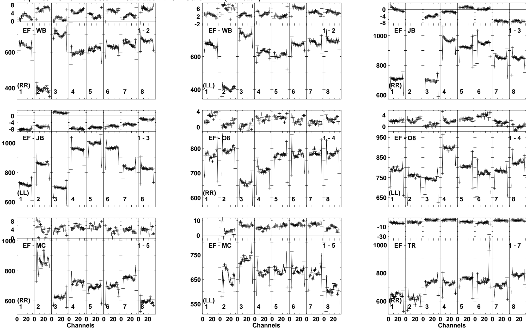
Lower frame: Milli Ampl Jy Top frame: Phas deg Vector averaged cross-power spectrum Baseline: EF (01) - WB (02) Timerange: 00/22:02:51 to 00/22:04:32
