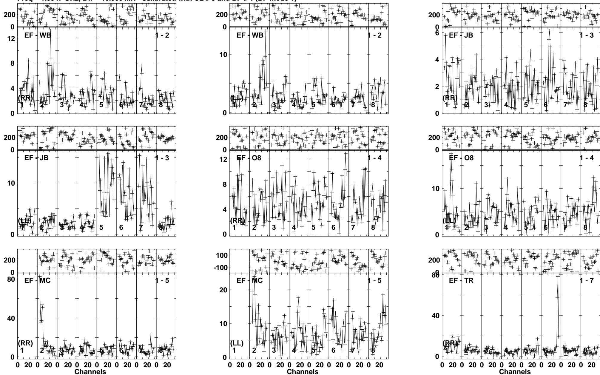
Lower frame: Milli Ampl Jy Top frame: Phas deg Vector averaged cross-power spectrum Baseline: EF (01) - WB (02) Timerange: 00/20:38:11 to 00/20:43:21
