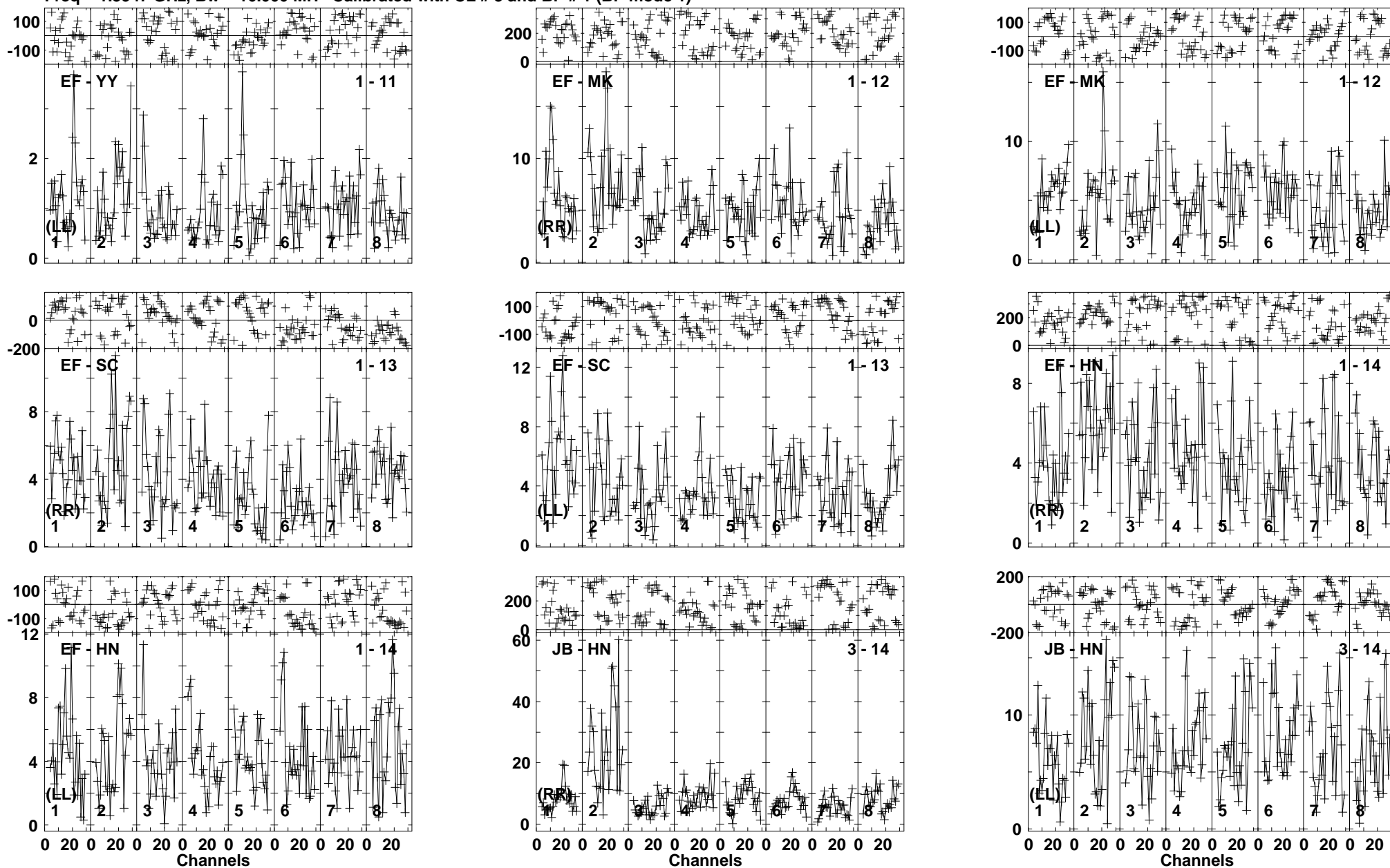
Lower frame: Milli Ampl Jy Top frame: Phas deg Vector averaged cross-power spectrum Baseline: EF (01) - YY (11) Timerange: 01/01:33:43 to 01/01:38:57
