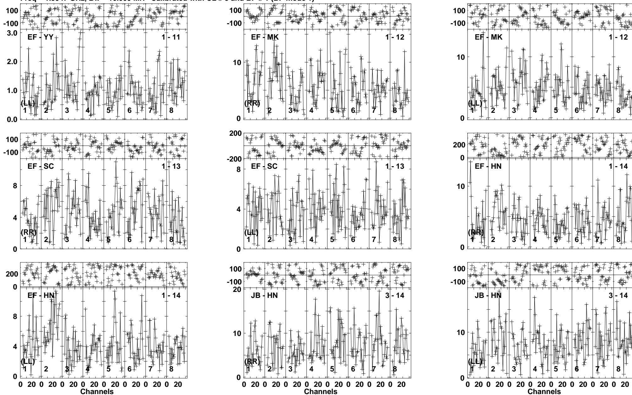
Lower frame: Milli Ampl Jy Top frame: Phas deg Vector averaged cross-power spectrum Baseline: EF (01) - YY (11) Timerange: 01/00:14:25 to 01/00:19:35
