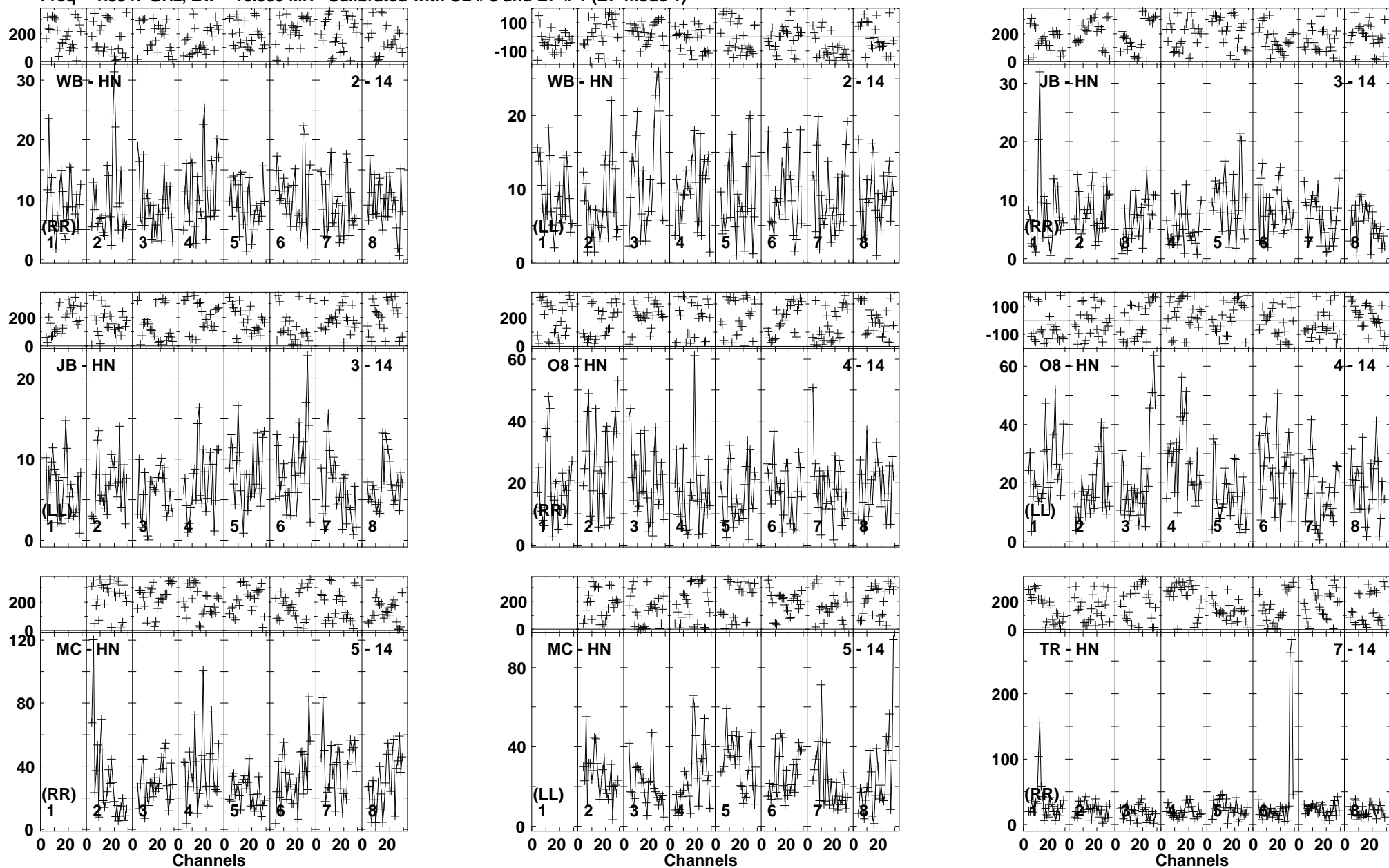
Lower frame: Milli Ampl Jy Top frame: Phas deg Vector averaged cross-power spectrum Baseline: WB (02) - HN (14) Timerange: 00/22:33:30 to 00/22:38:40
