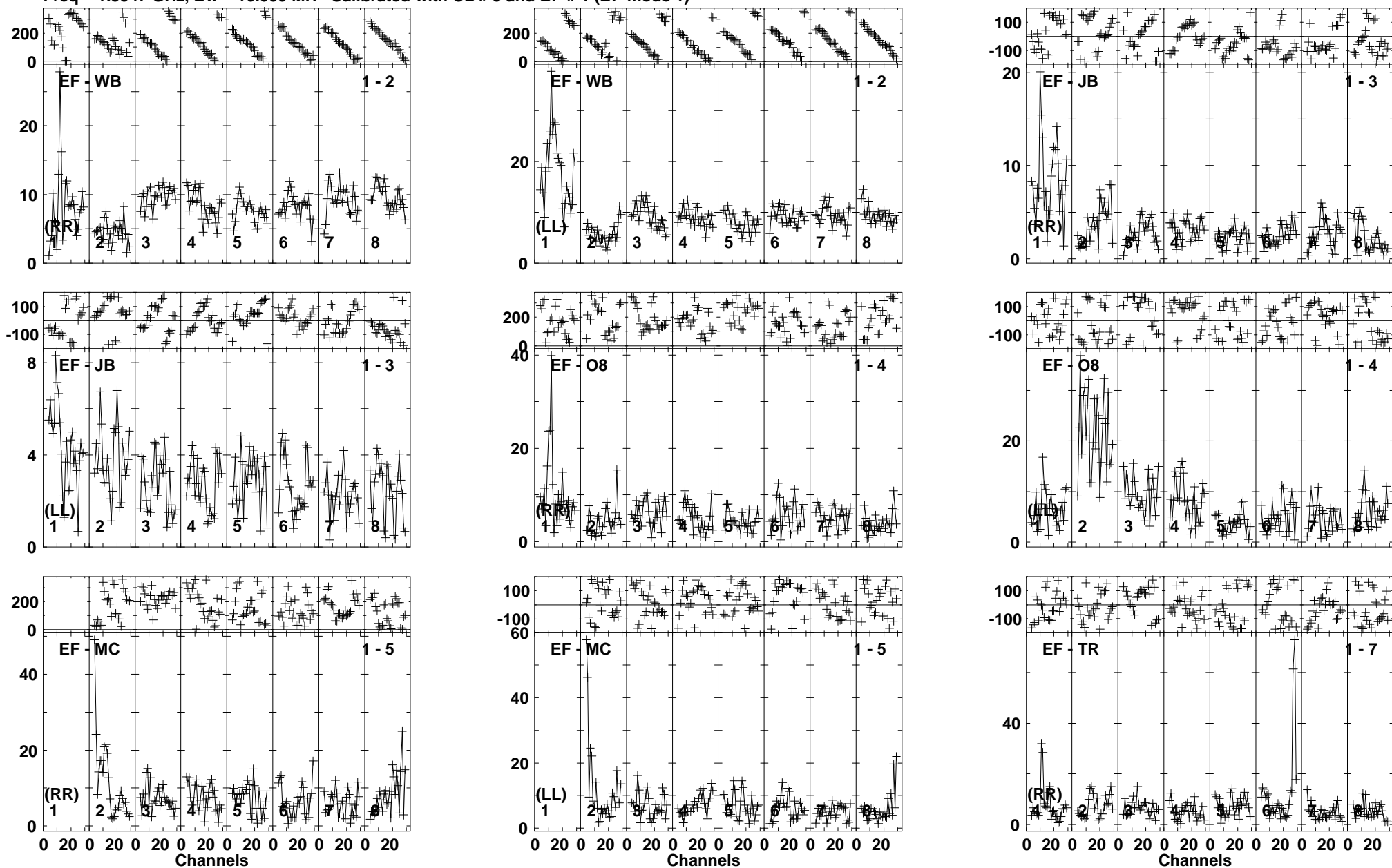
Lower frame: Milli Ampl Jy Top frame: Phas deg Vector averaged cross-power spectrum Baseline: EF (01) - WB (02) Timerange: 00/23:16:45 to 00/23:21:55
