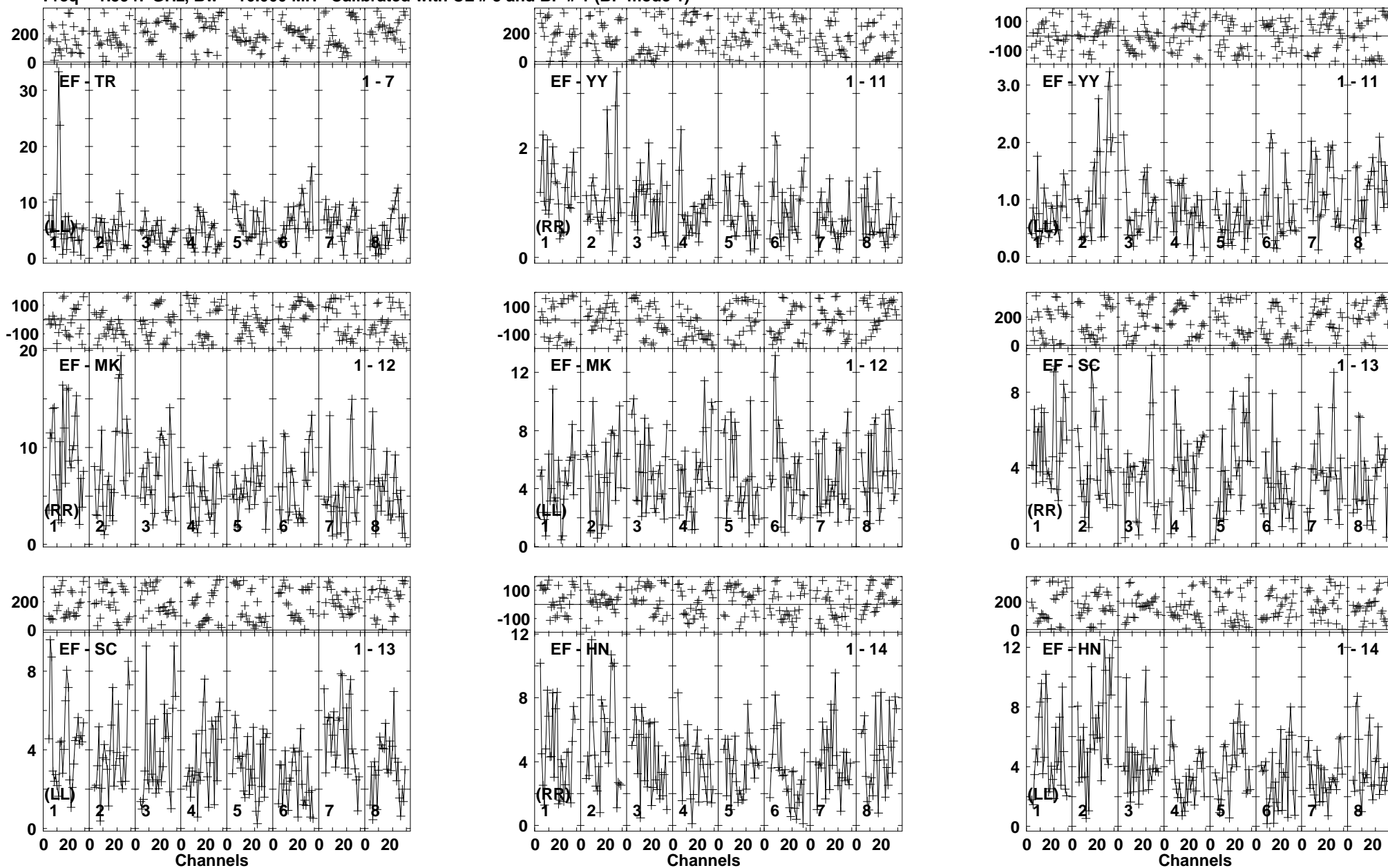
Lower frame: Milli Ampl Jy Top frame: Phas deg Vector averaged cross-power spectrum Baseline: EF (01) - TR (07) Timerange: 00/21:50:16 to 00/21:55:26
