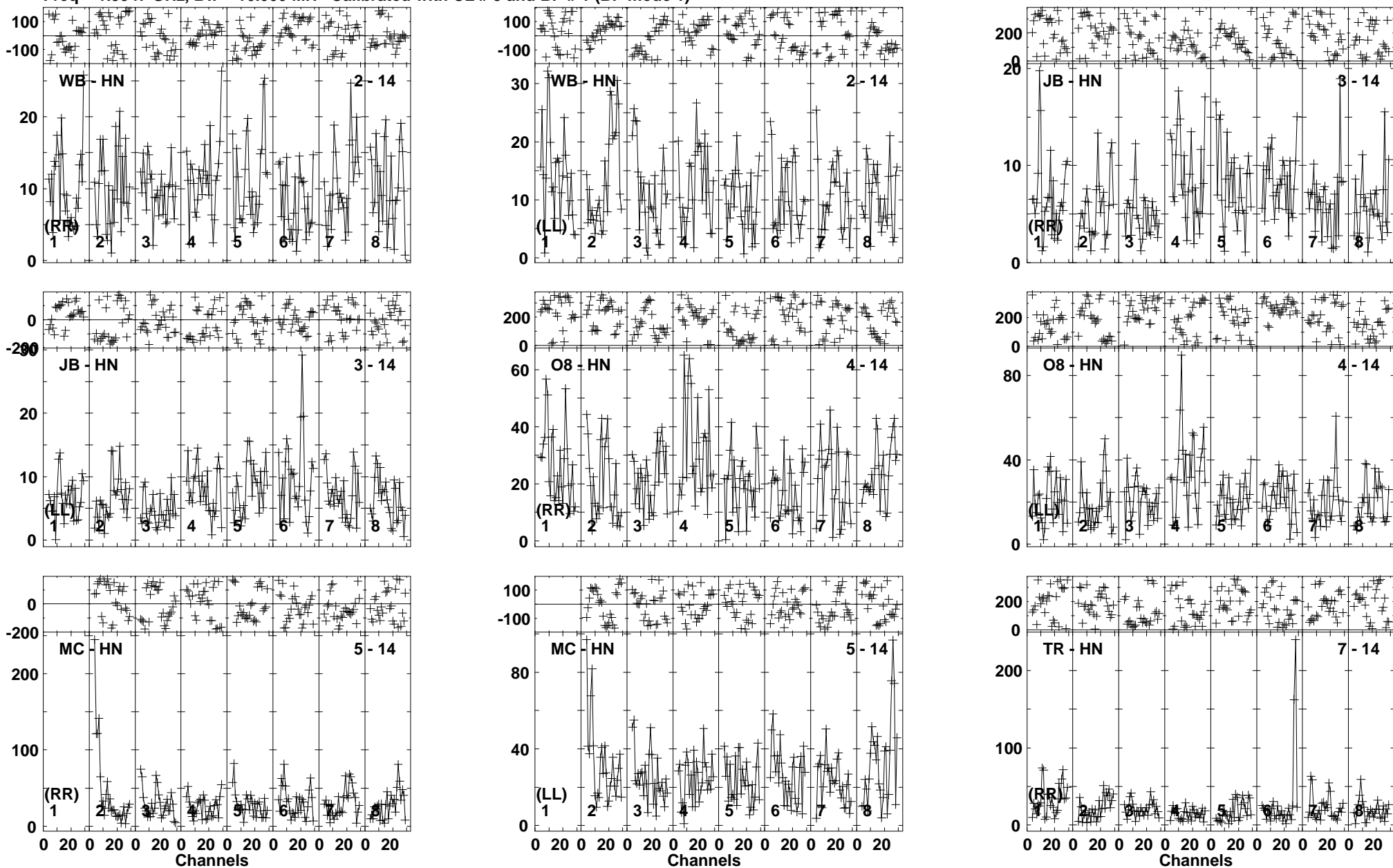
Lower frame: Milli Ampl Jy Top frame: Phas deg Vector averaged cross-power spectrum Baseline: WB (02) - HN (14) Timerange: 00/20:52:36 to 00/20:57:46
