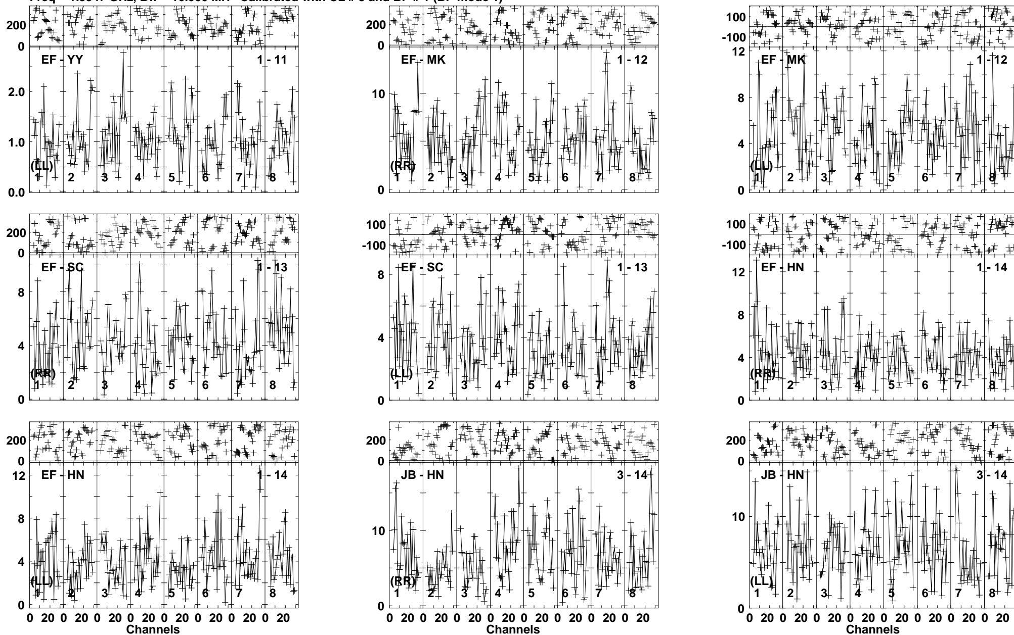
Lower frame: Milli Ampl Jy Top frame: Phas deg Vector averaged cross-power spectrum Baseline: EF (01) - YY (11) Timerange: 00/23:45:35 to 00/23:50:45
