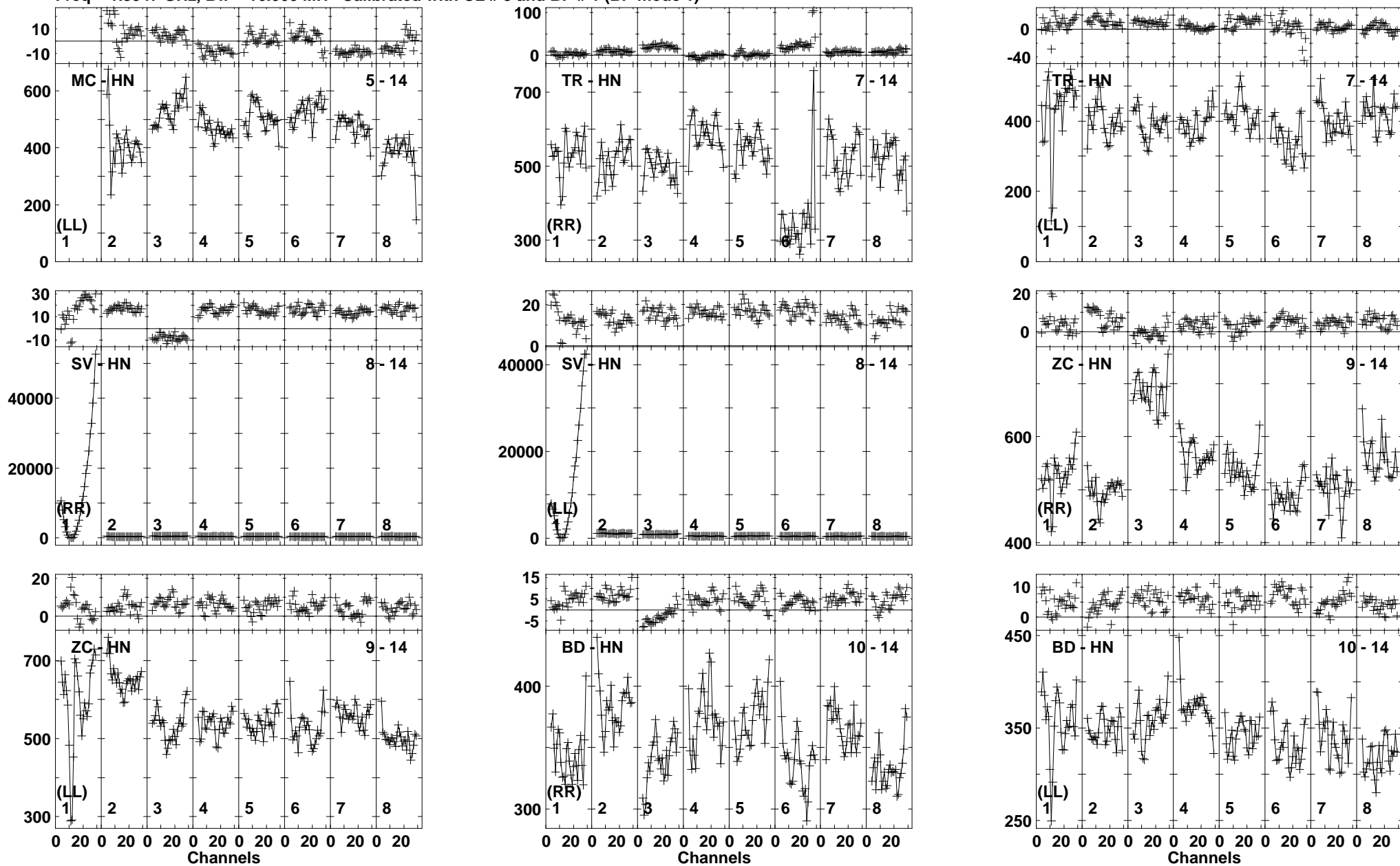
Lower frame: Milli Ampl Jy Top frame: Phas deg Vector averaged cross-power spectrum Baseline: MC (05) - HN (14) Timerange: 01/01:24:41 to 01/01:26:22
