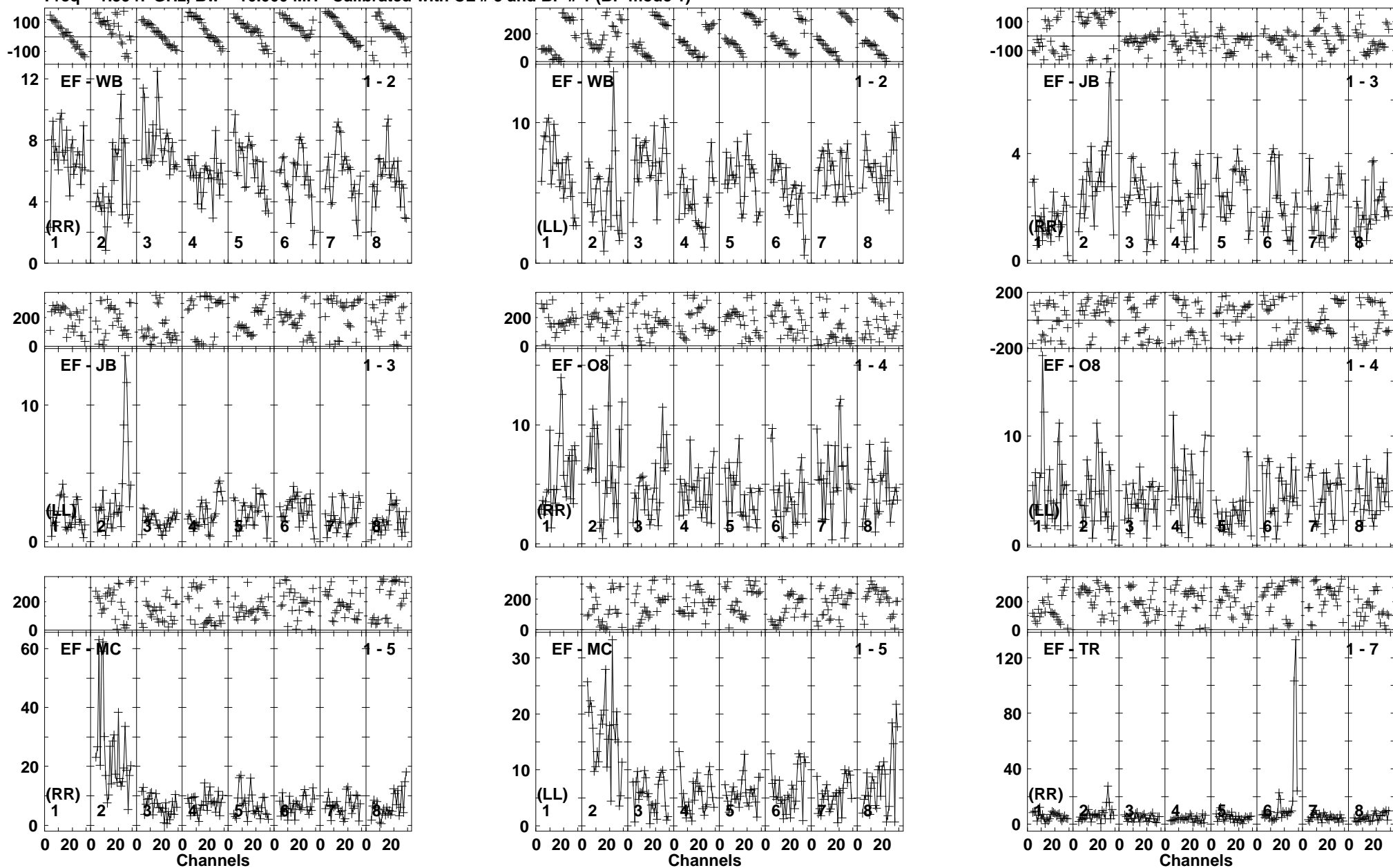
Lower frame: Milli Ampl Jy Top frame: Phas deg Vector averaged cross-power spectrum Baseline: EF (01) - WB (02) Timerange: 00/21:57:28 to 00/22:02:42
