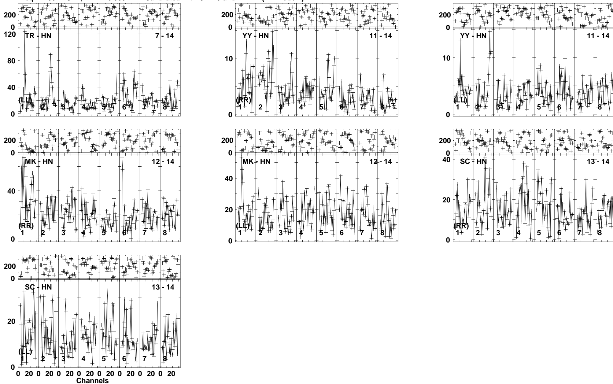
Lower frame: Milli Ampl Jy Top frame: Phas deg Vector averaged cross-power spectrum Baseline: TR (07) - HN (14) Timerange: 00/23:16:45 to 00/23:21:55
