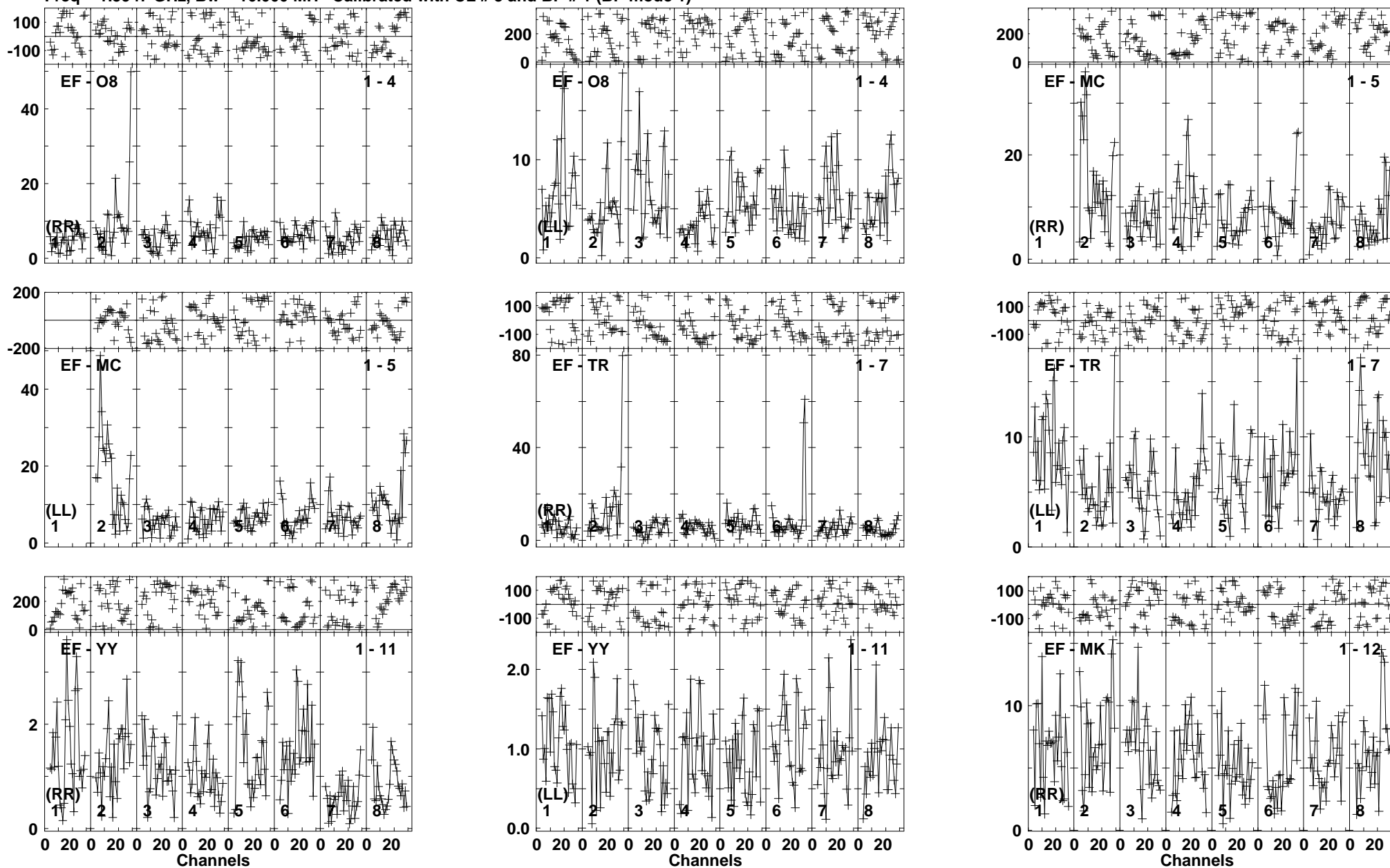
Lower frame: Milli Ampl Jy Top frame: Phas deg Vector averaged cross-power spectrum Baseline: EF (01) - O8 (04) Timerange: 01/01:48:11 to 01/01:53:23
