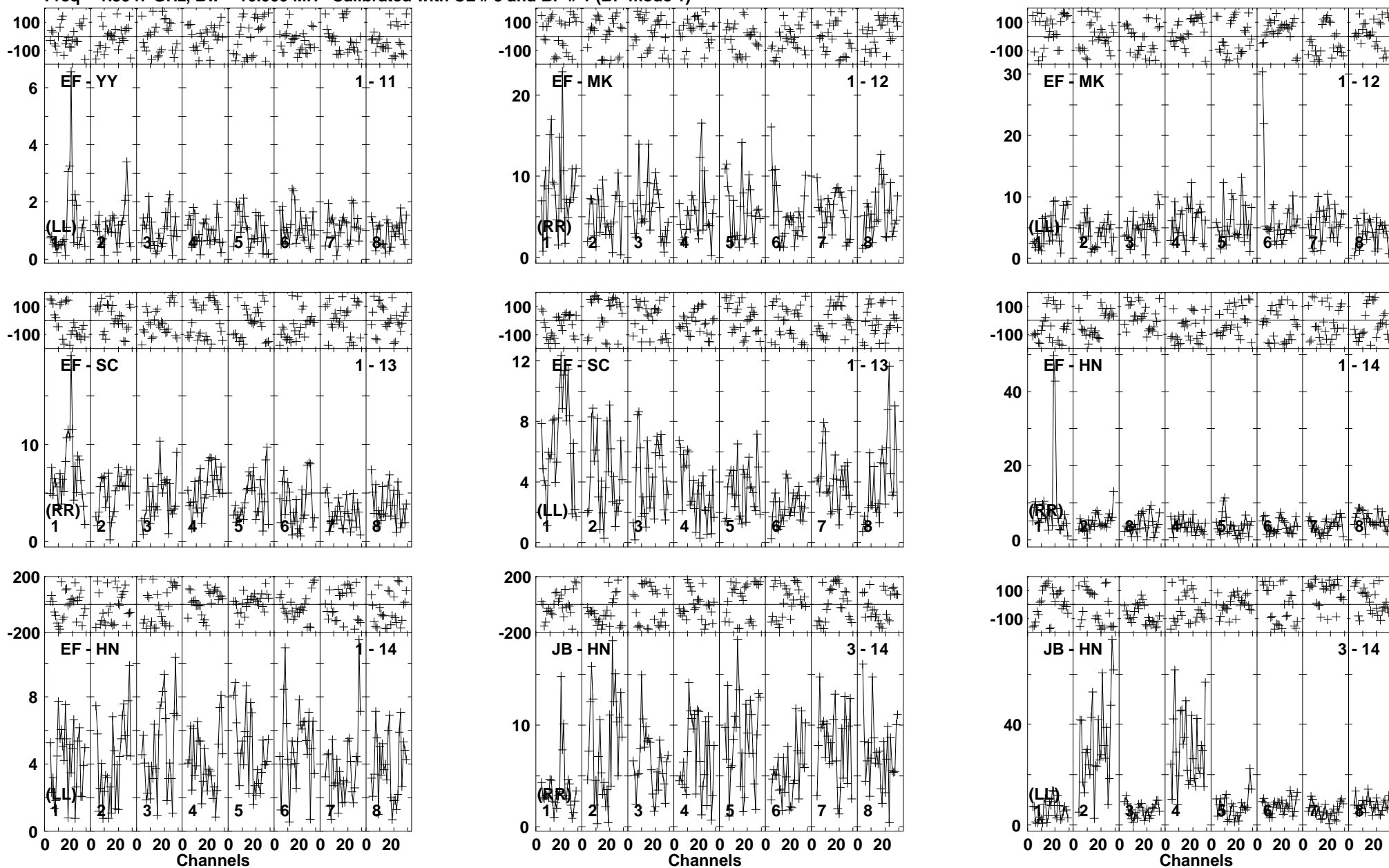
Lower frame: Milli Ampl Jy Top frame: Phas deg Vector averaged cross-power spectrum Baseline: EF (01) - YY (11) Timerange: 01/00:50:28 to 01/00:55:42
