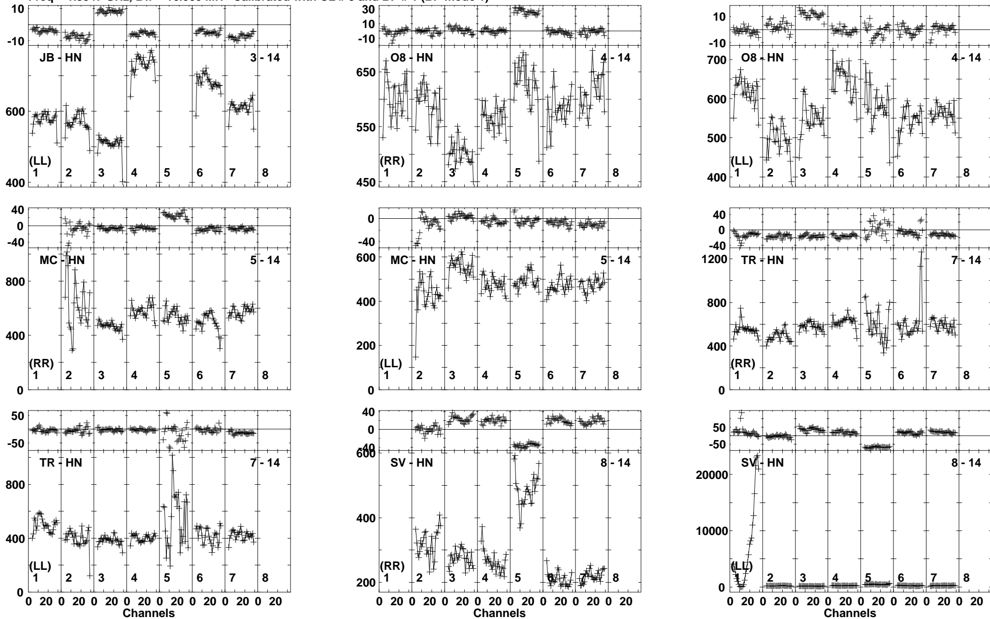
Lower frame: Milli Ampl Jy Top frame: Phas deg Vector averaged cross-power spectrum Baseline: JB (03) - HN (14) Timerange: 00/22:02:51 to 00/22:04:32
