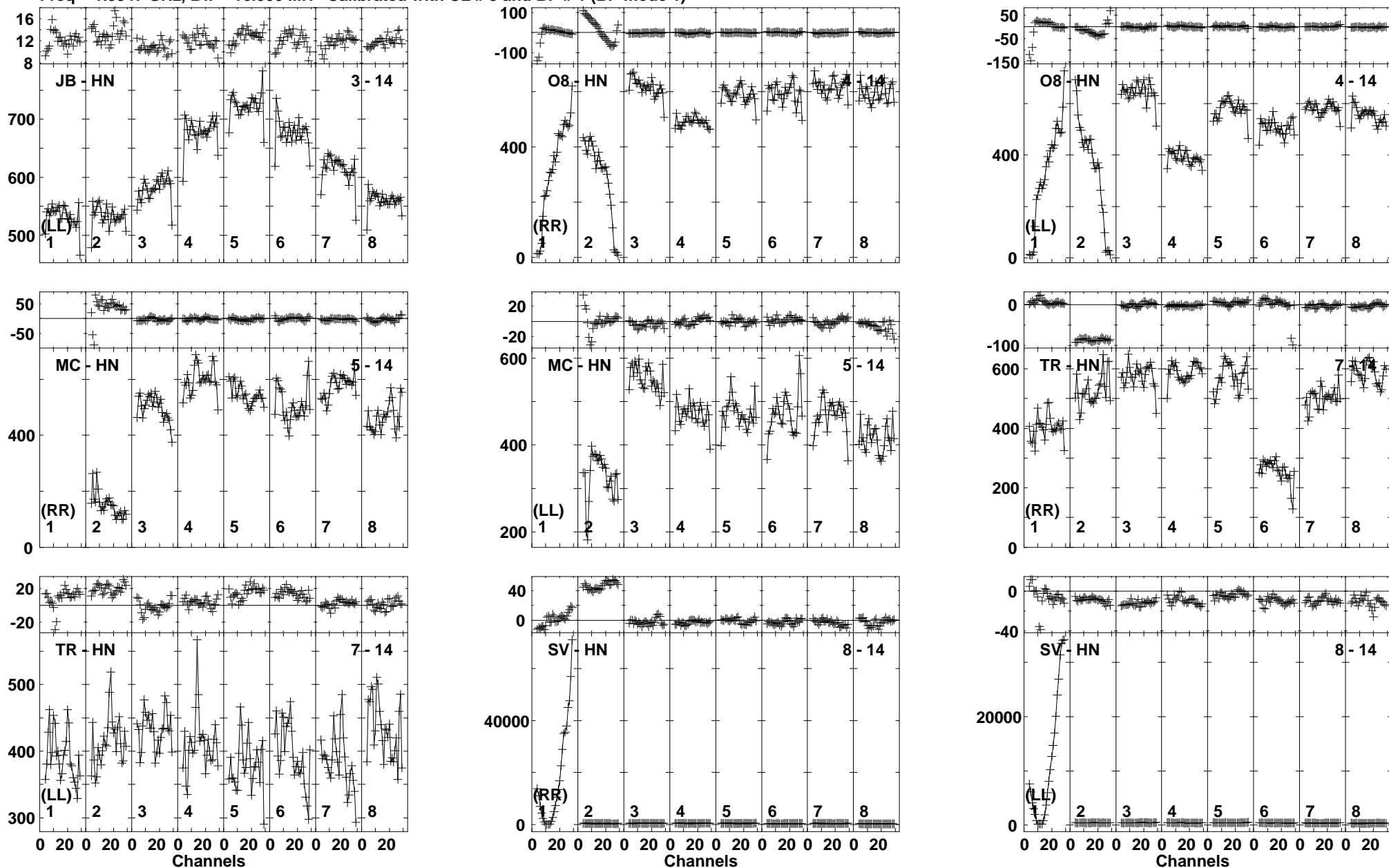
Lower frame: Milli Ampl Jy Top frame: Phas deg Vector averaged cross-power spectrum Baseline: JB (03) - HN (14) Timerange: 00/21:19:36 to 00/21:21:17
