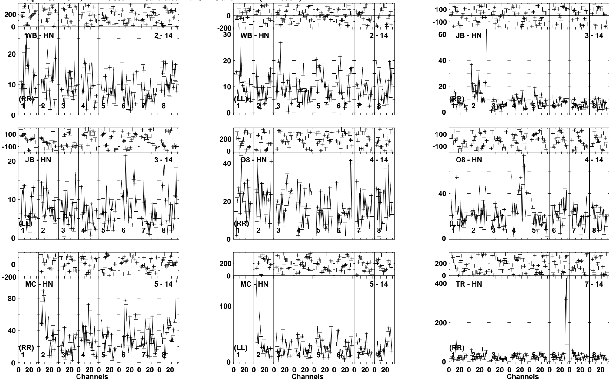
Lower frame: Milli Ampl Jy Top frame: Phas deg Vector averaged cross-power spectrum Baseline: WB (02) - HN (14) Timerange: 00/22:55:08 to 00/23:00:22
