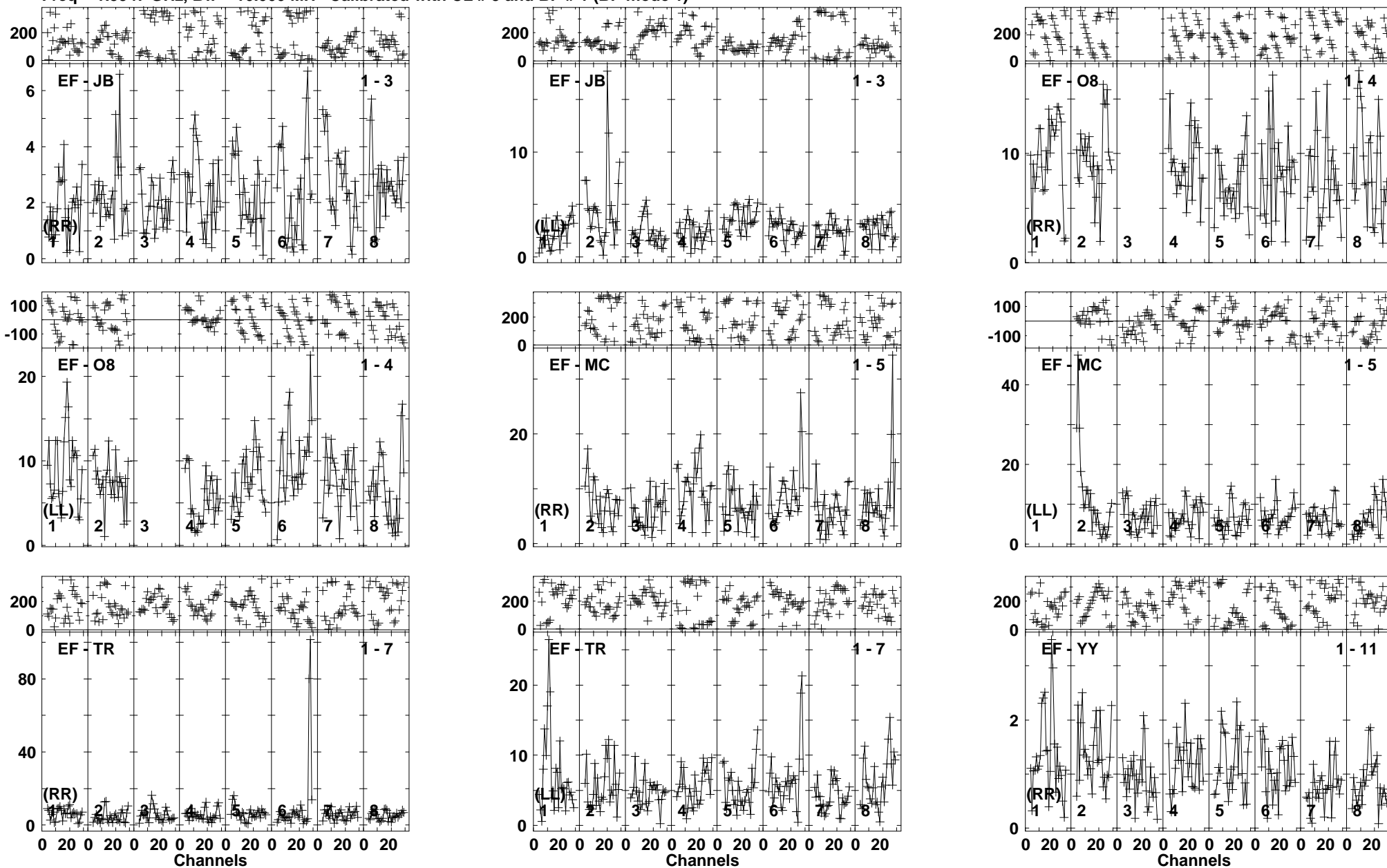
Lower frame: Milli Ampl Jy Top frame: Phas deg Vector averaged cross-power spectrum Baseline: EF (01) - JB (03) Timerange: 01/00:28:51 to 01/00:34:01
