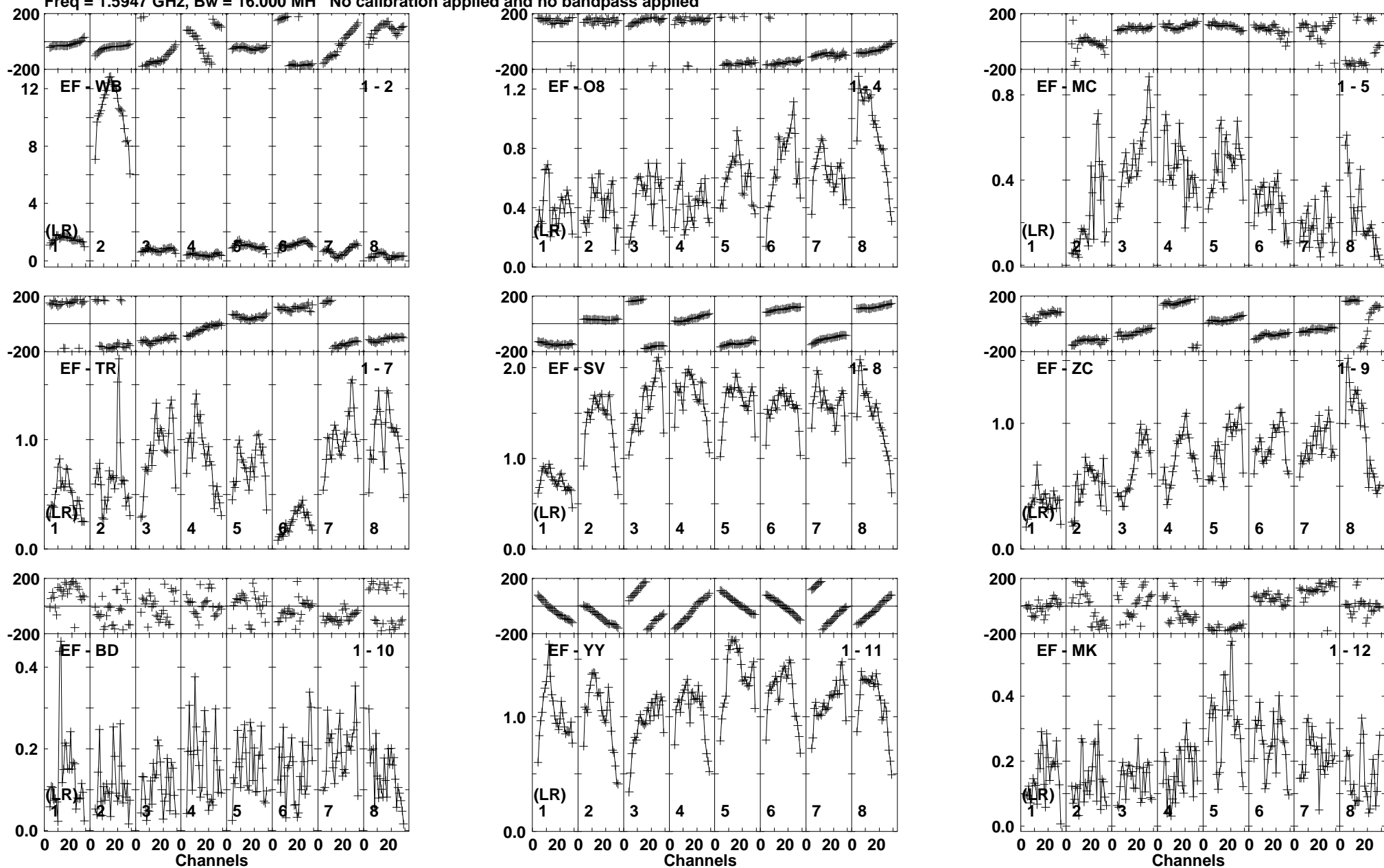
Lower frame: Milli Ampl Jy Top frame: Phas deg Vector averaged cross-power spectrum Baseline: EF (01) - WB (02) Timerange: 00/23:36:28 to 00/23:38:18
