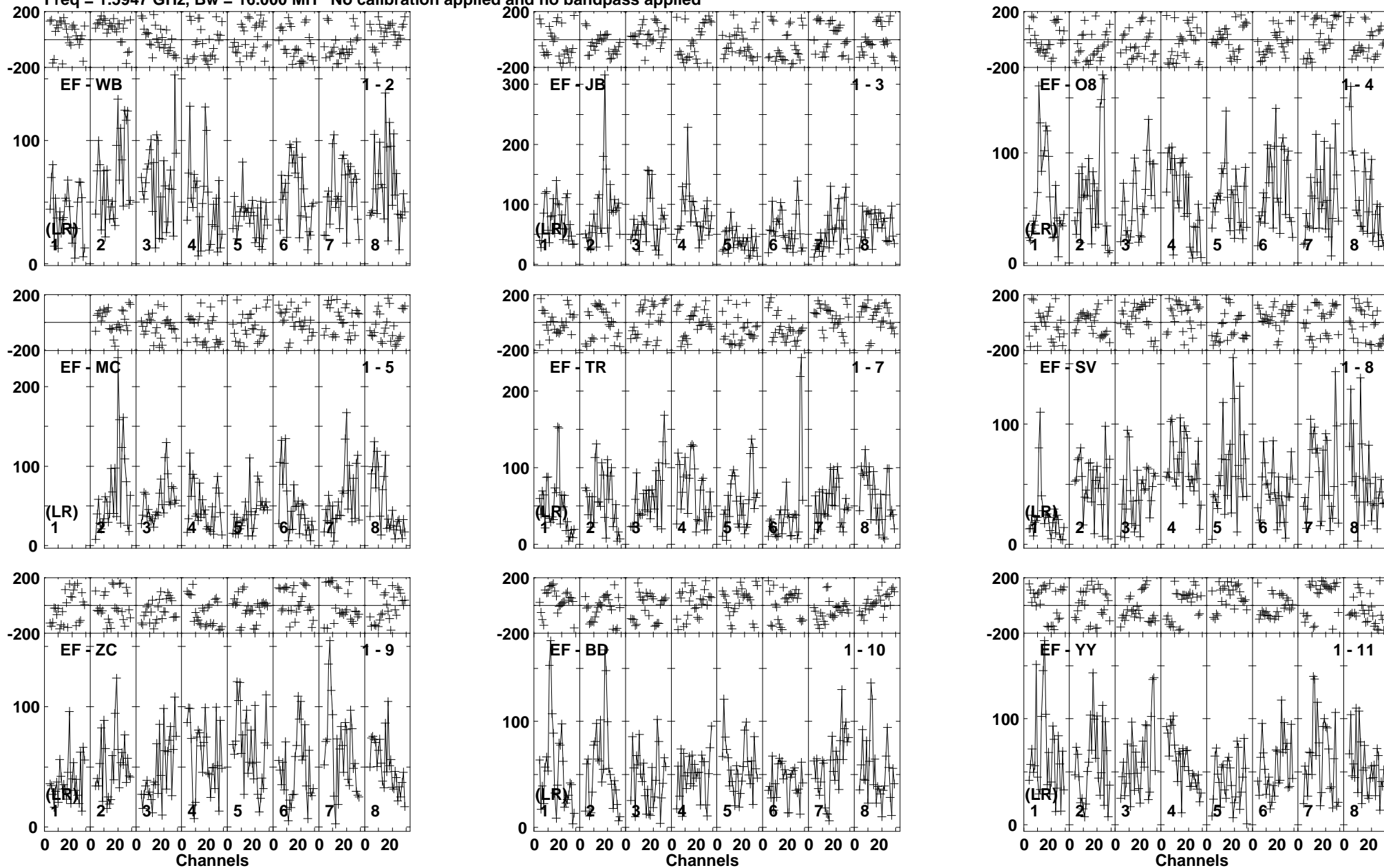
Lower frame: Micro Ampl Jy Top frame: Phas deg Vector averaged cross-power spectrum Baseline: EF (01) - WB (02) Timerange: 00/20:30:58 to 00/20:36:12
