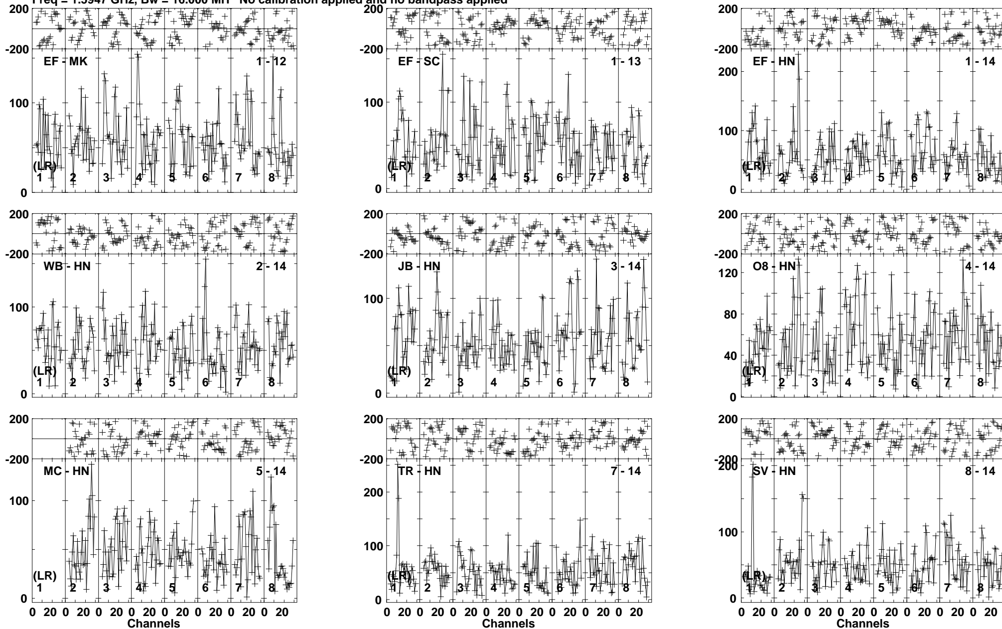
Lower frame: Micro Ampl Jy Top frame: Phas deg Vector averaged cross-power spectrum Baseline: EF (01) - MK (12) Timerange: 00/22:19:05 to 00/22:24:15
