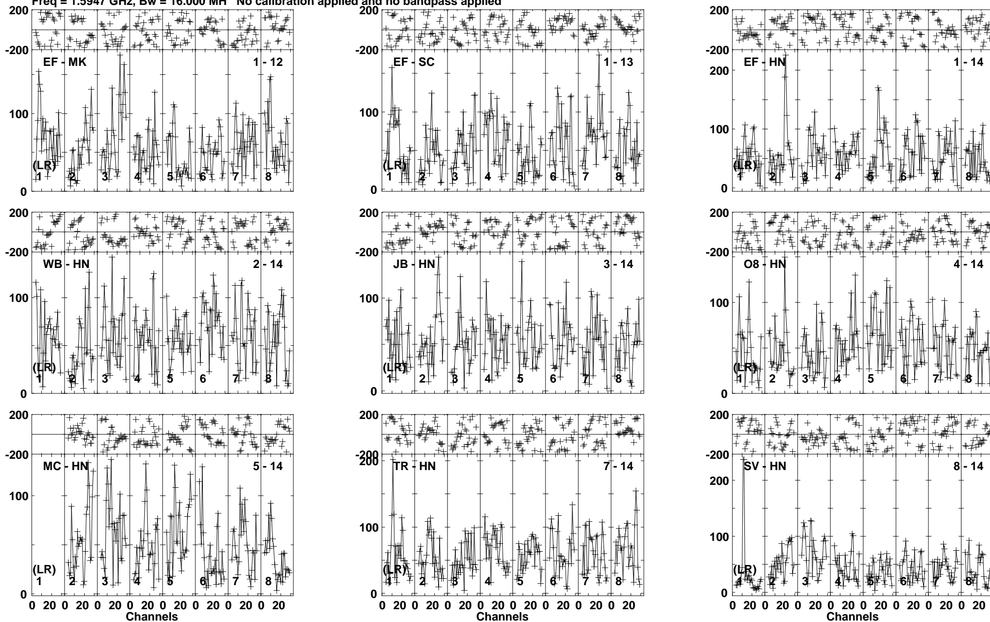
Lower frame: Micro Ampl Jy Top frame: Phas deg Vector averaged cross-power spectrum Baseline: EF (01) - MK (12) Timerange: 00/20:59:48 to 00/21:05:02
