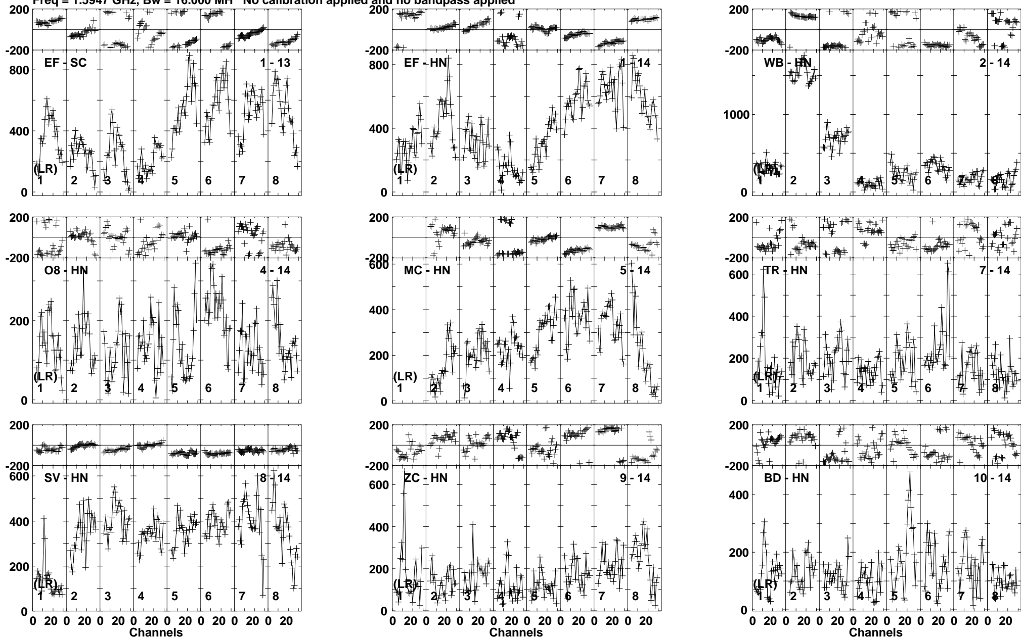
Lower frame: Micro Ampl Jy Top frame: Phas deg Vector averaged cross-power spectrum Baseline: EF (01) - SC (13) Timerange: 00/22:24:23 to 00/22:26:13
