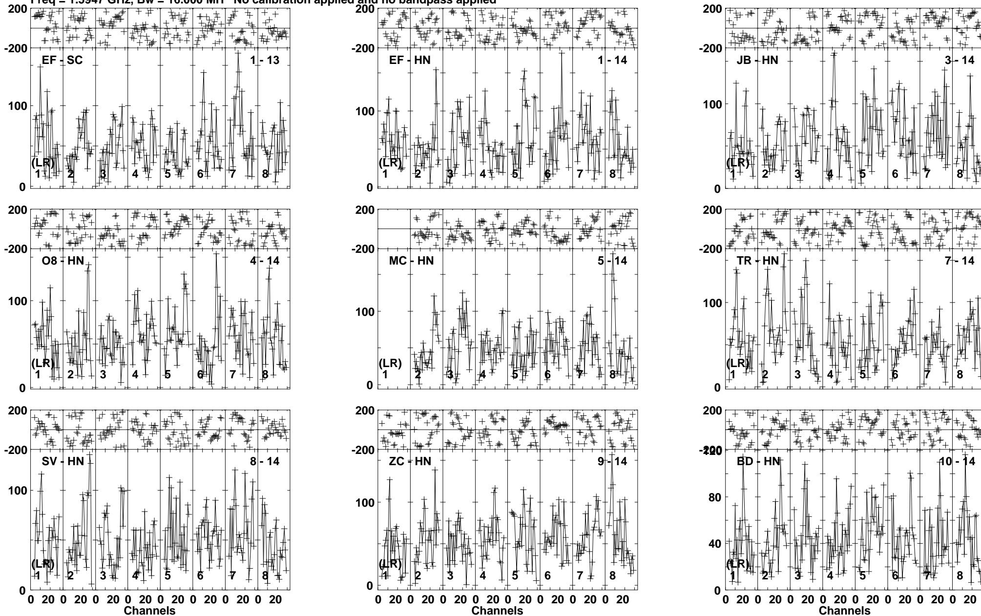
Lower frame: Micro Ampl Jy Top frame: Phas deg Vector averaged cross-power spectrum Baseline: EF (01) - SC (13) Timerange: 01/01:40:56 to 01/01:46:06
