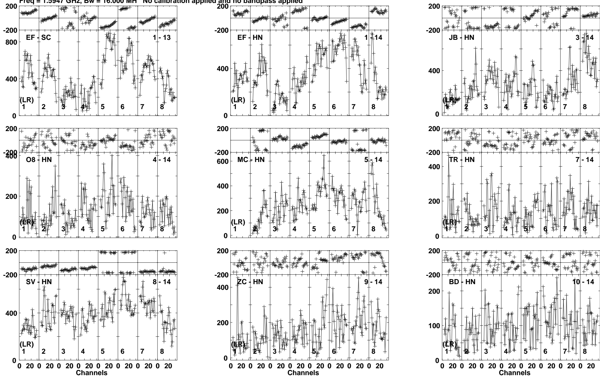
Lower frame: Micro Ampl Jy Top frame: Phas deg Vector averaged cross-power spectrum Baseline: EF (01) - SC (13) Timerange: 01/00:12:35 to 01/00:14:17
