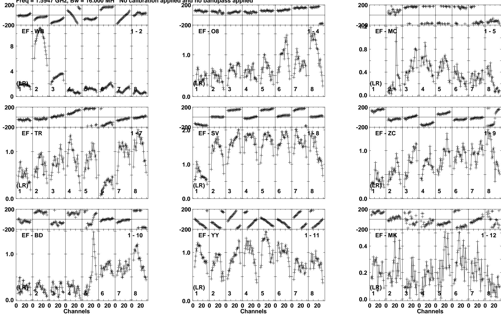
Lower frame: Milli Ampl Jy Top frame: Phas deg Vector averaged cross-power spectrum Baseline: EF (01) - WB (02) Timerange: 00:21:41:09 to 00:21:42:58
