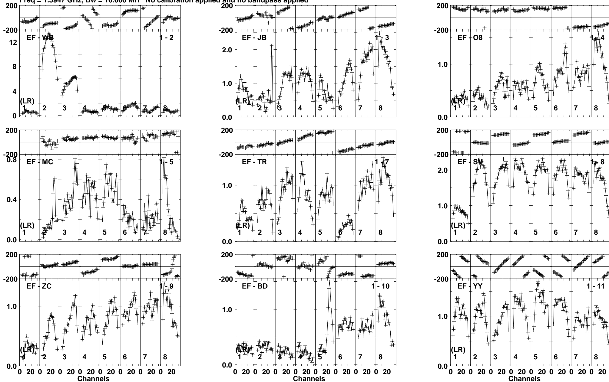
Lower frame: Milli Ampl Jy Top frame: Phas deg Vector averaged cross-power spectrum Baseline: EF (01) - WB (02) Timerange: 00/21:34:01 to 00/21:35:42
