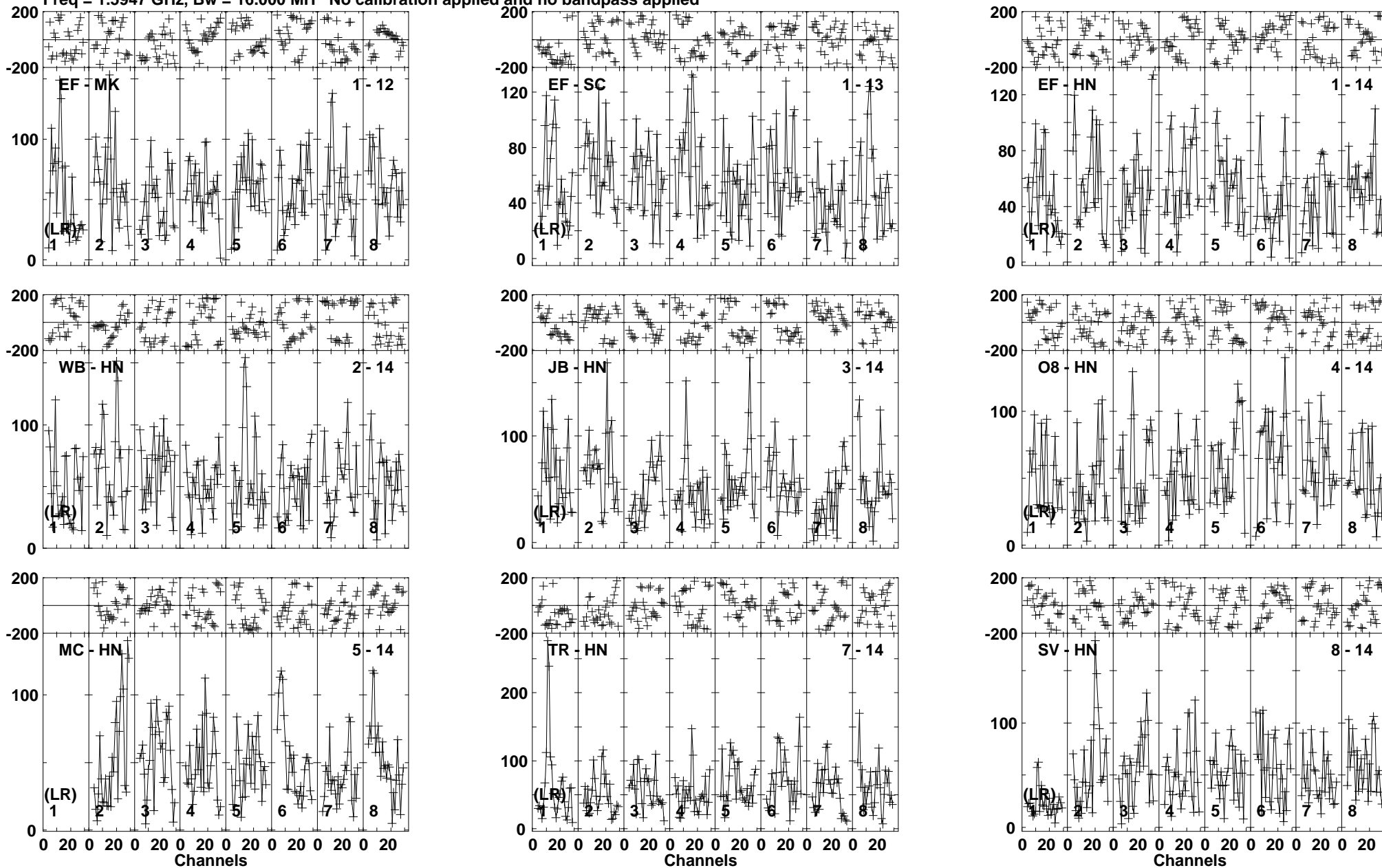
Lower frame: Micro Ampl Jy Top frame: Phas deg Vector averaged cross-power spectrum Baseline: EF (01) - MK (12) Timerange: 00/20:52:36 to 00/20:57:46
