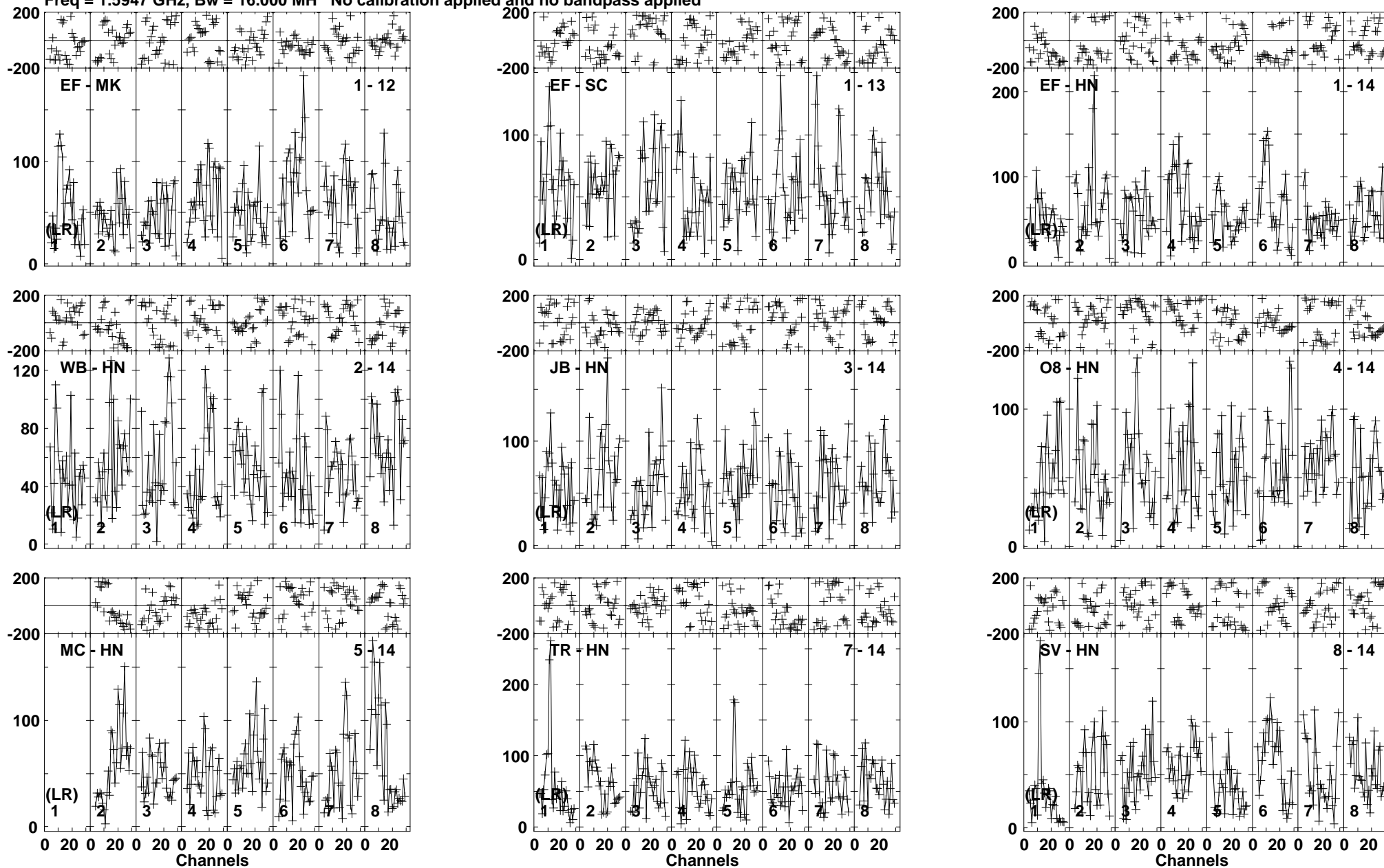
Lower frame: Micro Ampl Jy Top frame: Phas deg Vector averaged cross-power spectrum Baseline: EF (01) - MK (12) Timerange: 00/21:50:16 to 00/21:55:26
