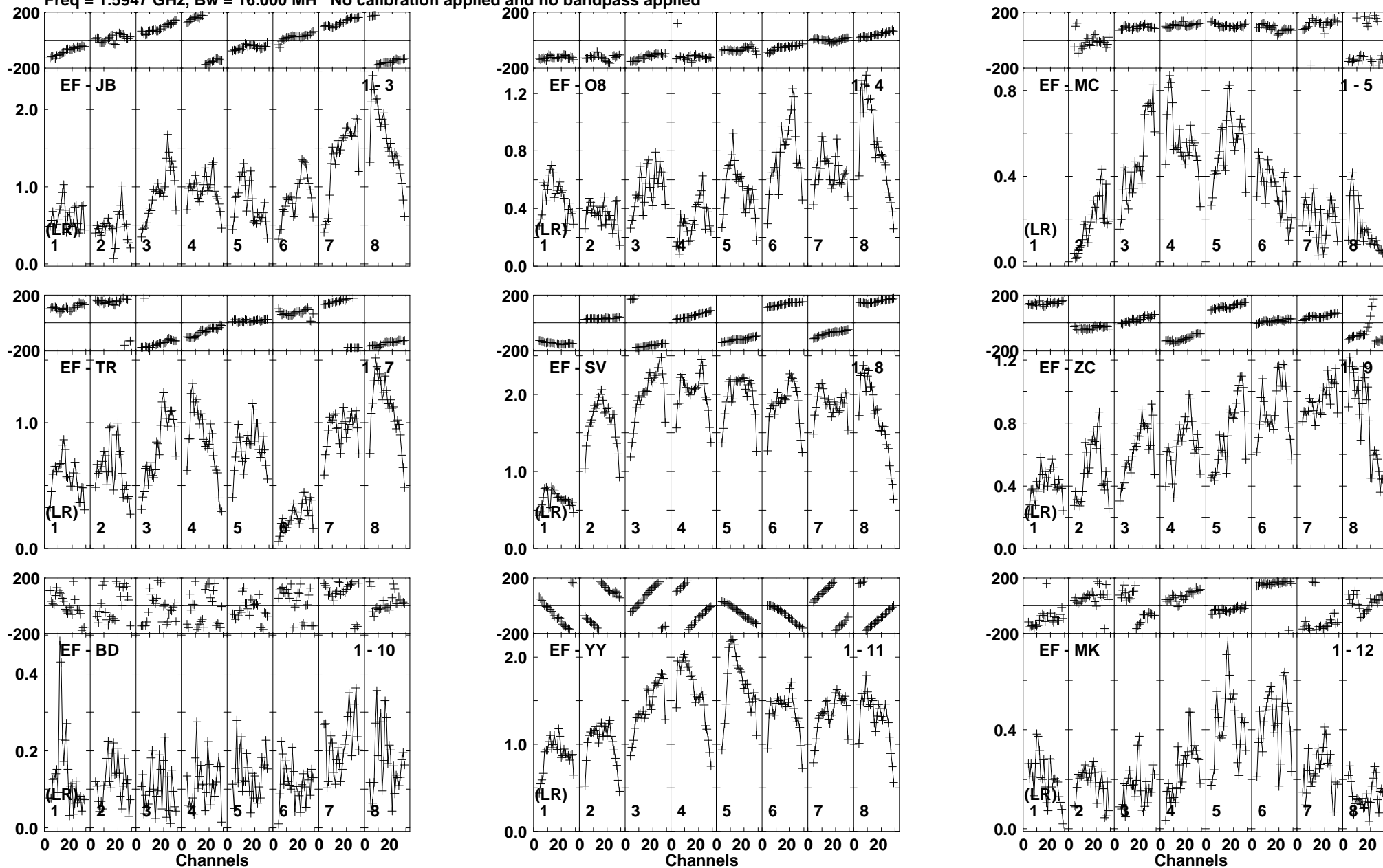
Lower frame: Milli Ampl Jy Top frame: Phas deg Vector averaged cross-power spectrum Baseline: EF (01) - JB (03) Timerange: 01/00:12:35 to 01/00:14:17
