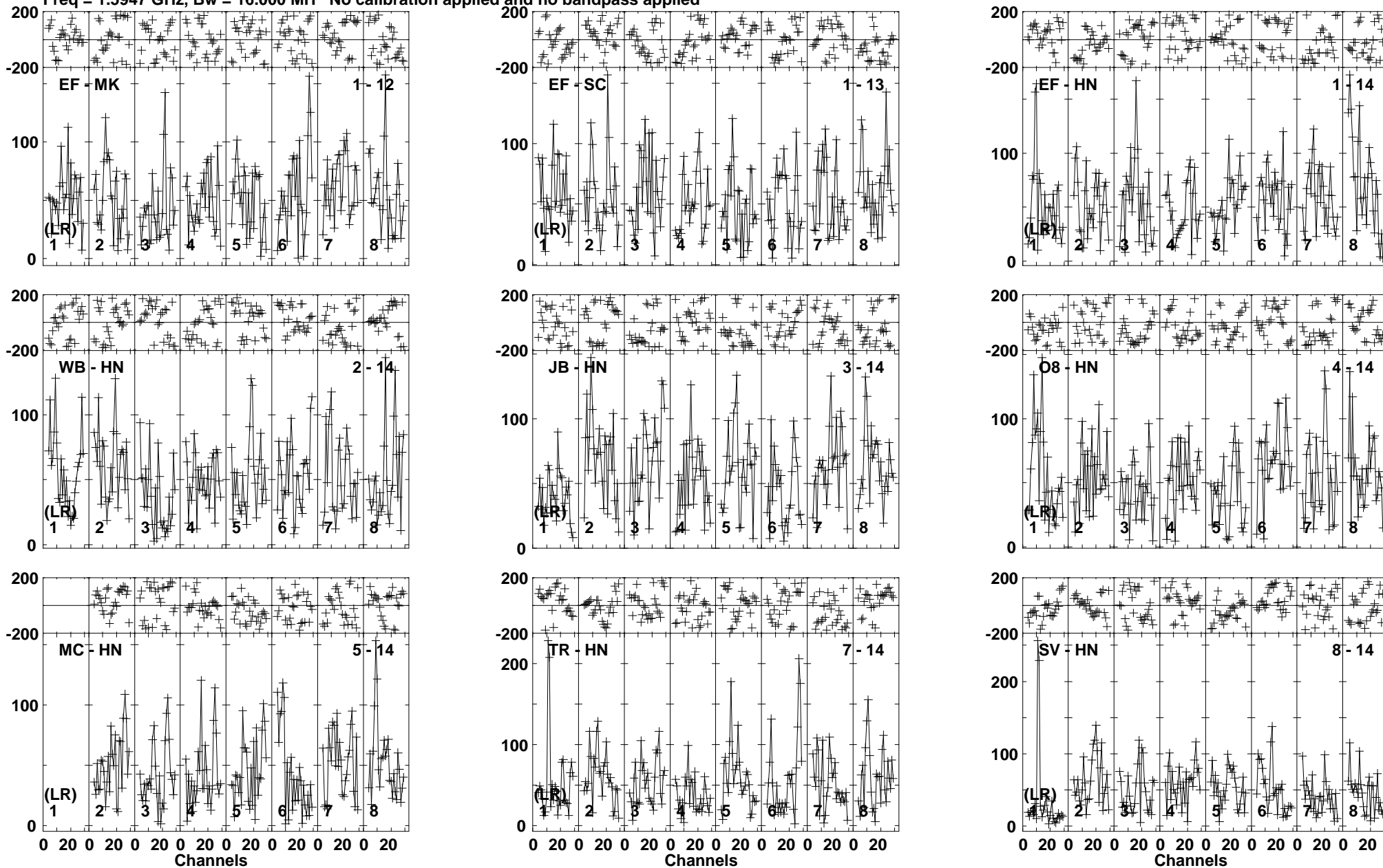
Lower frame: Micro Ampl Jy Top frame: Phas deg Vector averaged cross-power spectrum Baseline: EF (01) - MK (12) Timerange: 00/21:07:01 to 00/21:12:11
