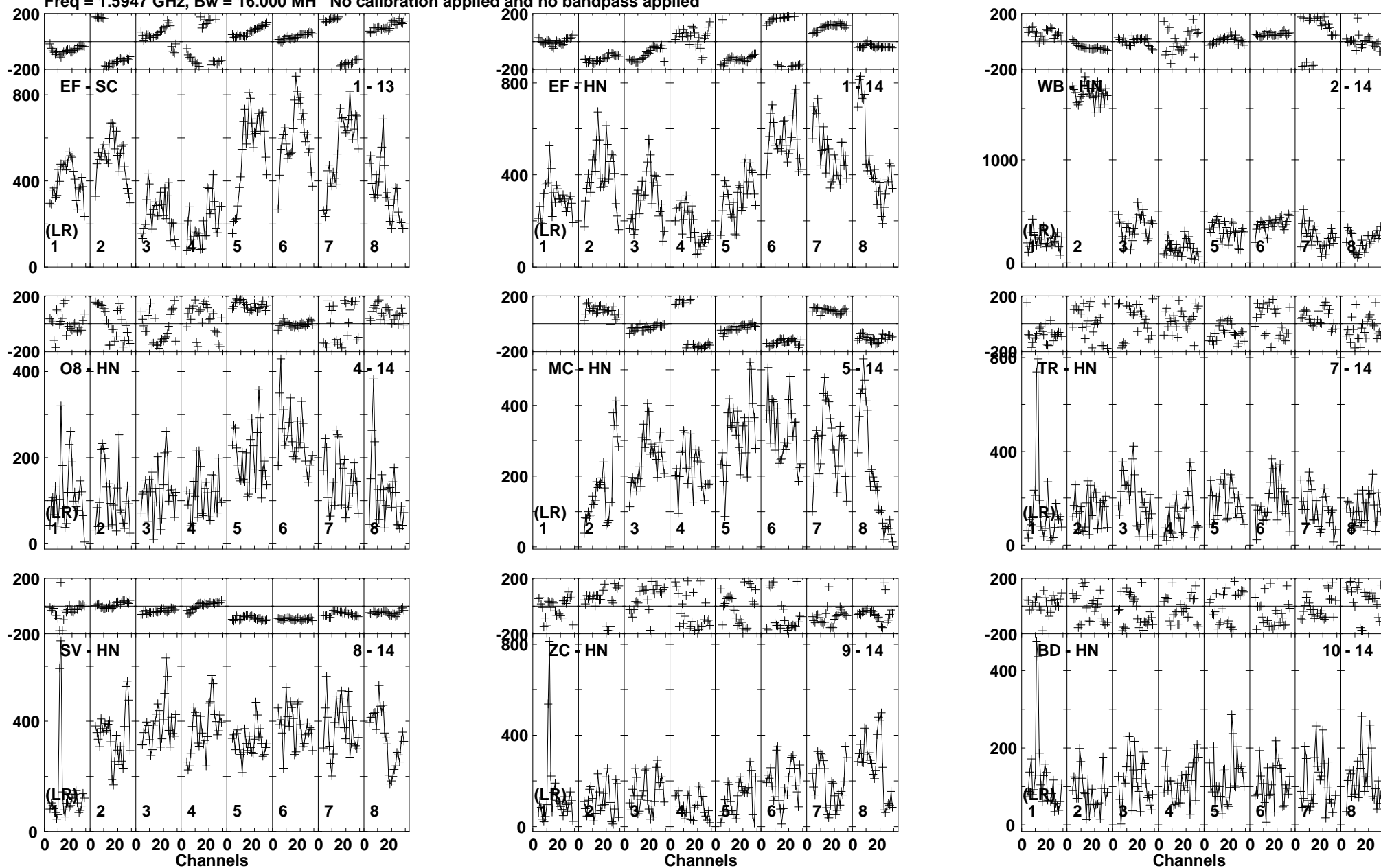
Lower frame: Micro Ampl Jy Top frame: Phas deg Vector averaged cross-power spectrum Baseline: EF (01) - SC (13) Timerange: 00/22:53:13 to 00/22:55:03
