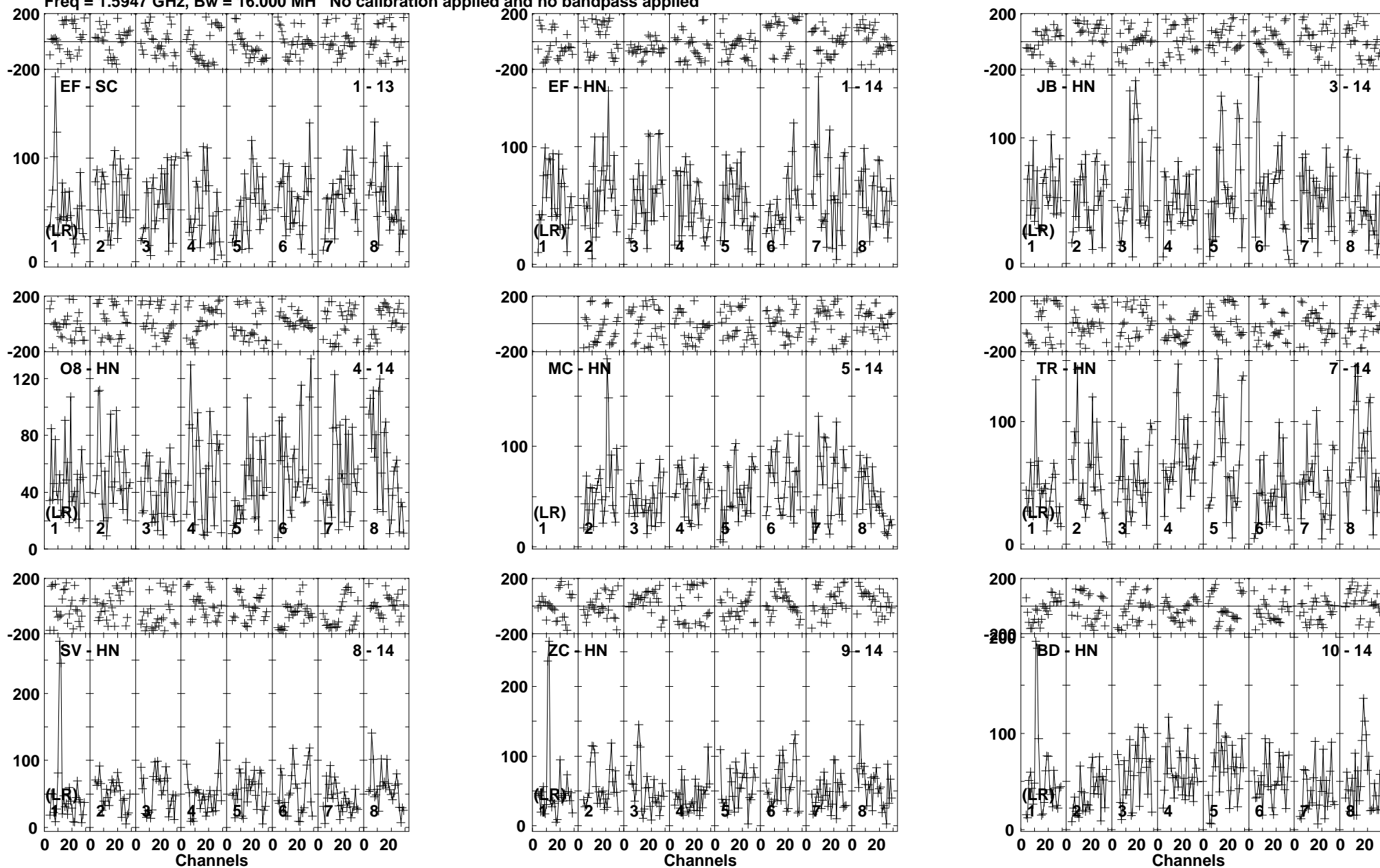
Lower frame: Micro Ampl Jy Top frame: Phas deg Vector averaged cross-power spectrum Baseline: EF (01) - SC (13) Timerange: 01/00:00:00 to 01/00:05:10
