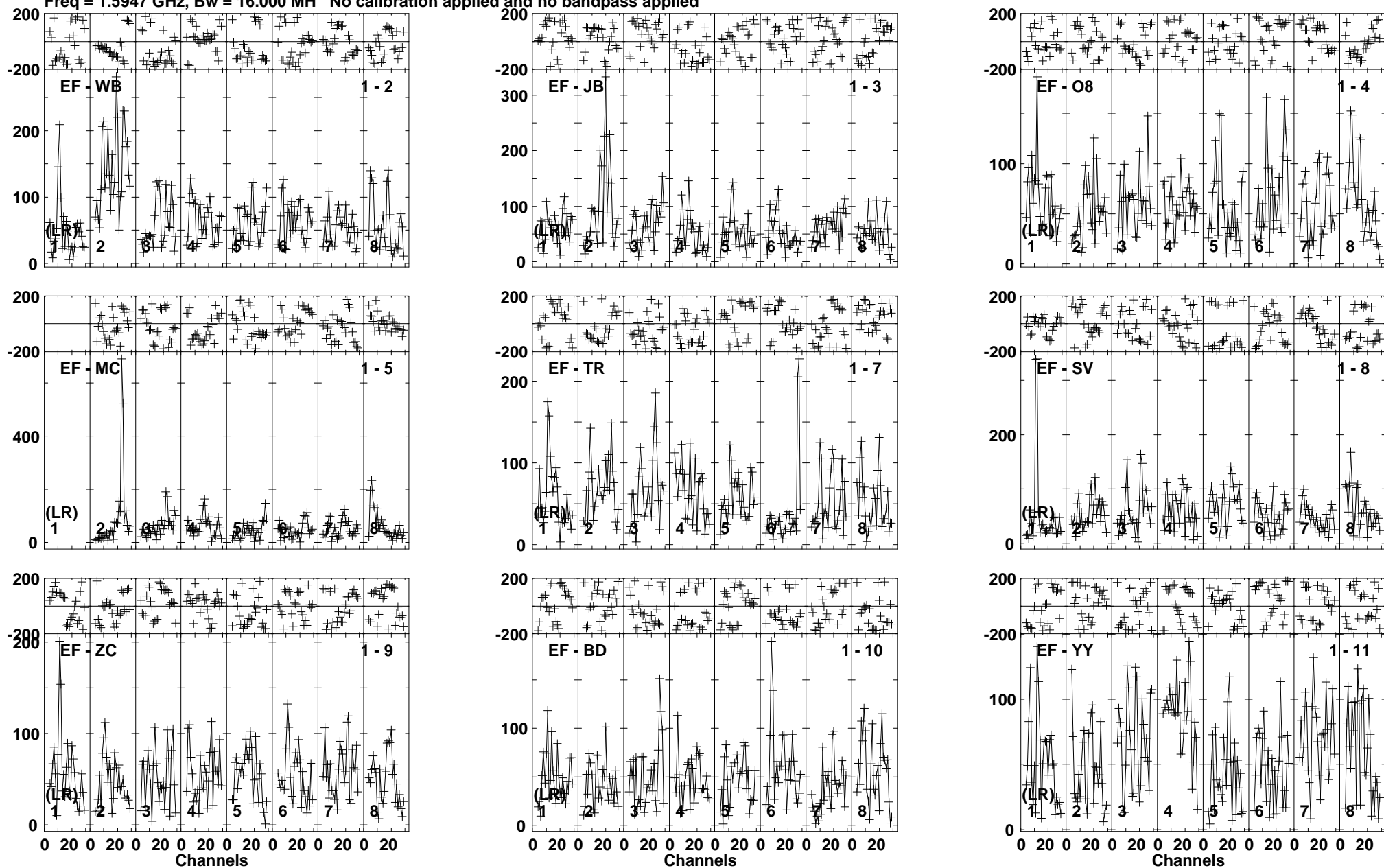
Lower frame: Micro Ampl Jy Top frame: Phas deg Vector averaged cross-power spectrum Baseline: EF (01) - WB (02) Timerange: 00/22:26:18 to 00/22:31:32
