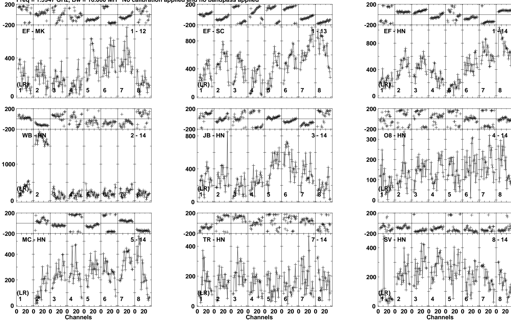
Lower frame: Micro Ampl Jy Top frame: Phas deg Vector averaged cross-power spectrum Baseline: EF (01) - MK (12) Timerange: 00/20:36:21 to 00/20:38:02
