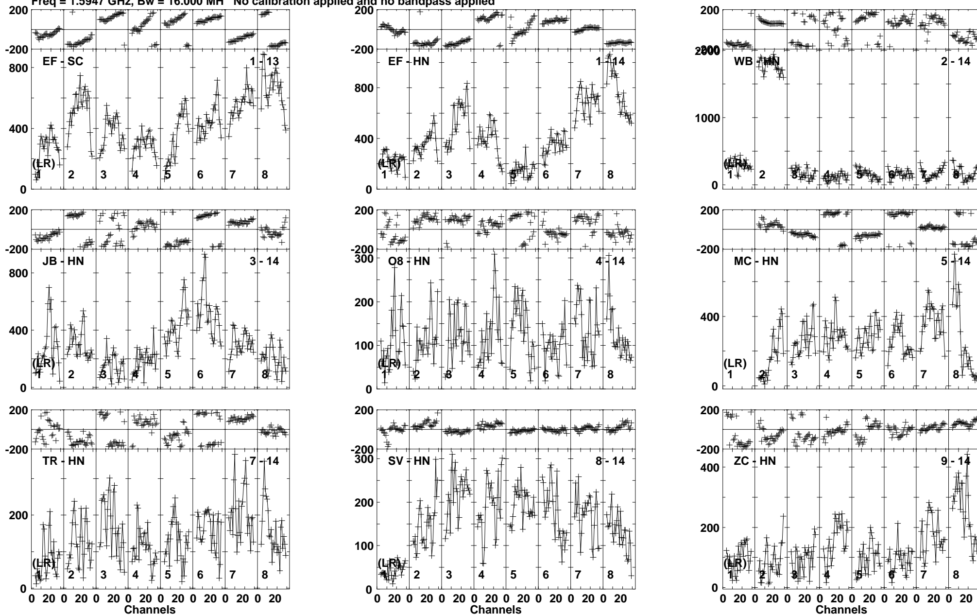
Lower frame: Micro Ampl Jy Top frame: Phas deg Vector averaged cross-power spectrum Baseline: EF (01) - SC (13) Timerange: 00/20:05:17 to 00/20:09:12
