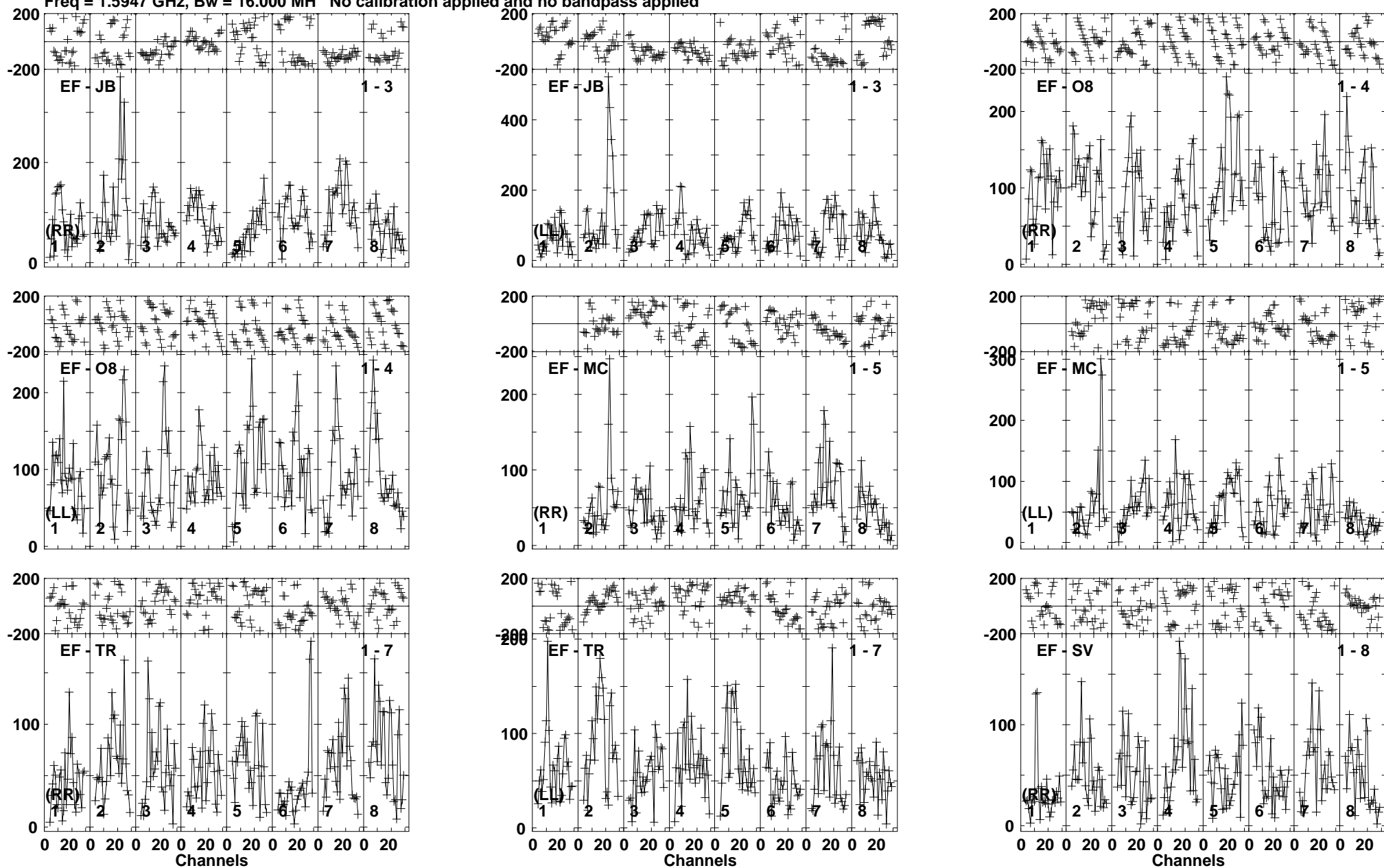
Lower frame: Micro Ampl Jy Top frame: Phas deg Vector averaged cross-power spectrum Baseline: EF (01) - JB (03) Timerange: 01/00:14:25 to 01/00:19:35
