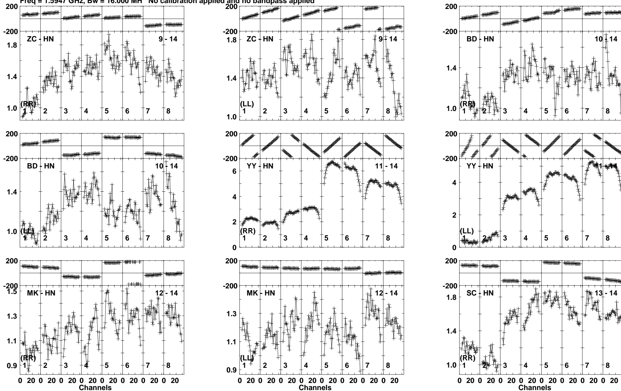
Lower frame: Milli Ampl Jy Top frame: Phas deg Vector averaged cross-power spectrum Baseline: ZC (09) - HN (14) Timerange: 00/20:50:46 to 00/20:52:27
