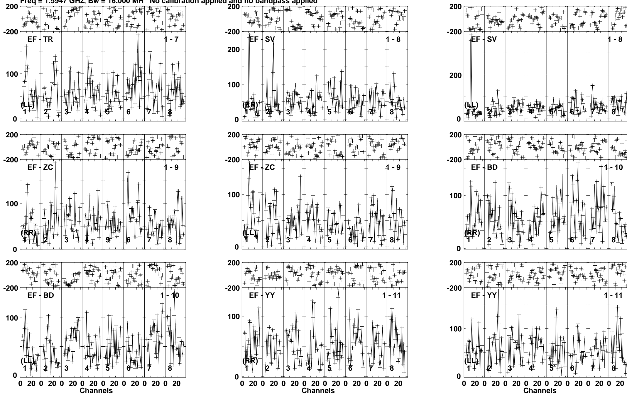
Lower frame: Micro Ampl Jy Top frame: Phas deg Vector averaged cross-power spectrum Baseline: EF (01) - TR (07) Timerange: 00/21:57:28 to 00/22:02:42
