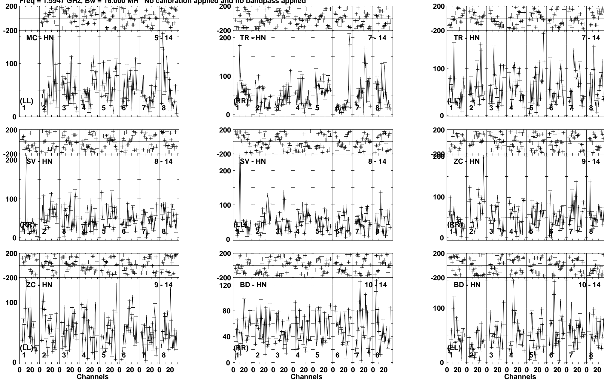
Lower frame: Micro Ampl Jy Top frame: Phas deg Vector averaged cross-power spectrum Baseline: MC (05) - HN (14) Timerange: 01/01:33:43 to 01/01:38:57
