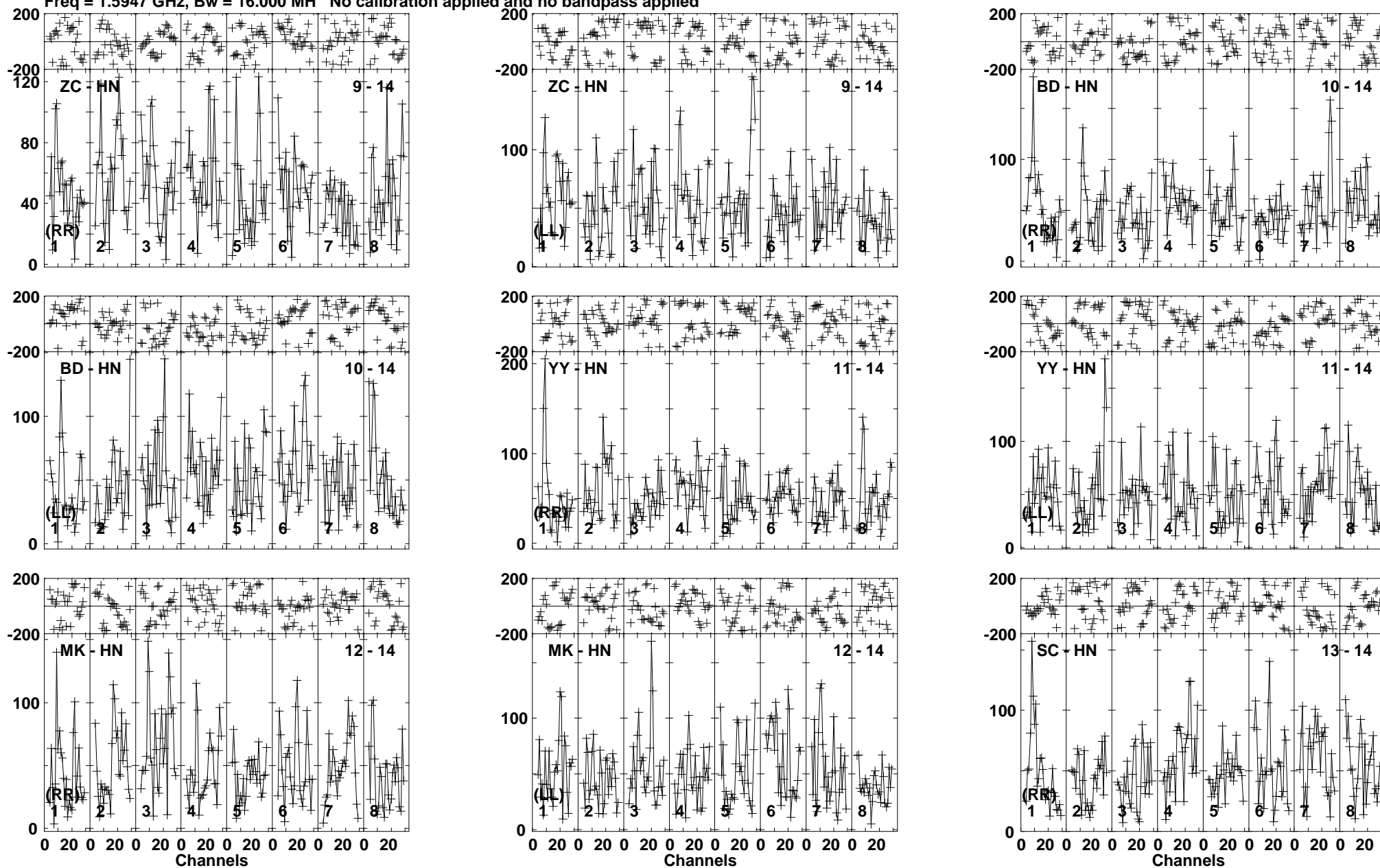
Lower frame: Micro Ampl Jy Top frame: Phas deg Vector averaged cross-power spectrum Baseline: ZC (09) - HN (14) Timerange: 00/21:14:13 to 00/21:19:27
