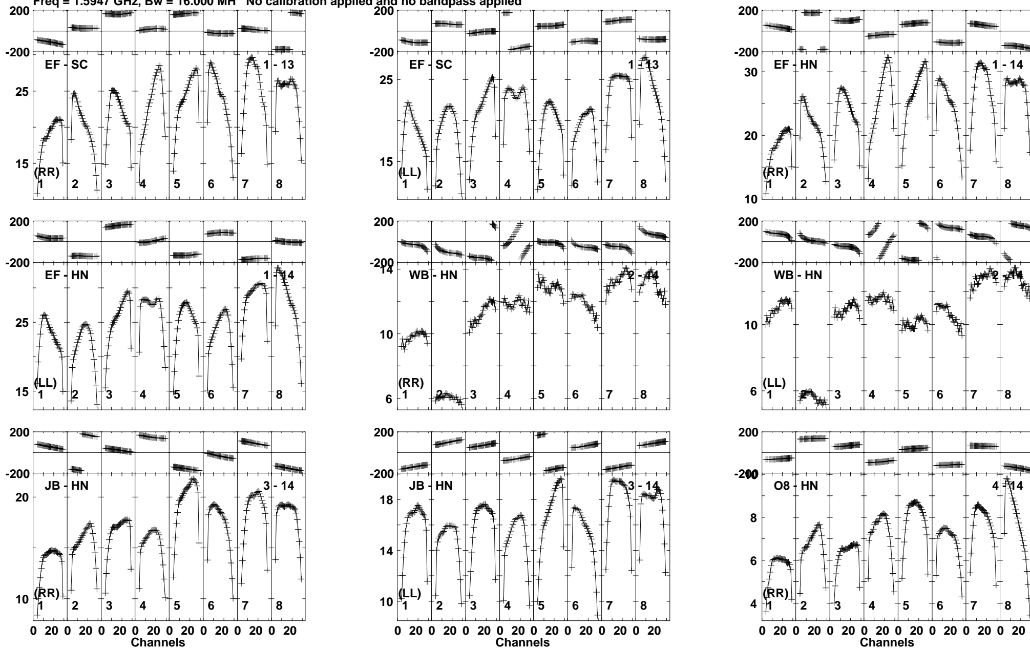
Lower frame: Milli Ampl Jy Top frame: Phas deg Vector averaged cross-power spectrum Baseline: EF (01) - SC (13) Timerange: 00/20:00:01 to 00/20:04:55
