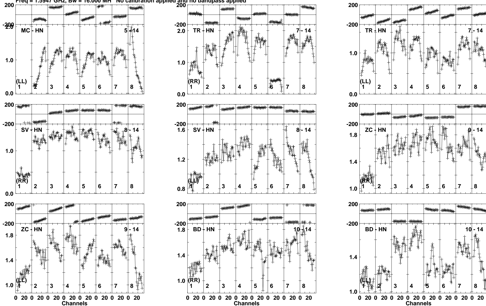
Lower frame: Milli Ampl Jy Top frame: Phas deg Vector averaged cross-power spectrum Baseline: MC (05) - HN (14) Timerange: 01/00:41:26 to 01/00:43:07
