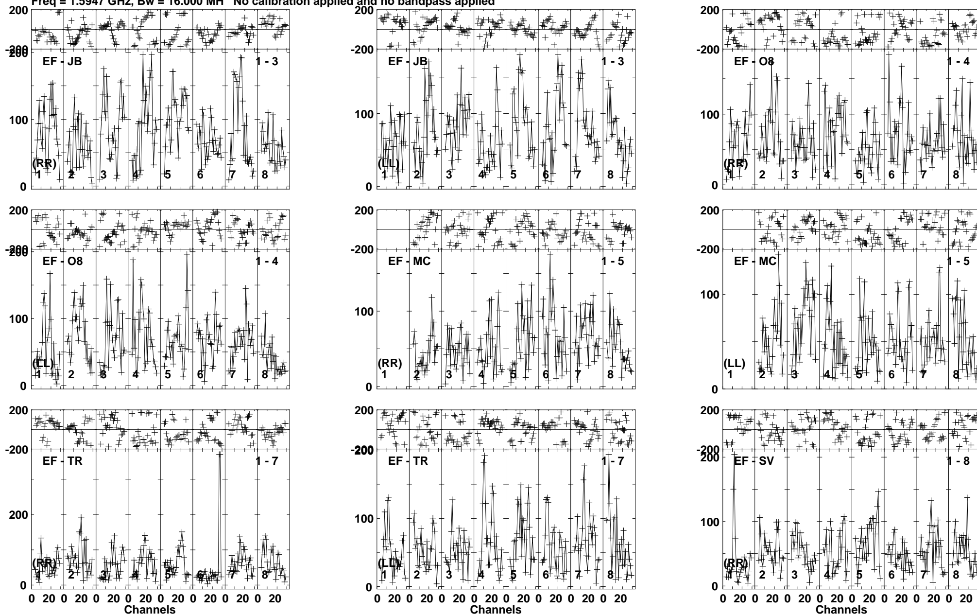
Lower frame: Micro Ampl Jy Top frame: Phas deg Vector averaged cross-power spectrum Baseline: EF (01) - JB (03) Timerange: 01/00:00:00 to 01/00:05:10
