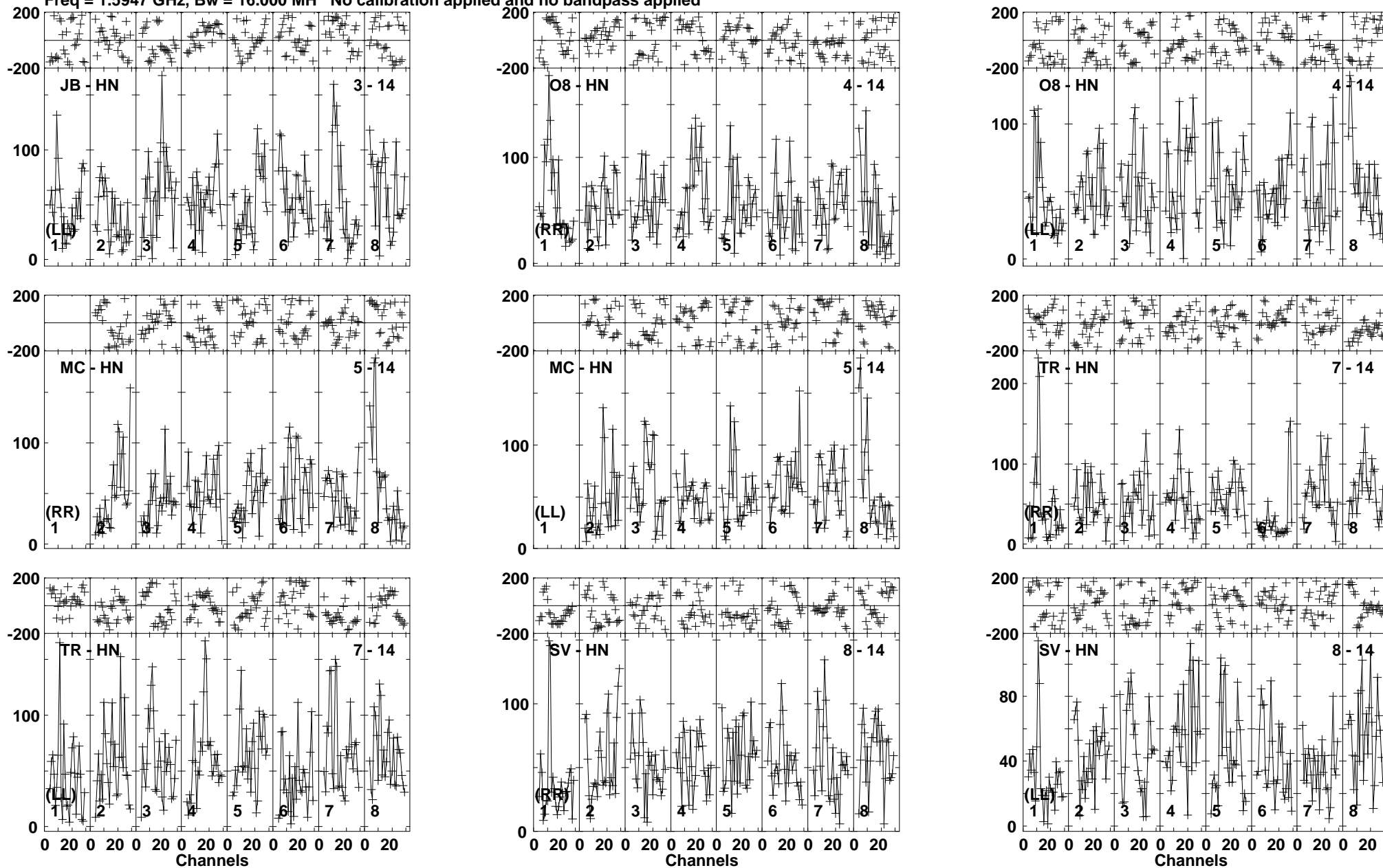
Lower frame: Micro Ampl Jy Top frame: Phas deg Vector averaged cross-power spectrum Baseline: JB (03) - HN (14) Timerange: 00/22:11:53 to 00/22:17:07
