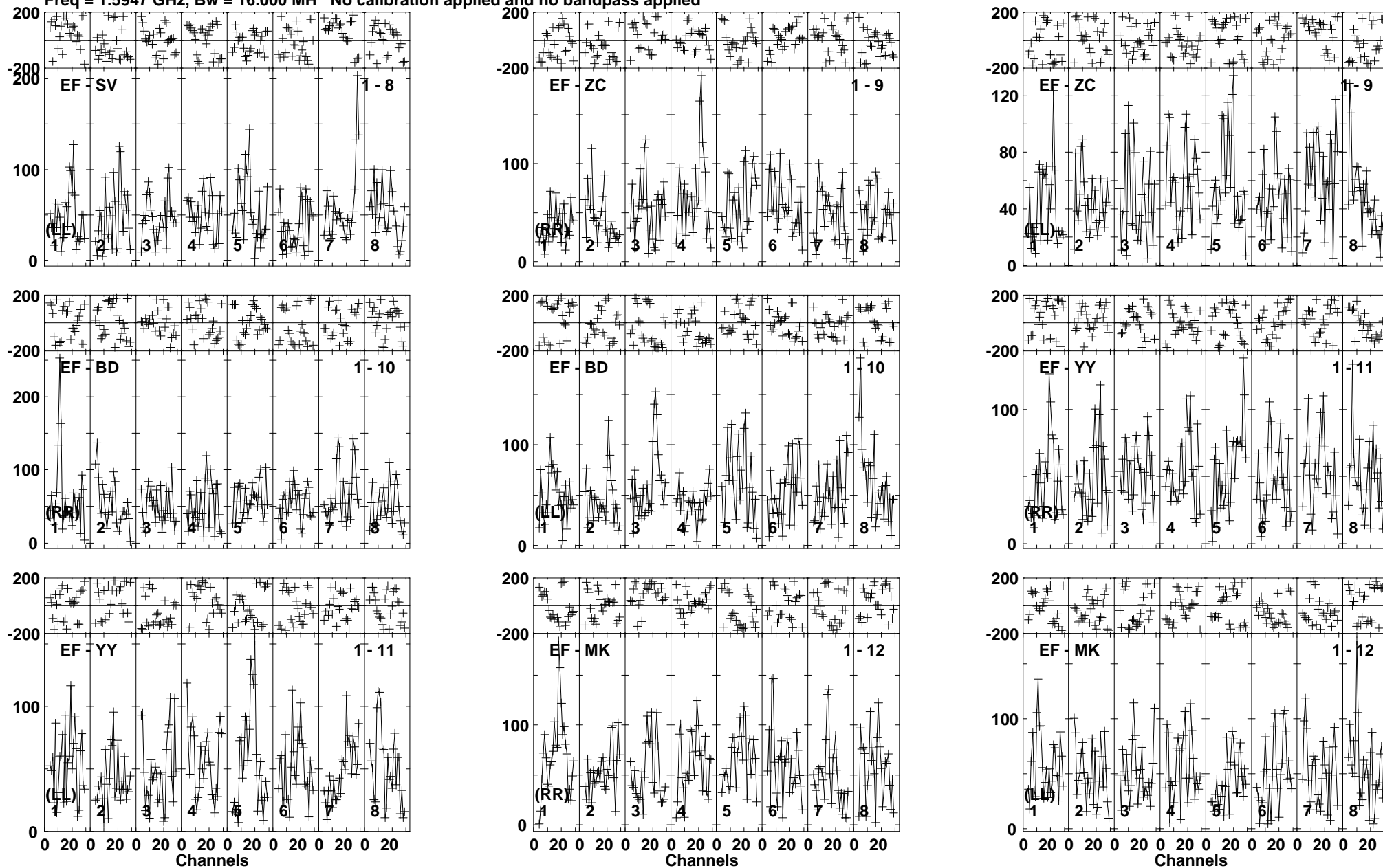
Lower frame: Micro Ampl Jy Top frame: Phas deg Vector averaged cross-power spectrum Baseline: EF (01) - SV (08) Timerange: 01/00:21:38 to 01/00:26:52
