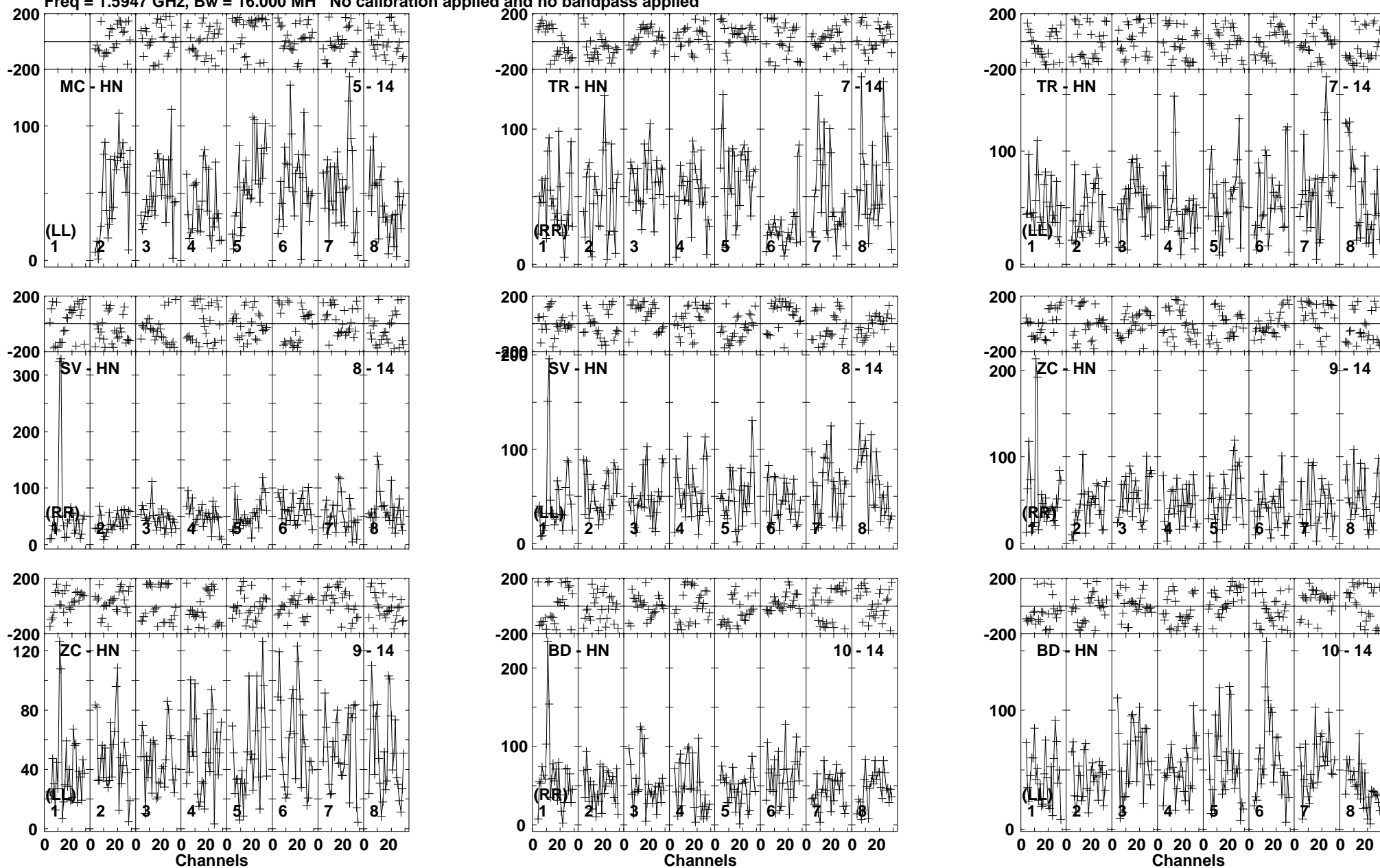
Lower frame: Micro Ampl Jy Top frame: Phas deg Vector averaged cross-power spectrum Baseline: MC (05) - HN (14) Timerange: 01/00:00:00 to 01/00:05:10
