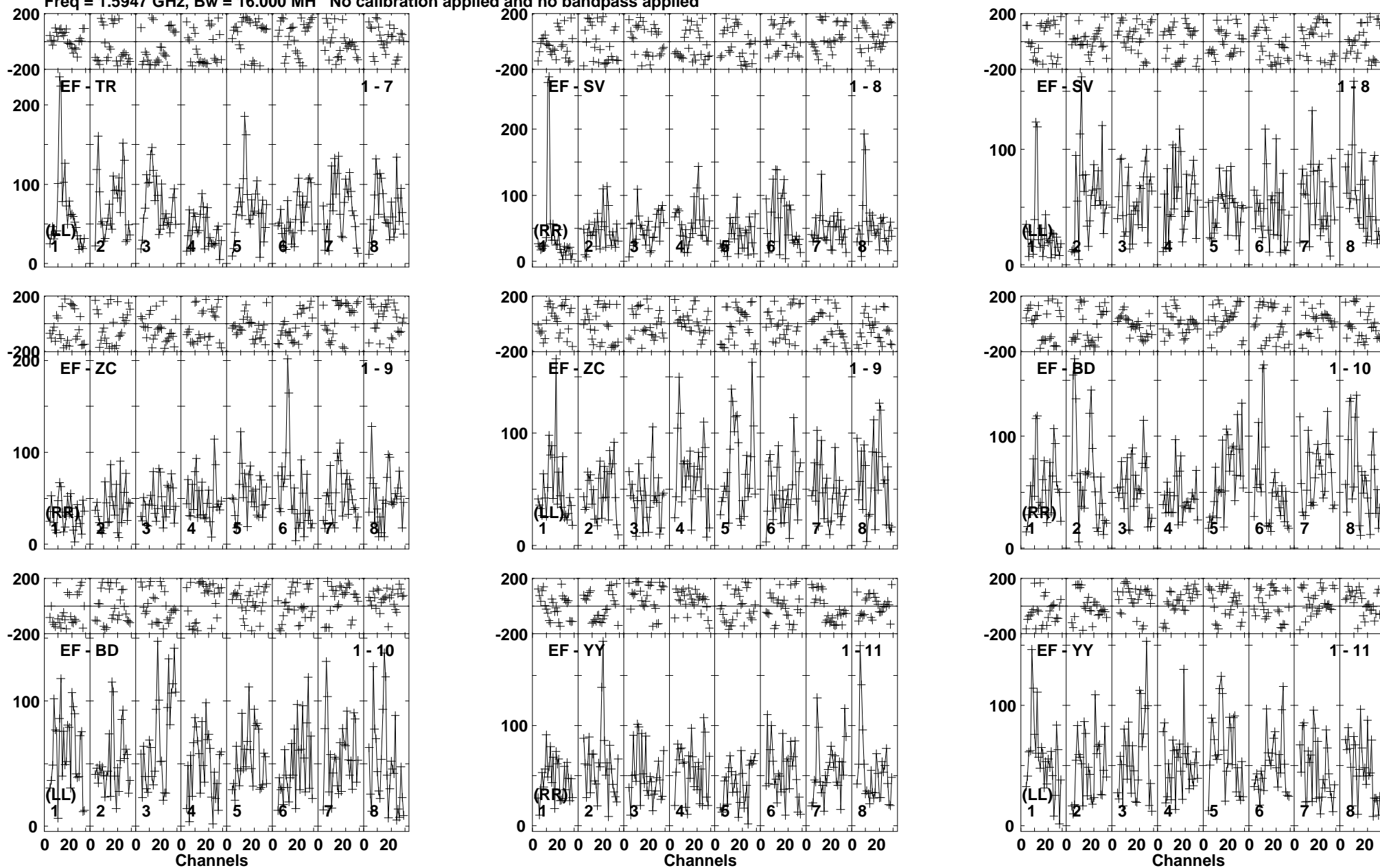
Lower frame: Micro Ampl Jy Top frame: Phas deg Vector averaged cross-power spectrum Baseline: EF (01) - TR (07) Timerange: 00/20:38:11 to 00/20:43:21
