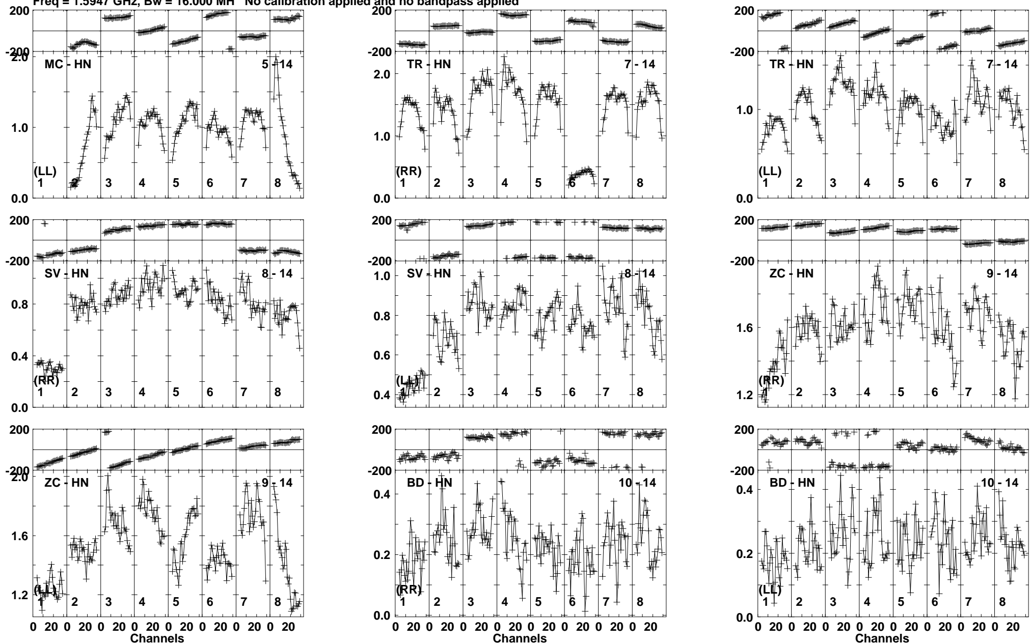
Lower frame: Milli Ampl Jy Top frame: Phas deg Vector averaged cross-power spectrum Baseline: MC (05) - HN (14) Timerange: 00/23:58:10 to 00/23:59:52
