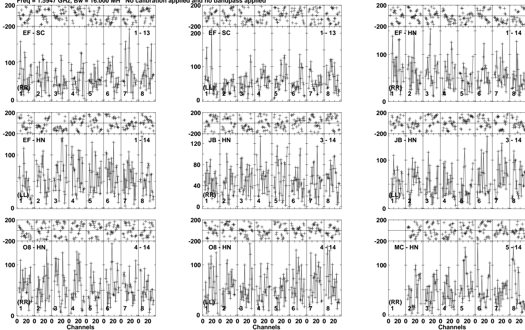
Lower frame: Micro Ampl Jy Top frame: Phas deg Vector averaged cross-power spectrum Baseline: EF (01) - SC (13) Timerange: 00/23:52:48 to 00/23:58:02
