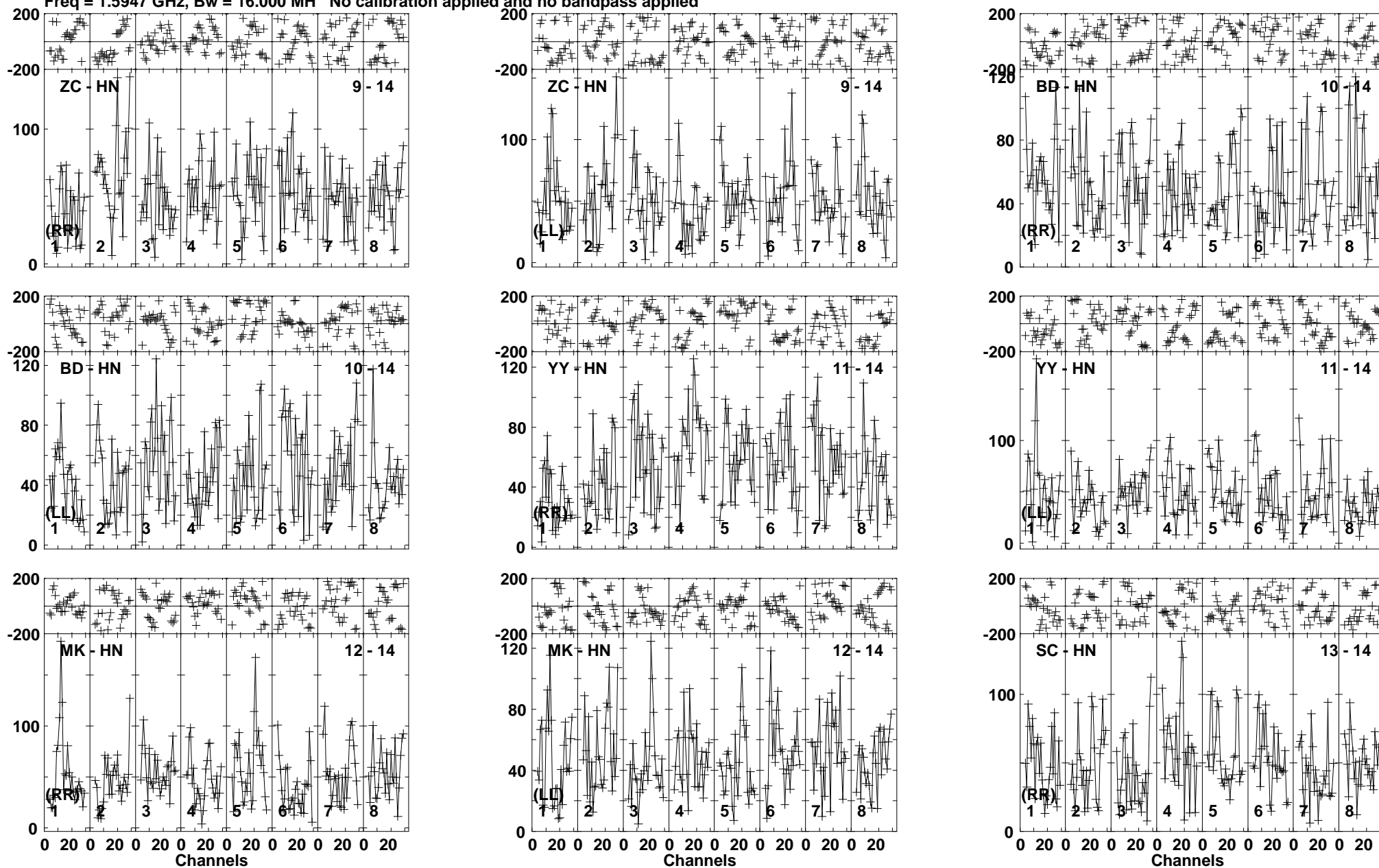
Lower frame: Micro Ampl Jy Top frame: Phas deg Vector averaged cross-power spectrum Baseline: ZC (09) - HN (14) Timerange: 00/22:26:18 to 00/22:31:32
