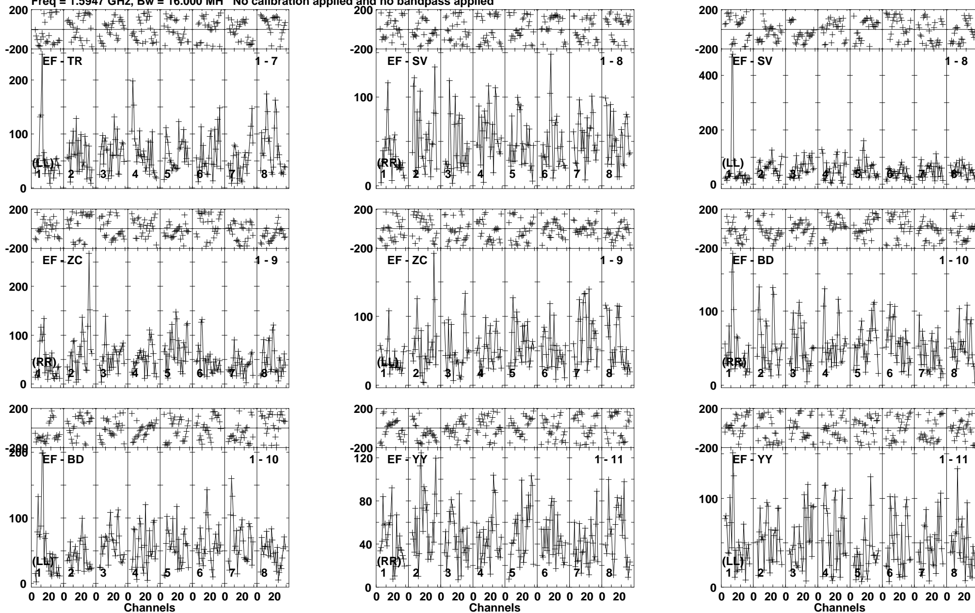
Lower frame: Micro Ampl Jy Top frame: Phas deg Vector averaged cross-power spectrum Baseline: EF (01) - TR (07) Timerange: 00/23:16:45 to 00/23:21:55
