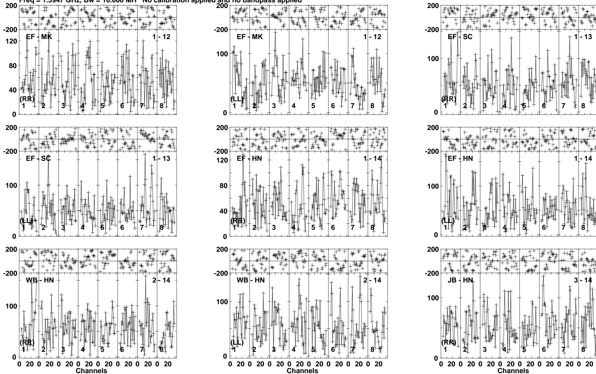
Lower frame: Micro Ampl Jy Top frame: Phas deg Vector averaged cross-power spectrum Baseline: EF (01) - MK (12) Timerange: 00/23:38:23 to 00/23:43:37
