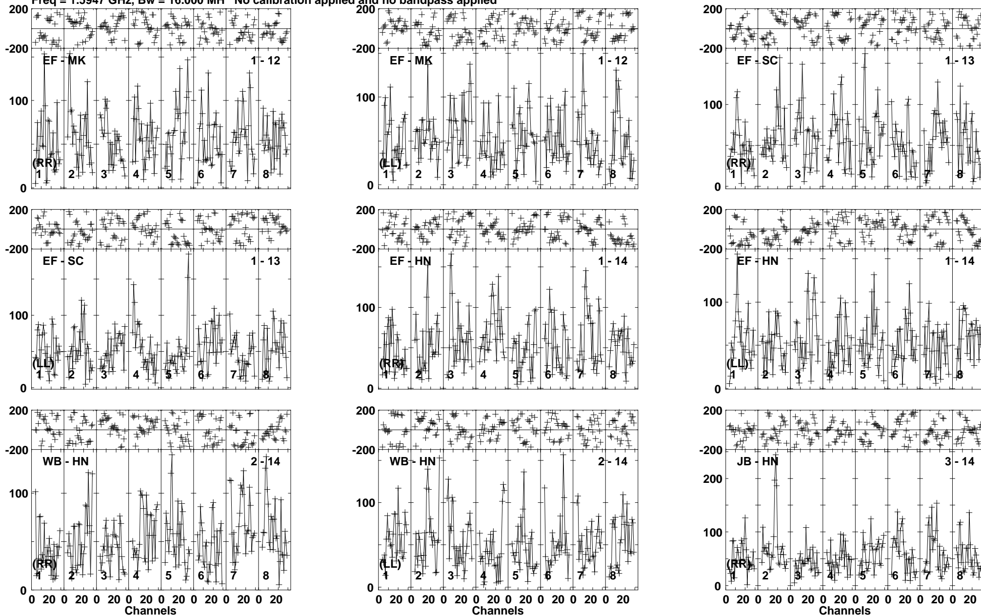
Lower frame: Micro Ampl Jy Top frame: Phas deg Vector averaged cross-power spectrum Baseline: EF (01) - MK (12) Timerange: 00/23:02:20 to 00/23:07:30
