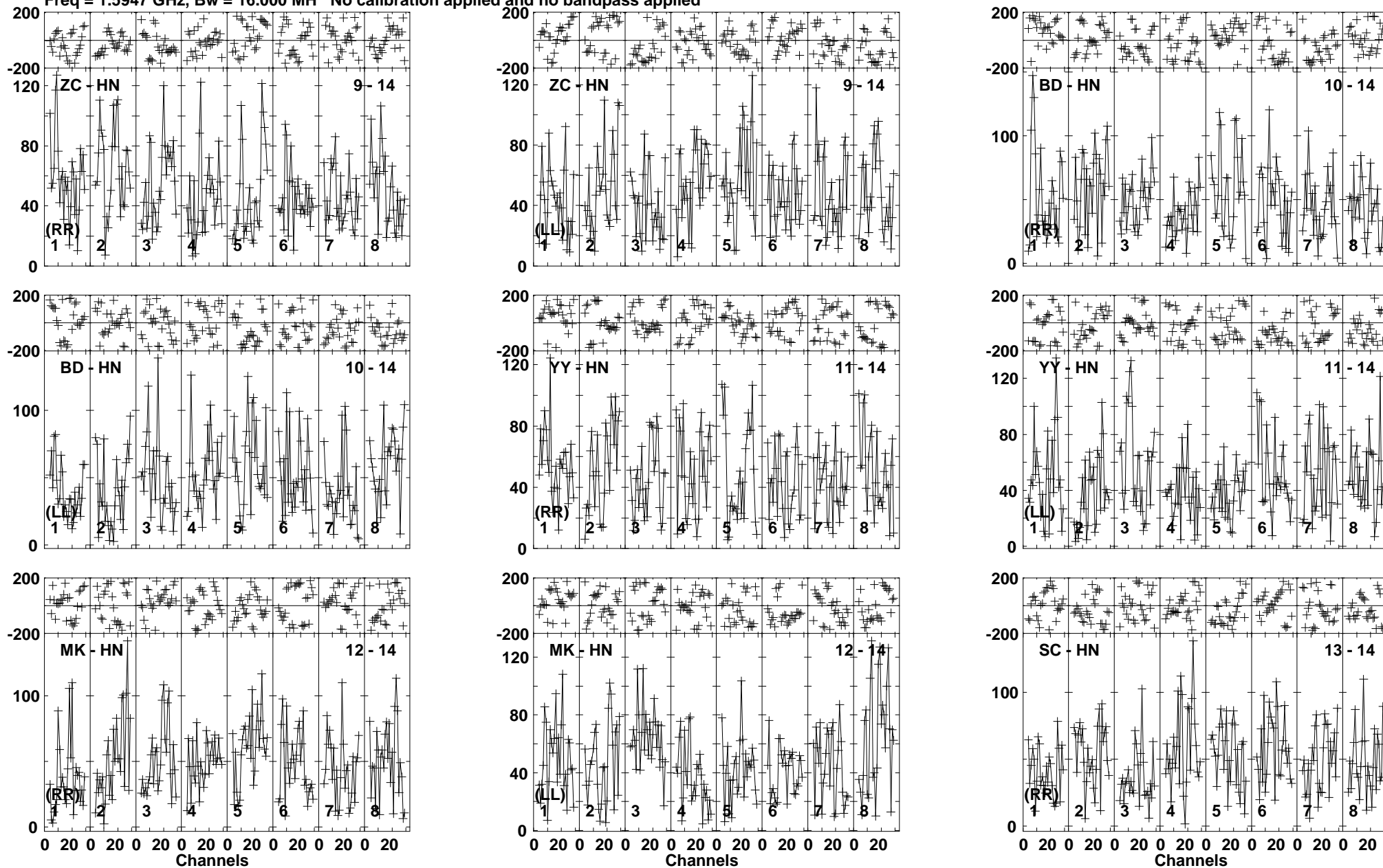
Lower frame: Micro Ampl Jy Top frame: Phas deg Vector averaged cross-power spectrum Baseline: ZC (09) - HN (14) Timerange: 00/23:31:10 to 00/23:36:20
