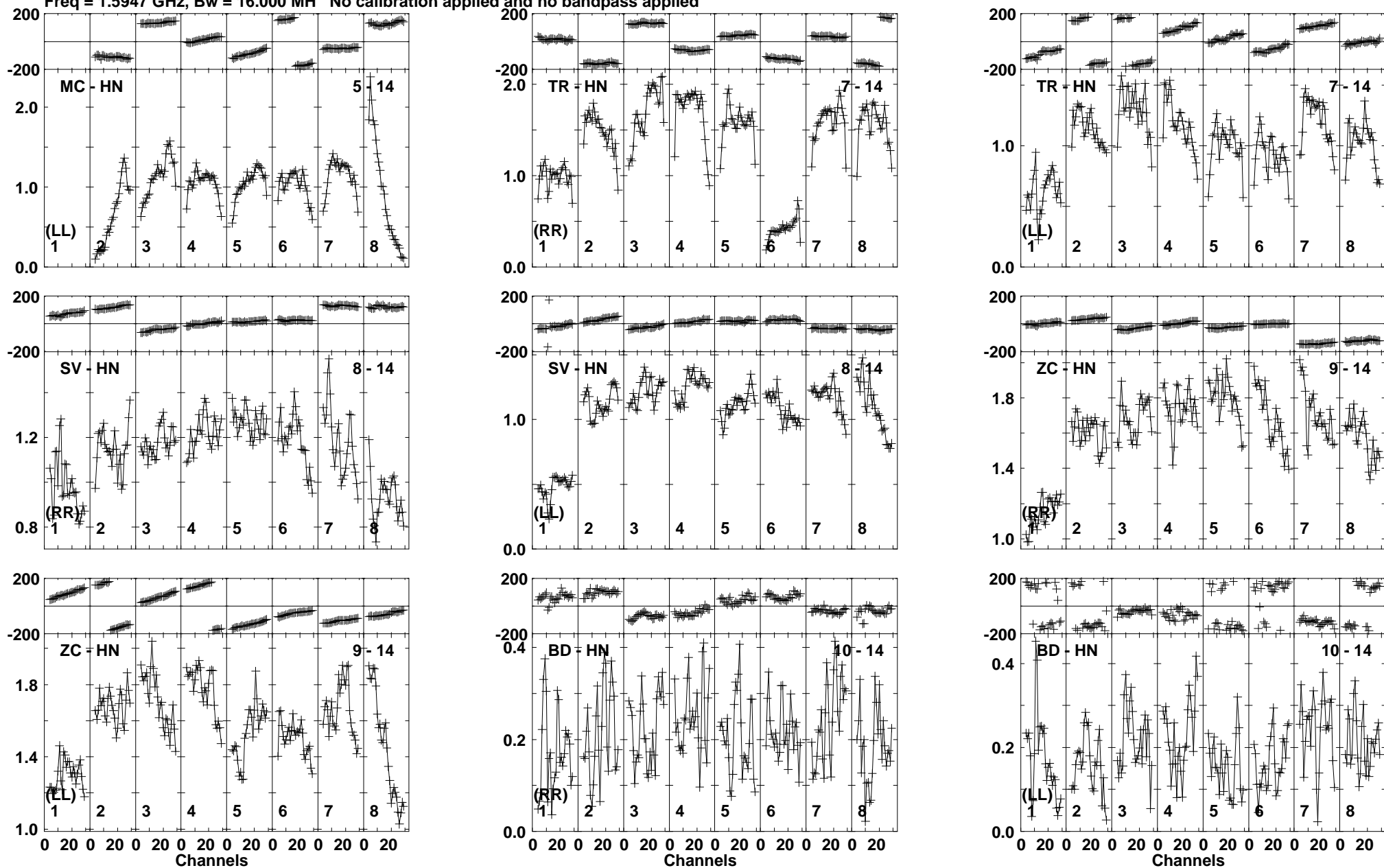
Lower frame: Milli Ampl Jy Top frame: Phas deg Vector averaged cross-power spectrum Baseline: MC (05) - HN (14) Timerange: 00/23:22:03 to 00/23:23:53
