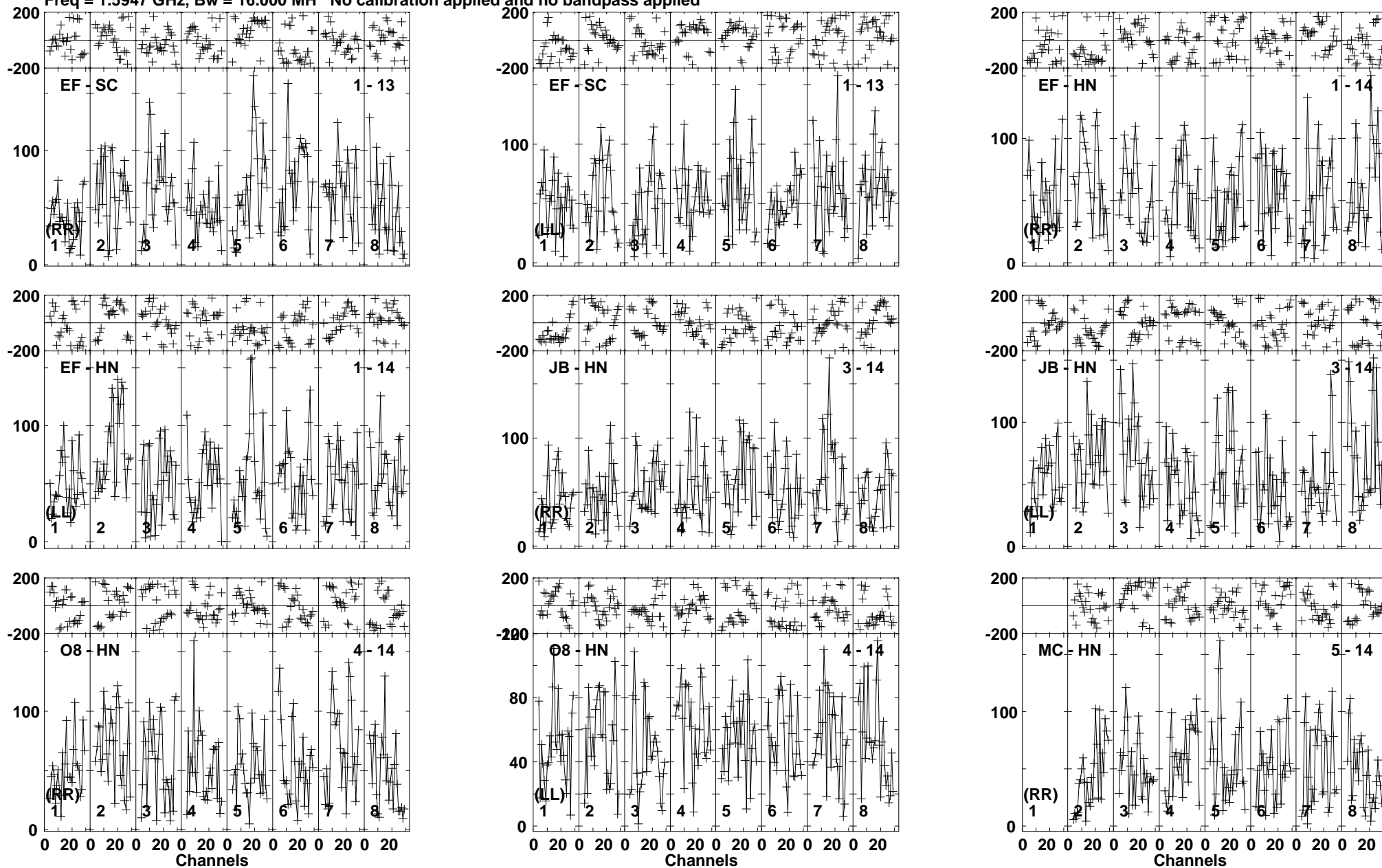
Lower frame: Micro Ampl Jy Top frame: Phas deg Vector averaged cross-power spectrum Baseline: EF (01) - SC (13) Timerange: 01/00:14:25 to 01/00:19:35
