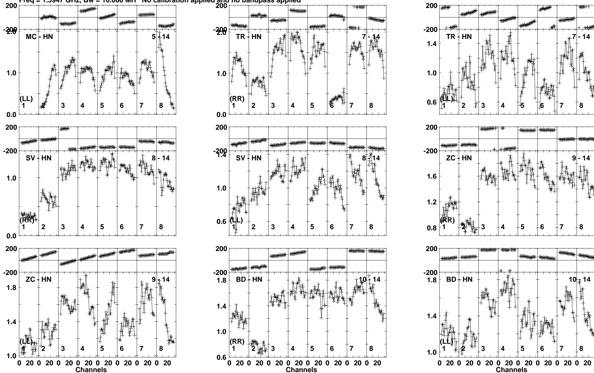
Lower frame: Milli Ampl Jy Top frame: Phas deg Vector averaged cross-power spectrum Baseline: MC (05) - HN (14) Timerange: 01/01:10:16 to 01/01:11:57
