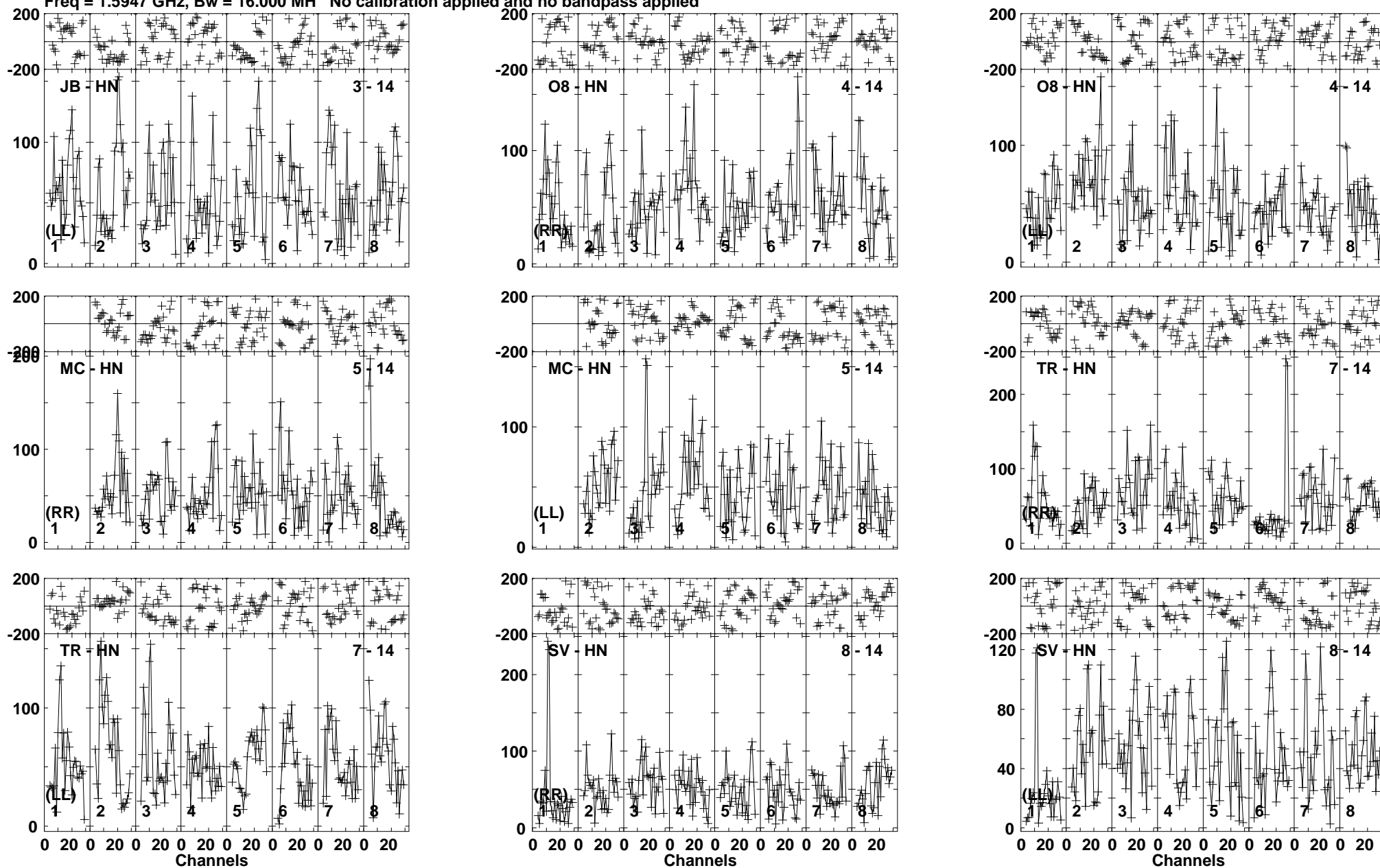
Lower frame: Micro Ampl Jy Top frame: Phas deg Vector averaged cross-power spectrum Baseline: JB (03) - HN (14) Timerange: 00/21:35:51 to 00/21:41:01
