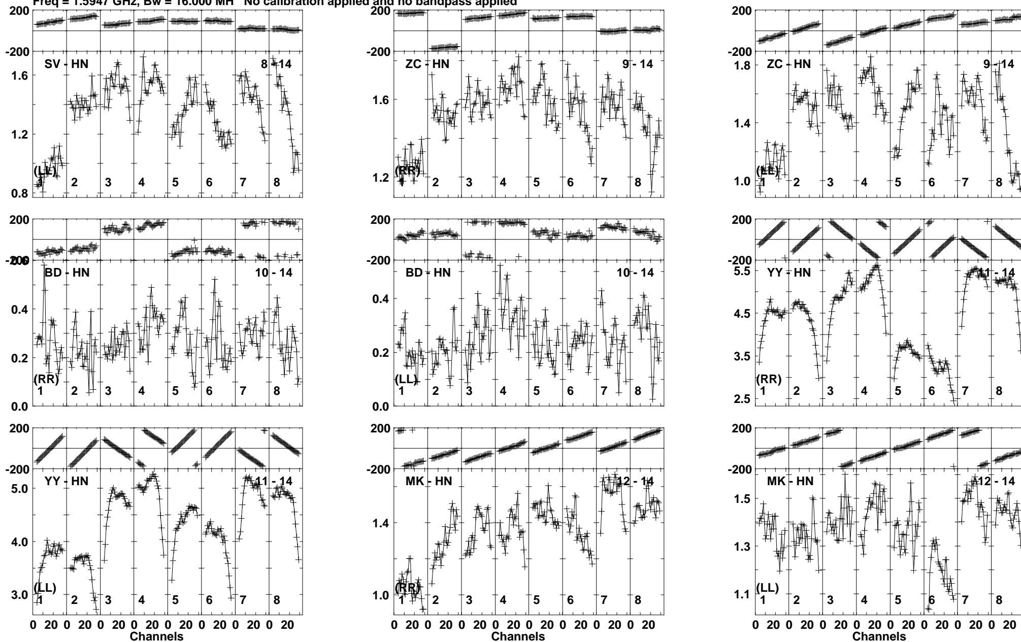
Lower frame: Milli Ampl Jy Top frame: Phas deg Vector averaged cross-power spectrum Baseline: SV (08) - HN (14) Timerange: 01/00:19:43 to 01/00:21:33
