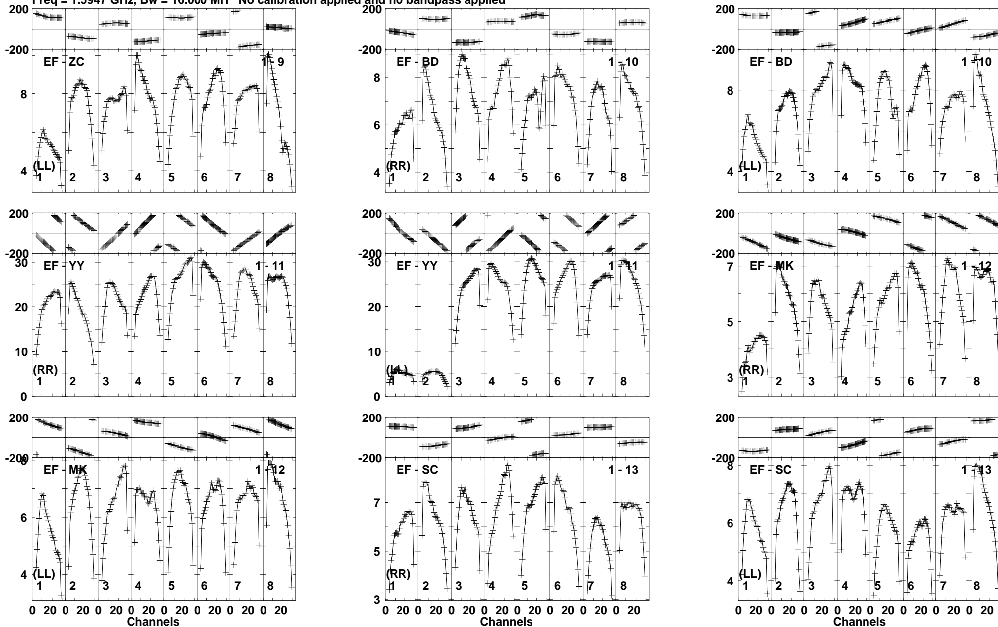
Lower frame: Milli Ampl Jy Top frame: Phas deg Vector averaged cross-power spectrum Baseline: EF (01) - ZC (09) Timerange: 01/01:53:31 to 01/01:55:12
