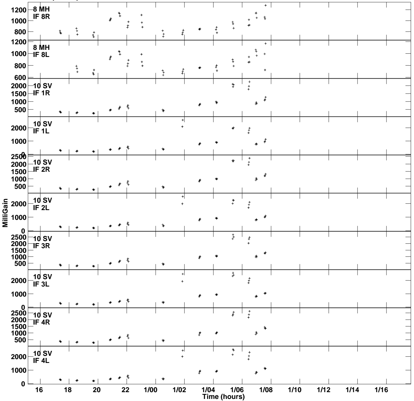
Plot file version 12 created 21-JAN-2022 19:16:52 Gain amp vs UTC time for NRAO150.MULTI.1 SN 2 Rpol & Lpol IF 1 - 8
