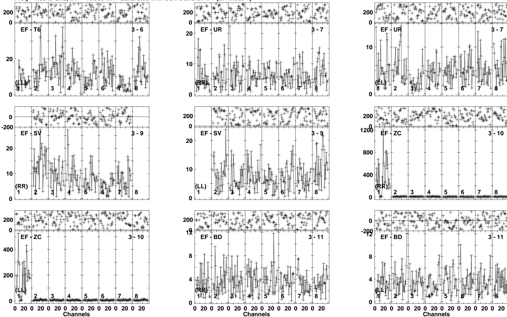
Lower frame: Milli Ampl Jy Top frame: Phas deg Vector averaged cross-power spectrum Baseline: EF (03) - T6 (06) Timerange: 00/15:20:57 to 00/15:24:19
