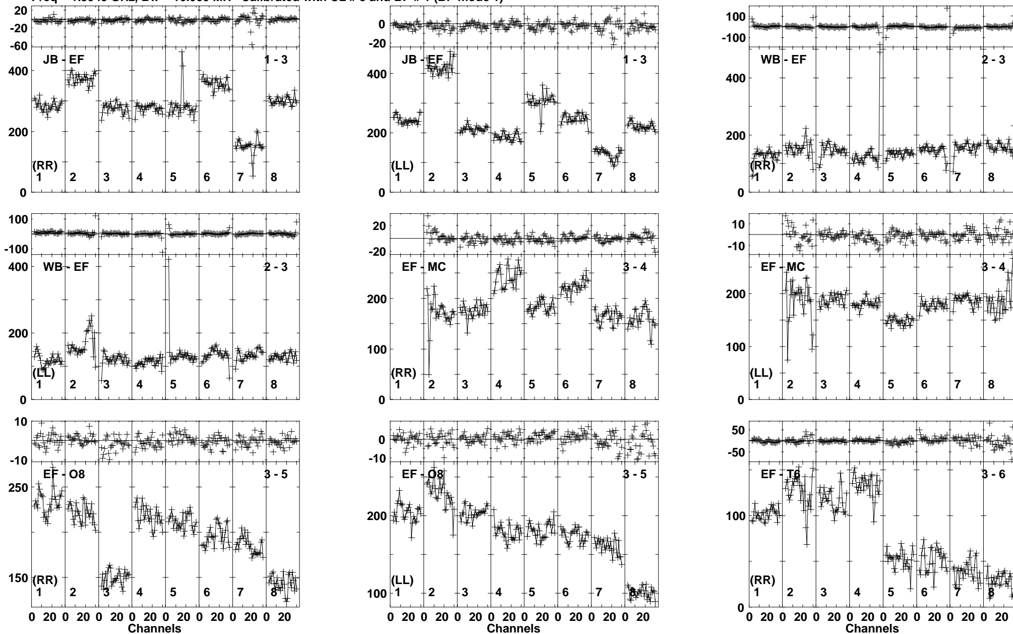
Lower frame: Milli Ampl Jy Top frame: Phas deg Vector averaged cross-power spectrum Baseline: JB (01) - EF (03) Timerange: 00/17:42:11 to 00/17:43:09
