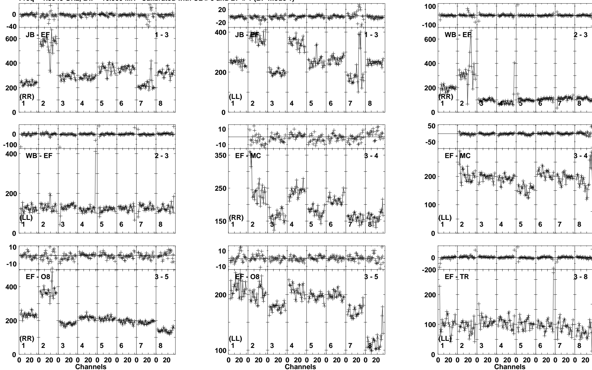
Lower frame: Milli Ampl Jy Top frame: Phas deg Vector averaged cross-power spectrum Baseline: JB (01) - EF (03) Timerange: 00/22:30:14 to 00/22:31:34
