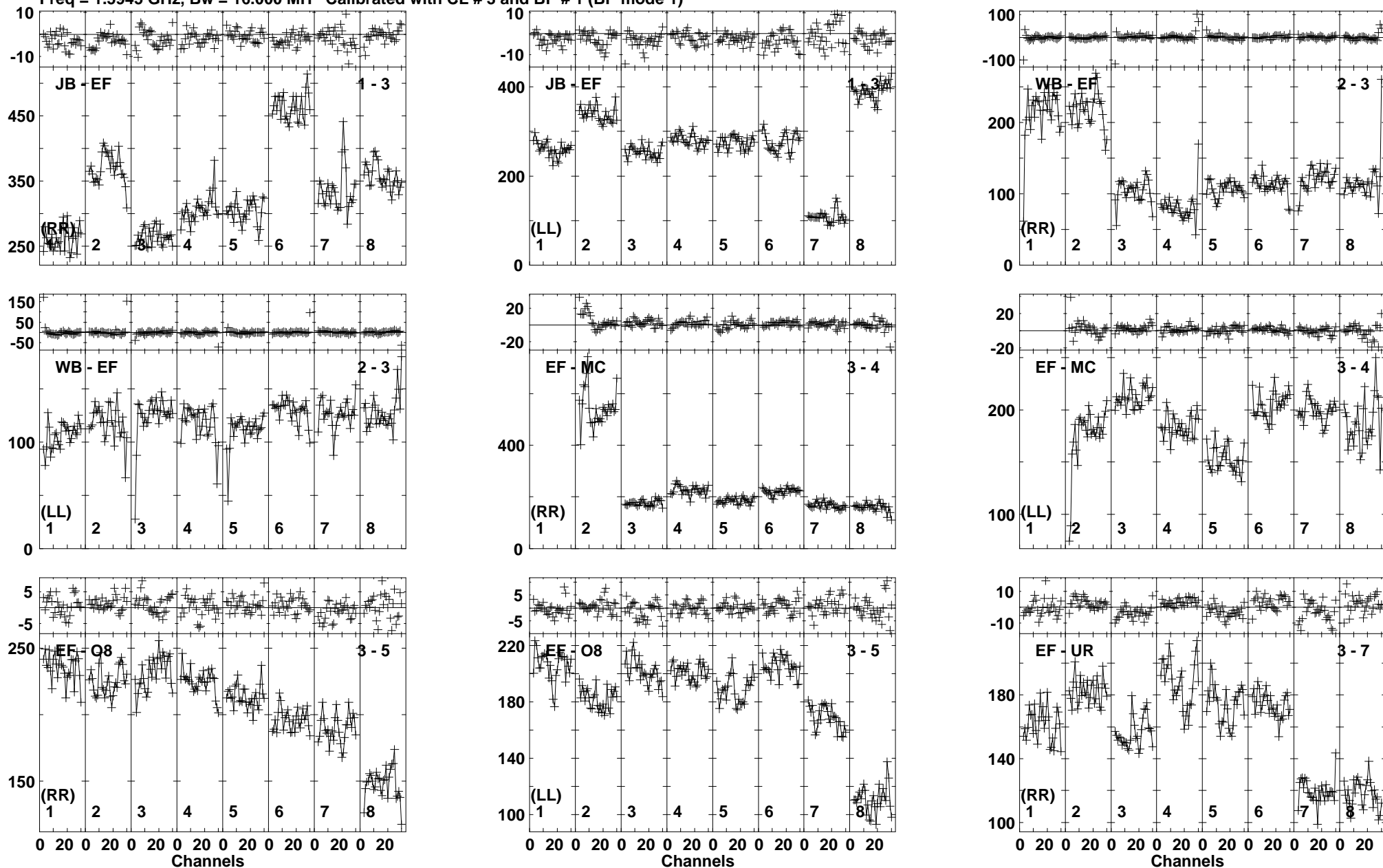
Lower frame: Milli Ampl Jy Top frame: Phas deg Vector averaged cross-power spectrum Baseline: JB (01) - EF (03) Timerange: 00/20:13:26 to 00/20:14:24
