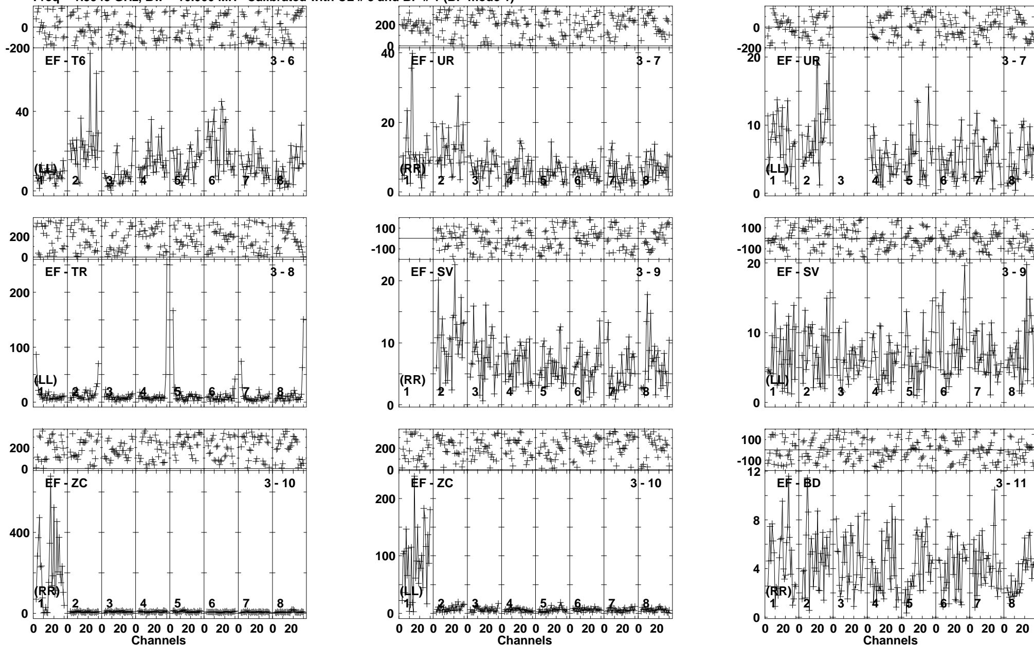
Lower frame: Milli Ampl Jy Top frame: Phas deg Vector averaged cross-power spectrum Baseline: EF (03) - T6 (06) Timerange: 00/18:08:32 to 00/18:11:54
