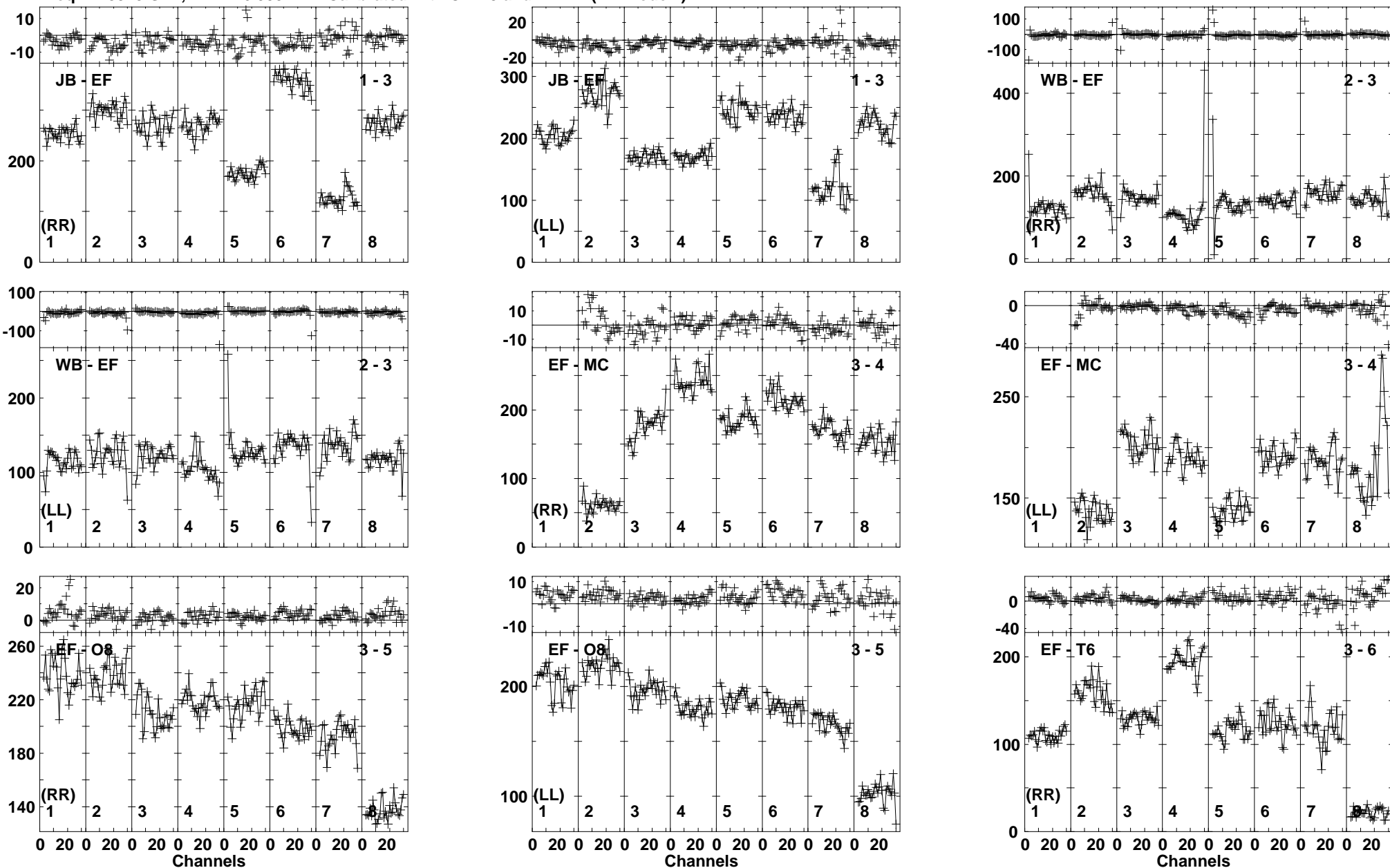
Lower frame: Milli Ampl Jy Top frame: Phas deg Vector averaged cross-power spectrum Baseline: JB (01) - EF (03) Timerange: 00/16:55:57 to 00/16:57:19
