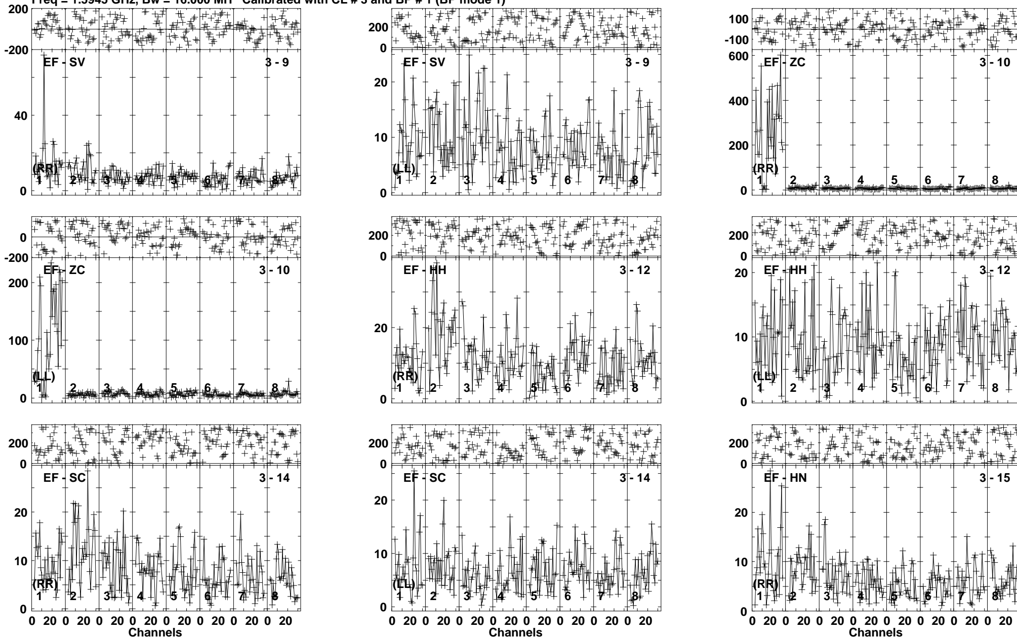
Lower frame: Milli Ampl Jy Top frame: Phas deg Vector averaged cross-power spectrum Baseline: EF (03) - SV (09) Timerange: 00/23:07:22 to 00/23:10:44
