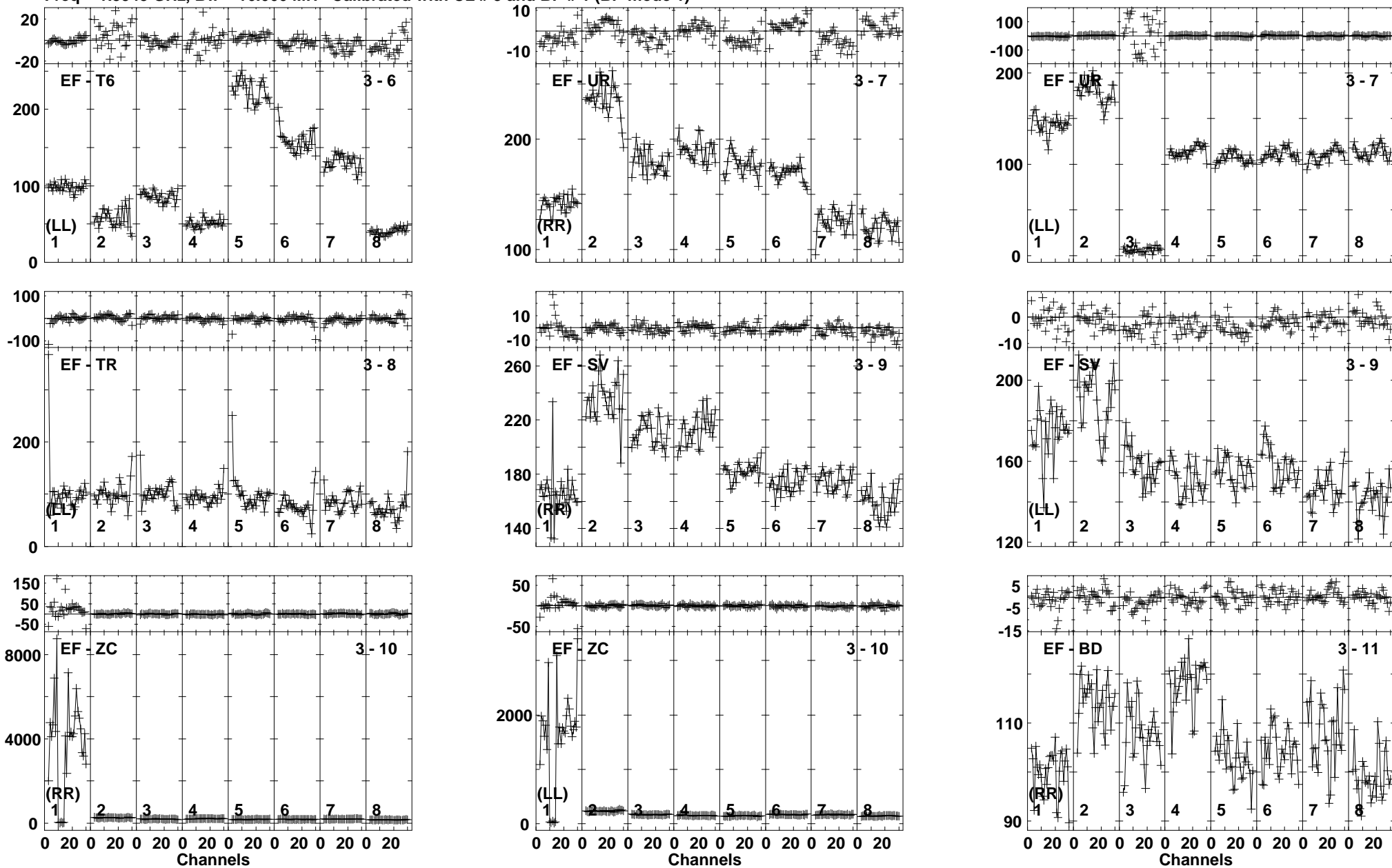
Lower frame: Milli Ampl Jy Top frame: Phas deg Vector averaged cross-power spectrum Baseline: EF (03) - T6 (06) Timerange: 00/17:01:31 to 00/17:02:29
