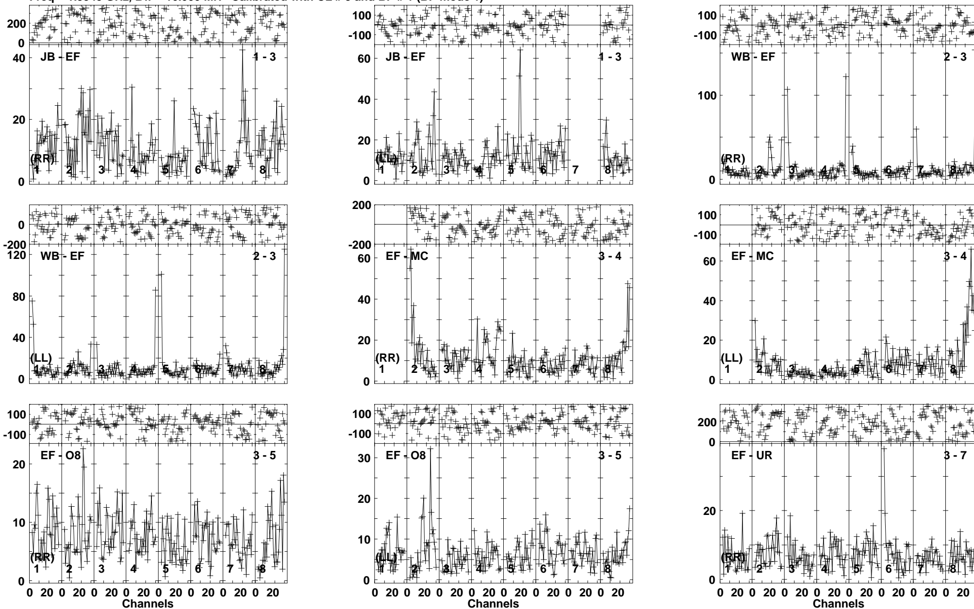
Lower frame: Milli Ampl Jy Top frame: Phas deg Vector averaged cross-power spectrum Baseline: JB (01) - EF (03) Timerange: 00/18:39:02 to 00/18:42:24
