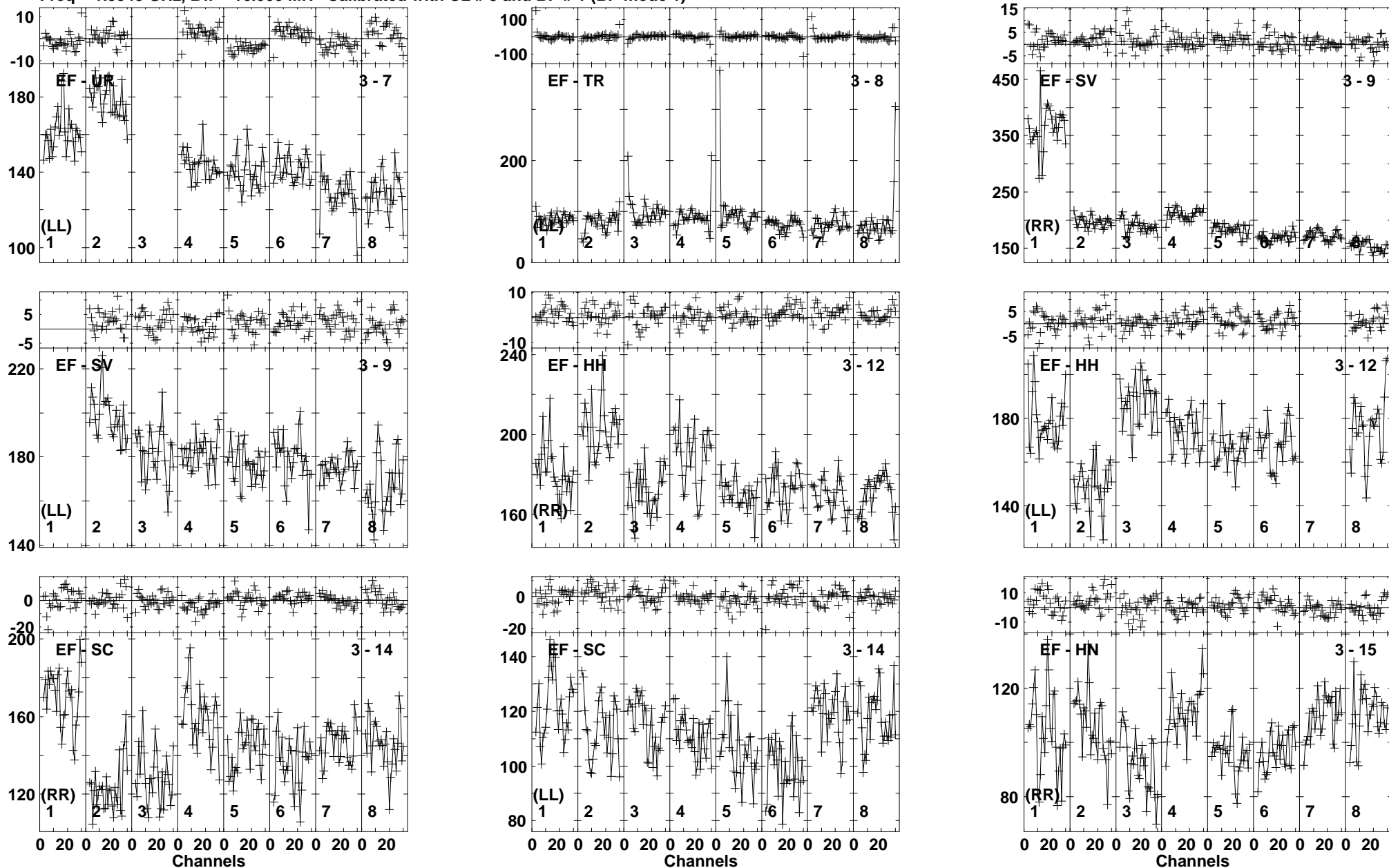
Lower frame: Milli Ampl Jy Top frame: Phas deg Vector averaged cross-power spectrum Baseline: EF (03) - UR (07) Timerange: 00/20:33:46 to 00/20:34:44
