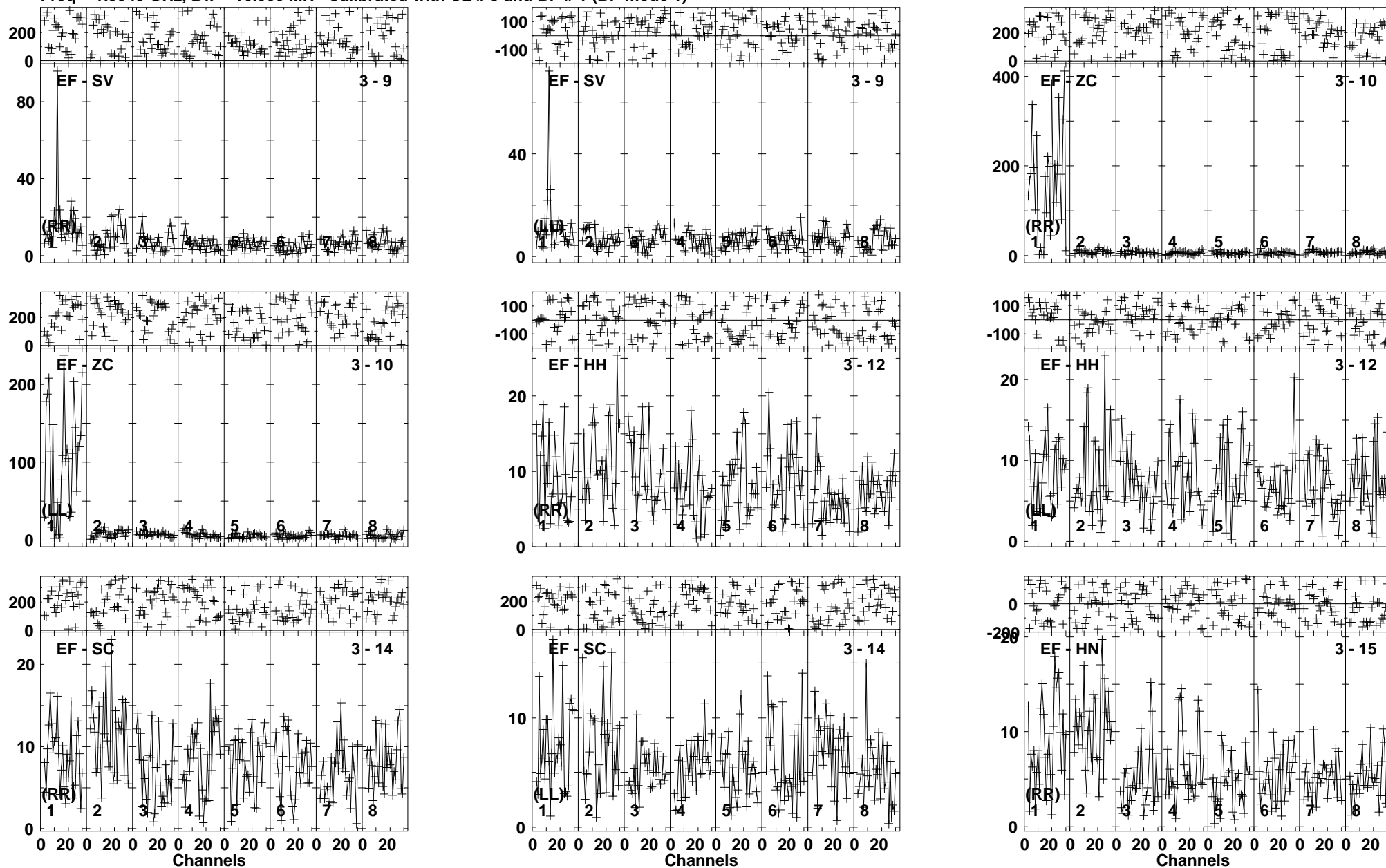
Lower frame: Milli Ampl Jy Top frame: Phas deg Vector averaged cross-power spectrum Baseline: EF (03) - SV (09) Timerange: 00/22:16:32 to 00/22:19:54
