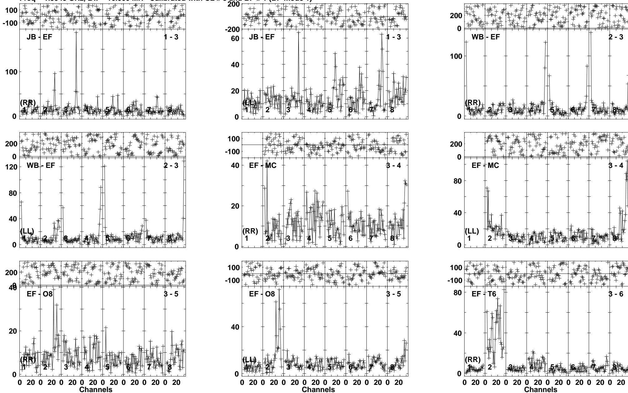
Lower frame: Milli Ampl Jy Top frame: Phas deg Vector averaged cross-power spectrum Baseline: JB (01) - EF (03) Timerange: 00/15:25:57 to 00/15:29:19
