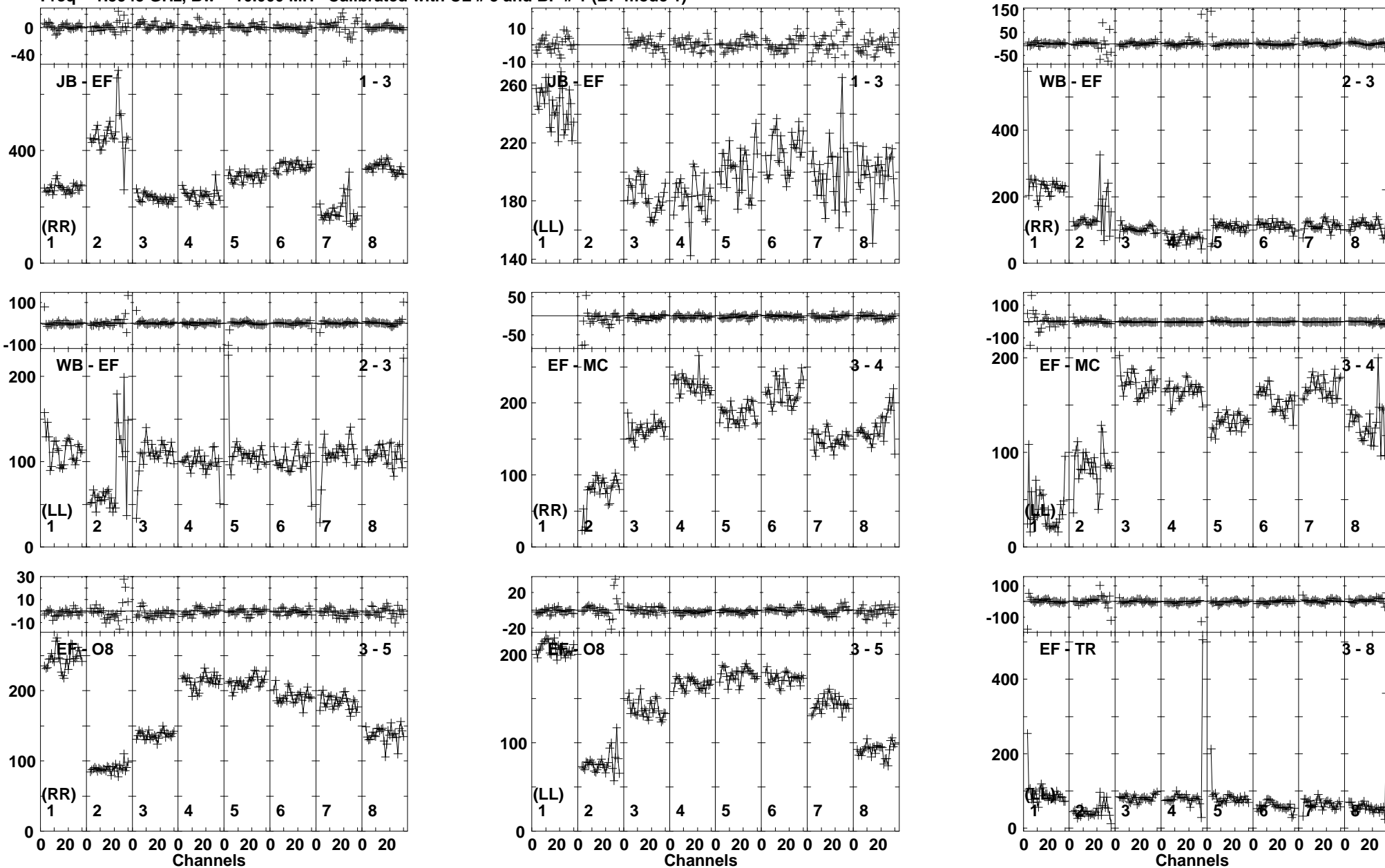
Lower frame: Milli Ampl Jy Top frame: Phas deg Vector averaged cross-power spectrum Baseline: JB (01) - EF (03) Timerange: 00/21:04:16 to 00/21:05:14
