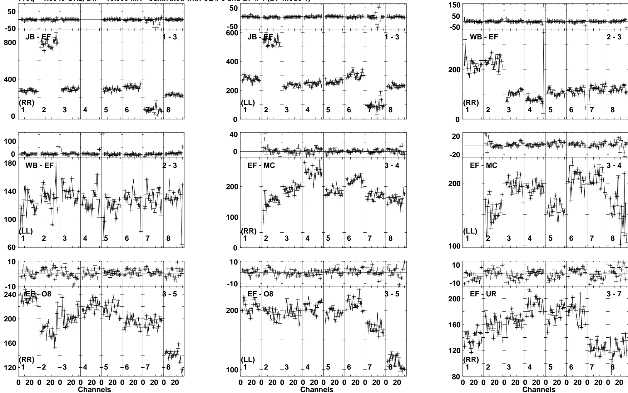
Lower frame: Milli Ampl Jy Top frame: Phas deg Vector averaged cross-power spectrum Baseline: JB (01) - EF (03) Timerange: 00/20:33:46 to 00/20:34:44
