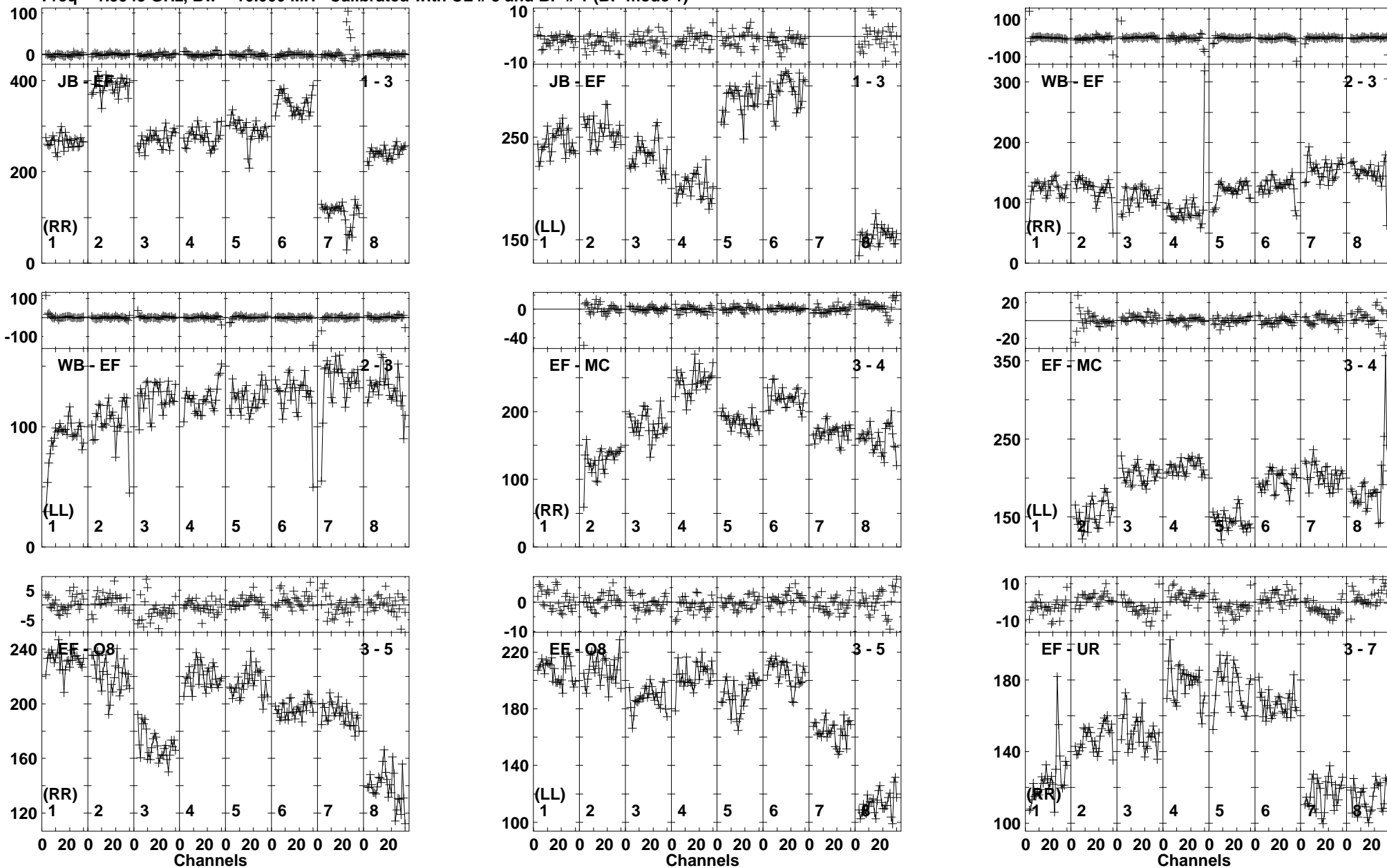
Lower frame: Milli Ampl Jy Top frame: Phas deg Vector averaged cross-power spectrum Baseline: JB (01) - EF (03) Timerange: 00:18:58:16 to 00:18:59:14
