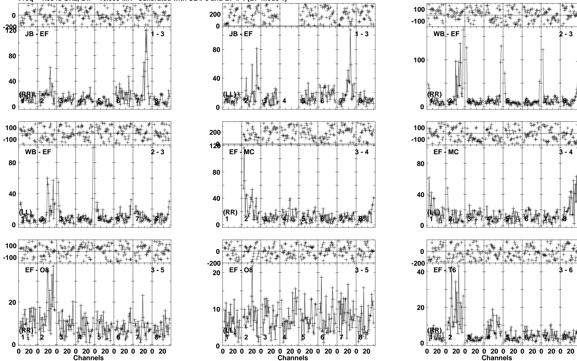
Lower frame: Milli Ampl Jy Top frame: Phas deg Vector averaged cross-power spectrum Baseline: JB (01) - EF (03) Timerange: 00/15:10:47 to 00/15:14:09
