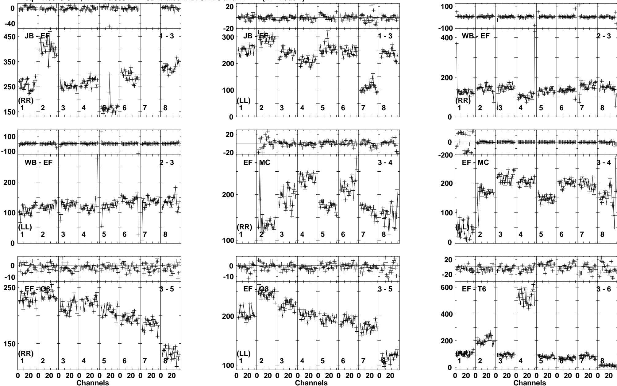
Lower frame: Milli Ampl Jy Top frame: Phas deg Vector averaged cross-power spectrum Baseline: JB (01) - EF (03) Timerange: 00/17:11:41 to 00/17:12:39
