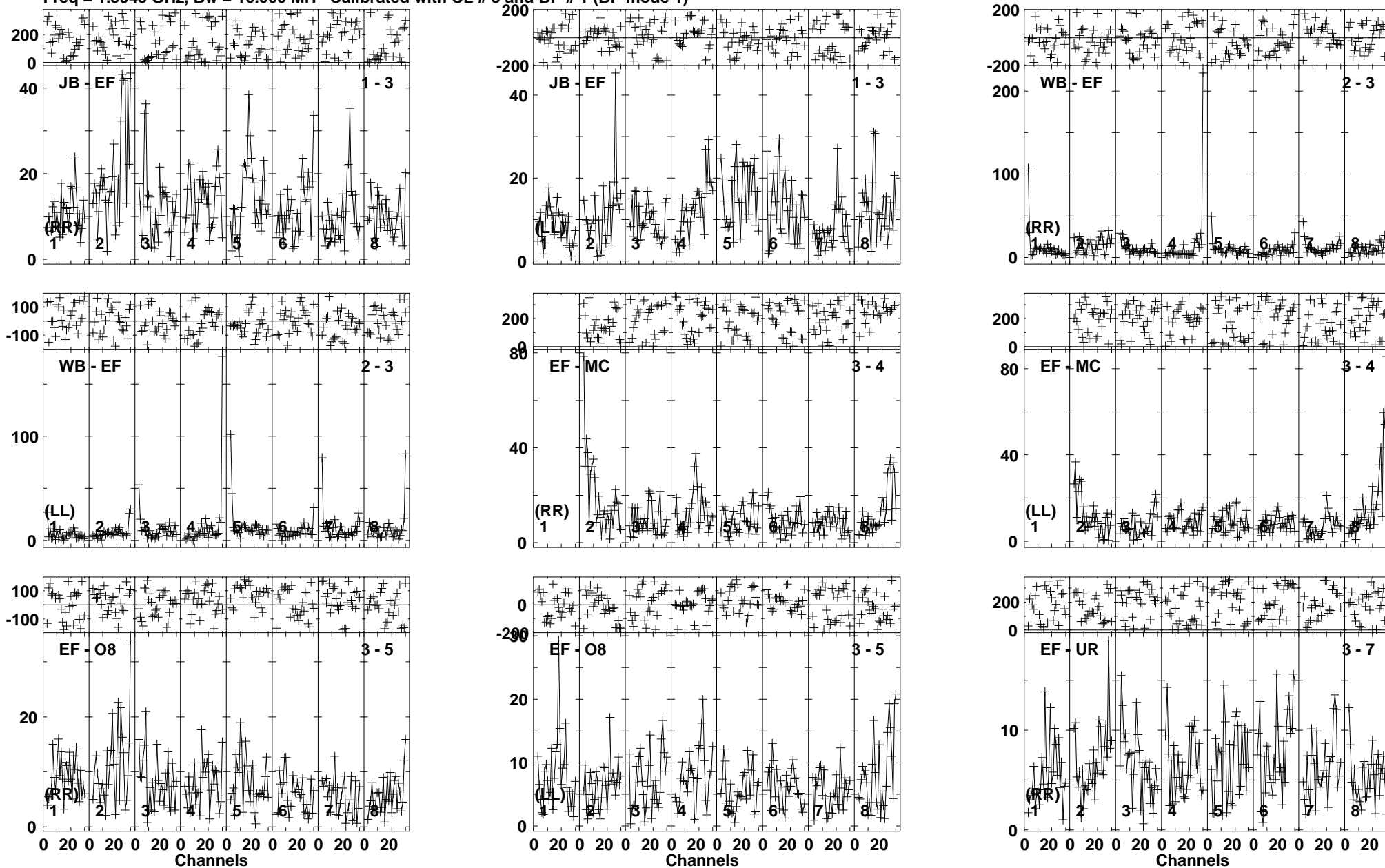
Lower frame: Milli Ampl Jy Top frame: Phas deg Vector averaged cross-power spectrum Baseline: JB (01) - EF (03) Timerange: 00/19:30:01 to 00/19:33:19
