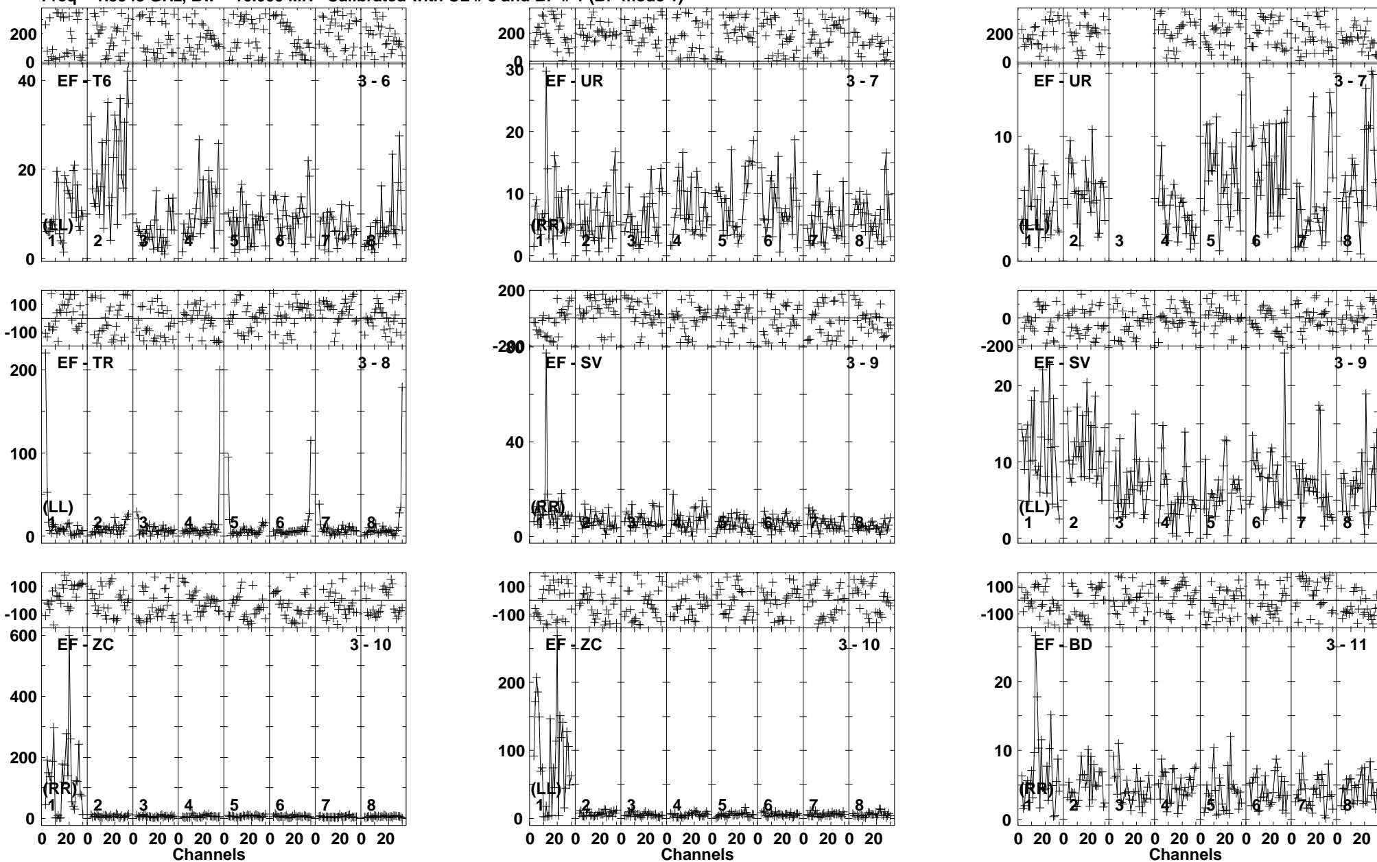
Lower frame: Milli Ampl Jy Top frame: Phas deg Vector averaged cross-power spectrum Baseline: EF (03) - T6 (06) Timerange: 00:18:18:42 to 00:18:22:04
