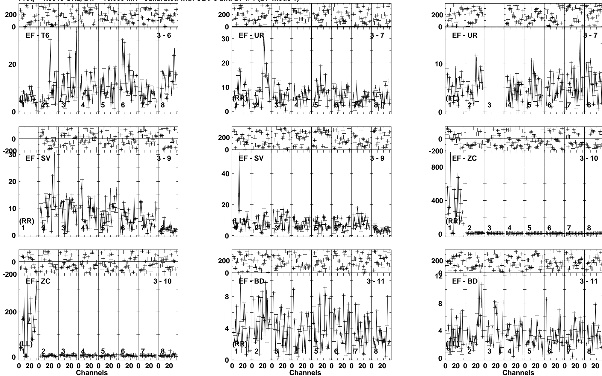
Lower frame: Milli Ampl Jy Top frame: Phas deg Vector averaged cross-power spectrum Baseline: EF (03) - T6 (06) Timerange: 00/15:31:07 to 00/15:34:29
