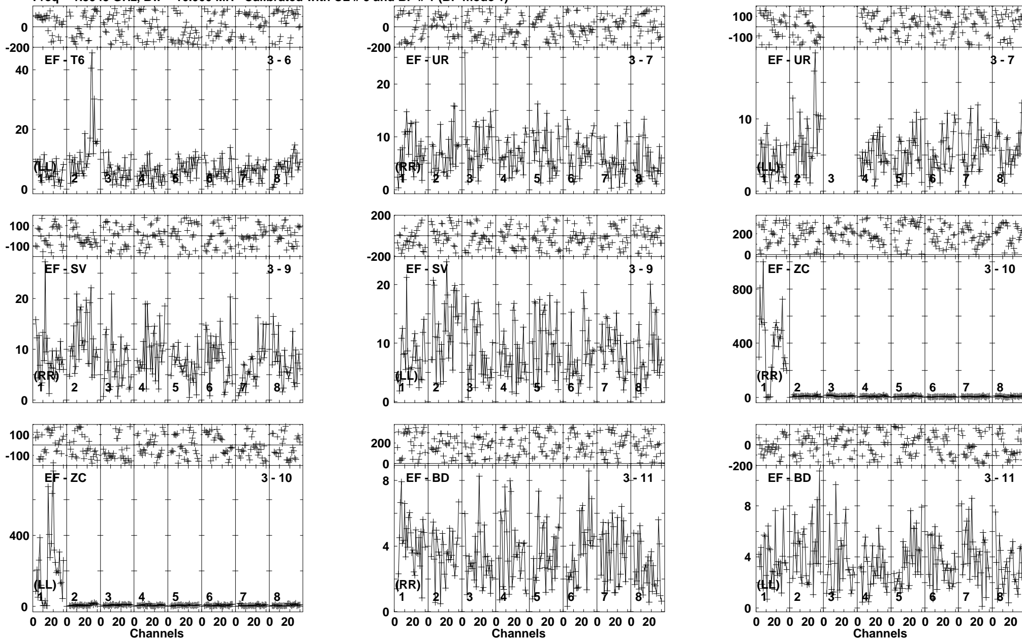
Lower frame: Milli Ampl Jy Top frame: Phas deg Vector averaged cross-power spectrum Baseline: EF (03) - T6 (06) Timerange: 00/15:15:47 to 00/15:19:09
