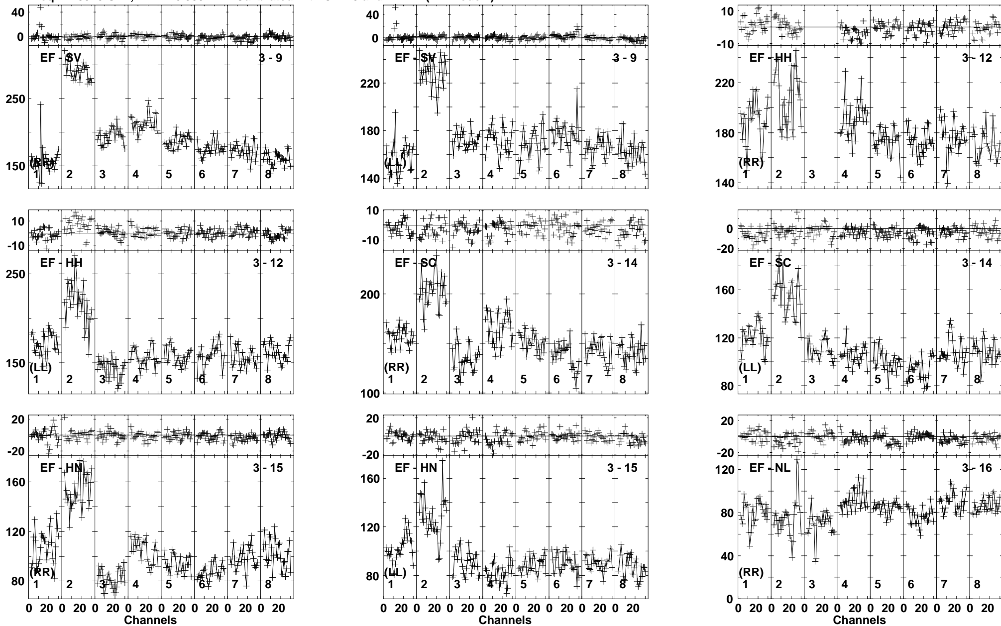
Lower frame: Milli Ampl Jy Top frame: Phas deg Vector averaged cross-power spectrum Baseline: EF (03) - SV (09) Timerange: 00/21:49:34 to 00/21:50:54
