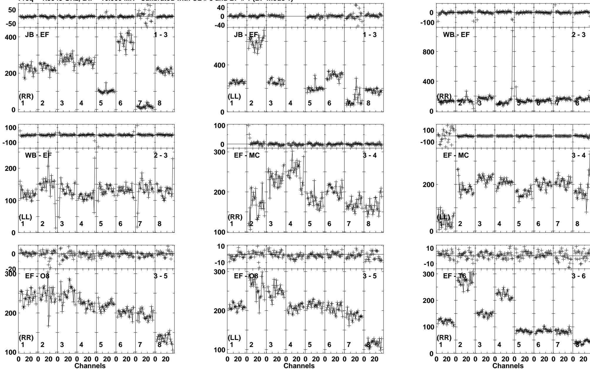
Lower frame: Milli Ampl Jy Top frame: Phas deg Vector averaged cross-power spectrum Baseline: JB (01) - EF (03) Timerange: 00/15:09:41 to 00/15:10:39
