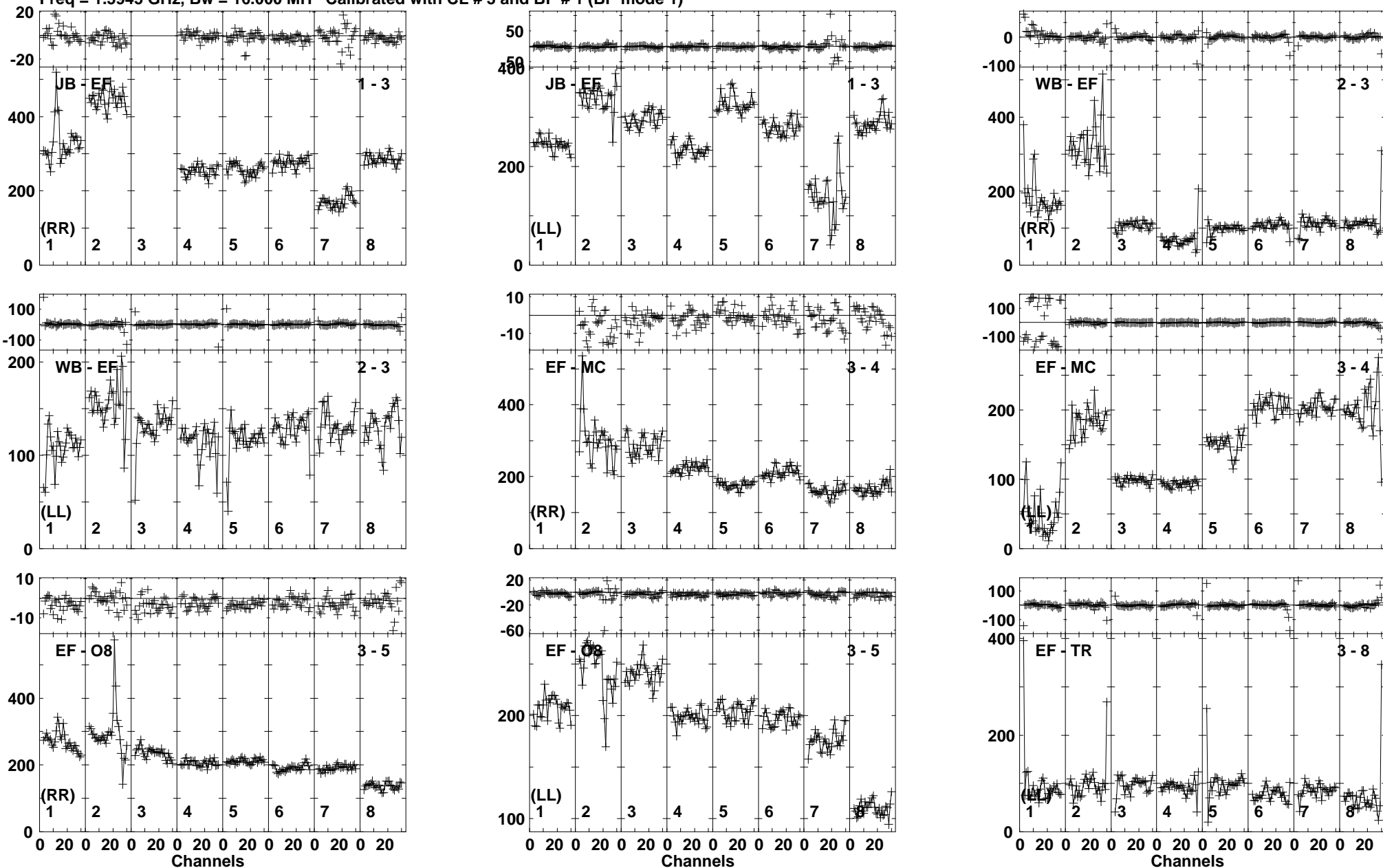
Lower frame: Milli Ampl Jy Top frame: Phas deg Vector averaged cross-power spectrum Baseline: JB (01) - EF (03) Timerange: 00/21:14:26 to 00/21:15:24
