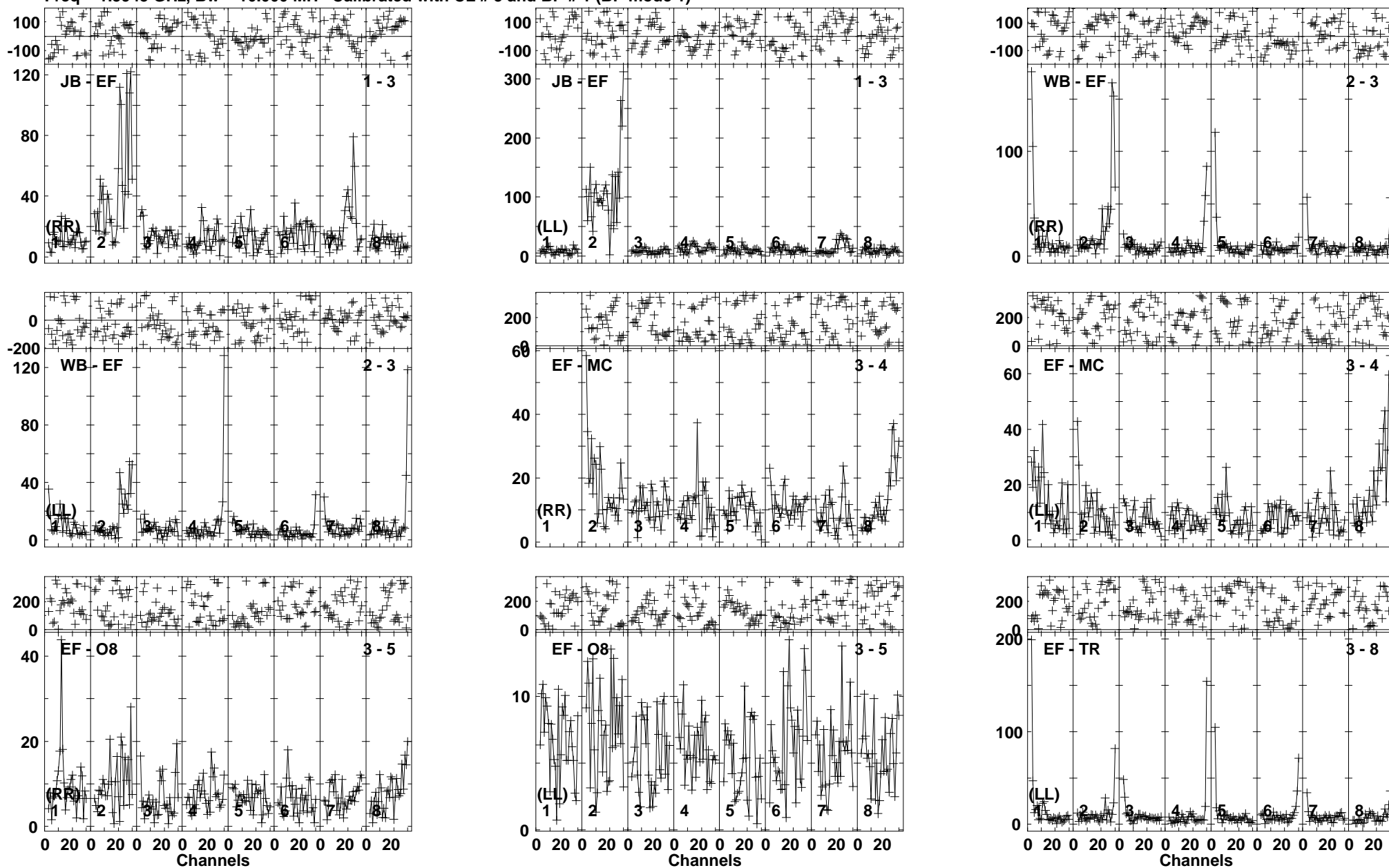
Lower frame: Milli Ampl Jy Top frame: Phas deg Vector averaged cross-power spectrum Baseline: JB (01) - EF (03) Timerange: 00/21:10:24 to 00/21:13:44
