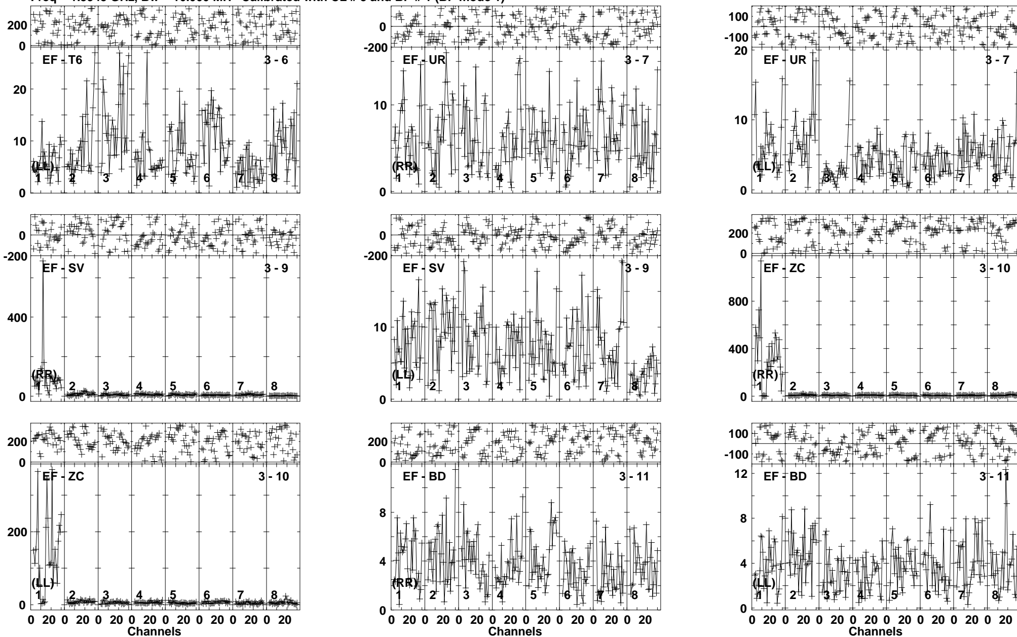
Lower frame: Milli Ampl Jy Top frame: Phas deg Vector averaged cross-power spectrum Baseline: EF (03) - T6 (06) Timerange: 00/15:36:07 to 00/15:39:29
