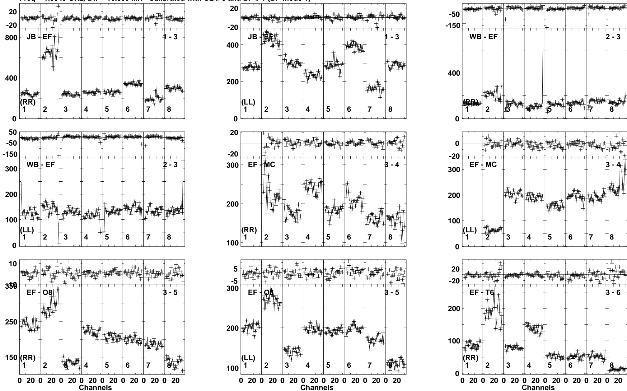
Lower frame: Milli Ampl Jy Top frame: Phas deg Vector averaged cross-power spectrum Baseline: JB (01) - EF (03) Timerange: 00/17:36:37 to 00/17:37:59
