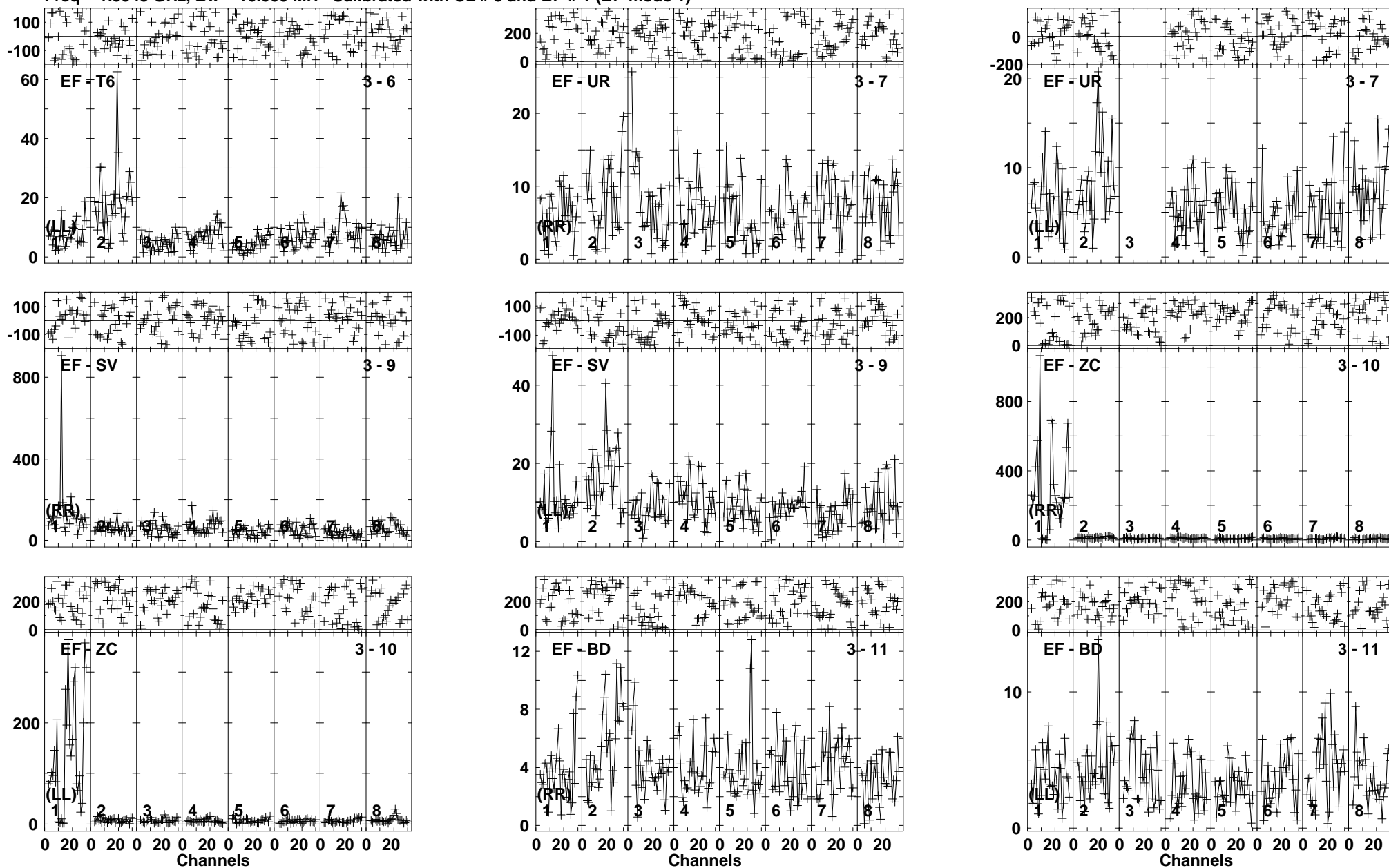
Lower frame: Milli Ampl Jy Top frame: Phas deg Vector averaged cross-power spectrum Baseline: EF (03) - T6 (06) Timerange: 00/14:55:27 to 00/14:58:49
