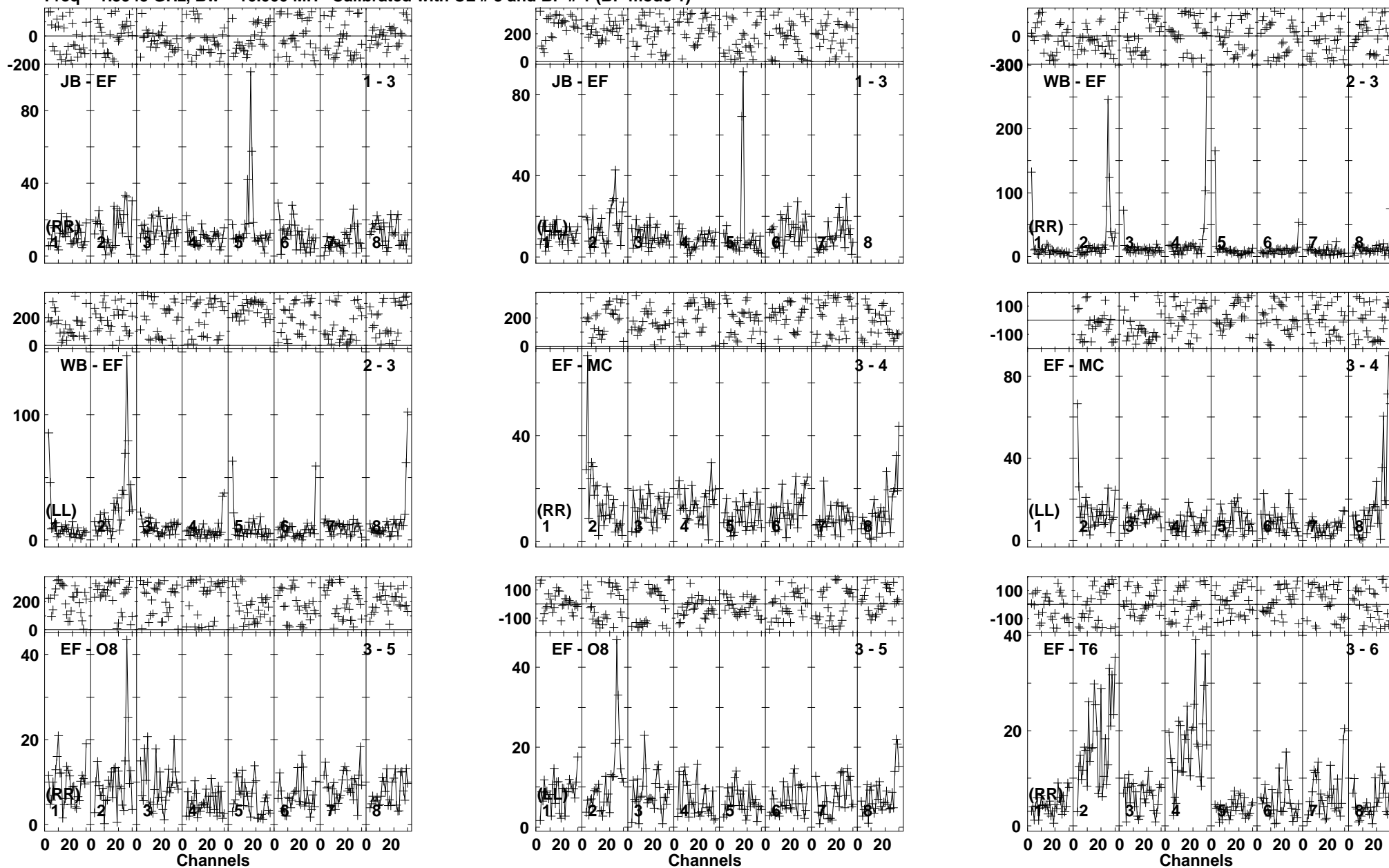
Lower frame: Milli Ampl Jy Top frame: Phas deg Vector averaged cross-power spectrum Baseline: JB (01) - EF (03) Timerange: 00/16:11:47 to 00/16:15:09
