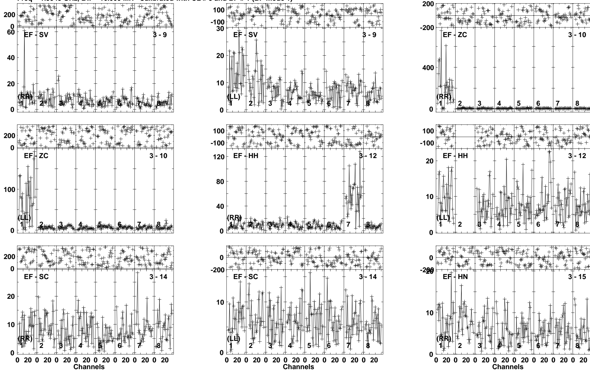
Lower frame: Milli Ampl Jy Top frame: Phas deg Vector averaged cross-power spectrum Baseline: EF (03) - SV (09) Timerange: 00/22:11:22 to 00/22:14:44
