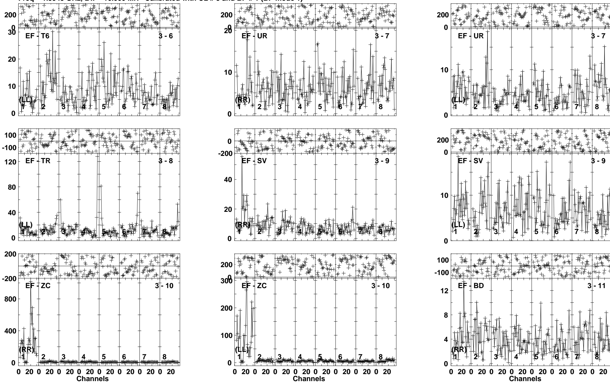
Lower frame: Milli Ampl Jy Top frame: Phas deg Vector averaged cross-power spectrum Baseline: EF (03) - T6 (06) Timerange: 00/16:37:07 to 00/16:40:29
