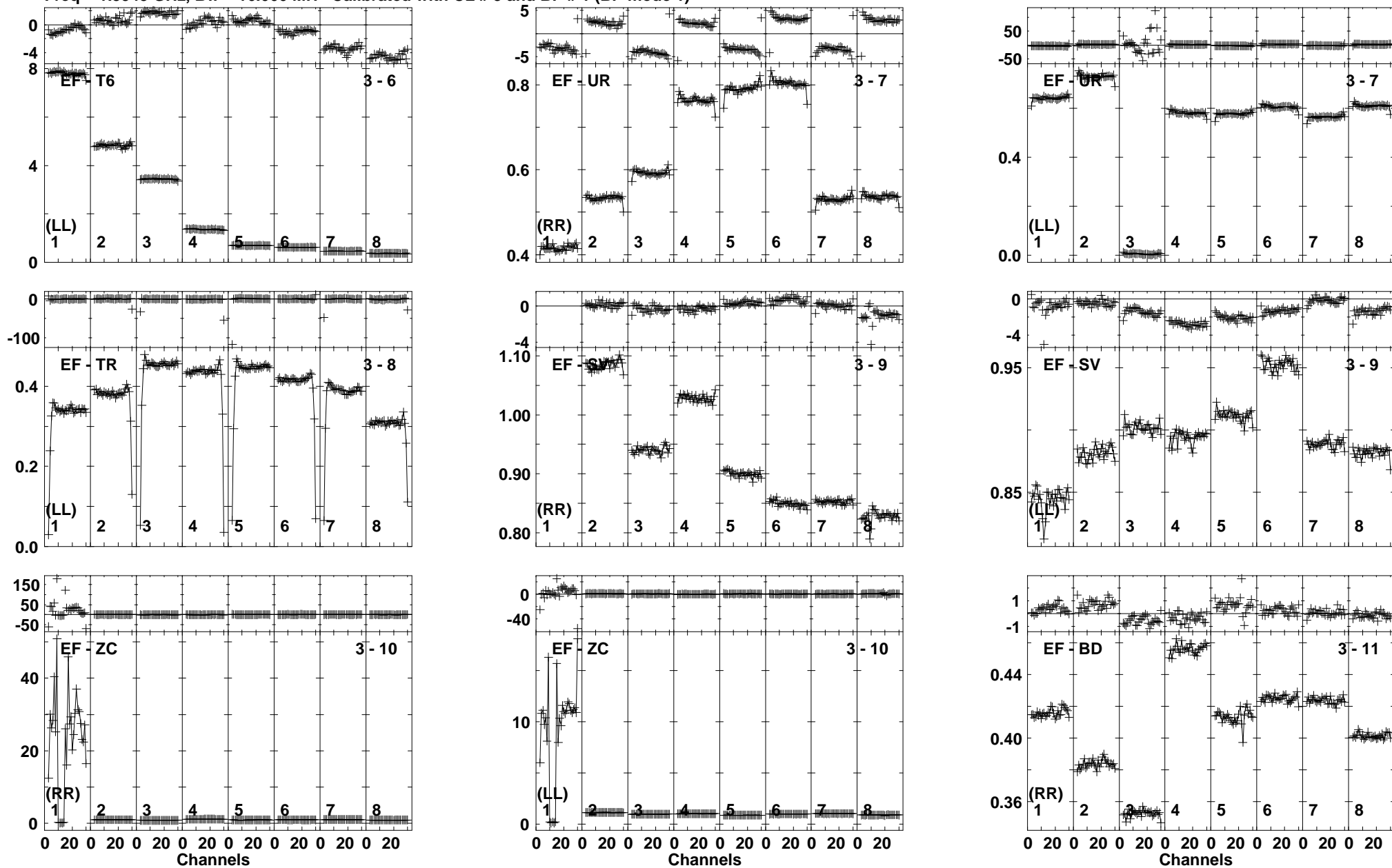
Lower frame: Ampl Jy Top frame: Phas deg Vector averaged cross-power spectrum Baseline: EF (03) - T6 (06) Timerange: 00/17:55:26 to 00/17:59:58
