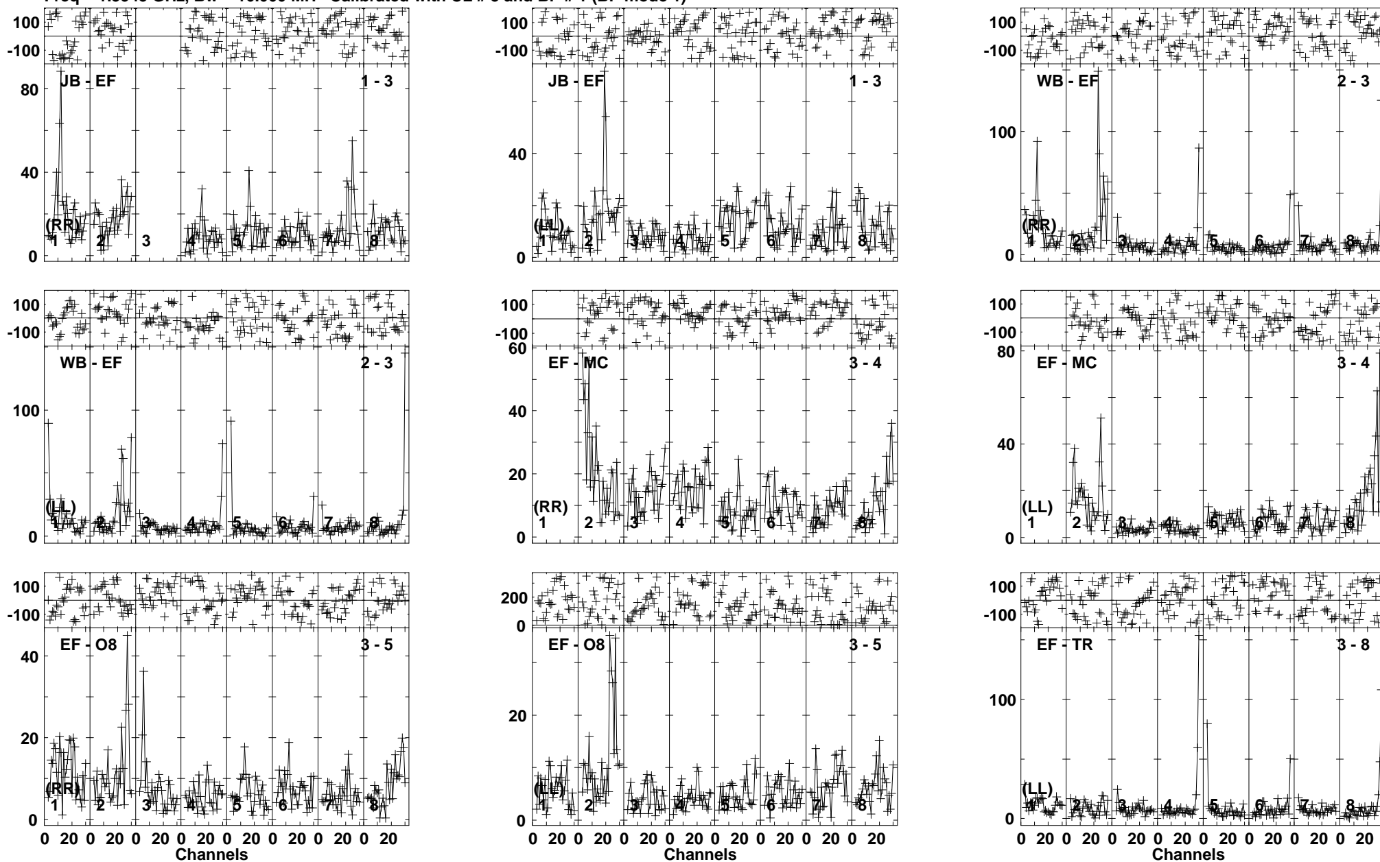
Lower frame: Milli Ampl Jy Top frame: Phas deg Vector averaged cross-power spectrum Baseline: JB (01) - EF (03) Timerange: 00/21:15:34 to 00/21:18:54
