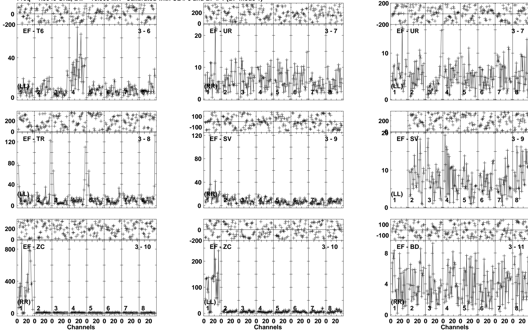
Lower frame: Milli Ampl Jy Top frame: Phas deg Vector averaged cross-power spectrum Baseline: EF (03) - T6 (06) Timerange: 00/16:52:27 to 00/16:55:49
