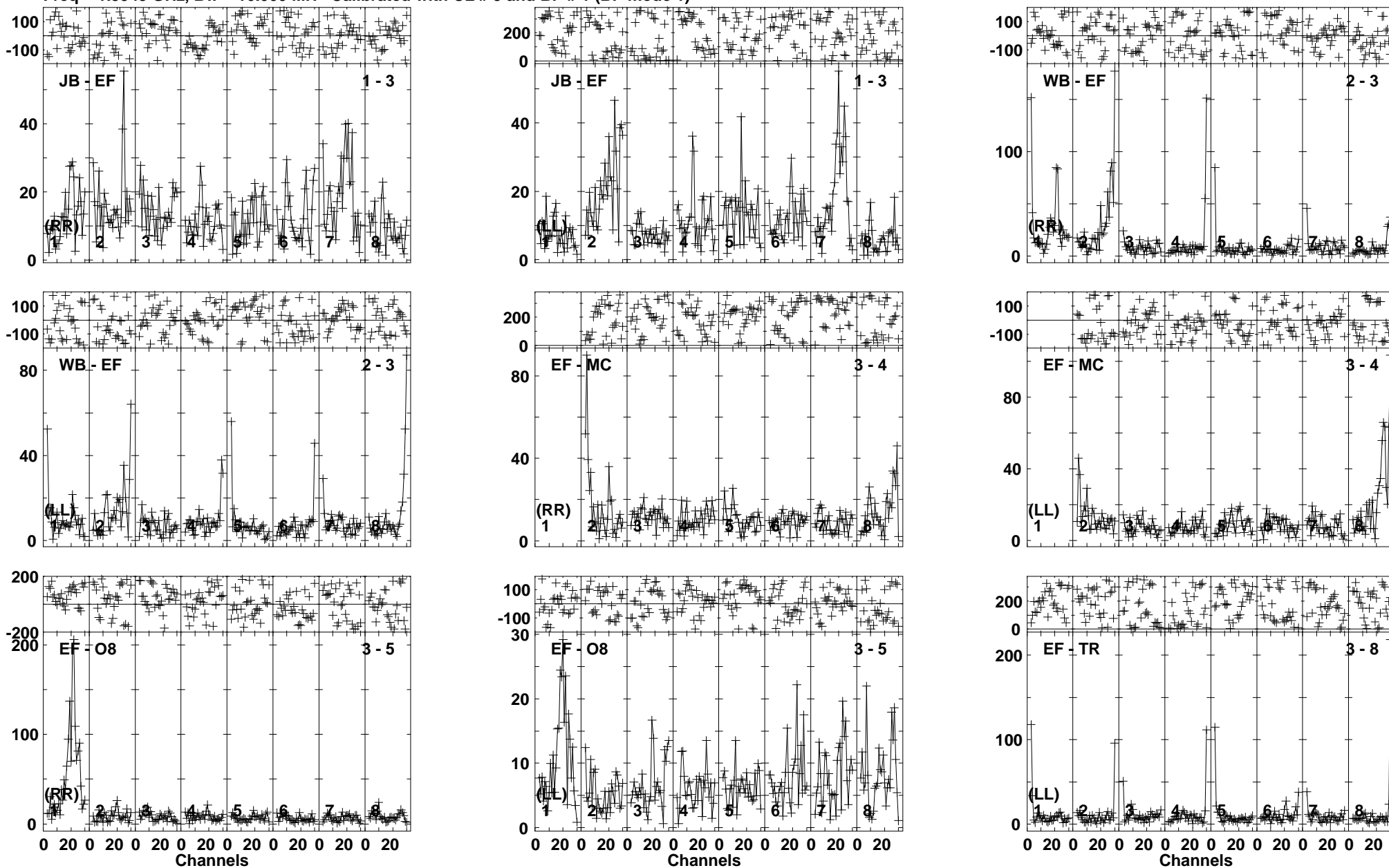
Lower frame: Milli Ampl Jy Top frame: Phas deg Vector averaged cross-power spectrum Baseline: JB (01) - EF (03) Timerange: 00/22:52:02 to 00/22:55:24
