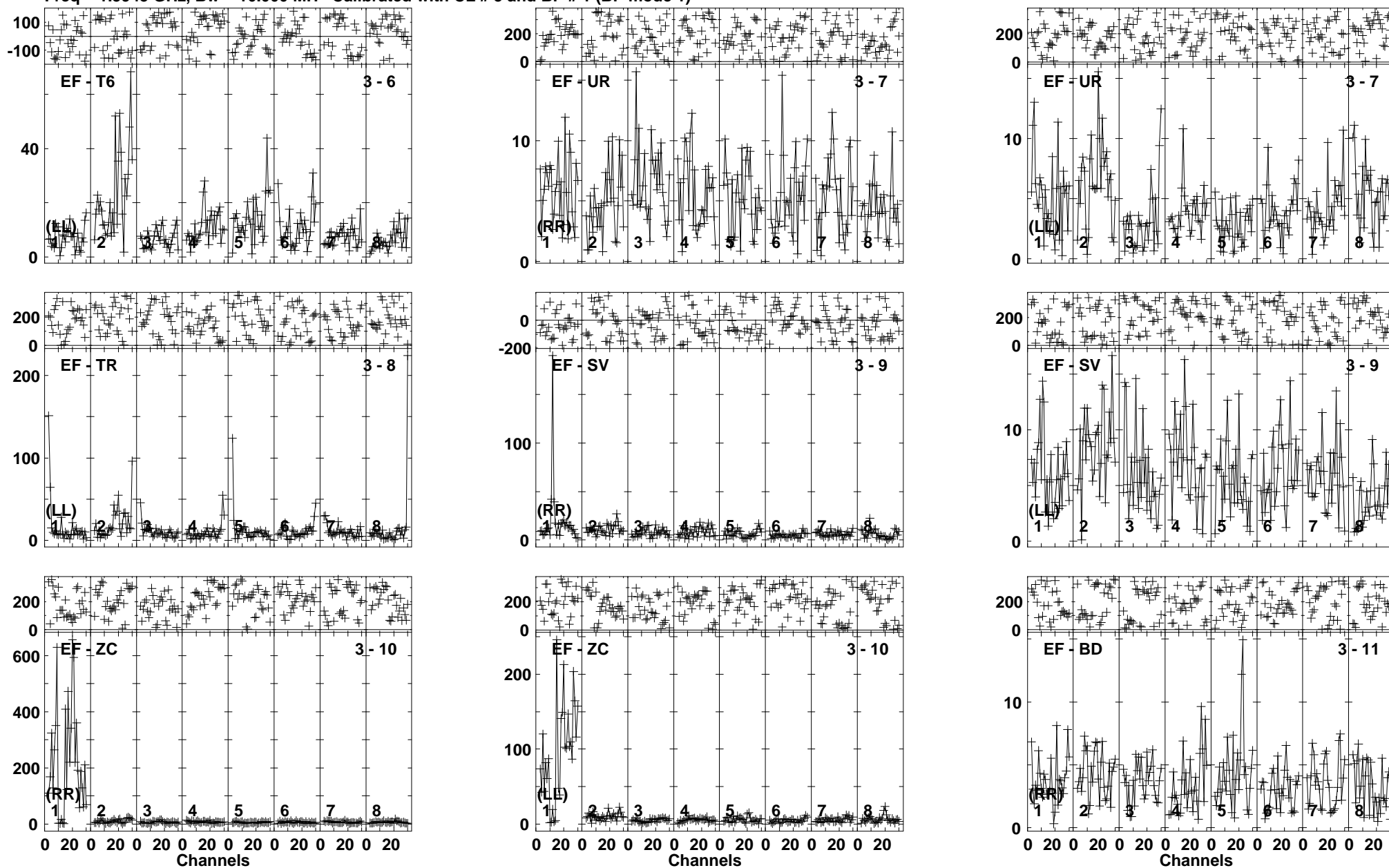
Lower frame: Milli Ampl Jy Top frame: Phas deg Vector averaged cross-power spectrum Baseline: EF (03) - T6 (06) Timerange: 00/16:32:07 to 00/16:35:29
