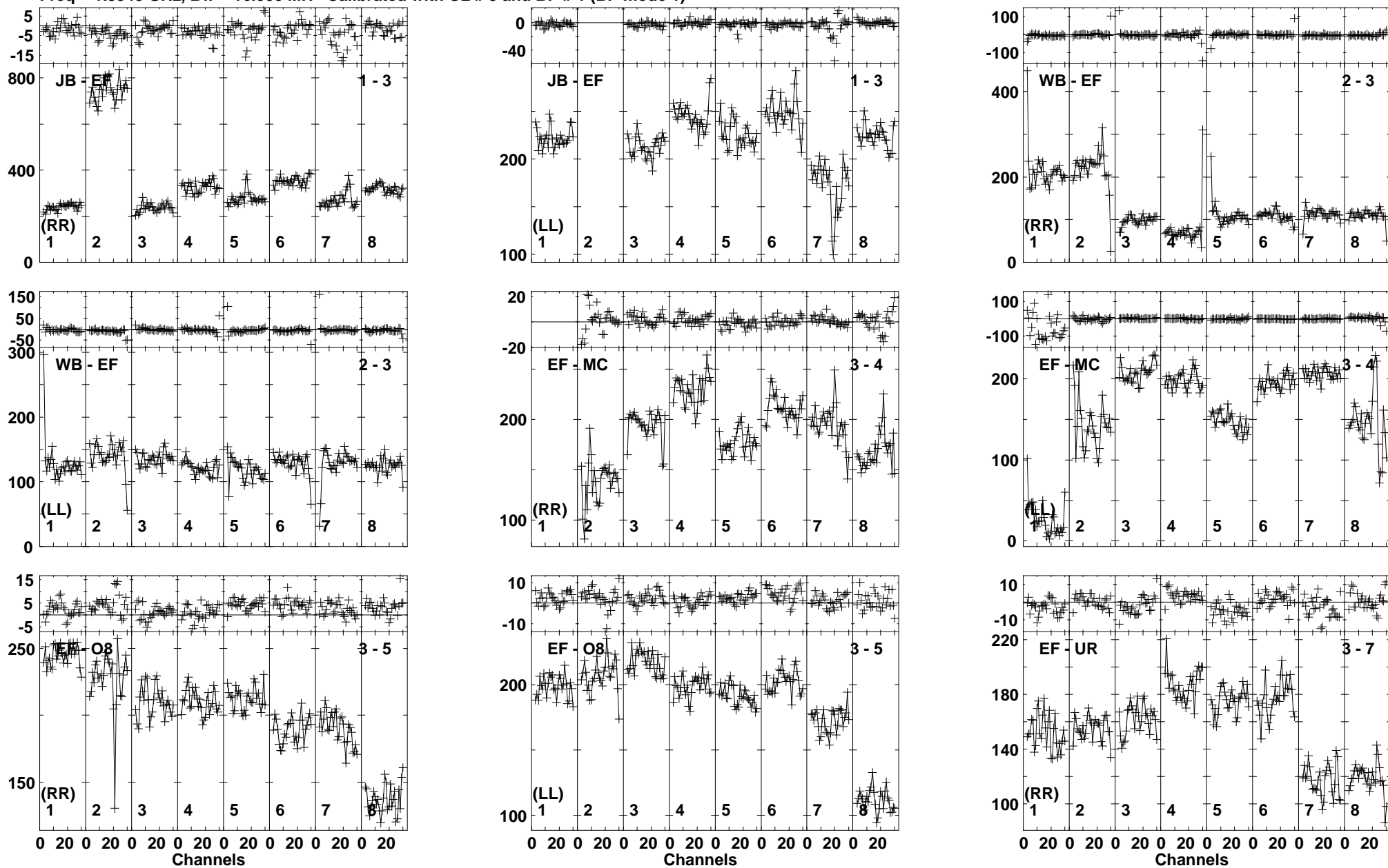
Lower frame: Milli Ampl Jy Top frame: Phas deg Vector averaged cross-power spectrum Baseline: JB (01) - EF (03) Timerange: 00/20:58:40 to 00/21:00:04
