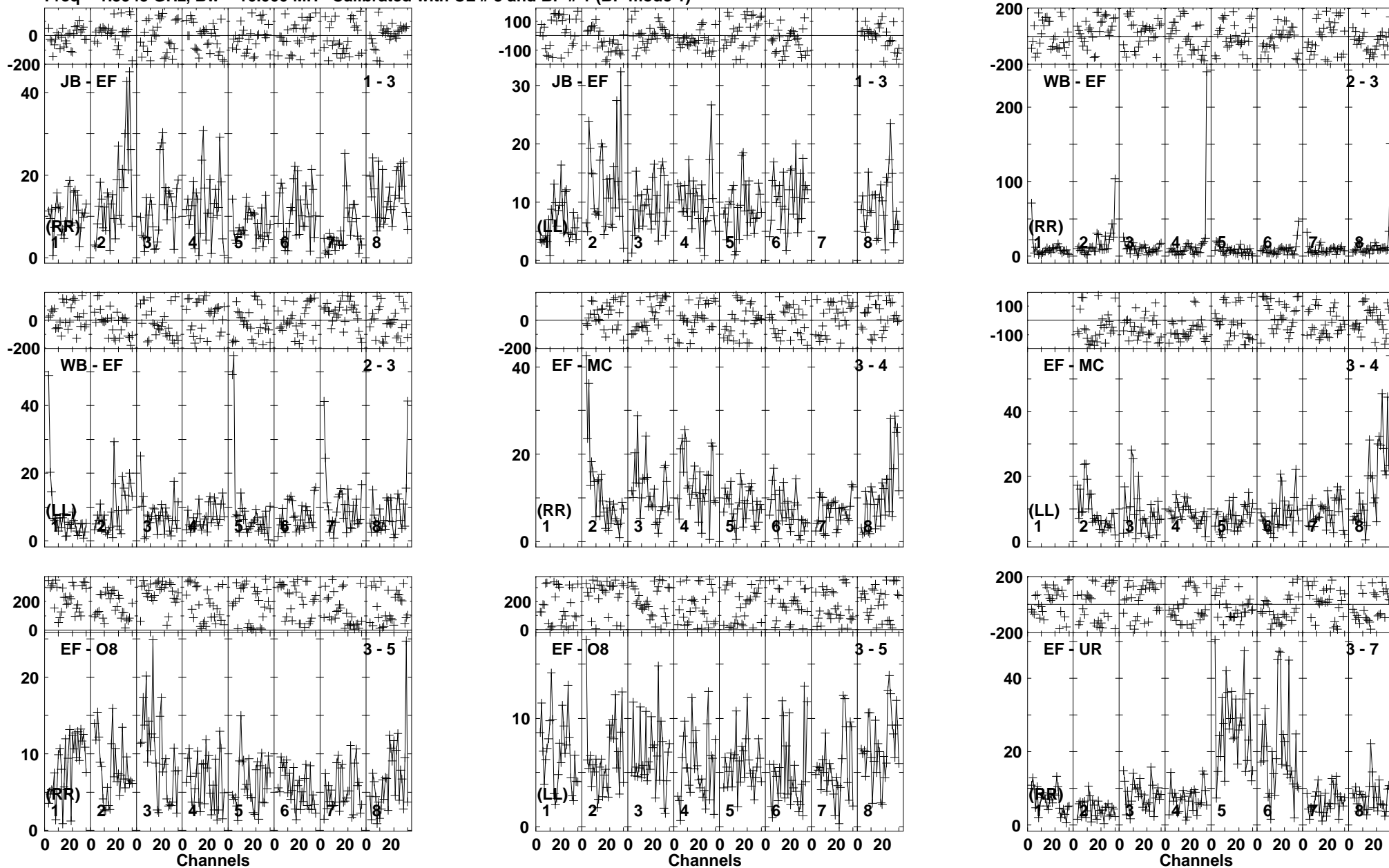
Lower frame: Milli Ampl Jy Top frame: Phas deg Vector averaged cross-power spectrum Baseline: JB (01) - EF (03) Timerange: 00:18:54:12 to 00:18:57:34
