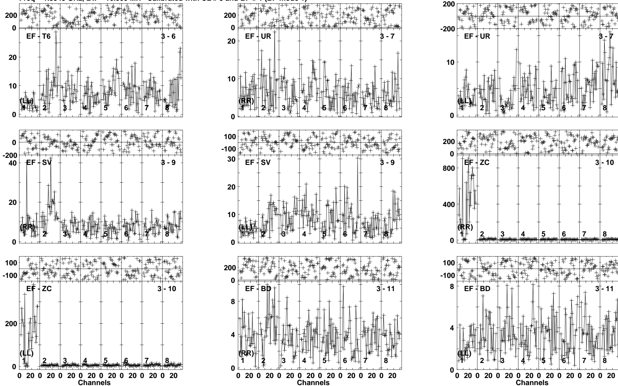
Lower frame: Milli Ampl Jy Top frame: Phas deg Vector averaged cross-power spectrum Baseline: EF (03) - T6 (06) Timerange: 00/15:10:47 to 00/15:14:09
