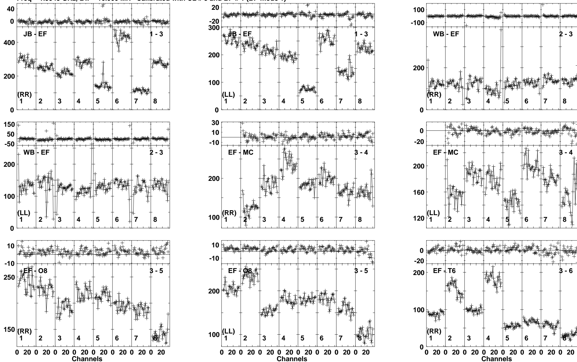
Lower frame: Milli Ampl Jy Top frame: Phas deg Vector averaged cross-power spectrum Baseline: JB (01) - EF (03) Timerange: 00/16:25:27 to 00/16:26:49
