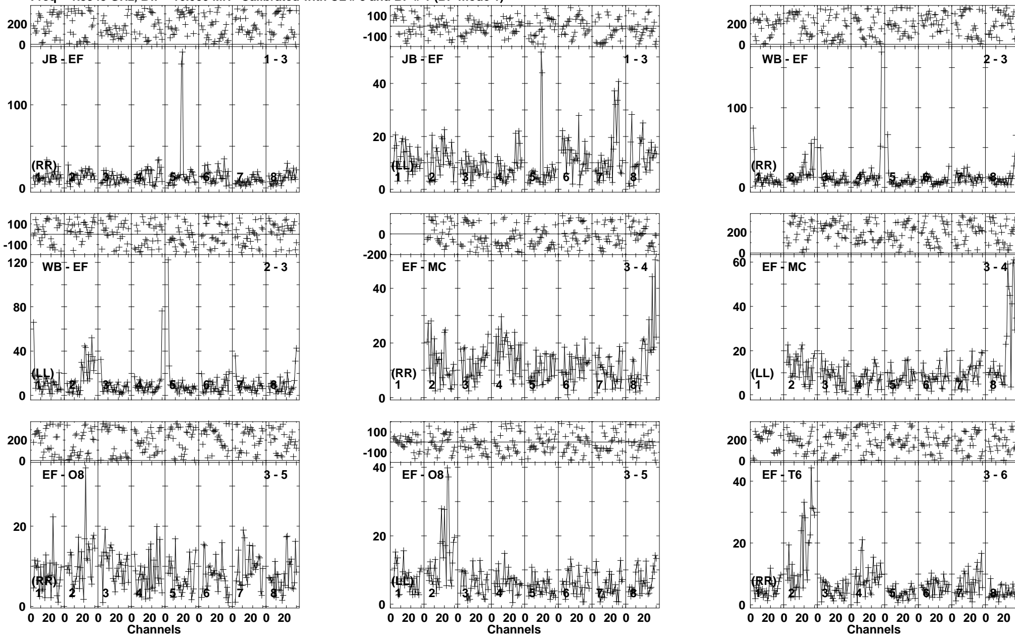
Lower frame: Milli Ampl Jy Top frame: Phas deg Vector averaged cross-power spectrum Baseline: JB (01) - EF (03) Timerange: 00/16:21:57 to 00/16:25:19
