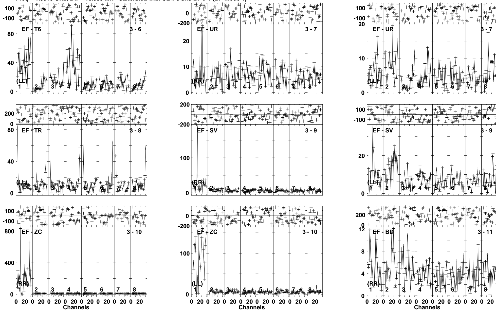
Lower frame: Milli Ampl Jy Top frame: Phas deg Vector averaged cross-power spectrum Baseline: EF (03) - T6 (06) Timerange: 00/17:22:57 to 00/17:26:19
