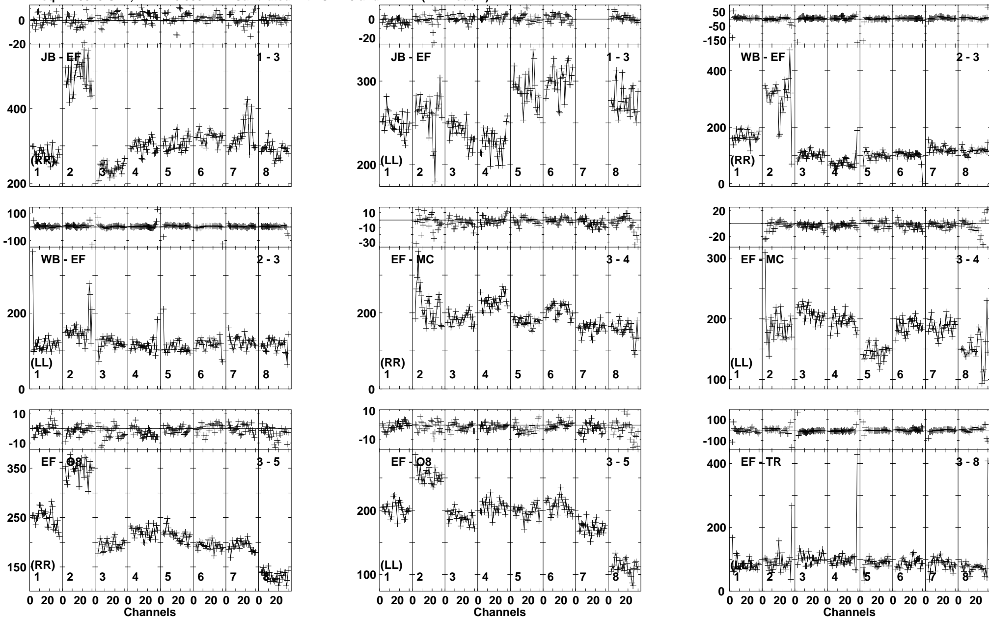
Lower frame: Milli Ampl Jy Top frame: Phas deg Vector averaged cross-power spectrum Baseline: JB (01) - EF (03) Timerange: 00/22:40:24 to 00/22:41:44
