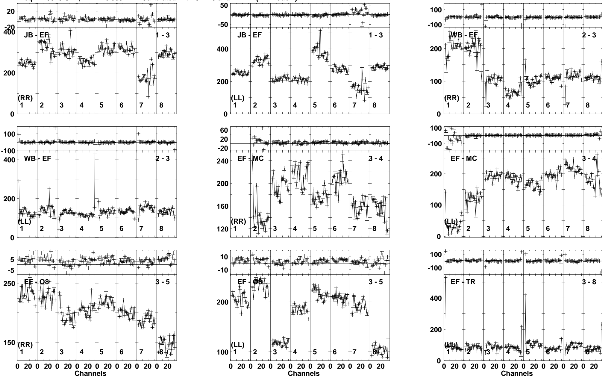
Lower frame: Milli Ampl Jy Top frame: Phas deg Vector averaged cross-power spectrum Baseline: JB (01) - EF (03) Timerange: 00/21:59:44 to 00/22:01:04
