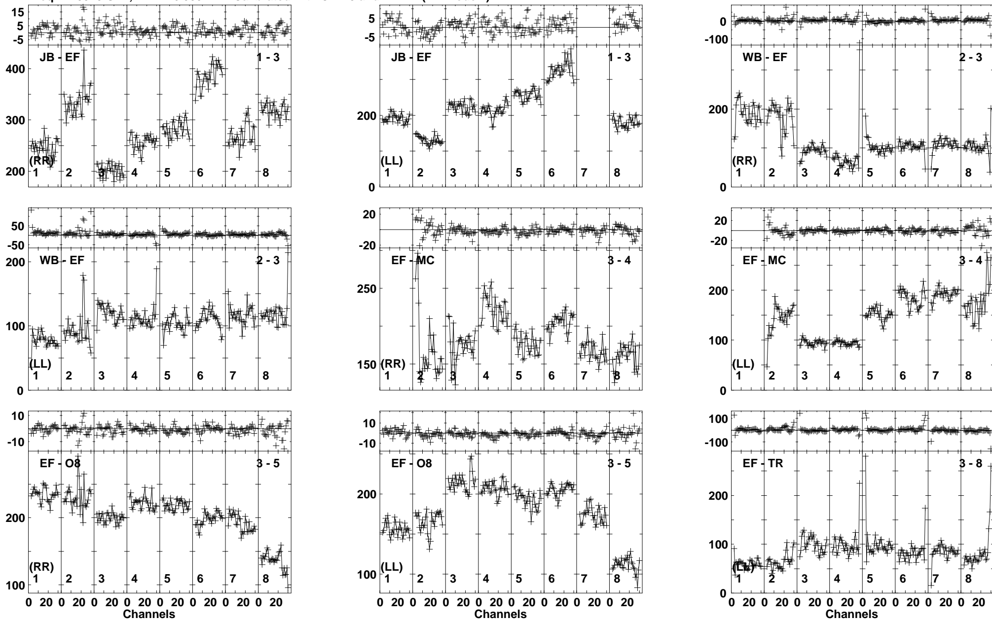
Lower frame: Milli Ampl Jy Top frame: Phas deg Vector averaged cross-power spectrum Baseline: JB (01) - EF (03) Timerange: 00/23:16:26 to 00/23:17:24
