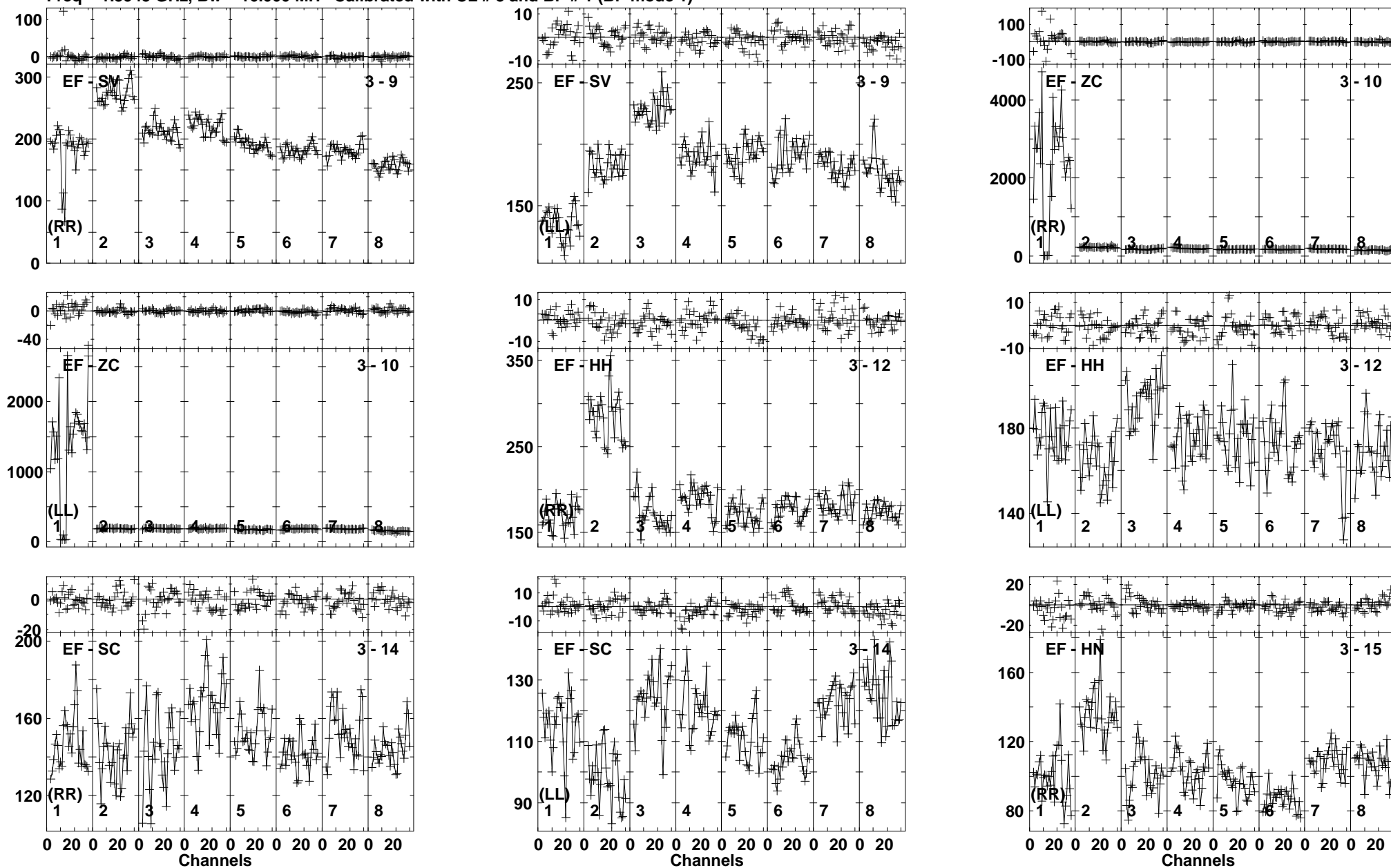
Lower frame: Milli Ampl Jy Top frame: Phas deg Vector averaged cross-power spectrum Baseline: EF (03) - SV (09) Timerange: 00/23:06:16 to 00/23:07:14
