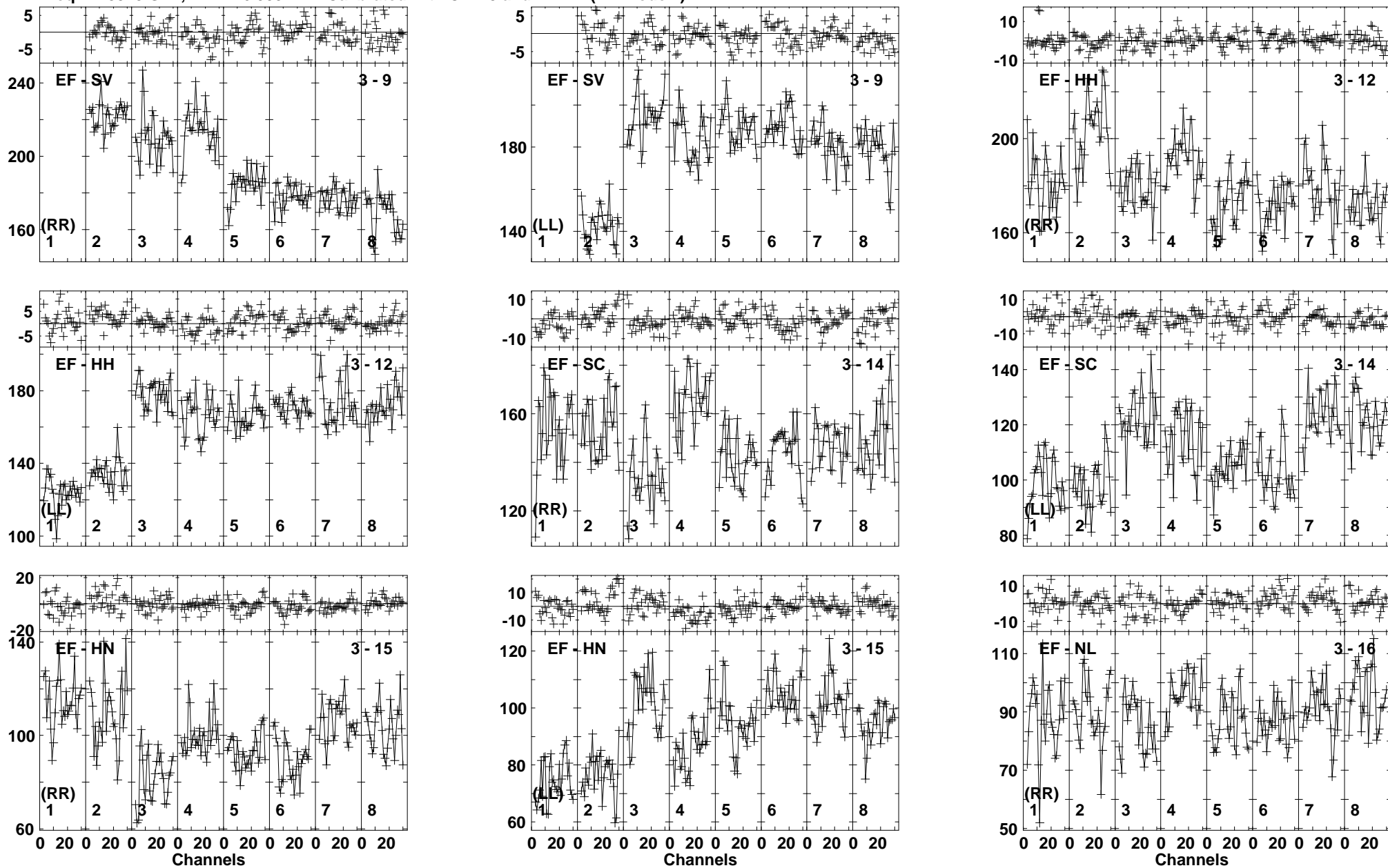
Lower frame: Milli Ampl Jy Top frame: Phas deg Vector averaged cross-power spectrum Baseline: EF (03) - SV (09) Timerange: 00/21:34:46 to 00/21:35:44
