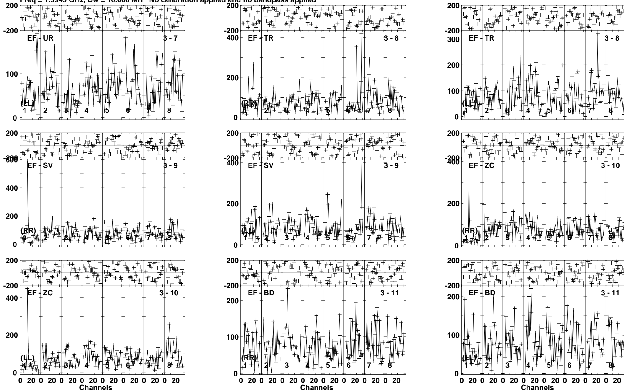
Lower frame: Micro Ampl Jy Top frame: Phas deg Vector averaged cross-power spectrum Baseline: EF (03) - UR (07) Timerange: 00/18:59:22 to 00/19:02:44
