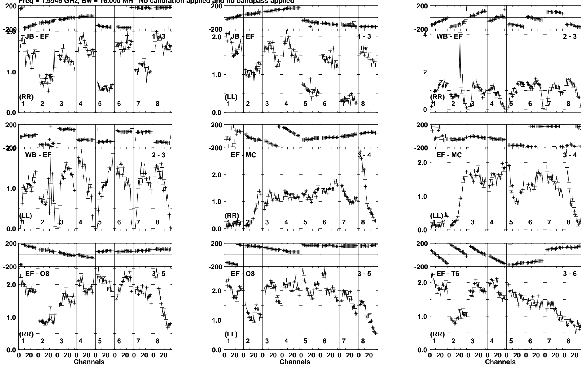
Lower frame: Milli Ampl Jy Top frame: Phas deg Vector averaged cross-power spectrum Baseline: JB (01) - EF (03) Timerange: 00/15:04:07 to 00/15:05:29
