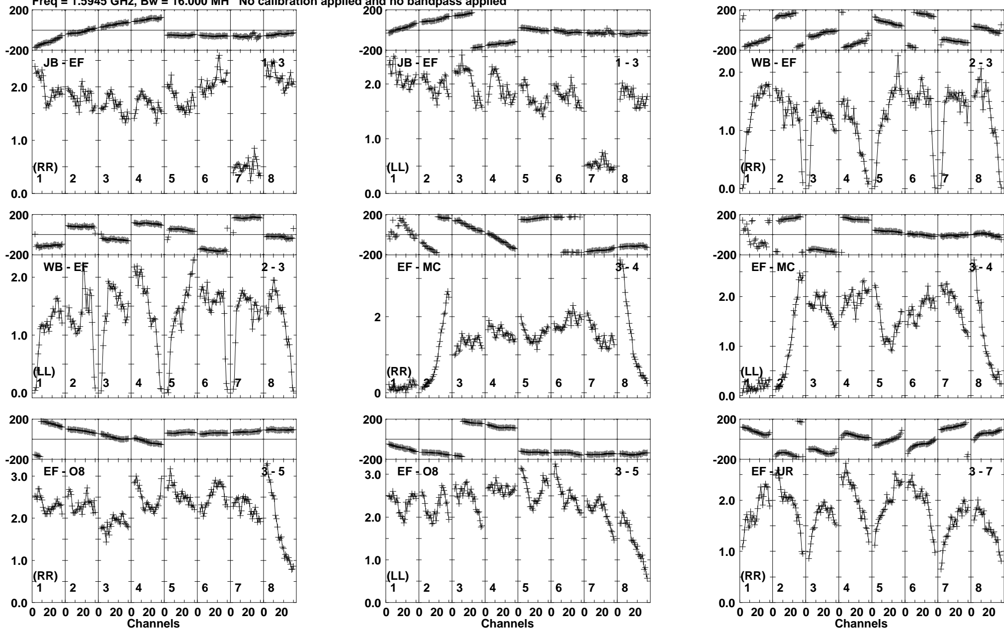
Lower frame: Milli Ampl Jy Top frame: Phas deg Vector averaged cross-power spectrum Baseline: JB (01) - EF (03) Timerange: 00/19:08:26 to 00/19:09:24
