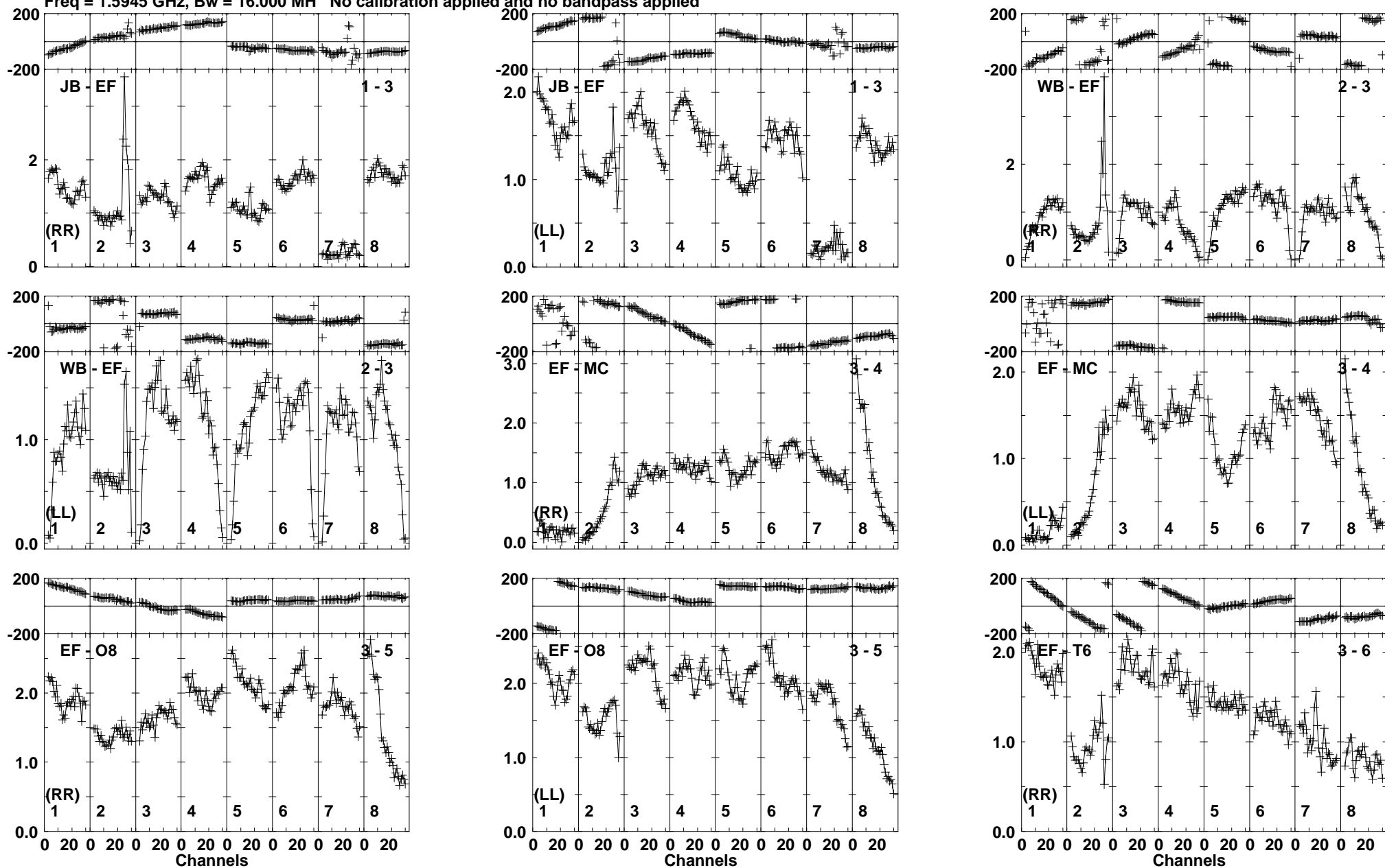
Lower frame: Milli Ampl Jy Top frame: Phas deg Vector averaged cross-power spectrum Baseline: JB (01) - EF (03) Timerange: 00/15:14:17 to 00/15:15:39
