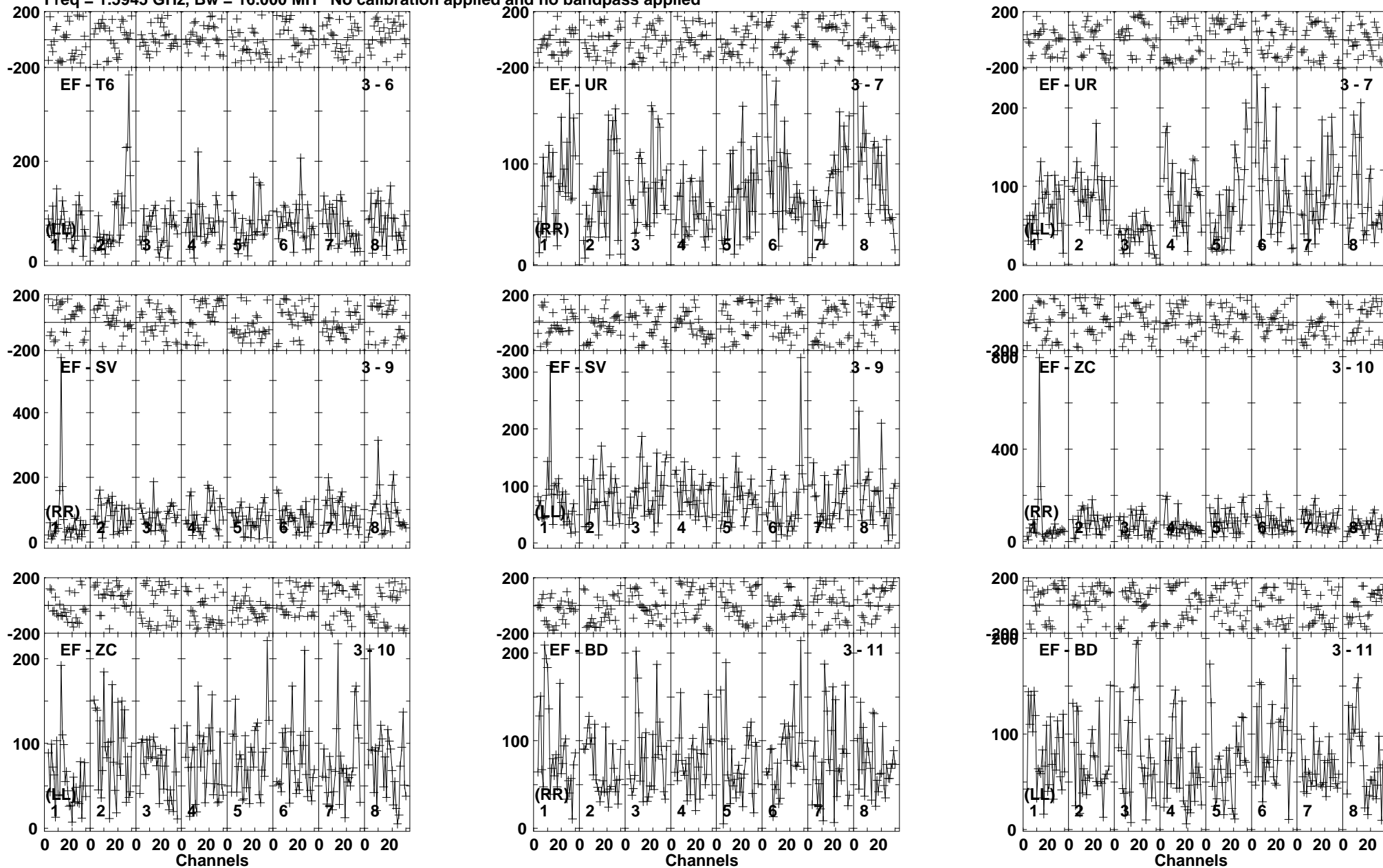
Lower frame: Micro Ampl Jy Top frame: Phas deg Vector averaged cross-power spectrum Baseline: EF (03) - T6 (06) Timerange: 00/15:25:57 to 00/15:29:19
