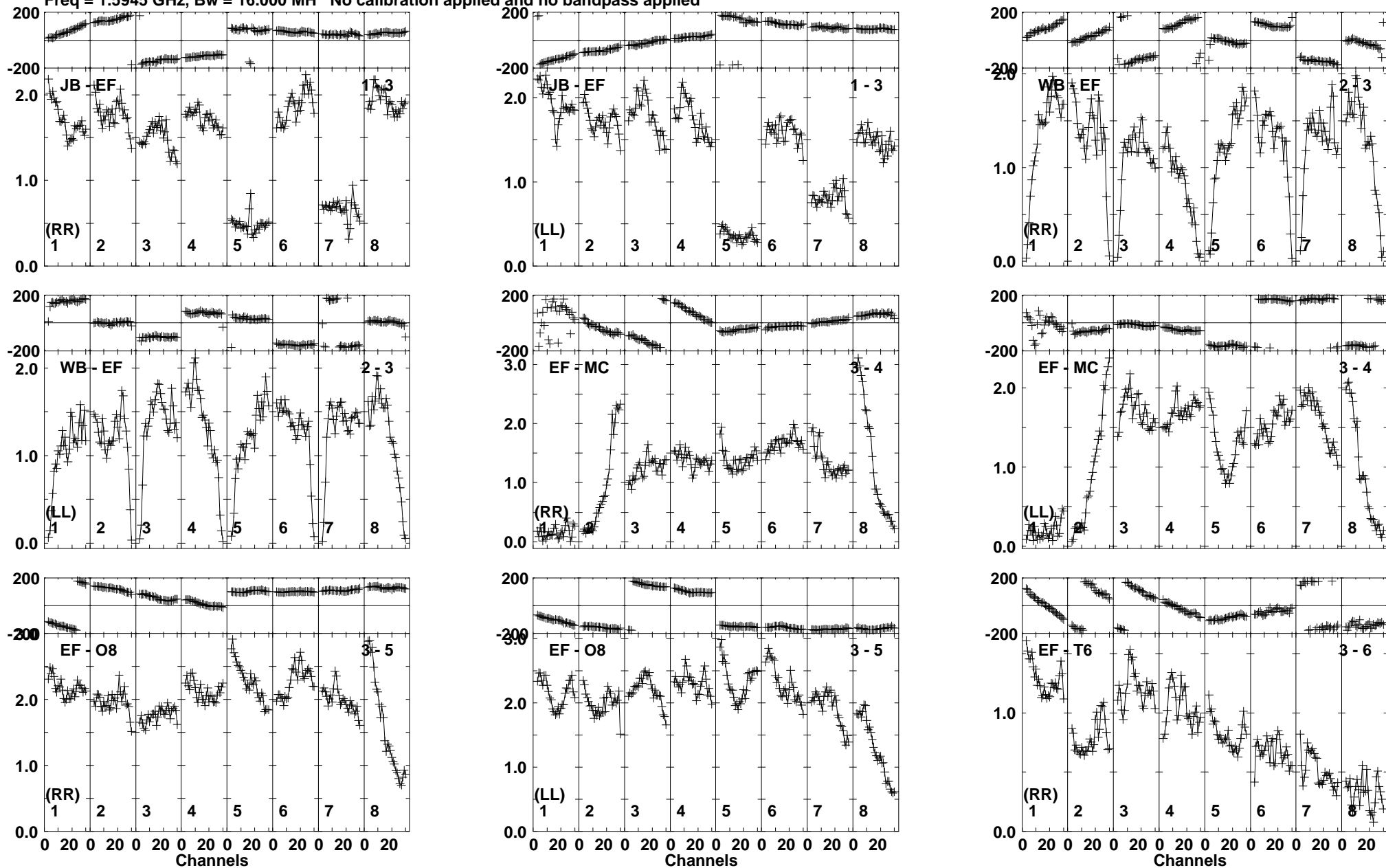
Lower frame: Milli Ampl Jy Top frame: Phas deg Vector averaged cross-power spectrum Baseline: JB (01) - EF (03) Timerange: 00/16:05:07 to 00/16:06:29
