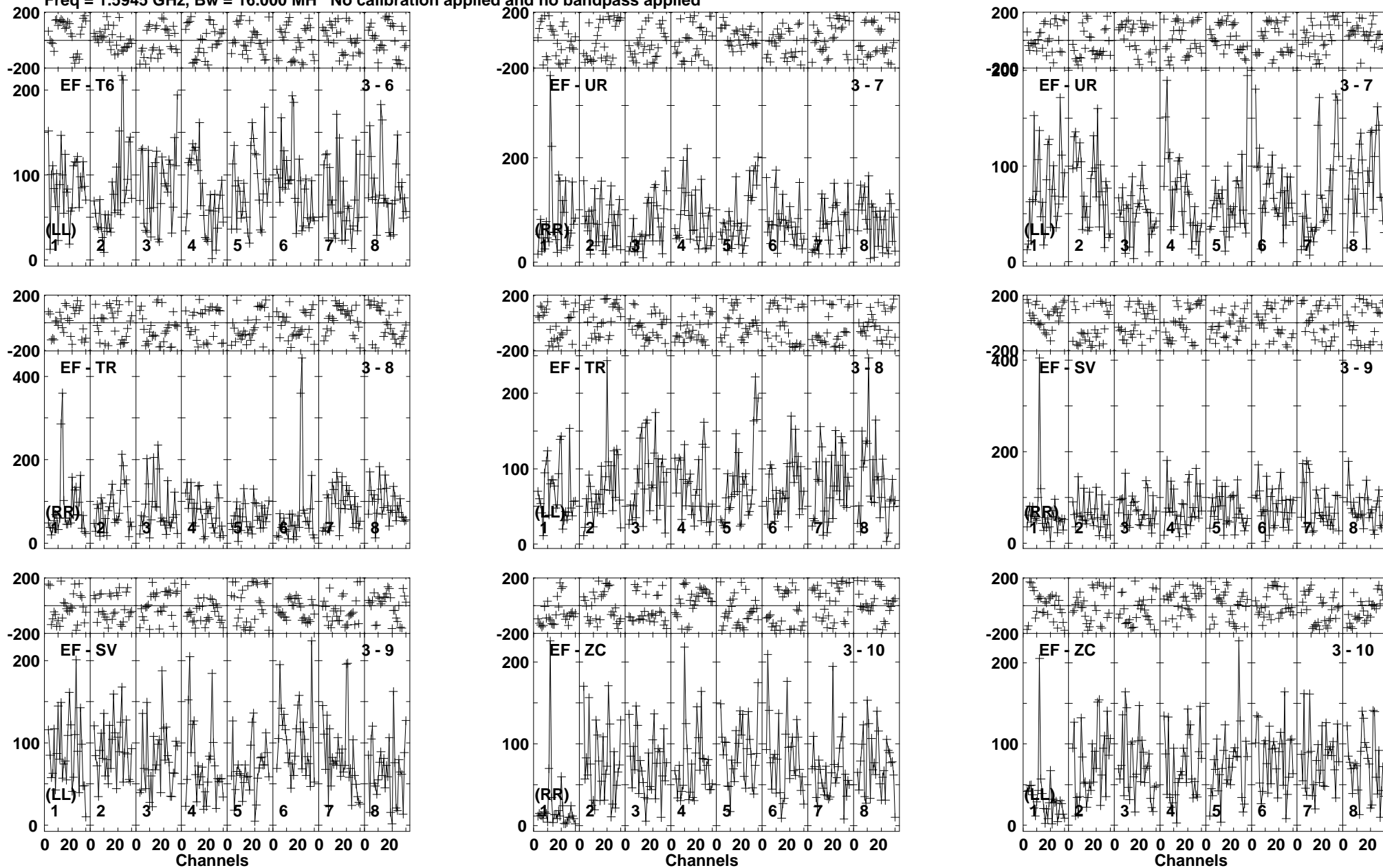
Lower frame: Micro Ampl Jy Top frame: Phas deg Vector averaged cross-power spectrum Baseline: EF (03) - T6 (06) Timerange: 00/18:18:42 to 00/18:22:04
