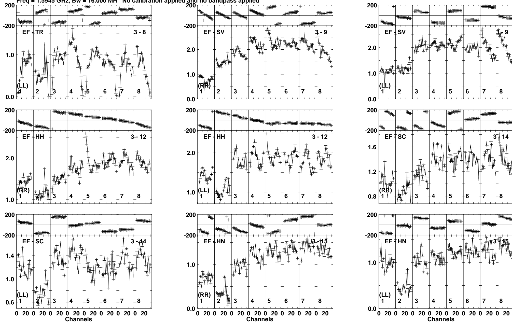
Lower frame: Milli Ampl Jy Top frame: Phas deg Vector averaged cross-power spectrum Baseline: EF (03) - TR (08) Timerange: 00/21:04:16 to 00/21:05:14
