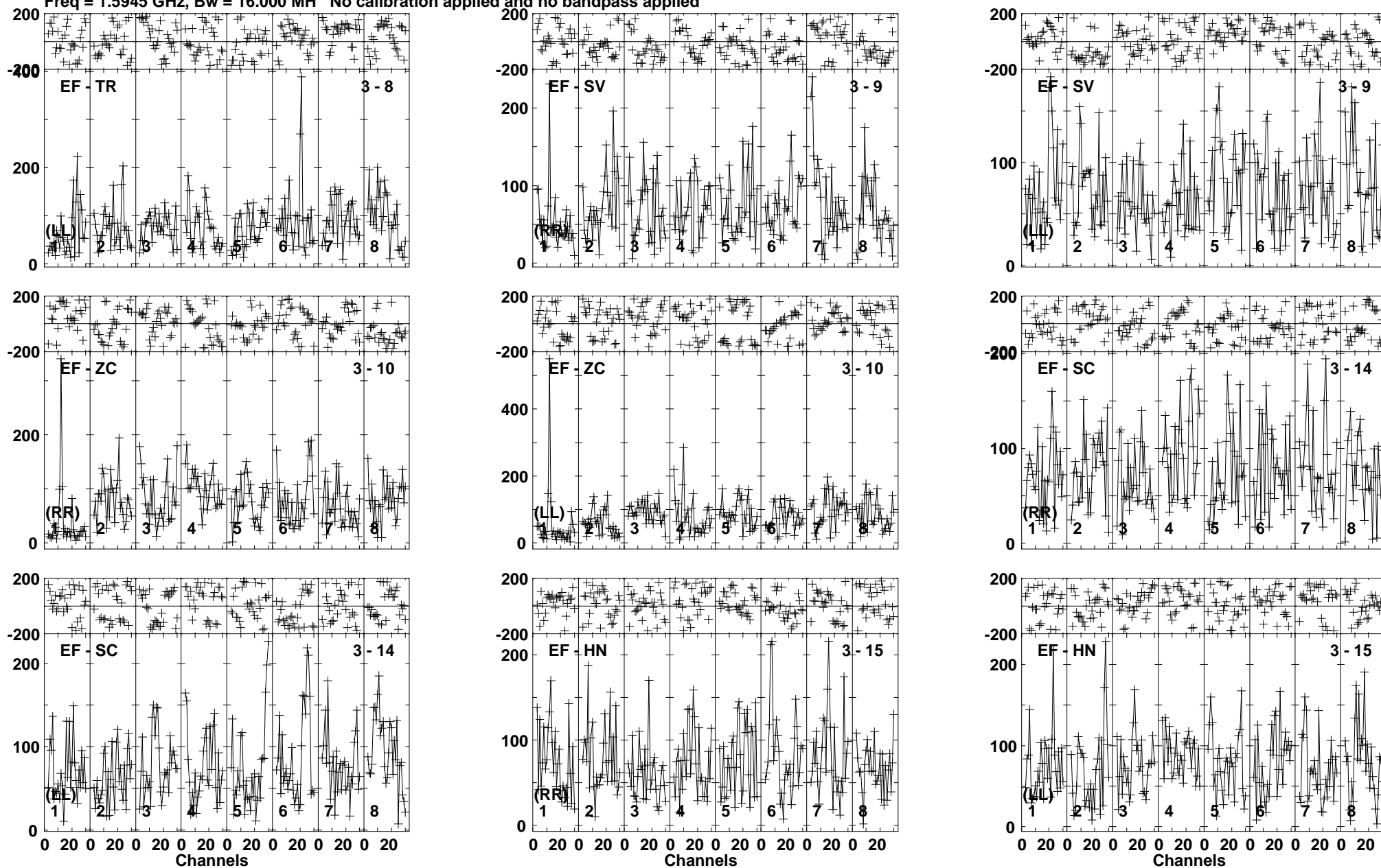
Lower frame: Micro Ampl Jy Top frame: Phas deg Vector averaged cross-power spectrum Baseline: EF (03) - TR (08) Timerange: 00/23:37:48 to 00/23:41:14
