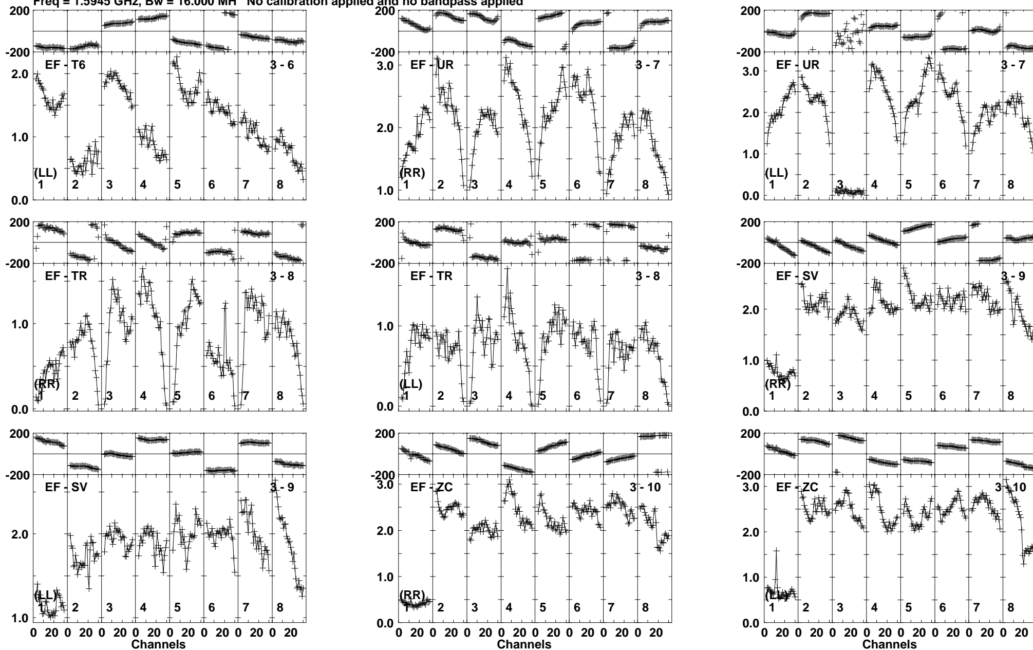
Lower frame: Milli Ampl Jy Top frame: Phas deg Vector averaged cross-power spectrum Baseline: EF (03) - T6 (06) Timerange: 00/16:25:27 to 00/16:26:49
