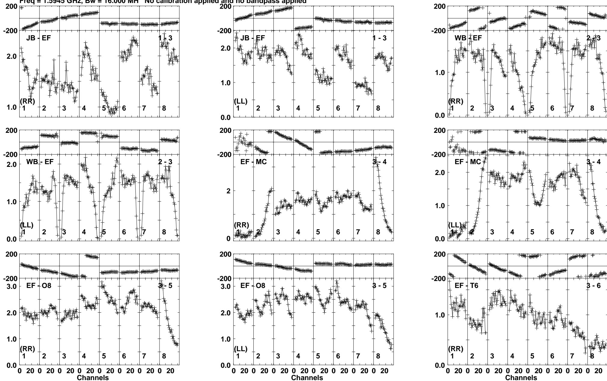
Lower frame: Milli Ampl Jy Top frame: Phas deg Vector averaged cross-power spectrum Baseline: JB (01) - EF (03) Timerange: 00/18:12:02 to 00/18:13:24
