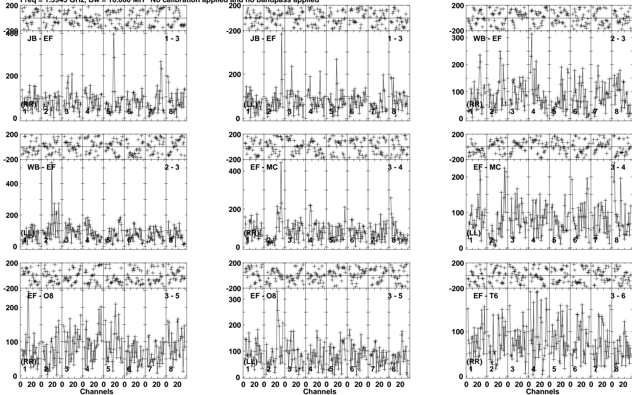
Lower frame: Micro Ampl Jy Top frame: Phas deg Vector averaged cross-power spectrum Baseline: JB (01) - EF (03) Timerange: 00/18:08:32 to 00/18:11:54
