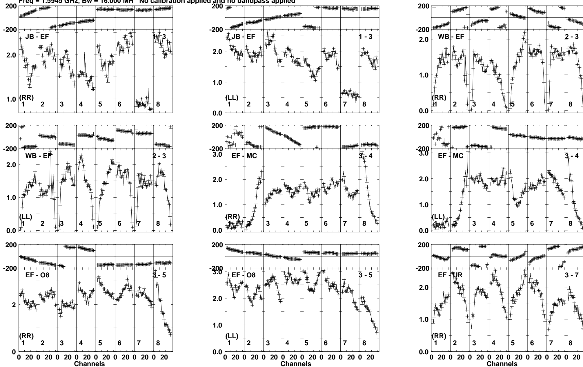
Lower frame: Milli Ampl Jy Top frame: Phas deg Vector averaged cross-power spectrum Baseline: JB (01) - EF (03) Timerange: 00/20:23:36 to 00/20:24:34
