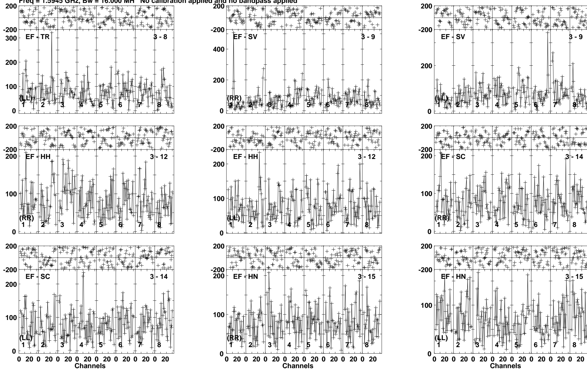
Lower frame: Micro Ampl Jy Top frame: Phas deg Vector averaged cross-power spectrum Baseline: EF (03) - TR (08) Timerange: 00/21:10:24 to 00/21:13:44
