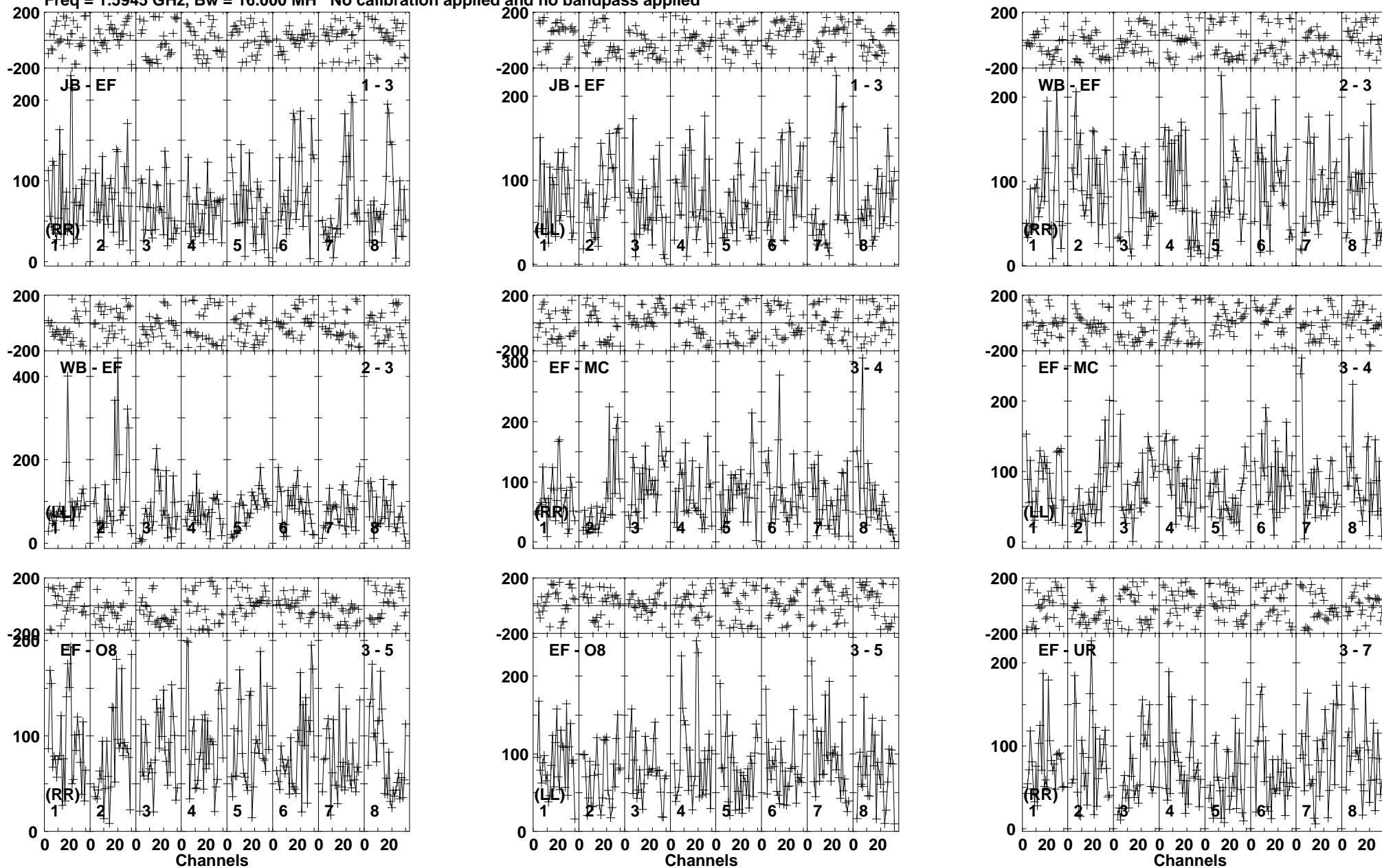
Lower frame: Micro Ampl Jy Top frame: Phas deg Vector averaged cross-power spectrum Baseline: JB (01) - EF (03) Timerange: 00/19:35:01 to 00/19:38:19
