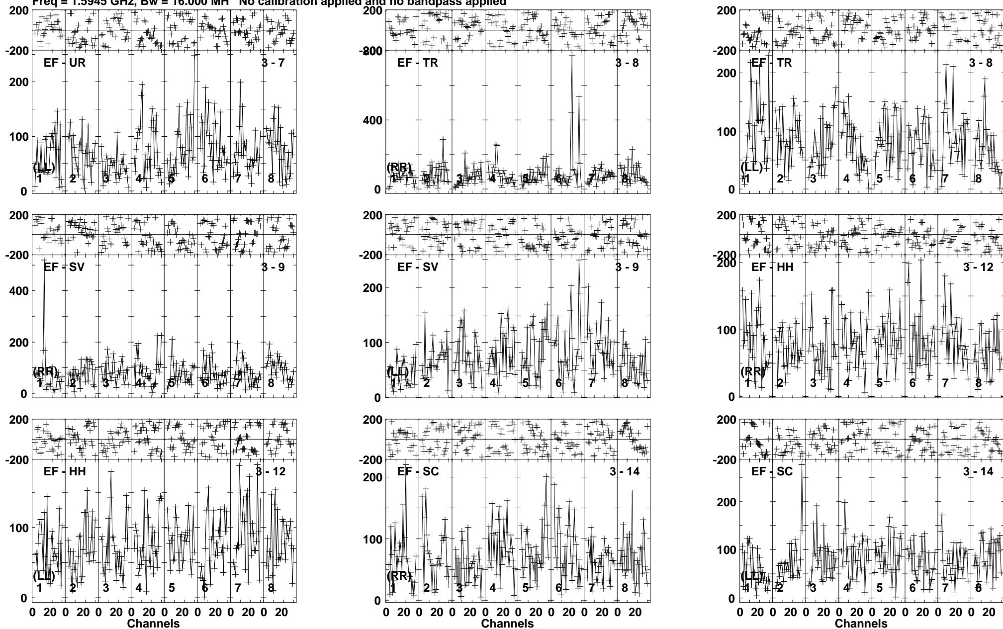
Lower frame: Micro Ampl Jy Top frame: Phas deg Vector averaged cross-power spectrum Baseline: EF (03) - UR (07) Timerange: 00/20:19:32 to 00/20:22:54
