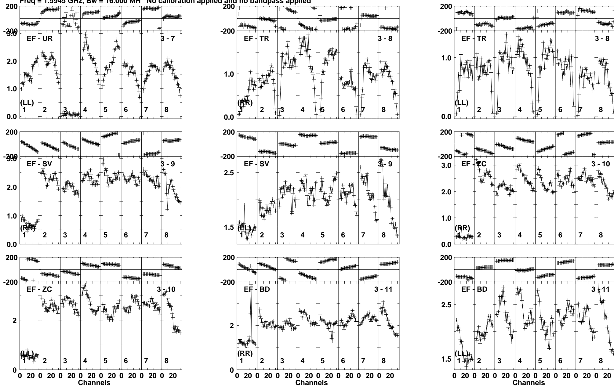
Lower frame: Milli Ampl Jy Top frame: Phas deg Vector averaged cross-power spectrum Baseline: EF (03) - UR (07) Timerange: 00:18:37:56 to 00:18:38:54
