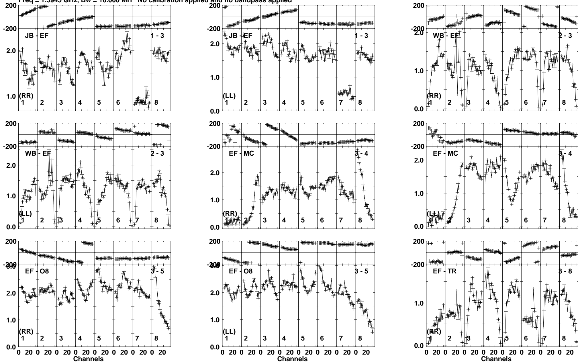
Lower frame: Milli Ampl Jy Top frame: Phas deg Vector averaged cross-power spectrum Baseline: JB (01) - EF (03) Timerange: 00/23:36:46 to 00/23:37:44
