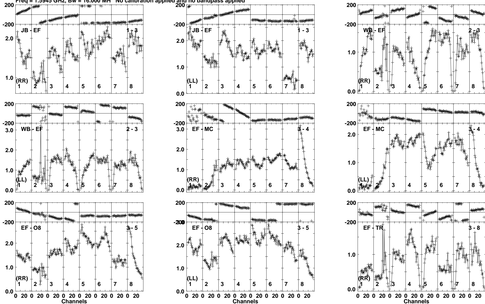
Lower frame: Milli Ampl Jy Top frame: Phas deg Vector averaged cross-power spectrum Baseline: JB (01) - EF (03) Timerange: 00/23:26:36 to 00/23:27:34
