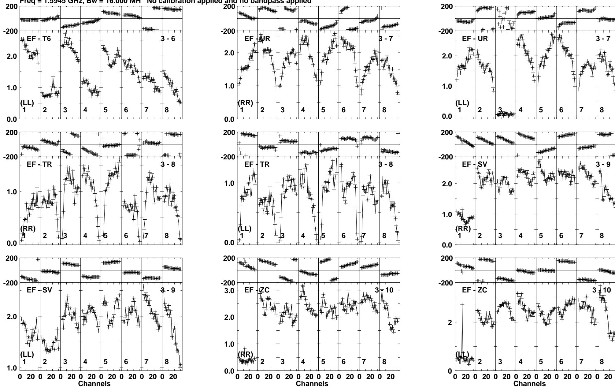
Lower frame: Milli Ampl Jy Top frame: Phas deg Vector averaged cross-power spectrum Baseline: EF (03) - T6 (06) Timerange: 00/17:42:11 to 00/17:43:09
