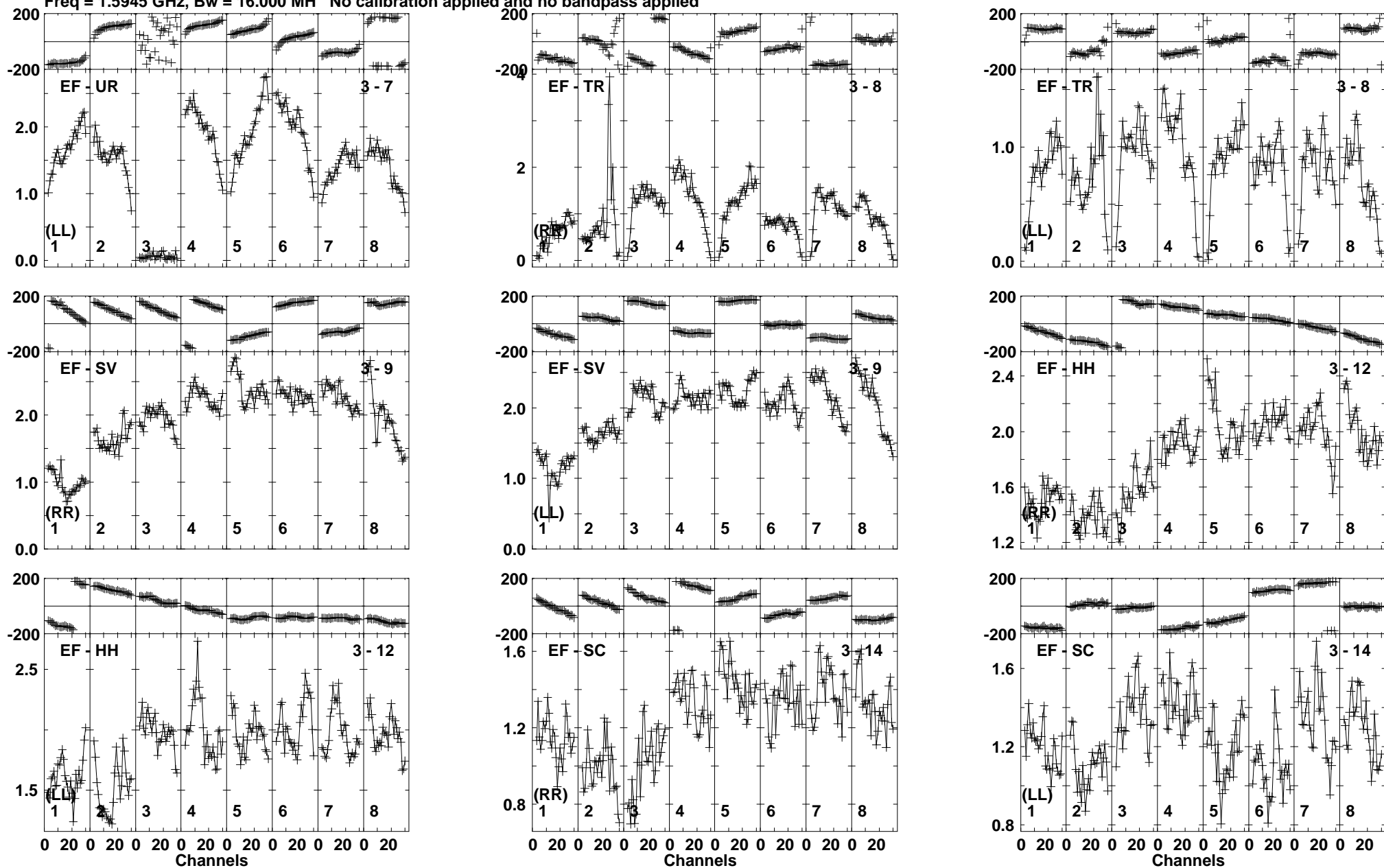
Lower frame: Milli Ampl Jy Top frame: Phas deg Vector averaged cross-power spectrum Baseline: EF (03) - UR (07) Timerange: 00/20:18:02 to 00/20:19:24
