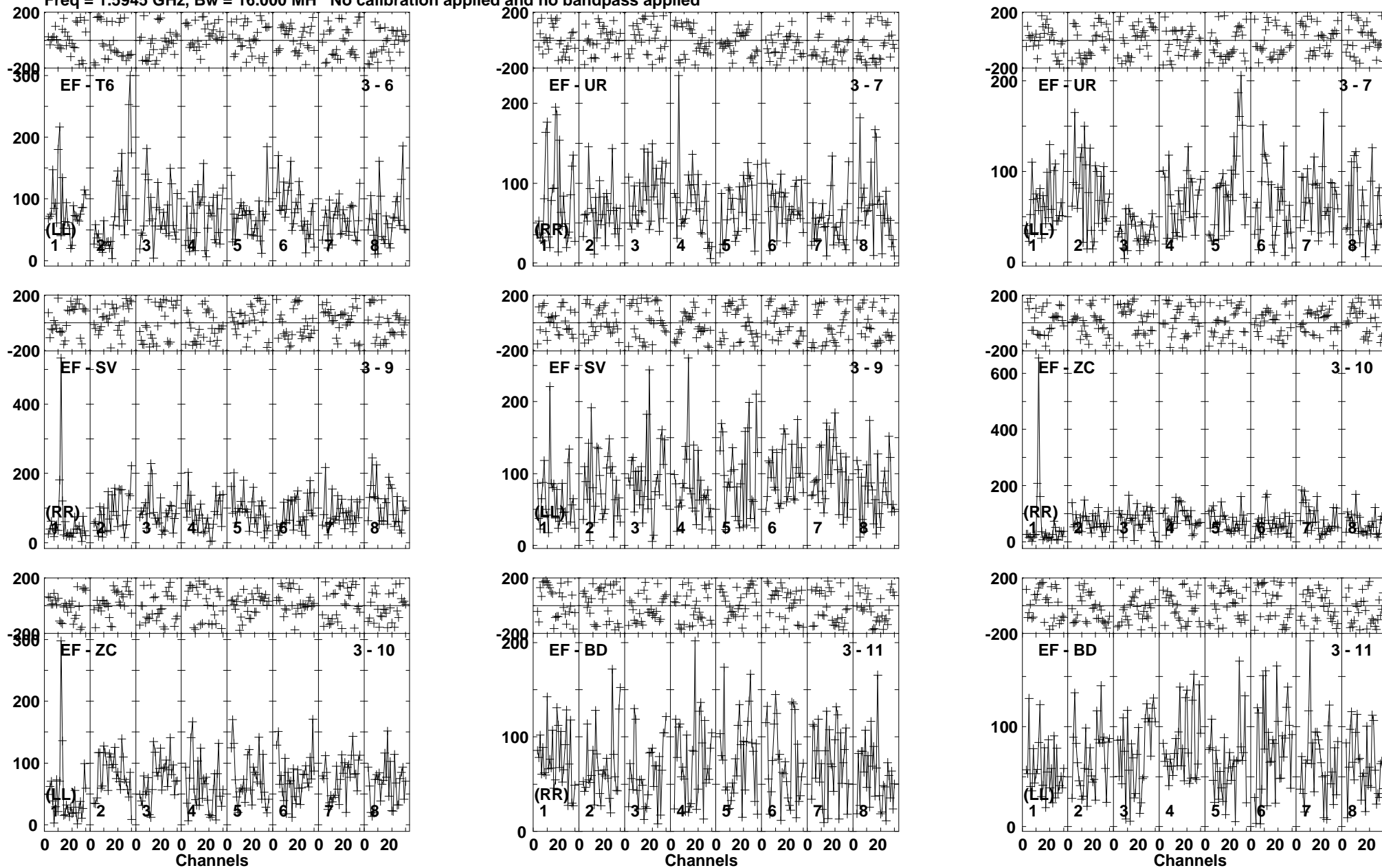
Lower frame: Micro Ampl Jy Top frame: Phas deg Vector averaged cross-power spectrum Baseline: EF (03) - T6 (06) Timerange: 00/14:31:07 to 00/14:34:39
