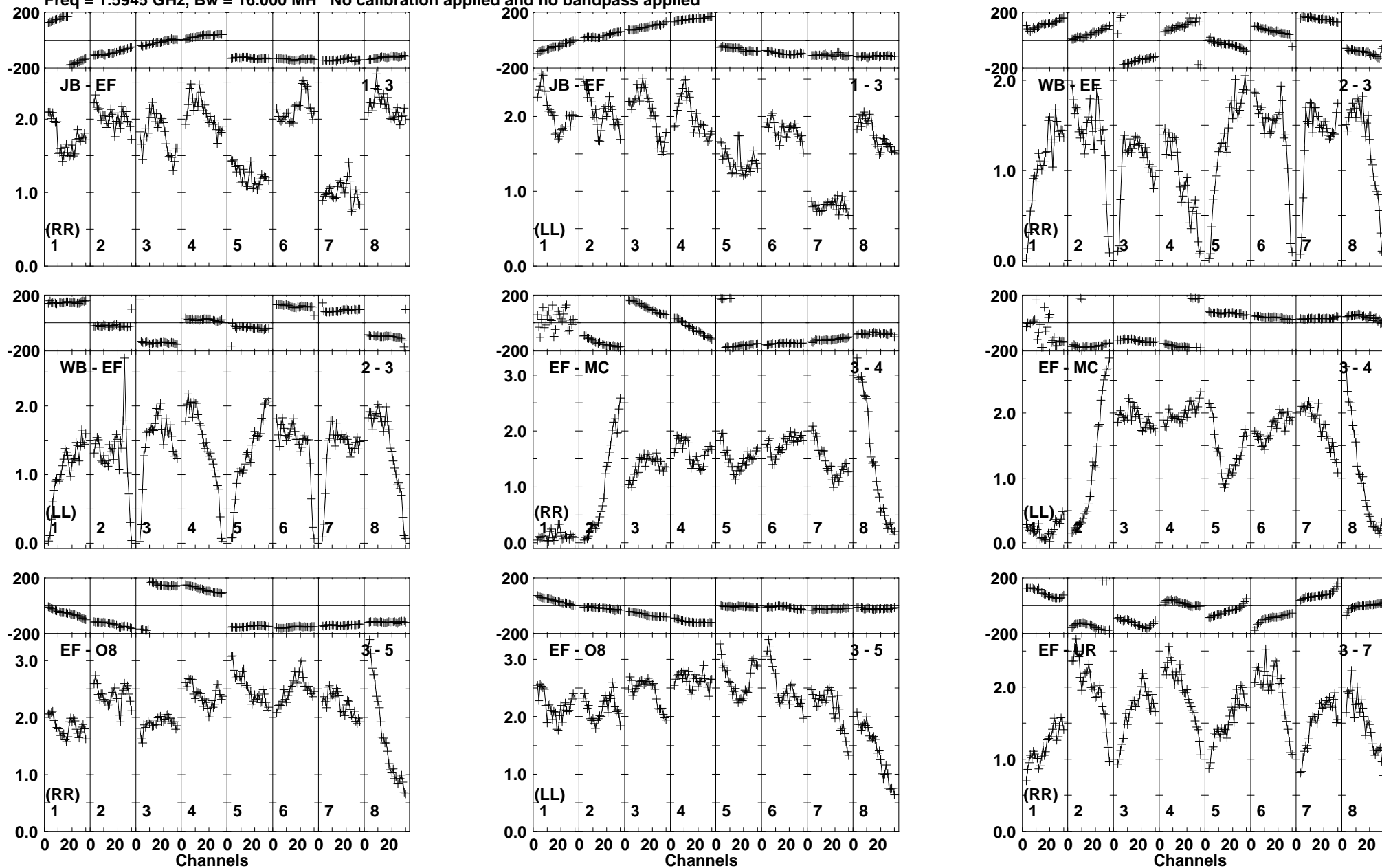
Lower frame: Milli Ampl Jy Top frame: Phas deg Vector averaged cross-power spectrum Baseline: JB (01) - EF (03) Timerange: 00/18:27:46 to 00/18:28:44
