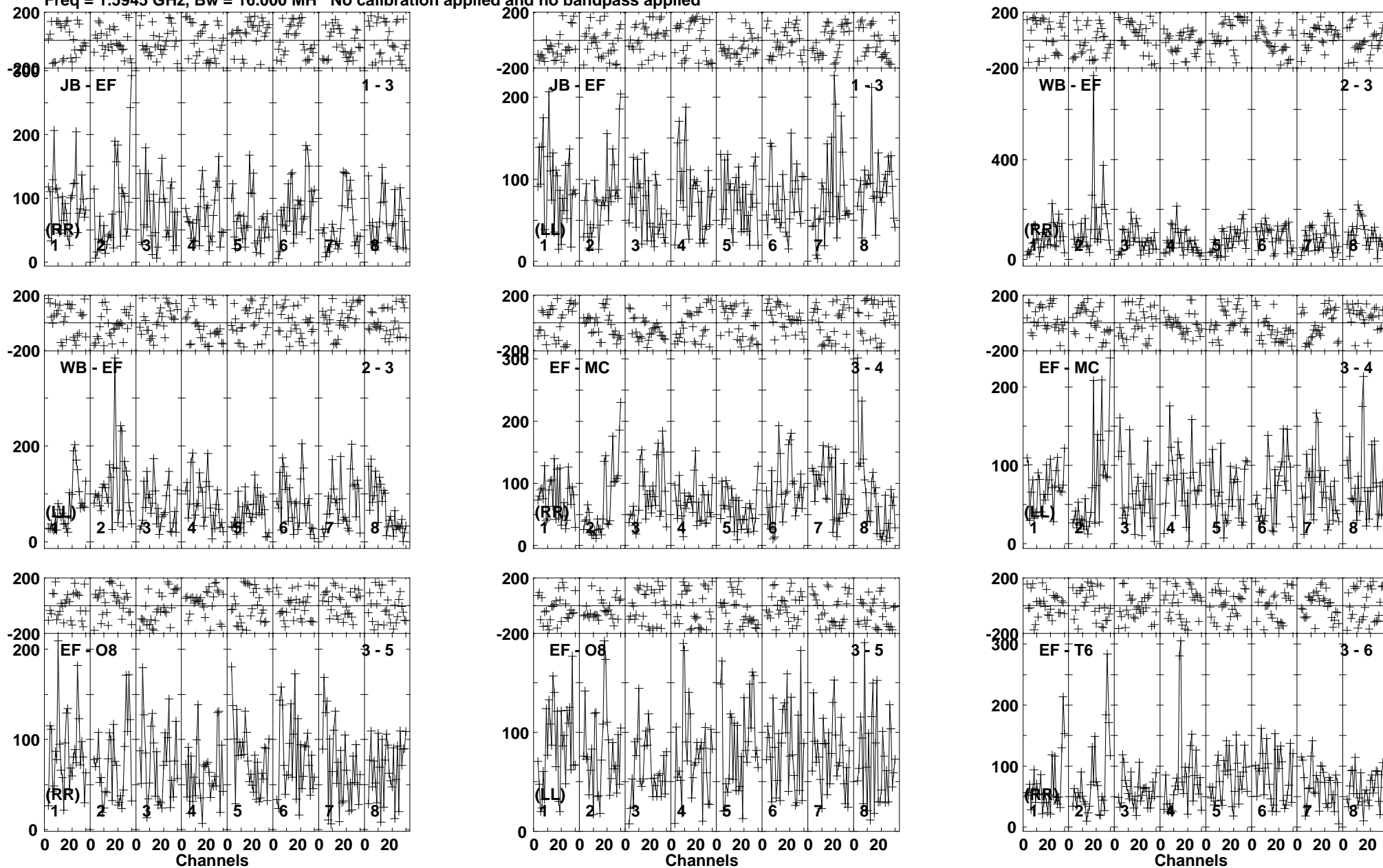
Lower frame: Micro Ampl Jy Top frame: Phas deg Vector averaged cross-power spectrum Baseline: JB (01) - EF (03) Timerange: 00/17:43:17 to 00/17:46:39
