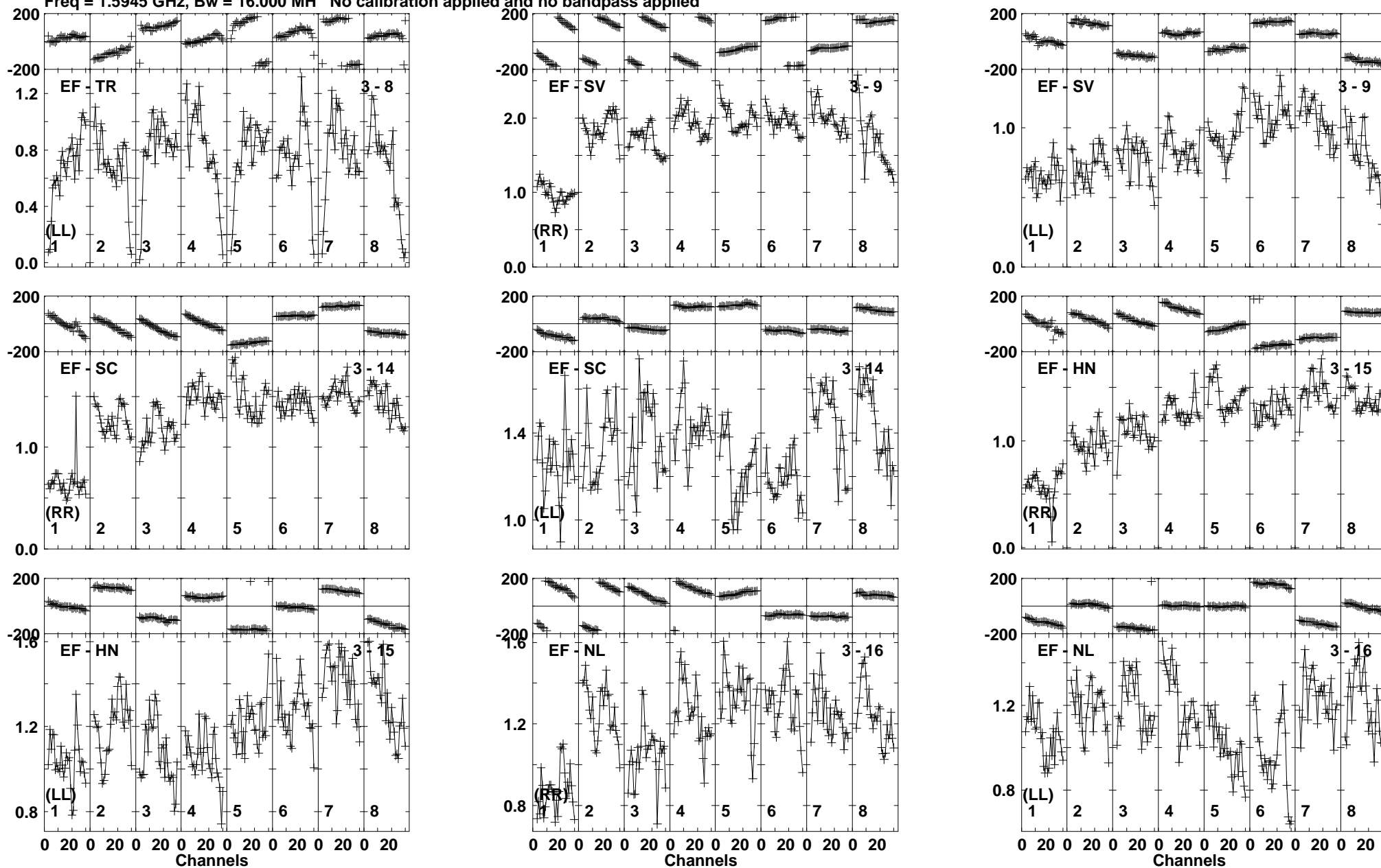
Lower frame: Milli Ampl Jy Top frame: Phas deg Vector averaged cross-power spectrum Baseline: EF (03) - TR (08) Timerange: 00/23:51:34 to 00/23:52:54
