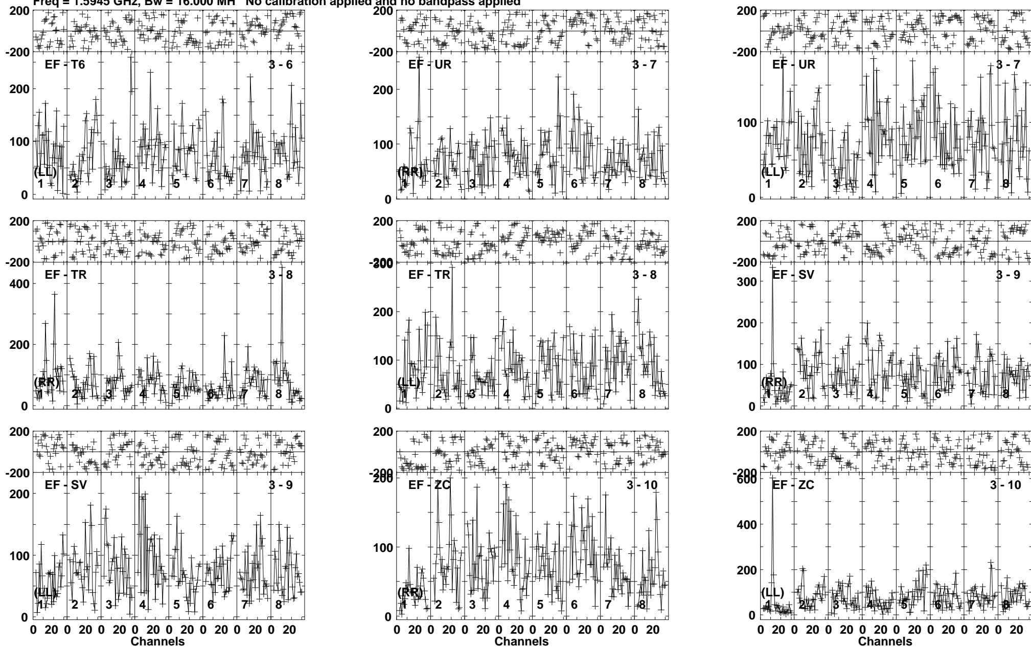
Lower frame: Micro Ampl Jy Top frame: Phas deg Vector averaged cross-power spectrum Baseline: EF (03) - T6 (06) Timerange: 00/16:52:27 to 00/16:55:49
