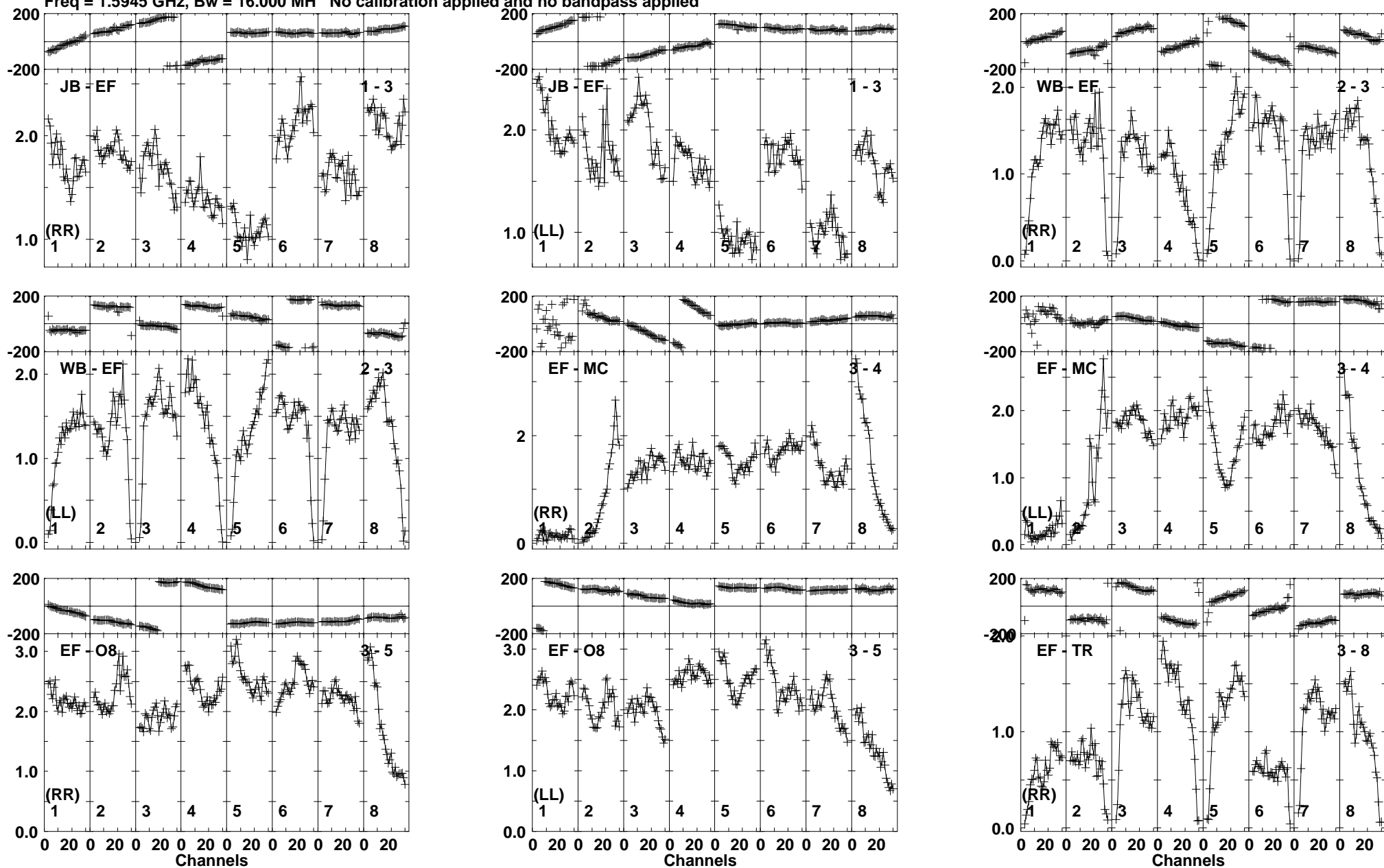
Lower frame: Milli Ampl Jy Top frame: Phas deg Vector averaged cross-power spectrum Baseline: JB (01) - EF (03) Timerange: 00:22:09:54 to 00:22:11:14
