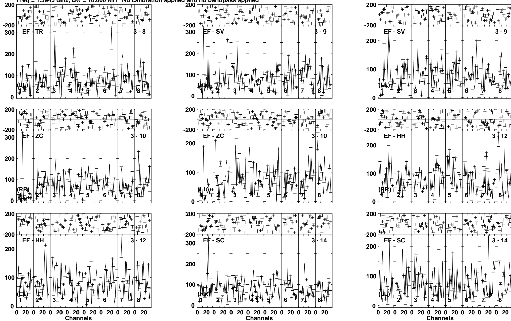
Lower frame: Micro Ampl Jy Top frame: Phas deg Vector averaged cross-power spectrum Baseline: EF (03) - TR (08) Timerange: 00/22:52:02 to 00/22:55:24
