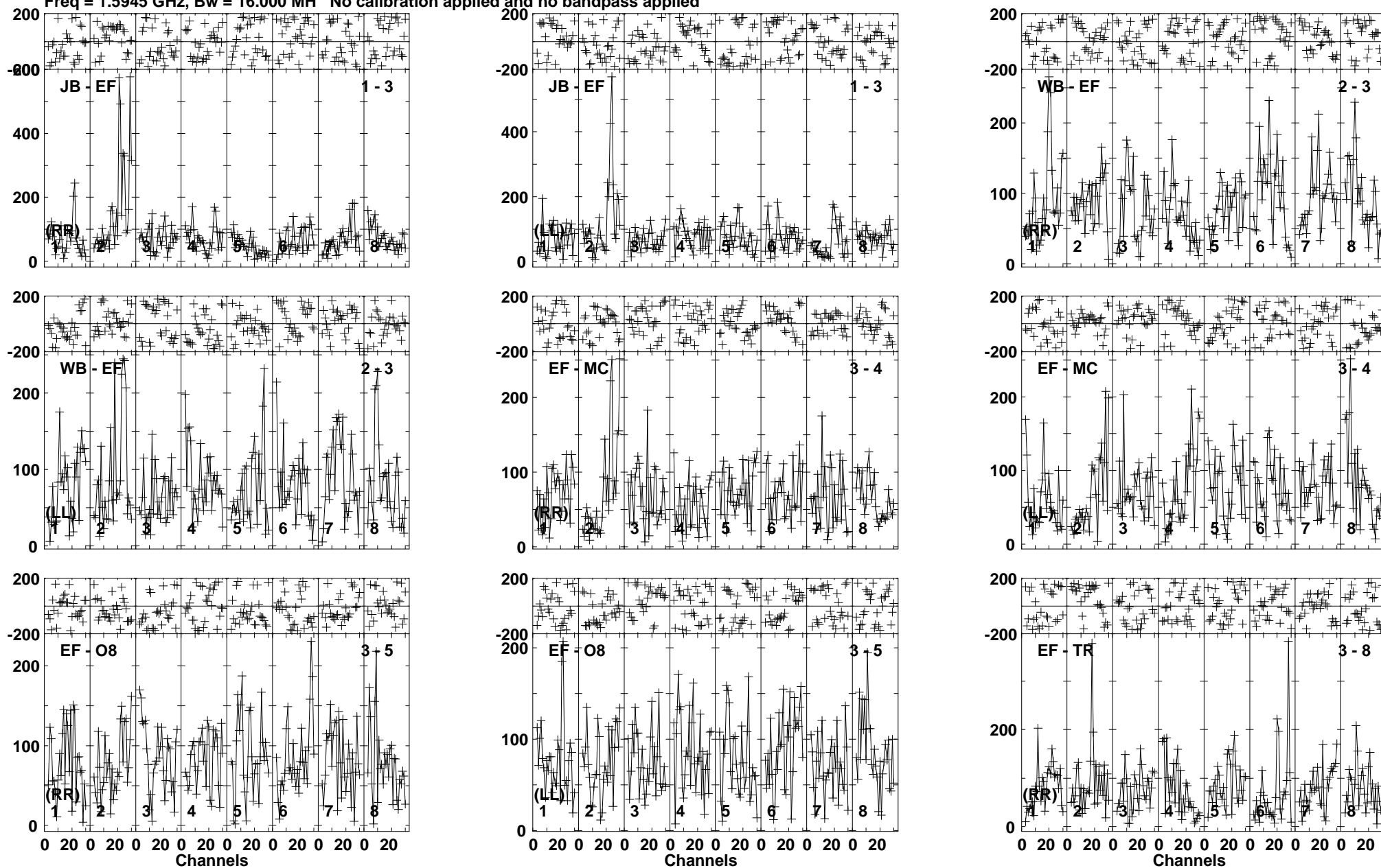
Lower frame: Micro Ampl Jy Top frame: Phas deg Vector averaged cross-power spectrum Baseline: JB (01) - EF (03) Timerange: 00/22:31:42 to 00/22:35:04
