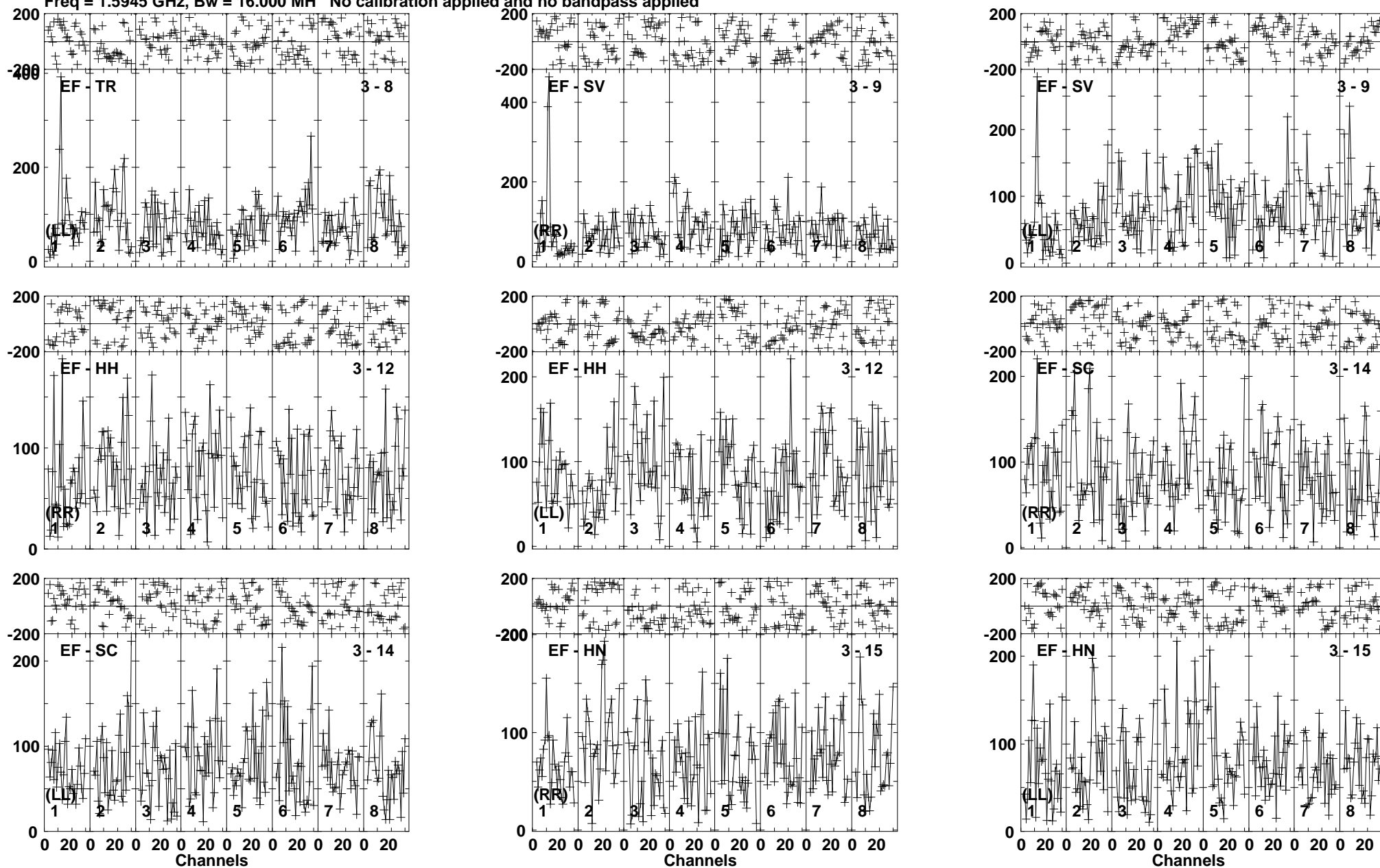
Lower frame: Micro Ampl Jy Top frame: Phas deg Vector averaged cross-power spectrum Baseline: EF (03) - TR (08) Timerange: 00/21:25:44 to 00/21:29:04
