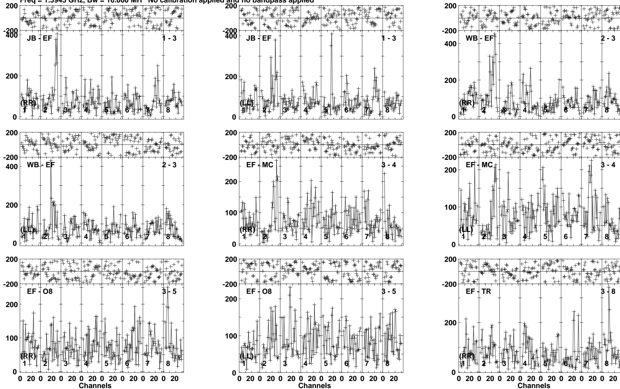
Lower frame: Micro Ampl Jy Top frame: Phas deg Vector averaged cross-power spectrum Baseline: JB (01) - EF (03) Timerange: 00/22:11:22 to 00/22:14:44
