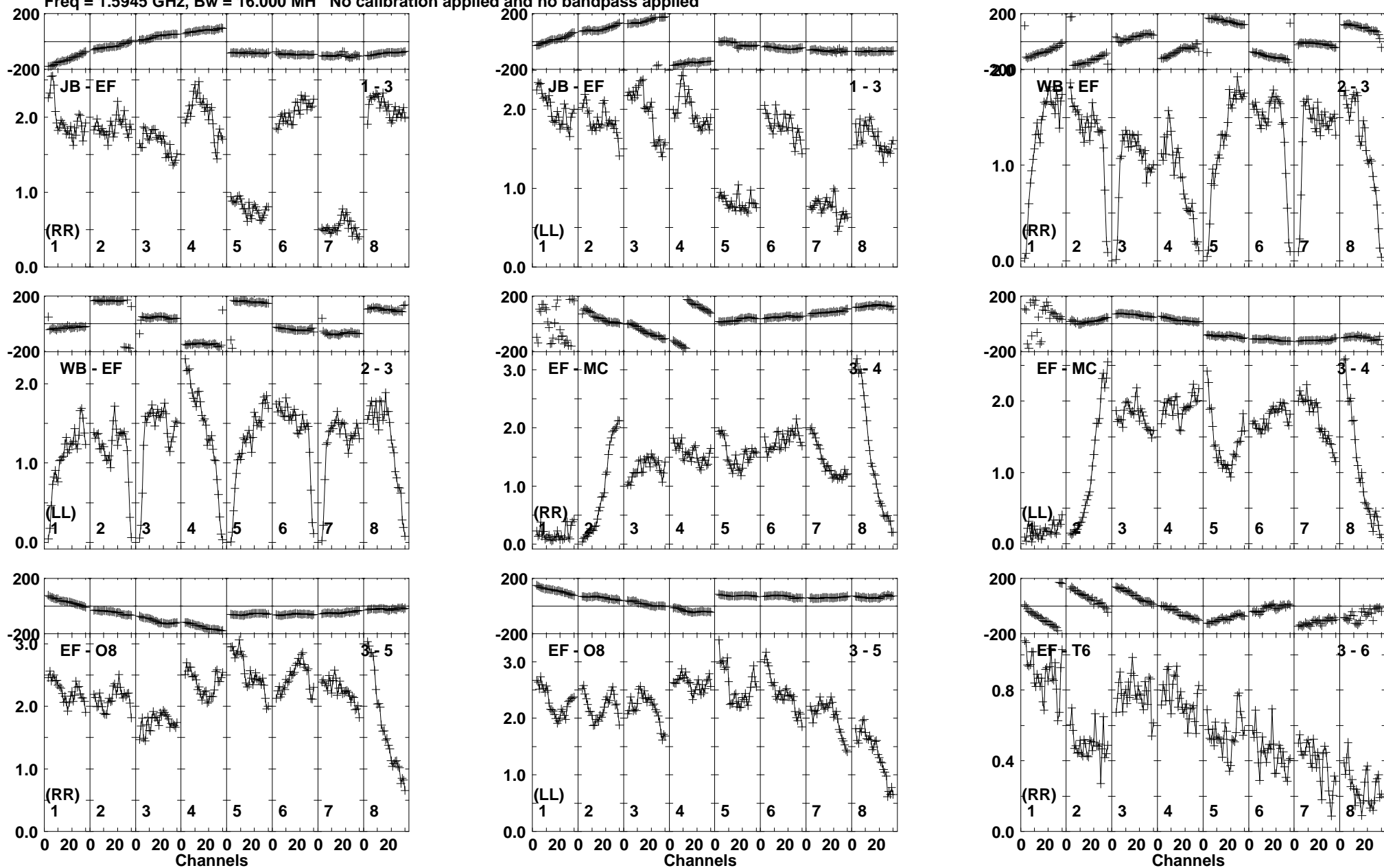
Lower frame: Milli Ampl Jy Top frame: Phas deg Vector averaged cross-power spectrum Baseline: JB (01) - EF (03) Timerange: 00/18:02:16 to 00/18:03:14
