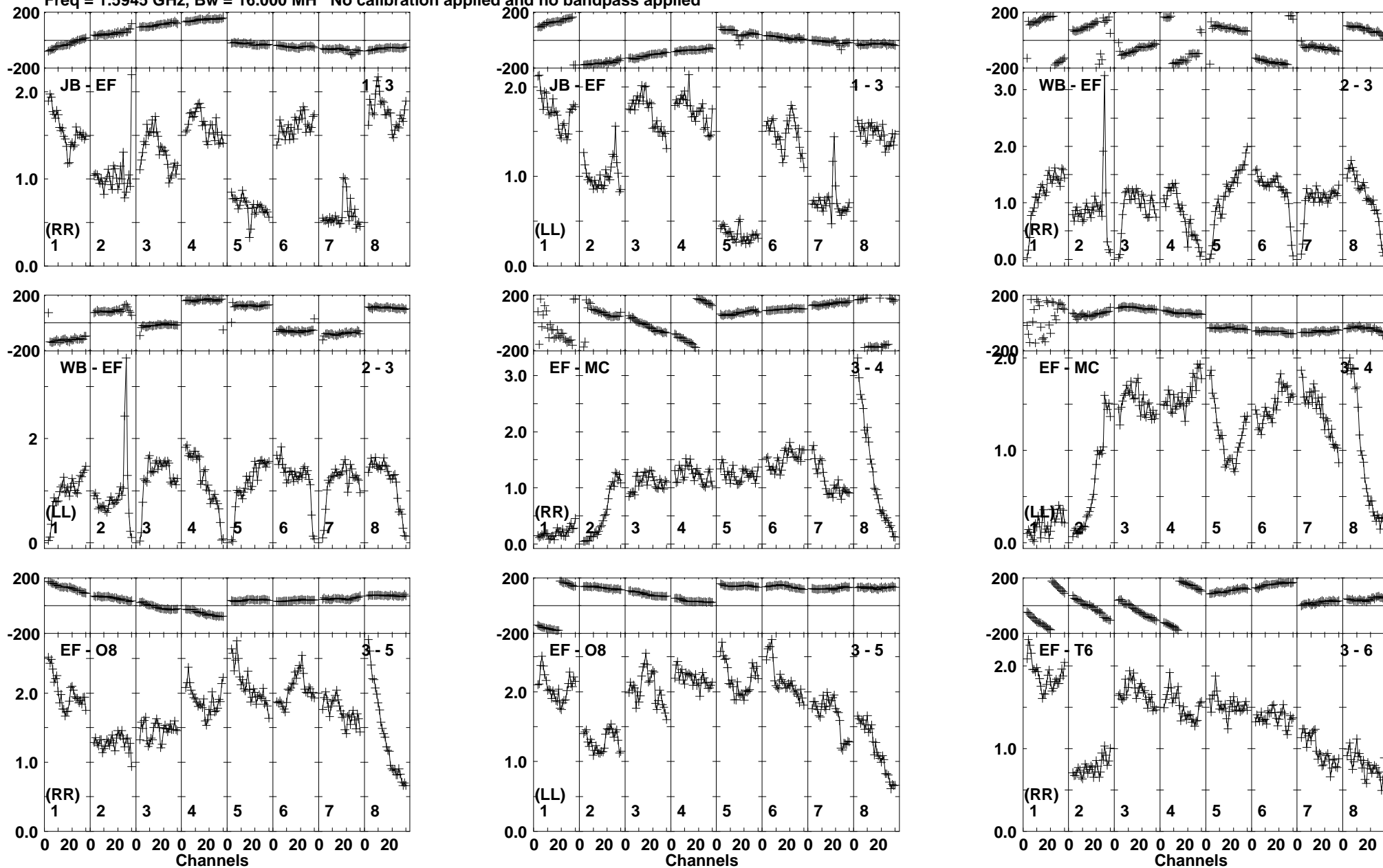
Lower frame: Milli Ampl Jy Top frame: Phas deg Vector averaged cross-power spectrum Baseline: JB (01) - EF (03) Timerange: 00/15:24:27 to 00/15:25:49
