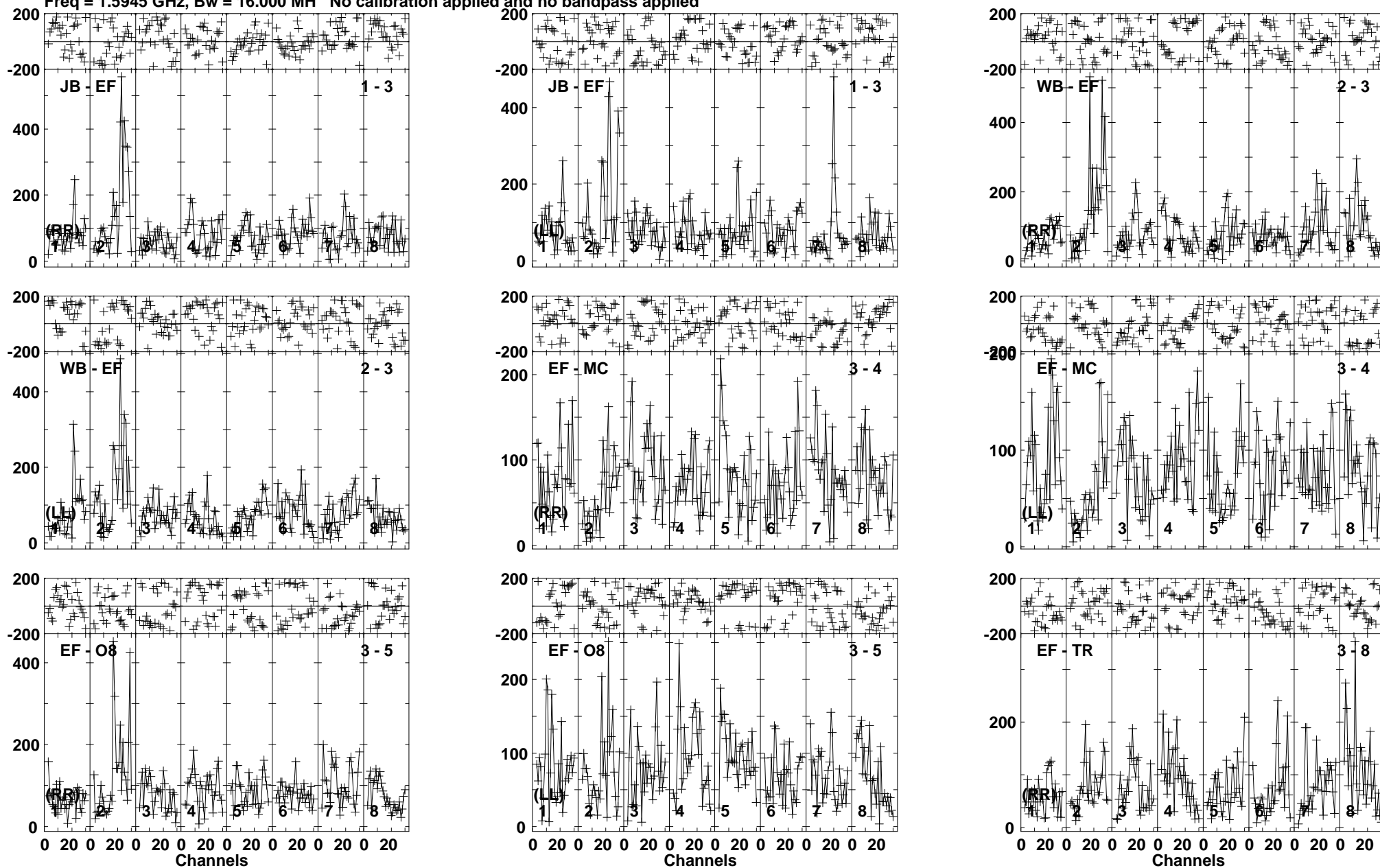
Lower frame: Micro Ampl Jy Top frame: Phas deg Vector averaged cross-power spectrum Baseline: JB (01) - EF (03) Timerange: 00/22:57:12 to 00/23:00:34
