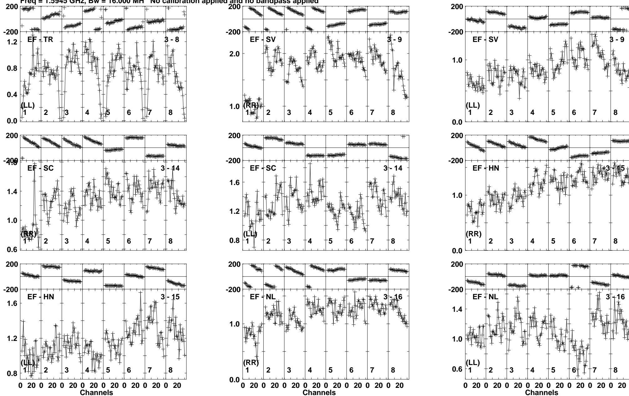
Lower frame: Milli Ampl Jy Top frame: Phas deg Vector averaged cross-power spectrum Baseline: EF (03) - TR (08) Timerange: 00/23:57:06 to 00/23:58:04
