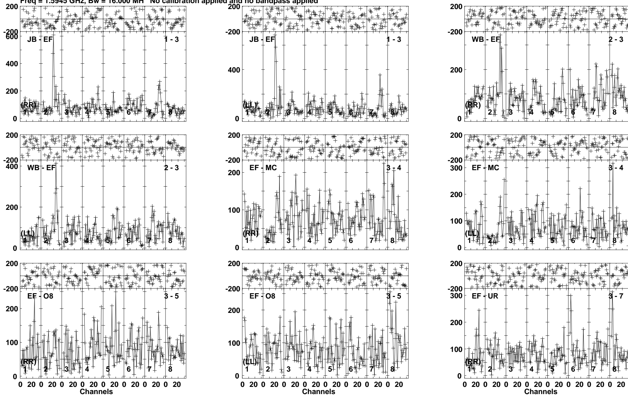
Lower frame: Micro Ampl Jy Top frame: Phas deg Vector averaged cross-power spectrum Baseline: JB (01) - EF (03) Timerange: 00/18:44:02 to 00/18:47:24
