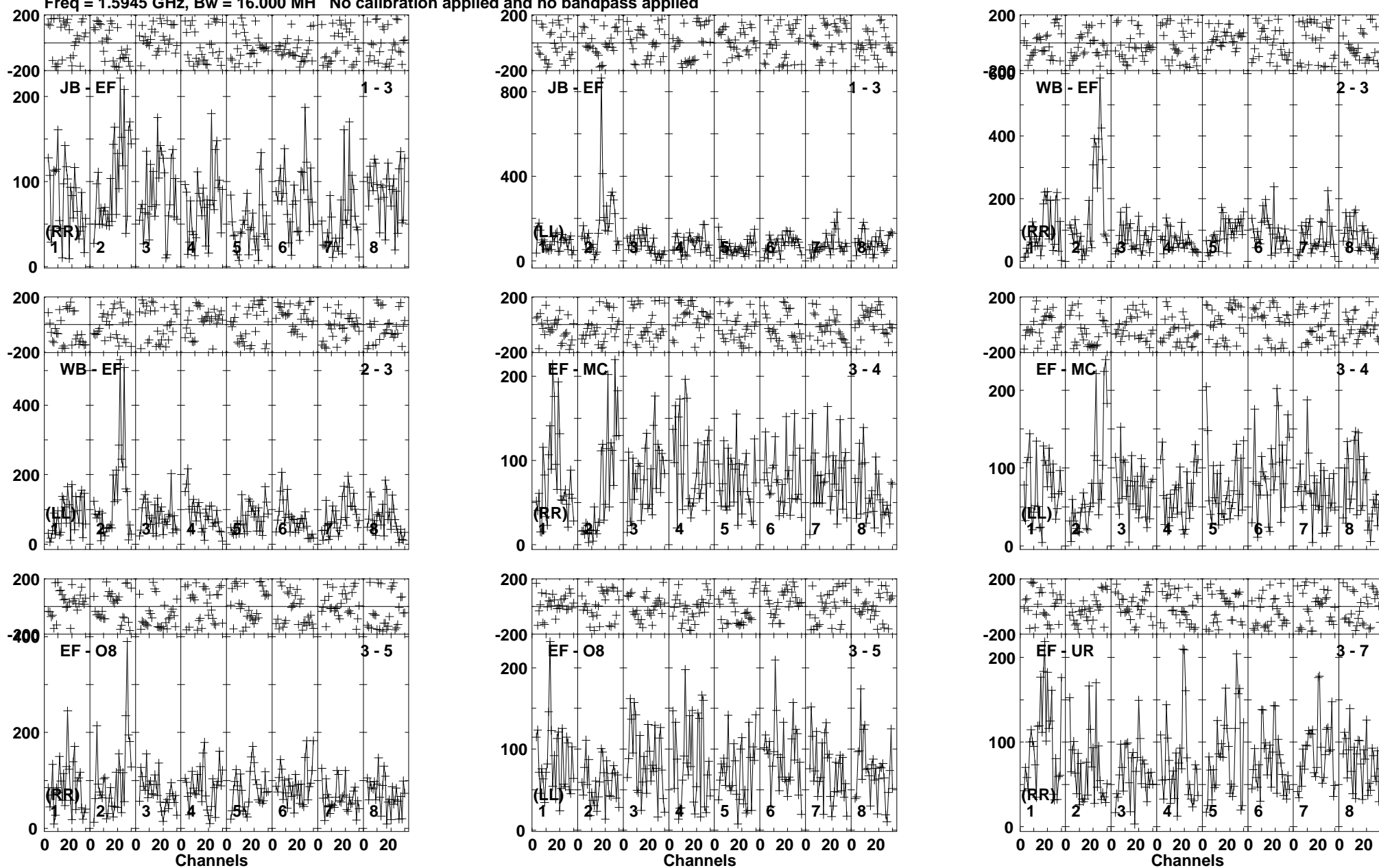
Lower frame: Micro Ampl Jy Top frame: Phas deg Vector averaged cross-power spectrum Baseline: JB (01) - EF (03) Timerange: 00:19:59:22 to 00:20:02:44
