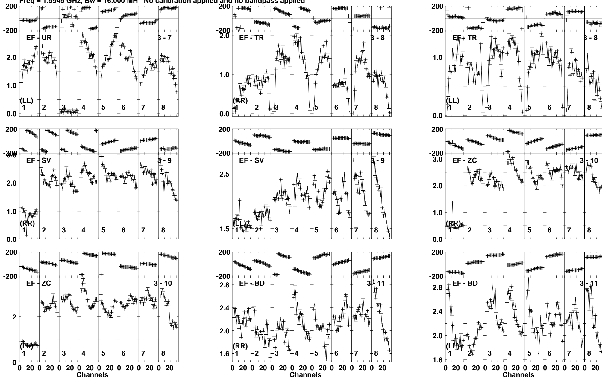
Lower frame: Milli Ampl Jy Top frame: Phas deg Vector averaged cross-power spectrum Baseline: EF (03) - UR (07) Timerange: 00/19:23:12 to 00/19:24:34
