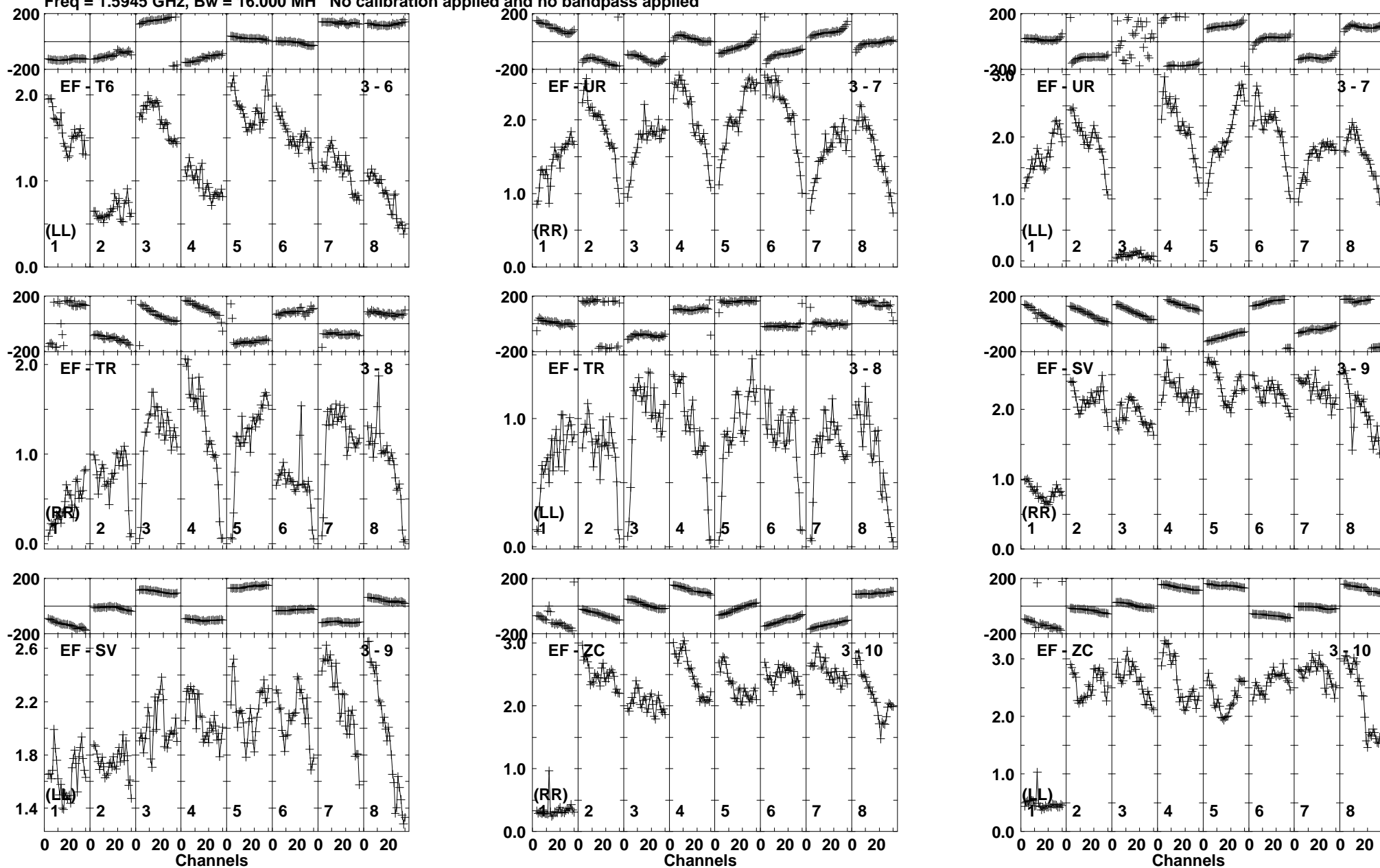
Lower frame: Milli Ampl Jy Top frame: Phas deg Vector averaged cross-power spectrum Baseline: EF (03) - T6 (06) Timerange: 00:18:12:02 to 00:18:13:24
