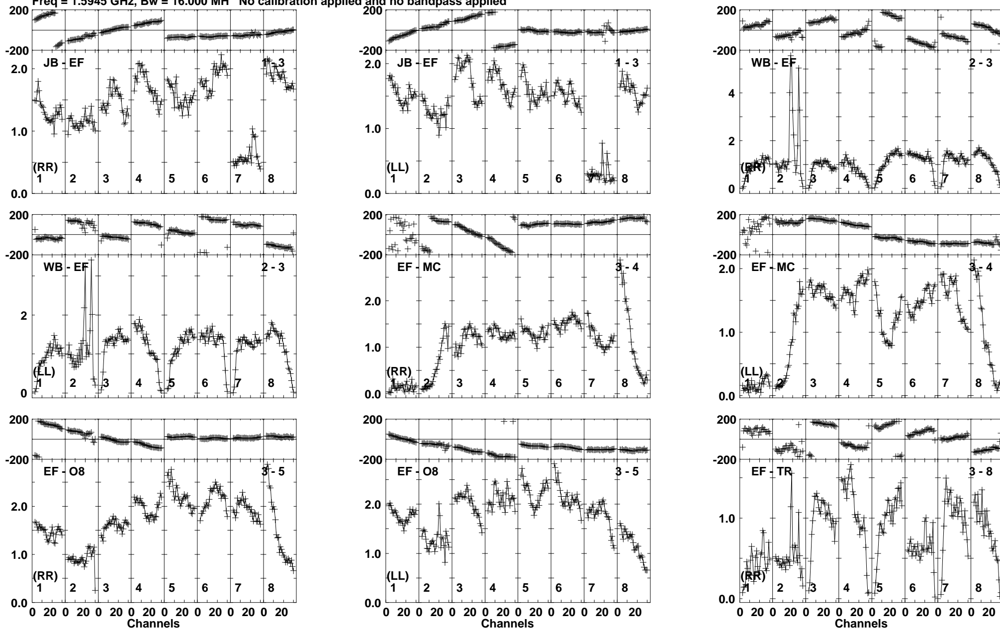
Lower frame: Milli Ampl Jy Top frame: Phas deg Vector averaged cross-power spectrum Baseline: JB (01) - EF (03) Timerange: 01/00:01:44 to 01/00:03:04
