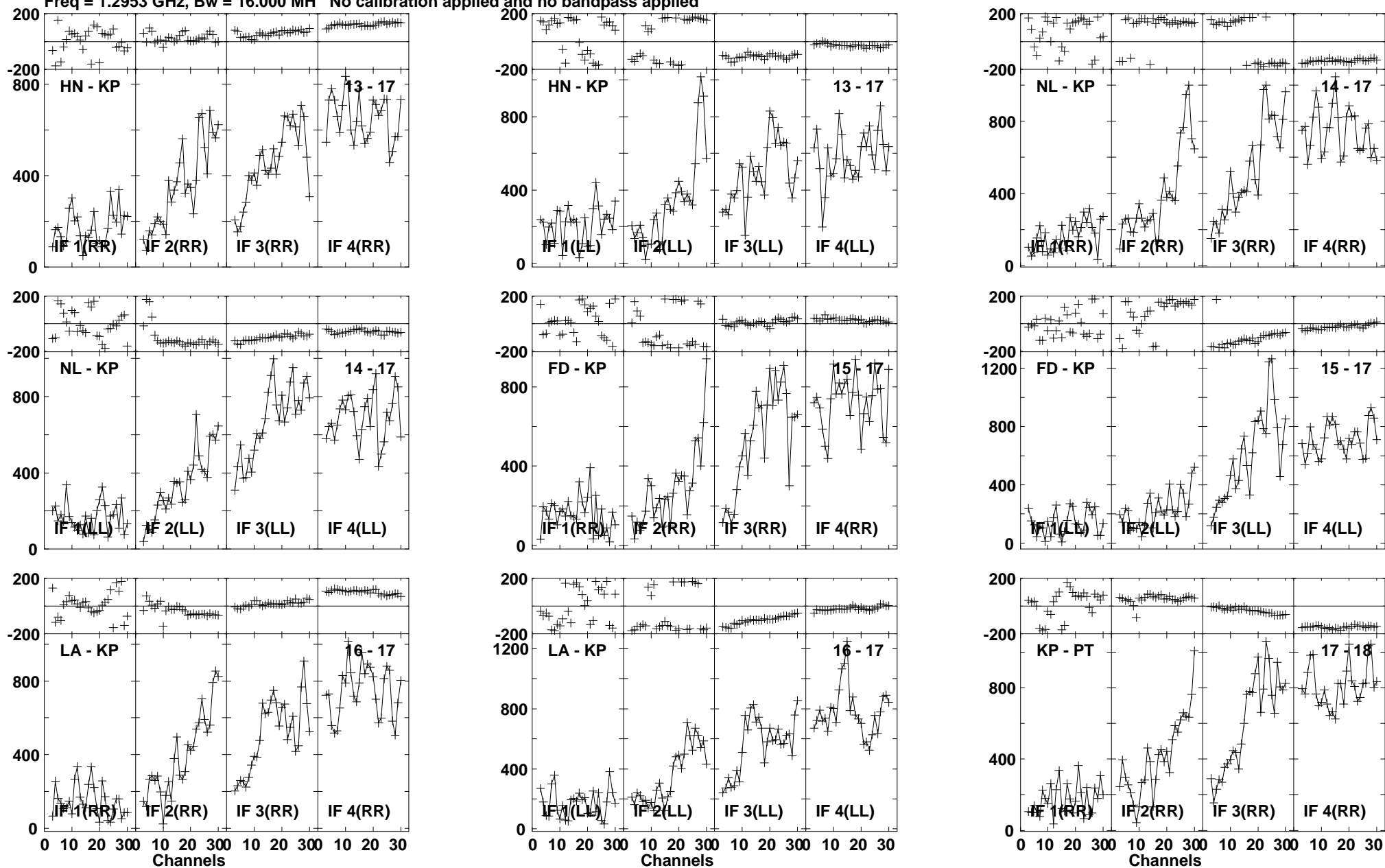
Lower frame: Micro Ampl Jy Top frame: Phas deg Vector averaged cross-power spectrum Baseline: HN (13) - KP (17) Timerange: 01/05:25:11 to 01/05:26:07
