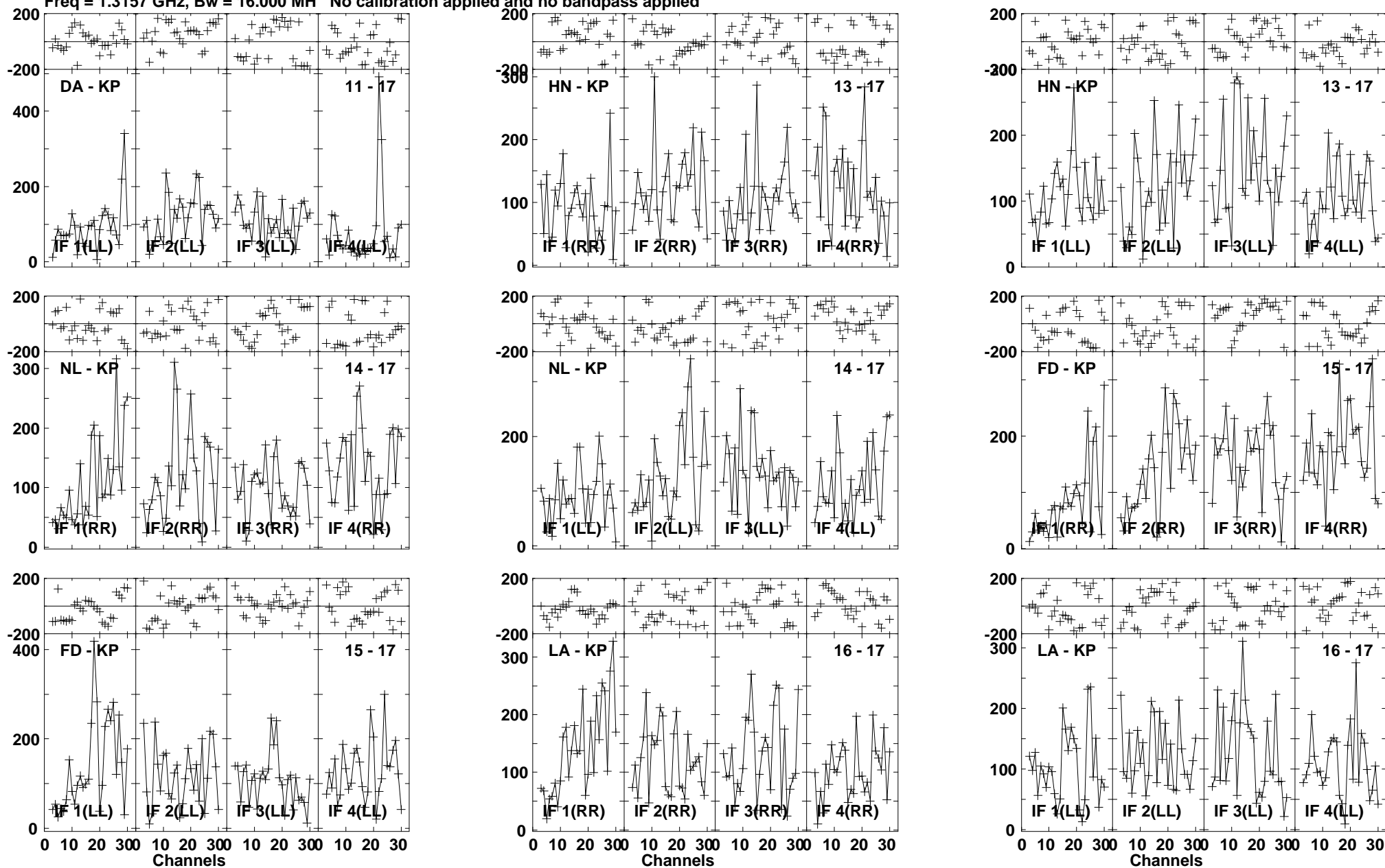
Lower frame: Micro Ampl Jy Top frame: Phas deg Vector averaged cross-power spectrum Baseline: DA (11) - KP (17) Timerange: 00/13:00:16 to 00/13:01:28
