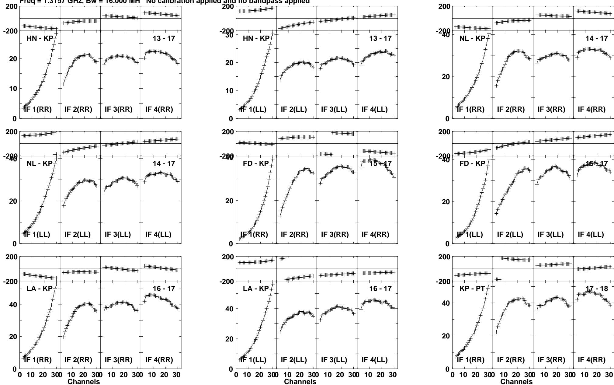
Lower frame: Milli Ampl Jy Top frame: Phas deg Vector averaged cross-power spectrum Baseline: HN (13) - KP (17) Timerange: 00/15:20:16 to 00/15:25:12
