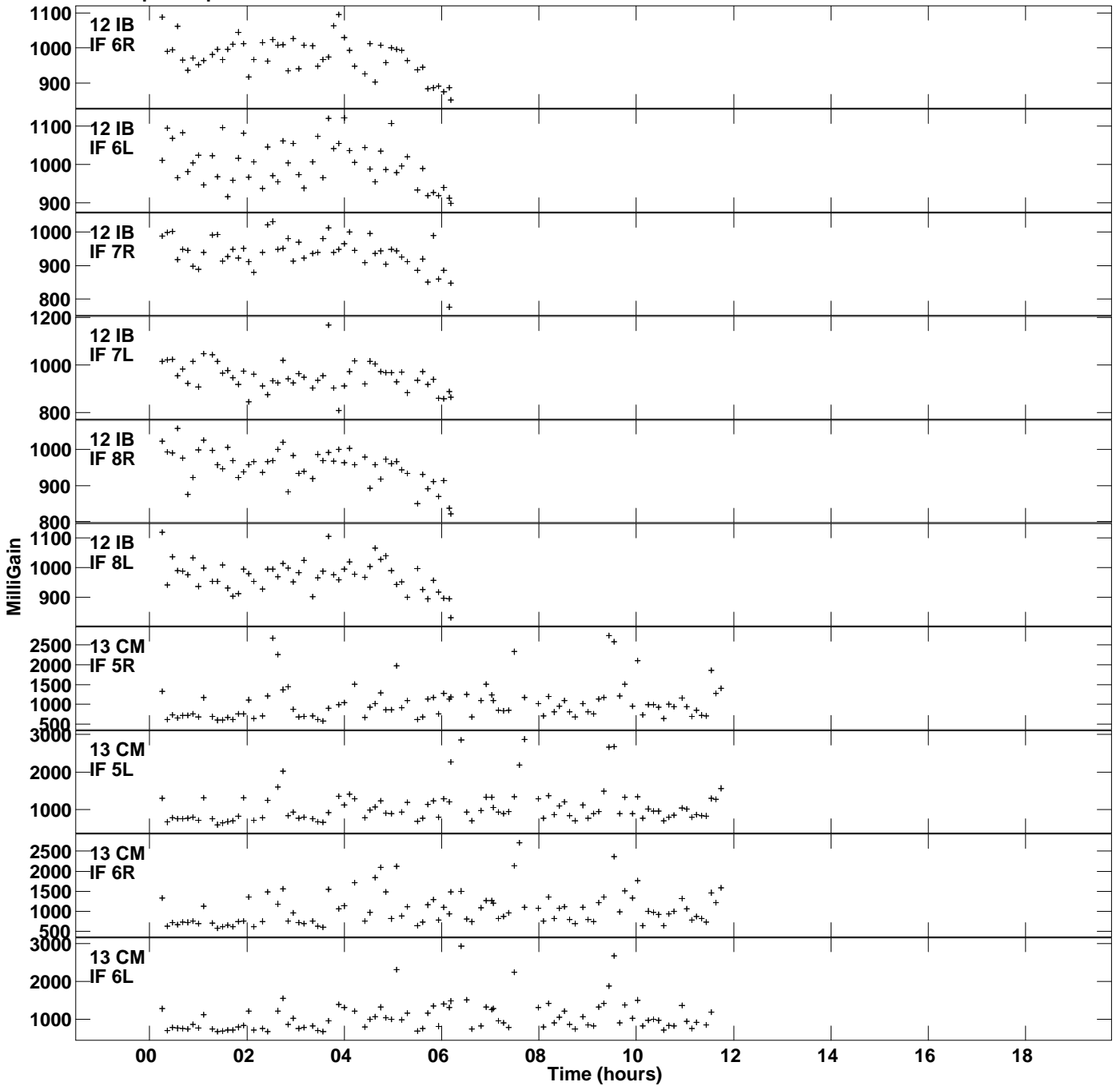
Plot file version 18 created 25-APR-2023 18:47:57 Gain amp vs UTC time for J1532+2344.MULTI.1 SN 2 Rpol & Lpol IF 1 - 8
