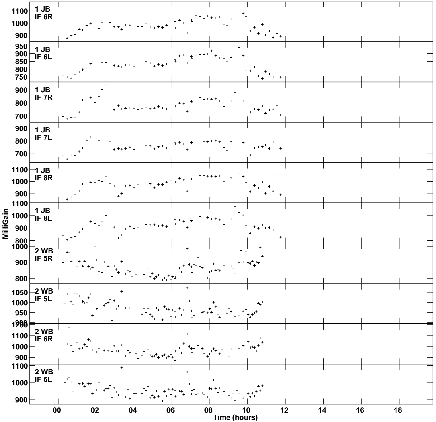
Plot file version 2 created 25-APR-2023 18:47:57 Gain amp vs UTC time for J1532+2344.MULTI.1 SN 2 Rpol & Lpol IF 1 - 8
